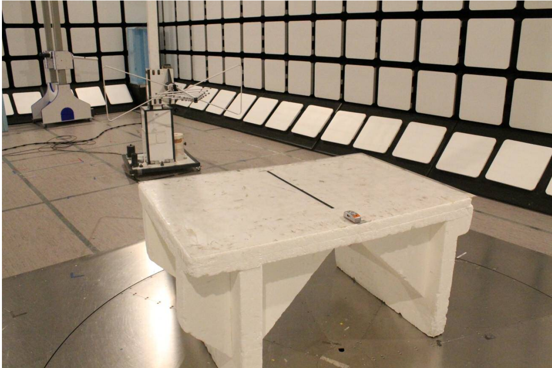
Photograph 1. Radiated Measurements 30 – 1000 MHz
