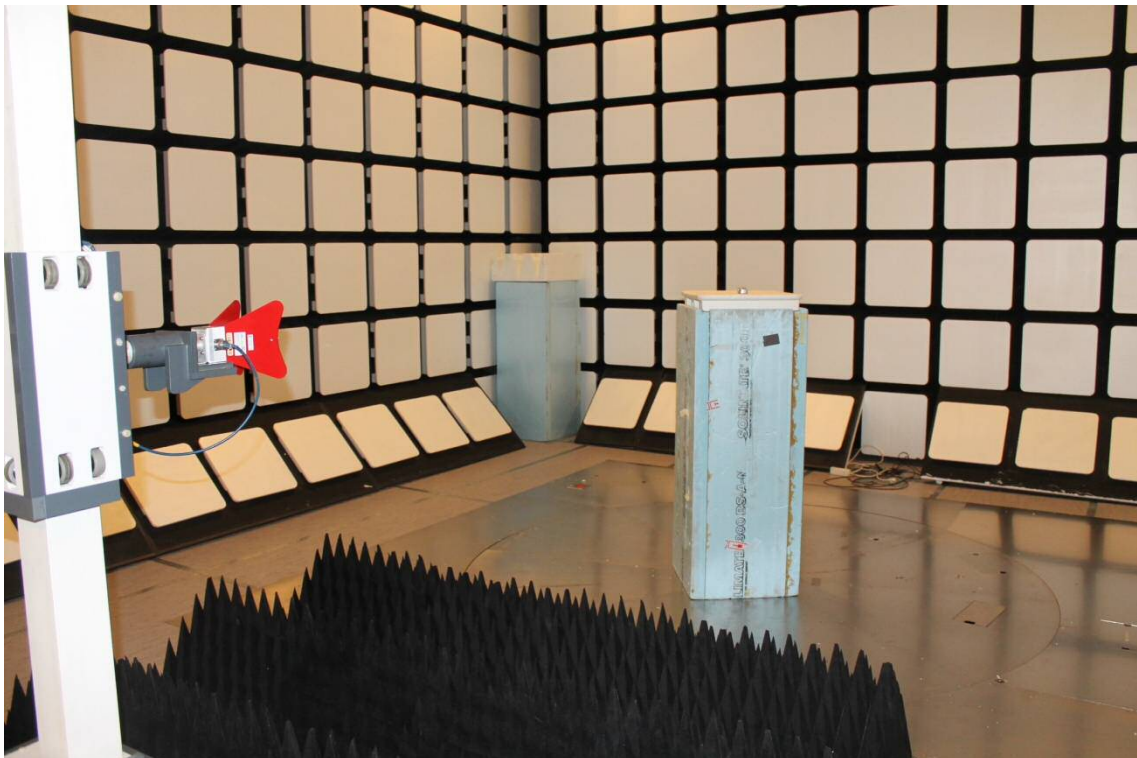
Photograph 2. Radiated Measurements 1 – 18 GHz
