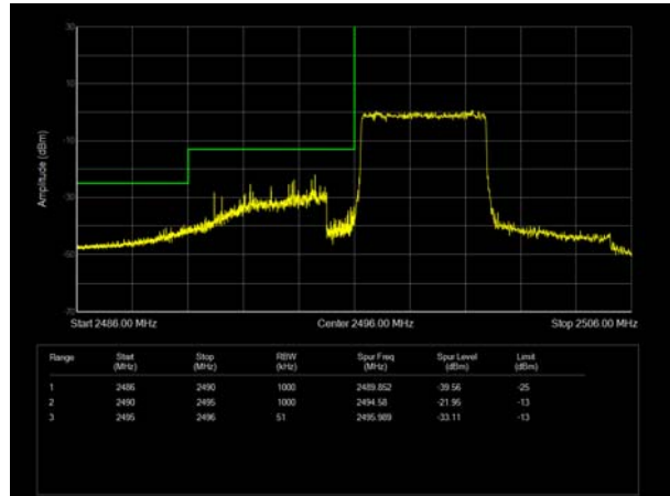
LTE Band 41 QPSK 10MHz CH-Low, 1 RB
