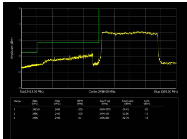
LTE Band 41 QPSK 10MHz CH-Low, 100%RB
