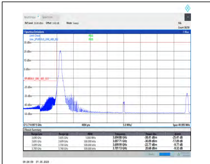
1-N78-3700-3800-PC2-30-40-L-1-DFT-PI2BPSK-Edge_1RB_Left-1@0-Ant1-1--PASS-see graph
