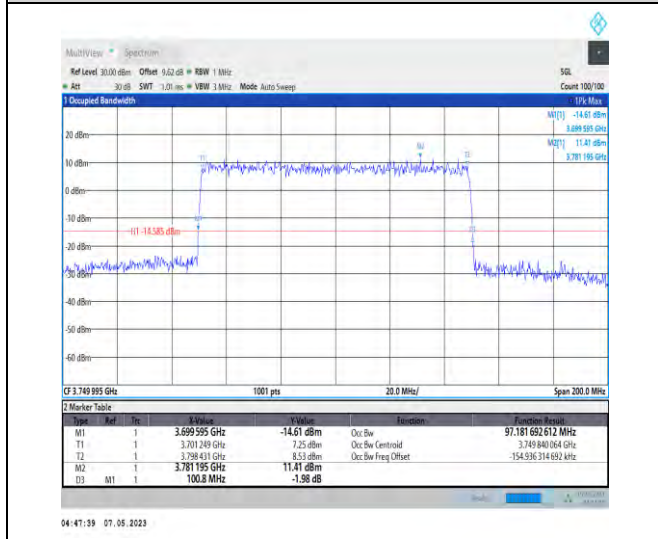
1-N78-3700-3800-PC2-30-100-M-6-CP-QPSK-Outer_Full-273@0-Ant1-97.182-100.800-≤100-PASS
