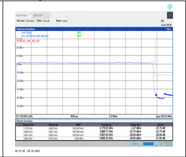
1-N78-3700-3800-PC2-30-80-H-3-DFT-PI2BPSK-Outer_Full-216@0-Ant1-1--PASS-see graph
