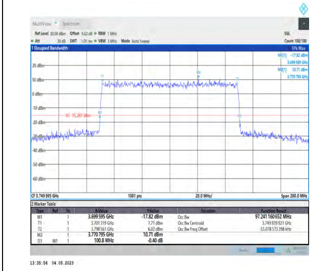
1-N78-3700-3800-PC2-30-100-H-9-CP-256QAM-Outer_Full-273@0-Ant1-97.241-100.800-≤100-PASS
