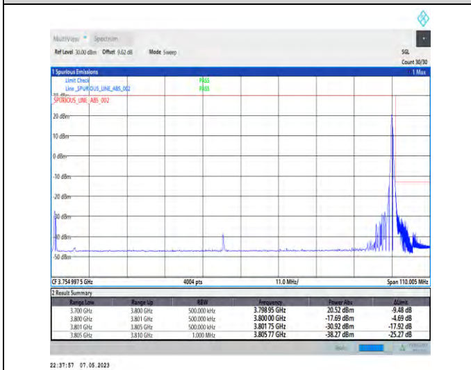
1-N78-3700-3800-PC2-30-100-H-5-CP-QPSK-Edge_1_RB_Right-1@272-Ant1-1--PASS-see graph
