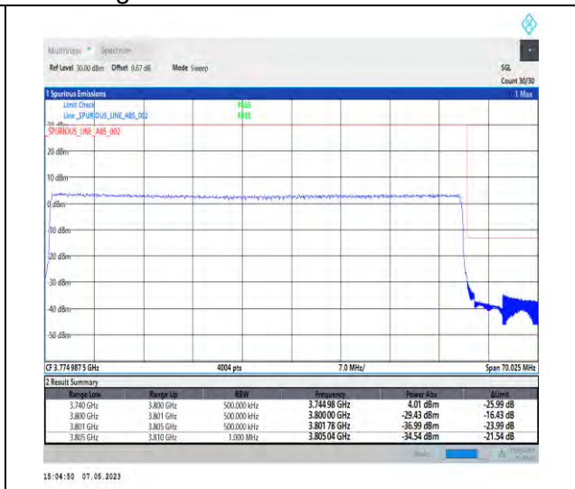
1-N78-3700-3800-PC2-30-60-H-3-DFT-PI2BPSK-Outer_Full-162@0-Ant1-1--PASS-see graph
