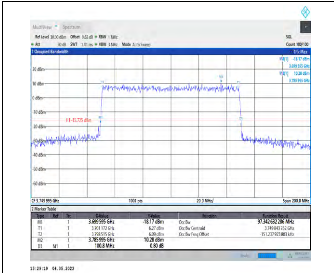
1-N78-3700-3800-PC2-30-100-L-9-CP-256QAM-Out er_Full-273@0-Ant1-97.343-100.800-≤100-PASS
