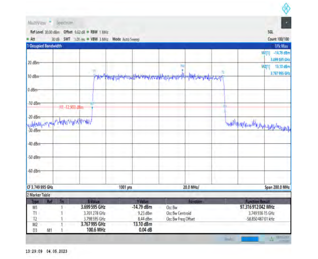
1-N78-3700-3800-PC2-30-100-L-8-CP-64QAM-Outer_Full-273@0-Ant1-97.317-100.600-≤100-PASS
