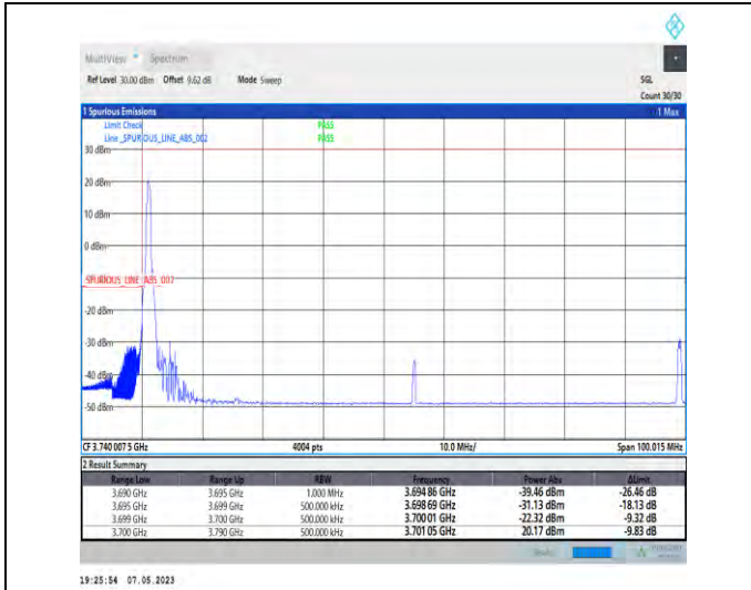
1-N78-3700-3800-PC2-30-90-L-1-DFT-PI2BPSK-Edge_1RB_Left-1@0-Ant1-1--PASS-see graph
