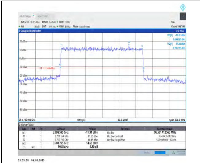
1-N78-3700-3800-PC2-30-100-H-3-DFT-16QAM-Out er_Full-270@0-Ant1-96.561-99.800-≤100-PASS
