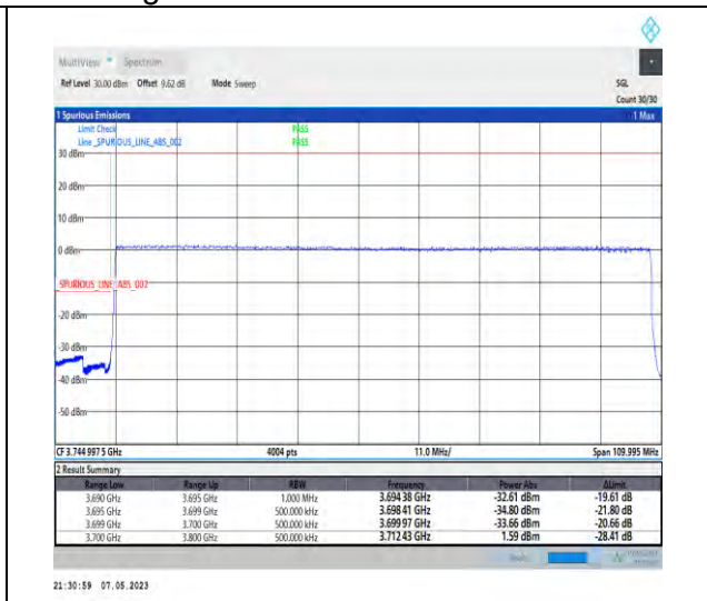
1-N78-3700-3800-PC2-30-100-L-3-DFT-PI2BPSK-Outer_Full-270@0-Ant1-1--PASS-see graph
