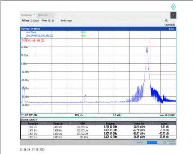
1-N78-3700-3800-PC2-30-50-H-5-CP-QPSK-Edge_1RB_Right-1@132-Ant1-1--PASS-see graph
