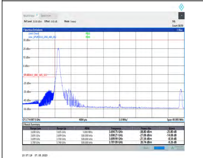
1-N78-3700-3800-PC2-30-40-L-4-CP-QPSK-Edge_1RB_Left-1@0-Ant1-1--PASS-see graph
