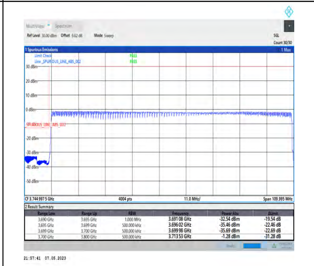
1-N78-3700-3800-PC2-30-100-L-6-CP-QPSK-Outer_Full-273@0-Ant1-1--PASS-see graph
