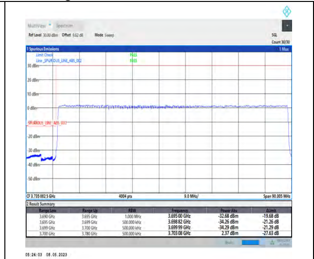
1-N78-3700-3800-PC2-30-80-L-3-DFT-PI2BPSK-Outer_Full-216@0-Ant1-1--PASS-see graph
