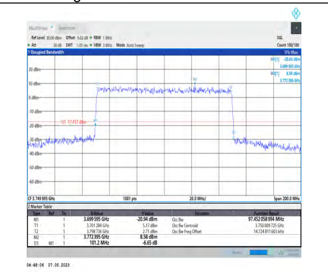
1-N78-3700-3800-PC2-30-100-M-9-CP-256QAM-Out er_Full-273@0-Ant1-97.452-101.200-≤100-PASS
