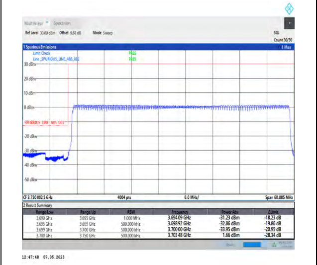
1-N78-3700-3800-PC2-30-50-L-6-CP-QPSK-Outer_Full-133@0-Ant1-1--PASS-see graph
