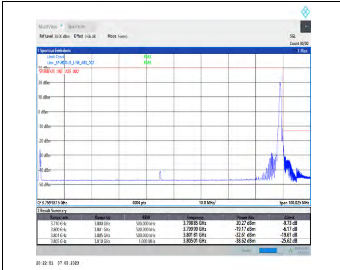
1-N78-3700-3800-PC2-30-90-H-2-DFT-PI2BPSK-Edge_1RB_Right-1@244-Ant1-1--PASS-see graph
