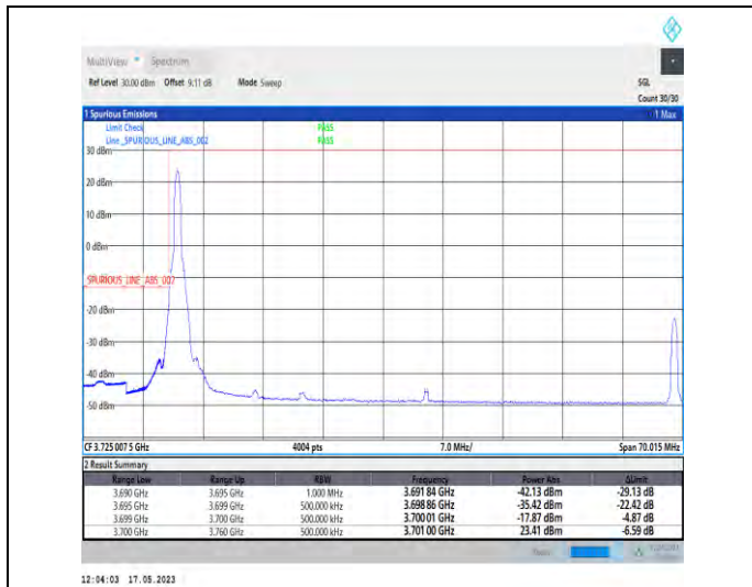
1-N78-3700-3800-PC2-30-60-L-1-DFT-PI2BPSK-Edge_1RB_Left-1@0-Ant1-1--PASS-see graph
