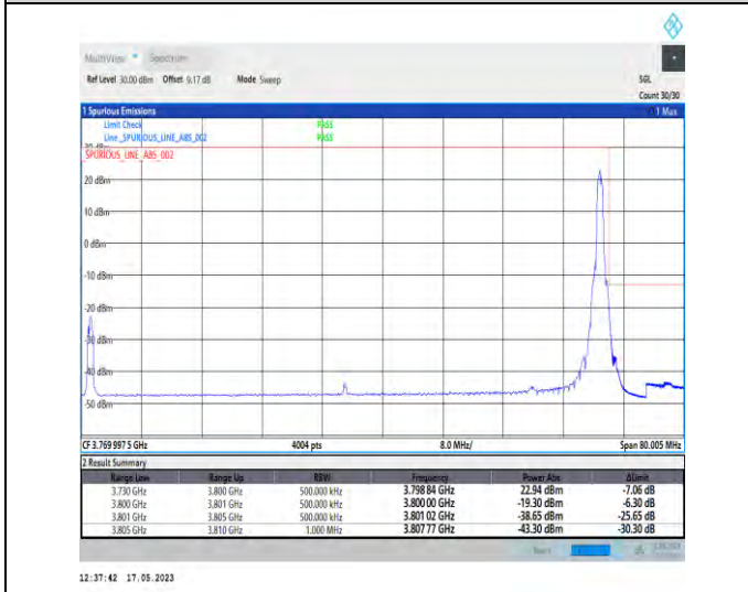
1-N78-3700-3800-PC2-30-70-H-5-CP-QPSK-Edge_1RB_Right-1@188-Ant1-1--PASS-see graph
