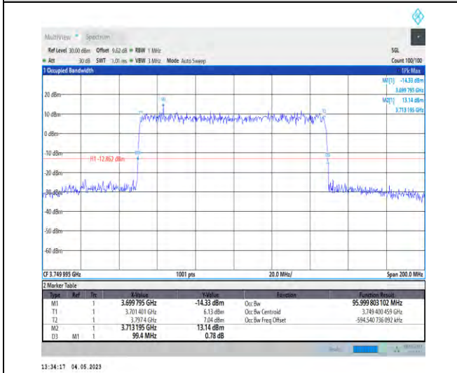
1-N78-3700-3800-PC2-30-100-H-5-DFT-256QAM-Out er_Full-270@0-Ant1-96-99.400-≤100-PASS
