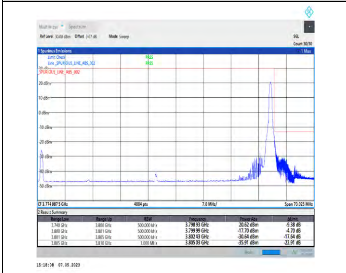
1-N78-3700-3800-PC2-30-60-H-5-CP-QPSK-Edge_1RB_Right-1@161-Ant1-1--PASS-see graph
