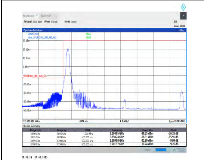
1-N78-3700-3800-PC2-30-30-L-4-CP-QPSK-Edge_1RB_Left-1@0-Ant1-1--PASS-see graph
