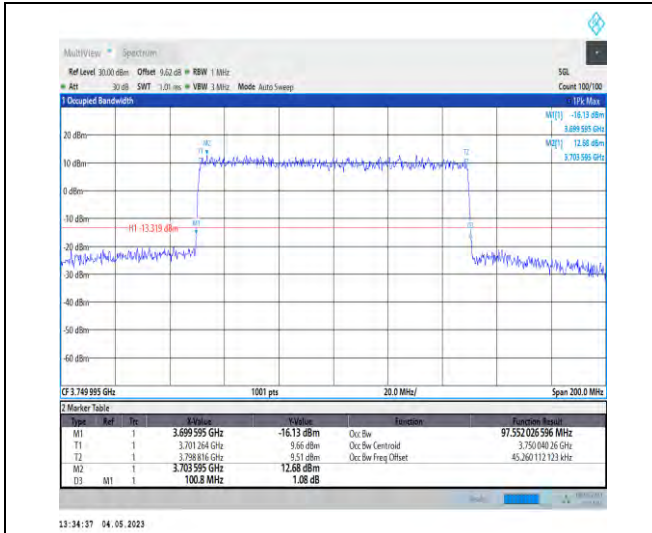
1-N78-3700-3800-PC2-30-100-H-7-CP-16QAM-Out er_Full-273@0-Ant1-97.552-100.800-≤100-PASS
