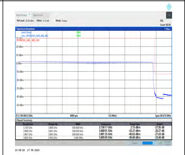
1-N78-3700-3800-PC2-30-80-H-6-CP-QPSK-Outer_Full-217@0-Ant1-1--PASS-see graph
