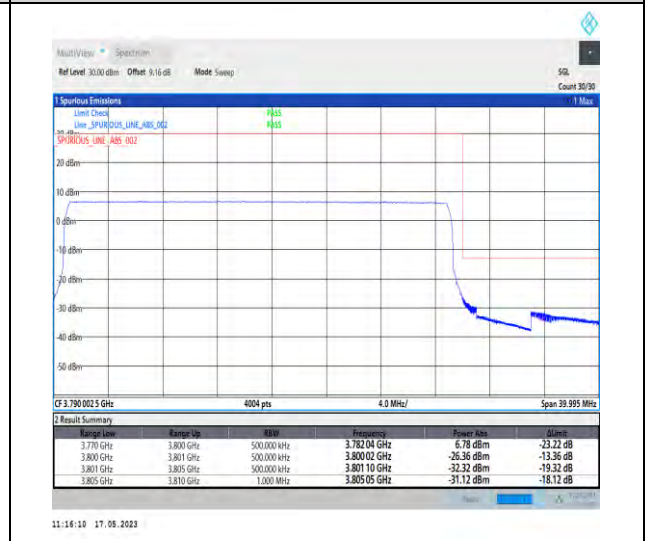
1-N78-3700-3800-PC2-30-30-H-6-CP-QPSK-Outer_Full-78@0-Ant1-1--PASS-see graph
