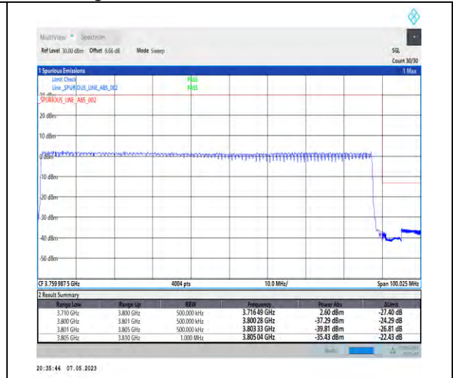
1-N78-3700-3800-PC2-30-90-H-3-DFT-PI2BPSK-Outer_Full-240@0-Ant1-1--PASS-see graph
