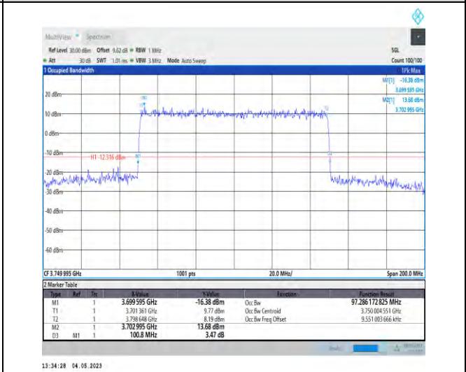
1-N78-3700-3800-PC2-30-100-H-6-CP-QPSK-Outer _Full-273@0-Ant1-97.286-100.800-≤100-PASS
