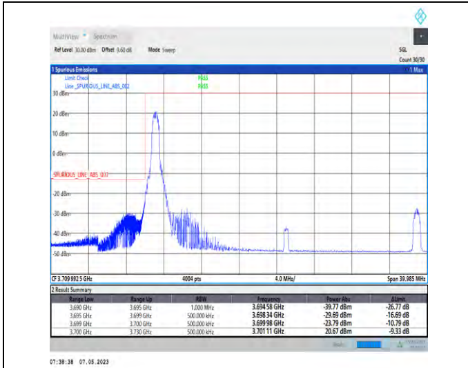
1-N78-3700-3800-PC2-30-30-L-1-DFT-PI2BPSK-Edge_1RB_Left-1@0-Ant1-1--PASS-see graph
