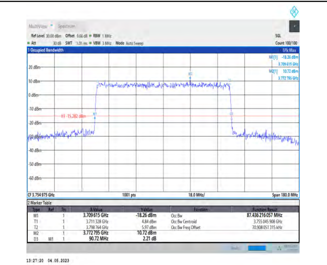
1-N78-3700-3800-PC2-30-90-H-9-CP-256QAM-Outer_Full-245@0-Ant1-87.436-90.720-≤90-PASS
