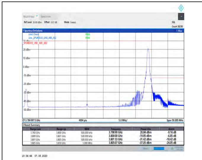
1-N78-3700-3800-PC2-30-40-H-2-DFT-PI2BPSK-Edge_1RB_Right-1@105-Ant1-1--PASS-see graph
