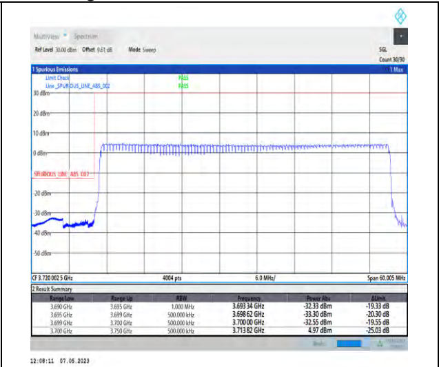
1-N78-3700-3800-PC2-30-50-L-3-DFT-PI2BPSK-Outer_Full-128@0-Ant1-1--PASS-see graph
