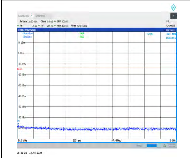
1-N78-3700-3800-PC2-30-100-H-1-DFT-PI2BPSK-In ner_1RB_Left-1@1-30-1000-Ant1-34.37--66.81--13- PASS
