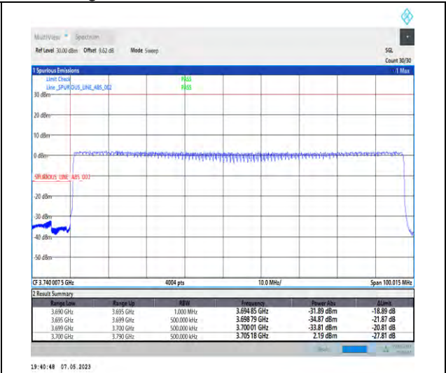
1-N78-3700-3800-PC2-30-90-L-3-DFT-PI2BPSK-Outer_Full-240@0-Ant1-1--PASS-see graph
