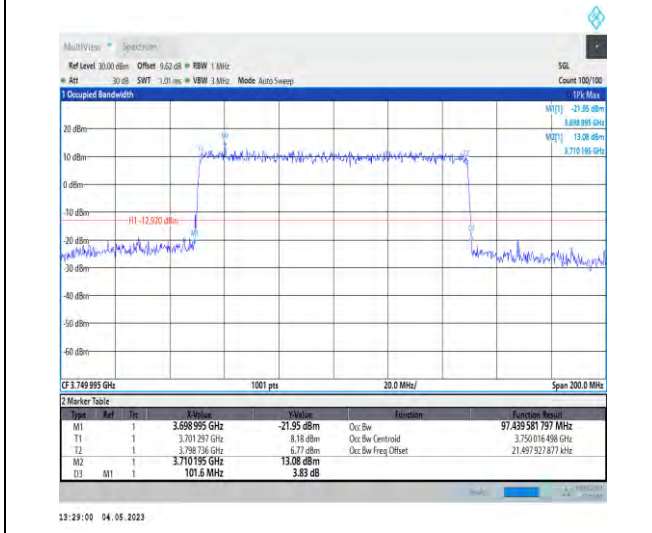
1-N78-3700-3800-PC2-30-100-L-7-CP-16QAM-Outer_Full-273@0-Ant1-97.44-101.600-≤100-PASS
