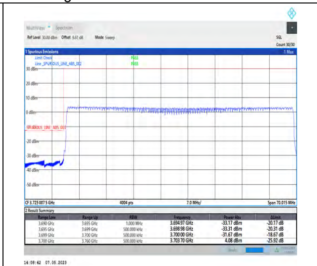
1-N78-3700-3800-PC2-30-60-L-3-DFT-PI2BPSK-Outer_Full-162@0-Ant1-1--PASS-see graph
