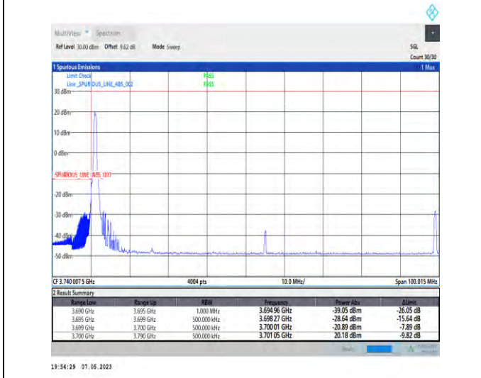
1-N78-3700-3800-PC2-30-90-L-4-CP-QPSK-Edge_1RB_Left-1@0-Ant1-1--PASS-see graph
