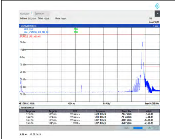
1-N78-3700-3800-PC2-30-80-H-5-CP-QPSK-Edge_1RB_Right-1@216-Ant1-1--PASS-see graph
