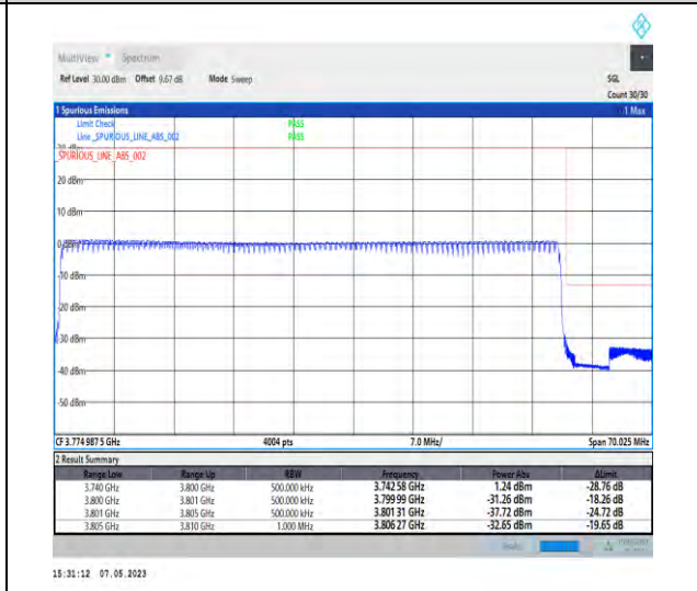
1-N78-3700-3800-PC2-30-60-H-6-CP-QPSK-Outer_Full-162@0-Ant1-1--PASS-see graph
