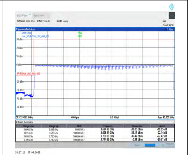
1-N78-3700-3800-PC2-30-80-L-6-CP-QPSK-Outer_Full-217@0-Ant1-1--PASS-see graph
