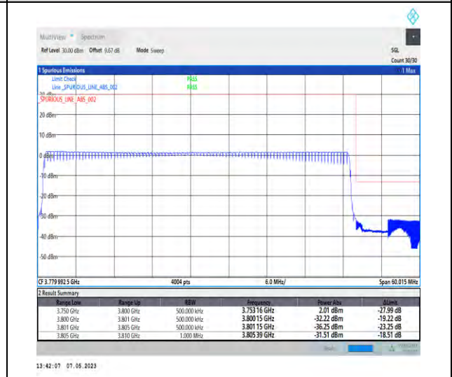
1-N78-3700-3800-PC2-30-50-H-6-CP-QPSK-Outer_Full-133@0-Ant1-1--PASS-see graph
