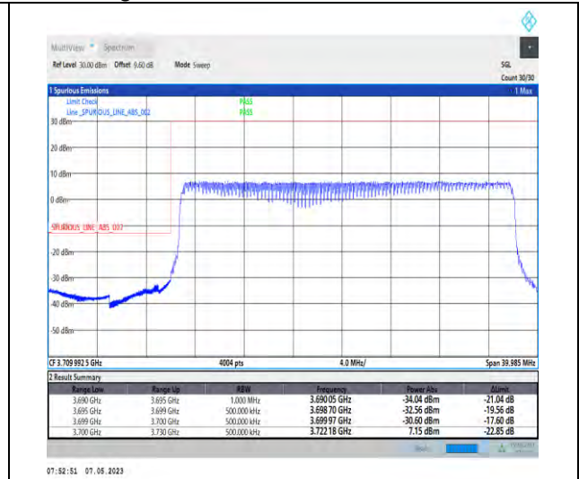
1-N78-3700-3800-PC2-30-30-L-3-DFT-PI2BPSK-Outer_Full-75@0-Ant1-1--PASS-see graph
