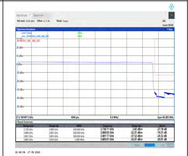
1-N78-3700-3800-PC2-30-70-H-6-CP-QPSK-Outer_Full-189@0-Ant1-1--PASS-see graph
