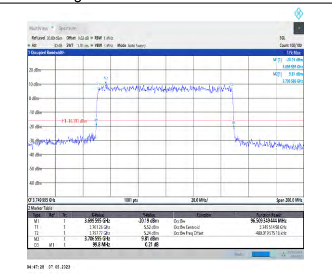
1-N78-3700-3800-PC2-30-100-M-5-DFT-256QAM-Outer_Full-270@0-Ant1-96.509-99.800-≤100-PASS
