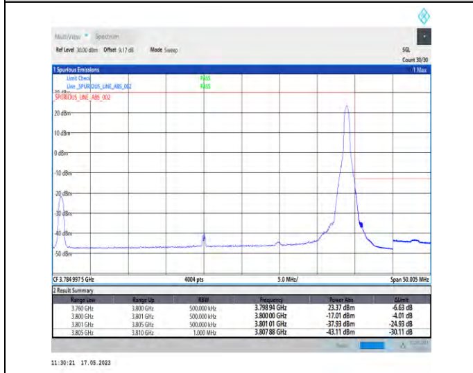
1-N78-3700-3800-PC2-30-40-H-5-CP-QPSK-Edge_1RB_Right-1@105-Ant1-1--PASS-see graph
