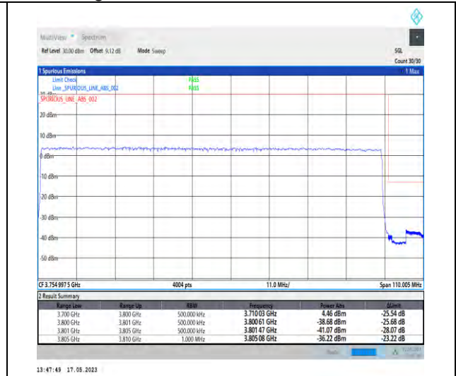
1-N78-3700-3800-PC2-30-100-H-3-DFT-PI2BPSK-Outer_Full-270@0-Ant1-1--PASS-see graph
