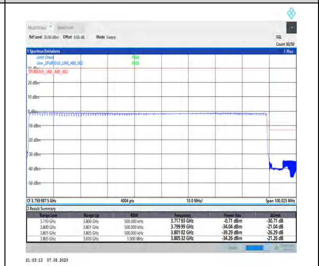
1-N78-3700-3800-PC2-30-90-H-6-CP-QPSK-Outer_Full-245@0-Ant1-1--PASS-see graph
