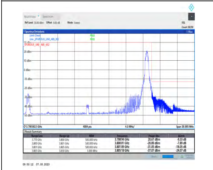
1-N78-3700-3800-PC2-30-30-H-5-CP-QPSK-Edge_1RB_Right-1@77-Ant1-1--PASS-see graph
