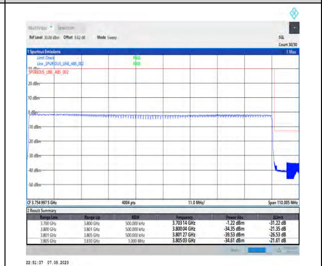
1-N78-3700-3800-PC2-30-100-H-6-CP-QPSK-Outer_Full-273@0-Ant1-1--PASS-see graph
