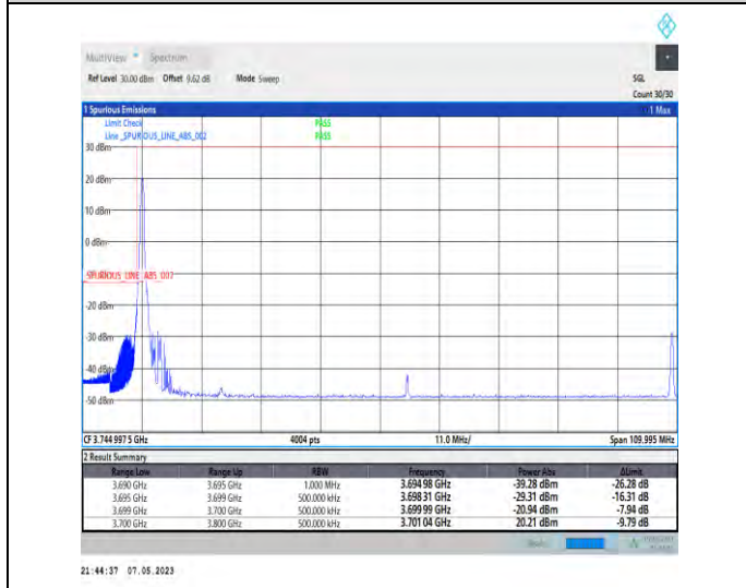
1-N78-3700-3800-PC2-30-100-L-4-CP-QPSK-Edge_1_RB_Left-1@0-Ant1-1--PASS-see graph
