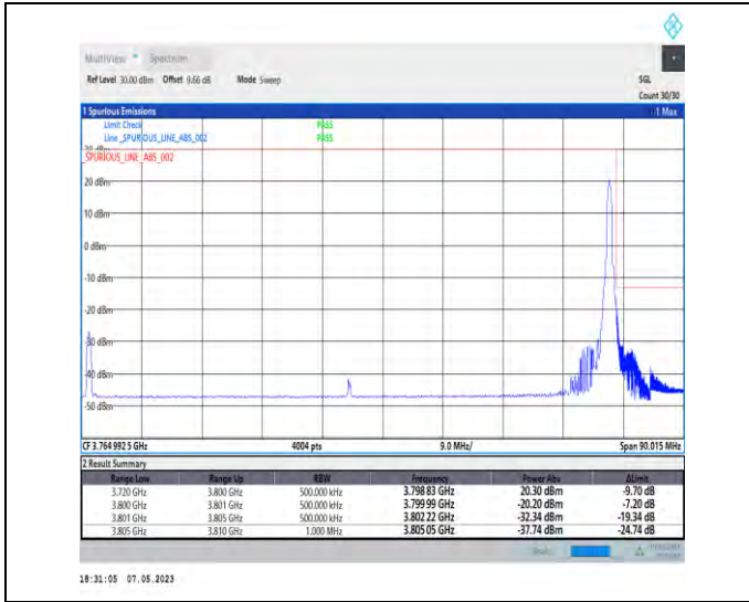
1-N78-3700-3800-PC2-30-80-H-2-DFT-PI2BPSK-Edge_1RB_Right-1@216-Ant1-1--PASS-see graph
