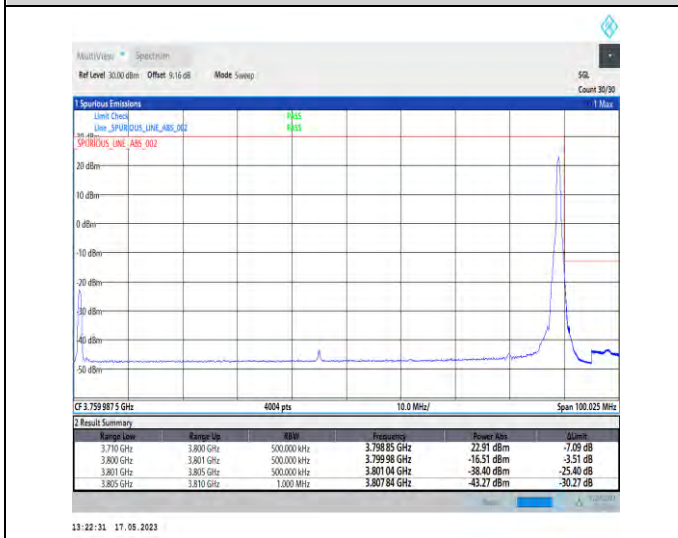
1-N78-3700-3800-PC2-30-90-H-5-CP-QPSK-Edge_1RB_Right-1@244-Ant1-1--PASS-see graph
