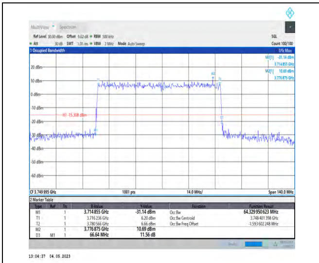
1-N78-3700-3800-PC2-30-70-M-5-DFT-256QAM-Outer_Full-180@0-Ant1-64.33-66.640-≤70-PASS
