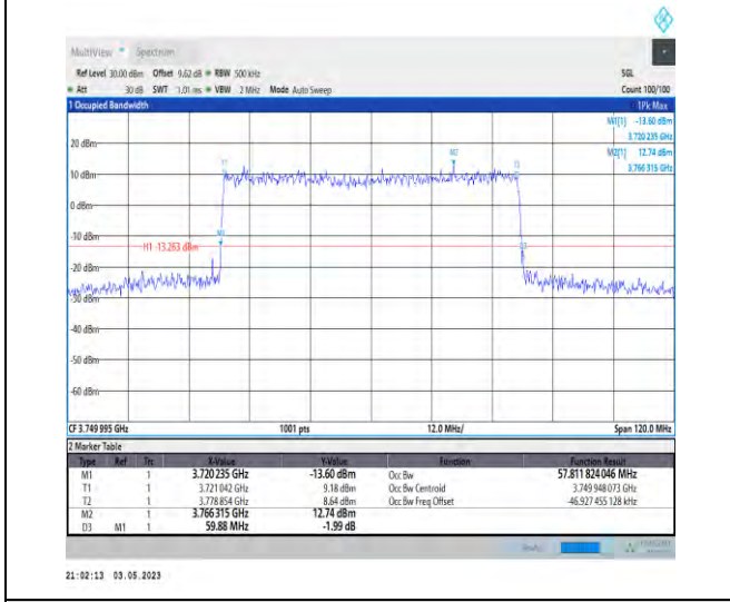
1-N78-3700-3800-PC2-30-60-M-6-CP-QPSK-Outer_Full-162@0-Ant1-57.812-59.880-≤60-PASS
