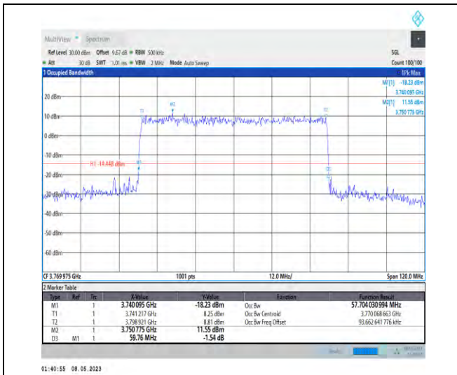
1-N78-3700-3800-PC2-30-60-H-3-DFT-16QAM-Outer_Full-162@0-Ant1-57.704-59.760-≤60-PASS
