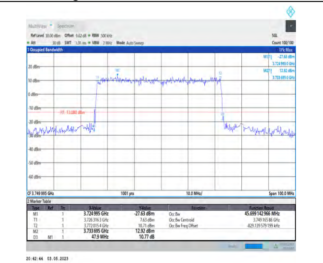
1-N78-3700-3800-PC2-30-50-M-4-DFT-64QAM-Outer_Full-128@0-Ant1-45.699-47.900-≤50-PASS
