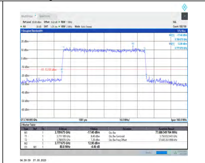
1-N78-3700-3800-PC2-30-80-M-7-CP-16QAM-Outer_Full-217@0-Ant1-77.687-80.800-≤80-PASS
