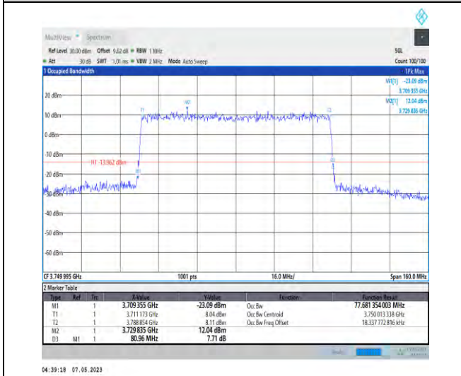
1-N78-3700-3800-PC2-30-80-M-8-CP-64QAM-Outer_Full-217@0-Ant1-77.681-80.960-≤80-PASS
