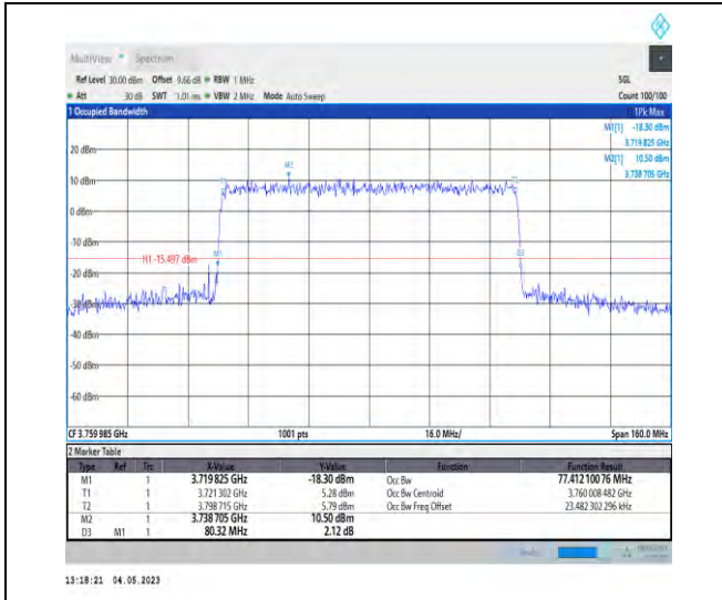
1-N78-3700-3800-PC2-30-80-H-9-CP-256QAM-Out er_Full-217@0-Ant1-77.412-80.320-≤80-PASS
