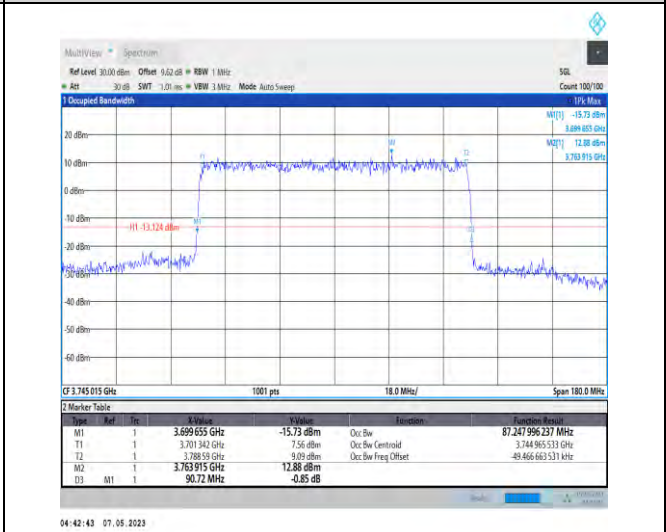
1-N78-3700-3800-PC2-30-90-L-7-CP-16QAM-Outer_Full-245@0-Ant1-87.248-90.720-≤90-PASS
