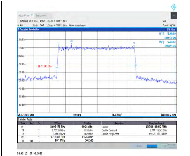
1-N78-3700-3800-PC2-30-90-L-4-DFT-64QAM-Out_r_Full-240@0-Ant1-85.709-89.100-≤90-PASS
