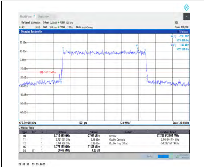
1-N78-3700-3800-PC2-30-60-M-8-CP-64QAM-Outer_Full-162@0-Ant1-57.787-60.480-≤60-PASS
