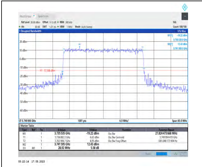
1-N78-3700-3800-PC2-30-30-M-9-CP-256QAM-Out er_Full-78@0-Ant1-27.824-28.920-≤30-PASS
