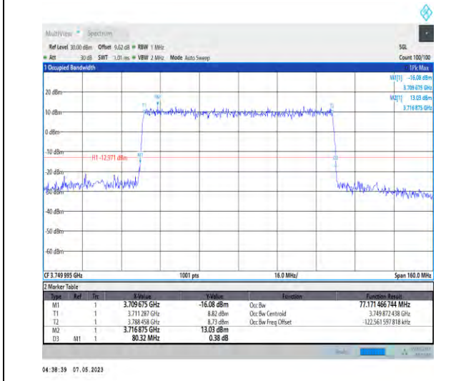
1-N78-3700-3800-PC2-30-80-M-4-DFT-64QAM-Outer_Full-216@0-Ant1-77.171-80.320-≤80-PASS
