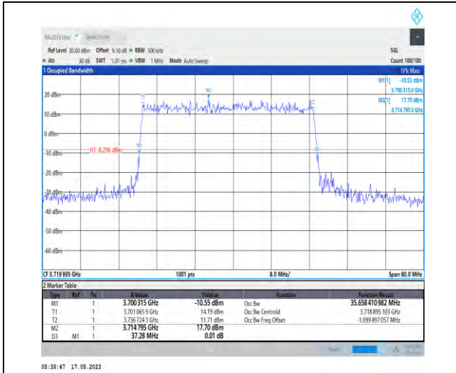
1-N78-3700-3800-PC2-30-40-L-3-DFT-16QAM-Outer_Full-100@0-Ant1-35.658-37.280-≤40-PASS
