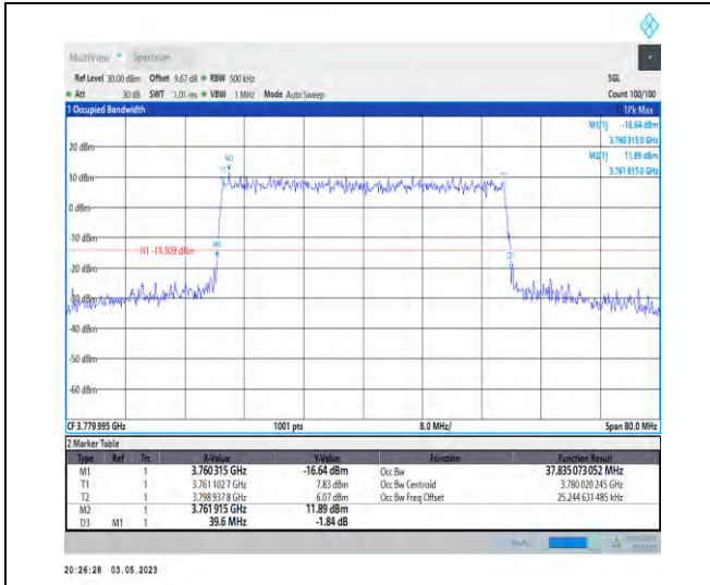
1-N78-3700-3800-PC2-30-40-H-9-CP-256QAM-Out er_Full-106@0-Ant1-37.835-39.600-≤40-PASS
