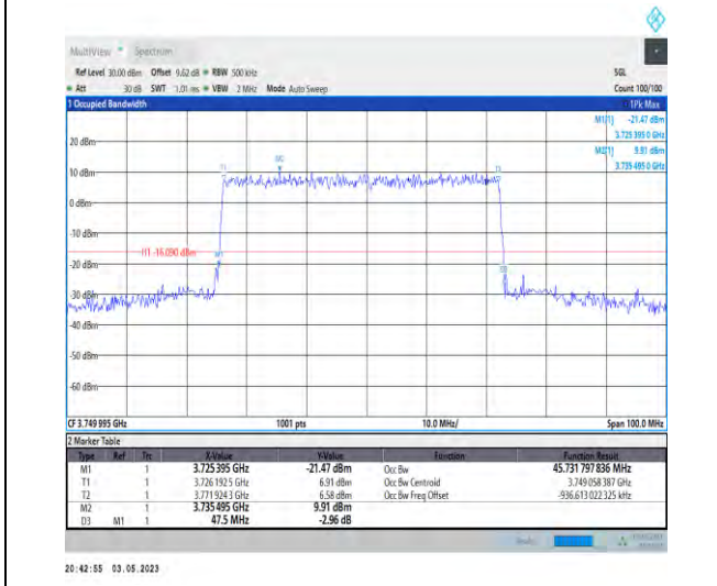
1-N78-3700-3800-PC2-30-50-M-5-DFT-256QAM-Outer_Full-128@0-Ant1-45.732-47.500-≤50-PASS
