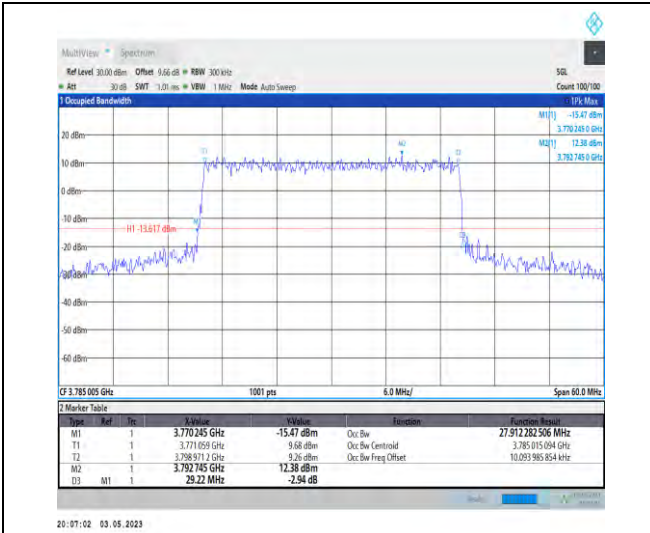
1-N78-3700-3800-PC2-30-30-H-8-CP-64QAM-Outer_Full-78@0-Ant1-27.912-29.220-≤30-PASS
