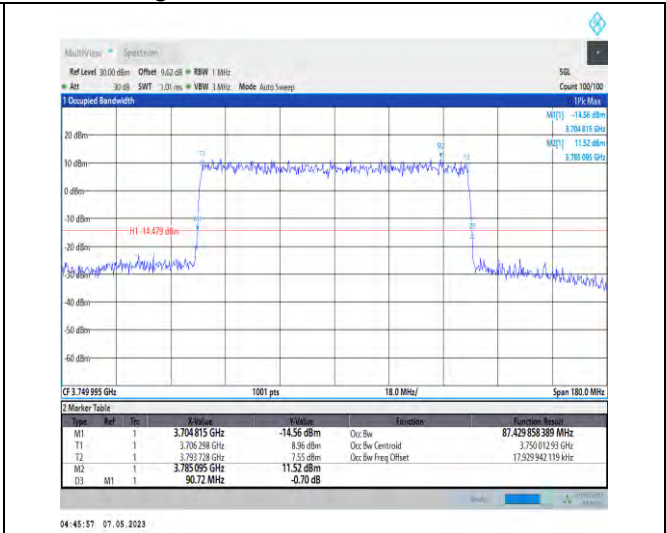
1-N78-3700-3800-PC2-30-90-M-8-CP-64QAM-Outer_Full-245@0-Ant1-87.43-90.720-≤90-PASS
