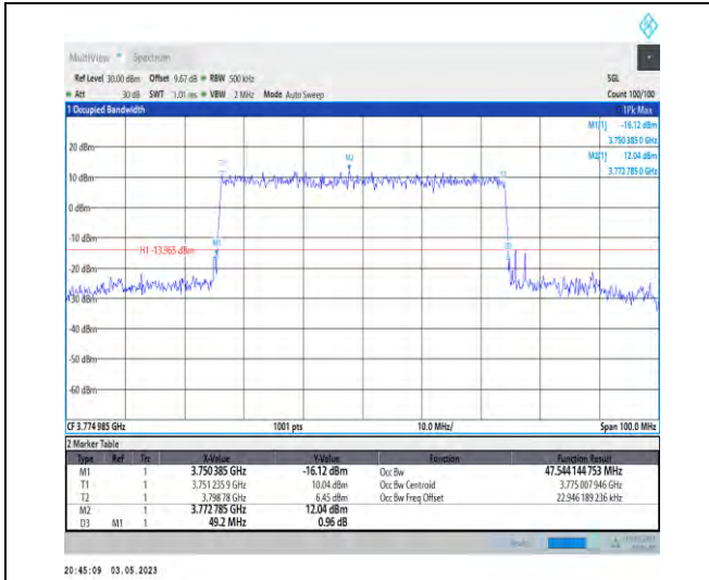
1-N78-3700-3800-PC2-30-50-H-6-CP-QPSK-Outer_Full-133@0-Ant1-47.544-49.200-≤50-PASS
