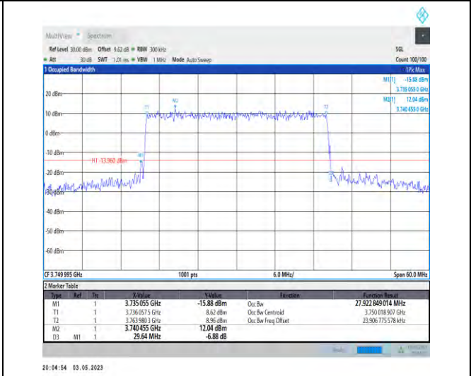
1-N78-3700-3800-PC2-30-30-M-8-CP-64QAM-Outer_Full-78@0-Ant1-27.923-29.640-≤30-PASS
