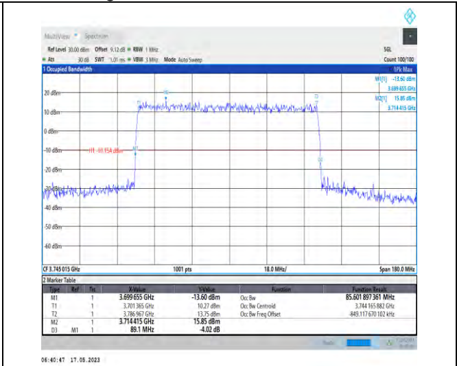
1-N78-3700-3800-PC2-30-90-L-5-DFT-256QAM-Out_er_Full-240@0-Ant1-85.602-89.100-≤90-PASS
