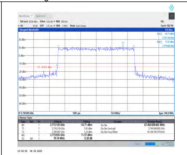
1-N78-3700-3800-PC2-30-70-M-6-CP-QPSK-Outer_Full-189@0-Ant1-67.463-70.140-≤70-PASS
