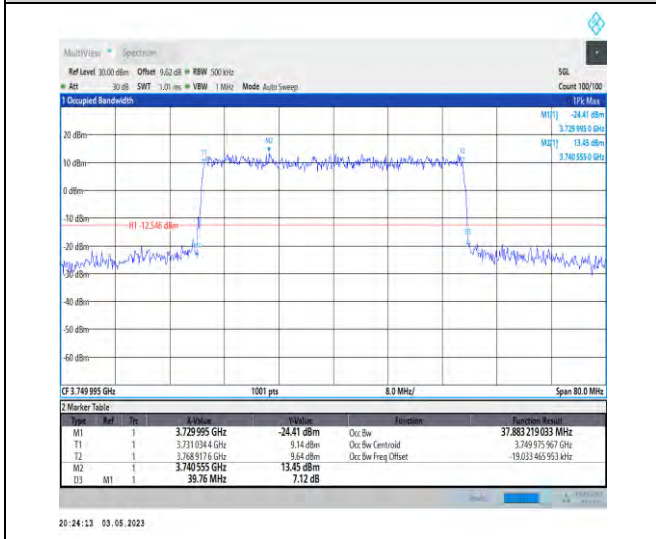
1-N78-3700-3800-PC2-30-40-M-8-CP-64QAM-Outer_Full-106@0-Ant1-37.883-39.760-≤40-PASS
