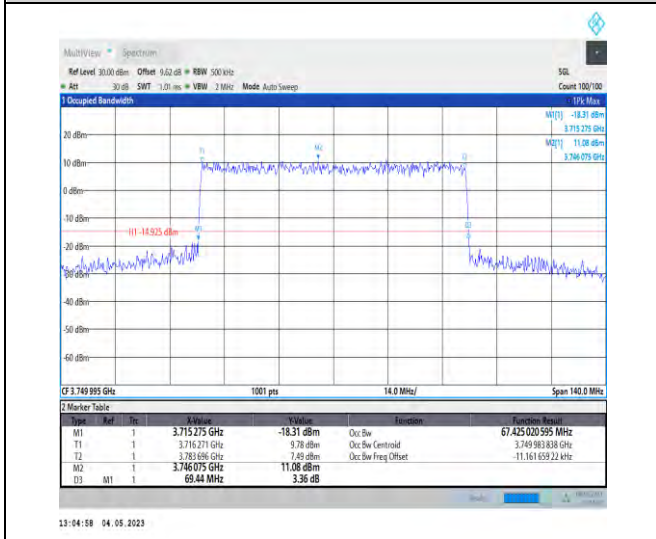
1-N78-3700-3800-PC2-30-70-M-7-CP-16QAM-Outer_Full-189@0-Ant1-67.425-69.440-≤70-PASS
