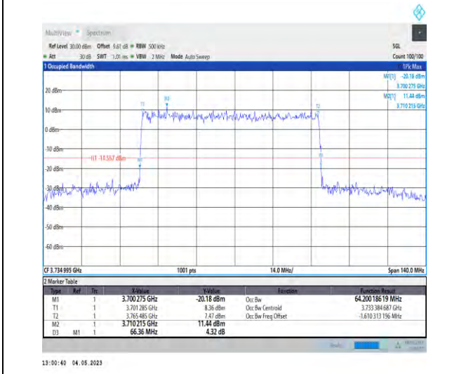
1-N78-3700-3800-PC2-30-70-L-5-DFT-256QAM-Outer_Full-180@0-Ant1-64.2-66.360-≤70-PASS
