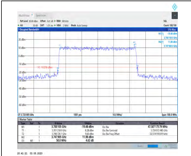
1-N78-3700-3800-PC2-30-50-L-8-CP-64QAM-Outer _Full-133@0-Ant1-47.507-50.000-≤50-PASS
