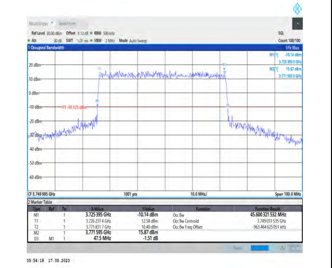
1-N78-3700-3800-PC2-30-50-M-2-DFT-PI2BPSK-Outer _Full-128@0-Ant1-45.600-47.500-≤50-PASS
