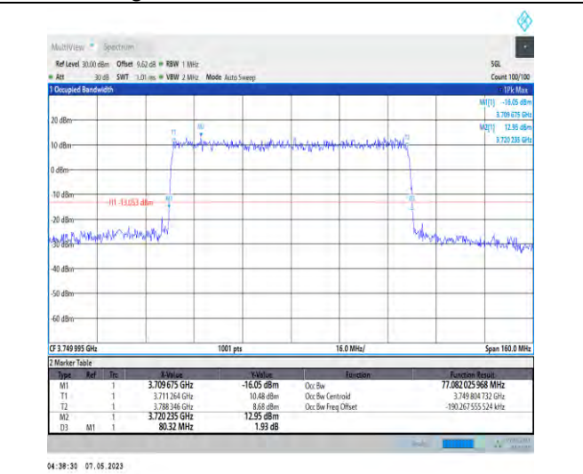
1-N78-3700-3800-PC2-30-80-M-3-DFT-16QAM-Outer_Full-216@0-Ant1-77.082-80.320-≤80-PASS
