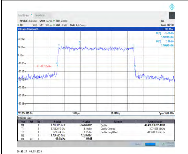
1-N78-3700-3800-PC2-30-50-H-8-CP-64QAM-Outer_Full-133@0-Ant1-47.456-49.400-≤50-PASS
