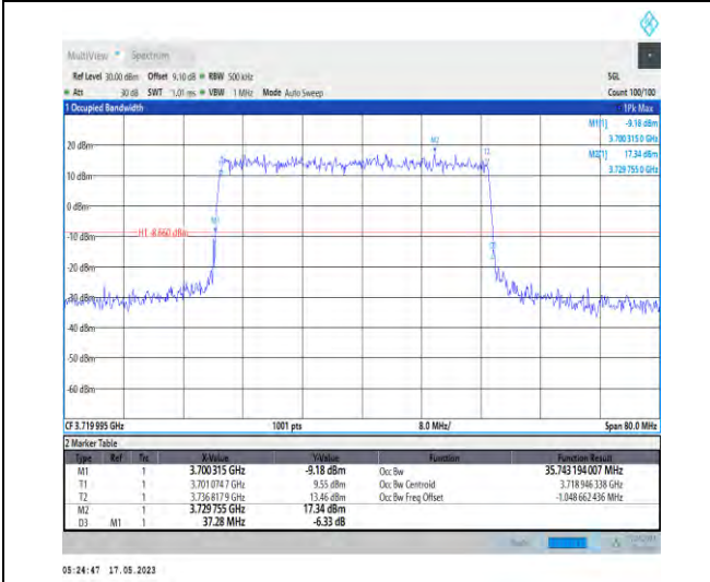
1-N78-3700-3800-PC2-30-40-L-1-DFT-QPSK-Outer_Full-100@0-Ant1-35.743-37.280-≤40-PASS
