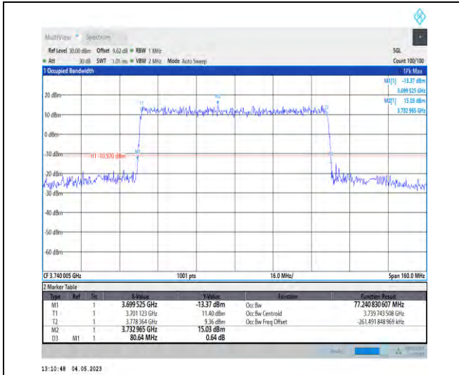
1-N78-3700-3800-PC2-30-80-L-3-DFT-16QAM-Outer_Full-216@0-Ant1-77.241-80.640-≤80-PASS
