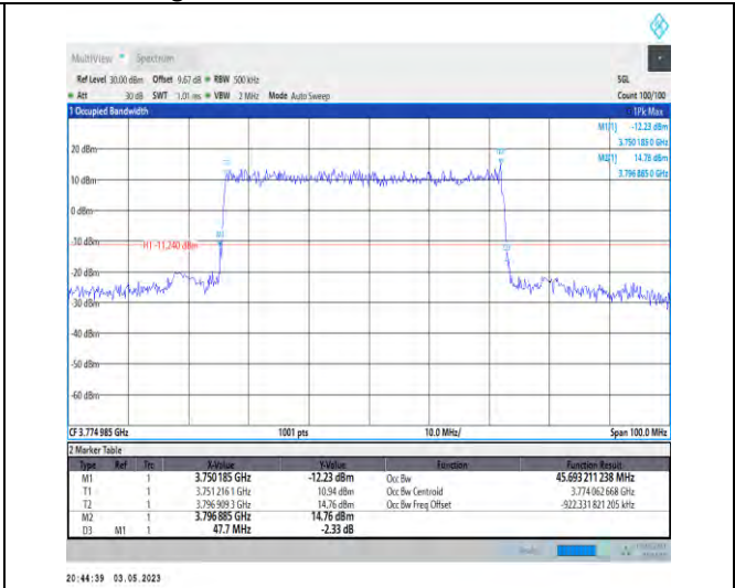
1-N78-3700-3800-PC2-30-50-H-3-DFT-16QAM-Outer_Full-128@0-Ant1-45.693-47.700-≤50-PASS
