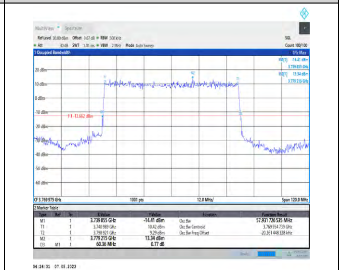
1-N78-3700-3800-PC2-30-60-H-2-DFT-PI2BPSK-Outer_Full-162@0-Ant1-57.932-60.360-≤60-PASS
