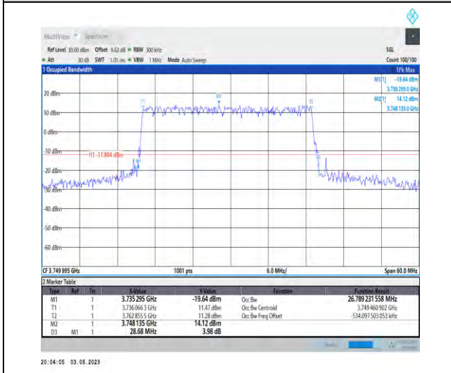
1-N78-3700-3800-PC2-30-30-M-3-DFT-16QAM-Outer_Full-75@0-Ant1-26.789-28.680-≤30-PASS
