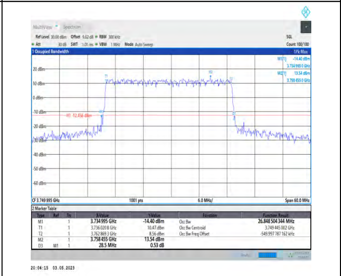
1-N78-3700-3800-PC2-30-30-M-4-DFT-64QAM-Outer_Full-75@0-Ant1-26.849-28.500-≤30-PASS
