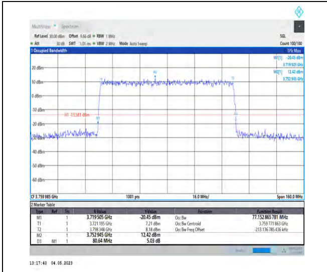
1-N78-3700-3800-PC2-30-80-H-5-DFT-256QAM-Out er_Full-216@0-Ant1-77.153-80.640-≤80-PASS
