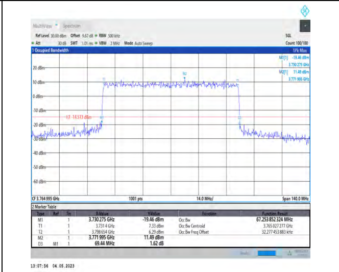
1-N78-3700-3800-PC2-30-70-H-7-CP-16QAM-Outer_Full-189@0-Ant1-67.254-69.440-≤70-PASS
