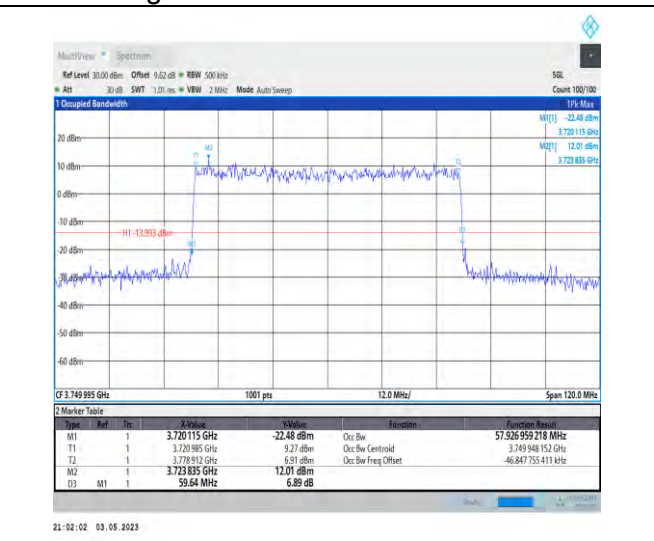
1-N78-3700-3800-PC2-30-60-M-5-DFT-256QAM-Out_er_Full-162@0-Ant1-57.927-59.640-≤60-PASS
