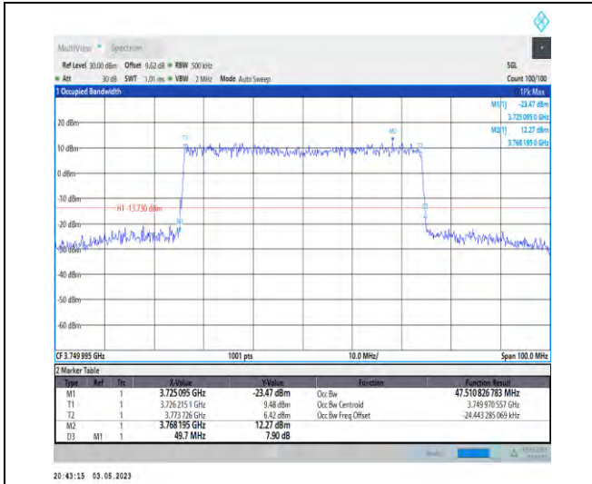
1-N78-3700-3800-PC2-30-50-M-7-CP-16QAM-Outer_Full-133@0-Ant1-47.511-49.700-≤50-PASS
