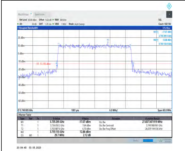
1-N78-3700-3800-PC2-30-30-M-7-CP-16QAM-Outer_Full-78@0-Ant1-27.837-29.700-≤30-PASS
