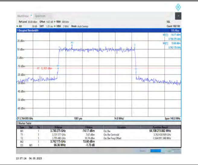
1-N78-3700-3800-PC2-30-70-H-3-DFT-16QAM-Outer_Full-180@0-Ant1-64.108-66.360-≤70-PASS
