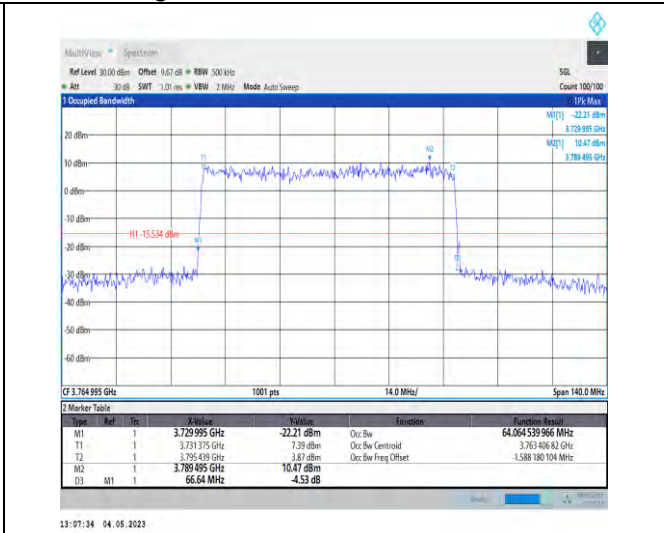
1-N78-3700-3800-PC2-30-70-H-5-DFT-256QAM-Outer_Full-180@0-Ant1-64.065-66.640-≤70-PASS
