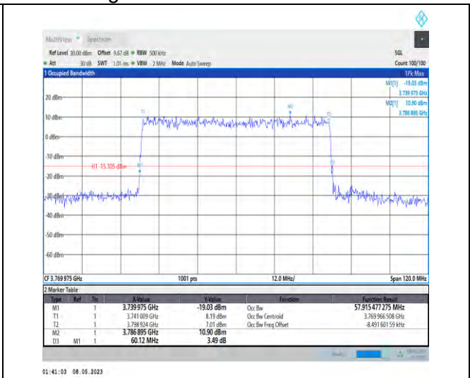
1-N78-3700-3800-PC2-30-60-H-4-DFT-64QAM-Outer_Full-162@0-Ant1-57.915-60.120-≤60-PASS
