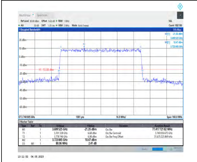
1-N78-3700-3800-PC2-30-80-L-9-CP-256QAM-Outer_Full-217@0-Ant1-77.418-80.960-≤80-PASS
