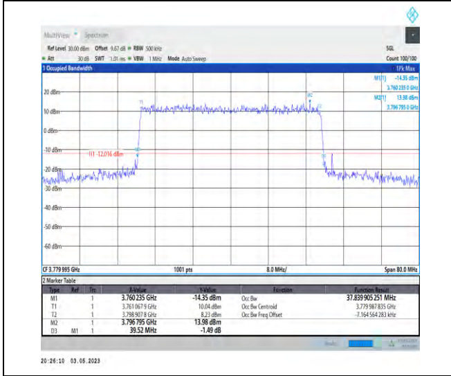
1-N78-3700-3800-PC2-30-40-H-7-CP-16QAM-Outer_Full-106@0-Ant1-37.84-39.520-≤40-PASS
