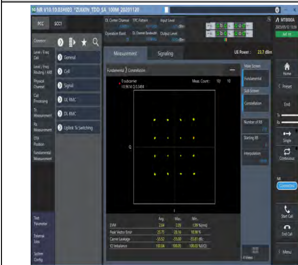
1-N78-3700-3800-PC2-30-100-M-3-DFT-16QAM-Out er_Full-270@0-Ant1-see graph-PASS
