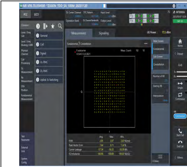
1-N78-3700-3800-PC2-30-100-M-9-CP-256QAM-Out er_Full-273@0-Ant1-see graph-PASS
