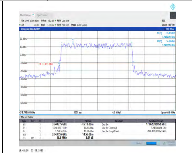
1-N78-3700-3800-PC2-30-20-M-1-DFT-QPSK-Outer_Full-50@0-Ant1-17.862-18.800-≤20-PASS
