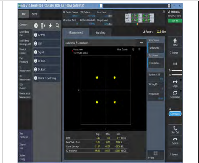
1-N78-3700-3800-PC2-30-100-M-6-CP-QPSK-Outer_Full-273@0-Ant1-see graph-PASS
