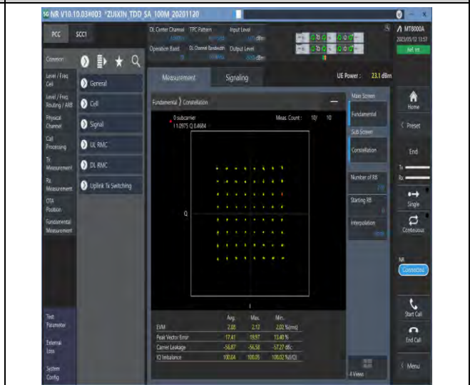
1-N78-3700-3800-PC2-30-100-M-4-DFT-64QAM-Out er_Full-270@0-Ant1-see graph-PASS
