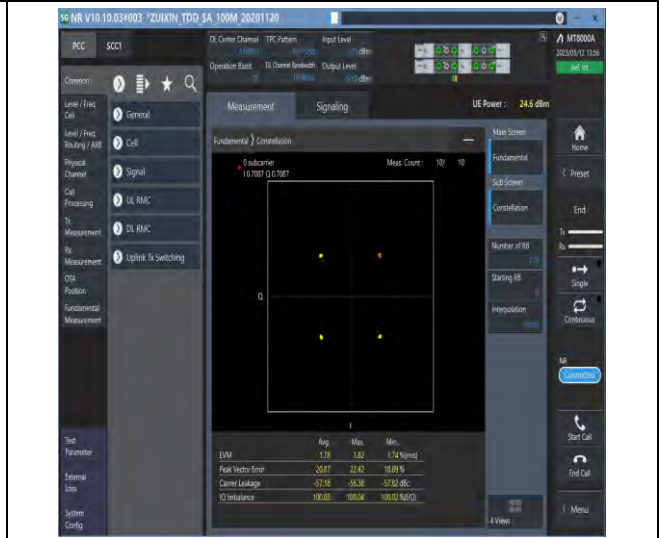
1-N78-3700-3800-PC2-30-100-M-2-DFT-QPSK-Out er_Full-270@0-Ant1-see graph-PASS
