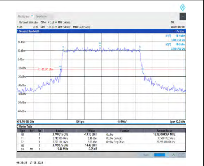
1-N78-3700-3800-PC2-30-20-M-7-CP-16QAM-Outer_Full-51@0-Ant1-18.194-19.440-≤20-PASS
