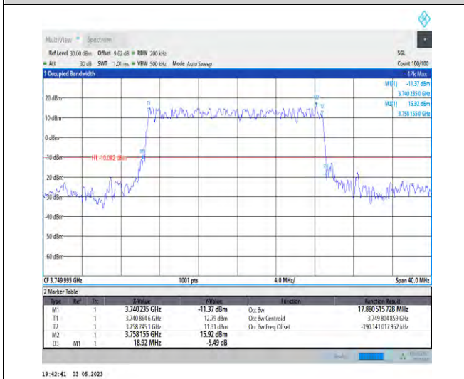
1-N78-3700-3800-PC2-30-20-M-2-DFT-PI2BPSK-Outer_Full-50@0-Ant1-17.881-18.920-≤20-PASS
