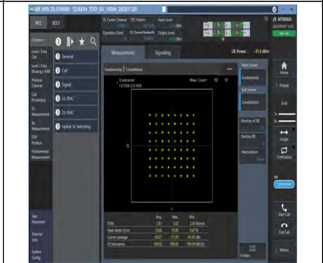
1-N78-3700-3800-PC2-30-100-M-8-CP-64QAM-Outer_Full-273@0-Ant1-see graph-PASS
