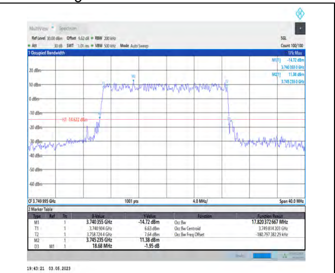
1-N78-3700-3800-PC2-30-20-M-5-DFT-256QAM-Out er_Full-50@0-Ant1-17.82-18.680-≤20-PASS
