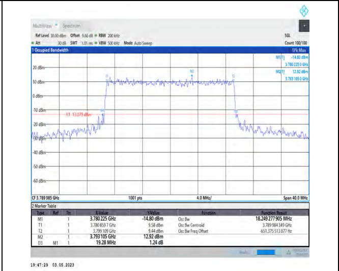
1-N78-3700-3800-PC2-30-20-H-6-CP-QPSK-Outer_Full-51@0-Ant1-18.249-19.280-≤20-PASS
