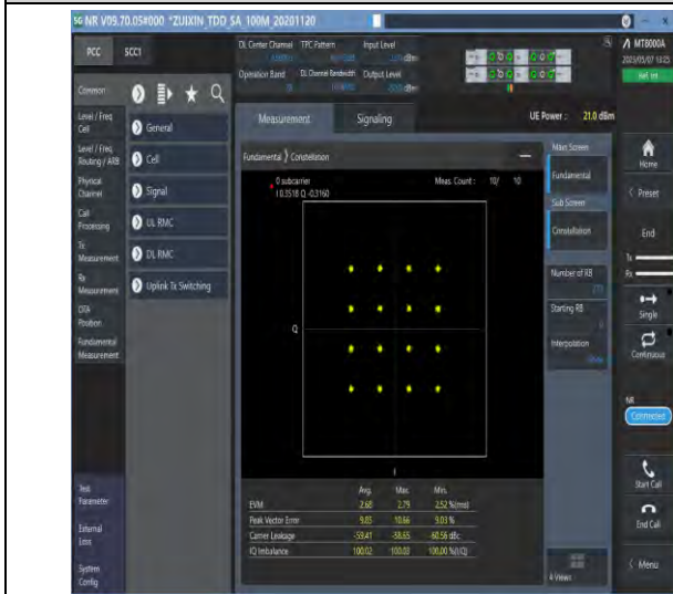
1-N78-3700-3800-PC2-30-100-M-7-CP-16QAM-Outer_Full-273@0-Ant1-see graph-PASS
