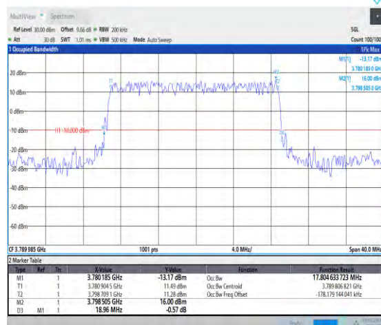
1-N78-3700-3800-PC2-30-20-H-2-DFT-PI2BPSK-Outer_Full-50@0-Ant1-17.805-18.960-≤20-PASS
