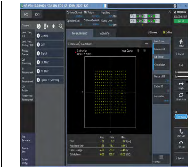
1-N78-3700-3800-PC2-30-100-M-5-DFT-256QAM-Outer_Full-270@0-Ant1-see graph-PASS
