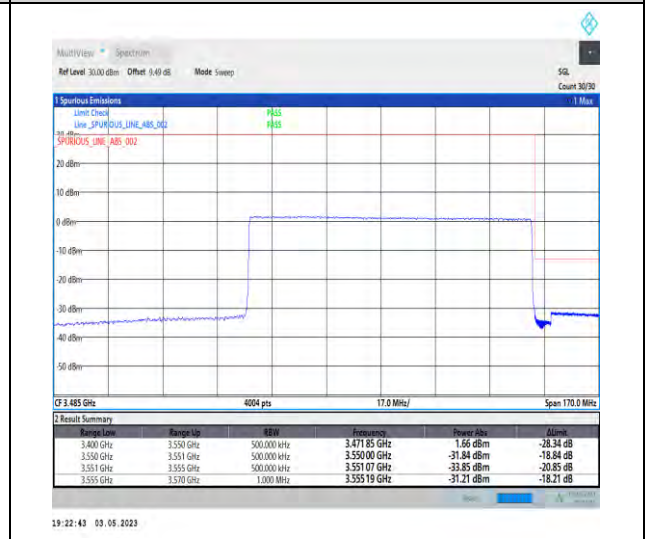
1-N78-3450-3550-PC2-30-90-H-6-CP-QPSK-Outer_Full-245@0-Ant1-1--PASS-see graph
