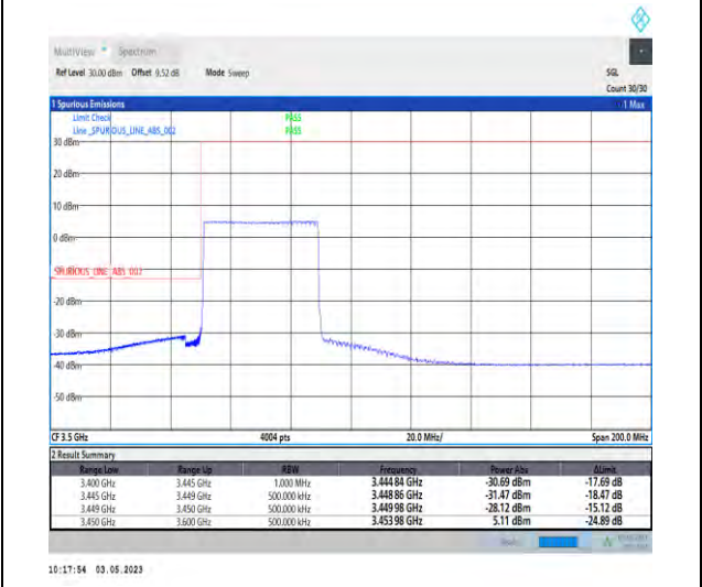
1-N78-3450-3550-PC2-30-40-L-6-CP-QPSK-Outer_Full-106@0-Ant1-1--PASS-see graph
