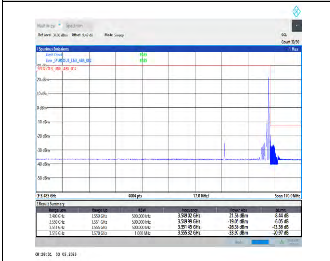
1-N78-3450-3550-PC2-30-30-H-5-CP-QPSK-Edge_1RB_Right-1@77-Ant1-1--PASS-see graph
