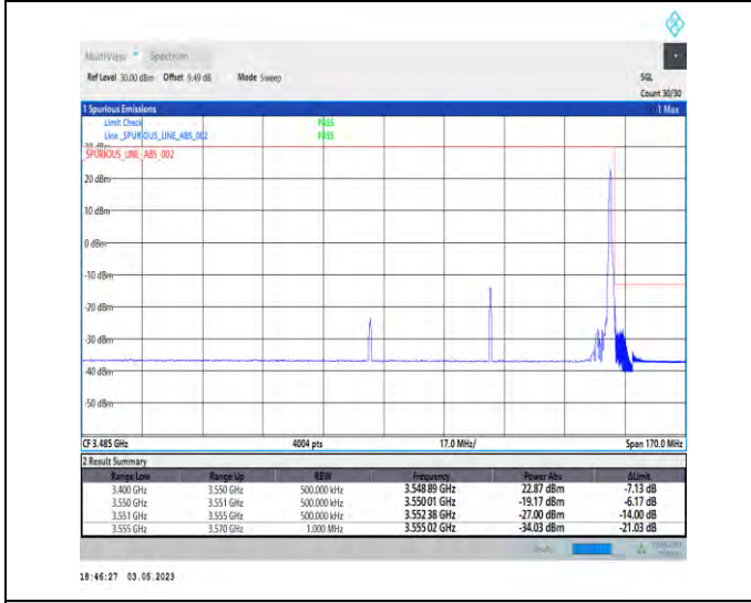
1-N78-3450-3550-PC2-30-70-H-5-CP-QPSK-Edge_1RB_Right-1@188-Ant1-1--PASS-see graph
