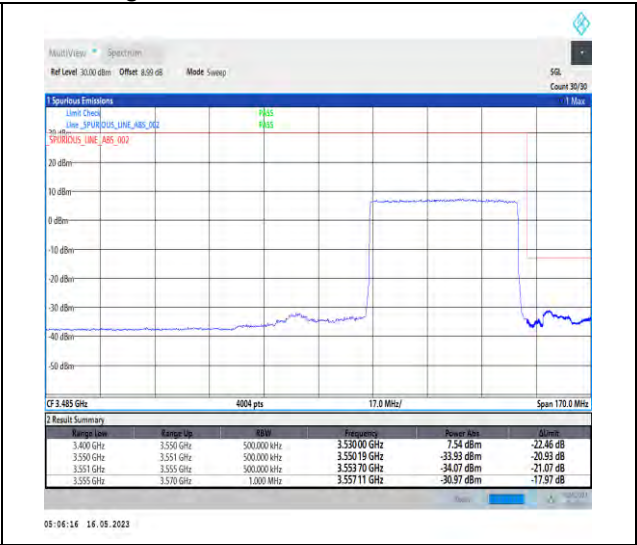
1-N78-3450-3550-PC2-30-50-H-3-DFT-PI2BPSK-Outer_Full-128@0-Ant1-1--PASS-see graph
