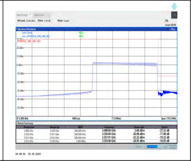
1-N78-3450-3550-PC2-30-70-H-6-CP-QPSK-Outer_Full-189@0-Ant1-1--PASS-see graph
