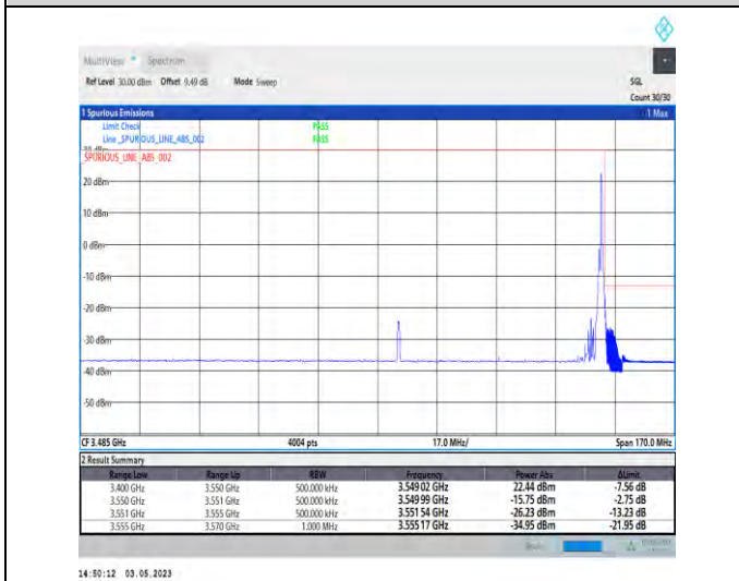
1-N78-3450-3550-PC2-30-60-H-5-CP-QPSK-Edge_1RB_Right-1@161-Ant1-1--PASS-see graph
