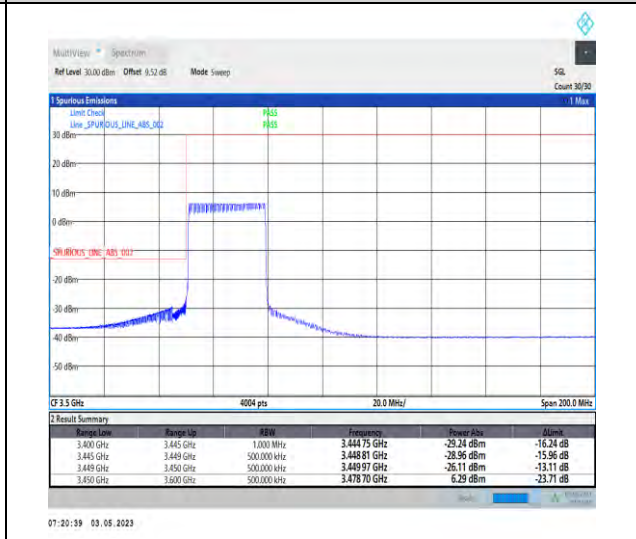
1-N78-3450-3550-PC2-30-30-L-6-CP-QPSK-Outer_Full-78@0-Ant1-1--PASS-see graph
