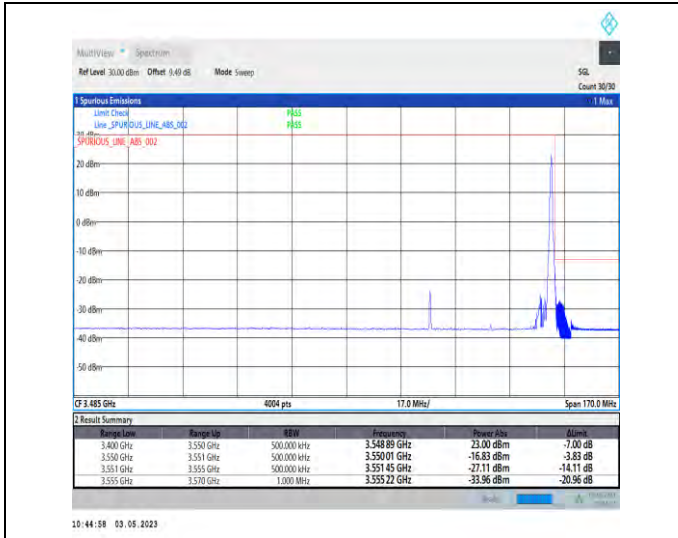
1-N78-3450-3550-PC2-30-40-H-2-DFT-PI2BPSK-Edge_1RB_Right-1@105-Ant1-1--PASS-see graph
