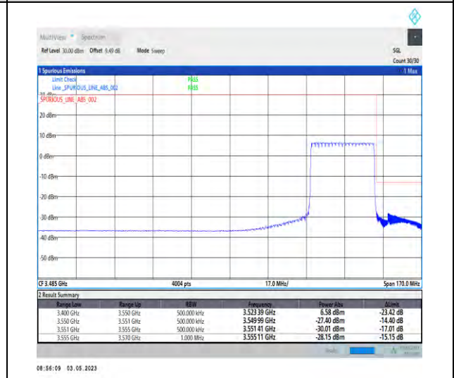
1-N78-3450-3550-PC2-30-30-H-6-CP-QPSK-Outer_Full-78@0-Ant1-1--PASS-see graph
