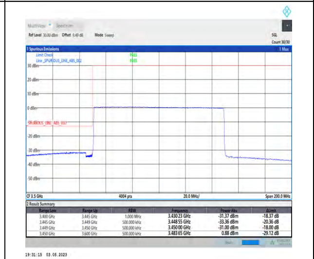
1-N78-3450-3550-PC2-30-100-L-6-CP-QPSK-Outer_Full-273@0-Ant1-1--PASS-see graph
