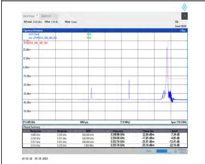
1-N78-3450-3550-PC2-30-80-H-5-CP-QPSK-Edge_1RB_Right-1@216-Ant1-1--PASS-see graph
