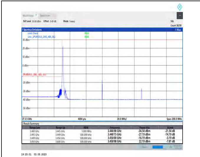
1-N78-3450-3550-PC2-30-100-L-1-DFT-PI2BPSK-Edge_1_RB_Left-1@0-Ant1-1--PASS-see graph
