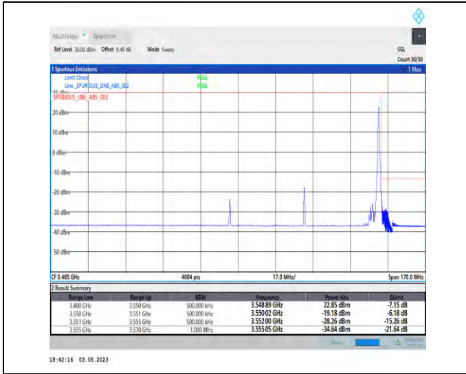
1-N78-3450-3550-PC2-30-70-H-2-DFT-PI2BPSK-Edge_1RB_Right-1@188-Ant1-1--PASS-see graph
