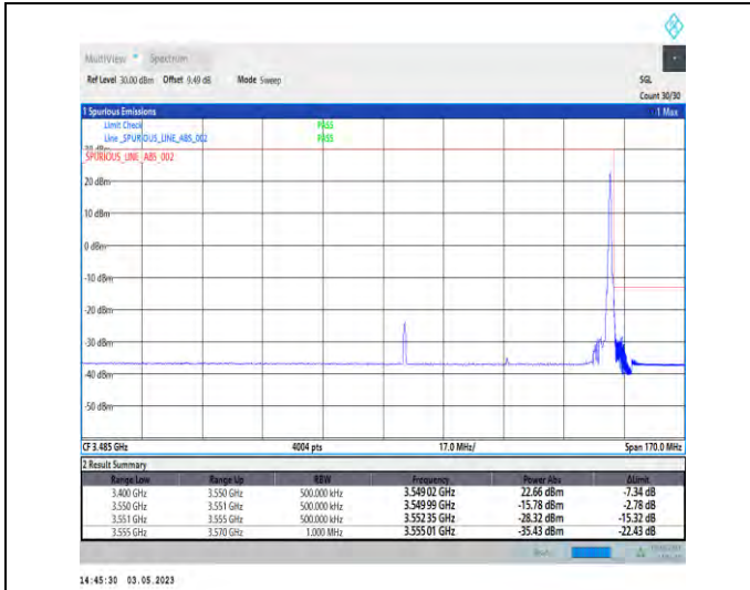
1-N78-3450-3550-PC2-30-60-H-2-DFT-PI2BPSK-Edge_1RB_Right-1@161-Ant1-1--PASS-see graph
