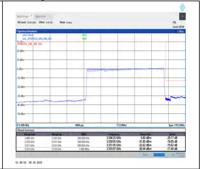
1-N78-3450-3550-PC2-30-80-H-3-DFT-PI2BPSK-Outer_Full-216@0-Ant1-1--PASS-see graph
