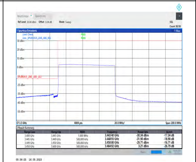
1-N78-3450-3550-PC2-30-70-L-6-CP-QPSK-Outer_Full-189@0-Ant1-1--PASS-see graph
