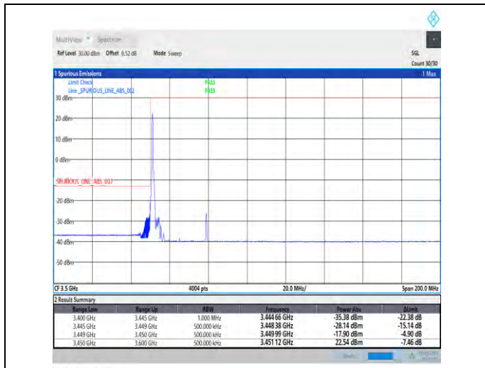
1-N78-3450-3550-PC2-30-30-L-1-DFT-PI2BPSK-Edge_1RB_Left-1@0-Ant1-1--PASS-see graph
