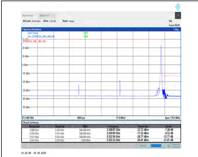
1-N78-3450-3550-PC2-30-90-H-2-DFT-PI2BPSK-Edge_1RB_Right-1@244-Ant1-1--PASS-see graph
