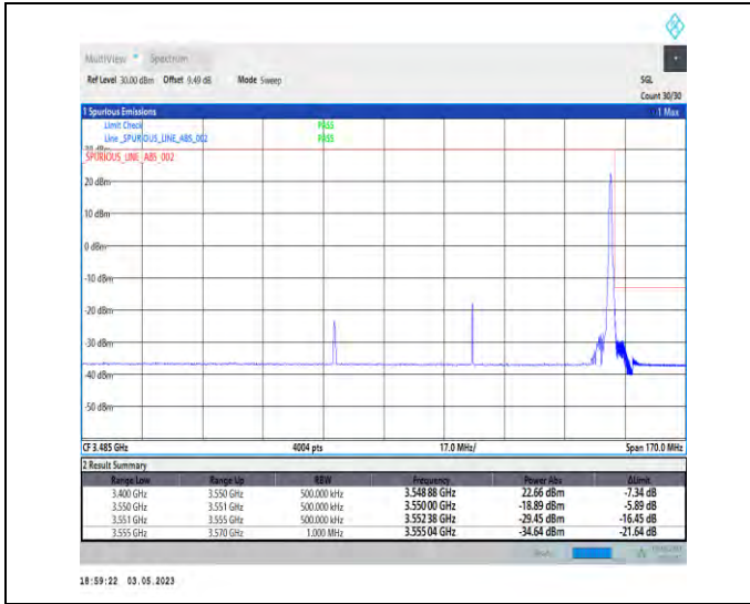
1-N78-3450-3550-PC2-30-80-H-2-DFT-PI2BPSK-Edge_1RB_Right-1@216-Ant1-1--PASS-see graph
