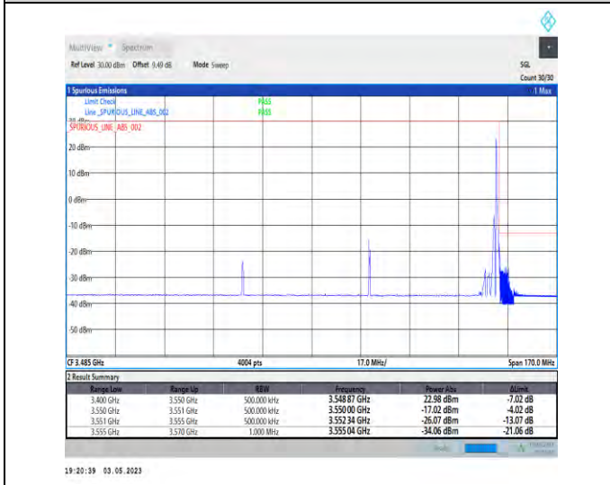
1-N78-3450-3550-PC2-30-90-H-5-CP-QPSK-Edge_1RB_Right-1@244-Ant1-1--PASS-see graph
