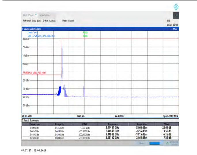
1-N78-3450-3550-PC2-30-30-L-4-CP-QPSK-Edge_1RB_Left-1@0-Ant1-1--PASS-see graph
