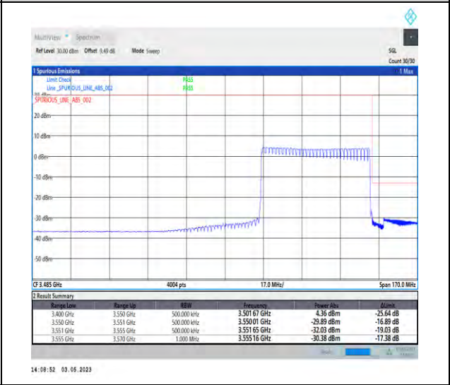
1-N78-3450-3550-PC2-30-50-H-6-CP-QPSK-Outer_Full-133@0-Ant1-1--PASS-see graph
