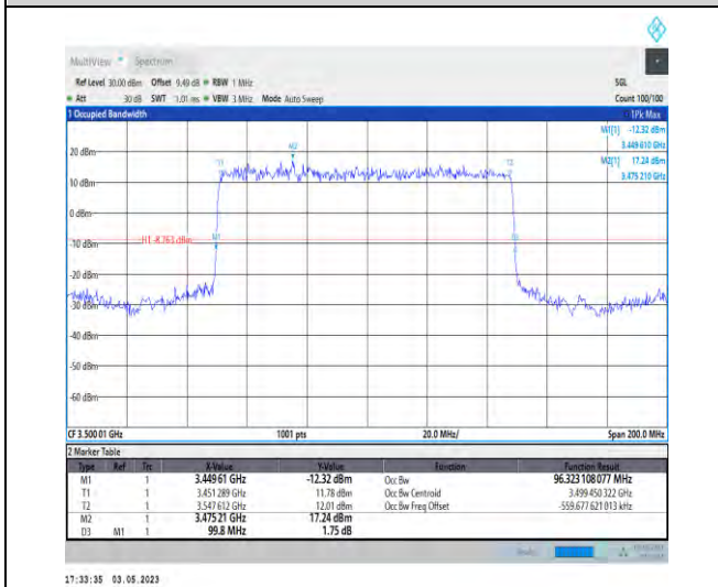
1-N78-3450-3550-PC2-30-100-M-2-DFT-PI2BPSK-Outer_Full-270@0-Ant1-96.323-99.800-≤100-PASS
