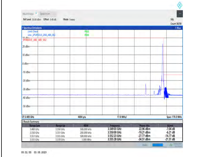
1-N78-3450-3550-PC2-30-20-H-5-CP-QPSK-Edge_1RB_Right-1@50-Ant1-1--PASS-see graph
