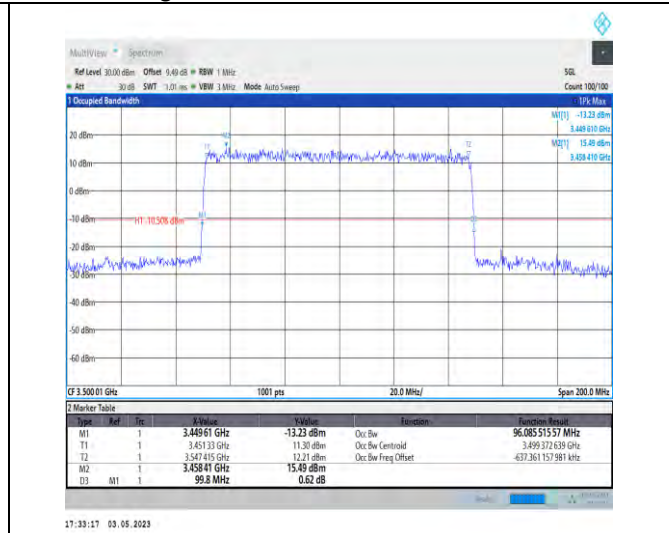
1-N78-3450-3550-PC2-30-100-M-1-DFT-QPSK-Outer_Full-270@0-Ant1-96.086-99.800-≤100-PASS
