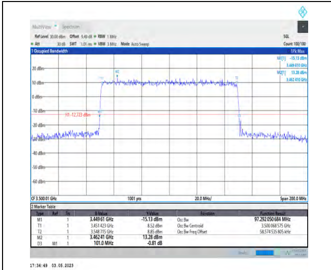
1-N78-3450-3550-PC2-30-100-M-8-CP-64QAM-Out er_Full-273@0-Ant1-97.292-101.000-≤100-PASS
