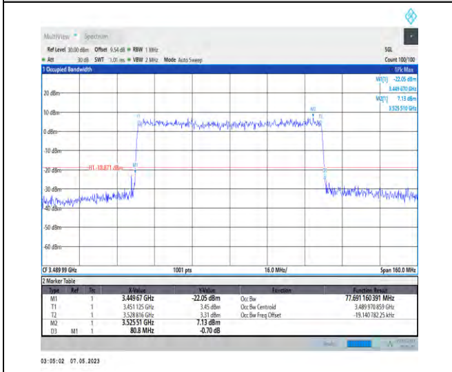
1-N78-3450-3550-PC2-30-80-L-9-CP-256QAM-Outer_Full-217@0-Ant1-77.691-80.800-≤80-PASS
