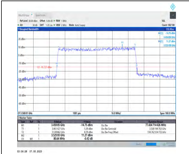
1-N78-3450-3550-PC2-30-80-M-6-CP-QPSK-Outer_Full-217@0-Ant1-77.435-80.640-≤80-PASS
