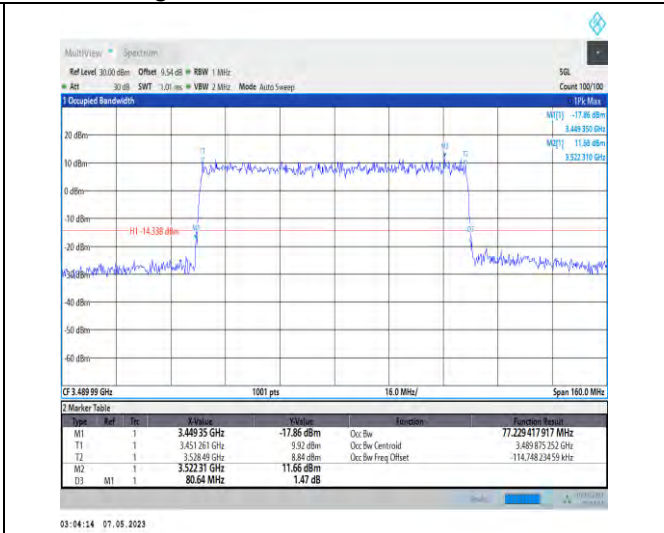
1-N78-3450-3550-PC2-30-80-L-4-DFT-64QAM-Outer_Full-216@0-Ant1-77.229-80.640-≤80-PASS
