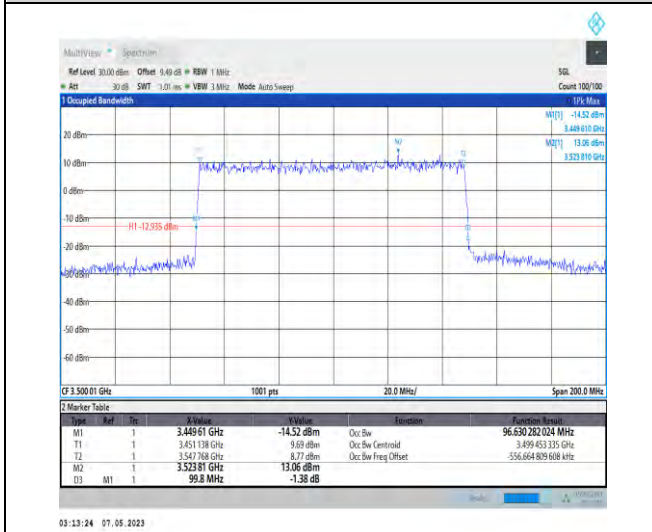
1-N78-3450-3550-PC2-30-100-H-1-DFT-QPSK-Out er_Full-270@0-Ant1-96.63-99.800-≤100-PASS
