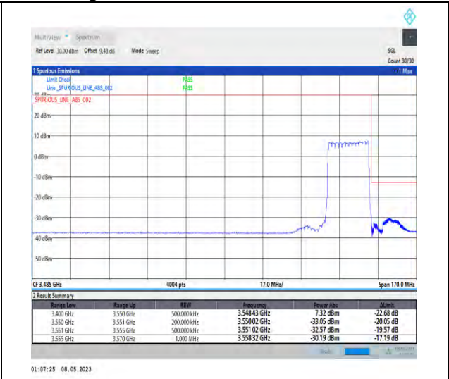
1-N78-3450-3550-PC2-30-20-H-3-DFT-PI2BPSK-Outer_Full-50@0-Ant1-1--PASS-see graph
