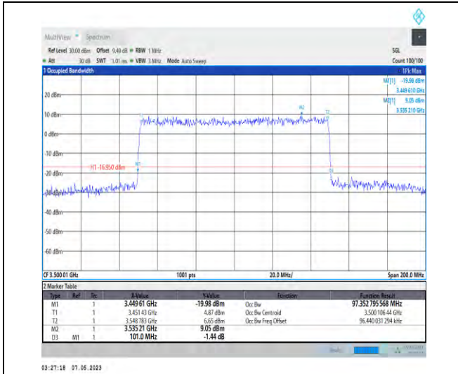
1-N78-3450-3550-PC2-30-100-H-7-CP-16QAM-Out er_Full-273@0-Ant1-97.353-101.000-≤100-PASS
