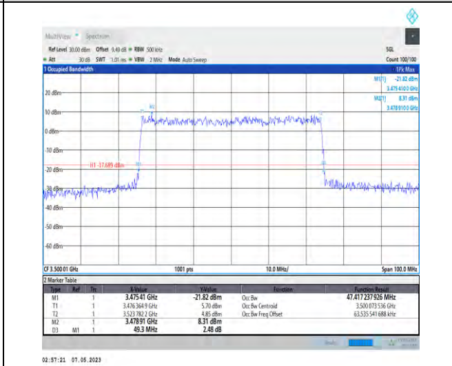
1-N78-3450-3550-PC2-30-50-M-6-CP-QPSK-Out_Full-133@0-Ant1-47.417-49.300-≤50-PASS
