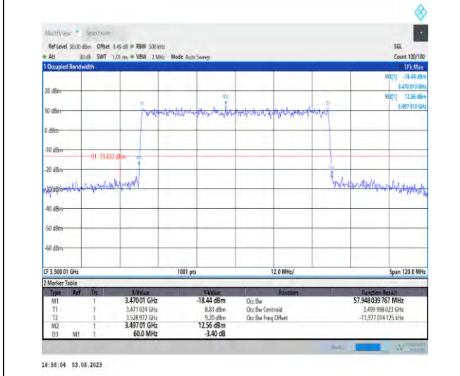
1-N78-3450-3550-PC2-30-60-M-6-CP-QPSK-Outer Full-162@0-Ant1-57.948-60.000-≤60-PASS
