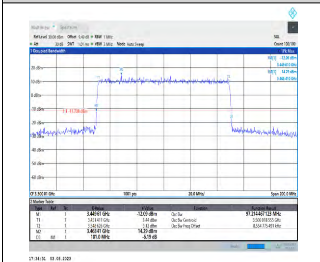
1-N78-3450-3550-PC2-30-100-M-6-CP-QPSK-Outer_Full-273@0-Ant1-97.214-101.000-≤100-PASS
