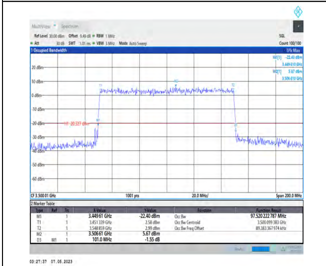
1-N78-3450-3550-PC2-30-100-H-9-CP-256QAM-Out er_Full-273@0-Ant1-97.52-101.000-≤100-PASS
