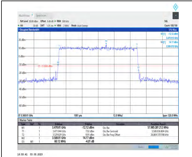
1-N78-3450-3550-PC2-30-60-M-4-DFT-64QAM-Out er_Full-162@0-Ant1-57.985-60.120-≤60-PASS
