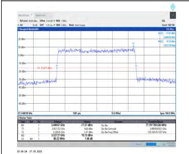
1-N78-3450-3550-PC2-30-80-L-5-DFT-256QAM-Outer_Full-216@0-Ant1-77.198-80.320-≤80-PASS
