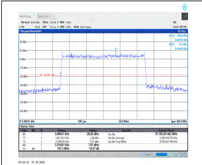
1-N78-3450-3550-PC2-30-100-L-9-CP-256QAM-Out er_Full-273@0-Ant1-97.195-101.200-≤100-PASS
