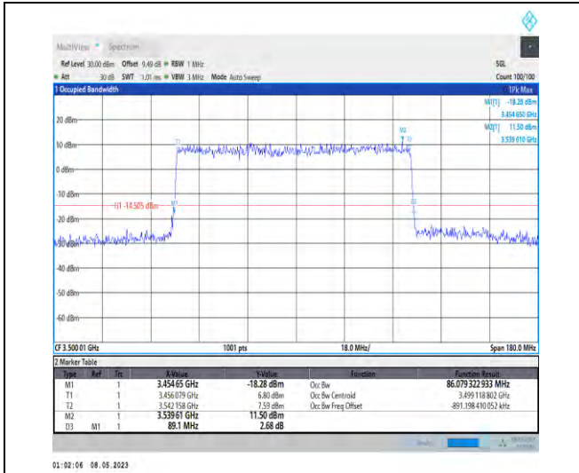
1-N78-3450-3550-PC2-30-90-M-3-DFT-16QAM-Out er_Full-240@0-Ant1-86.079-89.100-≤90-PASS
