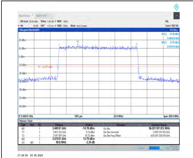
1-N78-3450-3550-PC2-30-100-M-4-DFT-64QAM-Outer_Full-270@0-Ant1-96.032-99.800-≤100-PASS
