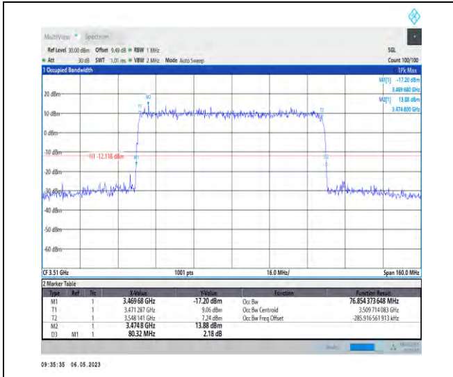
1-N78-3450-3550-PC2-30-80-H-5-DFT-256QAM-Out _Full-216@0-Ant1-76.854-80.320-≤80-PASS
