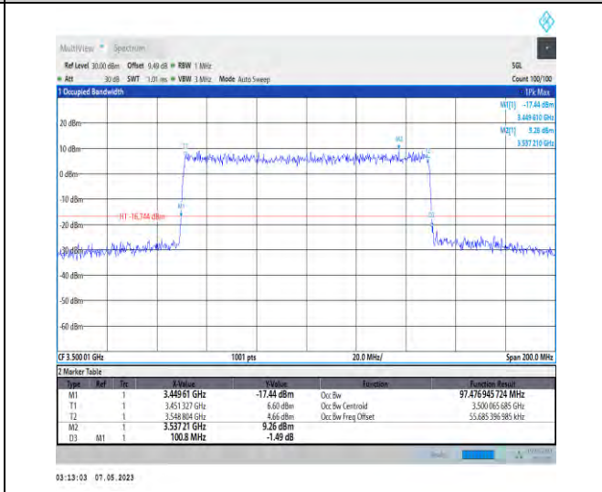
1-N78-3450-3550-PC2-30-100-L-8-CP-64QAM-Outer_Full-273@0-Ant1-97.477-100.800-≤100-PASS
