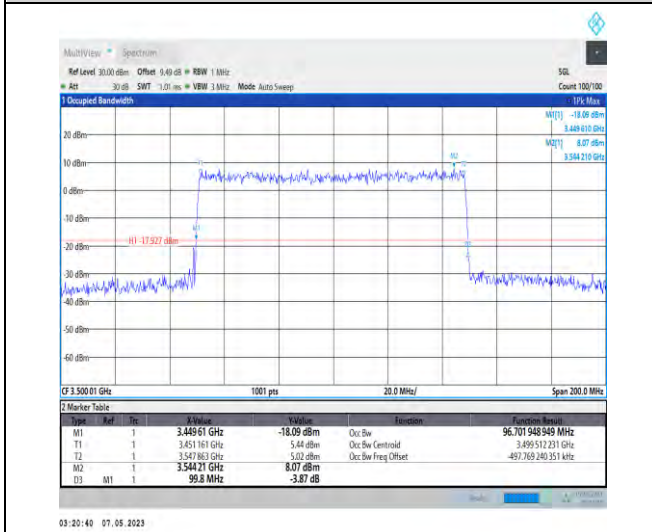
1-N78-3450-3550-PC2-30-100-H-5-DFT-256QAM-Out er_Full-270@0-Ant1-96.702-99.800-≤100-PASS
