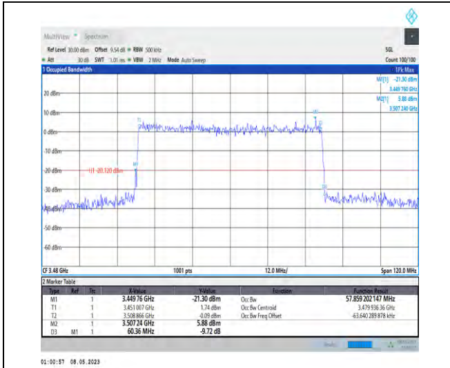
1-N78-3450-3550-PC2-30-60-L-9-CP-256QAM-Outer_Full-162@0-Ant1-57.859-60.360-≤60-PASS
