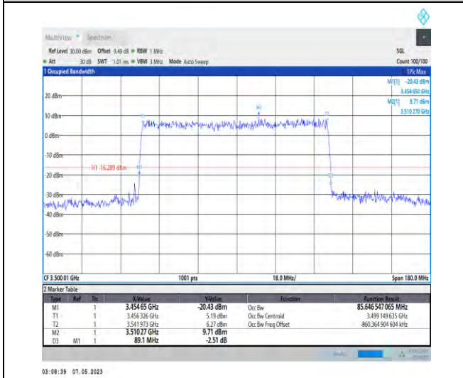
1-N78-3450-3550-PC2-30-90-M-5-DFT-256QAM-Out er_Full-240@0-Ant1-85.647-89.100-≤90-PASS
