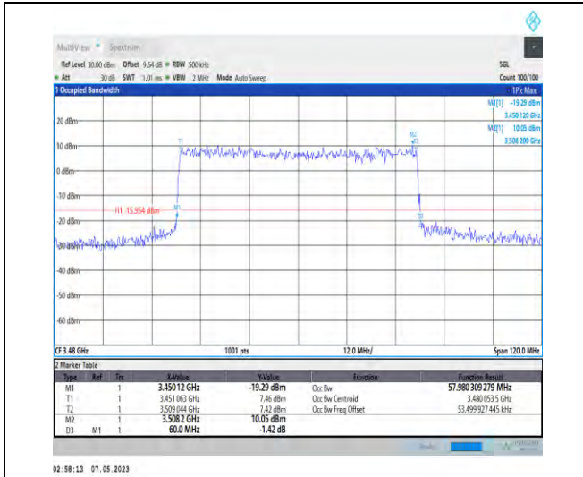
1-N78-3450-3550-PC2-30-60-L-1-DFT-QPSK-Outer_Full-162@0-Ant1-57.98-60.000-≤60-PASS
