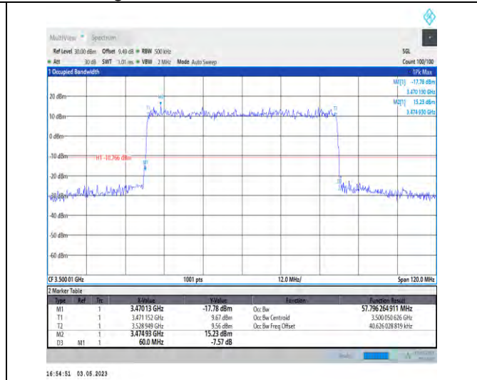
1-N78-3450-3550-PC2-30-60-M-1-DFT-QPSK-Outer_Full-162@0-Ant1-57.796-60.000-≤60-PASS
