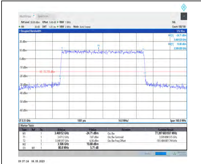
1-N78-3450-3550-PC2-30-80-H-9-CP-256QAM-Out er_Full-217@0-Ant1-77.398-80.800-≤80-PASS
