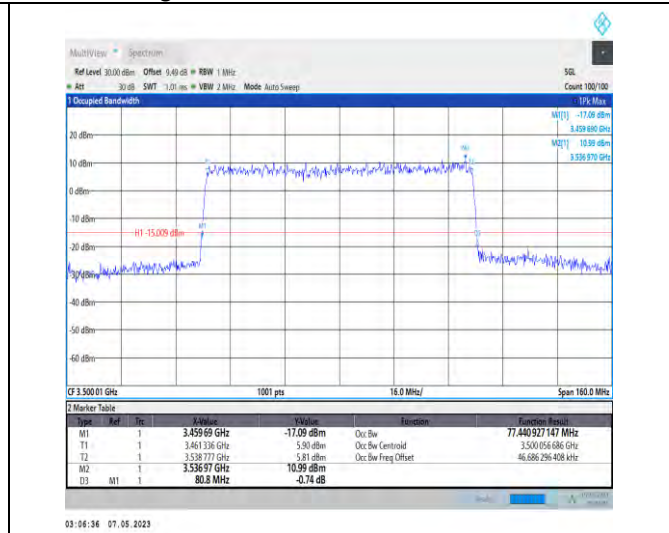
1-N78-3450-3550-PC2-30-80-M-7-CP-16QAM-Outer_Full-217@0-Ant1-77.441-80.800-≤80-PASS
