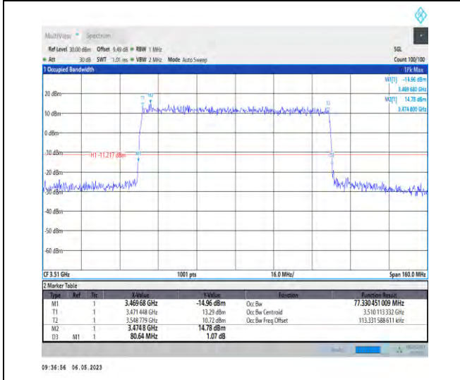
1-N78-3450-3550-PC2-30-80-H-7-CP-16QAM-Outer _Full-217@0-Ant1-77.33-80.640-≤80-PASS
