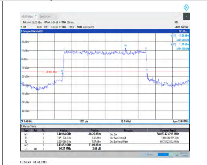
1-N78-3450-3550-PC2-30-60-L-2-DFT-PI2BPSK-Outer_Full-162@0-Ant1-58.07-60.240-≤60-PASS
