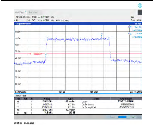
1-N78-3450-3550-PC2-30-80-L-3-DFT-16QAM-Outer_Full-216@0-Ant1-77.167-80.800-≤80-PASS
