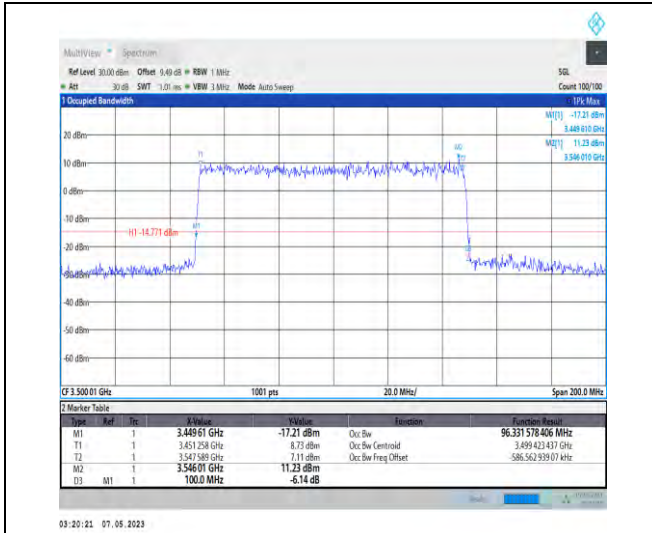
1-N78-3450-3550-PC2-30-100-H-3-DFT-16QAM-Out er_Full-270@0-Ant1-96.332-100.000-≤100-PASS
