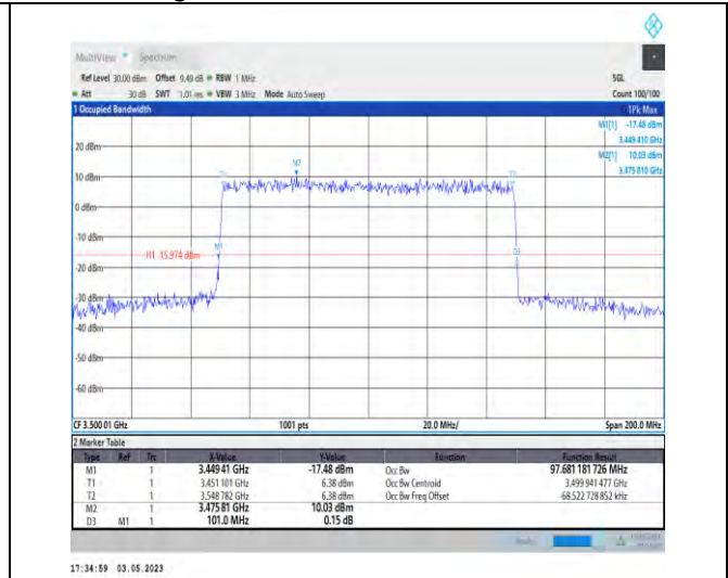
1-N78-3450-3550-PC2-30-100-M-9-CP-256QAM-Out er_Full-273@0-Ant1-97.681-101.000-≤100-PASS
