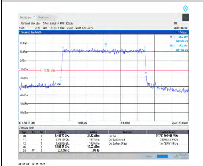
1-N78-3450-3550-PC2-30-60-M-2-DFT-PI2BPSK-Outer_Full-162@0-Ant1-57.798-60.120-≤60-PASS
