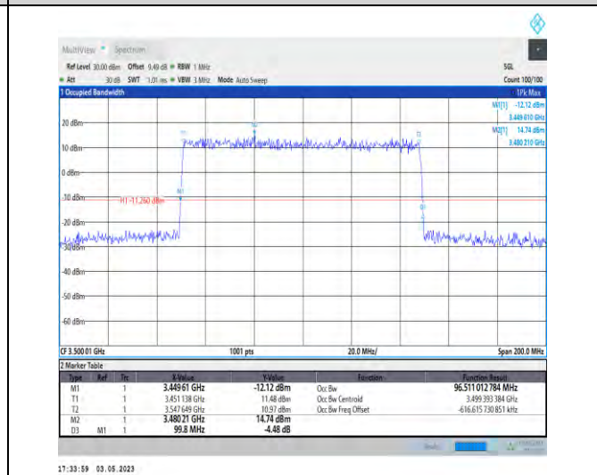
1-N78-3450-3550-PC2-30-100-M-3-DFT-16QAM-Outer_Full-270@0-Ant1-96.511-99.800-≤100-PASS
