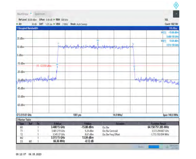
1-N78-3450-3550-PC2-30-70-H-3-DFT-16QAM-Outer_Full-180@0-Ant1-64.151-66.360-≤70-PASS
