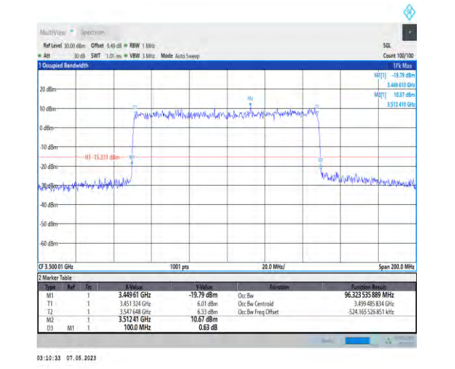
1-N78-3450-3550-PC2-30-100-L-4-DFT-64QAM-Outer_Full-270@0-Ant1-96.324-100.000-≤100-PASS
