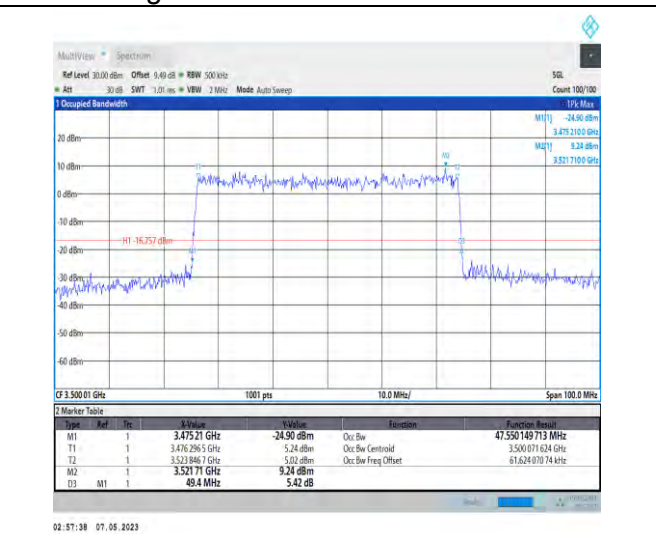
1-N78-3450-3550-PC2-30-50-M-8-CP-64QAM-Outer_Full-133@0-Ant1-47.55-49.400-≤50-PASS
