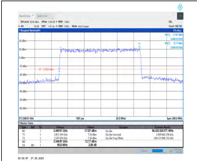
1-N78-3450-3550-PC2-30-100-L-1-DFT-QPSK-Outer_Full-270@0-Ant1-96.432-99.800-≤100-PASS
