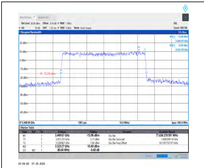
1-N78-3450-3550-PC2-30-80-L-7-CP-16QAM-Outer_Full-217@0-Ant1-77.636-80.640-≤80-PASS
