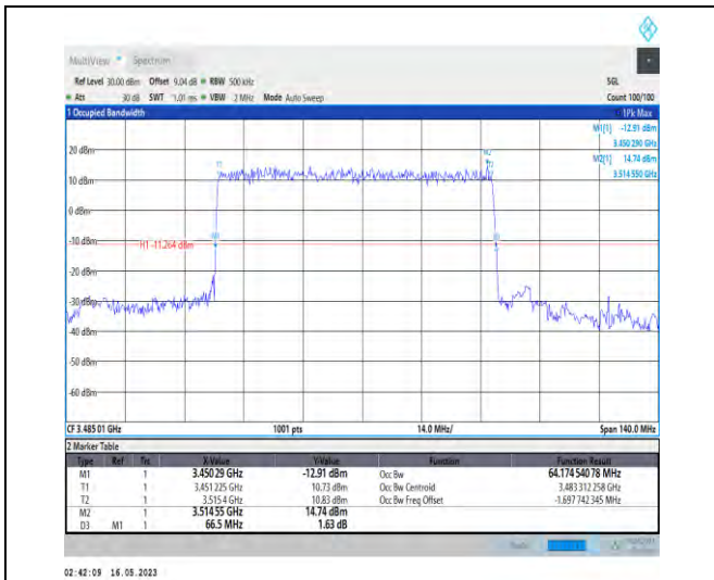
1-N78-3450-3550-PC2-30-70-L-2-DFT-PI2BPSK-Outer_Full-180@0-Ant1-64.175-66.500-≤70-PASS
