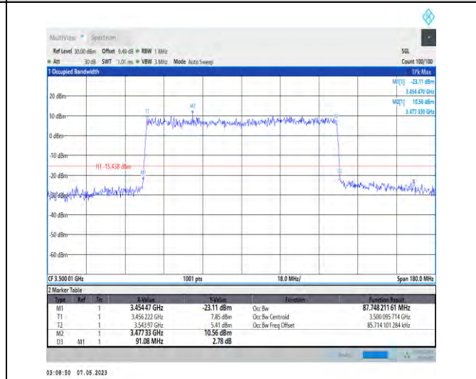
1-N78-3450-3550-PC2-30-90-M-6-CP-QPSK-Out er_Full-245@0-Ant1-87.748-91.080-≤90-PASS
