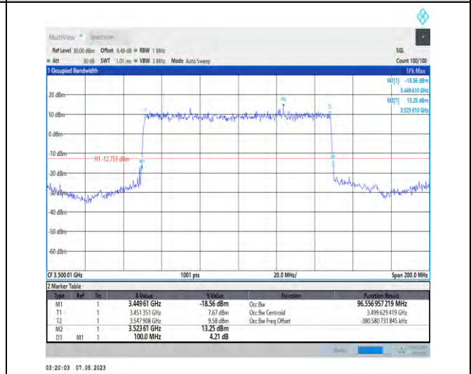
1-N78-3450-3550-PC2-30-100-H-2-DFT-PI2BPSK-Out er_Full-270@0-Ant1-96.557-100.000-≤100-PASS
