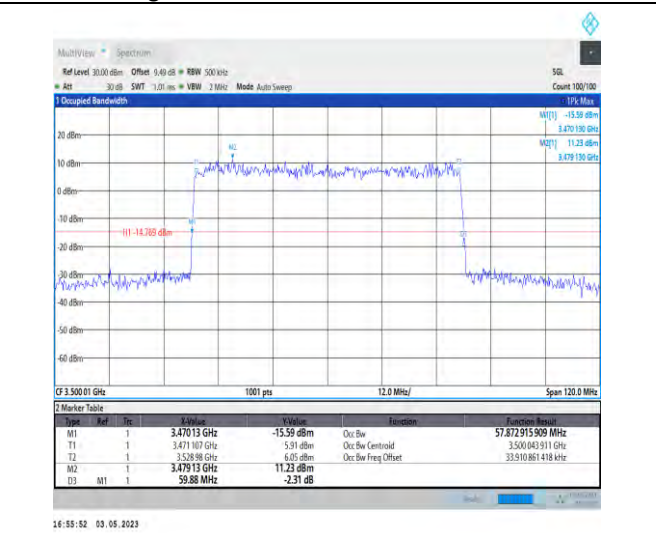
1-N78-3450-3550-PC2-30-60-M-5-DFT-256QAM-Out er_Full-162@0-Ant1-57.873-59.880-≤60-PASS
