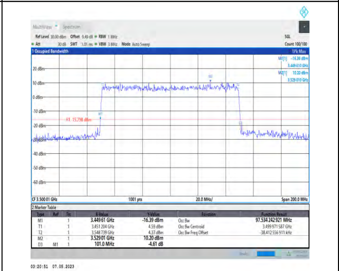
1-N78-3450-3550-PC2-30-100-H-6-CP-QPSK-Outer _Full-273@0-Ant1-97.534-101.000-≤100-PASS
