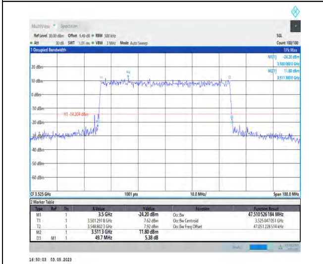
1-N78-3450-3550-PC2-30-50-H-8-CP-64QAM-Outer_Full-133@0-Ant1-47.511-49.700-≤50-PASS
