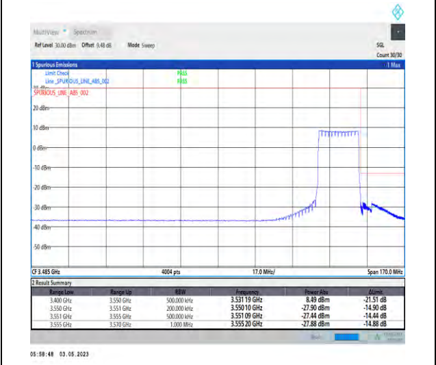
1-N78-3450-3550-PC2-30-20-H-6-CP-QPSK-Outer_Full-51@0-Ant1-1--PASS-see graph
