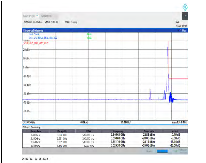
1-N78-3450-3550-PC2-30-20-H-2-DFT-PI2BPSK-Edge_1RB_Right-1@50-Ant1-1--PASS-see graph
