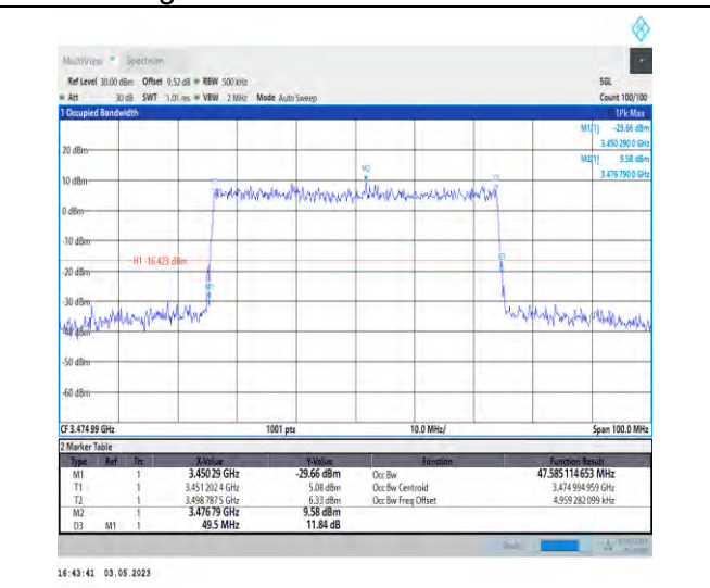
1-N78-3450-3550-PC2-30-50-L-9-CP-256QAM-Outer_Full-133@0-Ant1-47.585-49.500-≤50-PASS
