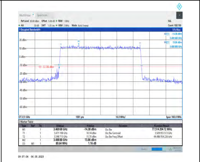
1-N78-3450-3550-PC2-30-80-H-8-CP-64QAM-Outer _Full-217@0-Ant1-77.514-80.640-≤80-PASS
