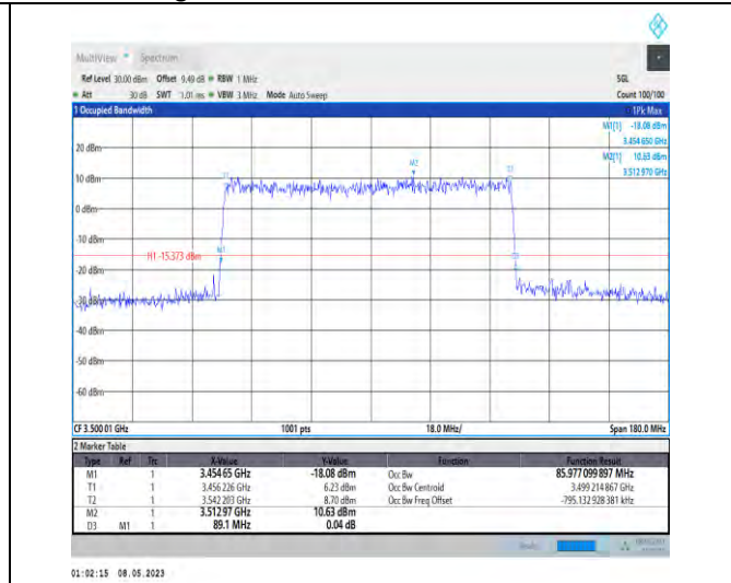
1-N78-3450-3550-PC2-30-90-M-4-DFT-64QAM-Out er_Full-240@0-Ant1-85.977-89.100-≤90-PASS
