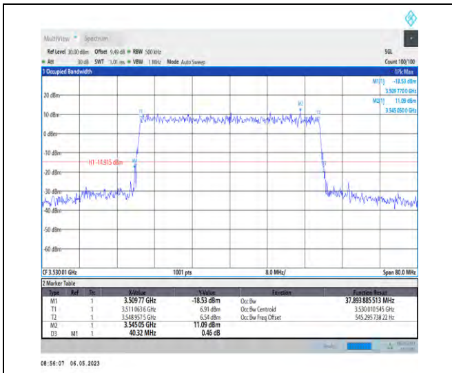
1-N78-3450-3550-PC2-30-40-H-9-CP-256QAM-Out er_Full-106@0-Ant1-37.894-40.320-≤40-PASS
