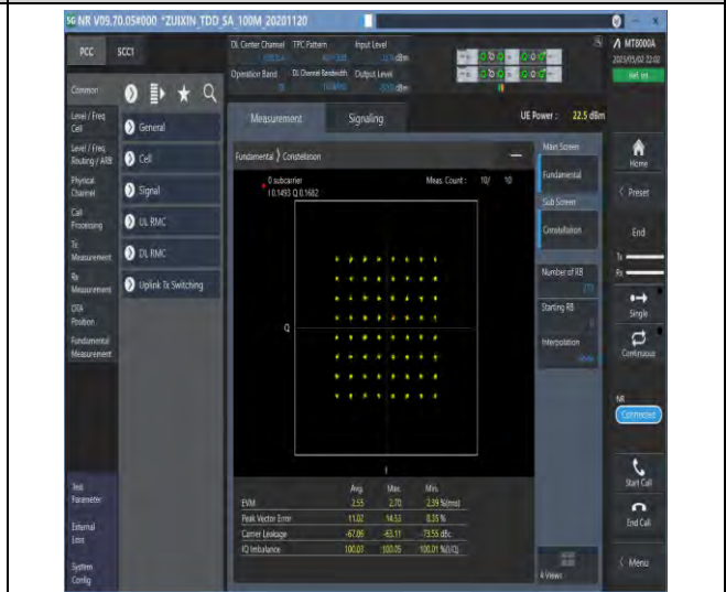
1-N78-3450-3550-PC2-30-100-M-8-CP-64QAM-Outer_Full-273@0-Ant1-see graph-PASS
