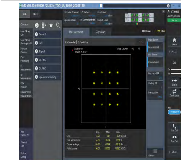
1-N78-3450-3550-PC2-30-100-M-7-CP-16QAM-Outer_Full-273@0-Ant1-see graph-PASS
