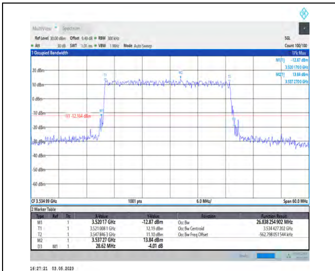
1-N78-3450-3550-PC2-30-30-H-4-DFT-64QAM-Outer_Full-75@0-Ant1-26.838-28.620-≤30-PASS
