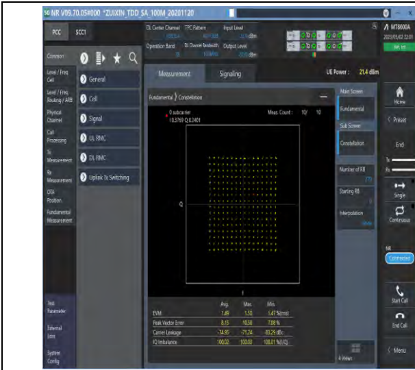
1-N78-3450-3550-PC2-30-100-M-5-DFT-256QAM-Outer_Full-270@0-Ant1-see graph-PASS
