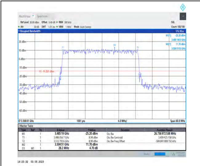
1-N78-3450-3550-PC2-30-30-M-5-DFT-256QAM-Outer_Full-75@0-Ant1-26.737-28.200-≤30-PASS
