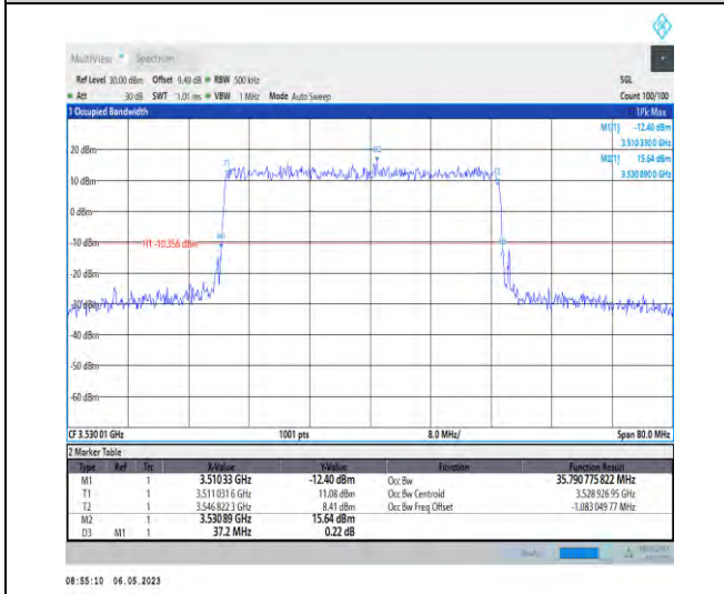
1-N78-3450-3550-PC2-30-40-H-3-DFT-16QAM-Outer_Full-100@0-Ant1-35.791-37.200-≤40-PASS
