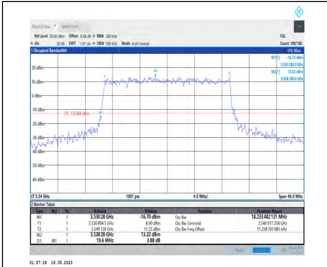
1-N78-3450-3550-PC2-30-20-H-7-CP-16QAM-Outer_Full-51@0-Ant1-18.233-19.600-≤20-PASS
