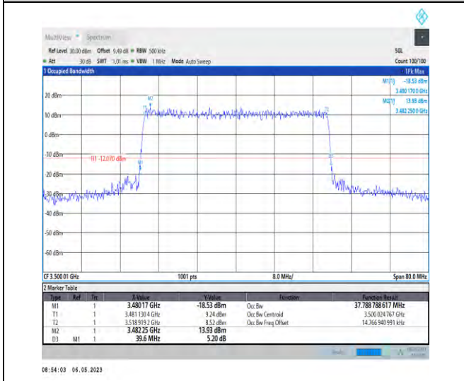
1-N78-3450-3550-PC2-30-40-M-8-CP-64QAM-Outer_Full-106@0-Ant1-37.789-39.600-≤40-PASS
