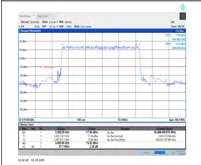
1-N78-3450-3550-PC2-30-50-L-2-DFT-PI2BPSK-Outer Full-128@0-Ant1-45.806-47.700-≤50-PASS
