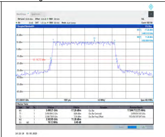
1-N78-3450-3550-PC2-30-20-M-5-DFT-256QAM-Out er_Full-50@0-Ant1-17.845-19.120-≤20-PASS
