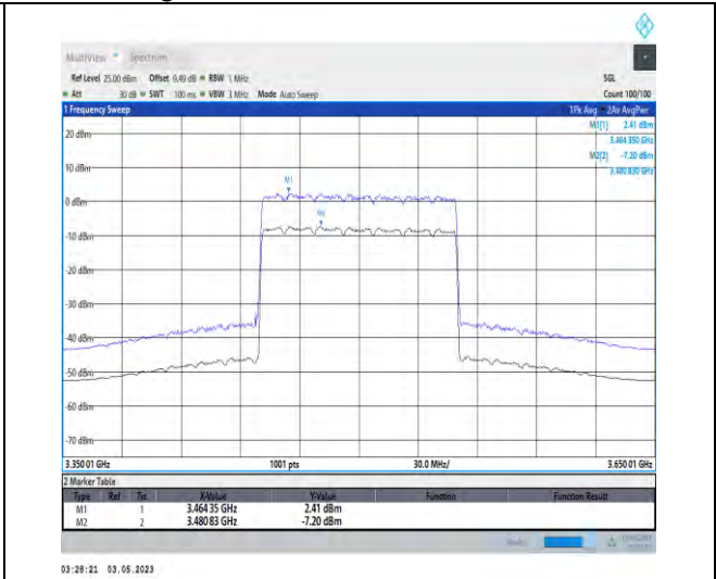
1-N78-3450-3550-PC2-30-100-H-2-CP-256QAM-Ou ter_Full-273@0-Ant1-9.61-100%-0.00-9.61-PASS-≤1
