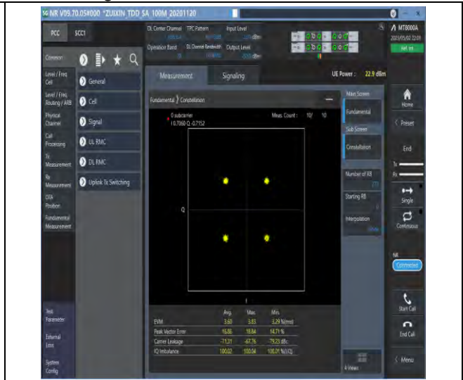
1-N78-3450-3550-PC2-30-100-M-6-CP-QPSK-Outer_Full-273@0-Ant1-see graph-PASS
