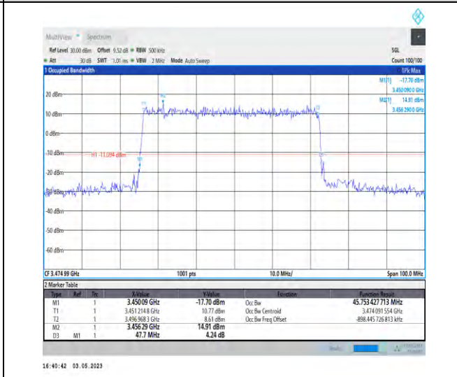
1-N78-3450-3550-PC2-30-50-L-3-DFT-16QAM-Outer Full-128@0-Ant1-45.753-47.700-≤50-PASS
