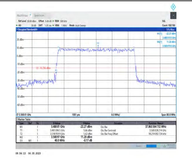
1-N78-3450-3550-PC2-30-40-M-9-CP-256QAM-Outer_Full-106@0-Ant1-37.863-40.000-≤40-PASS
