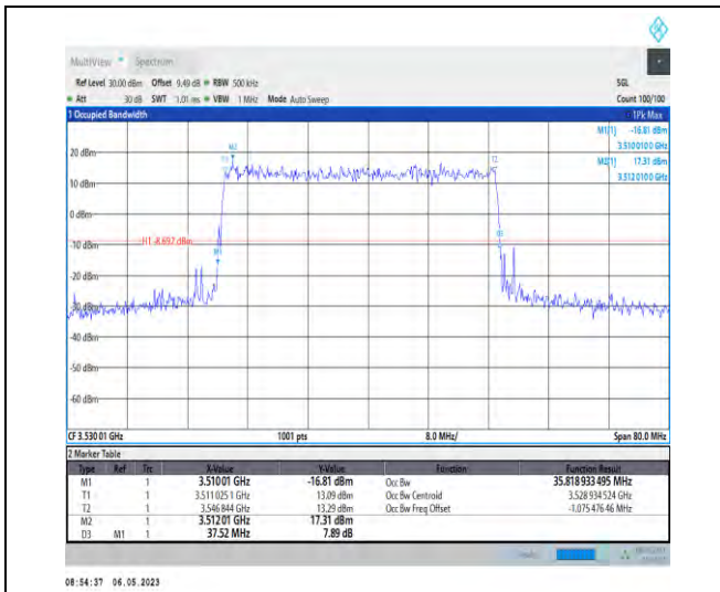
1-N78-3450-3550-PC2-30-40-H-1-DFT-QPSK-Outer_Full-100@0-Ant1-35.819-37.520-≤40-PASS
