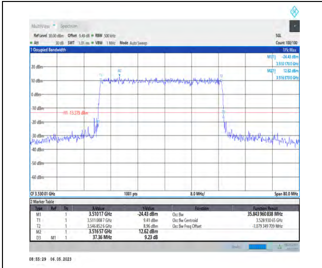
1-N78-3450-3550-PC2-30-40-H-5-DFT-256QAM-Out er_Full-100@0-Ant1-35.844-37.360-≤40-PASS
