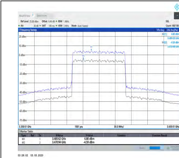
1-N78-3450-3550-PC2-30-100-H-1-DFT-256QAM-Ou ter_Full-270@0-Ant1-9.39-100%-0.00-9.39-PASS-≤1
