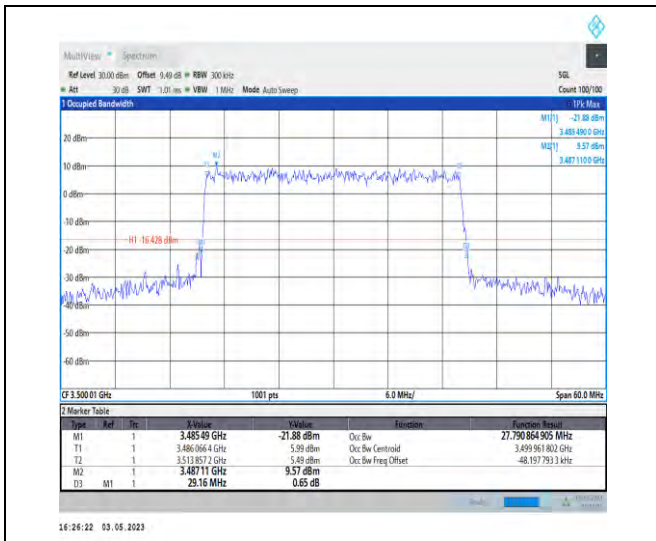
1-N78-3450-3550-PC2-30-30-M-9-CP-256QAM-Out er_Full-78@0-Ant1-27.791-29.160-≤30-PASS
