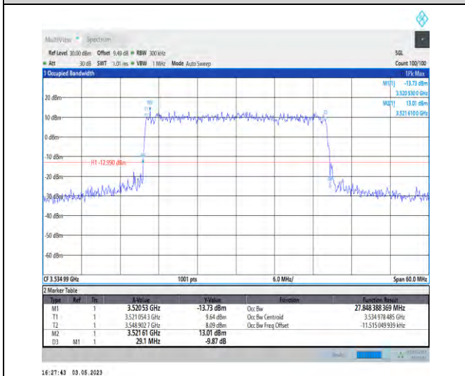
1-N78-3450-3550-PC2-30-30-H-6-CP-QPSK-Outer_Full-78@0-Ant1-27.848-29.100-≤30-PASS
