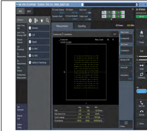
1-N78-3450-3550-PC2-30-100-M-9-CP-256QAM-Out er_Full-273@0-Ant1-see graph-PASS
