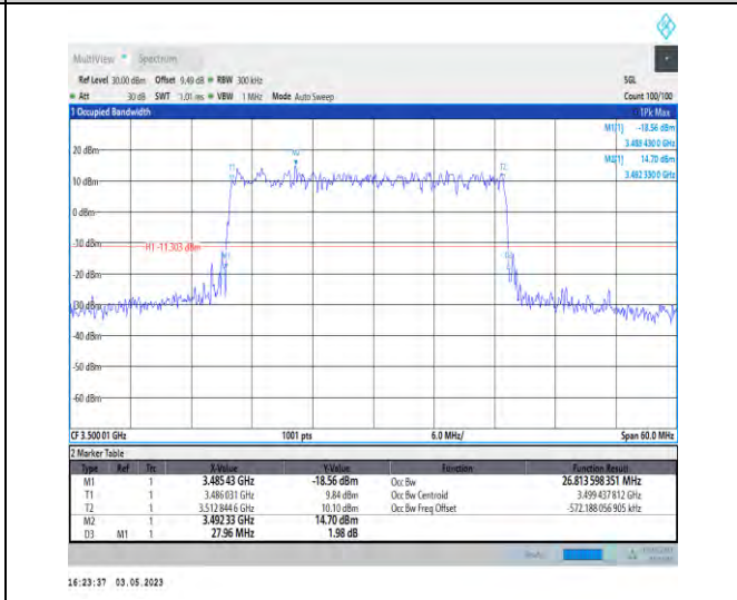
1-N78-3450-3550-PC2-30-30-M-4-DFT-64QAM-Outer_Full-75@0-Ant1-26.814-27.960-≤30-PASS
