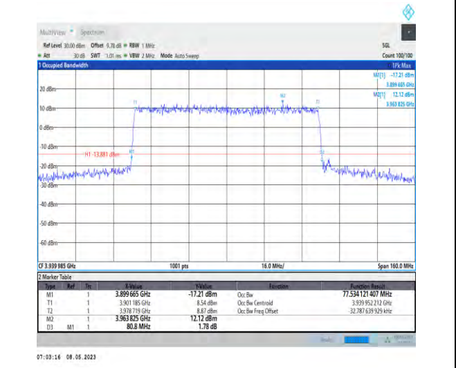
1-N77-3700-3980-PC2-30-80-H-6-CP-QPSK-Out er_Full-217@0-Ant1-77.534-80.800-≤80-PASS
