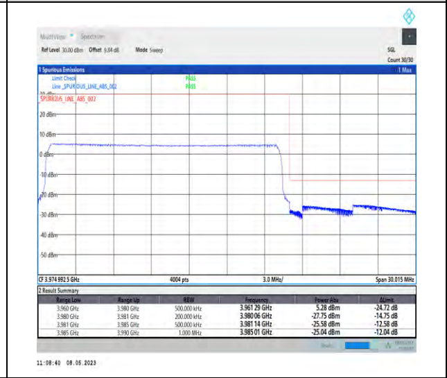
1-N77-3700-3980-PC2-30-20-H-6-CP-QPSK-Outer_Full-51@0-Ant1-1--PASS-see graph
