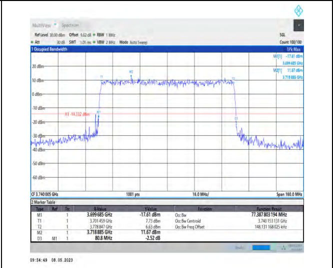
1-N77-3700-3980-PC2-30-80-L-8-CP-64QAM-Outer_Full-217@0-Ant1-77.388-80.800-≤80-PASS
