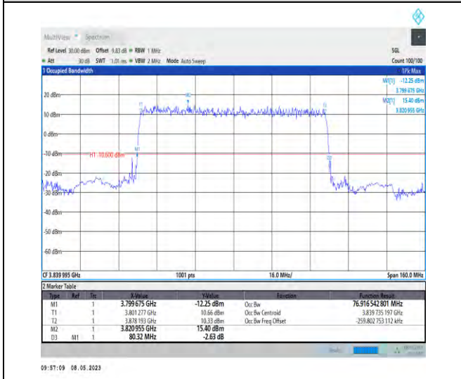
1-N77-3700-3980-PC2-30-80-M-2-DFT-PI2BPSK-Outer_Full-216@0-Ant1-76.917-80.320-≤80-PASS
