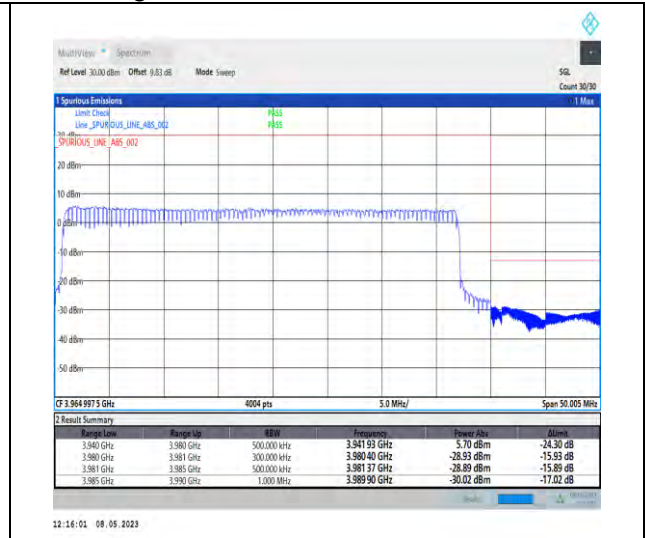
1-N77-3700-3980-PC2-30-40-H-3-DFT-PI2BPSK-Outer_Full-100@0-Ant1-1--PASS-see graph
