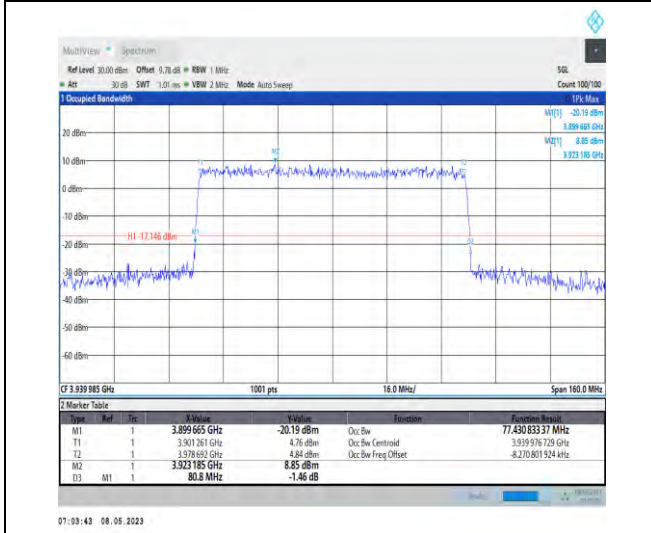
1-N77-3700-3980-PC2-30-80-H-9-CP-256QAM-Outer_Full-217@0-Ant1-77.431-80.800-≤80-PASS
