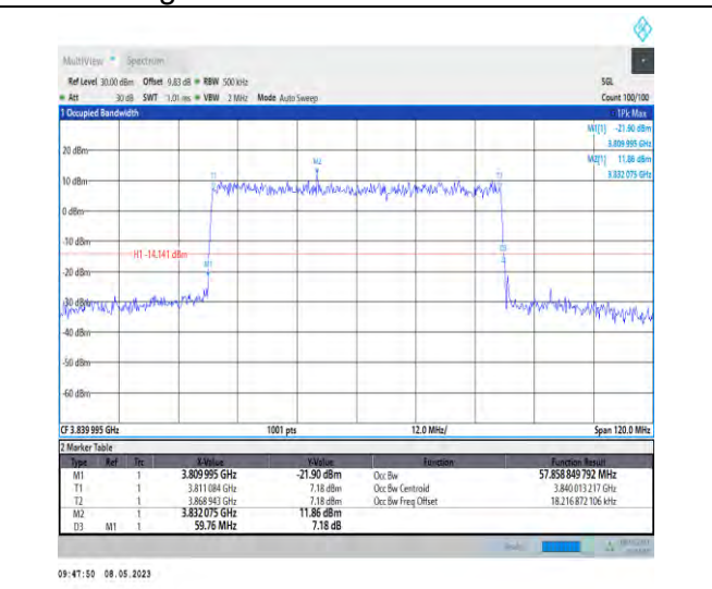
1-N77-3700-3980-PC2-30-60-M-4-DFT-64QAM-Out er_Full-162@0-Ant1-57.859-59.760-≤60-PASS
