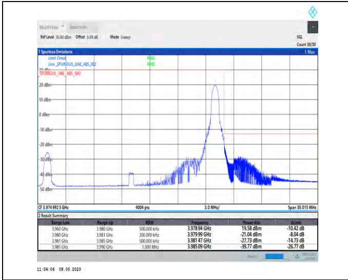
1-N77-3700-3980-PC2-30-20-H-2-DFT-PI2BPSK-Edge_1RB_Right-1@50-Ant1-1--PASS-see graph
