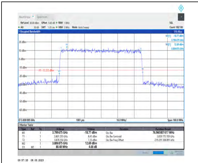
1-N77-3700-3980-PC2-30-80-M-4-DFT-64QAM-Out_er_Full-216@0-Ant1-76.961-80.480-≤80-PASS
