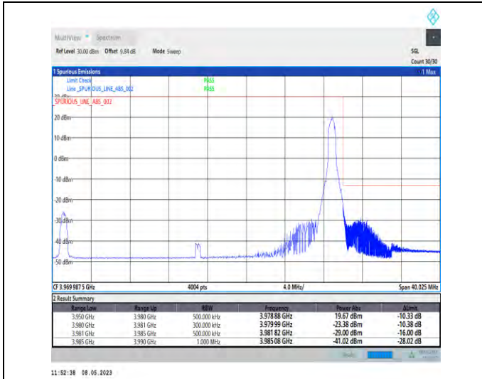
1-N77-3700-3980-PC2-30-30-H-2-DFT-PI2BPSK-Edge_1RB_Right-1@77-Ant1-1--PASS-see graph
