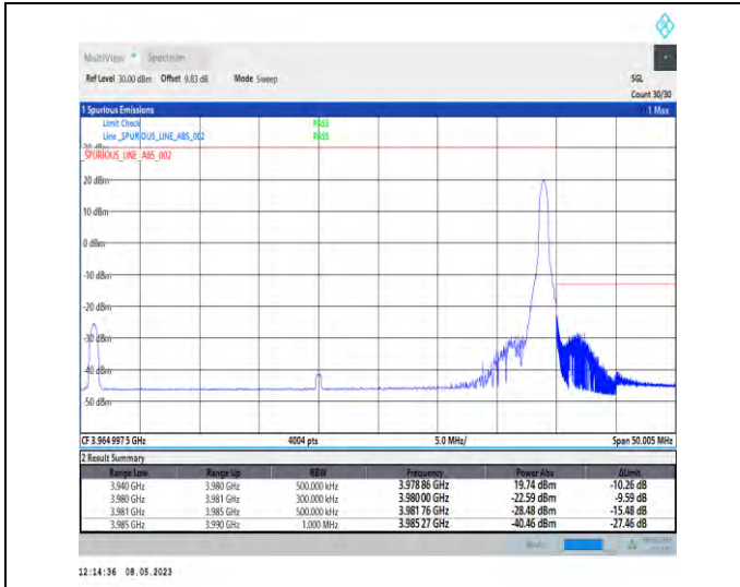
1-N77-3700-3980-PC2-30-40-H-2-DFT-PI2BPSK-Edge_1RB_Right-1@105-Ant1-1--PASS-see graph
