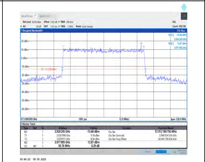
1-N77-3700-3980-PC2-30-60-H-1-DFT-QPSK-Outer_Full-162@0-Ant1-57.912-59.760-≤60-PASS
