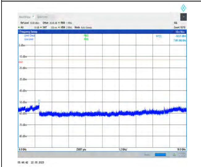
1-N77-3700-3980-PC2-30-100-M-1-DFT-PI2BPSK- Inner_1RB_Left-1@1-6000-18000-Ant1-7430.40--52. 21--13-PASS
