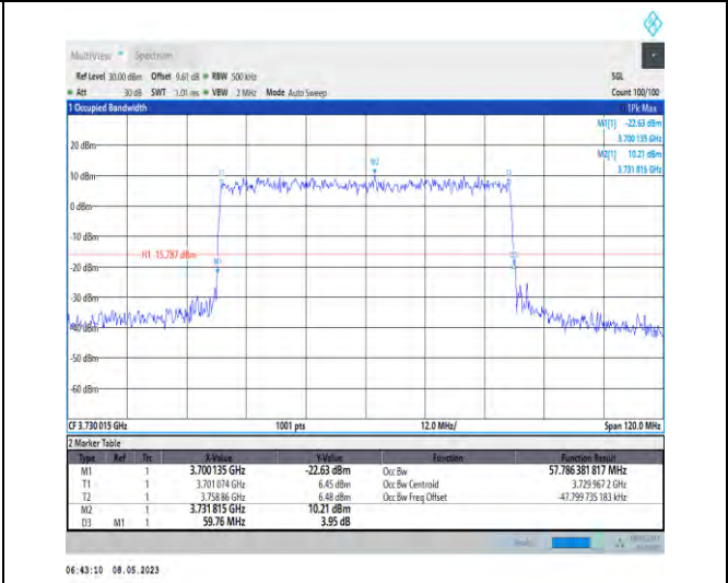
1-N77-3700-3980-PC2-30-60-L-7-CP-16QAM-Outer_Full-162@0-Ant1-57.786-59.760-≤60-PASS
