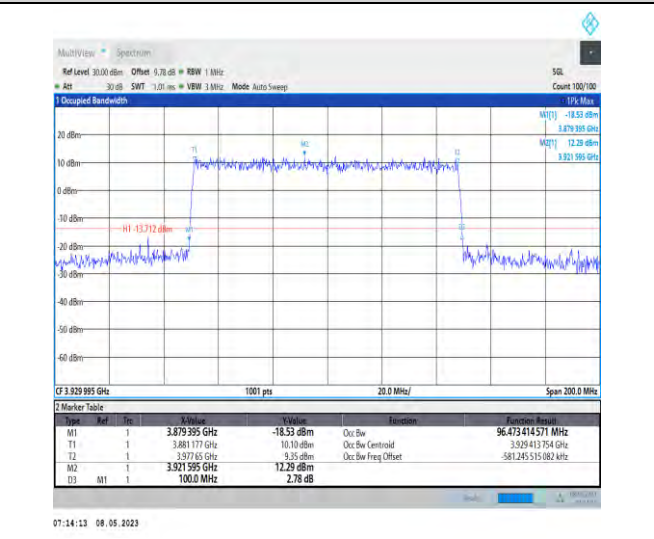
1-N77-3700-3980-PC2-30-100-H-3-DFT-16QAM-Outer_Full-270@0-Ant1-96.473-100.000-≤100-PASS
