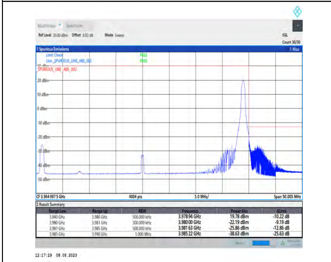
1-N77-3700-3980-PC2-30-40-H-5-CP-QPSK-Edge_1RB_Right-1@105-Ant1-1--PASS-see graph
