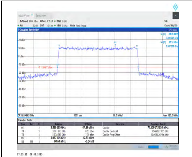
1-N77-3700-3980-PC2-30-80-H-7-CP-16QAM-Outer_Full-217@0-Ant1-77.51-80.640-≤80-PASS
