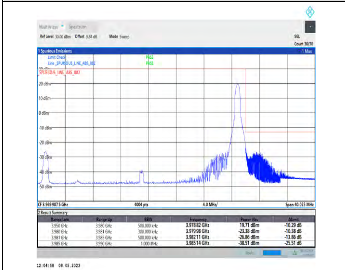
1-N77-3700-3980-PC2-30-30-H-5-CP-QPSK-Edge_1RB_Right-1@77-Ant1-1--PASS-see graph
