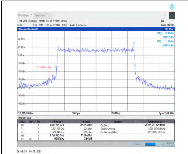
1-N77-3700-3980-PC2-30-60-L-8-CP-64QAM-Outer _Full-162@0-Ant1-57.786-60.000-≤60-PASS
