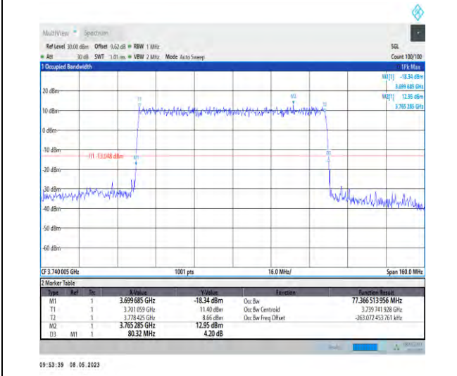
1-N77-3700-3980-PC2-30-80-L-3-DFT-16QAM-Outer_Full-216@0-Ant1-77.367-80.320-≤80-PASS
