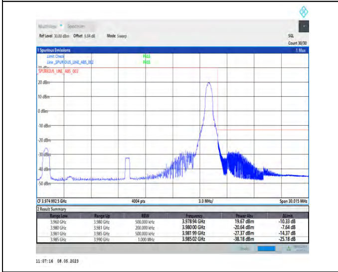
1-N77-3700-3980-PC2-30-20-H-5-CP-QPSK-Edge_1RB_Right-1@50-Ant1-1--PASS-see graph
