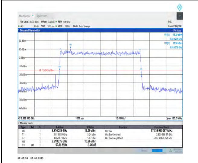
1-N77-3700-3980-PC2-30-60-M-5-DFT-256QAM-Out er_Full-162@0-Ant1-57.814-59.640-≤60-PASS
