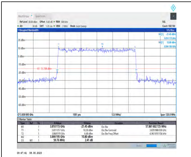
1-N77-3700-3980-PC2-30-60-M-3-DFT-16QAM-Out er_Full-162@0-Ant1-57.862-59.760-≤60-PASS
