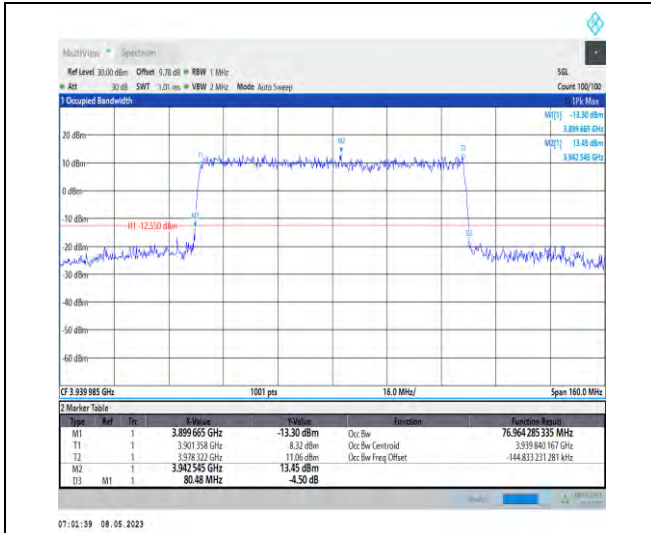
1-N77-3700-3980-PC2-30-80-H-3-DFT-16QAM-Out er_Full-216@0-Ant1-76.964-80.480-≤80-PASS
