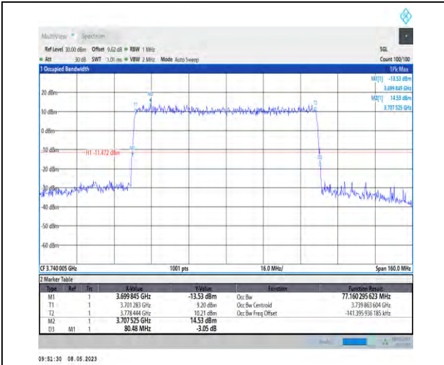
1-N77-3700-3980-PC2-30-80-L-1-DFT-QPSK-Outer_Full-216@0-Ant1-77.16-80.480-≤80-PASS
