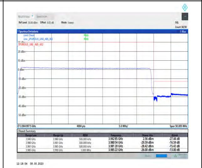
1-N77-3700-3980-PC2-30-40-H-6-CP-QPSK-Outer_Full-106@0-Ant1-1--PASS-see graph
