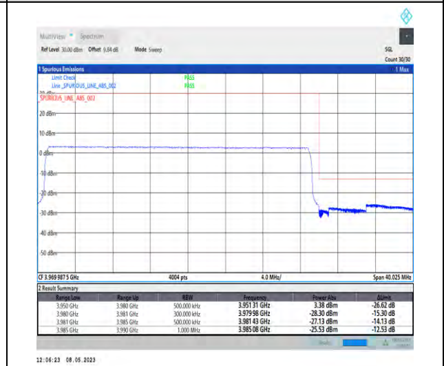
1-N77-3700-3980-PC2-30-30-H-6-CP-QPSK-Outer_Full-78@0-Ant1-1--PASS-see graph
