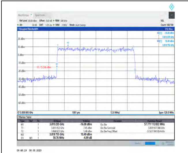
1-N77-3700-3980-PC2-30-60-M-7-CP-16QAM-Outer_Full-162@0-Ant1-57.771-59.760-≤60-PASS
