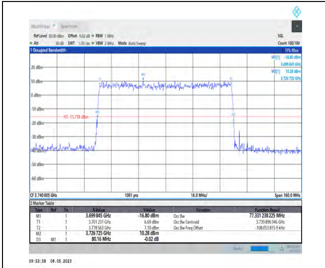
1-N77-3700-3980-PC2-30-80-L-5-DFT-256QAM-Out_er_Full-216@0-Ant1-77.331-80.160-≤80-PASS
