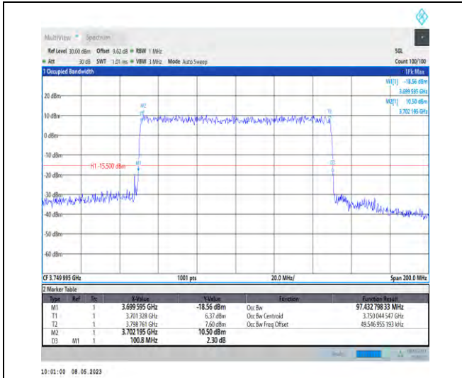
1-N77-3700-3980-PC2-30-100-L-6-CP-QPSK-Outer_Full-273@0-Ant1-97.433-100.800-≤100-PASS
