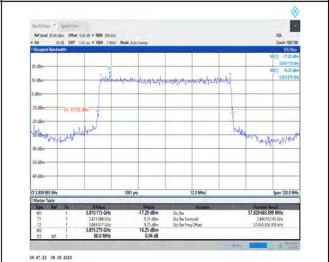
1-N77-3700-3980-PC2-30-60-M-2-DFT-PI2BPSK-Outer _Full-162@0-Ant1-57.93-60.000-≤60-PASS
