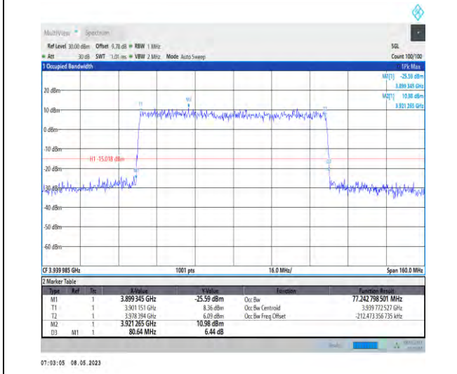
1-N77-3700-3980-PC2-30-80-H-5-DFT-256QAM-Out er_Full-216@0-Ant1-77.243-80.640-≤80-PASS
