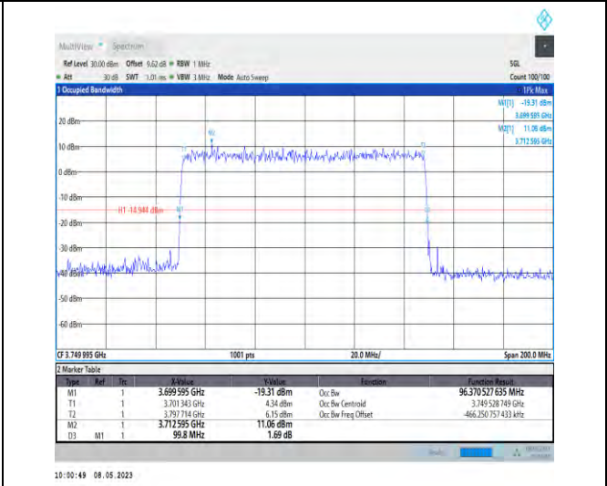
1-N77-3700-3980-PC2-30-100-L-5-DFT-256QAM-Outer_Full-270@0-Ant1-96.371-99.800-≤100-PASS
