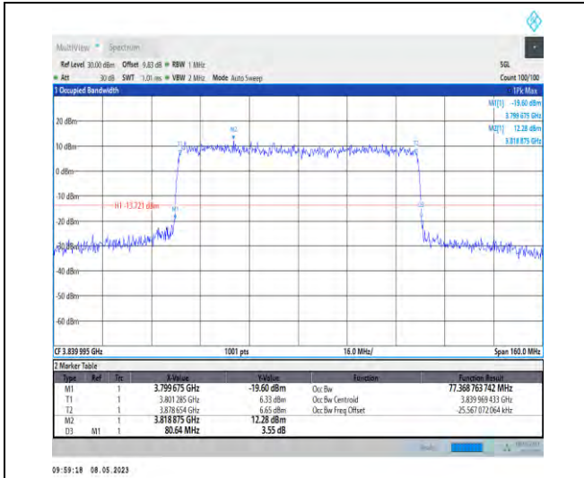
1-N77-3700-3980-PC2-30-80-M-8-CP-64QAM-Outer_Full-217@0-Ant1-77.369-80.640-≤80-PASS
