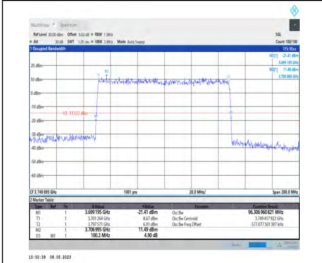
1-N77-3700-3980-PC2-30-100-L-4-DFT-64QAM-Outer_Full-270@0-Ant1-96.307-100.200-≤100-PASS
