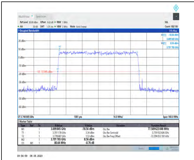
1-N77-3700-3980-PC2-30-80-L-9-CP-256QAM-Outer_Full-217@0-Ant1-77.51-80.640-≤80-PASS
