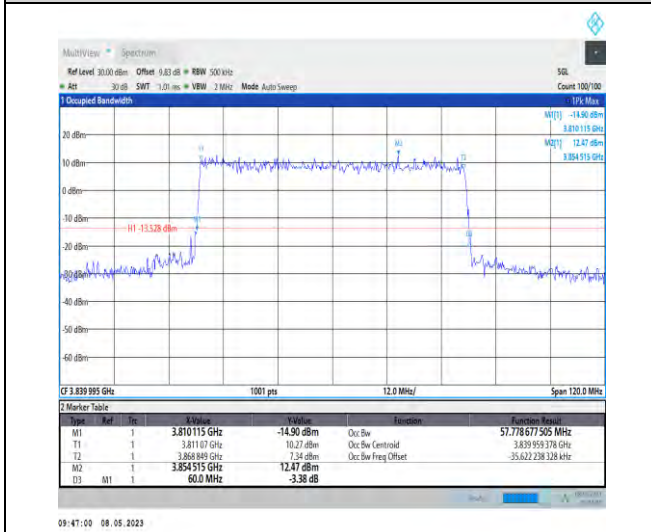
1-N77-3700-3980-PC2-30-60-M-1-DFT-QPSK-Outer _Full-162@0-Ant1-57.779-60.000-≤60-PASS
