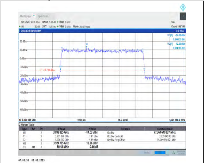
1-N77-3700-3980-PC2-30-80-H-8-CP-64QAM-Outer_Full-217@0-Ant1-77.365-80.480-≤80-PASS
