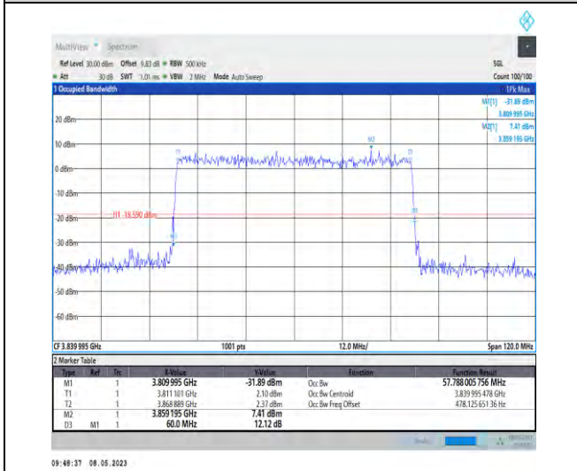
1-N77-3700-3980-PC2-30-60-M-9-CP-256QAM-Outer_Full-162@0-Ant1-57.788-60.000-≤60-PASS
