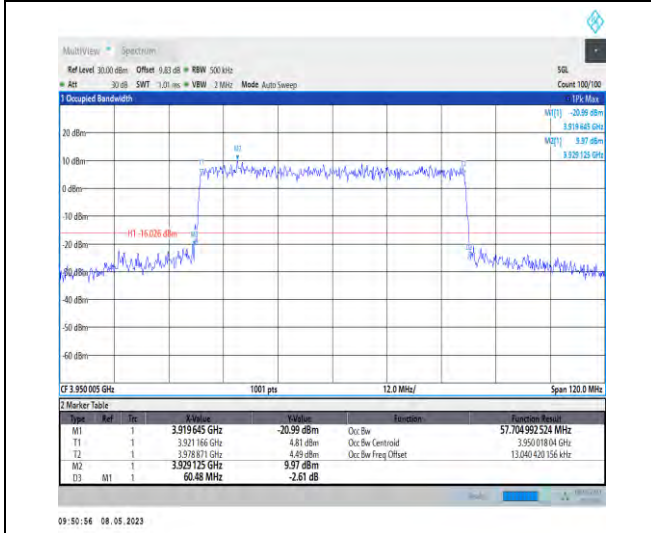
1-N77-3700-3980-PC2-30-60-H-8-CP-64QAM-Outer_Full-162@0-Ant1-57.705-60.480-≤60-PASS
