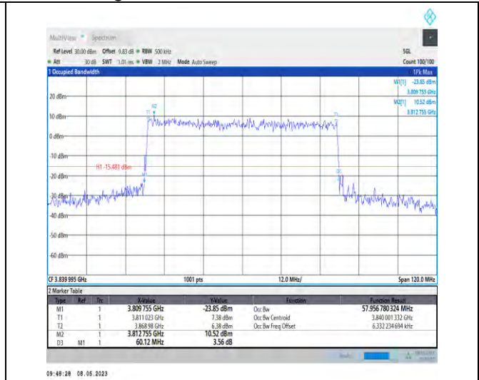
1-N77-3700-3980-PC2-30-60-M-8-CP-64QAM-Outer_Full-162@0-Ant1-57.957-60.120-≤60-PASS
