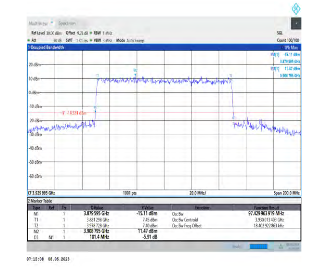
1-N77-3700-3980-PC2-30-100-H-7-CP-16QAM-Outer_Full-273@0-Ant1-97.43-101.400-≤100-PASS
