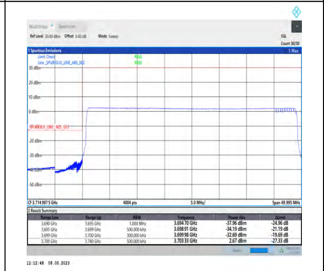
1-N77-3700-3980-PC2-30-40-L-6-CP-QPSK-Outer_Full-106@0-Ant1-1--PASS-see graph
