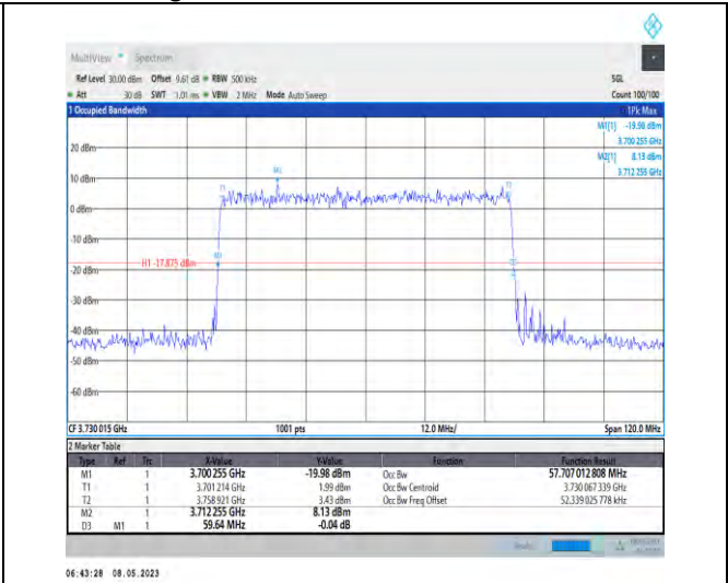
1-N77-3700-3980-PC2-30-60-L-9-CP-256QAM-Outer _Full-162@0-Ant1-57.707-59.640-≤60-PASS
