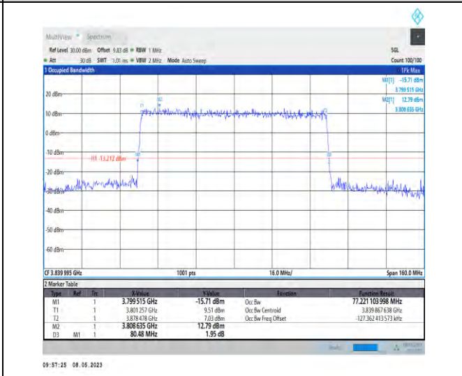
1-N77-3700-3980-PC2-30-80-M-3-DFT-16QAM-Outer_Full-216@0-Ant1-77.221-80.480-≤80-PASS
