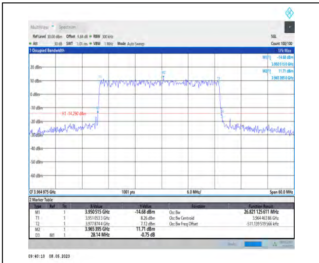
1-N77-3700-3980-PC2-30-30-H-4-DFT-64QAM-Out er_Full-75@0-Ant1-26.821-28.140-≤30-PASS
