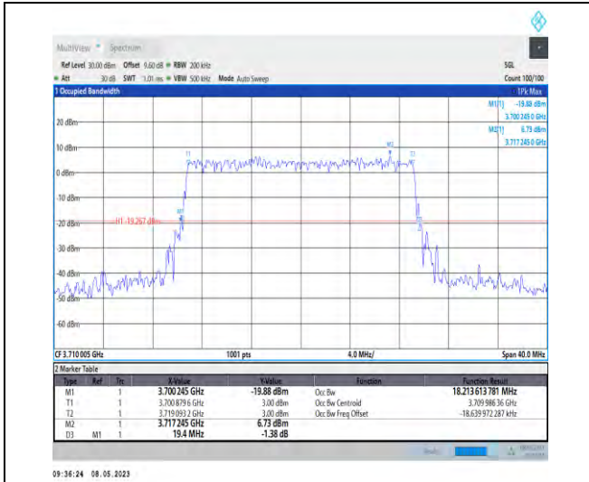
1-N77-3700-3980-PC2-30-20-L-9-CP-256QAM-Outer_Full-51@0-Ant1-18.214-19.400-≤20-PASS
