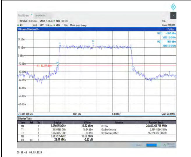
1-N77-3700-3980-PC2-30-30-H-2-DFT-PI2BPSK-Outer Full-75@0-Ant1-26.849-28.440-≤30-PASS
