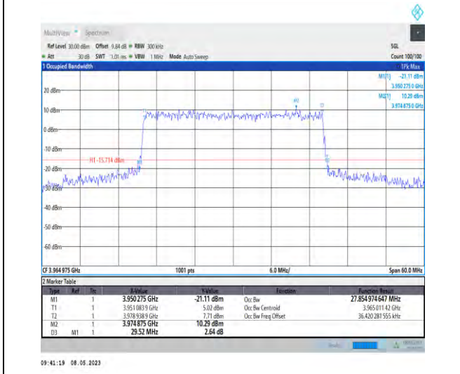
1-N77-3700-3980-PC2-30-30-H-6-CP-QPSK-Outer_Full-78@0-Ant1-27.855-29.520-≤30-PASS
