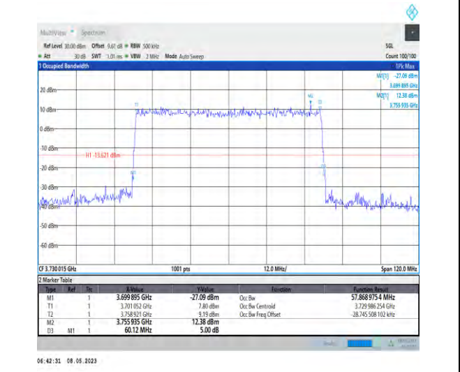
1-N77-3700-3980-PC2-30-60-L-3-DFT-16QAM-Outer_Full-162@0-Ant1-57.869-60.120-≤60-PASS
