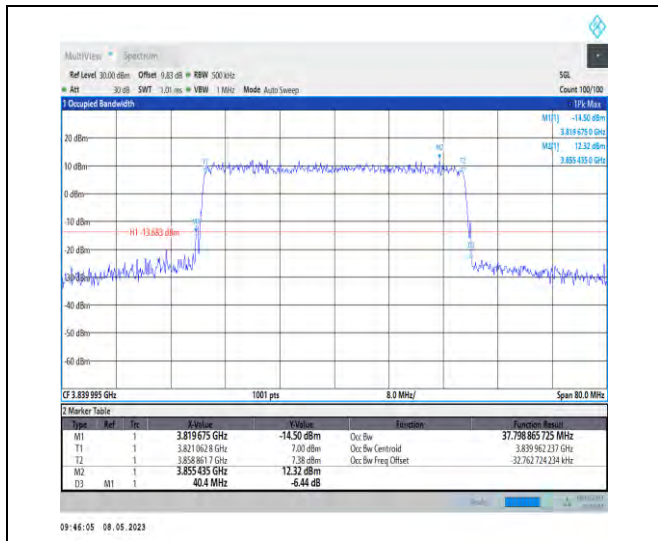
1-N77-3700-3980-PC2-30-40-M-6-CP-QPSK-Outer_Full-106@0-Ant1-37.799-40.400-≤40-PASS
