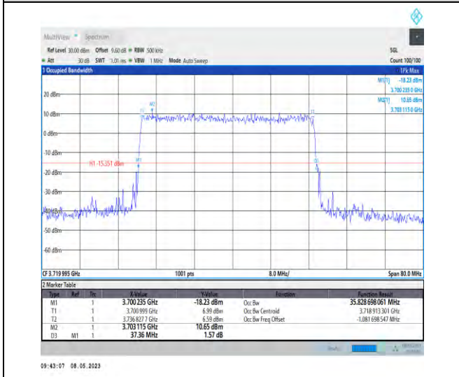
1-N77-3700-3980-PC2-30-40-L-5-DFT-256QAM-Outer_Full-100@0-Ant1-35.829-37.360-≤40-PASS
