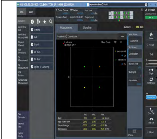
1-N77-3700-3980-PC2-30-100-M-1-DFT-PI2BPSK-Outer_Full-270@0-Ant1-see graph-PASS
