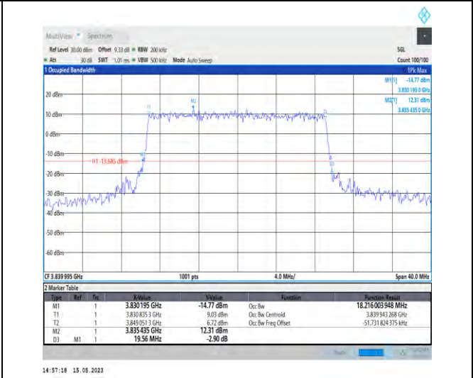
1-N77-3700-3980-PC2-30-20-H-6-CP-QPSK-Outer_Full-51@0-Ant1-18.216-19.560-≤20-PASS
