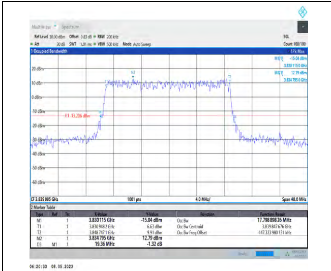
1-N77-3700-3980-PC2-30-20-M-4-DFT-64QAM-Out_er_Full-50@0-Ant1-17.799-19.360-≤20-PASS
