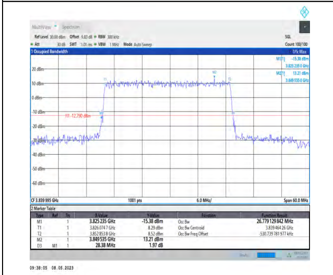
1-N77-3700-3980-PC2-30-30-M-3-DFT-16QAM-Outer_Full-75@0-Ant1-26.779-28.380-≤30-PASS
