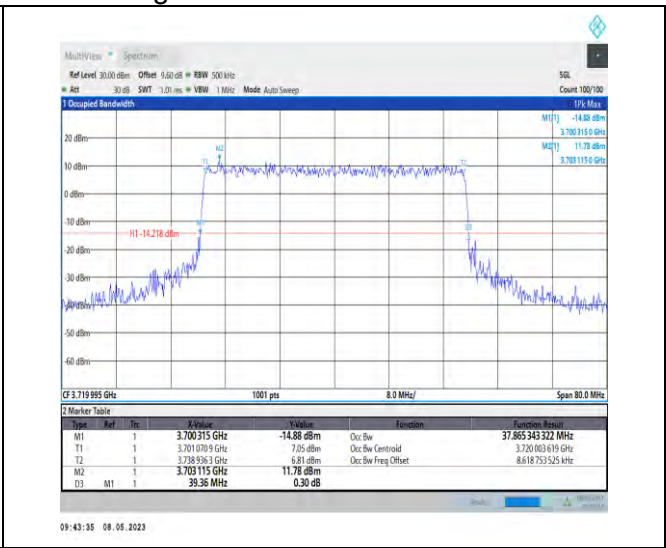
1-N77-3700-3980-PC2-30-40-L-8-CP-64QAM-Outer_Full-106@0-Ant1-37.865-39.360-≤40-PASS
