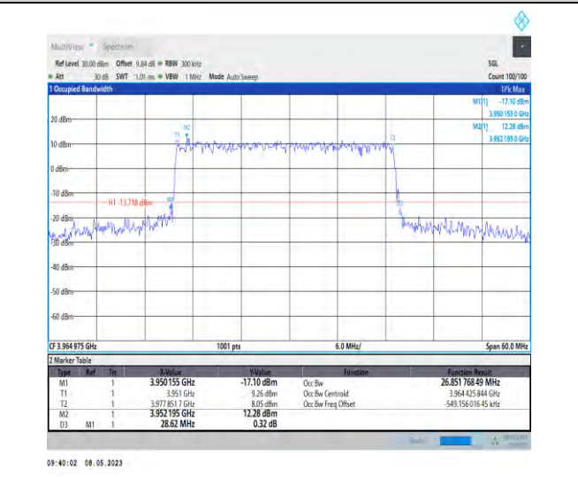
1-N77-3700-3980-PC2-30-30-H-3-DFT-16QAM-Outer Full-75@0-Ant1-26.852-28.620-≤30-PASS
