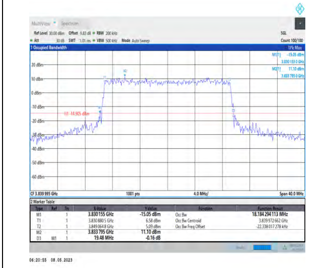
1-N77-3700-3980-PC2-30-20-M-6-CP-QPSK-Outer_Full-51@0-Ant1-18.184-19.480-≤20-PASS
