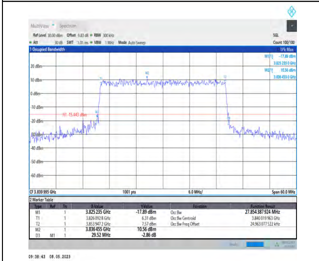
1-N77-3700-3980-PC2-30-30-M-7-CP-16QAM-Outer_Full-78@0-Ant1-27.854-29.520-≤30-PASS
