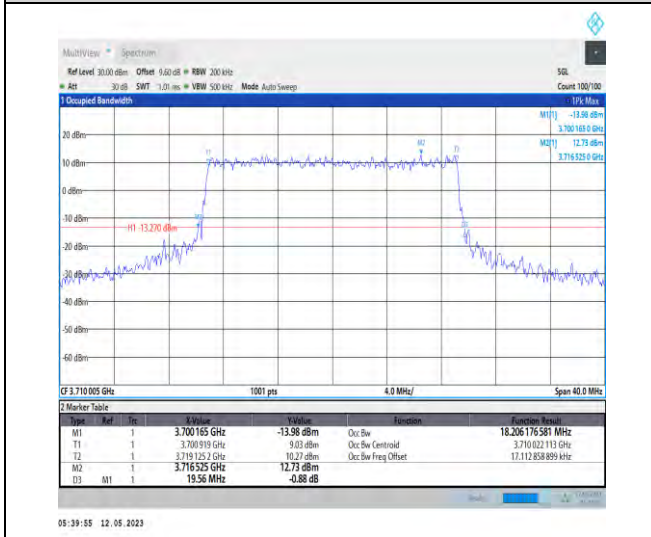
1-N77-3700-3980-PC2-30-20-L-7-CP-16QAM-Outer_Full-51@0-Ant1-18.206-19.560-≤20-PASS
