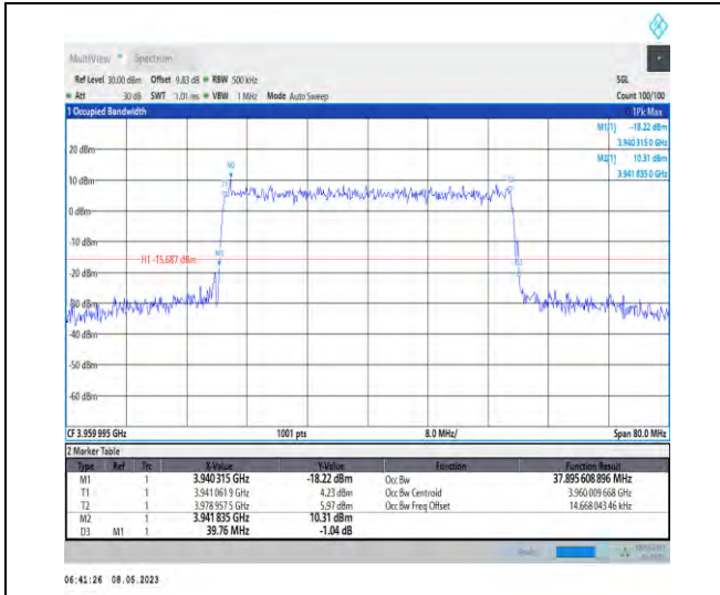
1-N77-3700-3980-PC2-30-40-H-9-CP-256QAM-Out er_Full-106@0-Ant1-37.896-39.760-≤40-PASS
