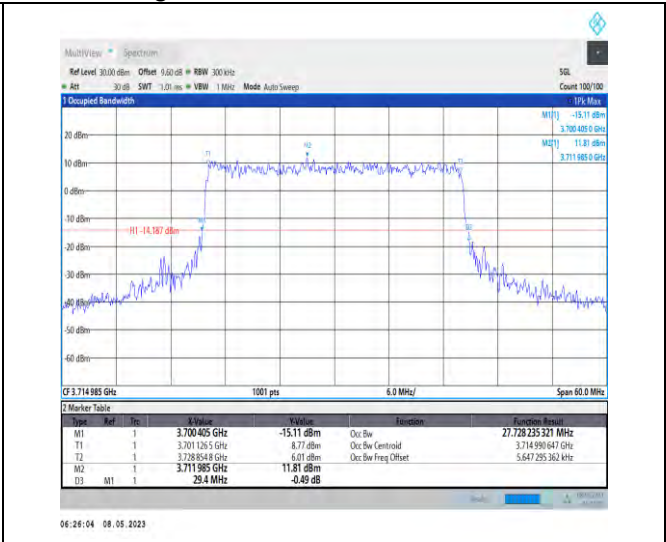
1-N77-3700-3980-PC2-30-30-L-7-CP-16QAM-Outer_Full-78@0-Ant1-27.728-29.400-≤30-PASS
