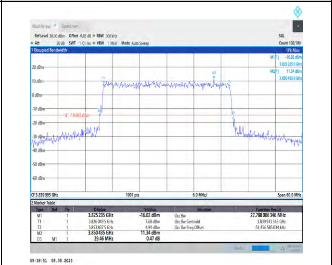
1-N77-3700-3980-PC2-30-30-M-8-CP-64QAM-Outer_Full-78@0-Ant1-27.788-29.460-≤30-PASS
