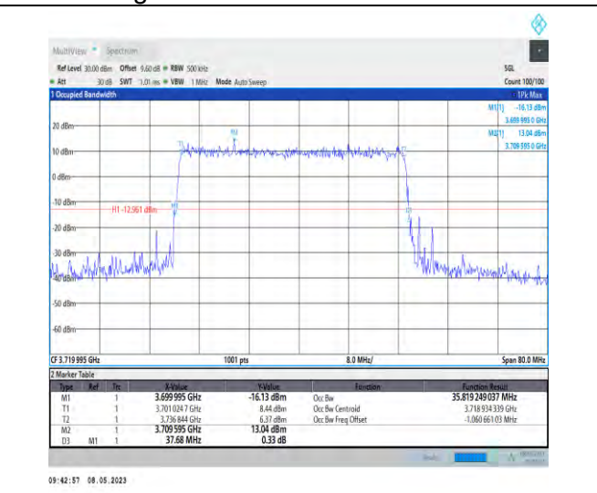
1-N77-3700-3980-PC2-30-40-L-4-DFT-64QAM-Outer_Full-100@0-Ant1-35.819-37.680-≤40-PASS
