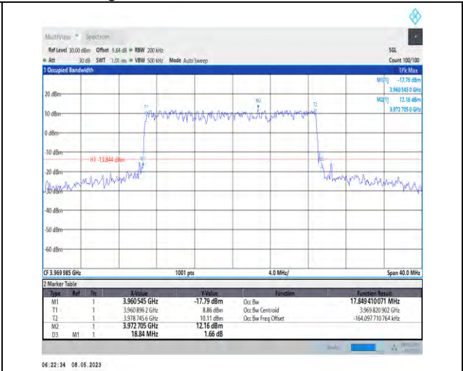
1-N77-3700-3980-PC2-30-20-H-4-DFT-64QAM-Outer_Full-50@0-Ant1-17.849-18.840-≤20-PASS
