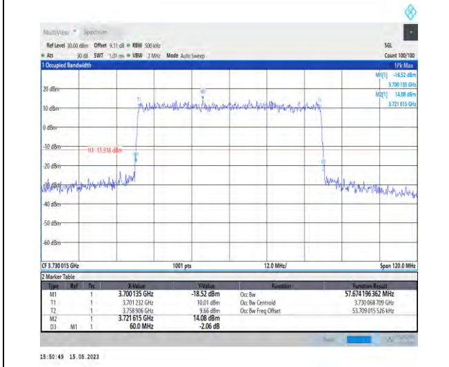
1-N77-3700-3980-PC2-30-60-L-2-DFT-PI2BPSK-Outer_Full-162@0-Ant1-57.674-60.000-≤60-PASS
