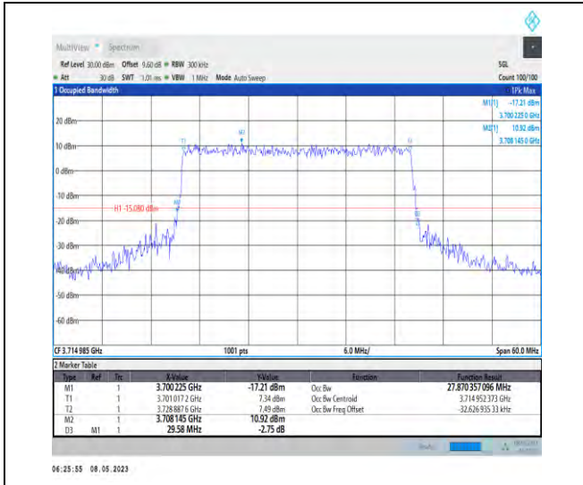
1-N77-3700-3980-PC2-30-30-L-6-CP-QPSK-Outer_Full-78@0-Ant1-27.87-29.580-≤30-PASS
