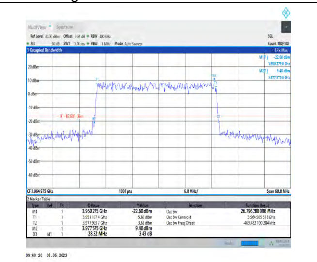
1-N77-3700-3980-PC2-30-30-H-5-DFT-256QAM-Out er_Full-75@0-Ant1-26.796-28.320-≤30-PASS
