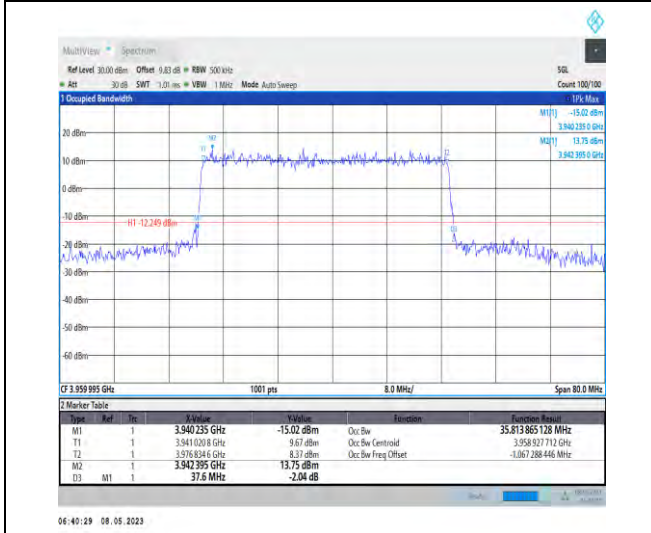
1-N77-3700-3980-PC2-30-40-H-3-DFT-16QAM-Outer_Full-100@0-Ant1-35.814-37.600-≤40-PASS
