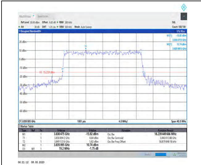
1-N77-3700-3980-PC2-30-20-M-8-CP-64QAM-Outer_Full-51@0-Ant1-18.239-19.200-≤20-PASS
