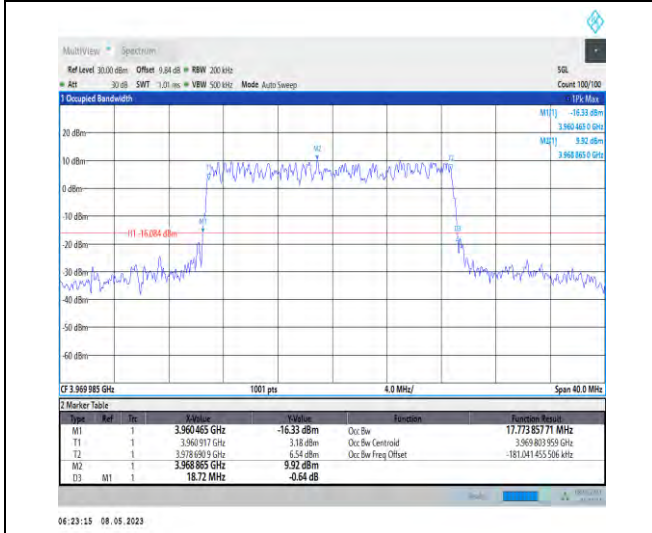
1-N77-3700-3980-PC2-30-20-H-5-DFT-256QAM-Outer_Full-50@0-Ant1-17.774-18.720-≤20-PASS
