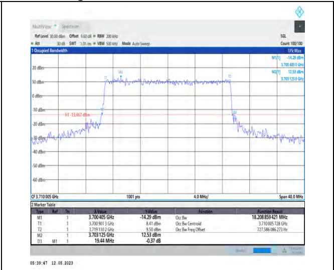
1-N77-3700-3980-PC2-30-20-L-6-CP-QPSK-Outer_Full-51@0-Ant1-18.209-19.440-≤20-PASS
