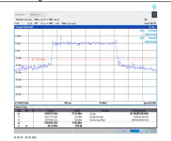
1-N77-3700-3980-PC2-30-30-H-1-DFT-QPSK-Outer Full-75@0-Ant1-26.707-28.140-≤30-PASS
