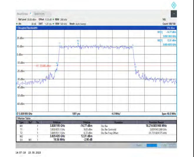
1-N77-3700-3980-PC2-30-20-M-7-CP-16QAM-Outer_Full-51@0-Ant1-18.216-19.560-≤20-PASS
