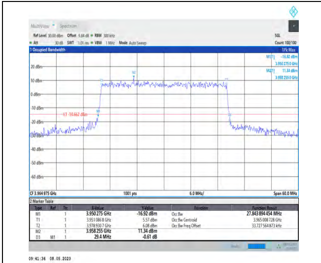
1-N77-3700-3980-PC2-30-30-H-8-CP-64QAM-Outer_Full-78@0-Ant1-27.844-29.400-≤30-PASS
