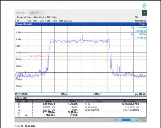
1-N77-3700-3980-PC2-30-30-L-5-DFT-256QAM-Outer_Full-75@0-Ant1-26.709-28.680-≤30-PASS
