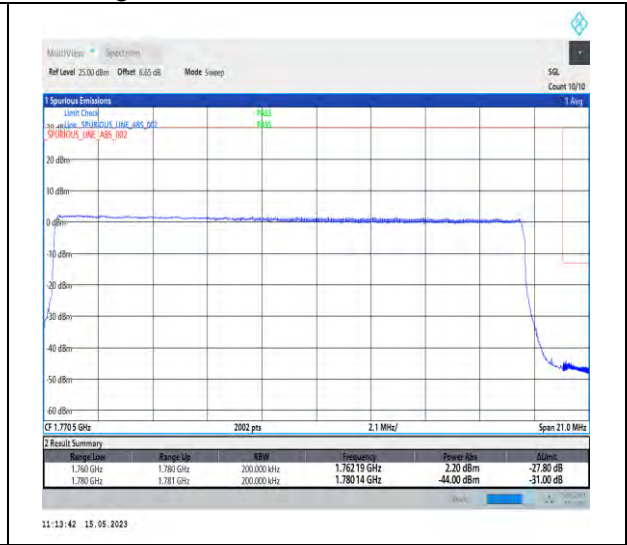
1-DC_5A_n66A-PC3-15-5+20-M+H-3-QPSK-Outer_Full-Outer_Full@N/A-DFT-PI2BPSK-Outer_Full-100@0-1-seegraph-PASS-see graph
