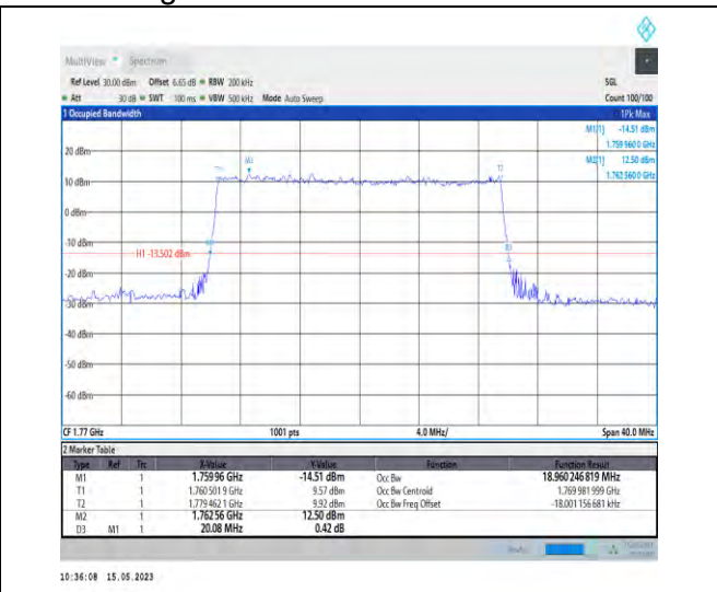
1-DC_5A_n66A-PC3-15-5+20-M+H-7-N/A-N/A-N/A-CP-16QAM-Outer_Full-106@0-Ant1-18.96-20.080-≤20-PASS
