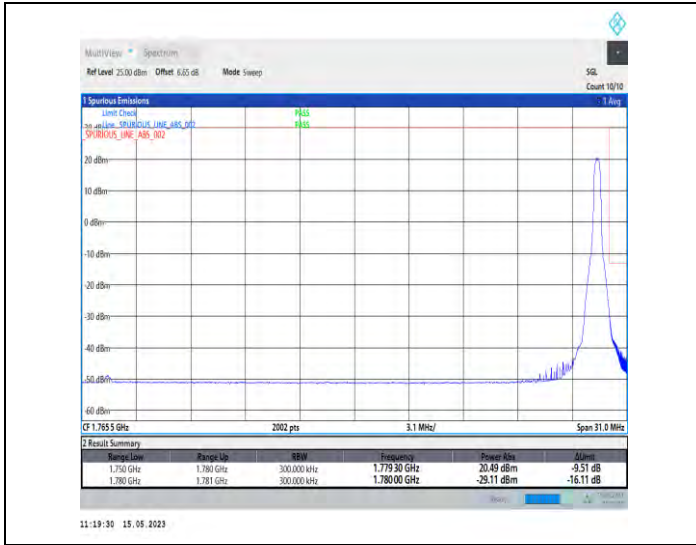
1-DC_5A_n66A-PC3-15-5+30-M+H-2-QPSK-Edge_1RB_Right-Edge_1_Right@N/A-DFT-PI2BPSK-Edge_1RB_Right-1@159-1-seegraph-PASS-see graph
