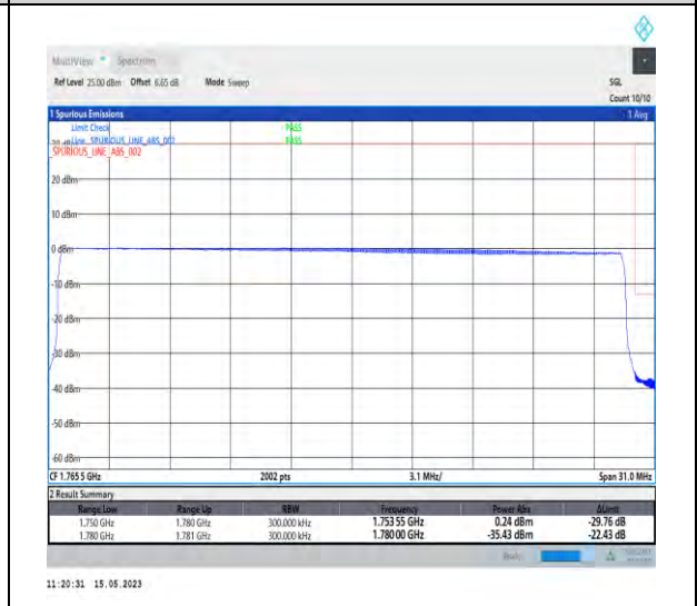
1-DC_5A_n66A-PC3-15-5+30-M+H-6-QPSK-Outer_Full-Outer_Full@N/A-CP-QPSK-Outer_Full-160@0-1-seegraph-PASS-see graph
