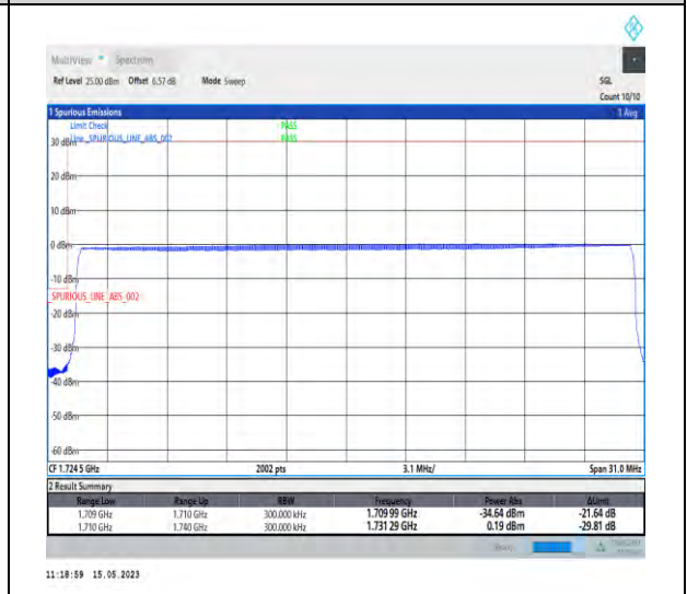
1-DC_5A_n66A-PC3-15-5+30-M+L-6-QPSK-Outer_Full-Outer_Full@N/A-CP-QPSK-Outer_Full-160@0-1-seegraph-PASS-see graph
