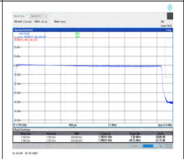
1-DC_5A_n66A-PC3-15-5+20-M+H-6-QPSK-Outer_Full-Outer_Full@N/A-CP-QPSK-Outer_Full-106@0-1-seegraph-PASS-see graph
