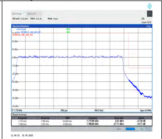
1-DC_5A_n66A-PC3-15-5+5-M+H-3-QPSK-Outer_Full-Outer_Full@N/A-DFT-PI2BPSK-Outer_Full-25@0-1-seegraph-PASS-see graph
