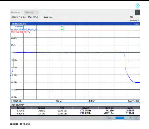
1-DC_5A_n66A-PC3-15-5+10-M+H-6-QPSK-Outer_Full-Outer_Full@N/A-CP-QPSK-Outer_Full-52@0-1-seegraph-PASS-see graph
