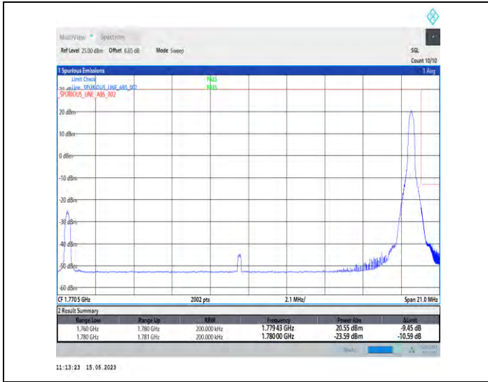
1-DC_5A_n66A-PC3-15-5+20-M+H-2-QPSK-Edge_1RB_Right-Edge_1_Right@N/A-DFT-PI2BPSK-Edge_1RB_Right-1@105-1-seegraph-PASS-see graph
