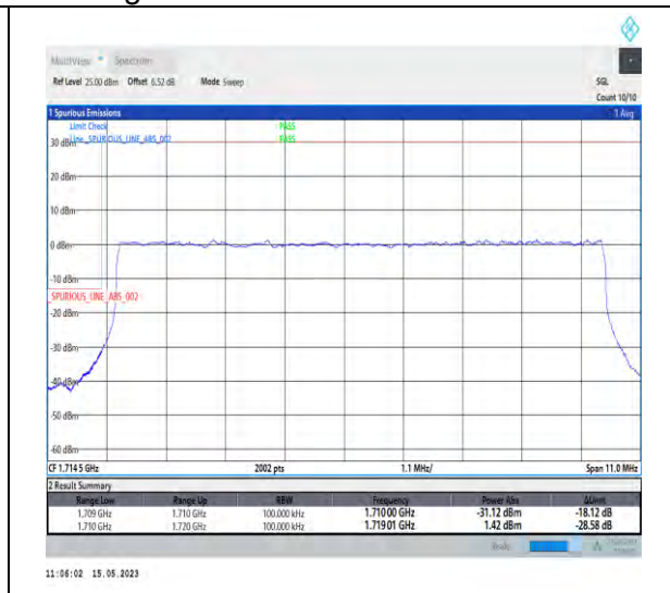
1-DC_5A_n66A-PC3-15-5+10-M+L-3-QPSK-Outer_Full-Outer_Full@N/A-DFT-PI2BPSK-Outer_Full-50@0-1-seegraph-PASS-see graph
