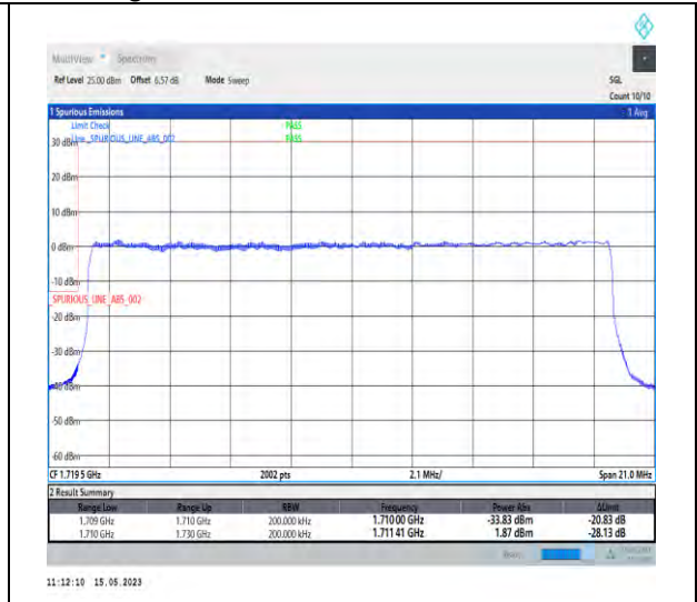
1-DC_5A_n66A-PC3-15-5+20-M+L-3-QPSK-Outer_Full-Outer_Full@N/A-DFT-PI2BPSK-Outer_Full-100@0-1-seegraph-PASS-see graph
