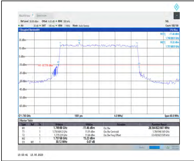
1-DC_5A_n66A-PC3-15-5+30-M+H-2-N/A-N/A-N/A-DFT-PI2BPSK-Outer_Full-160@0-Ant1-28.565-30.1 20-<=30-PASS
