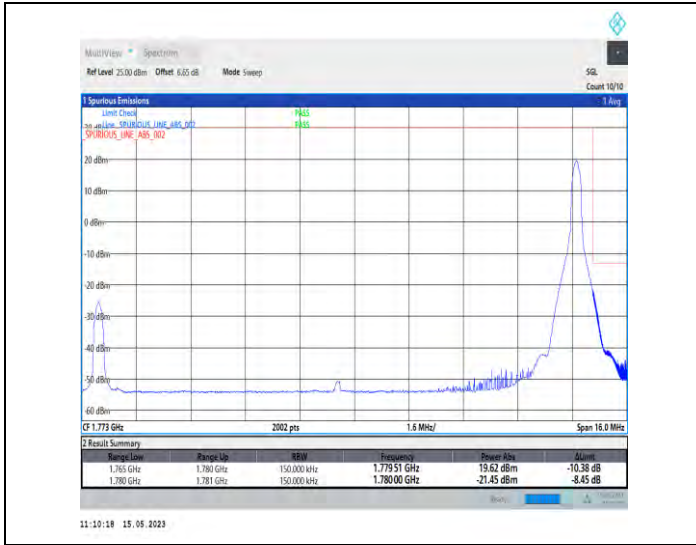
1-DC_5A_n66A-PC3-15-5+15-M+H-2-QPSK-Edge_1RB_Right-Edge_1_Right@N/A-DFT-PI2BPSK-Edge_1RB_Right-1@78-1-seegraph-PASS-see graph
