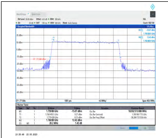
1-DC_5A_n66A-PC3-15-5+20-M+H-6-N/A-N/A-N/A-CP-QPSK-Outer_Full-106@0-Ant1-18.933-20.200-≤20-PASS
