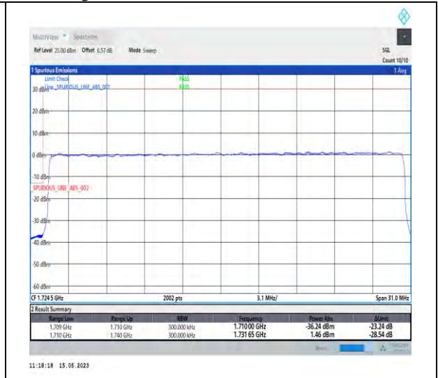
1-DC_5A_n66A-PC3-15-5+30-M+L-3-QPSK-Outer_Full-Outer_Full@N/A-DFT-PI2BPSK-Outer_Full-160@0-1-seegraph-PASS-see graph
