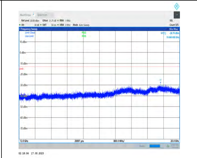
1-N66-PC3-15-30-M-1-DFT-PI2BPSK-Inner_1RB_L ef t-1@1-12000-20000-Ant1-19049.60--28.79--13-PASS
