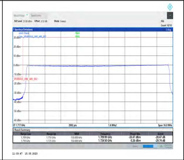
1-DC_5A_n66A-PC3-15-5+15-M+L-6-QPSK-Out er_Full-Outer_Full@N/A-CP-QPSK-Outer_Full-79 @0-1-seegraph-PASS-see graph
