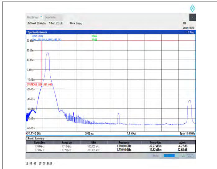
1-DC_5A_n66A-PC3-15-5+10-M+L-1-QPSK-Edge_1RB_Left-Edge_1_Left@N/A-DFT-PI2BPSK-Edge_1RB_Left-1@0-1-seegraph-PASS-see graph
