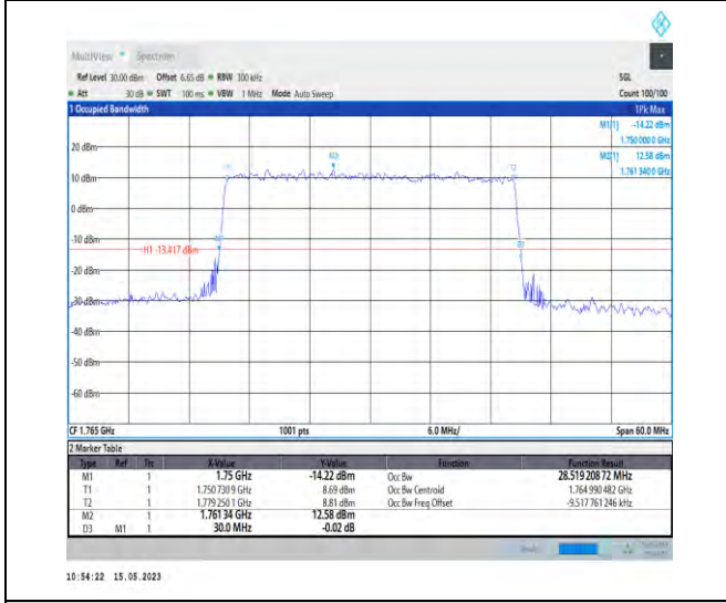
1-DC_5A_n66A-PC3-15-5+30-M+H-4-N/A-N/A-N/A-DFT-64QAM-Outer_Full-160@0-Ant1-28.519-30.000 -<=30-PASS
