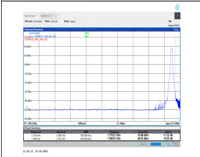
1-DC_5A_n66A-PC3-15-5+30-M+H-5-QPSK-Edge_1RB_Right-Edge_1_Right@N/A-CP-QPSK-Edge_1RB_Right-1@159-1-seegraph-PASS-see graph
