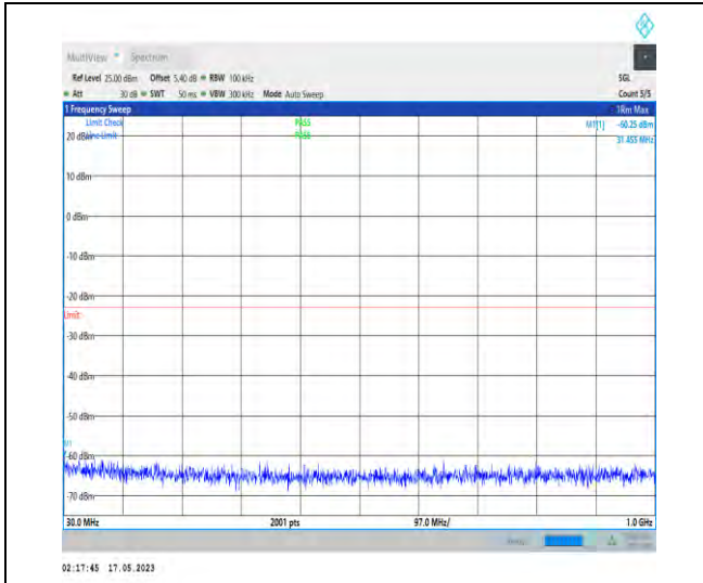
1-N66-PC3-15-30-M-1-DFT-PI2BPSK-Inner_1RB_L eft-1@1-30-1000-Ant1-31.46--60.25--23-PASS
