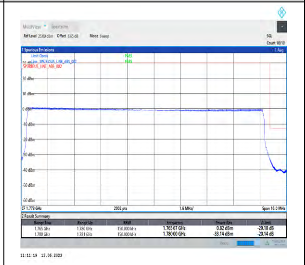
1-DC_5A_n66A-PC3-15-5+15-M+H-6-QPSK-Outer_Full-Outer_Full@N/A-CP-QPSK-Outer_Full-79@0-1-seegraph-PASS-see graph
