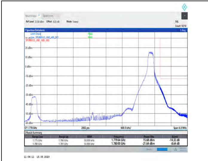
1-DC_5A_n66A-PC3-15-5+5-M+H-2-QPSK-Edge_1RB_Right-Edge_1_Right@N/A-DFT-PI2BPSK-Edge_1RB_Right-1@24-1-seegraph-PASS-see graph
