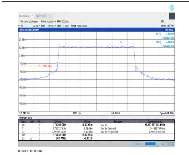
1-DC_5A_n66A-PC3-15-5+30-M+M-7-N/A-N/A-N/A-CP-16QAM-Outer_Full-160@0-Ant1-28.537-30.000-≤30-PASS
