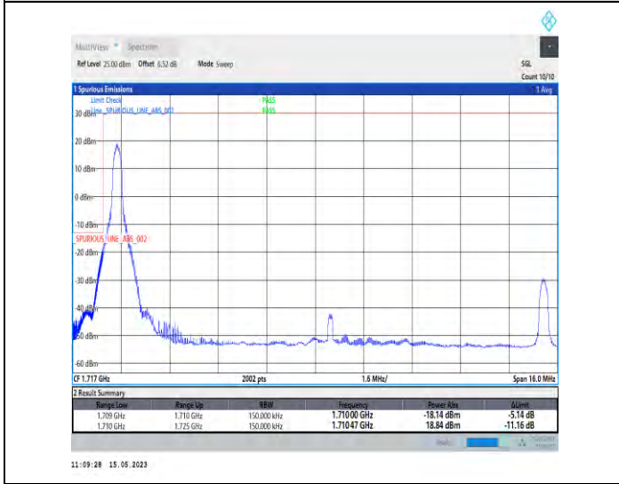
1-DC_5A_n66A-PC3-15-5+15-M+L-4-QPSK-Edge_1RB_Left-Edge_1_Left@N/A-CP-QPSK-Edge_1RB_Left-1 @0-1-seegraph-PASS-see graph
