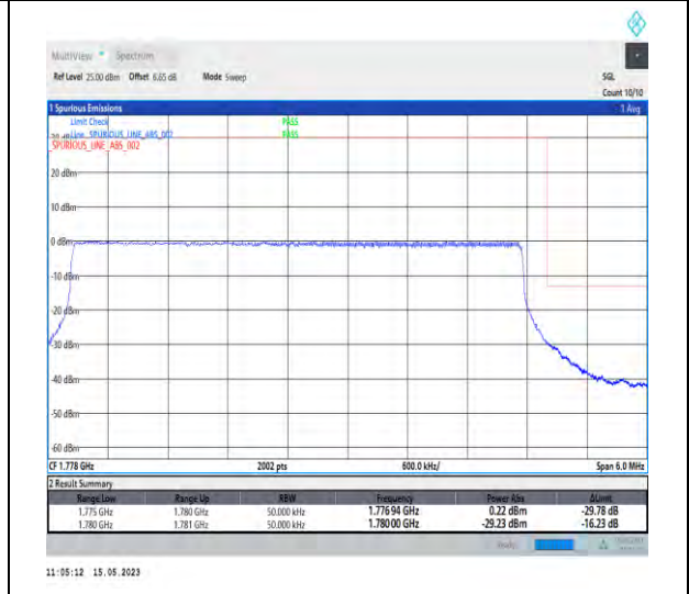
1-DC_5A_n66A-PC3-15-5+5-M+H-6-QPSK-Outer_Full-Outer_Full@N/A-CP-QPSK-Outer_Full-25@0-1-seegraph-PASS-see graph
