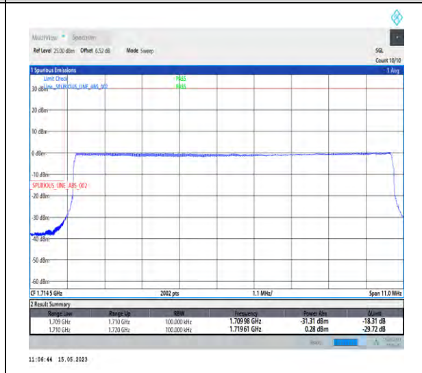
1-DC_5A_n66A-PC3-15-5+10-M+L-6-QPSK-Outer_Full-Outer_Full@N/A-CP-QPSK-Outer_Full-52@0-1-seegraph-PASS-see graph
