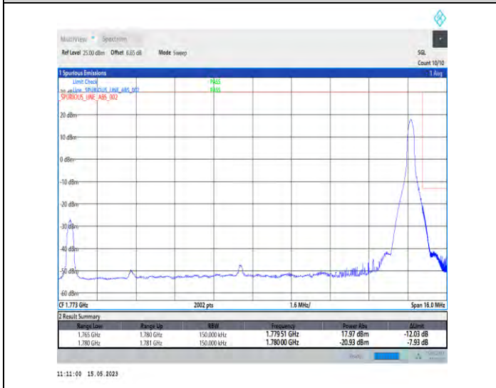
1-DC_5A_n66A-PC3-15-5+15-M+H-5-QPSK-Edge_1RB_Right-Edge_1_Right@N/A-CP-QPSK-Edge_1RB_Right-1@78-1-seegraph-PASS-see graph
