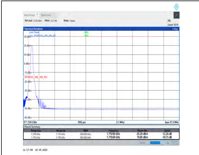
1-DC_5A_n66A-PC3-15-5+30-M+L-1-QPSK-Edge_1RB_Left-Edge_1_Left@N/A-DFT-PI2BPSK-Edge_1RB_Left-1@0-1-seegraph-PASS-see graph
