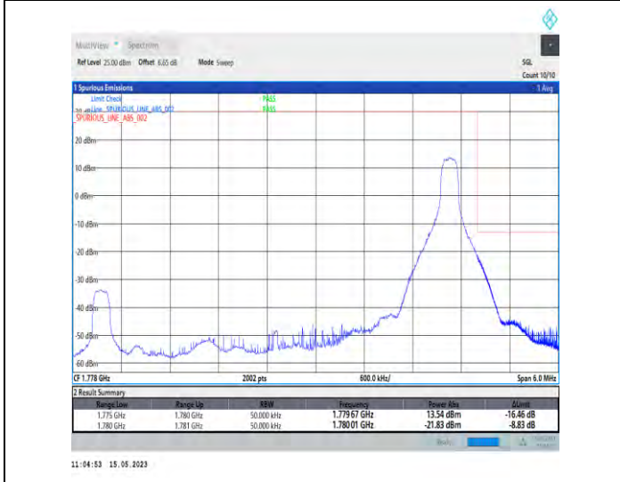
1-DC_5A_n66A-PC3-15-5+5-M+H-5-QPSK-Edge_1RB_Right-Edge_1_Right@N/A-CP-QPSK-Edge_1RB_Right-1@24-1-seegraph-PASS-see graph
