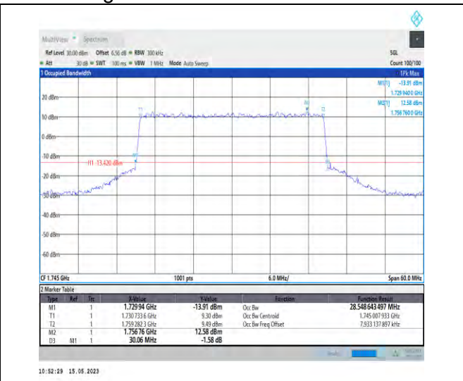
1-DC_5A_n66A-PC3-15-5+30-M+M-8-N/A-N/A-N/A-CP-64QAM-Outer_Full-160@0-Ant1-28.549-30.060-≤30-PASS
