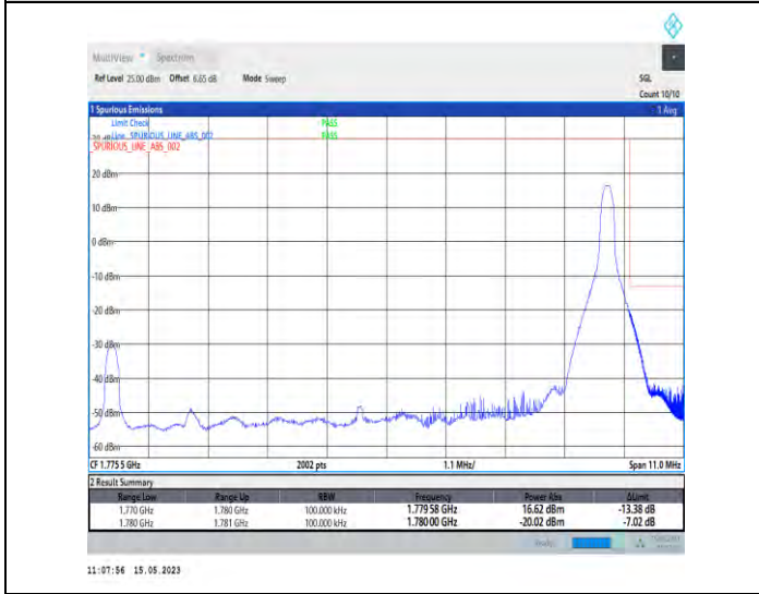
1-DC_5A_n66A-PC3-15-5+10-M+H-5-QPSK-Edge_1RB_Right-Edge_1_Right@N/A-CP-QPSK-Edge_1RB_Right-1@51-1-seegraph-PASS-see graph
