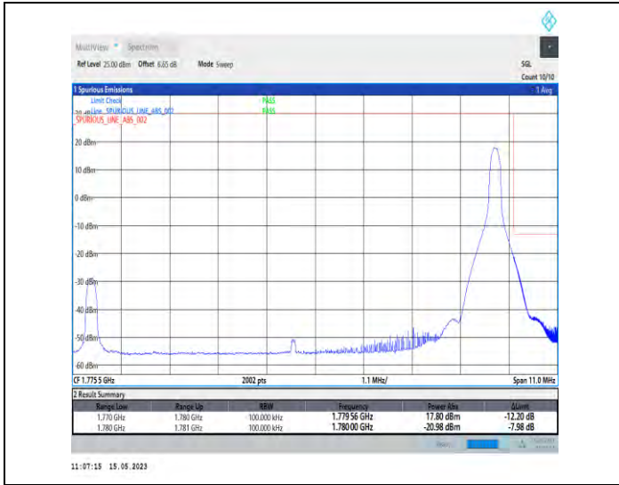
1-DC_5A_n66A-PC3-15-5+10-M+H-2-QPSK-Edge_1RB_Right-Edge_1_Right@N/A-DFT-PI2BPSK-Edge_1RB_Right-1@51-1-seegraph-PASS-see graph
