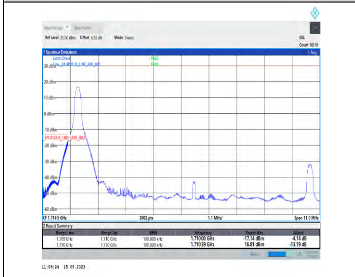
1-DC_5A_n66A-PC3-15-5+10-M+L-4-QPSK-Edge_1RB_Left-Edge_1_Left@N/A-CP-QPSK-Edge_1RB_Left-1@0-1-seegraph-PASS-see graph
