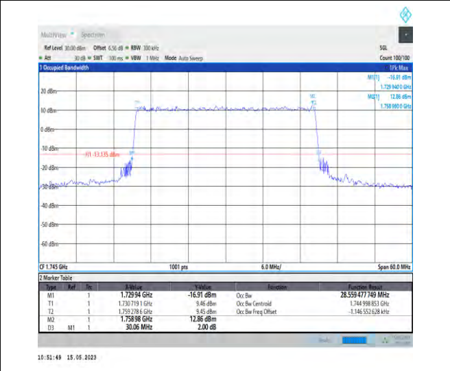
1-DC_5A_n66A-PC3-15-5+30-M+M-6-N/A-N/A-N/A-CP-QPSK-Outer_Full-160@0-Ant1-28.559-30.060-≤30-PASS
