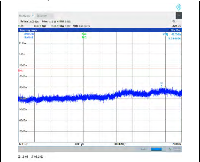
1-N66-PC3-15-30-H-1-DFT-PI2BPSK-Inner_1RB_Lef t-1@1-12000-20000-Ant1-19018.40--29.72--13-PASS
