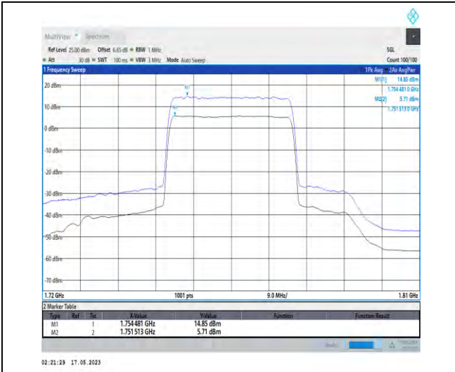
1-N66-PC3-15-30-H-1-DFT-256QAM-Outer_Full-160 @0-Ant1-9.14-100%-0.00-9.14-PASS-≤13
