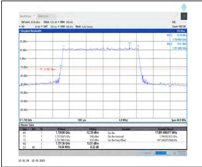
1-DC_5A_n66A-PC3-15-5+20-M+M-3-N/A-N/A-N/A-DFT-16QAM-Outer_Full-100@0-Ant1-17.891-19.040 -≤20-PASS
