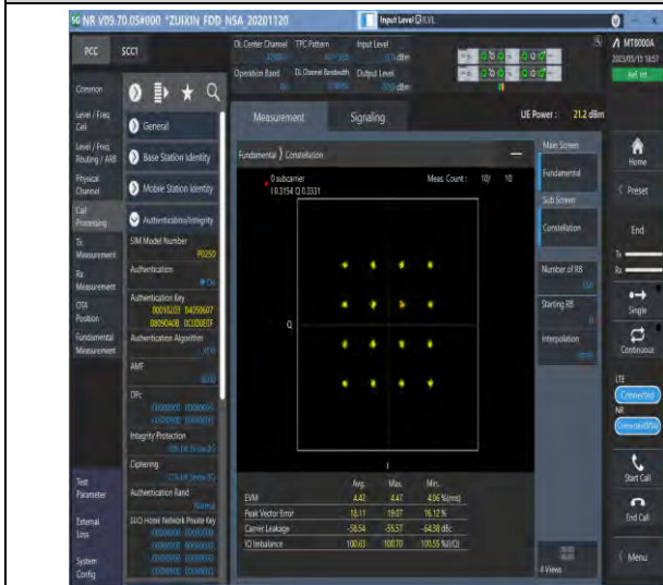
1-DC_5A_n66A-PC3-15-5+30-M+M-7-N/A-N/A-N/A-CP-16QAM-Outer_Full-160@0-see graph-PASS
