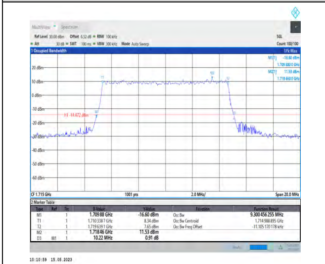
1-DC_5A_n66A-PC3-15-5+10-M+L-8-N/A-N/A-N/A-CP-64QAM-Outer_Full-52@0-Ant1-9.3-10.220-≤10-PASS
