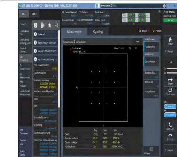
1-DC_5A_n66A-PC3-15-5+30-M+M-3-N/A-N/A-N/A-DFT-16QAM-Outer_Full-160@0-see graph-PASS
