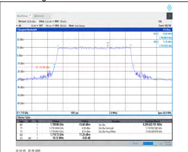
1-DC_5A_n66A-PC3-15-5+10-M+L-7-N/A-N/A-N/A-C-P-16QAM-Outer_Full-52@0-Ant1-9.296-10.120-≤10-PASS
