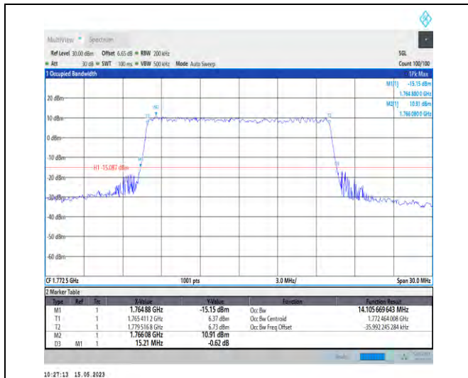
1-DC_5A_n66A-PC3-15-5+15-M+H-9-N/A-N/A-N/A-CP-256QAM-Outer_Full-79@0-Ant1-14.106-15.210-≤15-PASS
