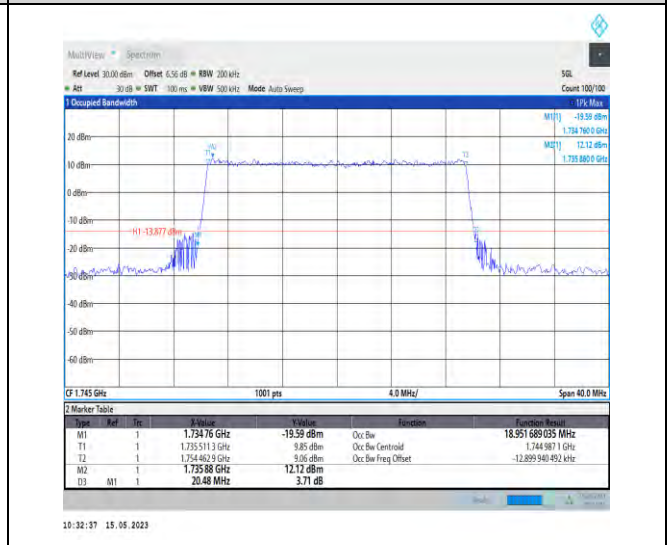
1-DC_5A_n66A-PC3-15-5+20-M+M-6-N/A-N/A-N/A-CP-QPSK-Outer_Full-106@0-Ant1-18.952-20.480-≤20-PASS
