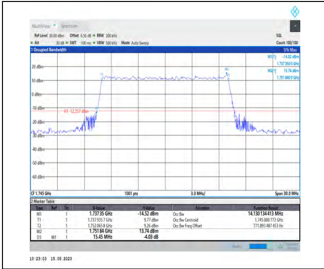
1-DC_5A_n66A-PC3-15-5+15-M+M-6-N/A-N/A-N/A-CP-QPSK-Outer_Full-79@0-Ant1-14.13-15.450-≤15-PASS
