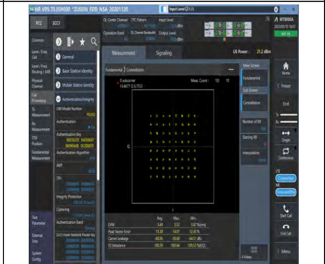
1-DC_5A_n66A-PC3-15-5+30-M+M-8-N/A-N/A-N/A-CP-64QAM-Outer_Full-160@0-see graph-PASS
