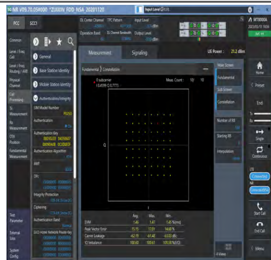
1-DC_5A_n66A-PC3-15-5+30-M+M-4-N/A-N/A-N/A-DFT-64QAM-Outer_Full-160@0-see graph-PASS
