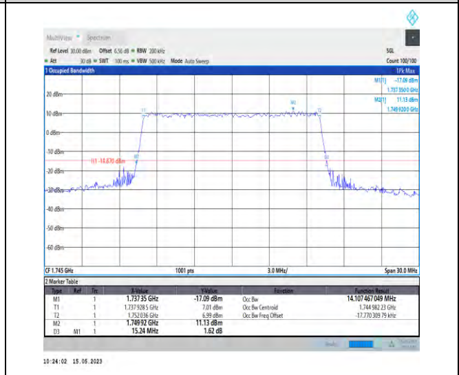
1-DC_5A_n66A-PC3-15-5+15-M+M-9-N/A-N/A-N/A-CP-256QAM-Outer_Full-79@0-Ant1-14.107-15.240-≤15-PASS
