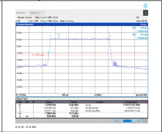
1-DC_5A_n66A-PC3-15-5+20-M+M-4-N/A-N/A-N/A-DFT-64QAM-Outer_Full-100@0-Ant1-17.915-18.960 -≤20-PASS
