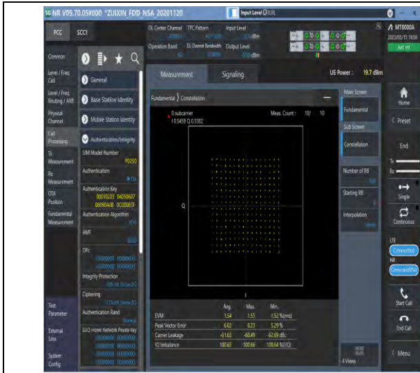
1-DC_5A_n66A-PC3-15-5+30-M+M-5-N/A-N/A-N/A-DFT-256QAM-Outer_Full-160@0-see graph-PASS
