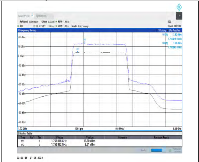
1-N66-PC3-15-30-H-2-CP-256QAM-Outer_Full-160 @0-Ant1-9.79-100%-0.00-9.79-PASS-≤13
