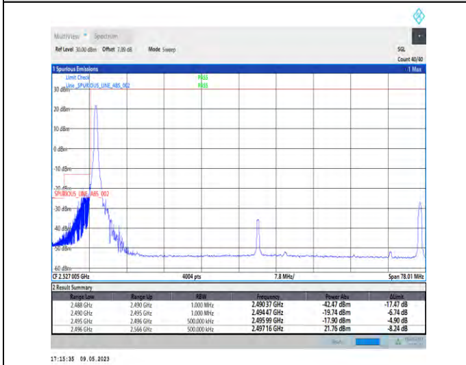
1-N41-PC3-30-70-L-4-CP-QPSK-Edge_1RB_Left-1@0-Ant1-1--PASS-see graph
