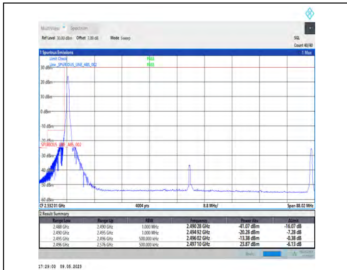
1-N41-PC3-30-80-L-1-DFT-PI2BPSK-Edge_1RB_Left-1@0-Ant1-1--PASS-see graph
