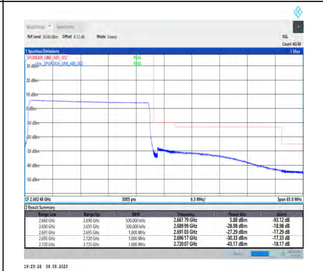
1-N41-PC3-30-30-H-6-CP-QPSK-Outer_Full-78@0-Ant1-1--PASS-see graph
