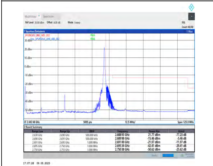
1-N41-PC3-30-60-H-5-CP-QPSK-Edge_1RB_Righ t-1@161-Ant1-1--PASS-see graph
