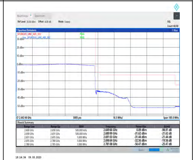
1-N41-PC3-30-90-H-6-CP-QPSK-Outer_Full-245 @0-Ant1-1--PASS-see graph
