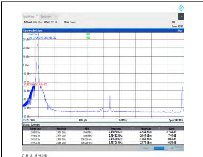
1-N41-PC3-30-90-L-1-DFT-PI2BPSK-Edge_1RB_Left-1@0-Ant1-1--PASS-see graph
