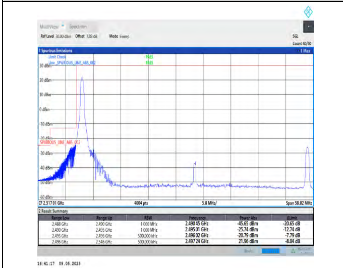
1-N41-PC3-30-50-L-4-CP-QPSK-Edge_1RB_Left-1@0-Ant1-1--PASS-see graph
