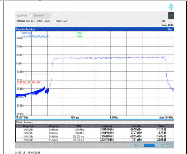
1-N41-PC3-30-30-L-3-DFT-PI2BPSK-Outer_Full-75@0-Ant1-1--PASS-see graph
