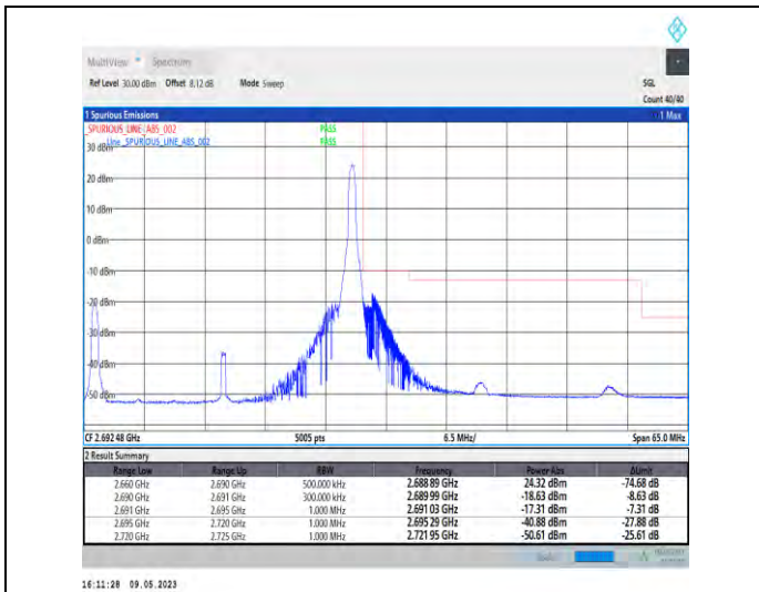
1-N41-PC3-30-30-H-2-DFT-PI2BPSK-Edge_1RB_Right-t-1@77-Ant1-1--PASS-see graph
