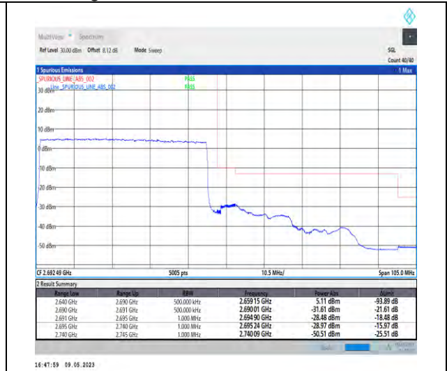
1-N41-PC3-30-50-H-3-DFT-PI2BPSK-Outer_Full-1 28@0-Ant1-1--PASS-see graph
