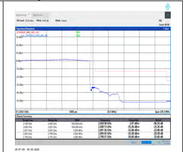
1-N41-PC3-30-100-H-3-DFT-PI2BPSK-Outer_Full-270@0-Ant1-1--PASS-see graph
