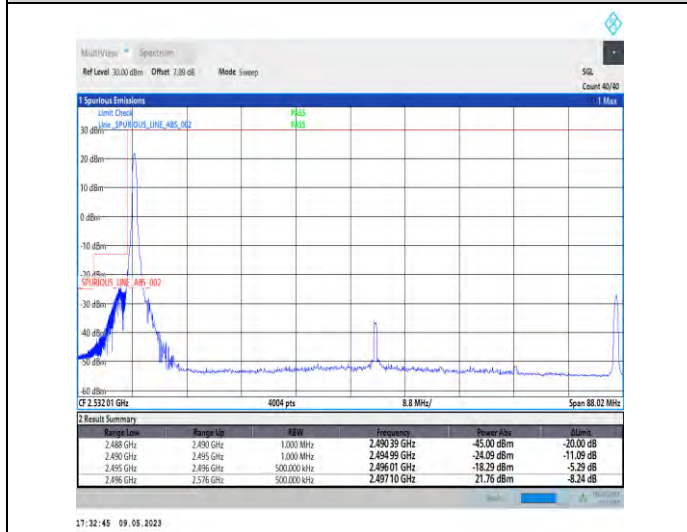
1-N41-PC3-30-80-L-4-CP-QPSK-Edge_1RB_Left-1@0-Ant1-1--PASS-see graph
