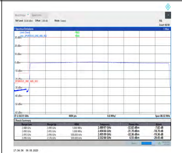
1-N41-PC3-30-80-L-6-CP-QPSK-Outer_Full-217@0-Ant1-1--PASS-see graph
