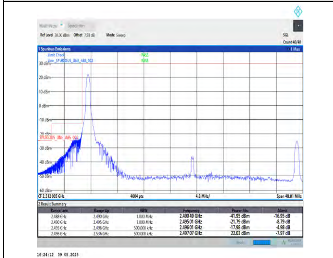
1-N41-PC3-30-40-L-4-CP-QPSK-Edge_1RB_Left-1@0-Ant1-1--PASS-see graph
