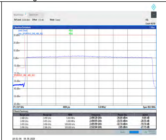
1-N41-PC3-30-90-L-3-DFT-PI2BPSK-Outer_Full-240@0-Ant1-1--PASS-see graph
