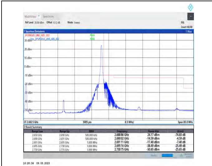
1-N41-PC3-30-40-H-2-DFT-PI2BPSK-Edge_1RB_Righ t-1@105-Ant1-1--PASS-see graph
