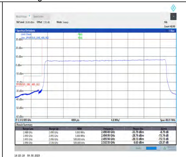
1-N41-PC3-30-40-L-3-DFT-PI2BPSK-Outer_Full-100@0-Ant1-1--PASS-see graph
