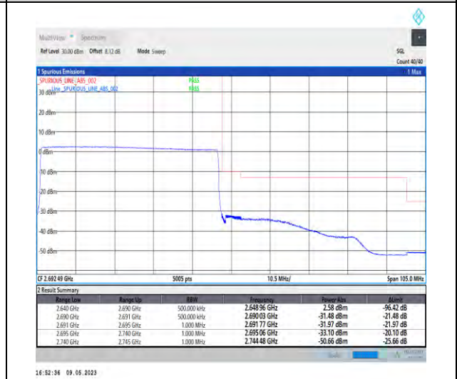
1-N41-PC3-30-50-H-6-CP-QPSK-Outer_Full-133 @0-Ant1-1--PASS-see graph
