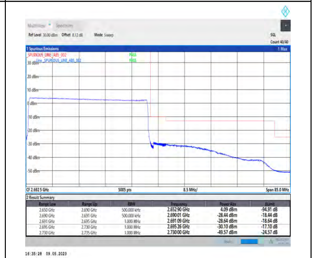
1-N41-PC3-30-40-H-6-CP-QPSK-Outer_Full-106 @0-Ant1-1--PASS-see graph
