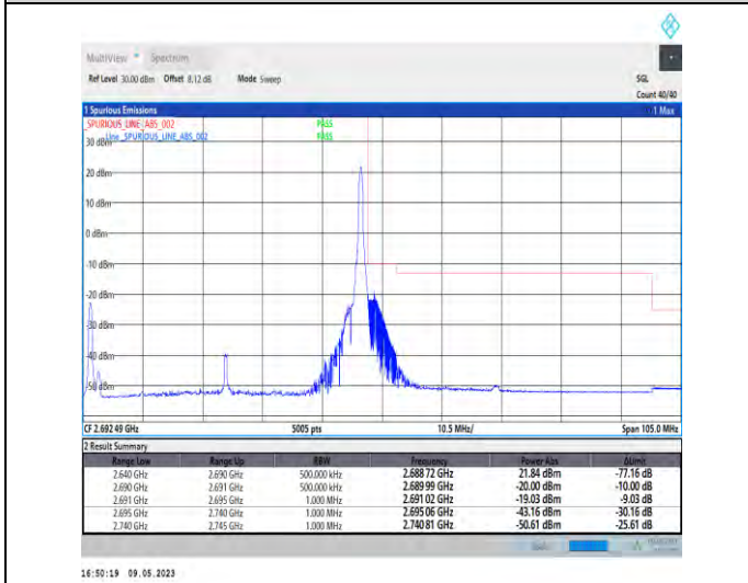
1-N41-PC3-30-50-H-5-CP-QPSK-Edge_1RB_Right-1 @132-Ant1-1--PASS-see graph
