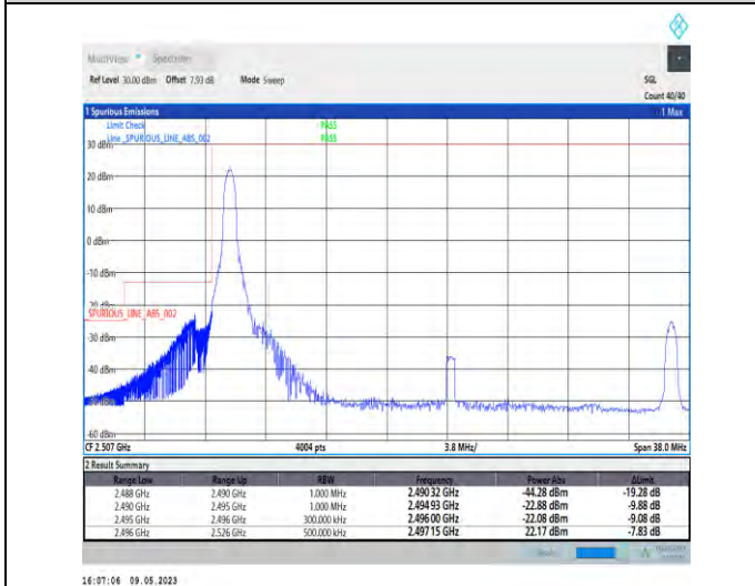
1-N41-PC3-30-30-L-4-CP-QPSK-Edge_1RB_Left-1@0-Ant1-1--PASS-see graph
