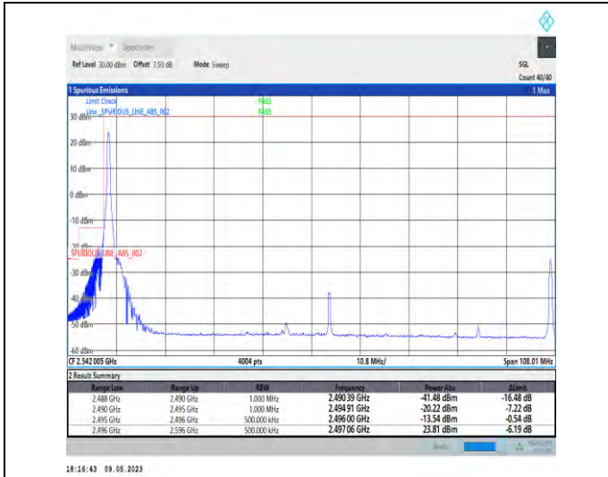
1-N41-PC3-30-100-L-1-DFT-PI2BPSK-Edge_1RB_Left-1@0-Ant1-1--PASS-see graph
