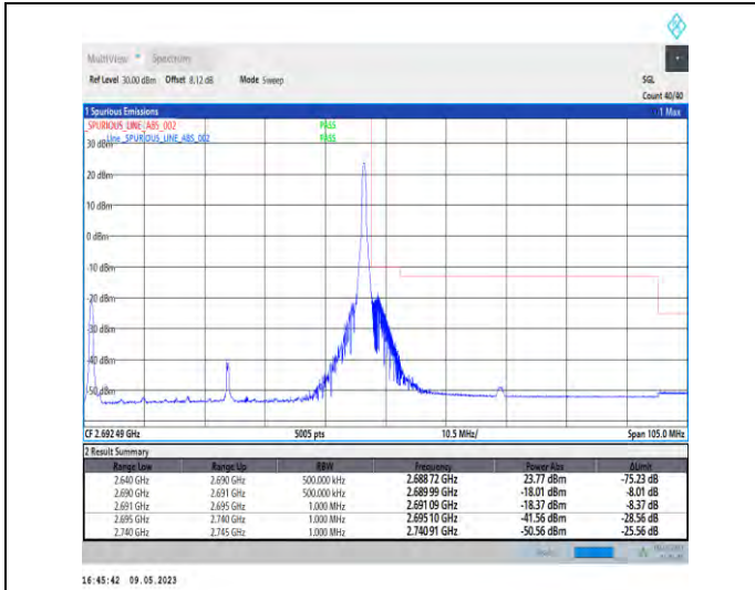
1-N41-PC3-30-50-H-2-DFT-PI2BPSK-Edge_1RB_Righ t-1@132-Ant1-1--PASS-see graph
