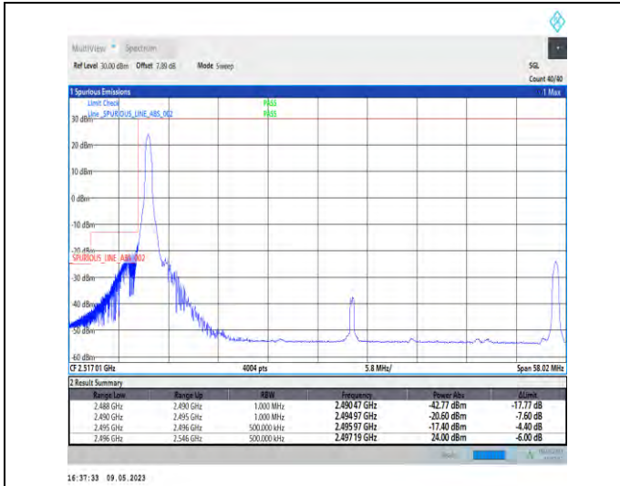
1-N41-PC3-30-50-L-1-DFT-PI2BPSK-Edge_1RB_Left-1@0-Ant1-1--PASS-see graph
