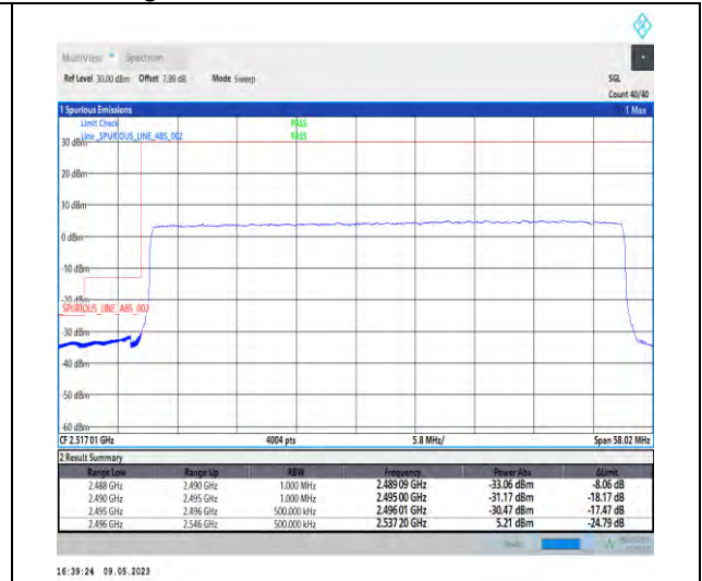
1-N41-PC3-30-50-L-3-DFT-PI2BPSK-Outer_Full-128@0-Ant1-1--PASS-see graph
