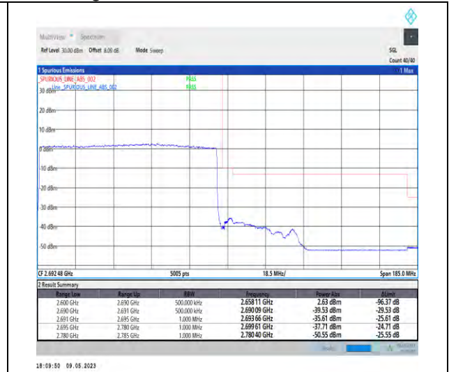
1-N41-PC3-30-90-H-3-DFT-PI2BPSK-Outer_Full-2 40@0-Ant1-1--PASS-see graph
