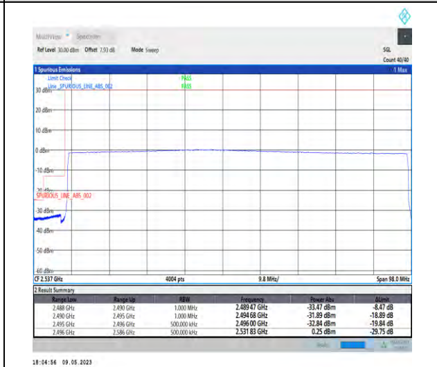
1-N41-PC3-30-90-L-6-CP-QPSK-Outer_Full-245@0-Ant1-1--PASS-see graph
