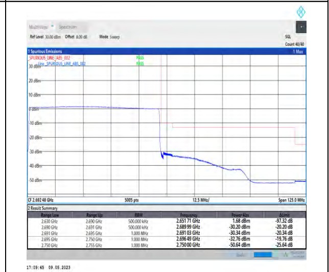
1-N41-PC3-30-60-H-6-CP-QPSK-Outer_Full-162 @0-Ant1-1--PASS-see graph
