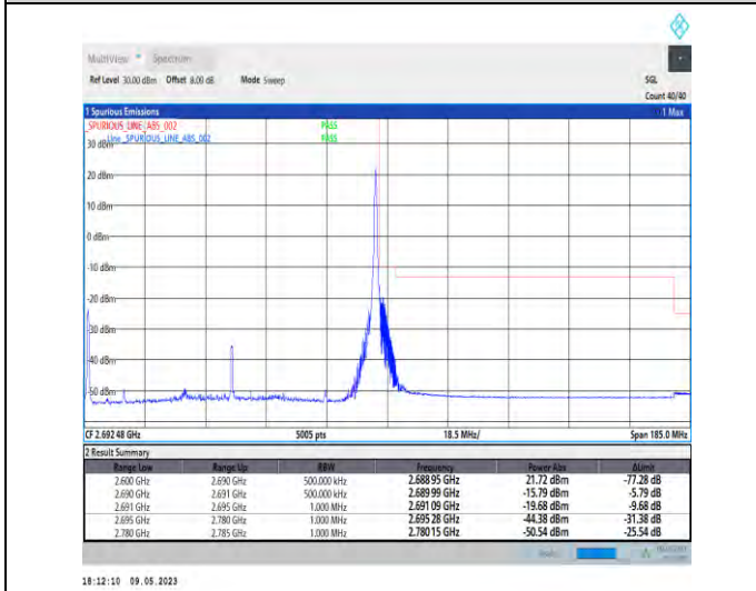
1-N41-PC3-30-90-H-5-CP-QPSK-Edge_1RB_Right-1 @244-Ant1-1--PASS-see graph
