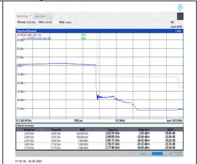
1-N41-PC3-30-80-H-3-DFT-PI2BPSK-Outer_Full-2 16@0-Ant1-1--PASS-see graph
