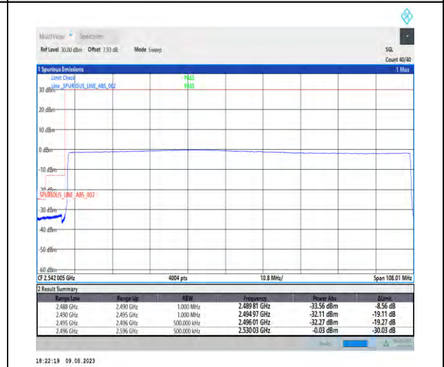
1-N41-PC3-30-100-L-6-CP-QPSK-Outer_Full-273@0-Ant1-1--PASS-see graph
