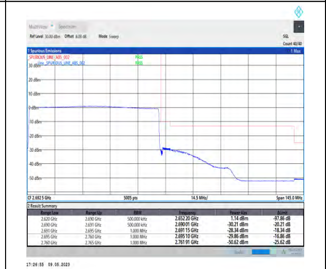
1-N41-PC3-30-70-H-6-CP-QPSK-Outer_Full-189 @0-Ant1-1--PASS-see graph
