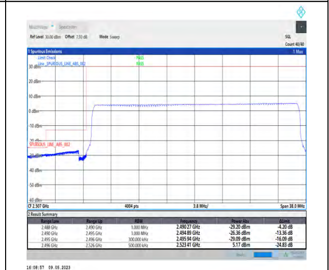
1-N41-PC3-30-30-L-6-CP-QPSK-Outer_Full-78@0-Ant1-1--PASS-see graph
