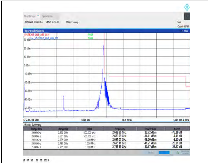
1-N41-PC3-30-90-H-2-DFT-PI2BPSK-Edge_1RB_Righ t-1@244-Ant1-1--PASS-see graph
