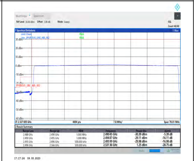
1-N41-PC3-30-70-L-6-CP-QPSK-Outer_Full-189@0-Ant1-1--PASS-see graph
