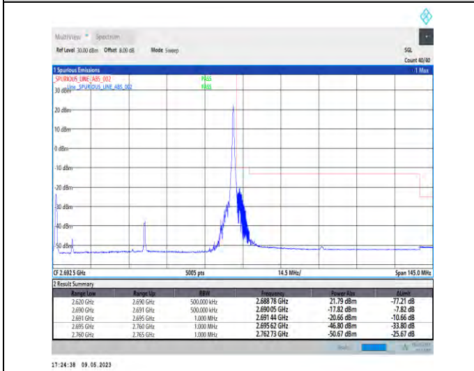
1-N41-PC3-30-70-H-5-CP-QPSK-Edge_1RB_Right-1 @188-Ant1-1--PASS-see graph
