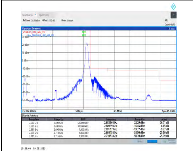
1-N41-PC3-30-20-H-5-CP-QPSK-Edge_1RB_Right-1 @50-Ant1-1--PASS-see graph
