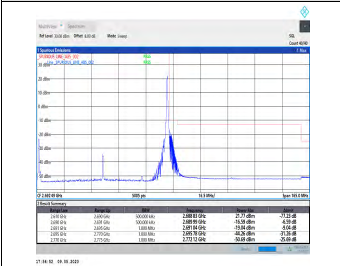
1-N41-PC3-30-80-H-5-CP-QPSK-Edge_1RB_Right-1 @216-Ant1-1--PASS-see graph
