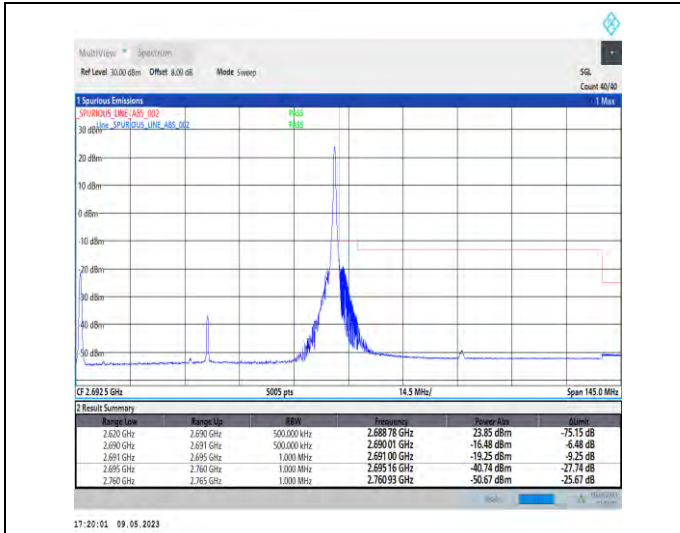
1-N41-PC3-30-70-H-2-DFT-PI2BPSK-Edge_1RB_Righ t-1@188-Ant1-1--PASS-see graph
