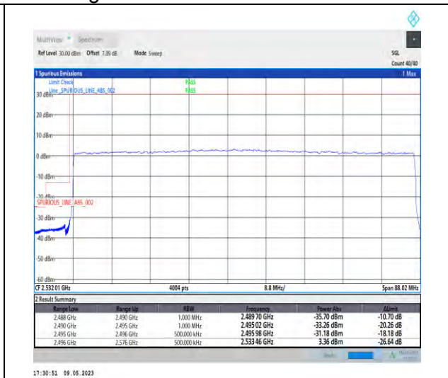
1-N41-PC3-30-80-L-3-DFT-PI2BPSK-Outer_Full-216@0-Ant1-1--PASS-see graph
