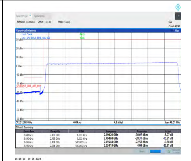
1-N41-PC3-30-40-L-6-CP-QPSK-Outer_Full-106@0-Ant1-1--PASS-see graph
