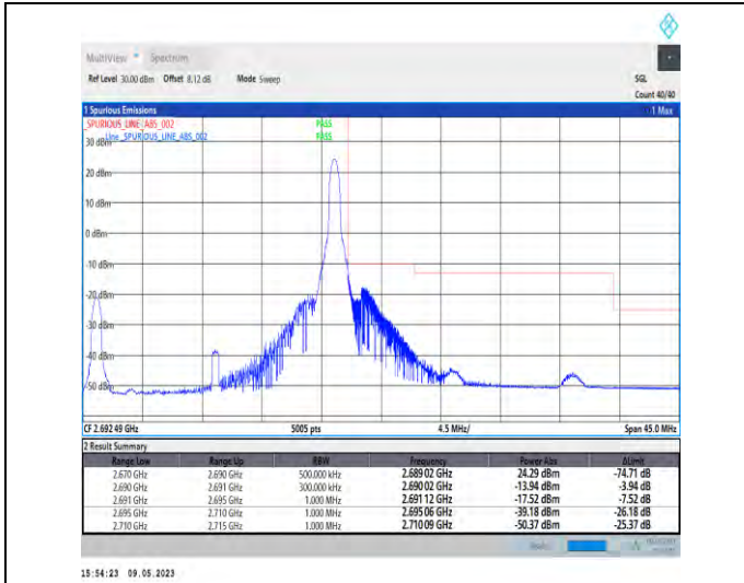
1-N41-PC3-30-20-H-2-DFT-PI2BPSK-Edge_1RB_Righ t-1@50-Ant1-1--PASS-see graph
