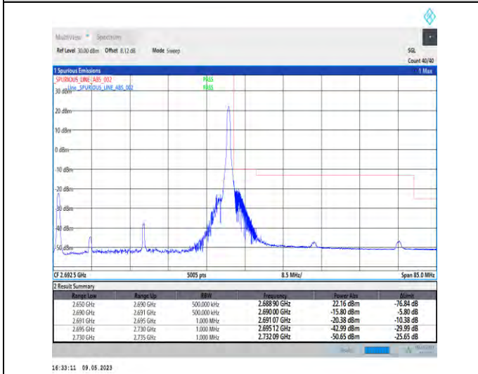
1-N41-PC3-30-40-H-5-CP-QPSK-Edge_1RB_Right-1 @105-Ant1-1--PASS-see graph
