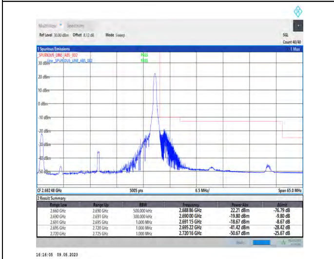
1-N41-PC3-30-30-H-5-CP-QPSK-Edge_1RB_Right-1@77-Ant1-1--PASS-see graph
