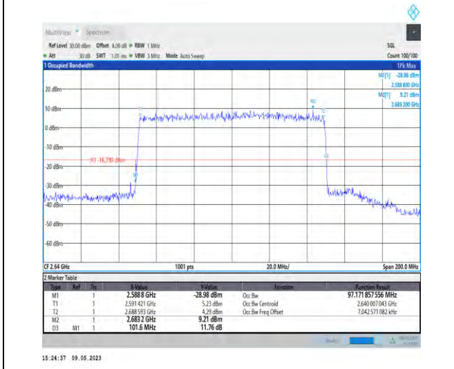
1-N41-PC3-30-100-H-9-CP-256QAM-Outer_Full-273 @0-Ant1-97.172-101.600-≤100-PASS
