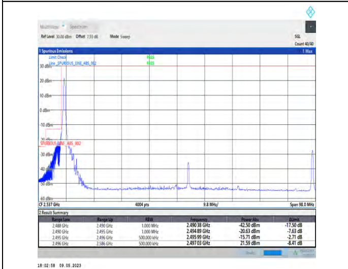
1-N41-PC3-30-90-L-4-CP-QPSK-Edge_1RB_Left-1@0-Ant1-1--PASS-see graph
