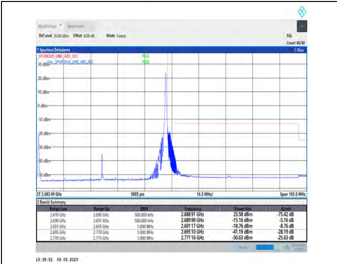
1-N41-PC3-30-80-H-2-DFT-PI2BPSK-Edge_1RB_Righ t-1@216-Ant1-1--PASS-see graph
