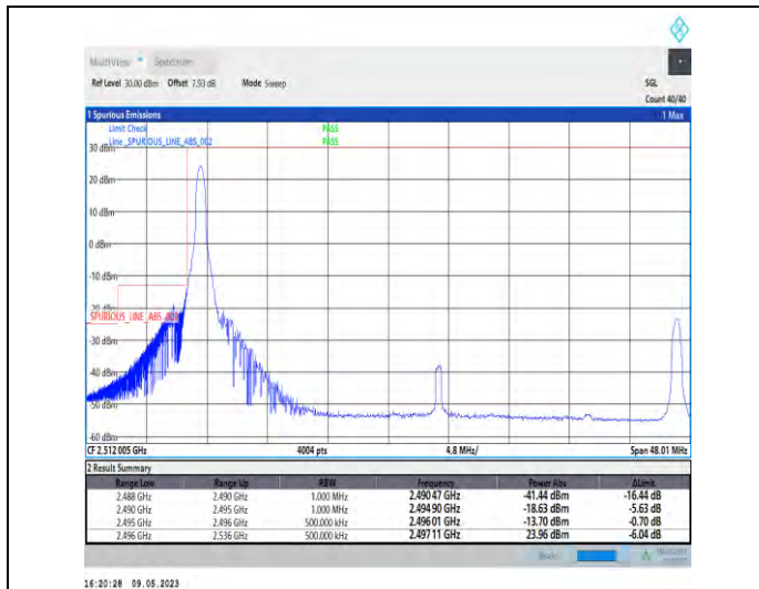
1-N41-PC3-30-40-L-1-DFT-PI2BPSK-Edge_1RB_Left-1@0-Ant1-1--PASS-see graph
