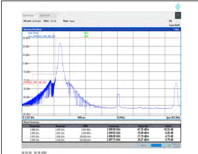
1-N41-PC3-30-30-L-1-DFT-PI2BPSK-Edge_1RB_Left-1@0-Ant1-1--PASS-see graph
