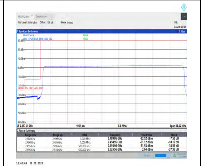
1-N41-PC3-30-50-L-6-CP-QPSK-Outer_Full-133@0-Ant1-1--PASS-see graph
