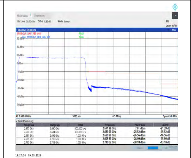
1-N41-PC3-30-20-H-6-CP-QPSK-Outer_Full-51@ 0-Ant1-1--PASS-see graph
