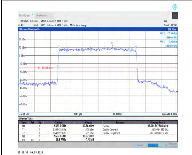
1-N41-PC3-30-100-H-5-DFT-256QAM-Outer_Full-27 @0-Ant1-96.065-99.800-≤100-PASS
