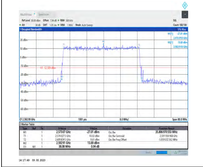
1-N41-PC3-30-40-M-4-DFT-64QAM-Outer_Full-100@0-Ant1-35.807-38.080-≤40-PASS
