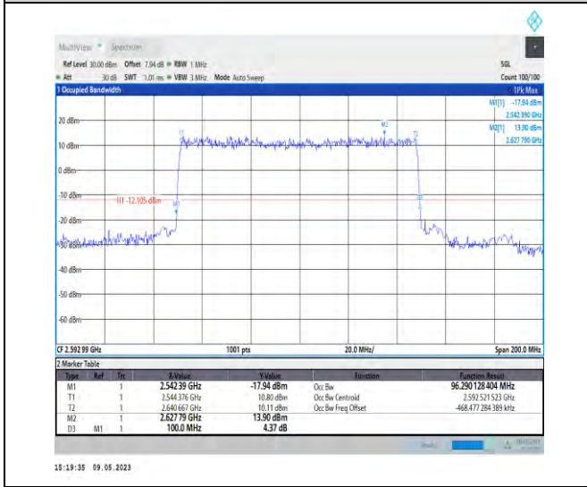
1-N41-PC3-30-100-M-2-DFT-PI2BPSK-Outer_Full-270 @0-Ant1-96.29-100.000-≤100-PASS
