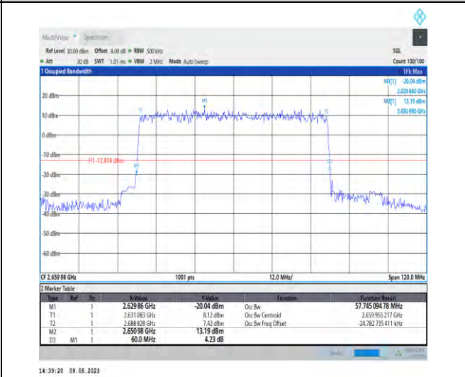
1-N41-PC3-30-60-H-2-DFT-PI2BPSK-Outer_Full-16 2@0-Ant1-57.745-60.000-≤60-PASS
