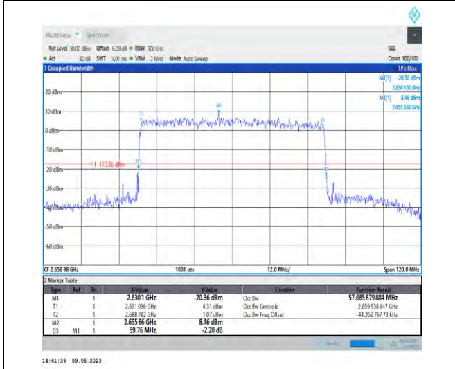
1-N41-PC3-30-60-H-9-CP-256QAM-Outer_Full-162 @0-Ant1-57.686-59.760-≤60-PASS
