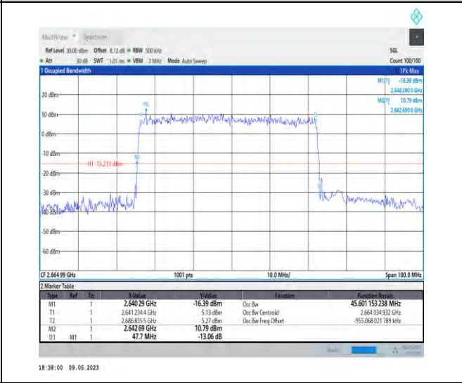
1-N41-PC3-30-50-H-5-DFT-256QAM-Outer_Full-128 @0-Ant1-45.601-47.700-≤50-PASS
