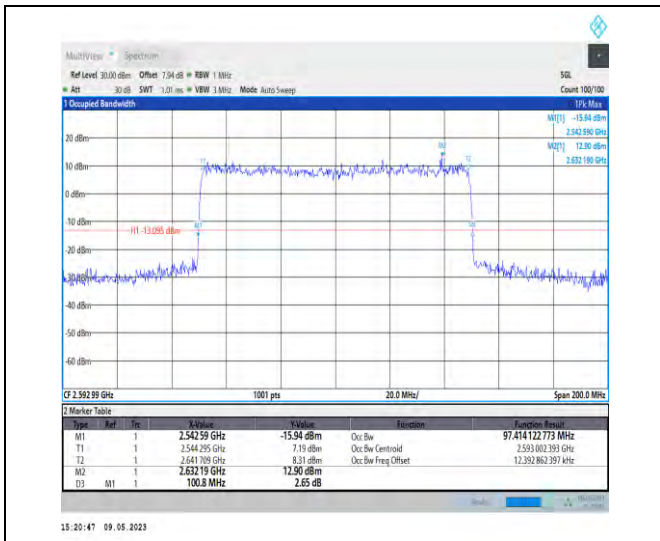
1-N41-PC3-30-100-M-8-CP-64QAM-Outer_Full-273 @0-Ant1-97.414-100.800-≤100-PASS
