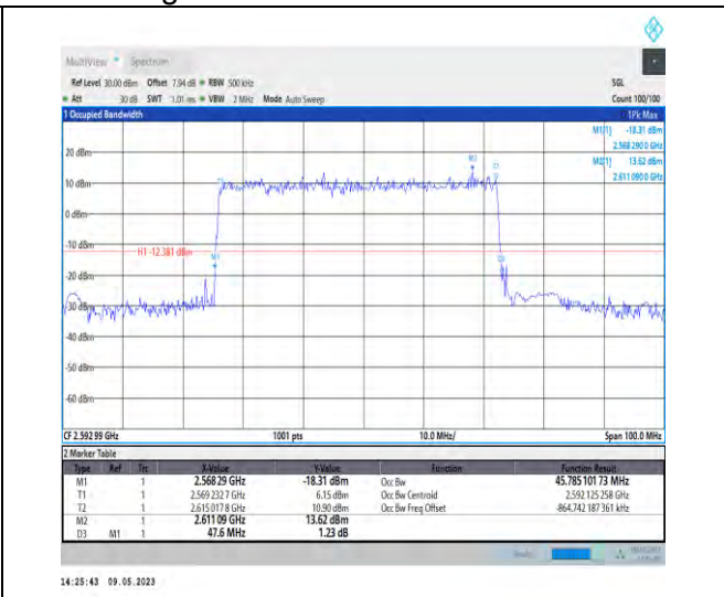
1-N41-PC3-30-50-M-4-DFT-64QAM-Outer_Full-128 @0-Ant1-45.785-47.600-≤50-PASS
