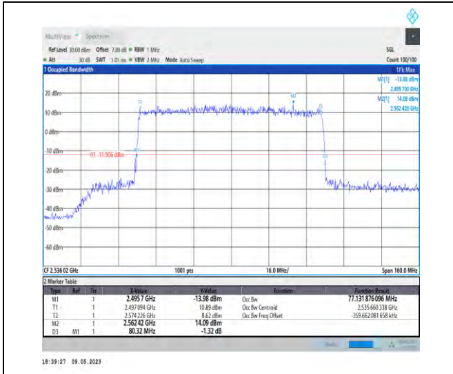
1-N41-PC3-30-80-L-3-DFT-16QAM-Outer_Full-216 @0-Ant1-77.132-80.320-≤80-PASS
