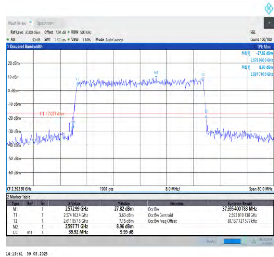
1-N41-PC3-30-40-M-9-CP-256QAM-Outer_Full-106 @0-Ant1-37.695-39.920-≤40-PASS
