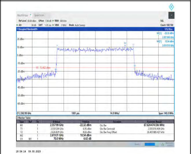
1-N41-PC3-30-70-M-8-CP-64QAM-Outer_Full-189@0-Ant1-67.624-70.000-≤70-PASS
