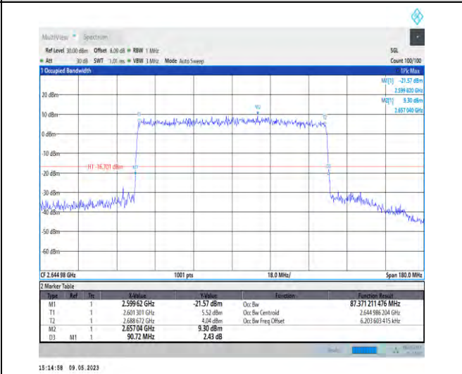
1-N41-PC3-30-90-H-9-CP-256QAM-Outer_Full-245@0-Ant1-87.371-90.720-<=90-PASS
