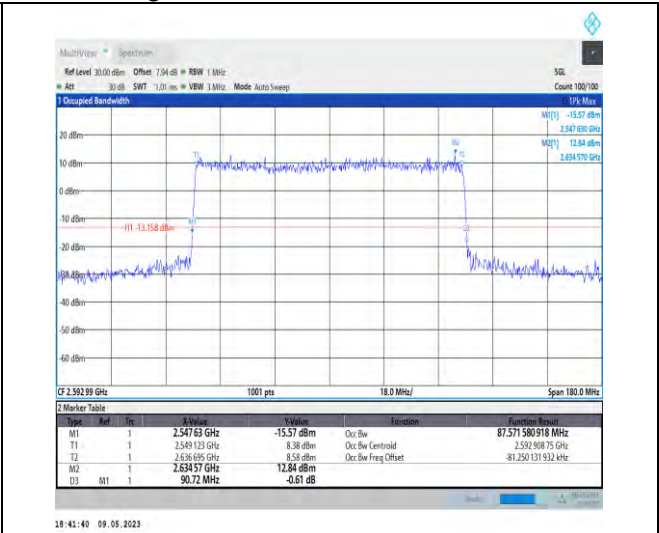
1-N41-PC3-30-90-M-8-CP-64QAM-Outer_Full-245@ 0-Ant1-87.572-90.720-≤90-PASS
