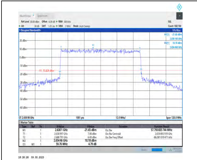
1-N41-PC3-30-60-H-7-CP-16QAM-Outer_Full-162@ 0-Ant1-57.794-59.760-≤60-PASS
