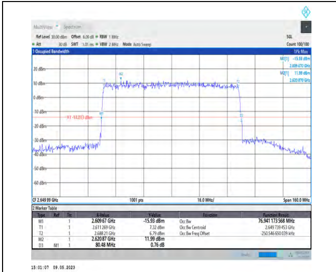
1-N41-PC3-30-80-H-5-DFT-256QAM-Outer_Full-216 @0-Ant1-76.941-80.480-≤80-PASS
