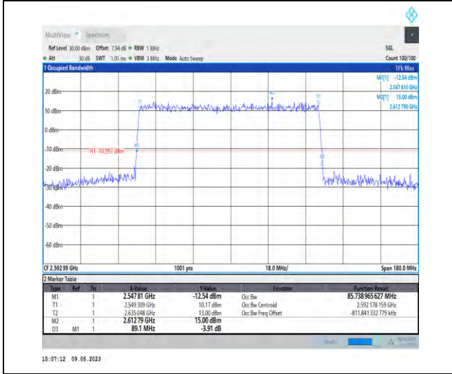
1-N41-PC3-30-90-M-1-DFT-QPSK-Outer_Full-240@ 0-Ant1-85.739-89.100-≤90-PASS
