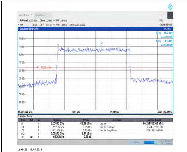
1-N41-PC3-30-70-M-5-DFT-256QAM-Outer_Full-180 @0-Ant1-64.355-66.360-≤70-PASS
