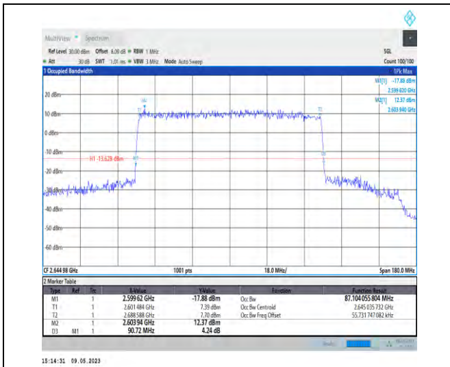
1-N41-PC3-30-90-H-6-CP-QPSK-Outer_Full-245@0-Ant1-87.104-90.720-<=90-PASS
