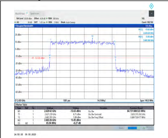
1-N41-PC3-30-70-H-1-DFT-QPSK-Outer_Full-180 @0-Ant1-64.152-65.940-≤70-PASS
