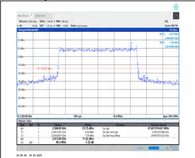
1-N41-PC3-30-50-M-8-CP-64QAM-Outer_Full-133@ 0-Ant1-47.602-49.300-≤50-PASS
