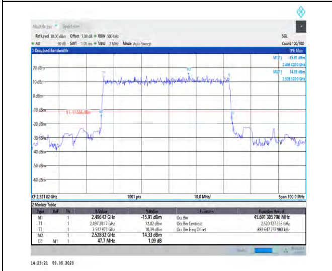
1-N41-PC3-30-50-L-2-DFT-PI2BPSK-Outer_Full-128 @0-Ant1-45.691-47.700-≤50-PASS
