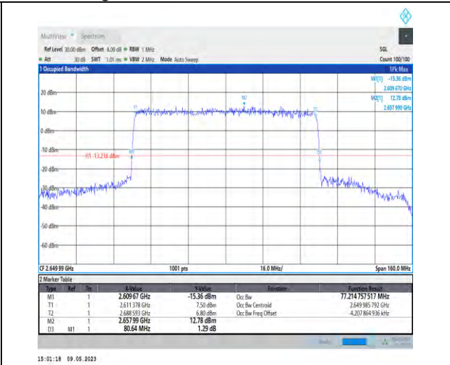
1-N41-PC3-30-80-H-6-CP-QPSK-Outer_Full-217@0-Ant1-77.215-80.640-≤80-PASS
