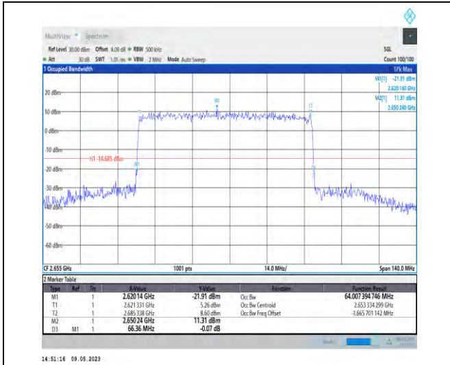
1-N41-PC3-30-70-H-4-DFT-64QAM-Outer_Full-180 @0-Ant1-64.007-66.360-≤70-PASS
