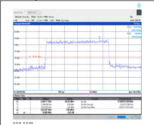
1-N41-PC3-30-60-M-9-CP-256QAM-Outer_Full-162 @0-Ant1-57.895-59.880-≤60-PASS
