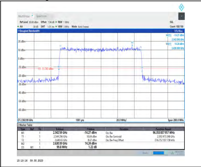
1-N41-PC3-30-100-M-1-DFT-QPSK-Outer_Full-270 @0-Ant1-96.354-99.800-≤100-PASS
