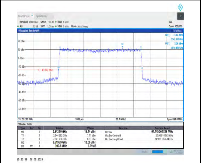
1-N41-PC3-30-100-M-7-CP-16QAM-Outer_Full-273 @0-Ant1-97.445-100.800-≤100-PASS
