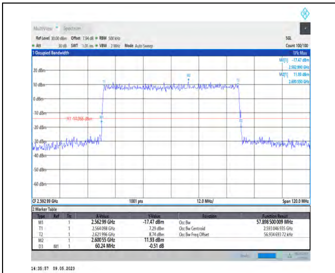
1-N41-PC3-30-60-M-4-DFT-64QAM-Outer_Full-162 @0-Ant1-57.899-60.240-≤60-PASS
