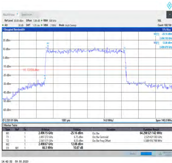
1-N41-PC3-30-70-L-4-DFT-64QAM-Outer_Full-180 @0-Ant1-64.299-66.500-≤70-PASS
