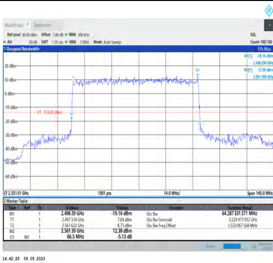
1-N41-PC3-30-70-L-2-DFT-PI2BPSK-Outer_Full-180 @0-Ant1-64.287-66.500-≤70-PASS
