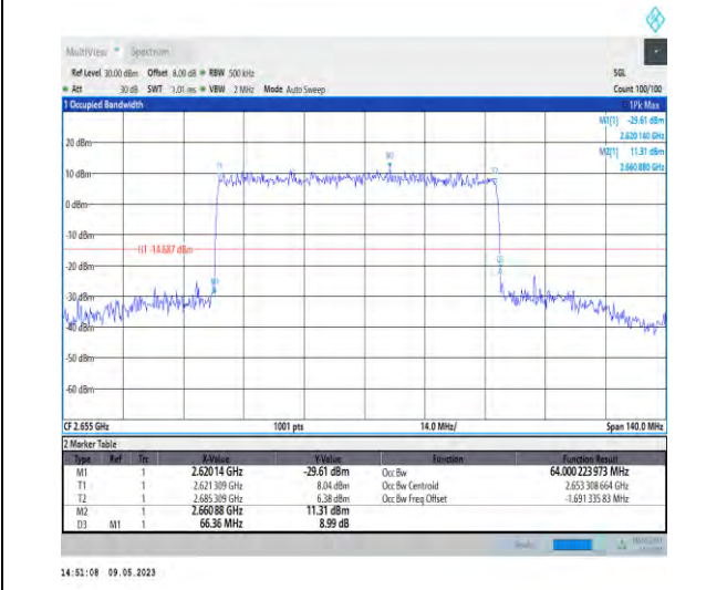
1-N41-PC3-30-70-H-3-DFT-16QAM-Outer_Full-180 @0-Ant1-64-66.360-≤70-PASS
