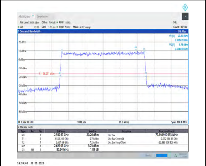
1-N41-PC3-30-80-M-9-CP-256QAM-Outer_Full-217@0 -Ant1-77.447-80.640-<80-PASS
