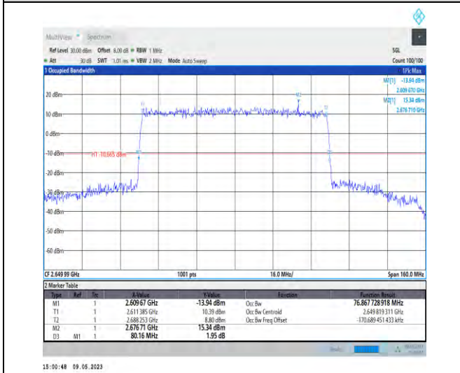
1-N41-PC3-30-80-H-3-DFT-16QAM-Outer_Full-216@0-Ant1-76.868-80.160-≤80-PASS
