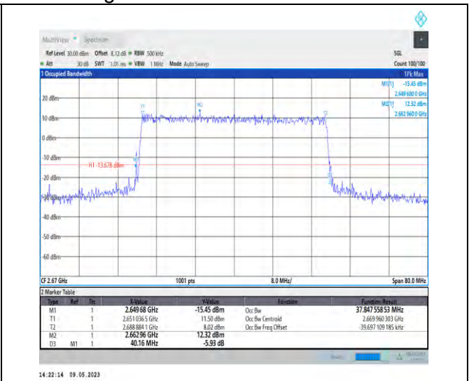
1-N41-PC3-30-40-H-6-CP-QPSK-Outer_Full-106@0-Ant1-37.848-40.160-<math>\leq 40</math>-PASS
