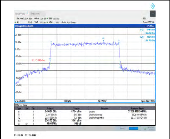
1-N41-PC3-30-60-L-8-CP-64QAM-Outer_Full-162@0-Ant1-57.739-59.640-≤60-PASS
