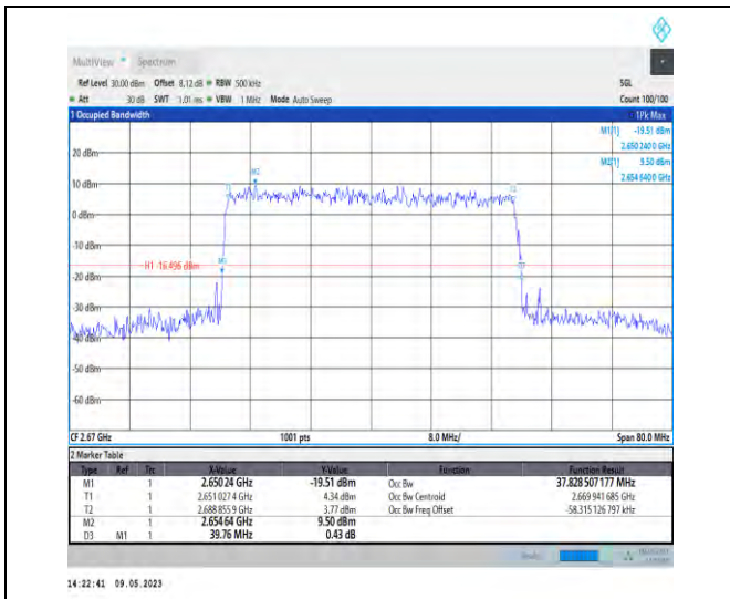
1-N41-PC3-30-40-H-9-CP-256QAM-Outer_Full-106 @0-Ant1-37.829-39.760-≤40-PASS
