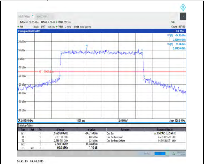
1-N41-PC3-30-60-H-8-CP-64QAM-Outer_Full-162@ 0-Ant1-57.651-60.000-≤60-PASS
