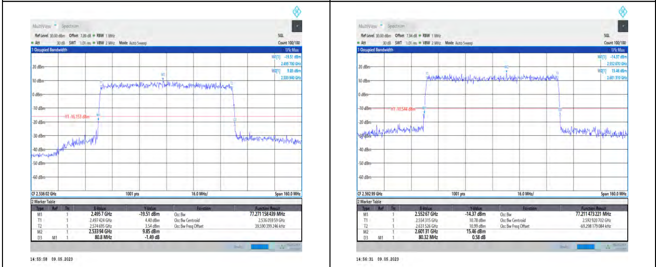
1-N41-PC3-30-80-L-9-CP-256QAM-Outer_Full-217 @0-Ant1-77.271-80.800-≤80-PASS 1-N41-PC3-30-80-M-1-DFT-QPSK-Outer_Full-216@ 0-Ant1-77.211-80.320-≤80-PASS
