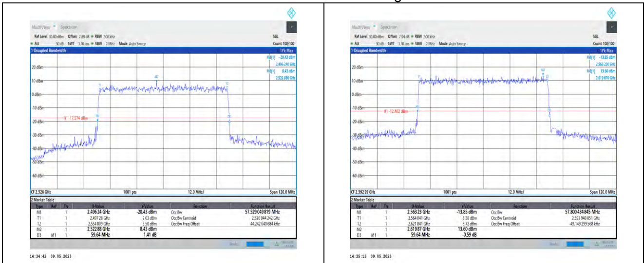
1-N41-PC3-30-60-L-9-CP-256QAM-Outer_Full-162 @0-Ant1-57.529-59.640-≤60-PASS 1-N41-PC3-30-60-M-1-DFT-QPSK-Outer_Full-162@ 0-Ant1-57.8-59.640-≤60-PASS
