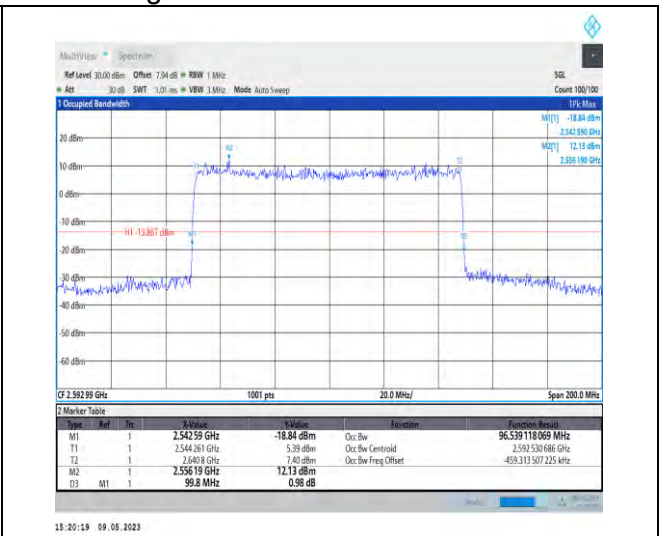
1-N41-PC3-30-100-M-5-DFT-256QAM-Outer_Full-270 @0-Ant1-96.539-99.800-≤100-PASS
