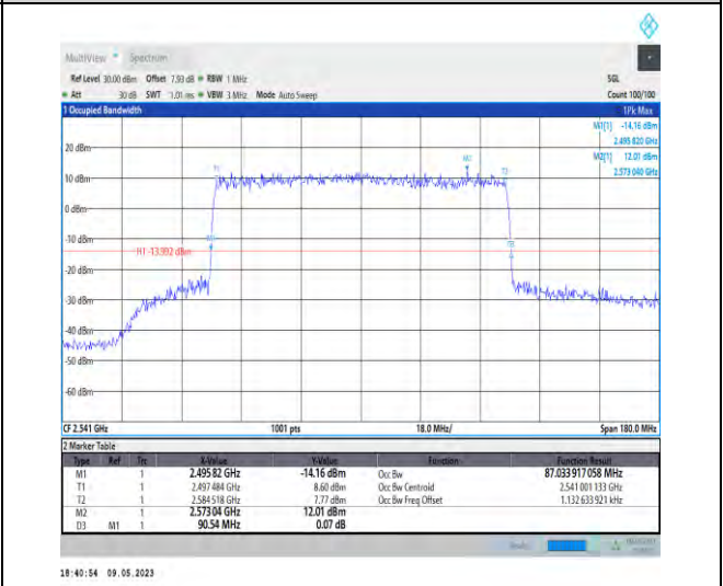
1-N41-PC3-30-90-L-7-CP-16QAM-Outer_Full-245@0-Ant1-87.034-90.540-≤90-PASS
