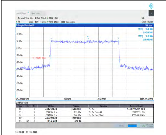
1-N41-PC3-30-100-M-6-CP-QPSK-Outer_Full-273 @0-Ant1-97.62-101.000-≤100-PASS
