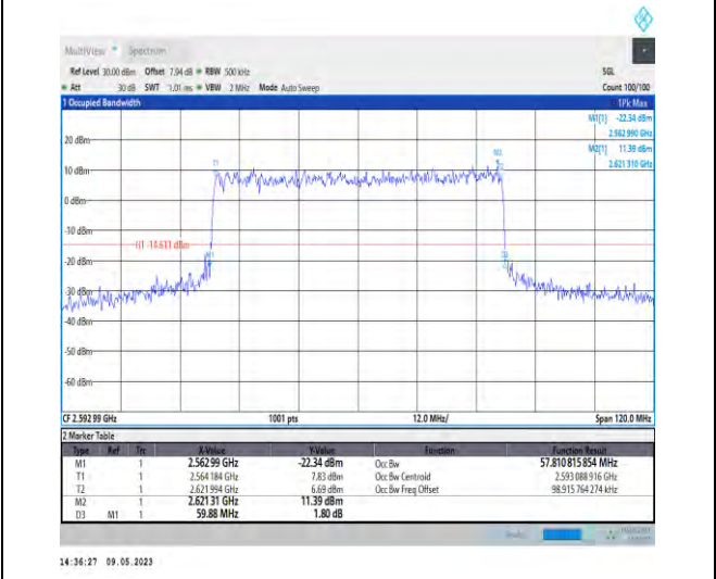
1-N41-PC3-30-60-M-7-CP-16QAM-Outer_Full-162@0 -Ant1-57.811-59.880-≤60-PASS
