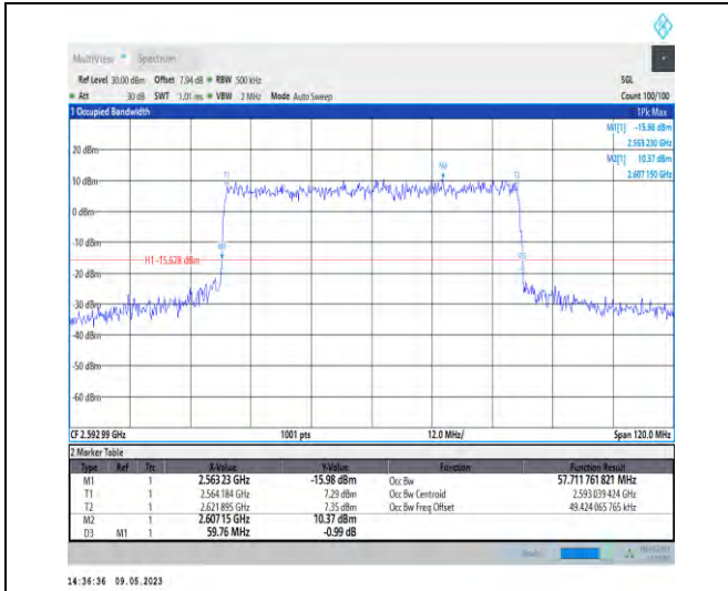
1-N41-PC3-30-60-M-8-CP-64QAM-Outer_Full-162@ 0-Ant1-57.712-59.760-≤60-PASS
