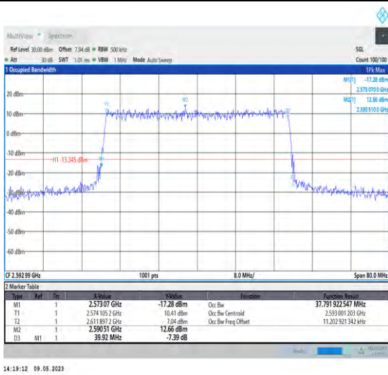
1-N41-PC3-30-40-M-6-CP-QPSK-Outer_Full-106@0 -Ant1-37.792-39.920-≤40-PASS
