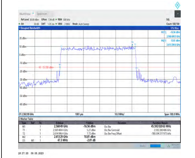
1-N41-PC3-30-50-M-5-DFT-256QAM-Outer_Full-128 @0-Ant1-45.592-47.300-≤50-PASS
