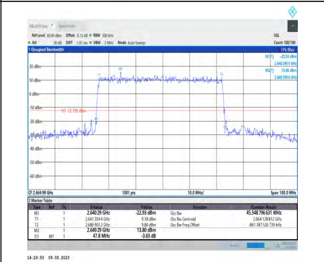
1-N41-PC3-30-50-H-1-DFT-QPSK-Outer_Full-128@ 0-Ant1-45.549-47.800-≤50-PASS
