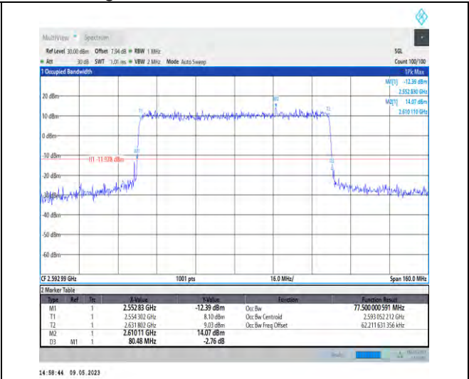
1-N41-PC3-30-80-M-7-CP-16QAM-Outer_Full-217@0 -Ant1-77.5-80.480-<80-PASS
