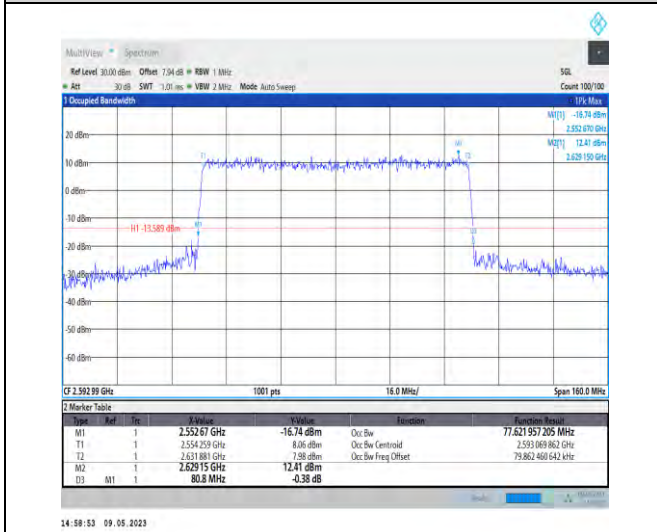
1-N41-PC3-30-80-M-8-CP-64QAM-Outer_Full-217@0 -Ant1-77.622-80.800-<80-PASS
