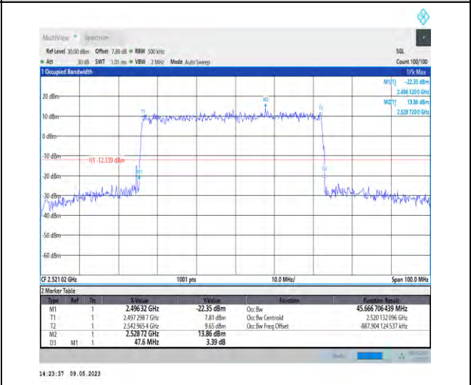
1-N41-PC3-30-50-L-3-DFT-16QAM-Outer_Full-128 @0-Ant1-45.667-47.600-≤50-PASS
