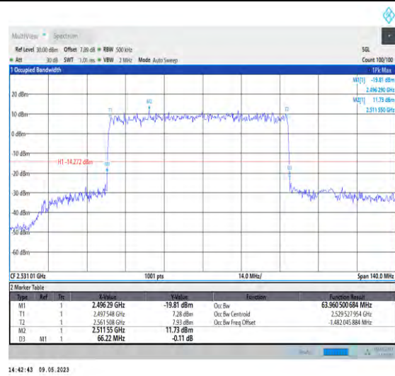
1-N41-PC3-30-70-L-3-DFT-16QAM-Outer_Full-180 @0-Ant1-63.961-66.220-≤70-PASS
