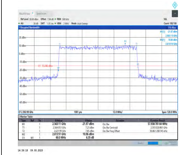
1-N41-PC3-30-60-M-6-CP-QPSK-Outer_Full-162@0 -Ant1-57.939-60.000-≤60-PASS
