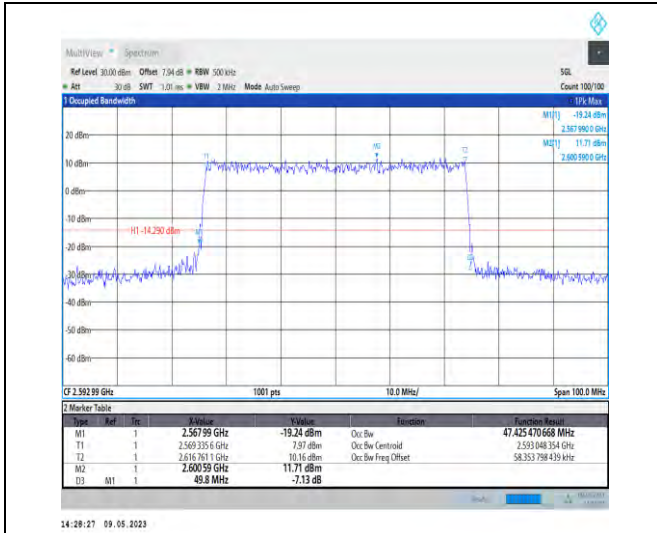
1-N41-PC3-30-50-M-7-CP-16QAM-Outer_Full-133@ 0-Ant1-47.425-49.800-≤50-PASS
