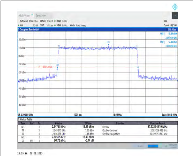
1-N41-PC3-30-90-M-7-CP-16QAM-Outer_Full-245@ 0-Ant1-87.522-90.720-≤90-PASS
