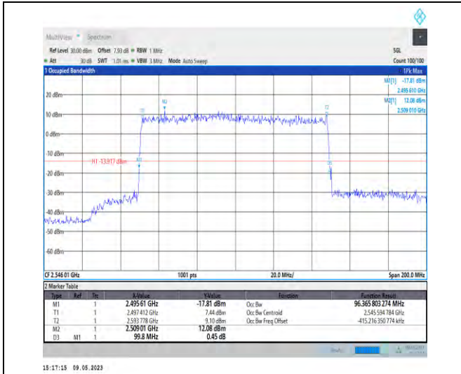
1-N41-PC3-30-100-L-5-DFT-256QAM-Outer_Full-27@0-Ant1-96.366-99.800-≤100-PASS
