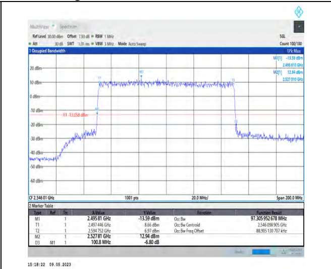
1-N41-PC3-30-100-L-6-CP-QPSK-Outer_Full-273@0-Ant1-97.306-100.800-≤100-PASS
