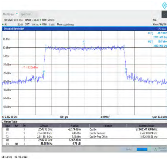
1-N41-PC3-30-40-M-8-CP-64QAM-Outer_Full-106@ 0-Ant1-37.843-39.680-≤40-PASS
