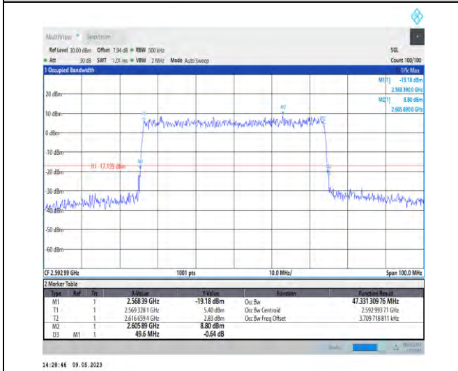
1-N41-PC3-30-50-M-9-CP-256QAM-Outer_Full-133 @0-Ant1-47.331-49.600-≤50-PASS
