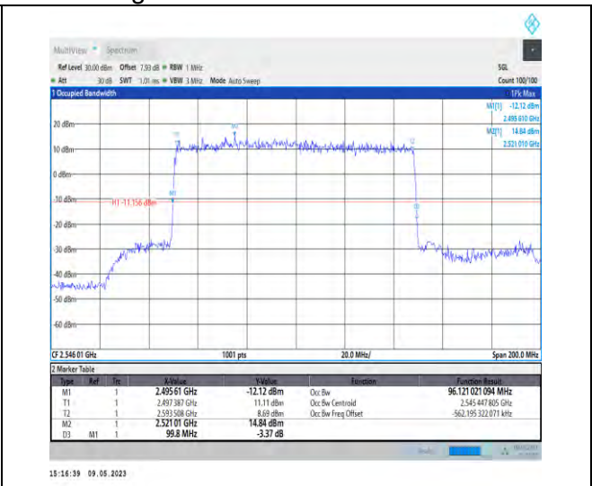
1-N41-PC3-30-100-L-2-DFT-PI2BPSK-Outer_Full-270@0-Ant1-96.121-99.800-≤100-PASS
