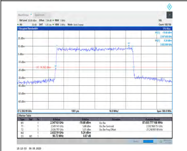
1-N41-PC3-30-90-M-9-CP-256QAM-Outer_Full-245 @0-Ant1-87.656-90.720-≤90-PASS
