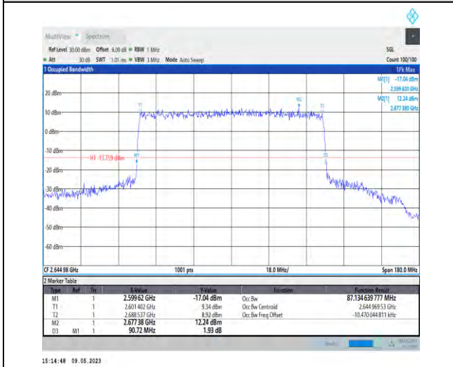
1-N41-PC3-30-90-H-8-CP-64QAM-Outer_Full-245@0-Ant1-87.135-90.720-<=90-PASS
