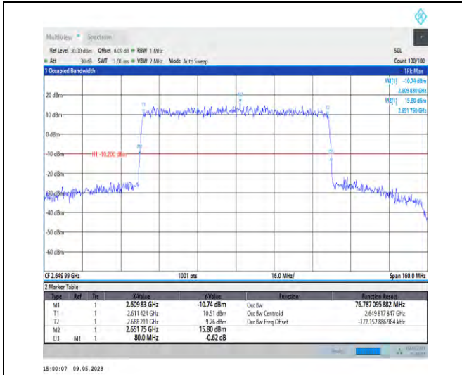
1-N41-PC3-30-80-H-1-DFT-QPSK-Outer_Full-216@0-Ant1-76.787-80.000-≤80-PASS
