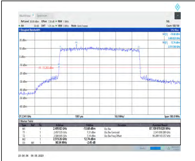
1-N41-PC3-30-90-L-8-CP-64QAM-Outer_Full-245@ 0-Ant1-87.11-90.540-≤90-PASS
