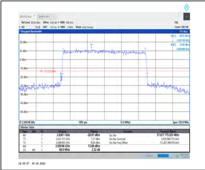
1-N41-PC3-30-60-H-3-DFT-16QAM-Outer_Full-162 @0-Ant1-57.672-60.000-≤60-PASS
