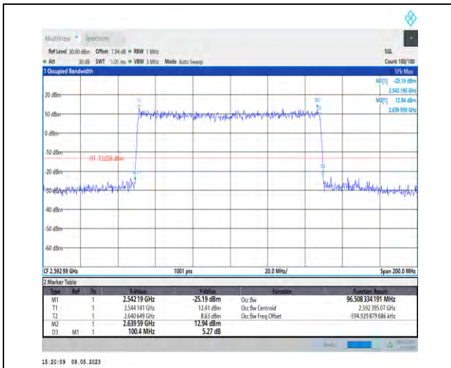
1-N41-PC3-30-100-M-4-DFT-64QAM-Outer_Full-270 @0-Ant1-96.508-100.400-≤100-PASS
