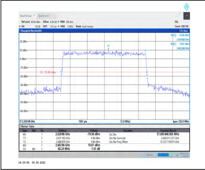
1-N41-PC3-30-60-H-5-DFT-256QAM-Outer_Full-162 @0-Ant1-57.696-60.240-≤60-PASS
