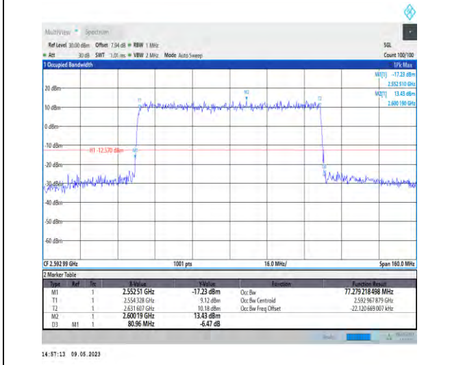
1-N41-PC3-30-80-M-4-DFT-64QAM-Outer_Full-216 @0-Ant1-77.279-80.960-≤80-PASS
