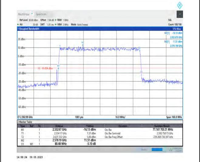
1-N41-PC3-30-80-M-5-DFT-256QAM-Outer_Full-216 @0-Ant1-77.162-80.480-≤80-PASS
