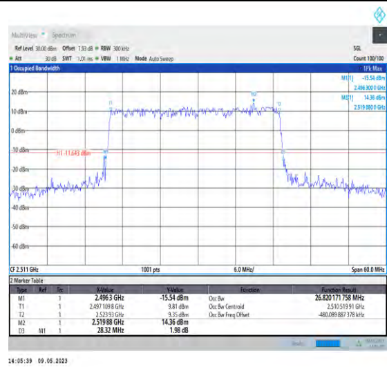
1-N41-PC3-30-30-L-3-DFT-16QAM-Outer_Full-75 @0-Ant1-26.82-28.320-≤30-PASS
