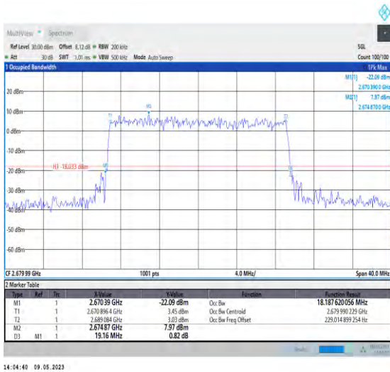
1-N41-PC3-30-20-H-9-CP-256QAM-Outer_Full-51@0 0-Ant1-18.188-19.160-≤20-PASS
