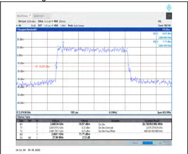
1-N41-PC3-30-30-H-5-DFT-256QAM-Outer_Full-75 @0-Ant1-26.731-27.960-≤30-PASS
