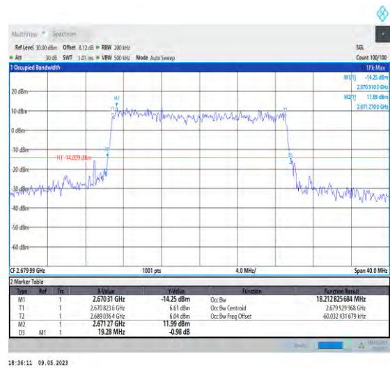
1-N41-PC3-30-20-H-8-CP-64QAM-Outer_Full-51@0 -Ant1-18.213-19.280-≤20-PASS
