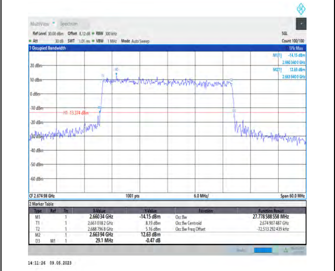
1-N41-PC3-30-30-H-7-CP-16QAM-Outer_Full-78@0- -Ant1-27.779-29.100-≤30-PASS
