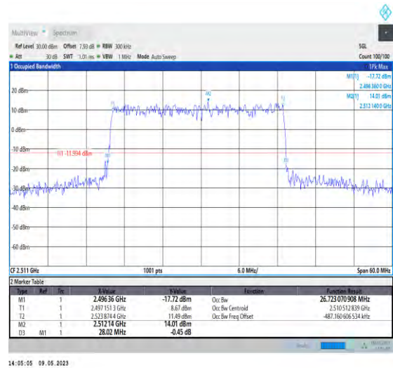
1-N41-PC3-30-30-L-1-DFT-QPSK-Outer_Full-75@0- Ant1-26.723-28.020-≤30-PASS
