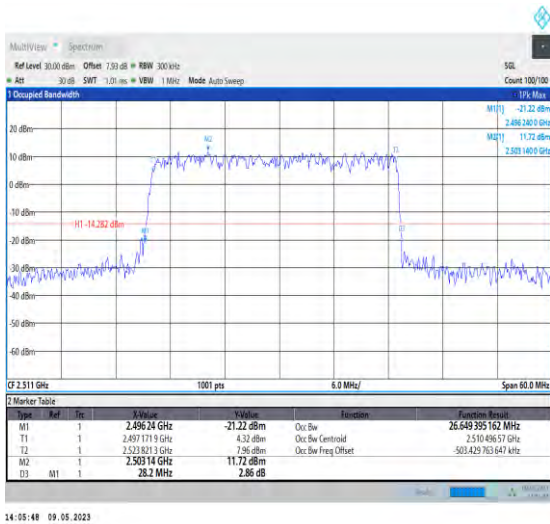
1-N41-PC3-30-30-L-4-DFT-64QAM-Outer_Full-75 @0-Ant1-26.649-28.200-≤30-PASS
