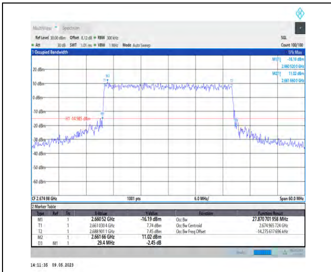
1-N41-PC3-30-30-H-8-CP-64QAM-Outer_Full-78@0 -Ant1-27.871-29.400-≤30-PASS
