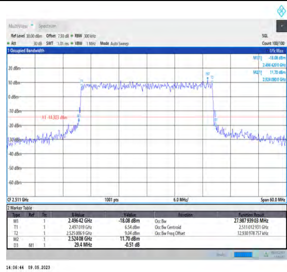
1-N41-PC3-30-30-L-7-CP-16QAM-Outer_Full-78@0-A Ant1-27.988-29.400-≤30-PASS
