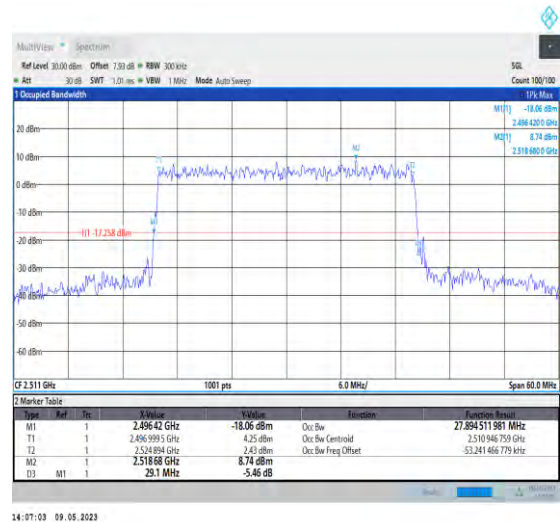
1-N41-PC3-30-30-L-9-CP-256QAM-Outer_Full-78@0-A Ant1-27.895-29.100-≤30-PASS
