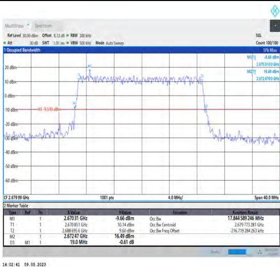
1-N41-PC3-30-20-H-1-DFT-QPSK-Outer_Full-50@0- Ant1-17.845-19.000-≤20-PASS
