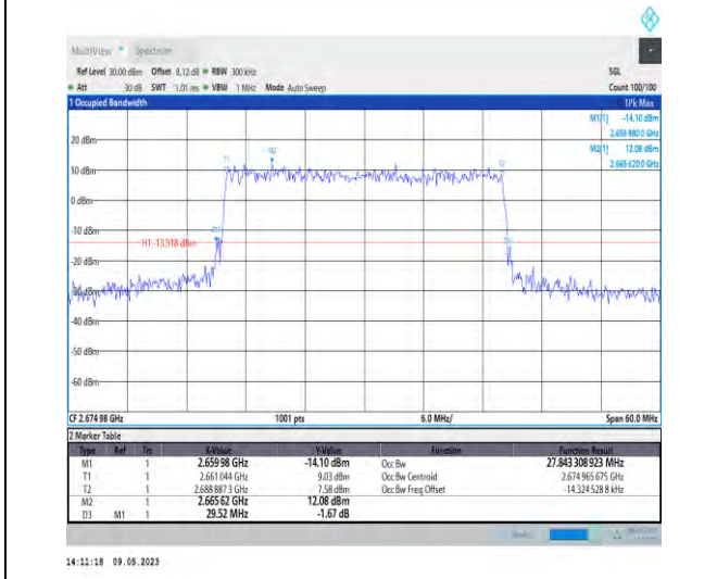
1-N41-PC3-30-30-H-6-CP-QPSK-Outer_Full-78@0- Ant1-27.843-29.520-≤30-PASS
