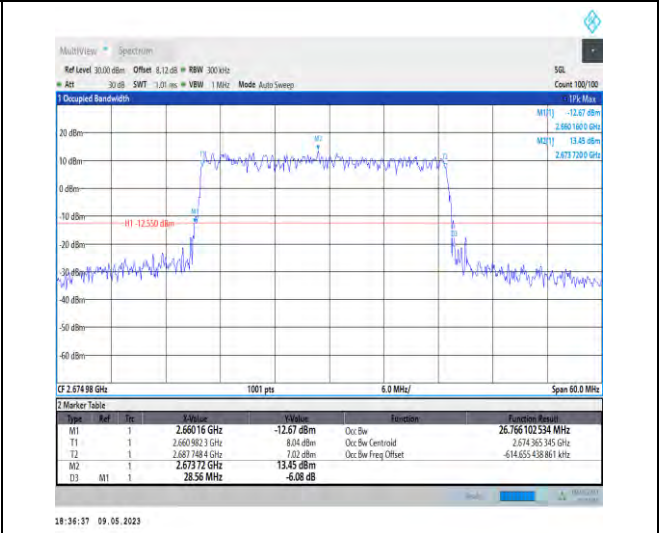
1-N41-PC3-30-30-H-3-DFT-16QAM-Outer_Full-75@ 0-Ant1-26.766-28.560-≤30-PASS
