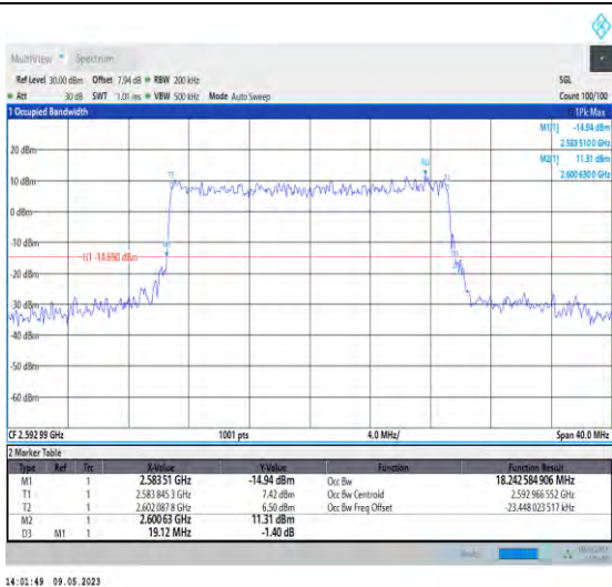
1-N41-PC3-30-20-M-8-CP-64QAM-Outer_Full-51@0 -Ant1-18.243-19.120-≤20-PASS
