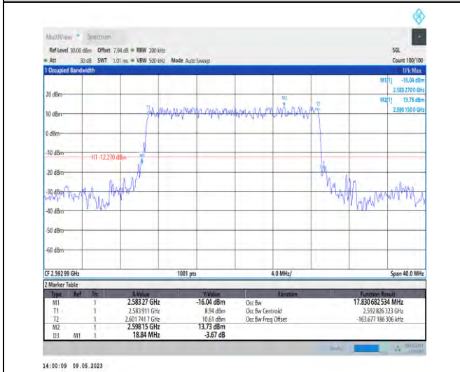
1-N41-PC3-30-20-M-2-DFT-PI2BPSK-Outer_Full-50@ 0-Ant1-17.831-18.840-<20-PASS
