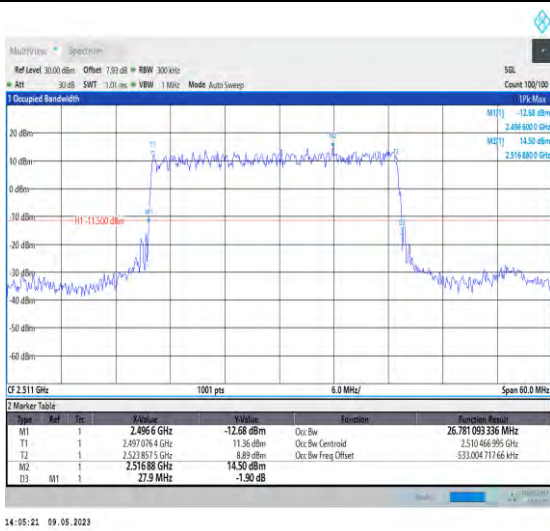
1-N41-PC3-30-30-L-2-DFT-PI2BPSK-Outer_Full-75 @0-Ant1-26.781-27.900-≤30-PASS
