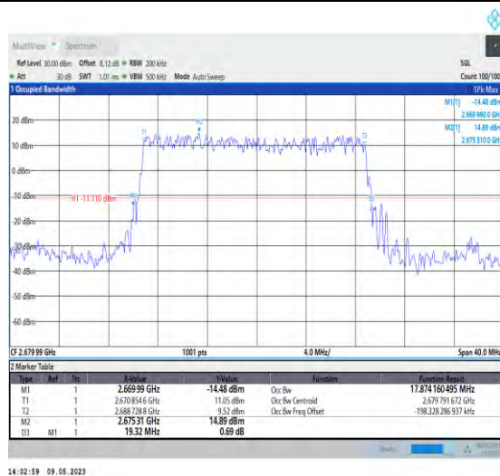
1-N41-PC3-30-20-H-2-DFT-PI2BPSK-Outer_Full-50 @0-Ant1-17.874-19.320-≤20-PASS
