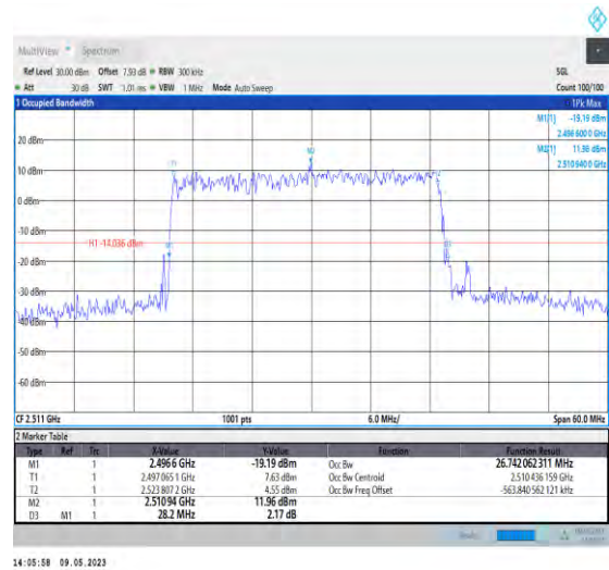
1-N41-PC3-30-30-L-5-DFT-256QAM-Outer_Full-75 @0-Ant1-26.742-28.200-≤30-PASS
