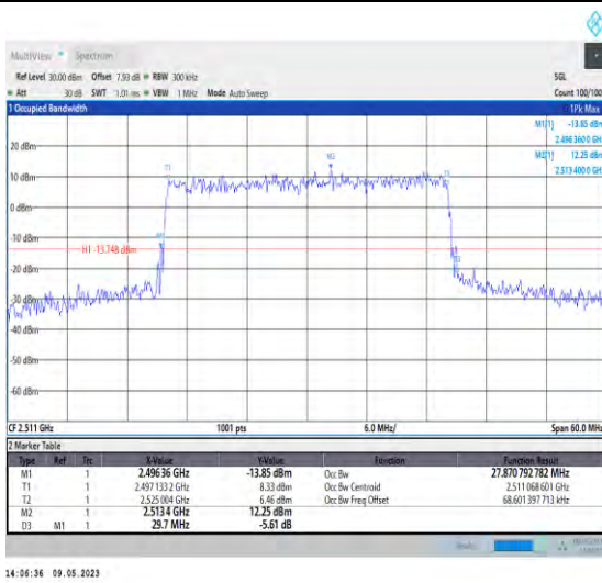
1-N41-PC3-30-30-L-6-CP-QPSK-Outer_Full-78@0-A nt1-27.871-29.700-≤30-PASS
