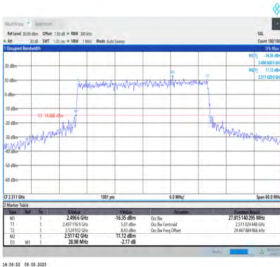
1-N41-PC3-30-30-L-8-CP-64QAM-Outer_Full-78@0-A Ant1-27.815-28.980-≤30-PASS
