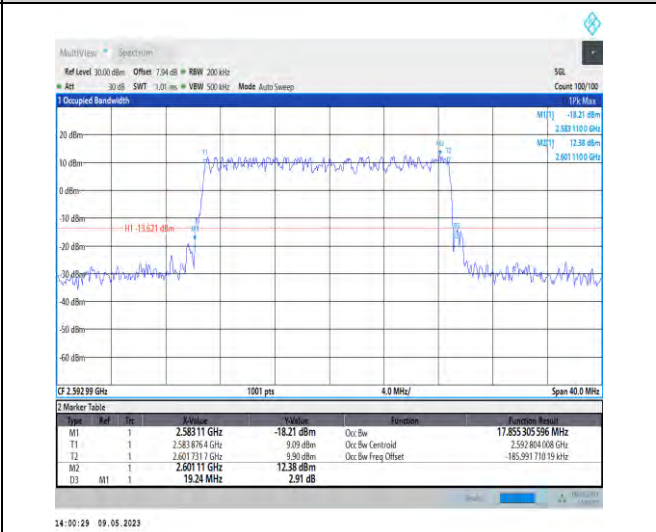
1-N41-PC3-30-20-M-3-DFT-16QAM-Outer_Full-50@ 0-Ant1-17.855-19.240-<20-PASS
