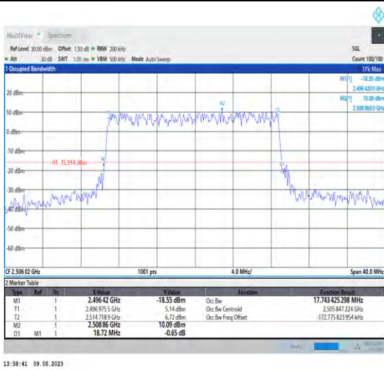
1-N41-PC3-30-20-L-5-DFT-256QAM-Outer_Full-50 @0-Ant1-17.743-18.720-≤20-PASS
