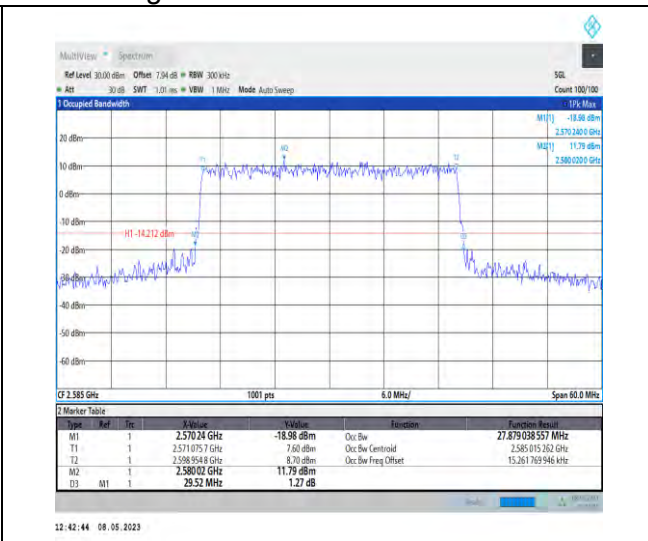
1-N38-PC3-30-30-L-7-CP-16QAM-Outer_Full-78@0- Ant1-27.879-29.520-≤30-PASS
