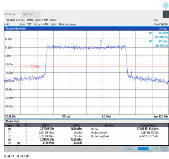
1-N38-PC3-30-40-L-6-CP-QPSK-Outer_Full-106@0-Ant1-37.897-39.680-≤40-PASS
