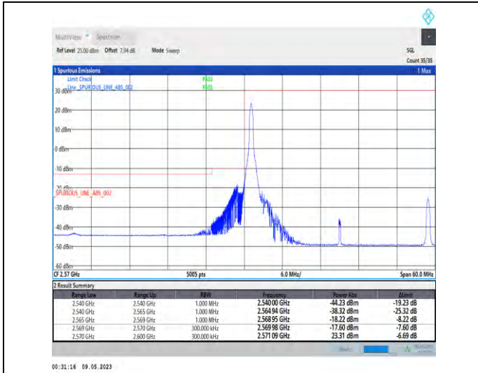
1-N38-PC3-30-30-L-1-DFT-PI2BPSK-Edge_1RB_Left-1@0-Ant1-1--PASS-see graph
