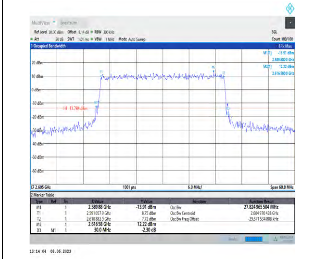
1-N38-PC3-30-30-H-6-CP-QPSK-Outer_Full-78@0- Ant1-27.825-30.000-<30-PASS
