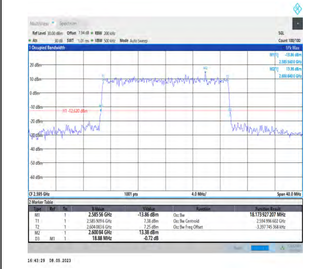
1-N38-PC3-30-20-M-7-CP-16QAM-Outer_Full-51@0- -Ant1-18.174-18.880-≤20-PASS
