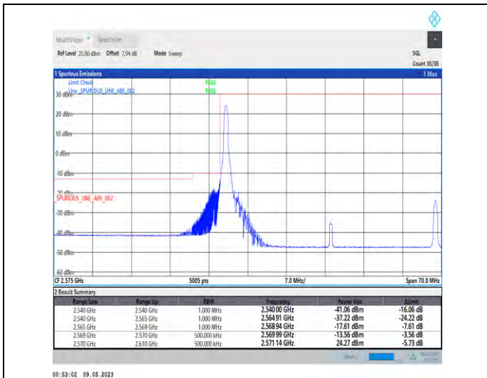
1-N38-PC3-30-40-L-1-DFT-PI2BPSK-Edge_1RB_Left-1@0-Ant1-1--PASS-see graph
