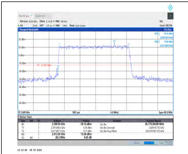
1-N38-PC3-30-30-H-4-DFT-64QAM-Outer_Full-75@ 0-Ant1-26.779-28.200-<30-PASS
