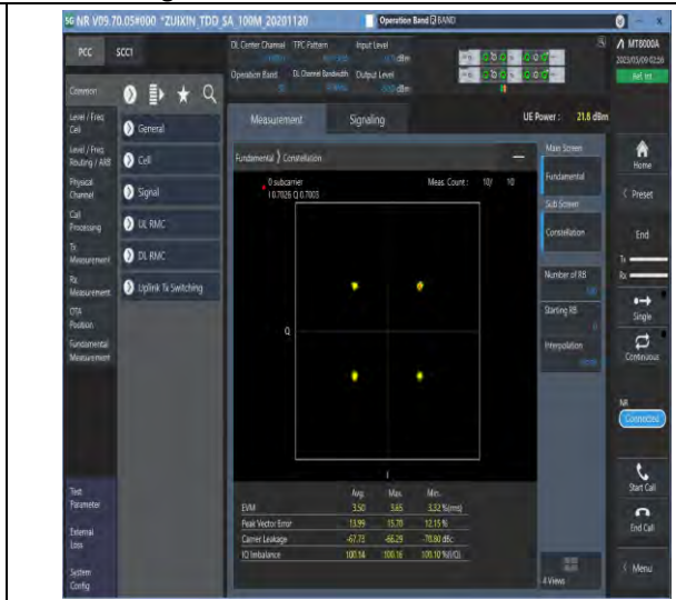
1-N38-PC3-30-40-M-6-CP-QPSK-Outer_Full-106@0-Ant1-see graph-PASS
