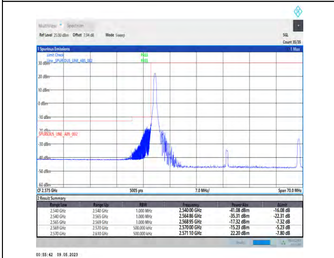
1-N38-PC3-30-40-L-4-CP-QPSK-Edge_1RB_Left-1@0-Ant1-1--PASS-see graph
