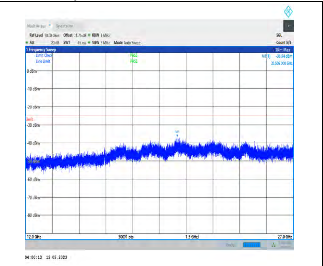
1-N38-PC3-30-40-H-1-DFT-PI2BPSK-Inner_1RB_Lef t-1@1-12000-27000-Ant1-20506.00--36.94--25-PASS
