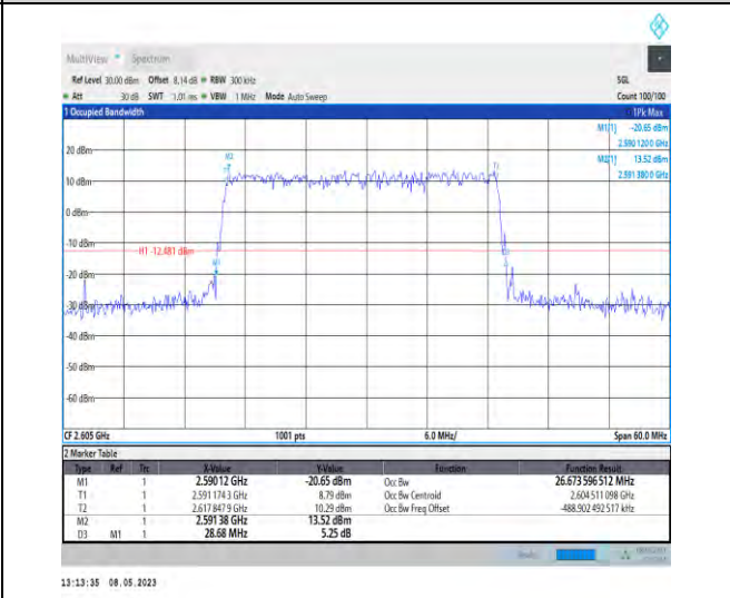
1-N38-PC3-30-30-H-3-DFT-16QAM-Outer_Full-75@ 0-Ant1-26.674-28.680-<30-PASS
