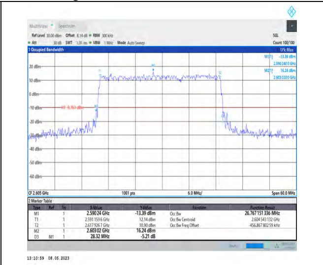
1-N38-PC3-30-30-H-1-DFT-QPSK-Outer_Full-75@ -Ant1-26.767-28.320-<30-PASS
