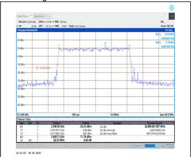
1-N38-PC3-30-30-H-5-DFT-256QAM-Outer_Full-75 @0-Ant1-26.807-28.320-<30-PASS
