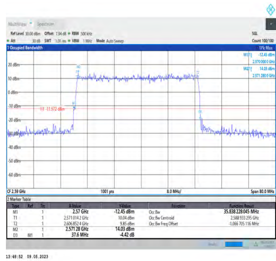
1-N38-PC3-30-40-L-4-DFT-64QAM-Outer_Full-100 @0-Ant1-35.838-37.600-≤40-PASS
