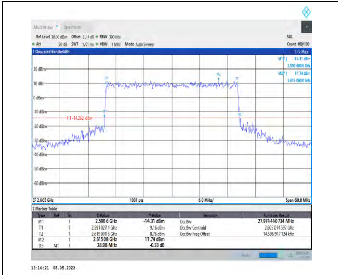
1-N38-PC3-30-30-H-8-CP-64QAM-Outer_Full-78@0 -Ant1-27.974-28.980-≤30-PASS
