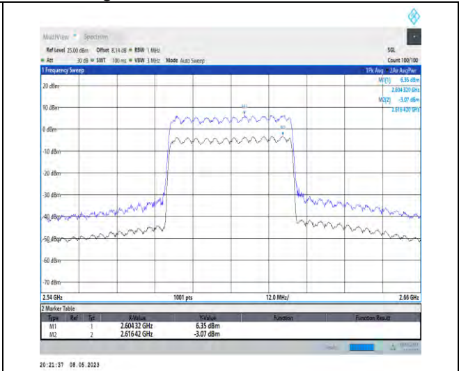
1-N38-PC3-30-40-H-2-CP-256QAM-Outer_Full-106 @0-Ant1-9.42-100%-0.00-9.42-PASS-≤13
