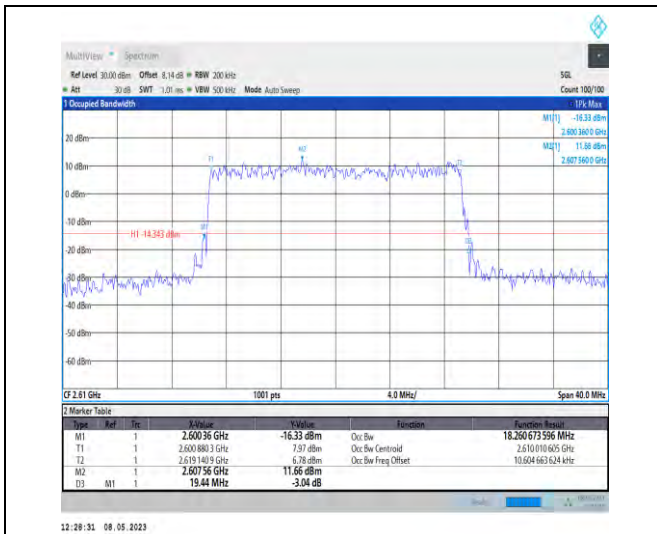
1-N38-PC3-30-20-H-7-CP-16QAM-Outer_Full-51@0 -Ant1-18.261-19.440-≤20-PASS
