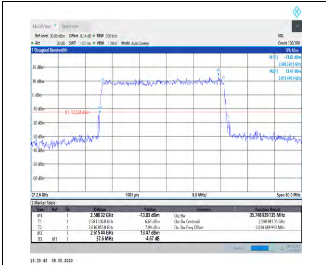
1-N38-PC3-30-40-H-5-DFT-256QAM-Outer_Full-100 @0-Ant1-35.749-37.600-≤40-PASS
