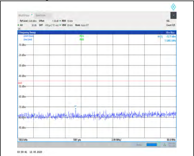
1-N38-PC3-30-40-H-1-DFT-PI2BPSK-Inner_1RB_Lef t-1@1-0.15-30-Ant1-11.05--72.77--45-PASS
