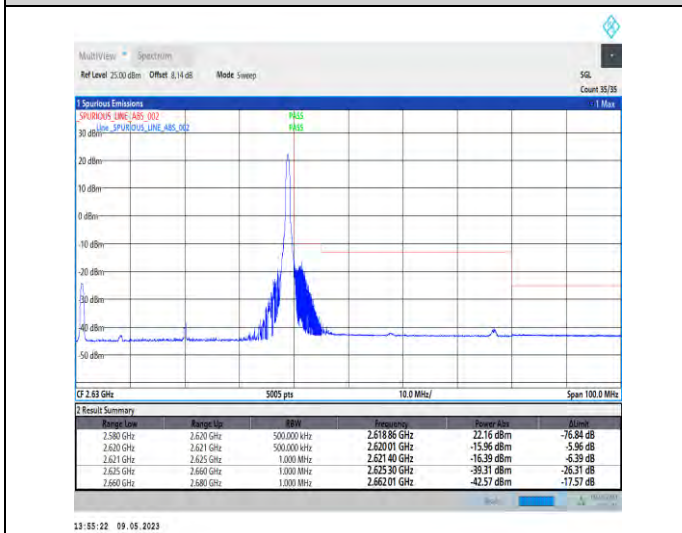
1-N38-PC3-30-40-H-5-CP-QPSK-Edge_1RB_Right-1 @105-Ant1-1--PASS-see graph
