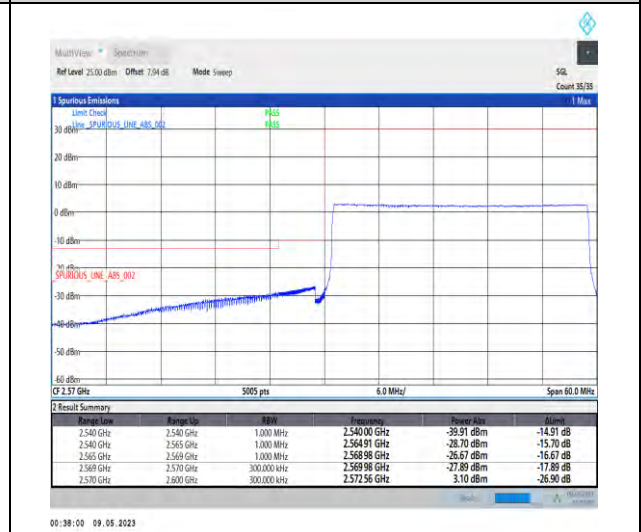
1-N38-PC3-30-30-L-6-CP-QPSK-Outer_Full-78@0-Ant1-1--PASS-see graph
