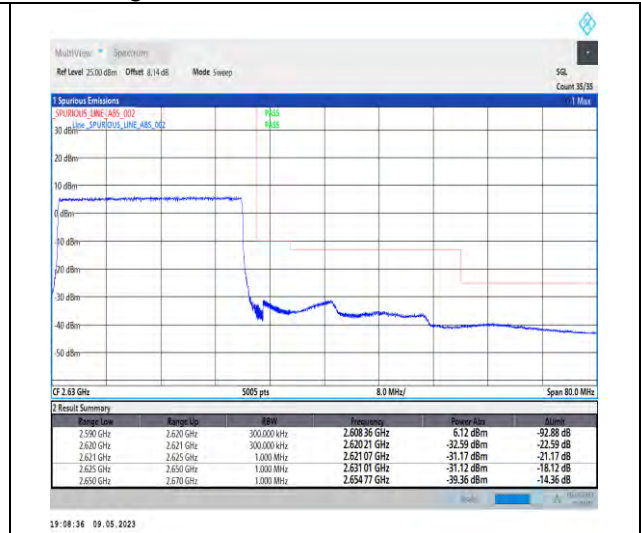
1-N38-PC3-30-30-H-3-DFT-PI2BPSK-Outer_Full-75@0-Ant1-1--PASS-see graph
