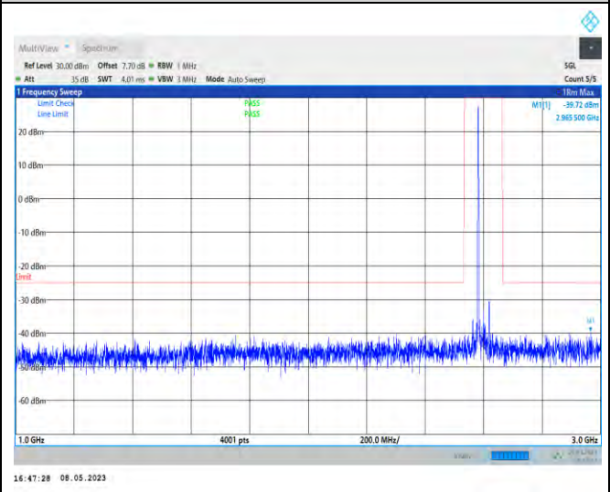
1-N38-PC3-30-40-H-1-DFT-PI2BPSK-Inner_1RB_Lef t-1@1-1000-3000-Ant1-2181.00--38.88--25-PASS
