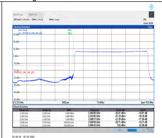
1-N38-PC3-30-40-L-3-DFT-PI2BPSK-Outer_Full-100@0-Ant1-1--PASS-see graph
