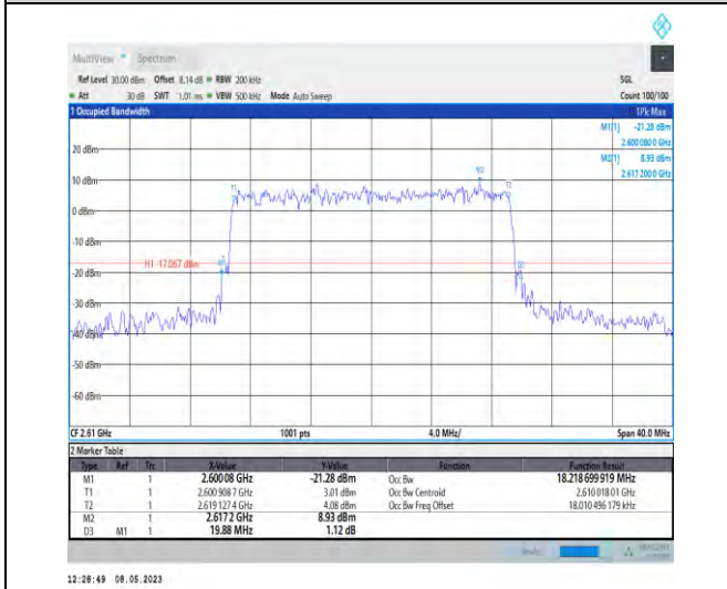
1-N38-PC3-30-20-H-9-CP-256QAM-Outer_Full-51@0 0-Ant1-18.219-19.880-≤20-PASS
