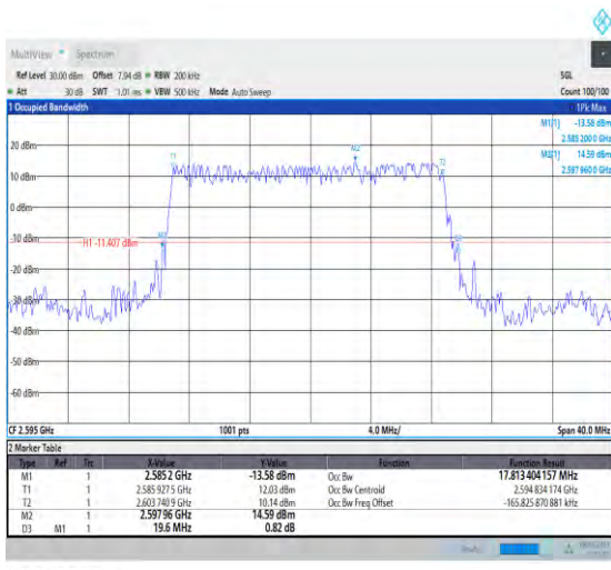
1-N38-PC3-30-20-M-2-DFT-PI2BPSK-Outer_Full-50@ 0-Ant1-17.813-19.600-<20-PASS
