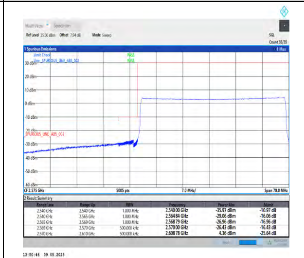
1-N38-PC3-30-40-L-6-CP-QPSK-Outer_Full-106@0-Ant1-1--PASS-see graph
