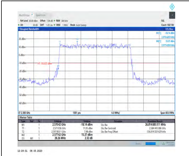
1-N38-PC3-30-30-L-2-DFT-PI2BPSK-Outer_Full-75 @0-Ant1-26.814-28.260-≤30-PASS
