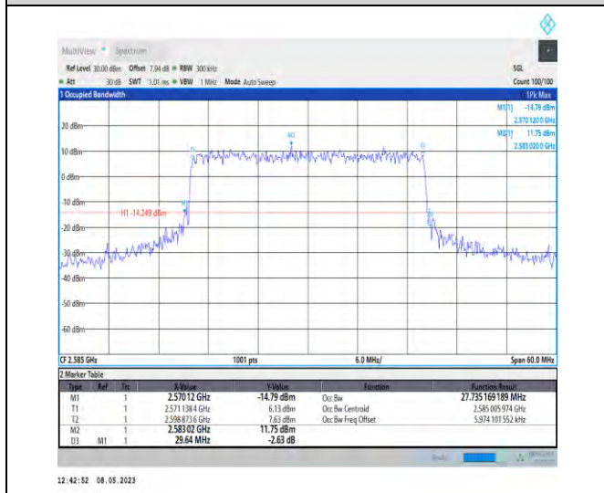
1-N38-PC3-30-30-L-8-CP-64QAM-Outer_Full-78@0- Ant1-27.735-29.640-≤30-PASS
