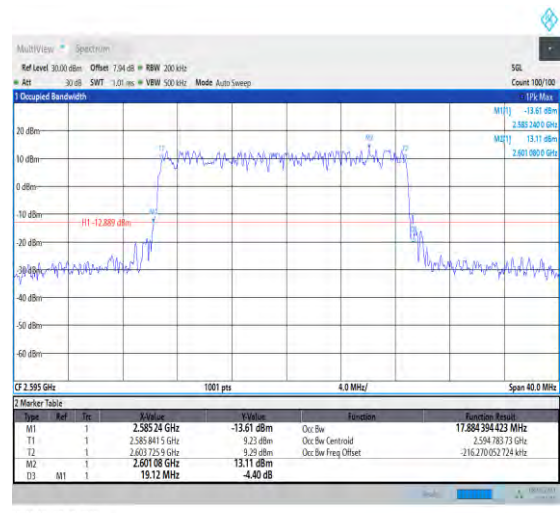
1-N38-PC3-30-20-M-3-DFT-16QAM-Outer_Full-50@ 0-Ant1-17.884-19.120-<20-PASS
