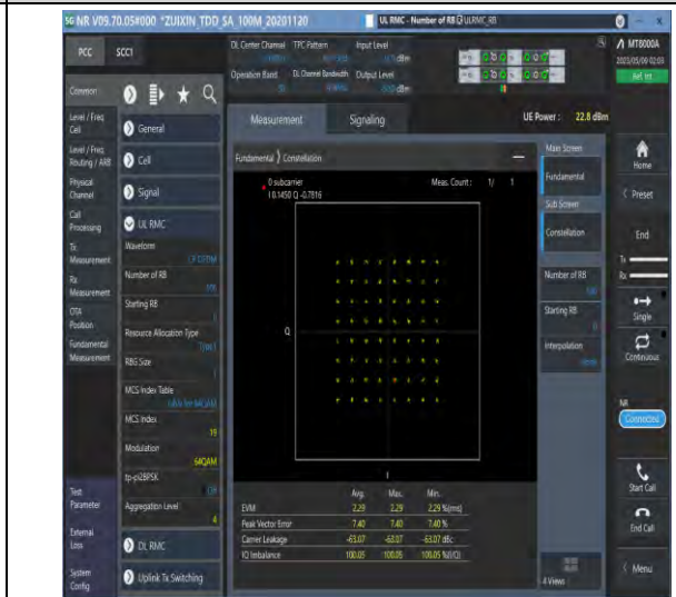
1-N38-PC3-30-40-M-8-CP-64QAM-Outer_Full-106@0-Ant1-see graph-PASS
