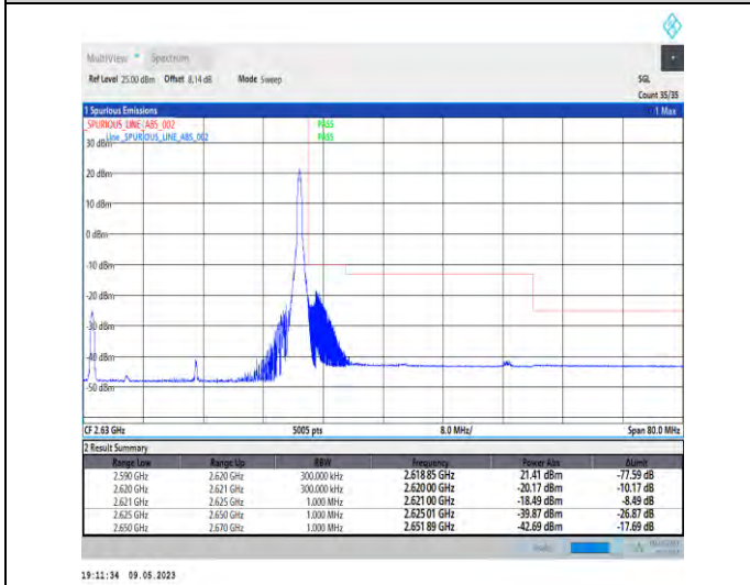
1-N38-PC3-30-30-H-5-CP-QPSK-Edge_1RB_Right-1@77-Ant1-1--PASS-see graph
