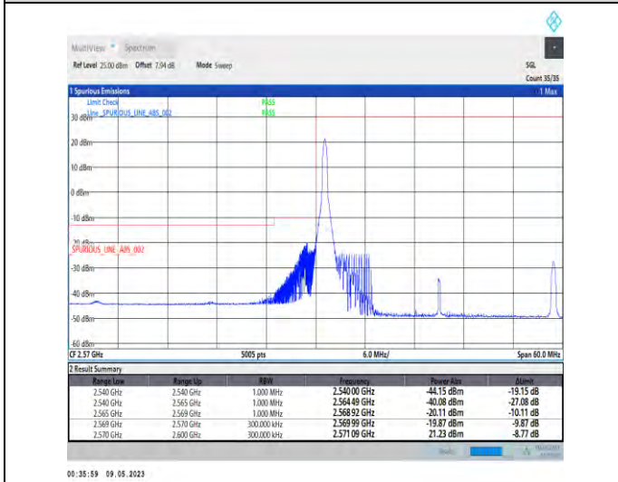
1-N38-PC3-30-30-L-4-CP-QPSK-Edge_1RB_Left-1@0-Ant1-1--PASS-see graph
