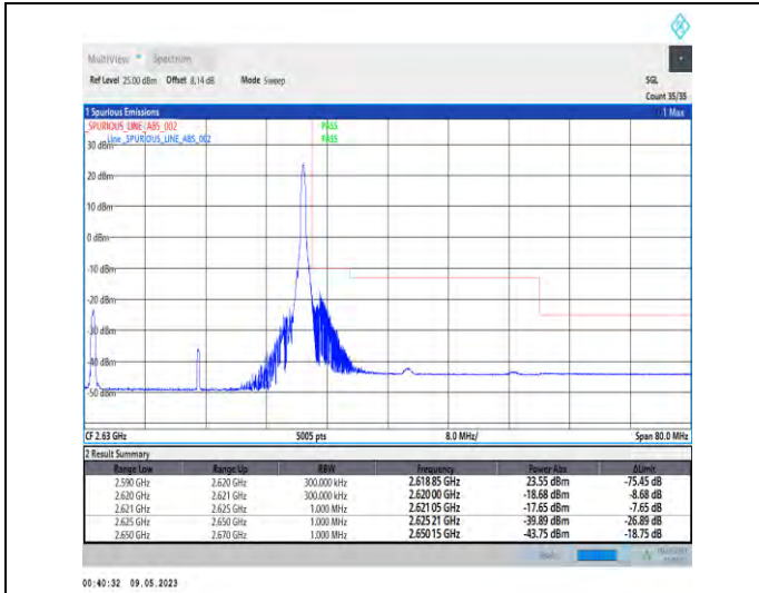
1-N38-PC3-30-30-H-2-DFT-PI2BPSK-Edge_1RB_Right-t-1@77-Ant1-1--PASS-see graph
