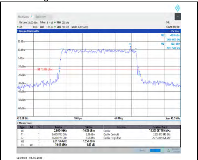
1-N38-PC3-30-20-H-8-CP-64QAM-Outer_Full-51@0 -Ant1-18.207-19.440-≤20-PASS
