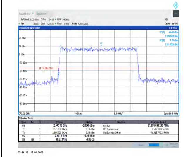
1-N38-PC3-30-40-L-9-CP-256QAM-Outer_Full-106 @0-Ant1-37.891-39.920-≤40-PASS
