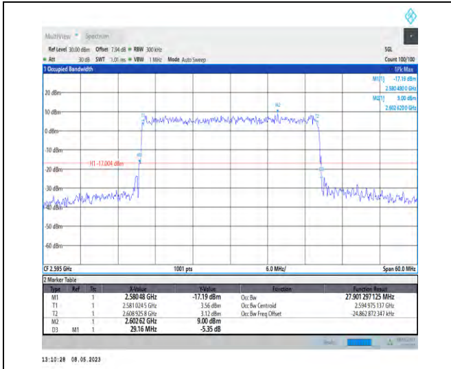
1-N38-PC3-30-30-M-9-CP-256QAM-Outer_Full-78@ 0-Ant1-27.901-29.160-<30-PASS
