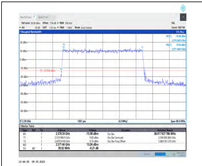
1-N38-PC3-30-40-L-7-CP-16QAM-Outer_Full-106@ 0-Ant1-38.018-39.920-≤40-PASS
