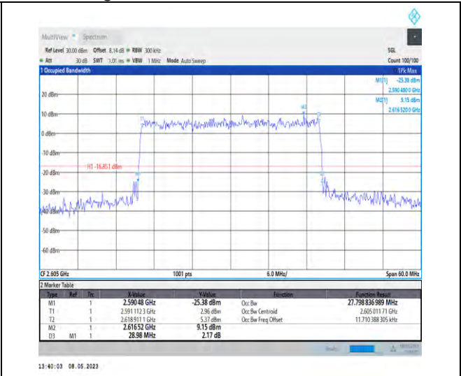
1-N38-PC3-30-30-H-9-CP-256QAM-Outer_Full-78@0 -Ant1-27.799-28.980-≤30-PASS
