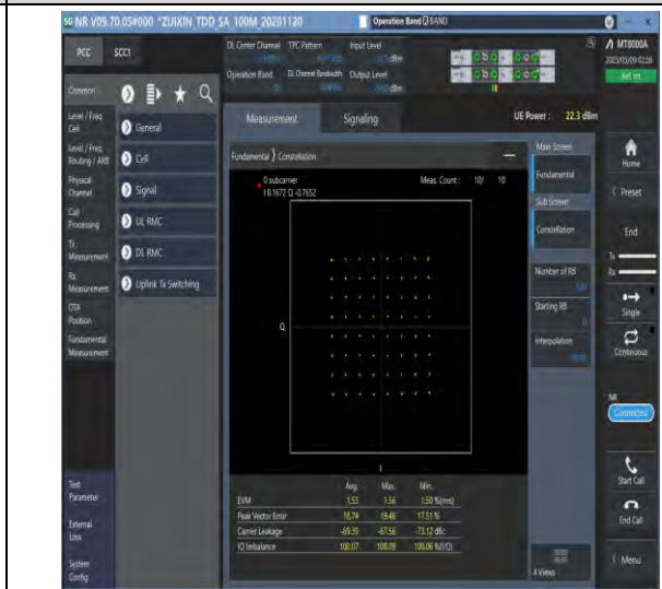
1-N38-PC3-30-40-M-4-DFT-64QAM-Outer_Full-100 @0-Ant1-see graph-PASS
