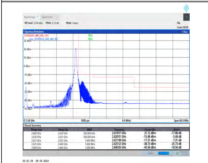
1-N38-PC3-30-20-H-5-CP-QPSK-Edge_1RB_Righ t-1@50-Ant1-1--PASS-see graph
