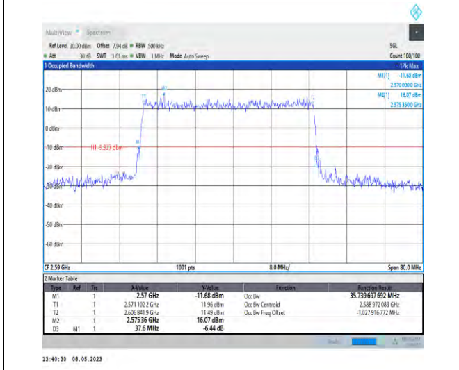
1-N38-PC3-30-40-L-1-DFT-QPSK-Outer_Full-100@0 -Ant1-35.74-37.600-≤40-PASS
