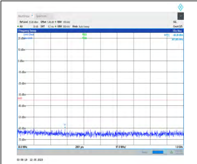
1-N38-PC3-30-40-M-1-DFT-PI2BPSK-Inner_1RB_L eft-1@1-30-1000-Ant1-307.91--60.28--35-PASS
