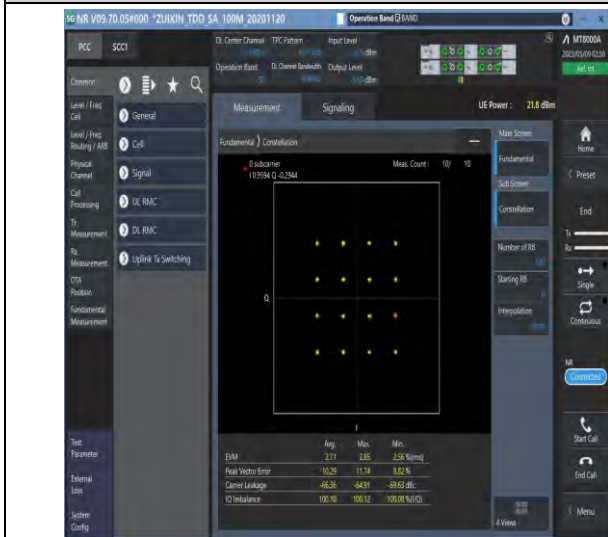
1-N38-PC3-30-40-M-7-CP-16QAM-Outer_Full-106@0-Ant1-see graph-PASS
