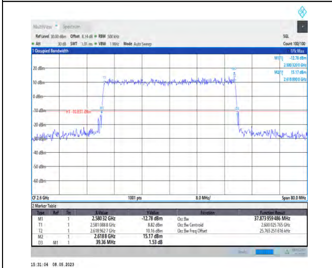
1-N38-PC3-30-40-H-7-CP-16QAM-Outer_Full-106@0-Ant1-37.874-39.360-≤40-PASS
