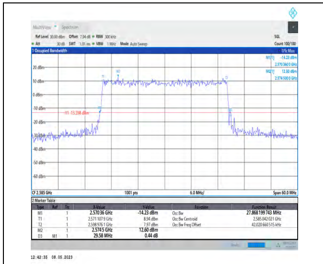
1-N38-PC3-30-30-L-6-CP-QPSK-Outer_Full-78@0-A Ant1-27.868-29.580-≤30-PASS
