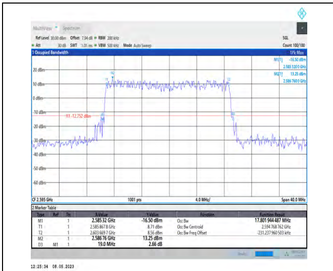
1-N38-PC3-30-20-M-4-DFT-64QAM-Outer_Full-50@ 0-Ant1-17.802-19.000-≤20-PASS
