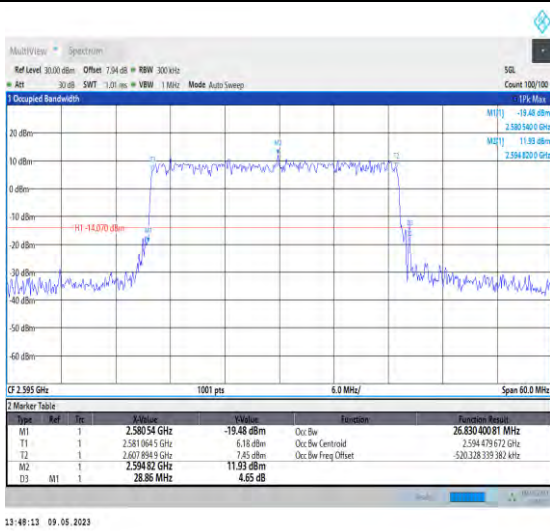
1-N38-PC3-30-30-M-5-DFT-256QAM-Outer_Full-75@0-Ant1-26.83-28.860-≤30-PASS
