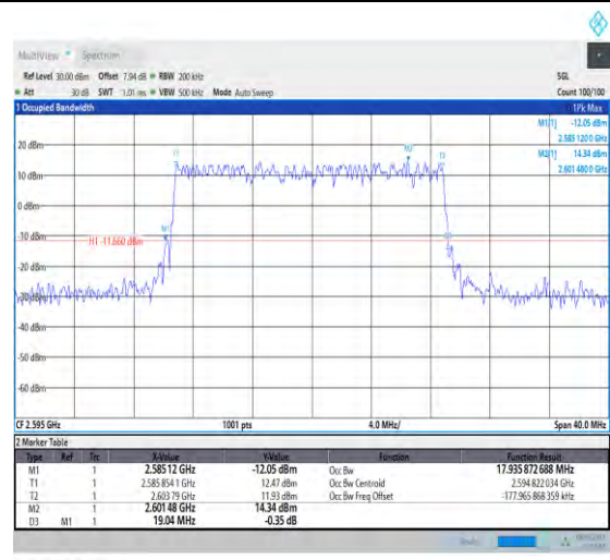
1-N38-PC3-30-20-M-1-DFT-QPSK-Outer_Full-50@ 0-Ant1-17.936-19.040-<20-PASS
