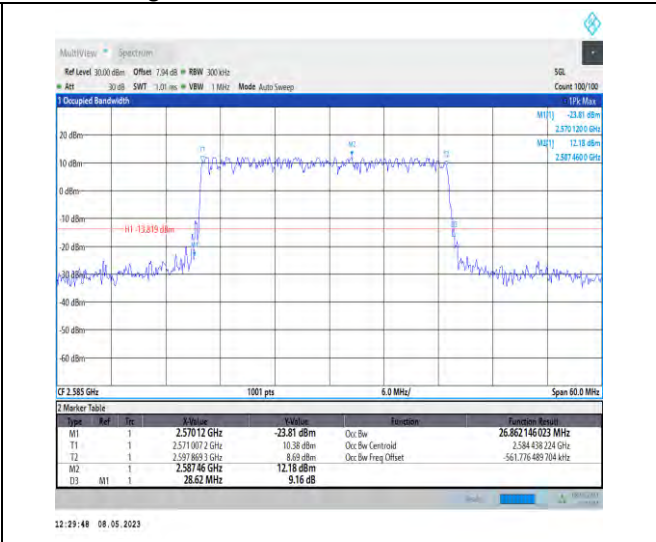
1-N38-PC3-30-30-L-3-DFT-16QAM-Outer_Full-75 @0-Ant1-26.862-28.620-≤30-PASS
