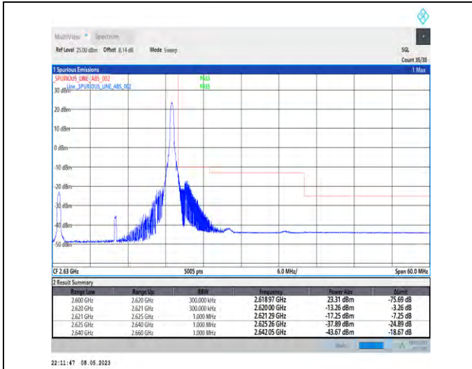
1-N38-PC3-30-20-H-2-DFT-PI2BPSK-Edge_1RB_Righ t-1@50-Ant1-1--PASS-see graph
