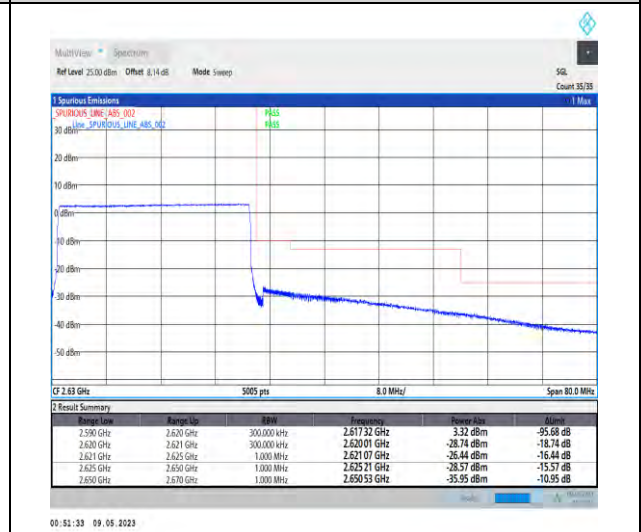
1-N38-PC3-30-30-H-6-CP-QPSK-Outer_Full-78@0-Ant1-1--PASS-see graph
