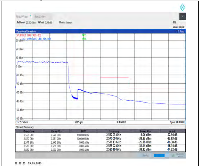
1-N7-PC3-15-10-H-3-DFT-PI2BPSK-Outer_Full-50@0-Ant1-1--PASS-see graph
