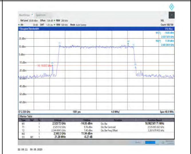
1-N7-PC3-15-20-M-6-CP-QPSK-Outer_Full-106@0- Ant1-18.983-21.280-≤20-PASS
