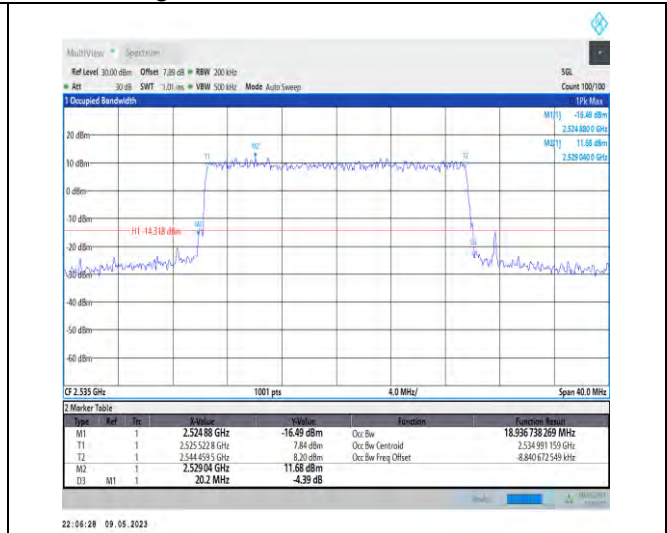
1-N7-PC3-15-20-M-8-CP-64QAM-Outer_Full-106@0 -Ant1-18.937-20.200-≤20-PASS
