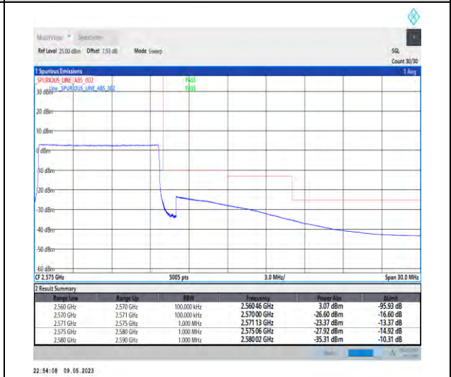
1-N7-PC3-15-10-H-6-CP-QPSK-Outer_Full-52@0-Ant1-1--PASS-see graph
