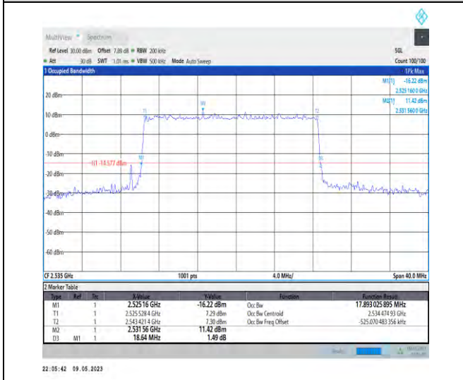
1-N7-PC3-15-20-M-5-DFT-256QAM-Outer_Full-100 @0-Ant1-17.893-18.640-≤20-PASS
