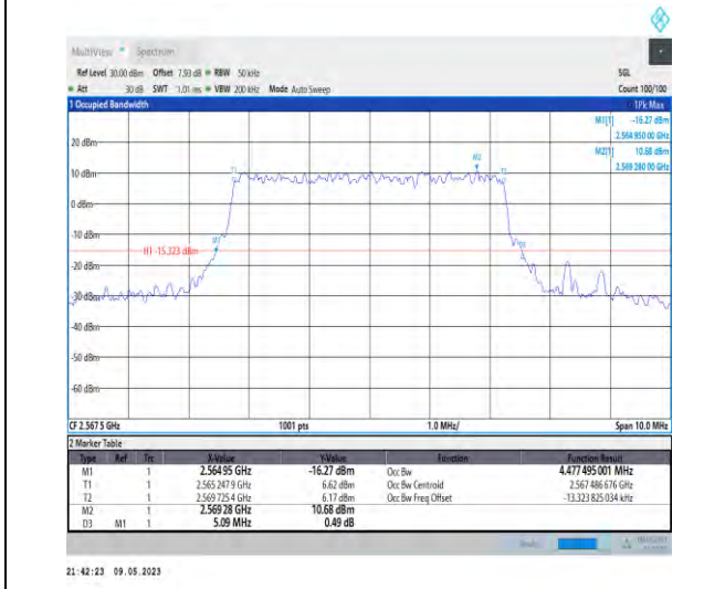
1-N7-PC3-15-5-H-5-DFT-256QAM-Outer_Full-25@0-Ant1-4.477-5.090-≤5-PASS
