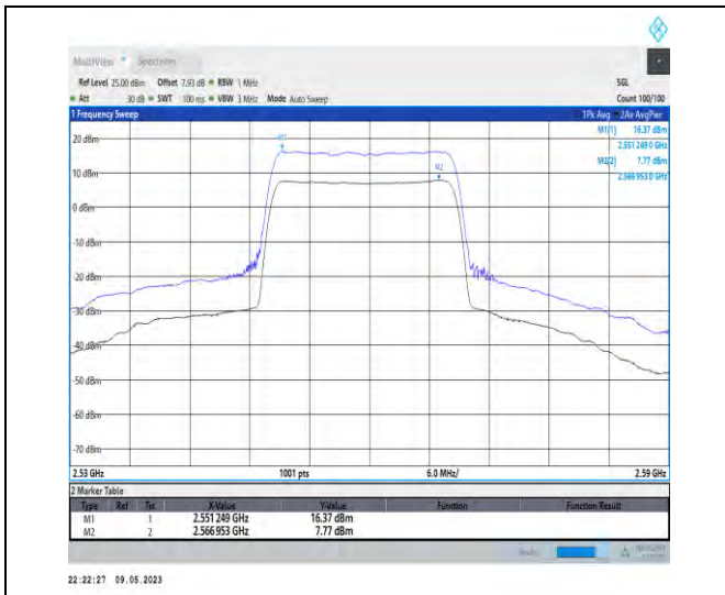
1-N7-PC3-15-20-H-1-DFT-256QAM-Outer_Full-100 @0-Ant1-8.60-100%-0.00-8.60-PASS-≤13
