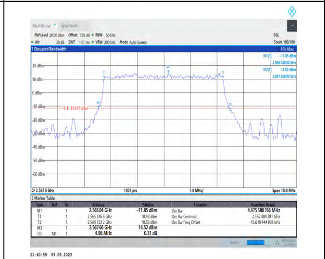
1-N7-PC3-15-5-H-2-DFT-PI2BPSK-Outer_Full-25@0-A -Ant1-4.476-4.960-≤5-PASS
