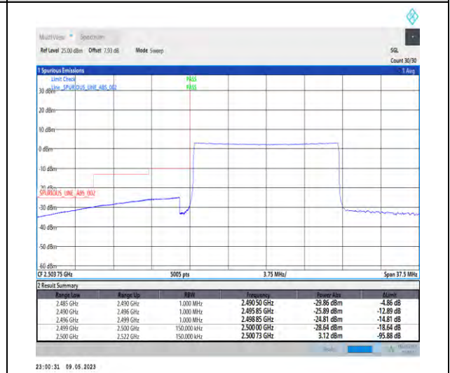
1-N7-PC3-15-15-L-6-CP-QPSK-Outer_Full-79@0-Ant1-1--PASS-see graph
