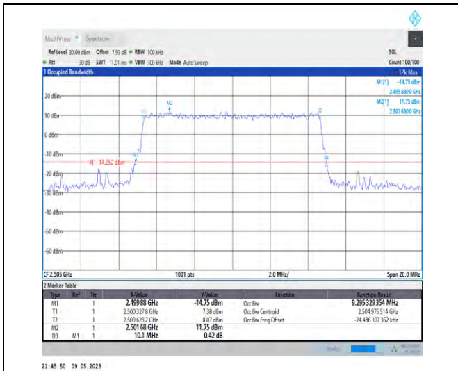
1-N7-PC3-15-10-L-6-CP-QPSK-Outer_Full-52@0-A nt1-9.295-10.100-≤10-PASS
