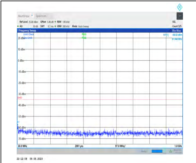
1-N7-PC3-15-20-M-1-DFT-PI2BPSK-Inner_1RB_Lef t-1@1-30-1000-Ant1-31.94--58.53--35-PASS
