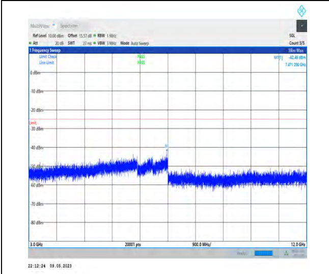
1-N7-PC3-15-20-M-1-DFT-PI2BPSK-Inner_1RB_Lef t-1@1-3000-12000-Ant1-7471.20--42.49--25-PASS
