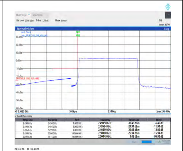
1-N7-PC3-15-10-L-6-CP-QPSK-Outer_Full-52@0-Ant1-1--PASS-see graph
