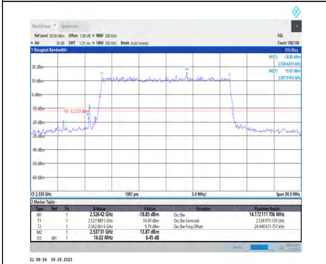
1-N7-PC3-15-15-M-8-CP-64QAM-Outer_Full-79@0- Ant1-14.172-16.020-≤15-PASS
