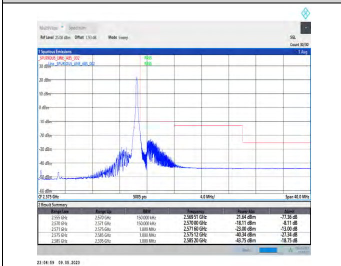
1-N7-PC3-15-15-H-5-CP-QPSK-Edge_1RB_Right-1@78-Ant1-1--PASS-see graph
