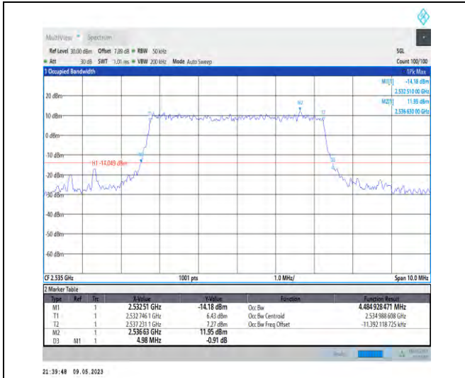
1-N7-PC3-15-5-M-8-CP-64QAM-Outer_Full-25@0-A nt1-4.485-4.980-≤5-PASS
