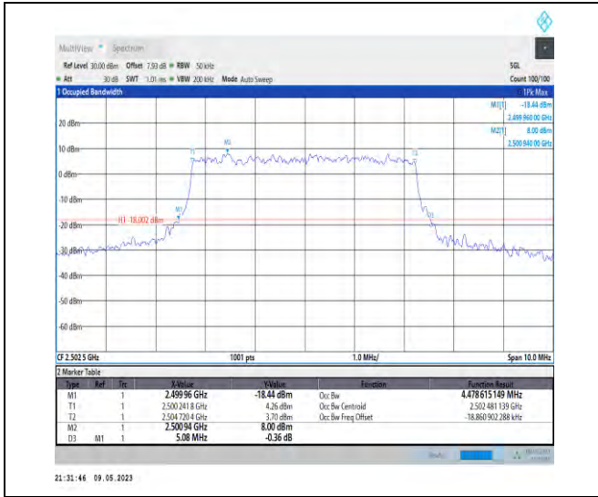
1-N7-PC3-15-5-L-9-CP-256QAM-Outer_Full-25@0-Ant1-4.479-5.080-≤5-PASS
