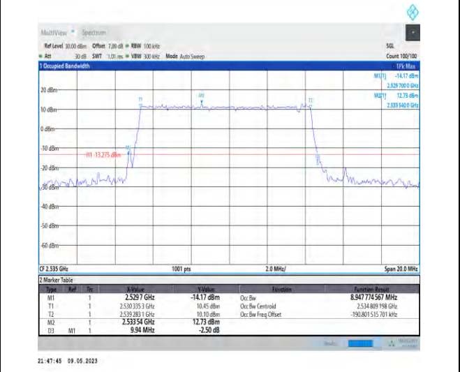
1-N7-PC3-15-10-M-4-DFT-64QAM-Outer_Full-50@0-Ant1-8.948-9.940-≤10-PASS
