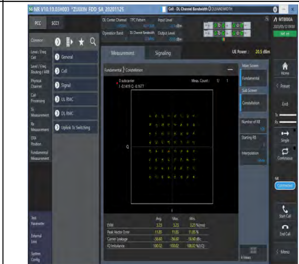
1-N7-PC3-15-20-M-8-CP-64QAM-Outer_Full-106@0-Ant1-see graph-PASS
