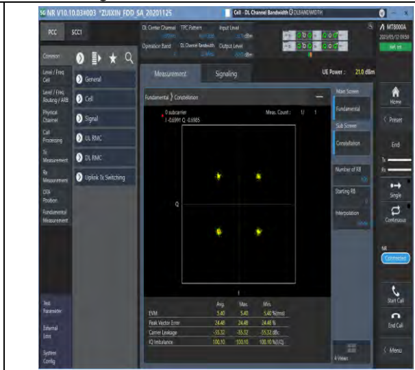
1-N7-PC3-15-20-M-6-CP-QPSK-Outer_Full-106@0-Ant1-see graph-PASS
