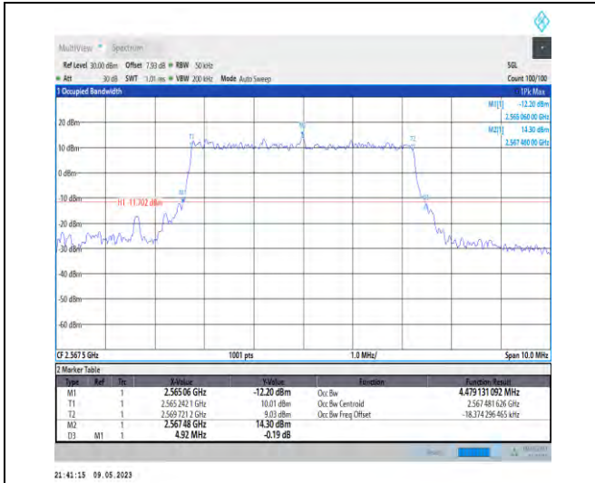
1-N7-PC3-15-5-H-3-DFT-16QAM-Outer_Full-25@0-Ant1-4.479-4.920-≤5-PASS
