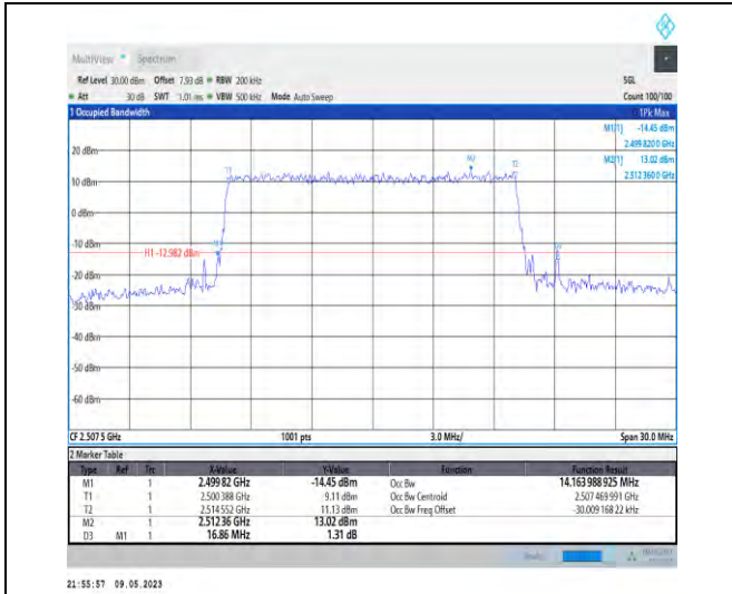
1-N7-PC3-15-15-L-7-CP-16QAM-Outer_Full-79@0-Ant1-14.164-16.860-≤15-PASS
