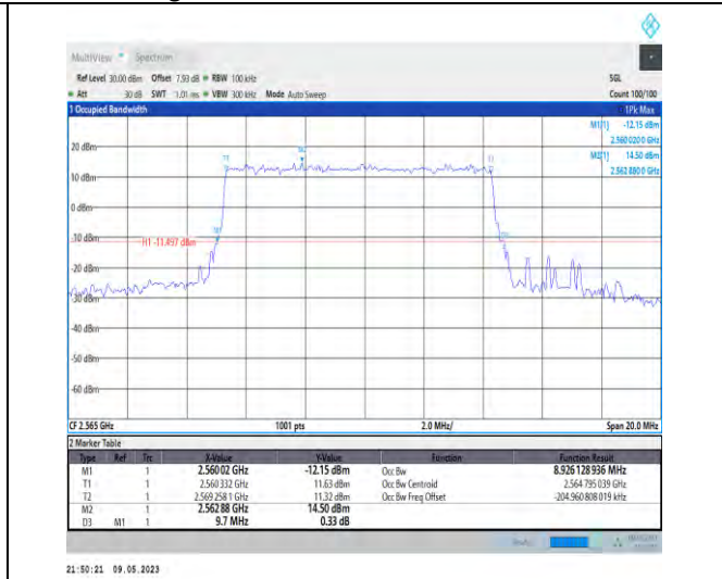
1-N7-PC3-15-10-H-1-DFT-QPSK-Outer_Full-50@0 -Ant1-8.926-9.700-≤10-PASS
