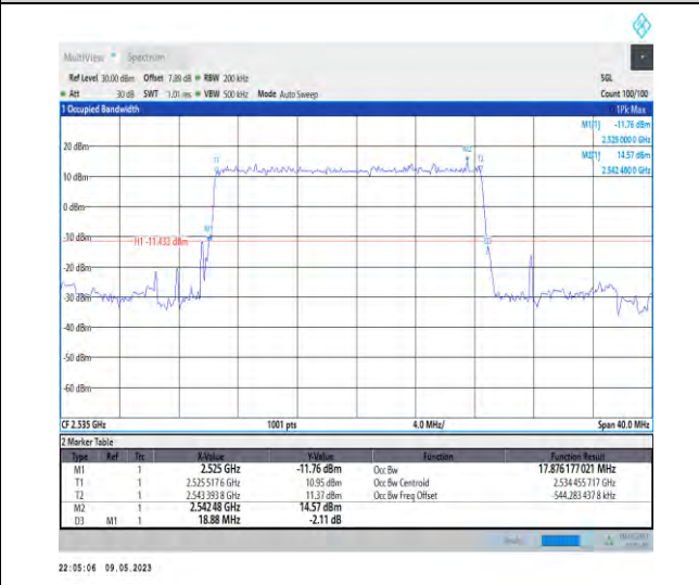
1-N7-PC3-15-20-M-2-DFT-PI2BPSK-Outer_Full-100@0-Ant1-17.876-18.880-<=20-PASS
