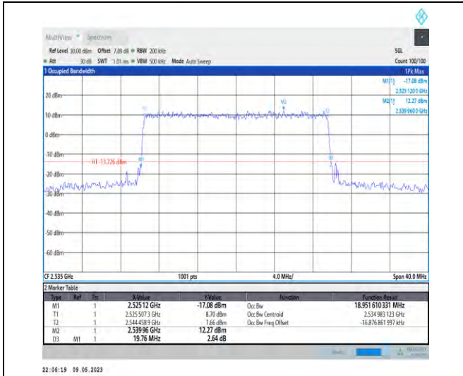
1-N7-PC3-15-20-M-7-CP-16QAM-Outer_Full-106@0 -Ant1-18.952-19.760-≤20-PASS
