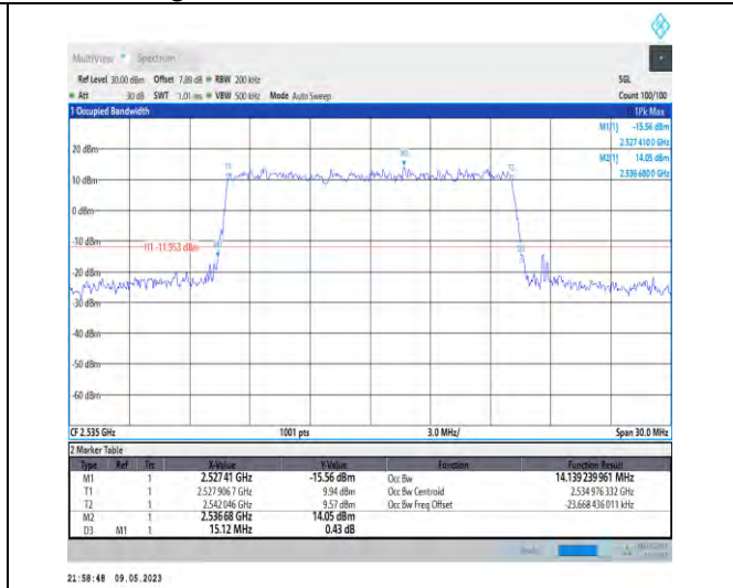
1-N7-PC3-15-15-M-7-CP-16QAM-Outer_Full-79@0- Ant1-14.139-15.120-≤15-PASS
