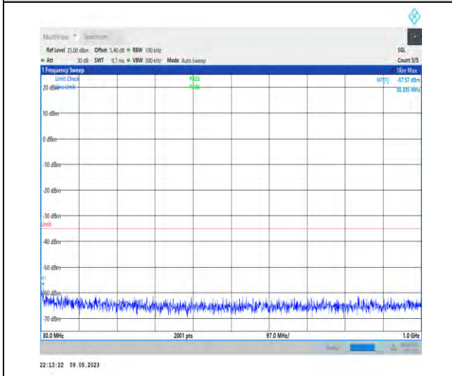
1-N7-PC3-15-20-H-1-DFT-PI2BPSK-Inner_1RB_Lef t-1@1-30-1000-Ant1-35.34--57.57--35-PASS
