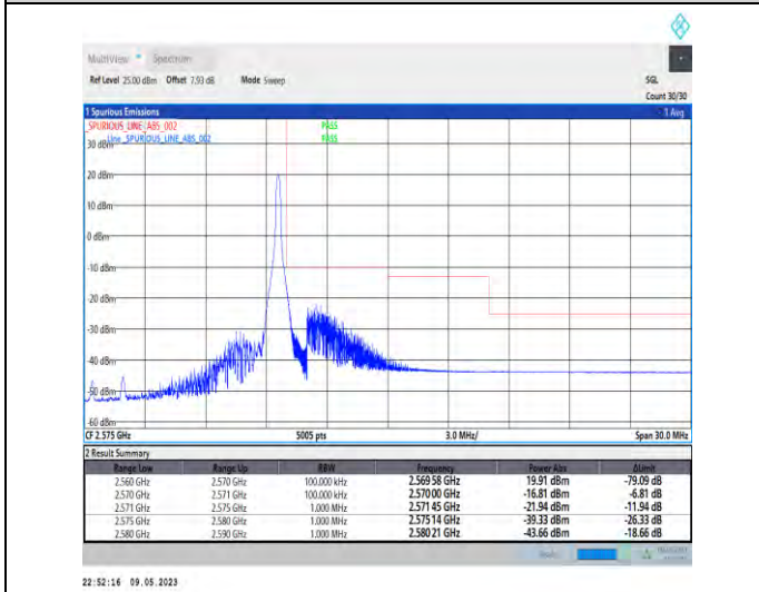
1-N7-PC3-15-10-H-5-CP-QPSK-Edge_1RB_Right-1@51-Ant1-1--PASS-see graph
