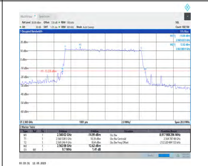
1-N7-PC3-15-10-H-3-DFT-16QAM-Outer_Full-50@0 -Ant1-8.918-9.700-≤10-PASS
