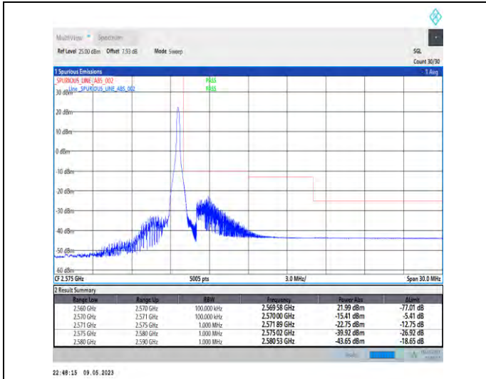
1-N7-PC3-15-10-H-2-DFT-PI2BPSK-Edge_1RB_Right-1@51-Ant1-1--PASS-see graph
