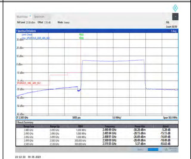
1-N7-PC3-15-20-L-6-CP-QPSK-Outer_Full-106@0-Ant1-1--PASS-see graph
