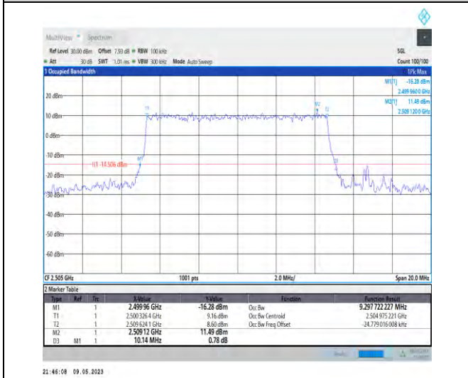
1-N7-PC3-15-10-L-8-CP-64QAM-Outer_Full-52@0-A Ant1-9.298-10.140-≤10-PASS
