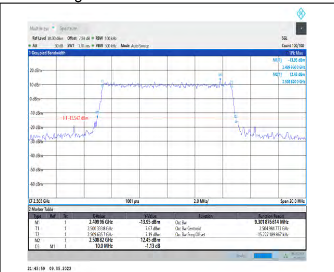
1-N7-PC3-15-10-L-7-CP-16QAM-Outer_Full-52@0-A nt1-9.302-10.000-≤10-PASS
