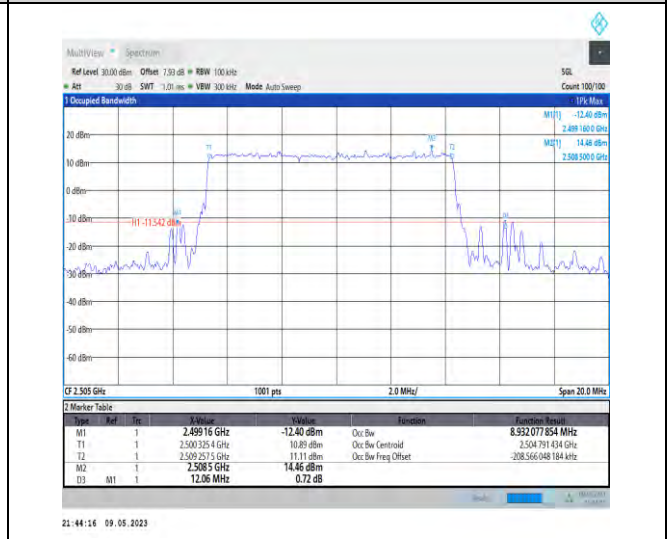
1-N7-PC3-15-10-L-1-DFT-QPSK-Outer_Full-50@0-A Ant1-8.932-12.060-≤10-PASS
