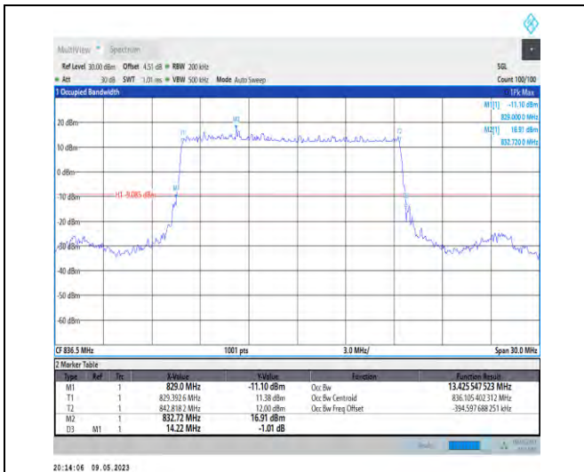
1-N5-PC3-15-15-M-2-DFT-PI2BPSK-Outer_Full-75 @0-Ant1-13.426-14.220-≤15-PASS
