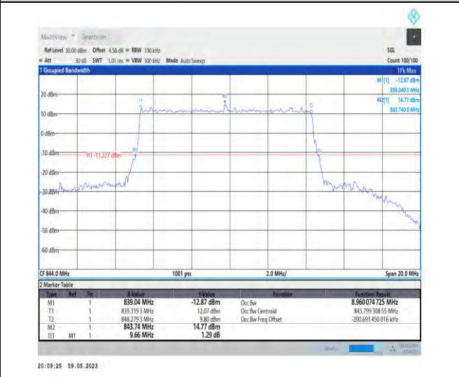
1-N5-PC3-15-10-H-3-DFT-16QAM-Outer_Full-50@0 Ant1-8.96-9.660-≤10-PASS
