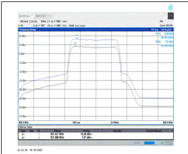
1-N5-PC3-15-20-H-1-DFT-256QAM-Outer_Full-100 @0-Ant1-8.67-100%-0.00-8.67-PASS-≤13
