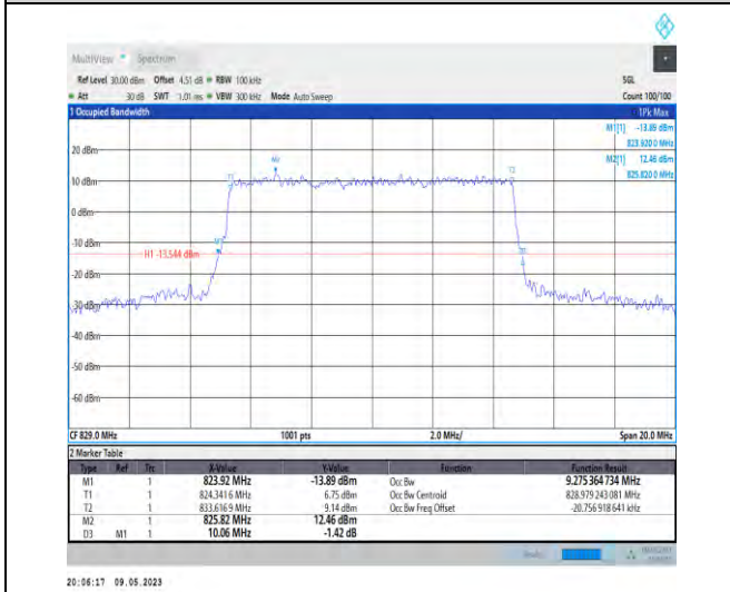
1-N5-PC3-15-10-L-8-CP-64QAM-Outer_Full-52@0-A Ant1-9.275-10.060-≤10-PASS
