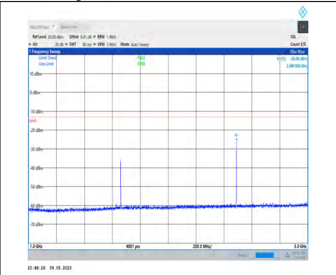
1-N5-PC3-15-20-H-1-DFT-PI2BPSK-Inner_1RB_Left -1@1-1000-3000-Ant1-2489.50--26.04--13-PASS
