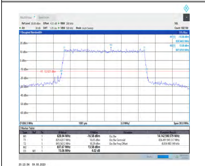
1-N5-PC3-15-15-M-8-CP-64QAM-Outer_Full-79@0- Ant1-14.143-15.060-≤15-PASS
