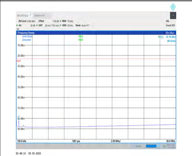
1-N5-PC3-15-20-H-1-DFT-PI2BPSK-Inner_1RB_Left -1@1-0.15-30-Ant1-0.60--81.78--23-PASS
