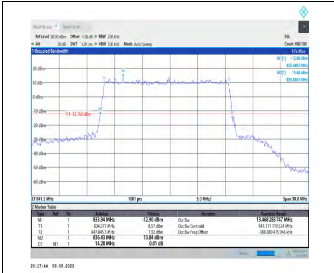
1-N5-PC3-15-15-H-5-DFT-256QAM-Outer_Full-75@ 0-Ant1-13.468-14.280-≤15-PASS
