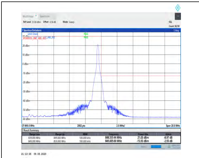
1-N5-PC3-15-10-H-2-DFT-PI2BPSK-Edge_1RB_Right-1@51-Ant1-1-seegraph-PASS-see graph
