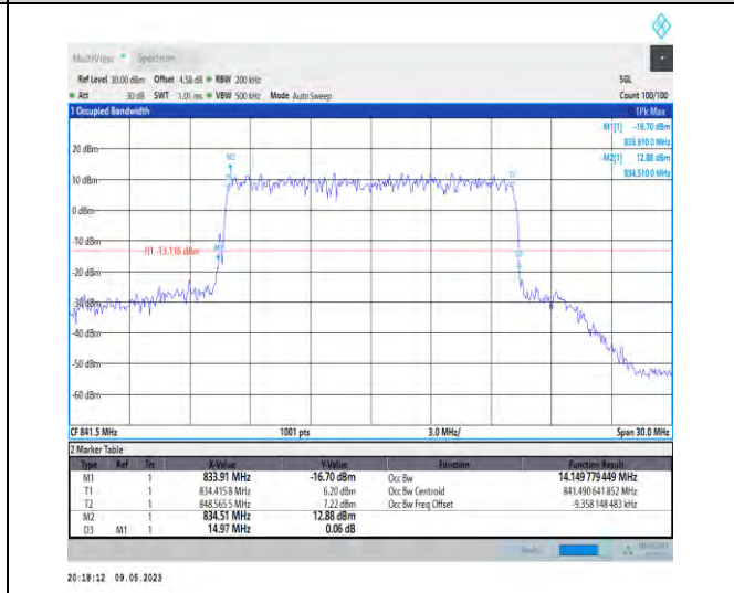
1-N5-PC3-15-15-H-8-CP-64QAM-Outer_Full-79@0- Ant1-14.15-14.970-≤15-PASS
