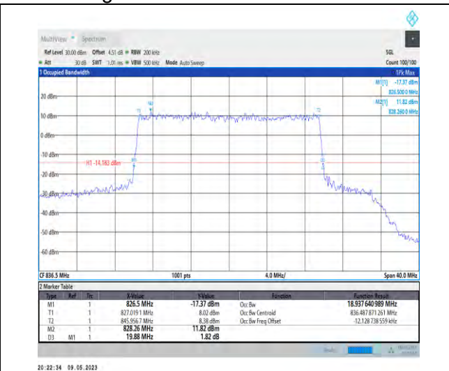
1-N5-PC3-15-20-M-8-CP-64QAM-Outer_Full-106@0 -Ant1-18.938-19.880-≤20-PASS
