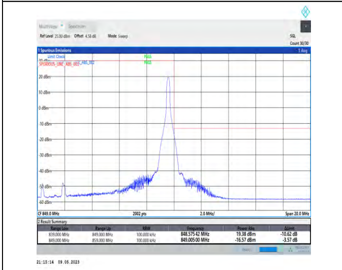
1-N5-PC3-15-10-H-5-CP-QPSK-Edge_1RB_Right-1@51-Ant1-1-seegraph-PASS-see graph
