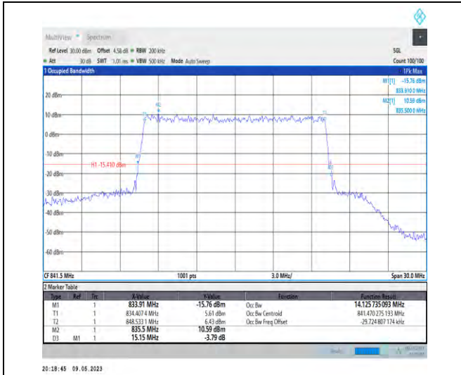
1-N5-PC3-15-15-H-9-CP-256QAM-Outer_Full-79@0 -Ant1-14.126-15.150-≤15-PASS
