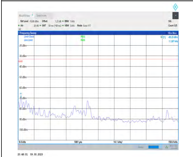
1-N5-PC3-15-20-H-1-DFT-PI2BPSK-Inner_1RB_Left -1@1-0.009-0.15-Ant1-0.01--69.23--33-PASS
