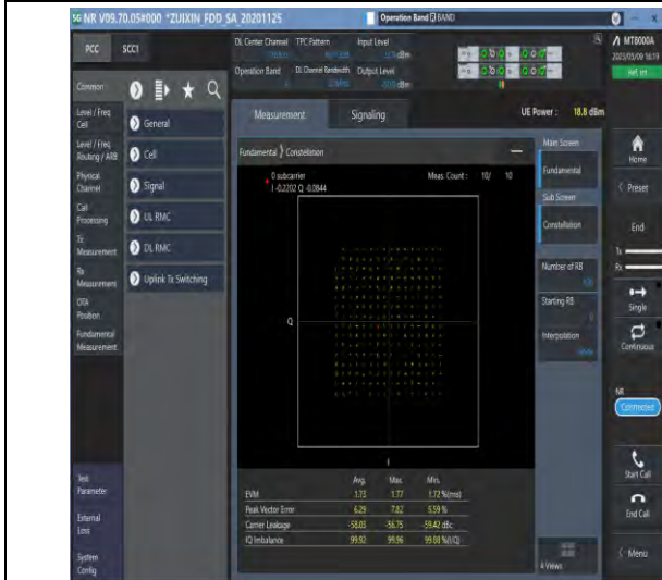
1-N5-PC3-15-20-M-9-CP-256QAM-Outer_Full-106@0-Ant1-see graph-PASS
