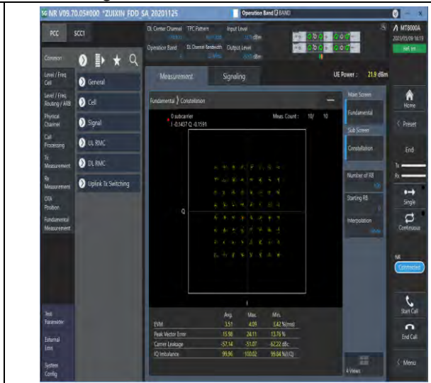
1-N5-PC3-15-20-M-8-CP-64QAM-Outer_Full-106@0-Ant1-see graph-PASS
