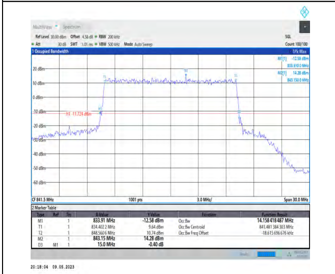
1-N5-PC3-15-15-H-7-CP-16QAM-Outer_Full-79@0- Ant1-14.158-15.000-≤15-PASS
