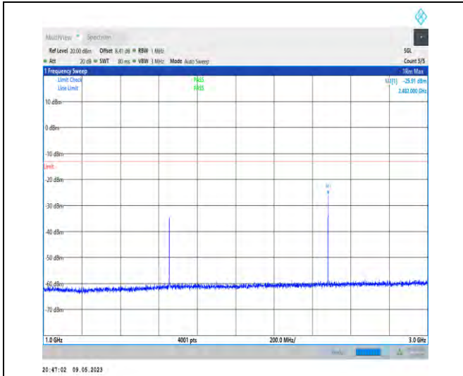
1-N5-PC3-15-20-M-1-DFT-PI2BPSK-Inner_1RB_Left -1@1-1000-3000-Ant1-2481.50--25.91--13-PASS
