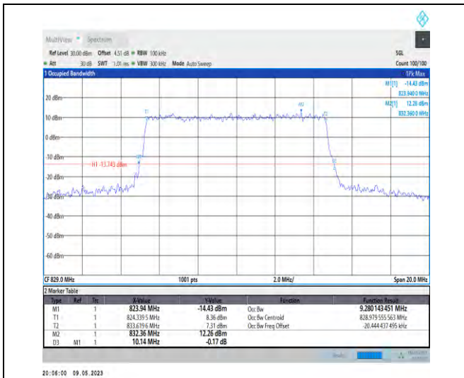
1-N5-PC3-15-10-L-6-CP-QPSK-Outer_Full-52@0-A nt1-9.28-10.140-≤10-PASS
