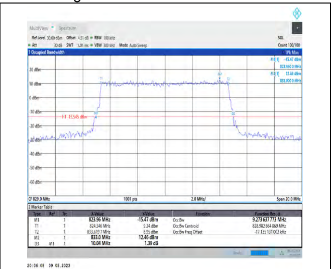
1-N5-PC3-15-10-L-7-CP-16QAM-Outer_Full-52@0-A nt1-9.274-10.040-≤10-PASS
