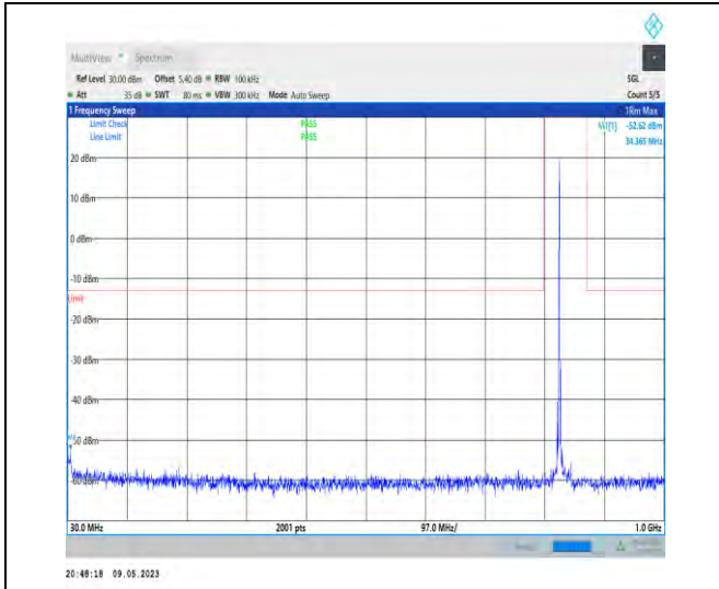
1-N5-PC3-15-20-H-1-DFT-PI2BPSK-Inner_1RB_Left -1@1-30-1000-Ant1-35.34--52.62--13-PASS
