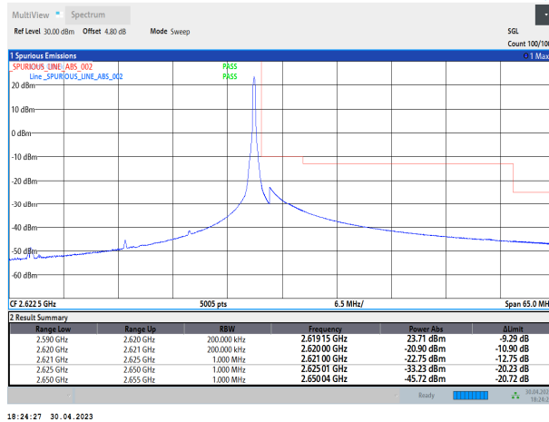
38-38-15MHz-15MHz-QPSK-QPSK-38025-38175-0RB#0-1RB#74
