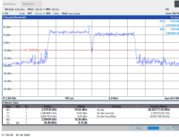
38-38-15MHz-15MHz-QPSK-QPSK-38025-38175-75RB#0-75RB#0
