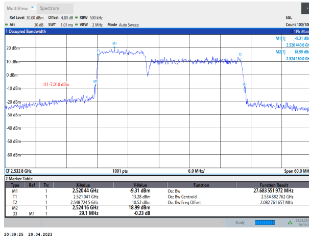
7-7-10MHz-20MHz-QPSK-QPSK-21006-21150-50RB#0-100RB#0
