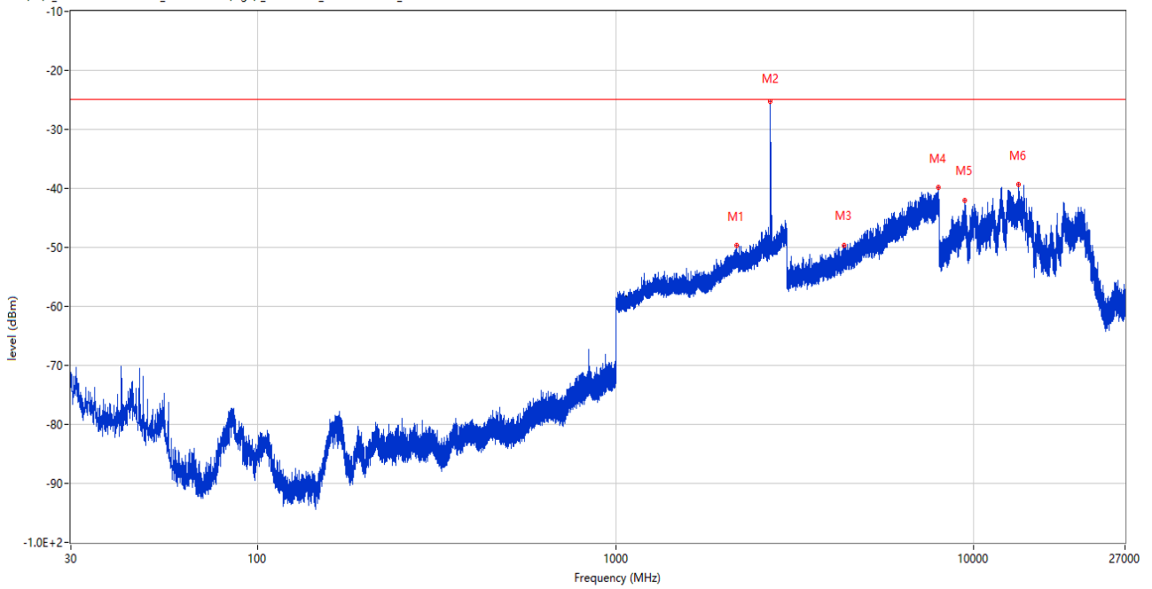
RSE (RF) _FCC PART22&24&27_LTE Band 41(high) _2620-2690_30MHz-27GHz_
