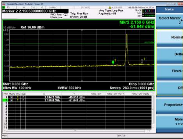
802.11g CH6, SPURIOUS 30 MHz ~ 3 GHz
