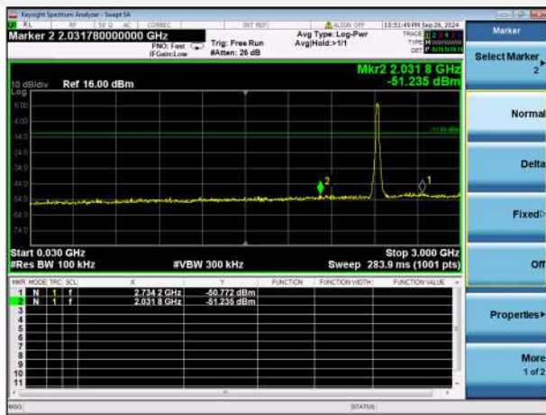
802.11n-20 MHz CH4, SPURIOUS 30 MHz ~ 3 GHz
