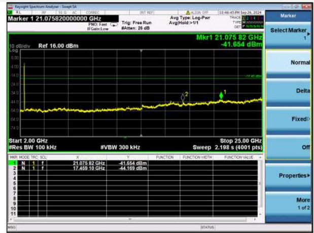
802.11n-20 MHz CH3, SPURIOUS 2 GHz ~ 25 GHz
