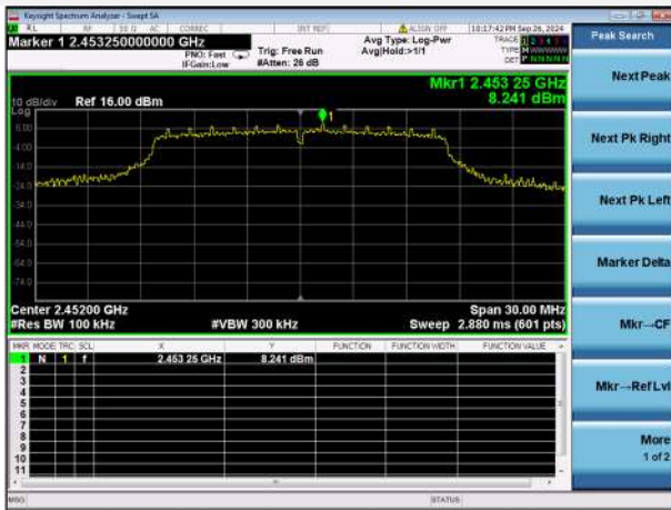
802.11g CH9 CARRIER LEVEL
