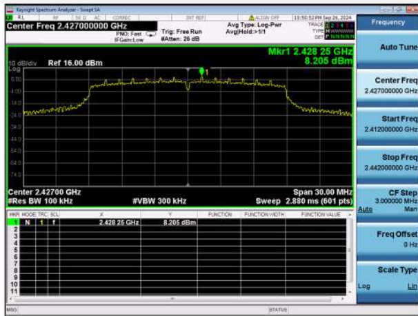
802.11n-20 MHz CH4 CARRIER LEVEL
