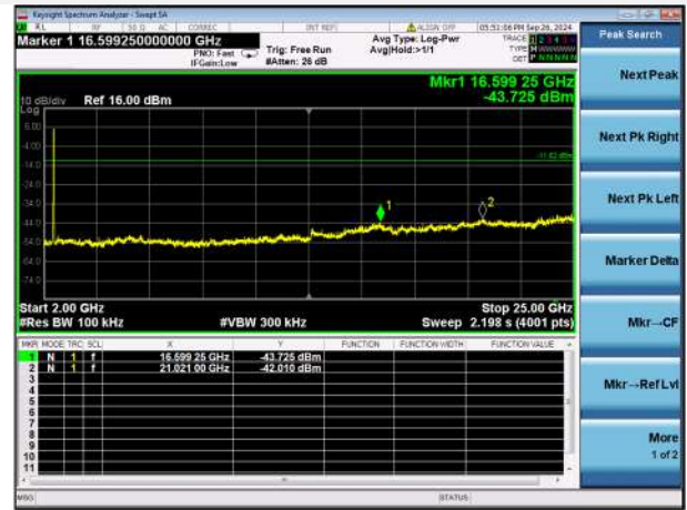
802.11g CH6, SPURIOUS 2 GHz ~ 25 GHz
