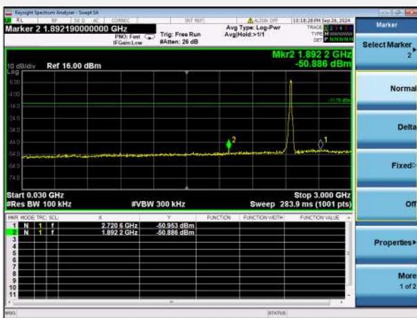
802.11g CH9, SPURIOUS 30 MHz ~ 3 GHz
