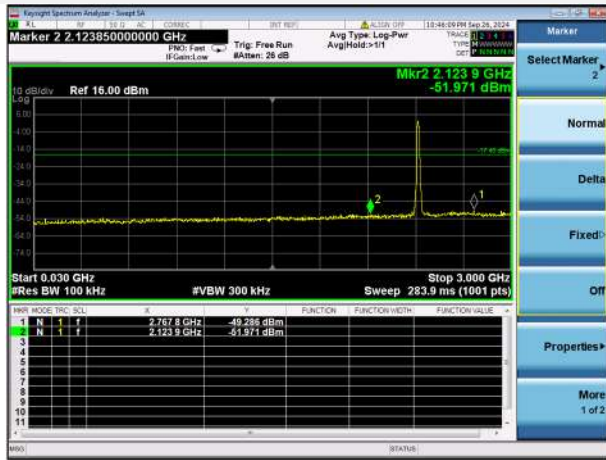
802.11n-20 MHz CH3, SPURIOUS 30 MHz ~ 3 GHz
