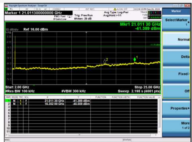
802.11g CH9, SPURIOUS 2 GHz ~ 25 GHz
