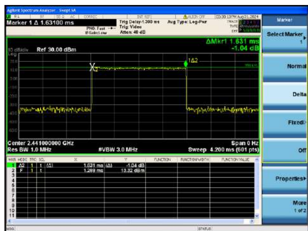
8-DPSK 3DH3
