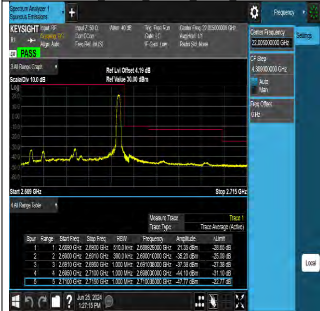
Band41_20MHz_16QAM_41490_1RB#99
