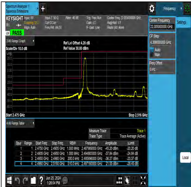
Band41_20MHz_16QAM_39750_1RB#0
