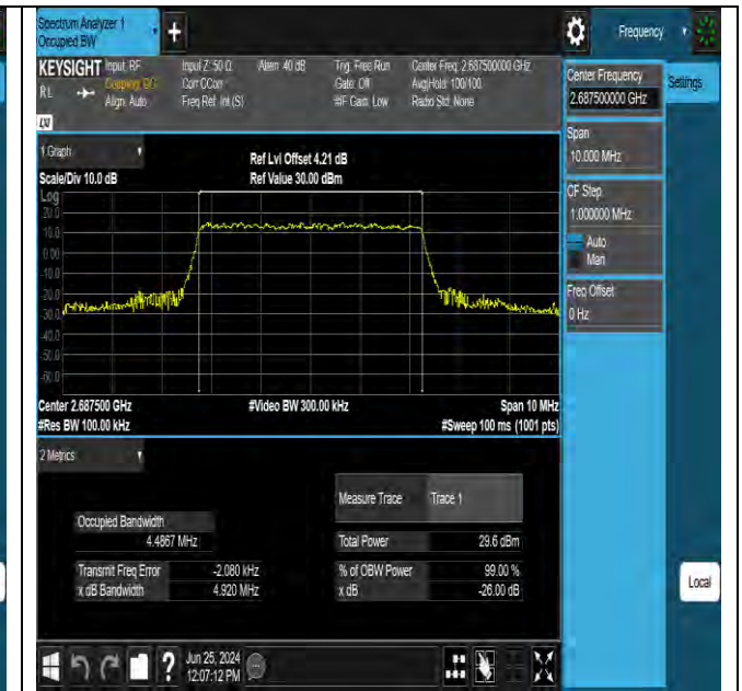
Band41-5MHz-16QAM-41565-25RB#0-PASS
