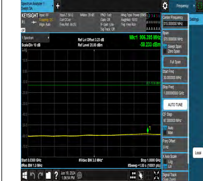
Band2 10MHz QPSK 18650 1RB#49 30~1000 30~1000
