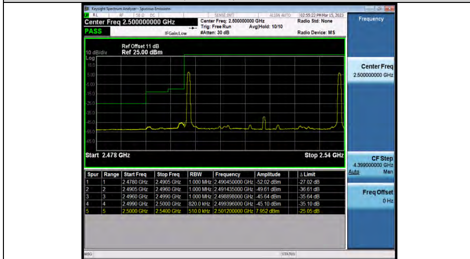
7-7-20MHz-20MHz-16QAM-16QAM-20850-21048-1RB#99-1RB#0
