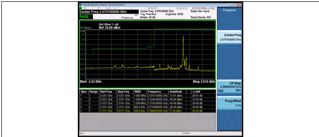
38-38-20MHz-20MHz-16QAM-16QAM-37952-38150-100RB#0-100RB#0
