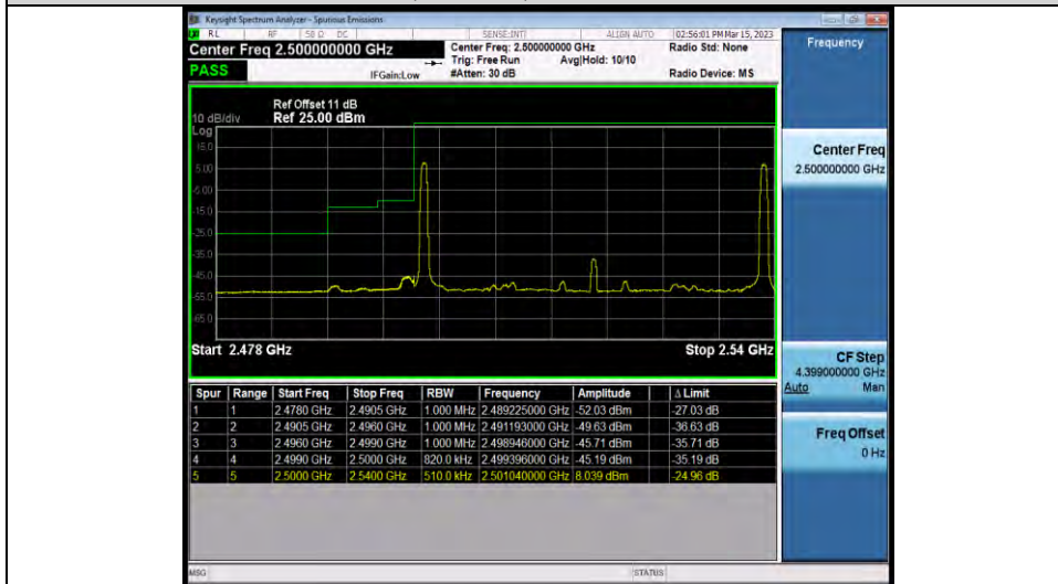
7-7-20MHz-20MHz-64QAM-64QAM-20850-21048-1RB#99-1RB#0
