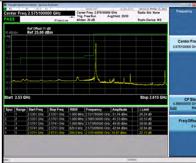
38-38-20MHz-20MHz-16QAM-16QAM-37901-38099-1RB#99-0RB#0
