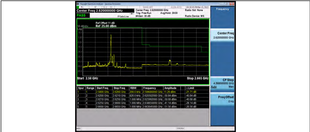
38-38-20MHz-20MHz-64QAM-64QAM-37850-38048-100RB#0-100RB#0
