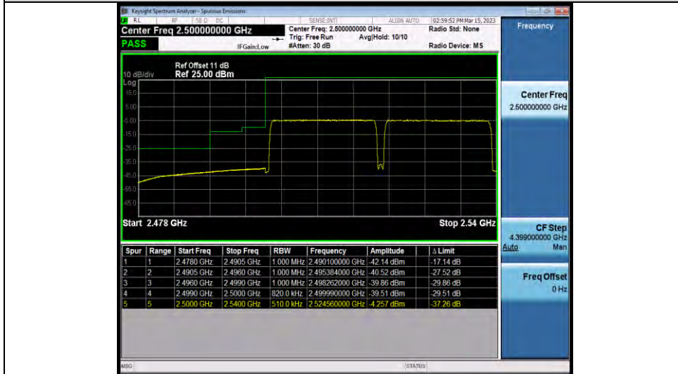
7-7-20MHz-20MHz-64QAM-64QAM-20850-21048-1RB#0-1RB#99
