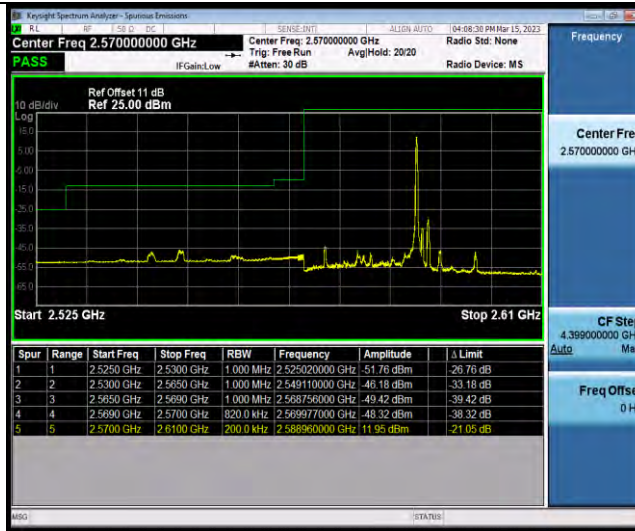
38-38-20MHz-20MHz-16QAM-16QAM-37901-38099-100RB#0-100RB#0
