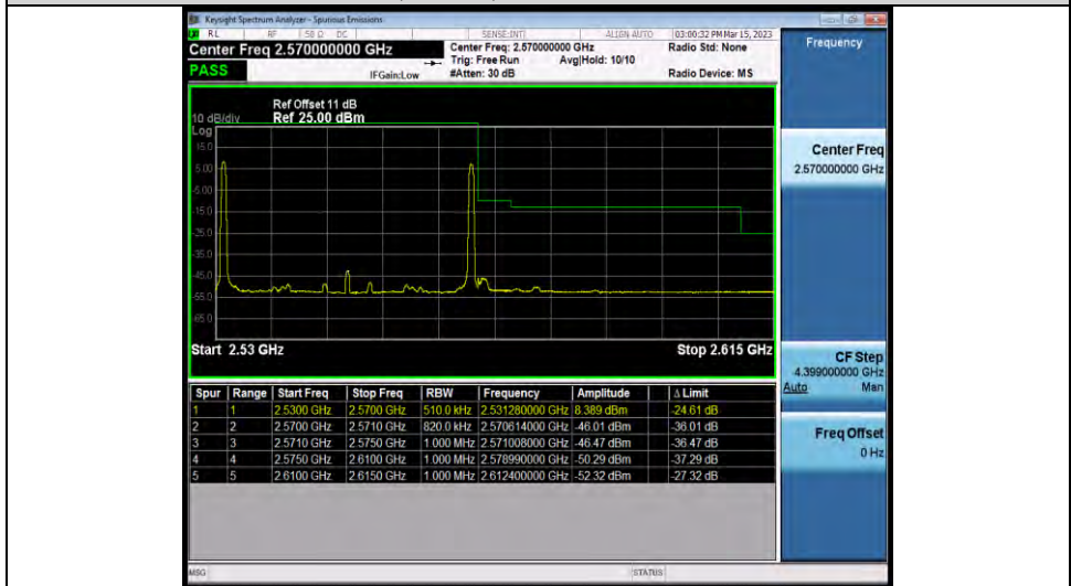
7-7-20MHz-20MHz-QPSK-QPSK-21152-21350-1RB#99-1RB#0
