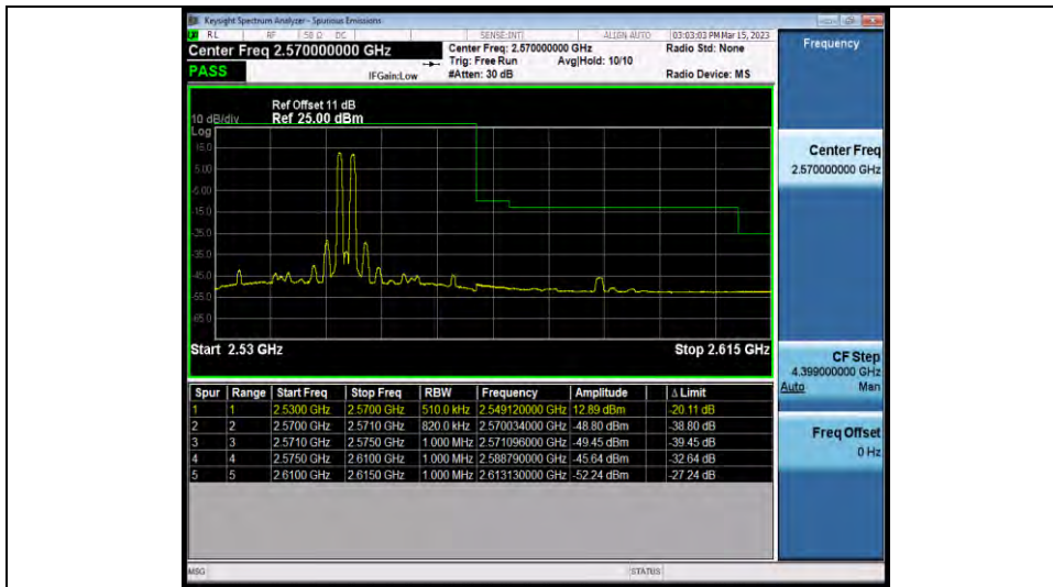
7-7-20MHz-20MHz-64QAM-64QAM-20850-21048-100RB#0-100RB#0
