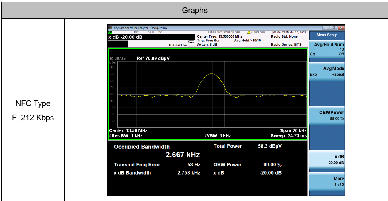
20dB Bandwidth & 99% Bandwidth Plot
