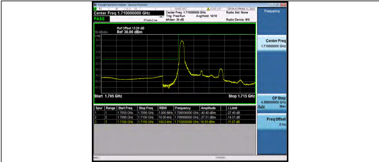
Band66-3MHz-64QAM-131987-15RB#0
