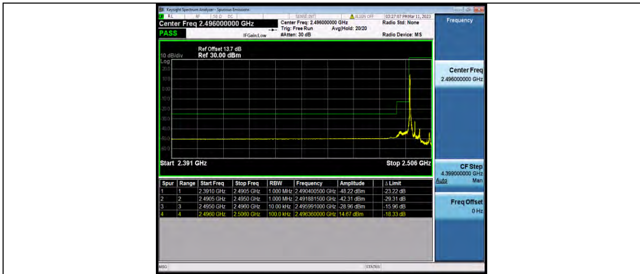
Band41-5MHz-64QAM-39675-25RB#0
