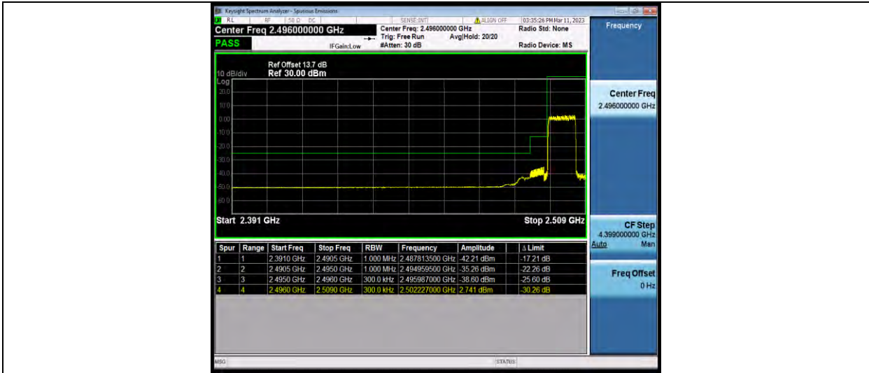
Band41-10MHz-16QAM-41540-1RB#49
