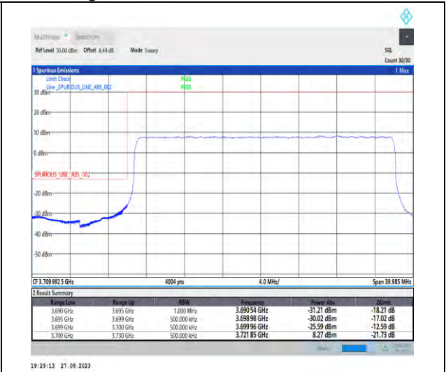
1-N78-3700-3800-PC2-30-30-L-3-DFT-PI2BPSK-Outer_Full-75@0-Ant7-1--PASS-see graph
