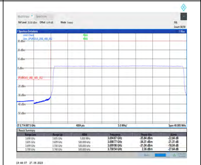
1-N78-3700-3800-PC2-30-40-L-6-CP-QPSK-Outer_Full-106@0-Ant7-1--PASS-see graph
