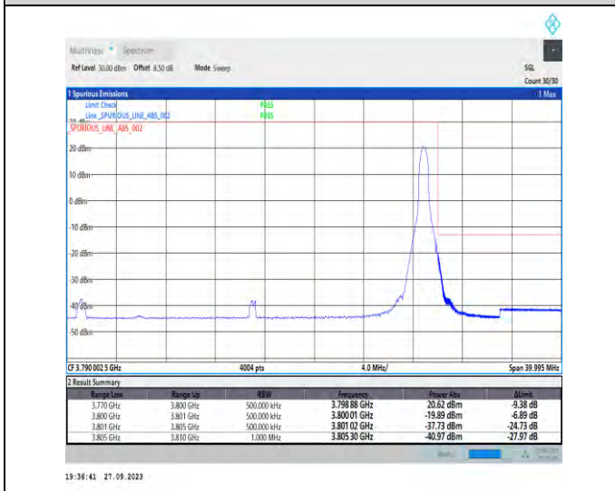
1-N78-3700-3800-PC2-30-30-H-5-CP-QPSK-Edge_1RB_Right-1@77-Ant7-1--PASS-see graph
