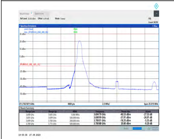
1-N78-3700-3800-PC2-30-15-L-4-CP-QPSK-Edge_1RB_Left-1@0-Ant7-1--PASS-see graph
