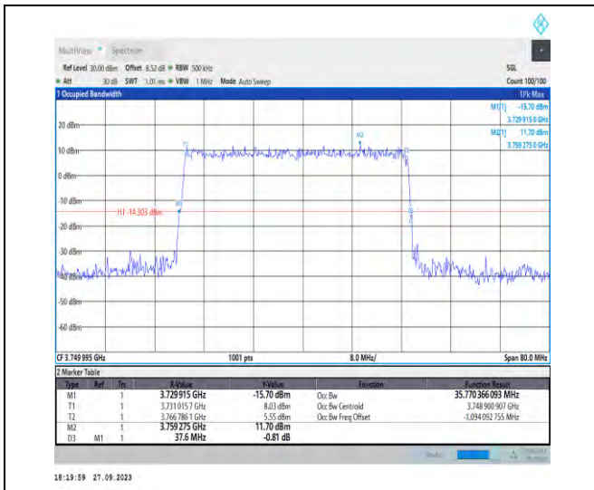
1-N78-3700-3800-PC2-30-40-M-5-DFT-256QAM-Out _Full-100@0-Ant7-35.77-37.600-≤40-PASS
