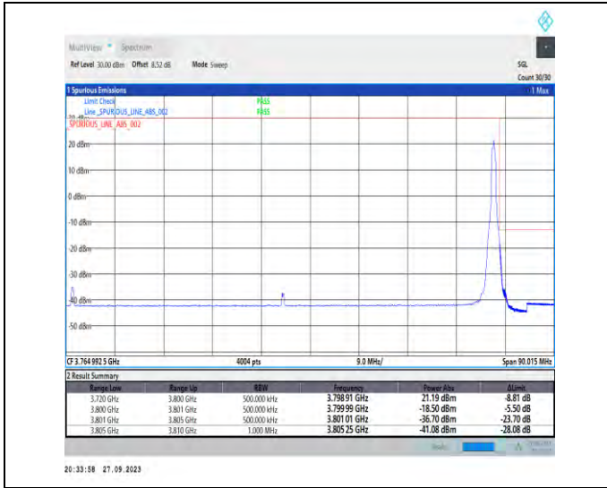
1-N78-3700-3800-PC2-30-80-H-2-DFT-PI2BPSK-Edge_1RB_Right-1@216-Ant7-1--PASS-see graph
