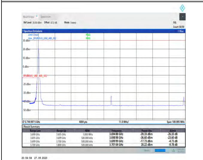
1-N78-3700-3800-PC2-30-100-L-4-CP-QPSK-Edge_1_RB_Left-1@0-Ant7-1--PASS-see graph
