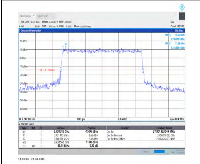
1-N78-3700-3800-PC2-30-40-M-7-CP-16QAM-Outer _Full-106@0-Ant7-37.805-39.440-≤40-PASS
