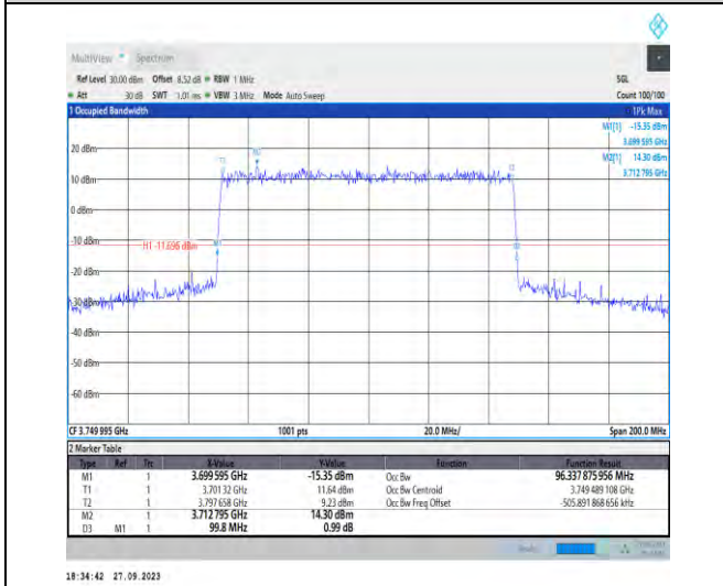
1-N78-3700-3800-PC2-30-100-M-1-DFT-QPSK-Outer_Full-270@0-Ant7-96.338-99.800-<=100-PASS
