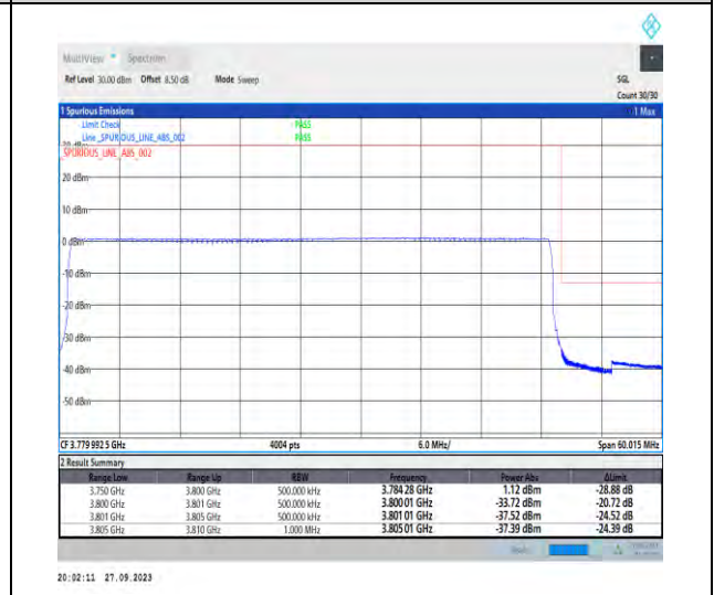
1-N78-3700-3800-PC2-30-50-H-6-CP-QPSK-Outer_Full-133@0-Ant7-1--PASS-see graph
