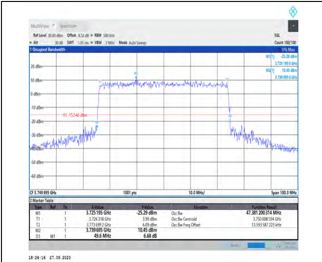
1-N78-3700-3800-PC2-30-50-M-8-CP-64QAM-Outer_Full-133@0-Ant7-47.381-49.600-≤50-PASS
