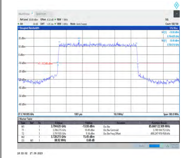
1-N78-3700-3800-PC2-30-90-M-2-DFT-PI2BPSK-Outer_Full-240@0-Ant7-85.66-88.920-≤90-PASS
