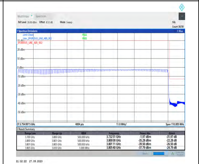
1-N78-3700-3800-PC2-30-100-H-6-CP-QPSK-Outer_Full-273@0-Ant7-1--PASS-see graph
