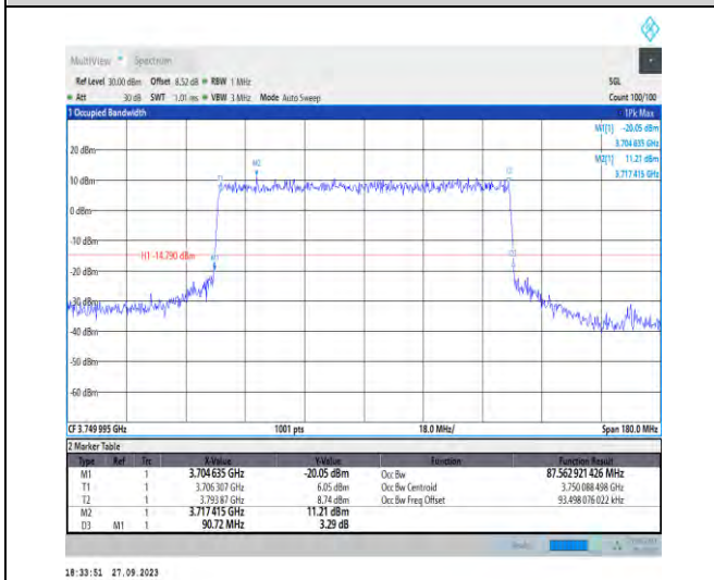
1-N78-3700-3800-PC2-30-90-M-6-CP-QPSK-Outer_Full-245@0-Ant7-87.563-90.720-≤90-PASS
