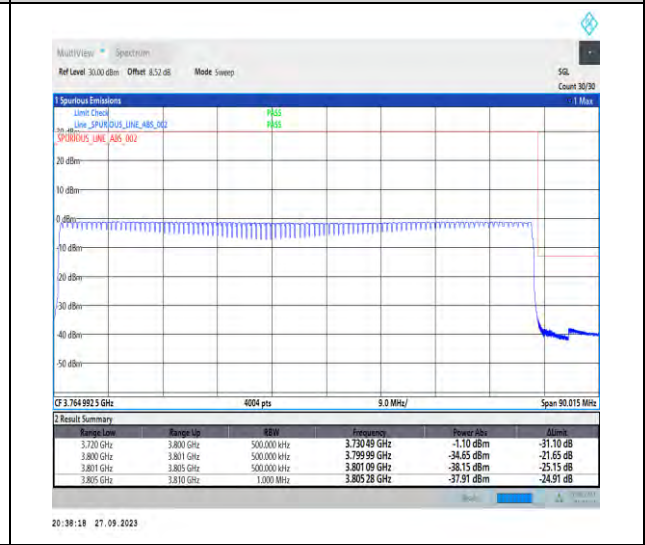
1-N78-3700-3800-PC2-30-80-H-6-CP-QPSK-Outer_Full-217@0-Ant7-1--PASS-see graph
