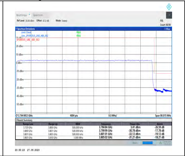
1-N78-3700-3800-PC2-30-80-H-3-DFT-PI2BPSK-Outer_Full-216@0-Ant7-1--PASS-see graph
