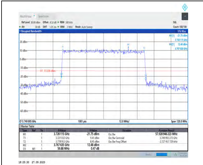
1-N78-3700-3800-PC2-30-60-M-3-DFT-16QAM-Outer_Full-162@0-Ant7-57.921-59.880-≤60-PASS
