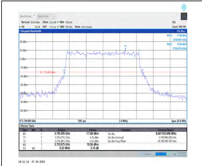
1-N78-3700-3800-PC2-30-10-M-5-DFT-256QAM-Out _Full-24@0-Ant7-8.602-9.320-≤10-PASS
