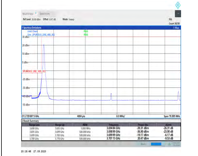
1-N78-3700-3800-PC2-30-70-L-4-CP-QPSK-Edge_1RB_Left-1@0-Ant7-1--PASS-see graph
