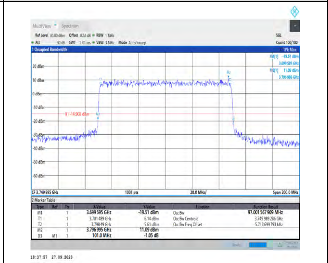
1-N78-3700-3800-PC2-30-100-M-6-CP-QPSK-Outer_Full-273@0-Ant7-97.002-101.000-≤100-PASS
