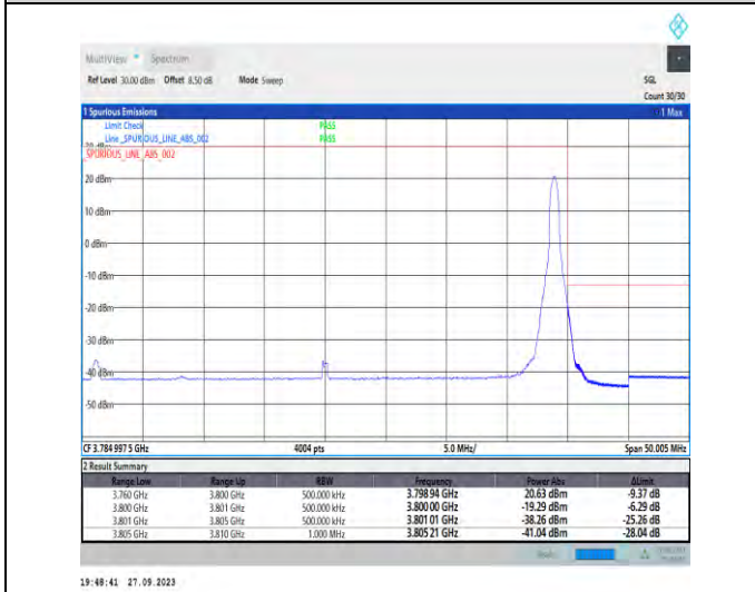
1-N78-3700-3800-PC2-30-40-H-5-CP-QPSK-Edge_1RB_Right-1@105-Ant7-1--PASS-see graph
