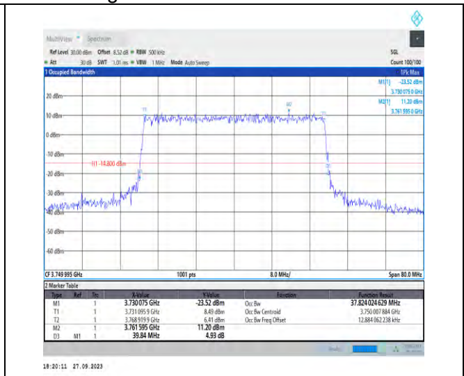
1-N78-3700-3800-PC2-30-40-M-6-CP-QPSK-Outer_ _Full-106@0-Ant7-37.824-39.840-≤40-PASS
