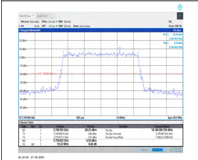
1-N78-3700-3800-PC2-30-20-M-9-CP-256QAM-Outer_Full-51@0-Ant7-18.18-19.320-≤20-PASS
