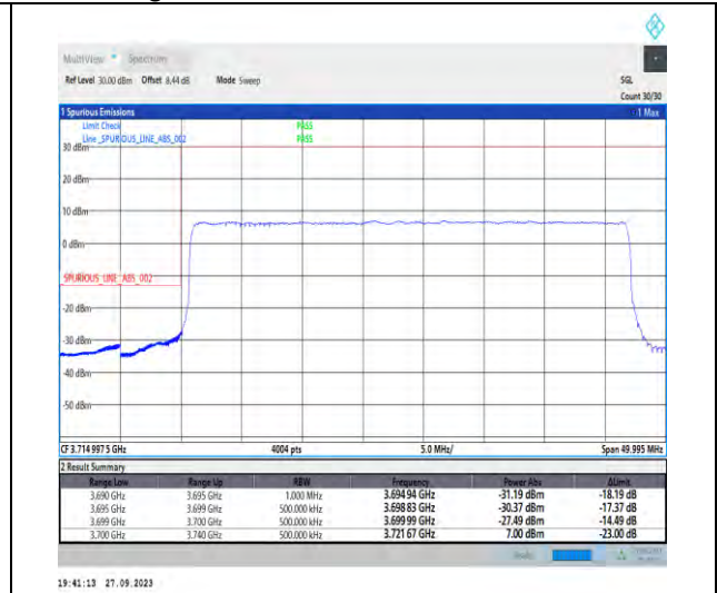
1-N78-3700-3800-PC2-30-40-L-3-DFT-PI2BPSK-Outer_Full-100@0-Ant7-1--PASS-see graph
