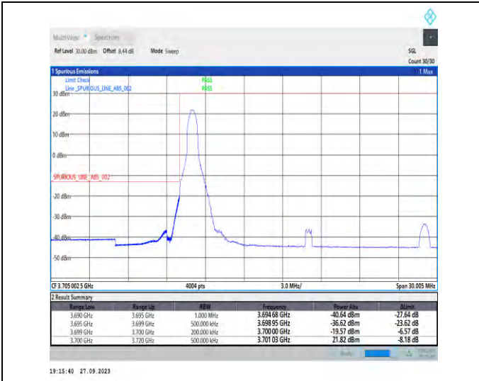
1-N78-3700-3800-PC2-30-20-L-1-DFT-PI2BPSK-Edge_1RB_Left-1@0-Ant7-1--PASS-see graph
