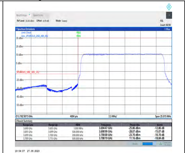
1-N78-3700-3800-PC2-30-15-L-3-DFT-PI2BPSK-Outer_Full-36@0-Ant7-1--PASS-see graph
