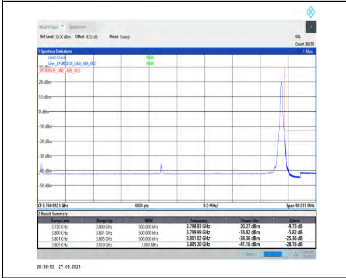
1-N78-3700-3800-PC2-30-80-H-5-CP-QPSK-Edge_1RB_Right-1@216-Ant7-1--PASS-see graph
