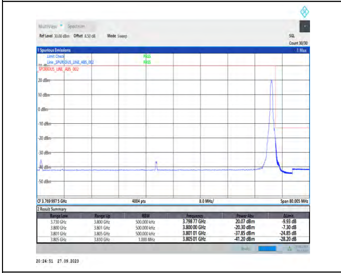
1-N78-3700-3800-PC2-30-70-H-5-CP-QPSK-Edge_1RB_Right-1@188-Ant7-1--PASS-see graph
