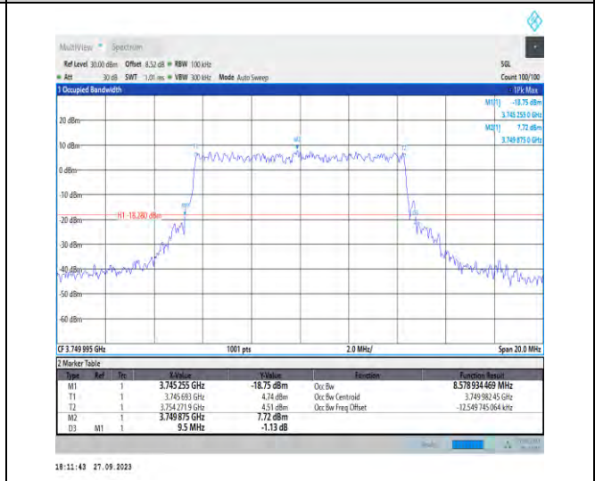
1-N78-3700-3800-PC2-30-10-M-8-CP-64QAM-Outer _Full-24@0-Ant7-8.579-9.500-≤10-PASS
