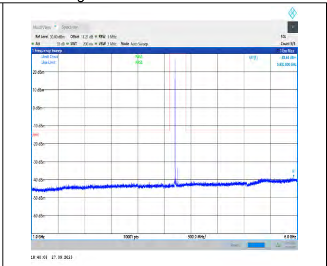
1-N78-3700-3800-PC2-30-100-M-1-DFT-PI2BPSK- Inner_1RB_Left-1@1-1000-6000-Ant7-5932.00--38.64-- 13-PASS
