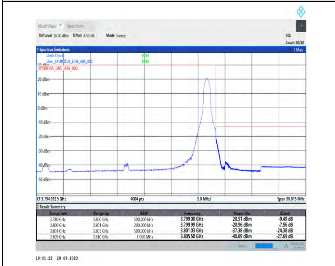
1-N78-3700-3800-PC2-30-20-H-5-CP-QPSK-Edge_1RB_Right-1@50-Ant7-1--PASS-see graph
