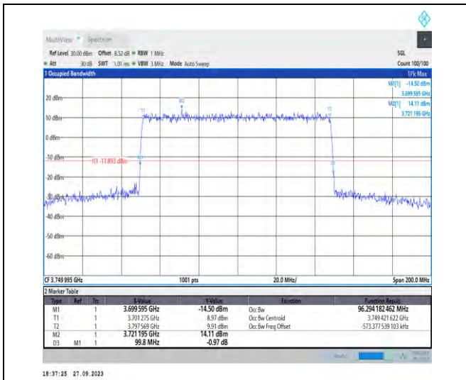
1-N78-3700-3800-PC2-30-100-M-3-DFT-16QAM-Out er_Full-270@0-Ant7-96.294-99.800-≤100-PASS
