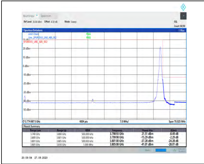
1-N78-3700-3800-PC2-30-60-H-2-DFT-PI2BPSK-Edge_1RB_Right-1@161-Ant7-1--PASS-see graph
