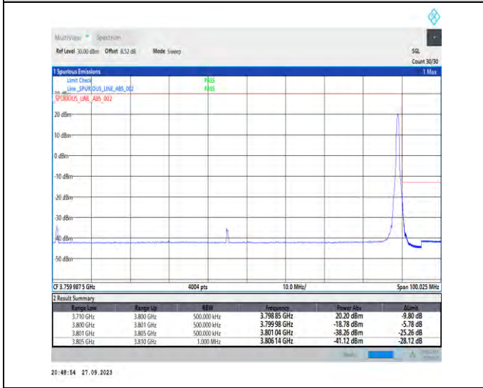
1-N78-3700-3800-PC2-30-90-H-5-CP-QPSK-Edge_1RB_Right-1@244-Ant7-1--PASS-see graph
