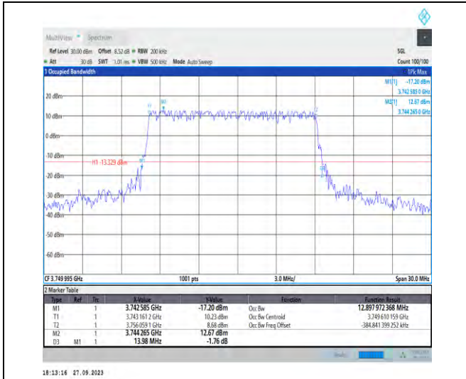
1-N78-3700-3800-PC2-30-15-M-4-DFT-64QAM-Outer_Full-36@0-Ant7-12.898-13.980-≤15-PASS
