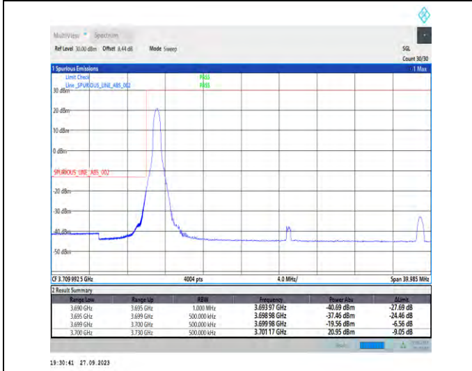
1-N78-3700-3800-PC2-30-30-L-4-CP-QPSK-Edge_1RB_Left-1@0-Ant7-1--PASS-see graph
