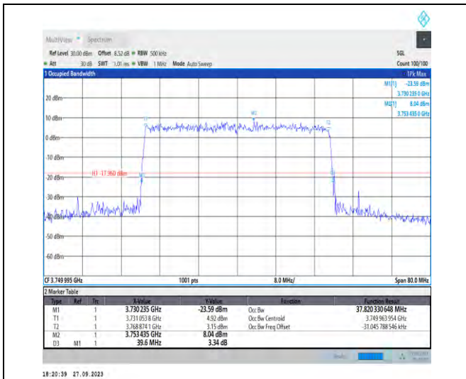
1-N78-3700-3800-PC2-30-40-M-9-CP-256QAM-Out er_Full-106@0-Ant7-37.82-39.600-≤40-PASS
