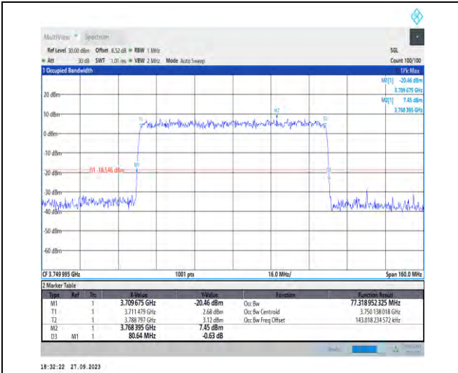
1-N78-3700-3800-PC2-30-80-M-9-CP-256QAM-Out er_Full-217@0-Ant7-77.319-80.640-≤80-PASS
