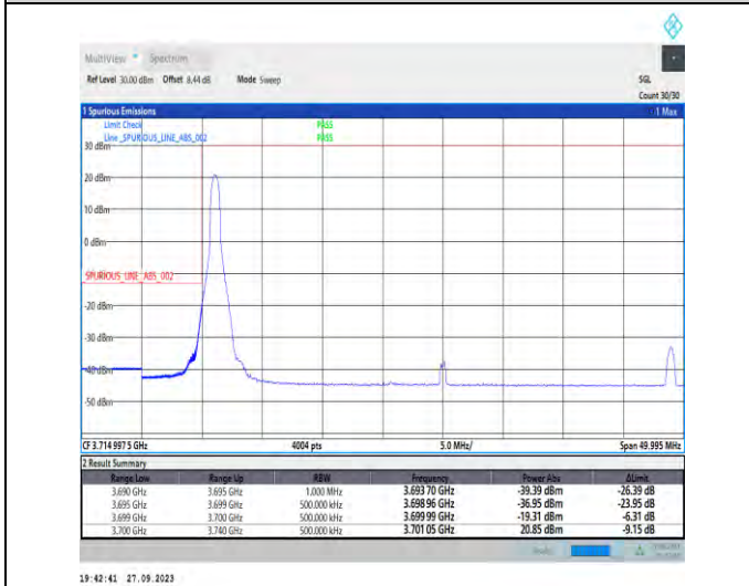
1-N78-3700-3800-PC2-30-40-L-4-CP-QPSK-Edge_1RB_Left-1@0-Ant7-1--PASS-see graph
