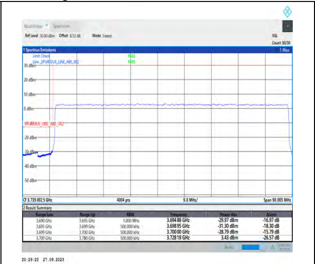
1-N78-3700-3800-PC2-30-80-L-3-DFT-PI2BPSK-Outer_Full-216@0-Ant7-1--PASS-see graph
