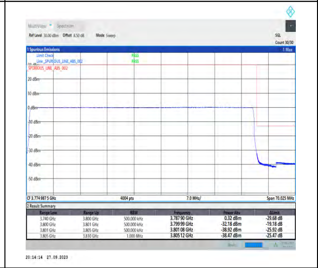
1-N78-3700-3800-PC2-30-60-H-6-CP-QPSK-Outer_Full-162@0-Ant7-1--PASS-see graph
