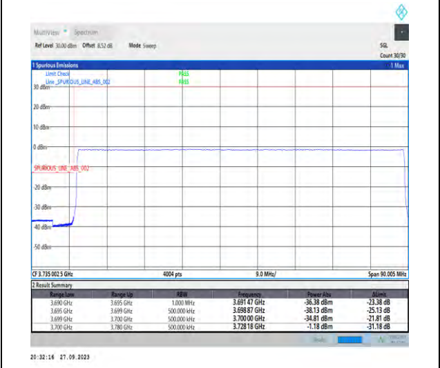
1-N78-3700-3800-PC2-30-80-L-6-CP-QPSK-Outer_Full-217@0-Ant7-1--PASS-see graph
