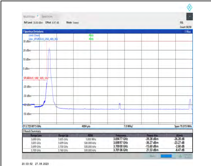
1-N78-3700-3800-PC2-30-60-L-1-DFT-PI2BPSK-Edge_1RB_Left-1@0-Ant7-1--PASS-see graph
