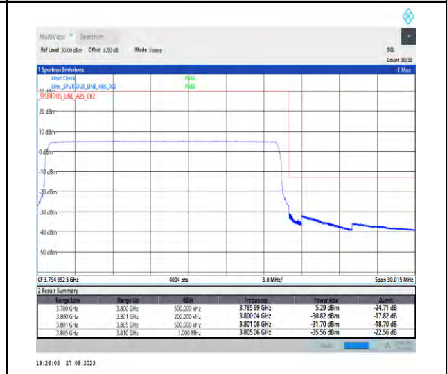
1-N78-3700-3800-PC2-30-20-H-6-CP-QPSK-Outer_Full-51@0-Ant7-1--PASS-see graph
