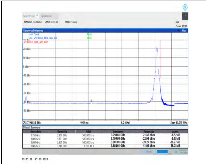
1-N78-3700-3800-PC2-30-50-H-2-DFT-PI2BPSK-Edge_1RB_Right-1@132-Ant7-1--PASS-see graph
