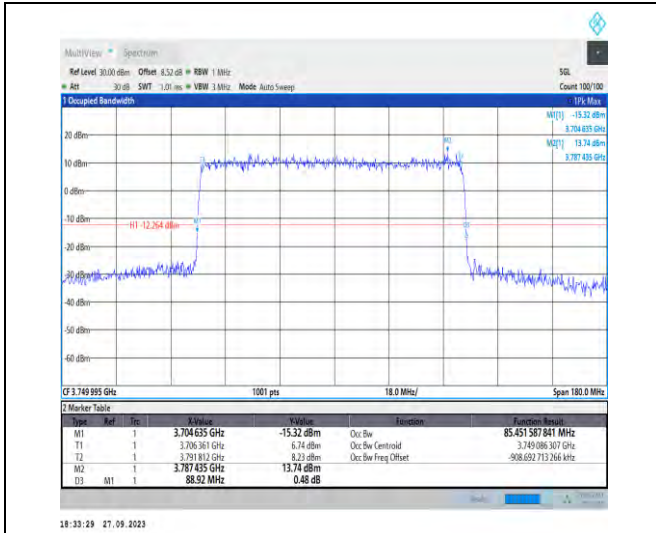
1-N78-3700-3800-PC2-30-90-M-4-DFT-64QAM-Outer_Full-240@0-Ant7-85.452-88.920-≤90-PASS
