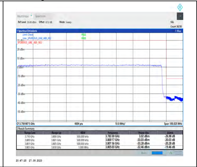
1-N78-3700-3800-PC2-30-90-H-3-DFT-PI2BPSK-Outer_Full-240@0-Ant7-1--PASS-see graph
