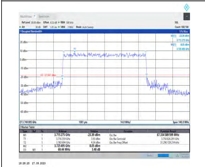
1-N78-3700-3800-PC2-30-70-M-8-CP-64QAM-Outer_Full-189@0-Ant7-67.335-69.440-≤70-PASS
