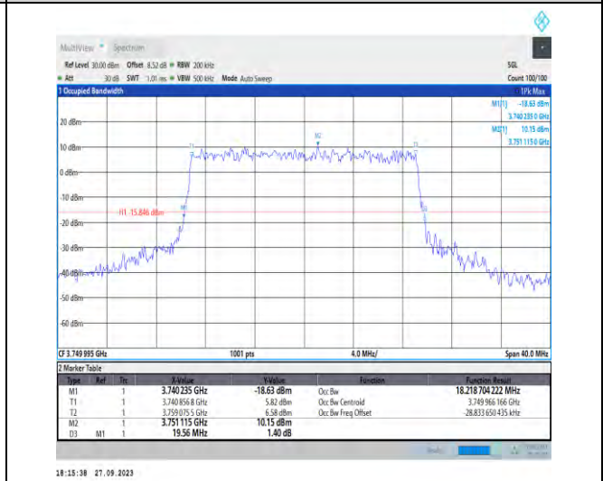
1-N78-3700-3800-PC2-30-20-M-6-CP-QPSK-Outer_Full-51@0-Ant7-18.219-19.560-≤20-PASS
