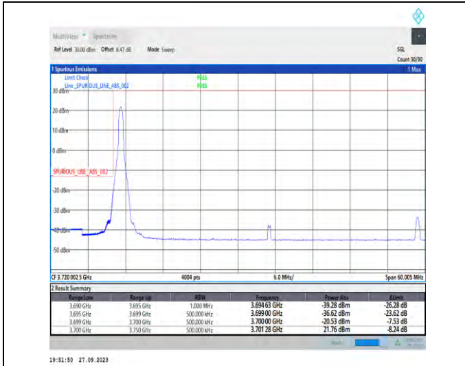
1-N78-3700-3800-PC2-30-50-L-1-DFT-PI2BPSK-Edge_1RB_Left-1@0-Ant7-1--PASS-see graph
