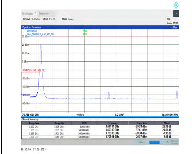
1-N78-3700-3800-PC2-30-80-L-4-CP-QPSK-Edge_1RB_Left-1@0-Ant7-1--PASS-see graph
