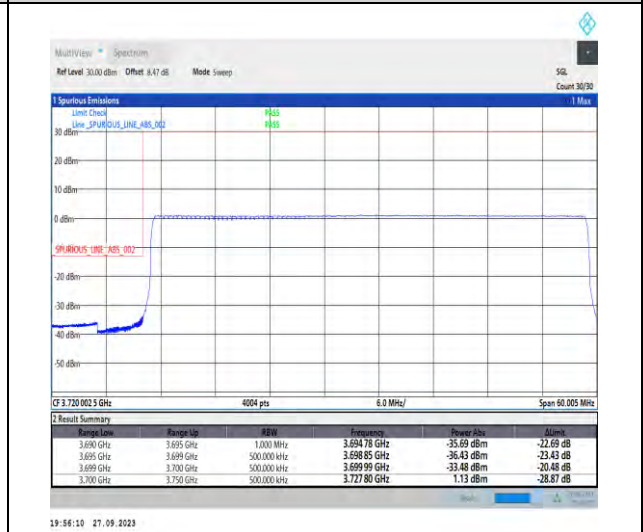
1-N78-3700-3800-PC2-30-50-L-6-CP-QPSK-Outer_Full-133@0-Ant7-1--PASS-see graph
