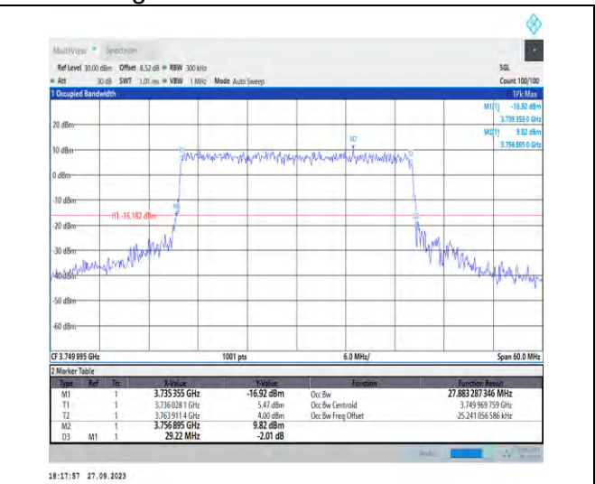
1-N78-3700-3800-PC2-30-30-M-7-CP-16QAM-Outer_Full-78@0-Ant7-27.883-29.220-≤30-PASS
