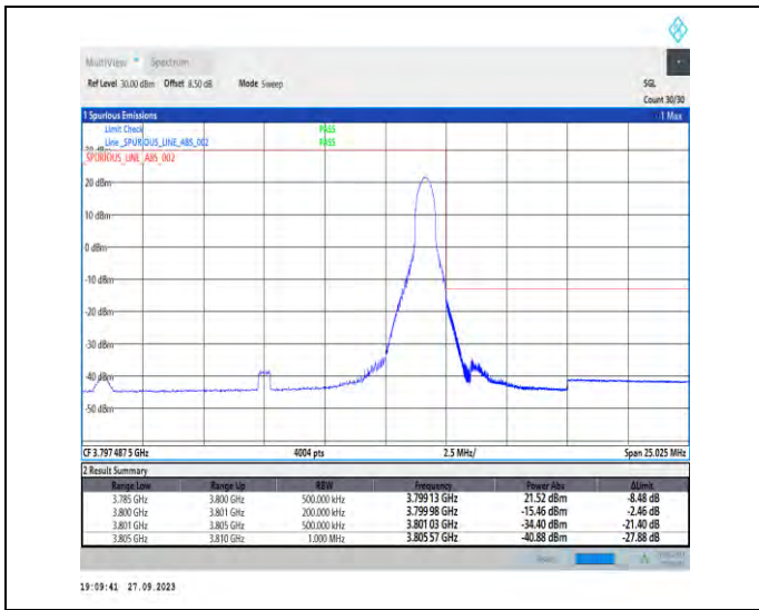
1-N78-3700-3800-PC2-30-15-H-2-DFT-PI2BPSK-Edge_1RB_Right-1@37-Ant7-1--PASS-see graph
