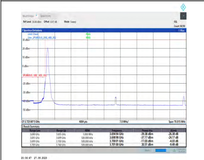
1-N78-3700-3800-PC2-30-60-L-4-CP-QPSK-Edge_1RB_Left-1@0-Ant7-1--PASS-see graph
