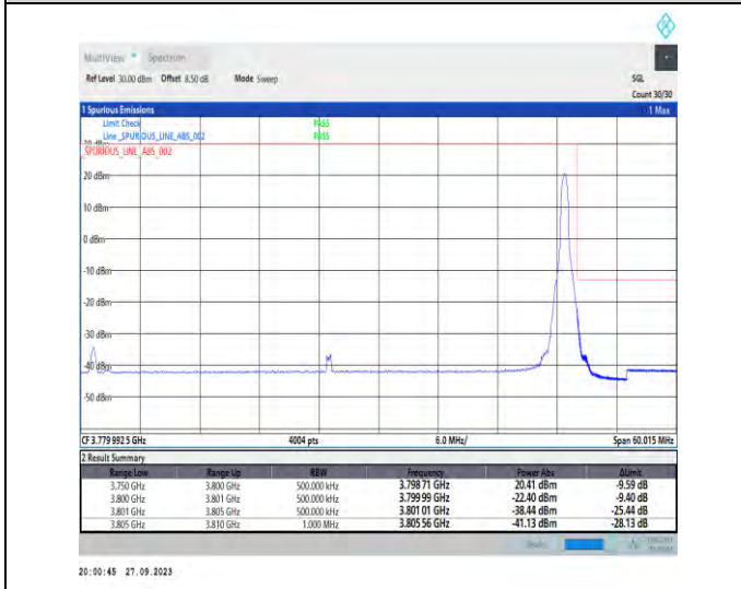
1-N78-3700-3800-PC2-30-50-H-5-CP-QPSK-Edge_1RB_Right-1@132-Ant7-1--PASS-see graph
