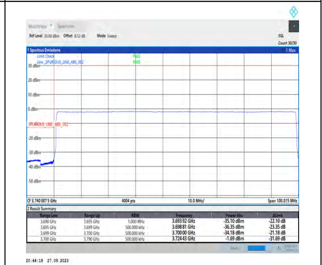
1-N78-3700-3800-PC2-30-90-L-6-CP-QPSK-Outer_Full-245@0-Ant7-1--PASS-see graph
