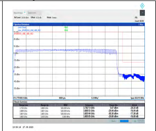
1-N78-3700-3800-PC2-30-50-H-3-DFT-PI2BPSK-Outer_Full-128@0-Ant7-1--PASS-see graph
