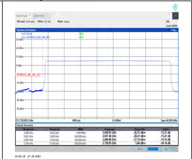
1-N78-3700-3800-PC2-30-50-L-3-DFT-PI2BPSK-Outer_Full-128@0-Ant7-1--PASS-see graph
