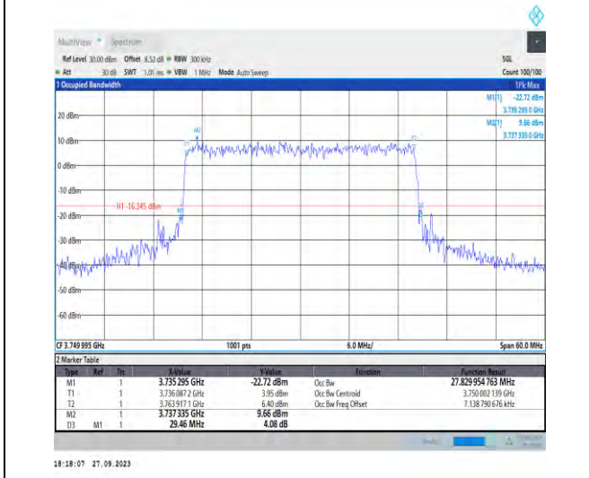
1-N78-3700-3800-PC2-30-30-M-8-CP-64QAM-Outer_Full-78@0-Ant7-27.83-29.460-≤30-PASS
