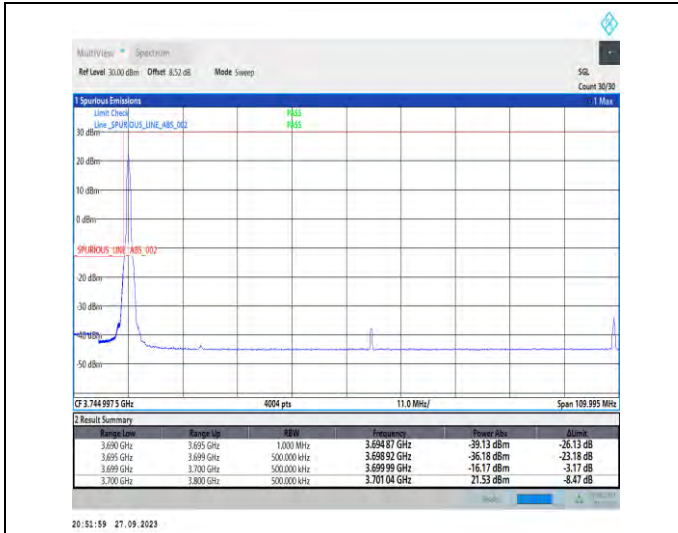
1-N78-3700-3800-PC2-30-100-L-1-DFT-PI2BPSK-Edge_1_RB_Left-1@0-Ant7-1--PASS-see graph
