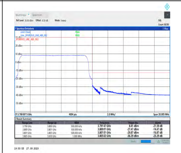
1-N78-3700-3800-PC2-30-10-H-6-CP-QPSK-Outer_Full-24@0-Ant7-1--PASS-see graph
