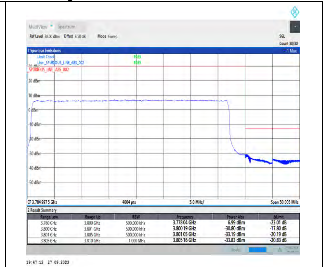
1-N78-3700-3800-PC2-30-40-H-3-DFT-PI2BPSK-Outer_Full-100@0-Ant7-1--PASS-see graph
