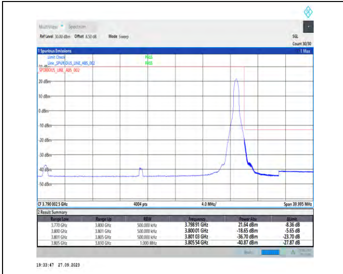
1-N78-3700-3800-PC2-30-30-H-2-DFT-PI2BPSK-Edge_1RB_Right-1@77-Ant7-1--PASS-see graph
