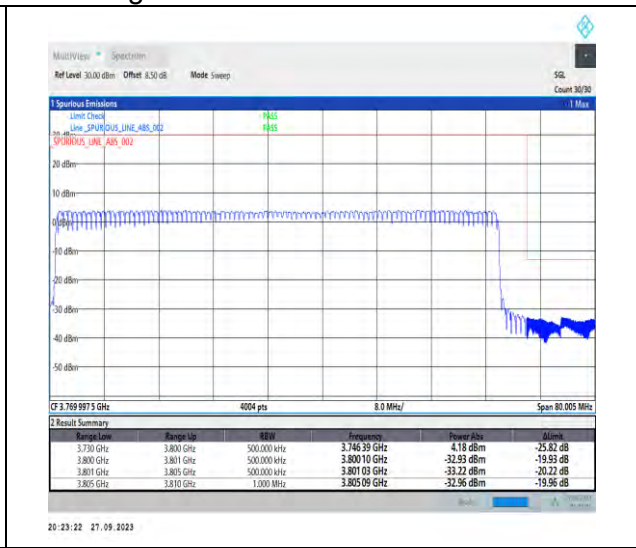
1-N78-3700-3800-PC2-30-70-H-3-DFT-PI2BPSK-Outer_Full-180@0-Ant7-1--PASS-see graph
