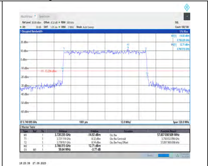
1-N78-3700-3800-PC2-30-60-M-4-DFT-64QAM-Outer_Full-162@0-Ant7-57.837-59.640-≤60-PASS
