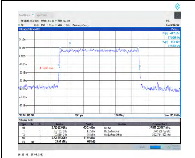
1-N78-3700-3800-PC2-30-60-M-5-DFT-256QAM-Outer_Full-162@0-Ant7-57.811-59.640-≤60-PASS
