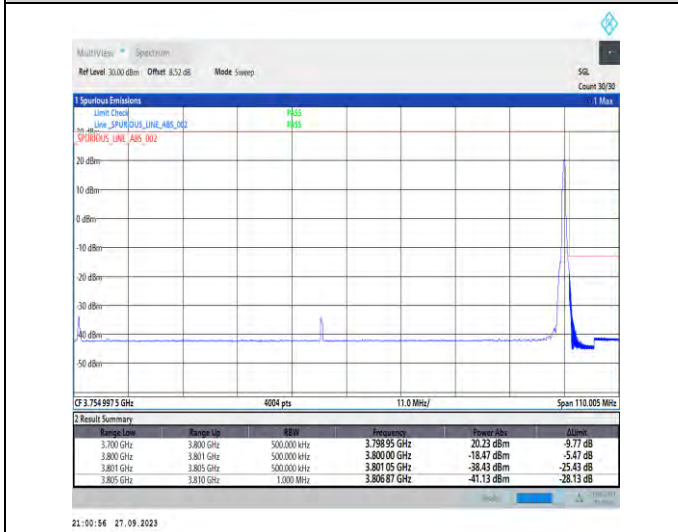
1-N78-3700-3800-PC2-30-100-H-5-CP-QPSK-Edge_1_RB_Right-1@272-Ant7-1--PASS-see graph
