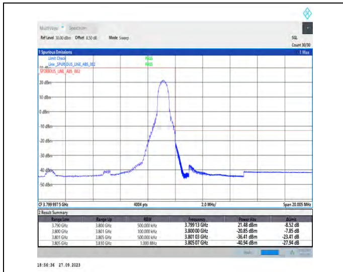
1-N78-3700-3800-PC2-30-10-H-2-DFT-PI2BPSK-Edge_1RB_Right-1@23-Ant7-1--PASS-see graph
