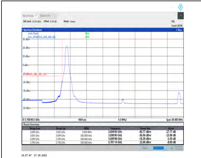
1-N78-3700-3800-PC2-30-30-L-1-DFT-PI2BPSK-Edge_1RB_Left-1@0-Ant7-1--PASS-see graph
