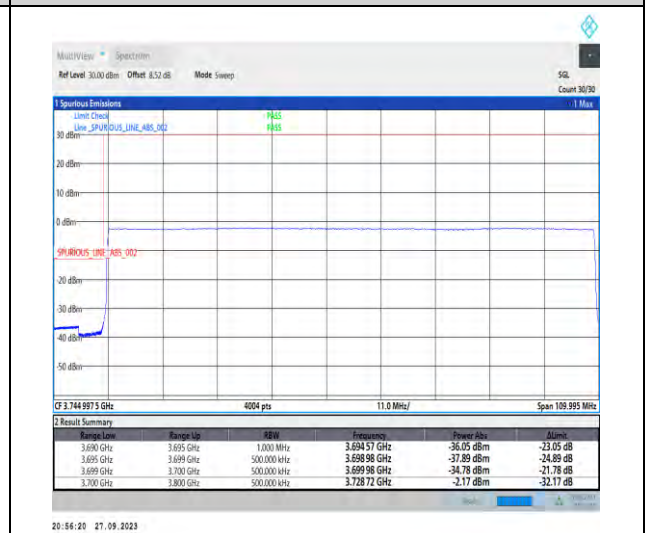
1-N78-3700-3800-PC2-30-100-L-6-CP-QPSK-Outer_Full-273@0-Ant7-1--PASS-see graph
