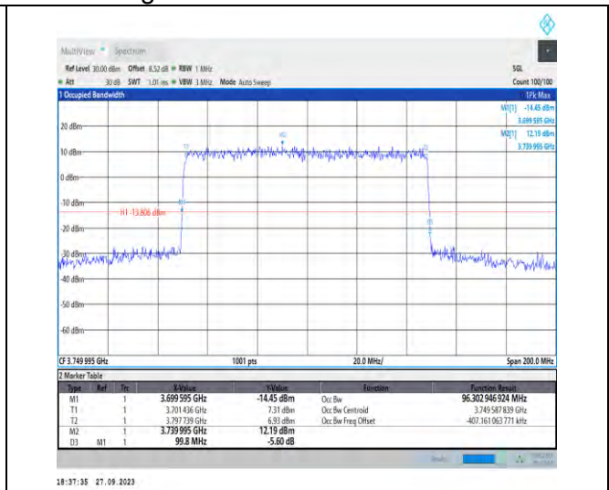
1-N78-3700-3800-PC2-30-100-M-4-DFT-64QAM-Out er_Full-270@0-Ant7-96.303-99.800-≤100-PASS
