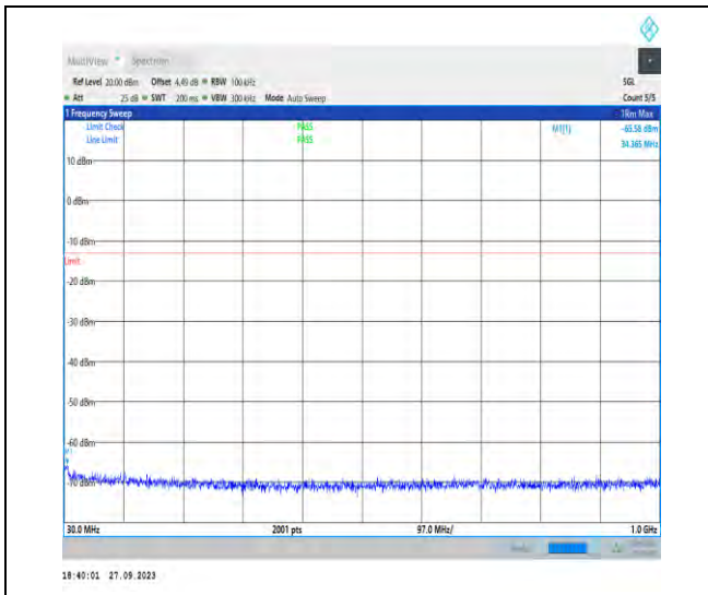
1-N78-3700-3800-PC2-30-100-M-1-DFT-PI2BPSK- Inner_1RB_Left-1@1-30-1000-Ant7-34.37--65.58--1 3-PASS
