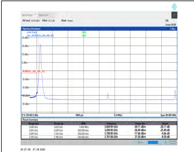
1-N78-3700-3800-PC2-30-80-L-1-DFT-PI2BPSK-Edge_1RB_Left-1@0-Ant7-1--PASS-see graph
