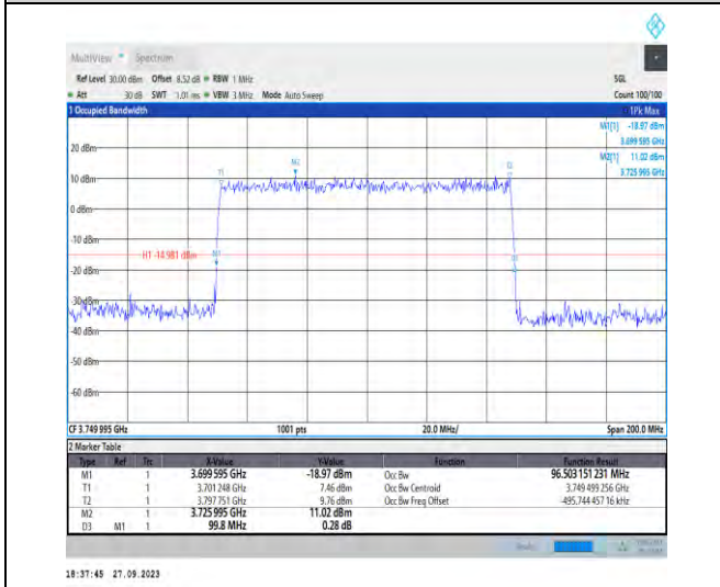
1-N78-3700-3800-PC2-30-100-M-5-DFT-256QAM-Out er_Full-270@0-Ant7-96.503-99.800-≤100-PASS
