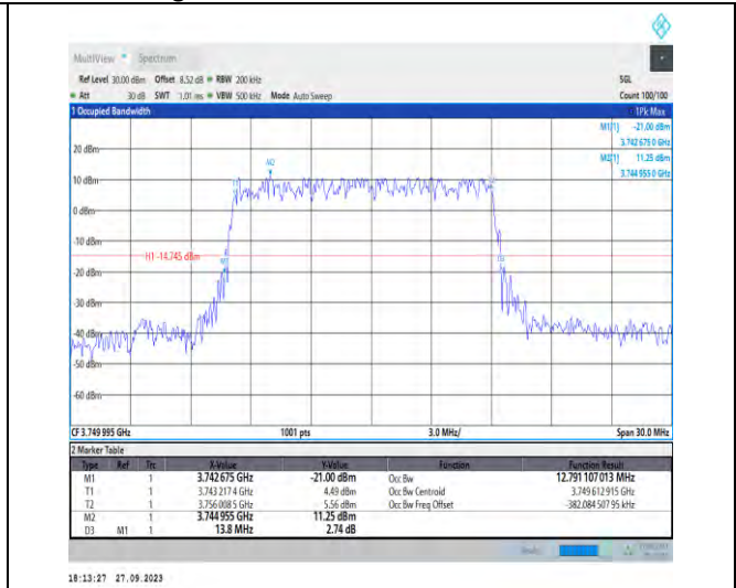
1-N78-3700-3800-PC2-30-15-M-5-DFT-256QAM-Outer_Full-36@0-Ant7-12.791-13.800-≤15-PASS
