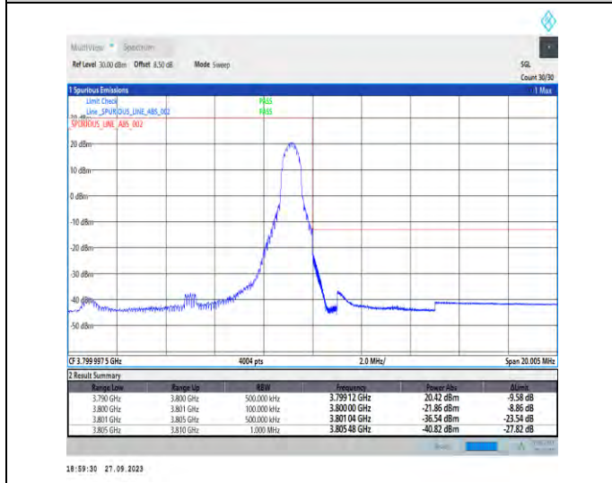
1-N78-3700-3800-PC2-30-10-H-5-CP-QPSK-Edge_1RB_Right-1@23-Ant7-1--PASS-see graph
