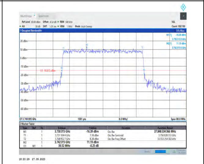
1-N78-3700-3800-PC2-30-40-M-8-CP-64QAM-Outer _Full-106@0-Ant7-37.848-39.520-≤40-PASS
