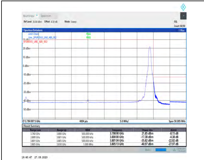
1-N78-3700-3800-PC2-30-40-H-2-DFT-PI2BPSK-Edge_1RB_Right-1@105-Ant7-1--PASS-see graph
