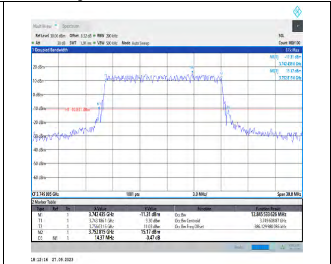
1-N78-3700-3800-PC2-30-15-M-1-DFT-QPSK-Outer_Full-36@0-Ant7-12.846-14.370-≤15-PASS
