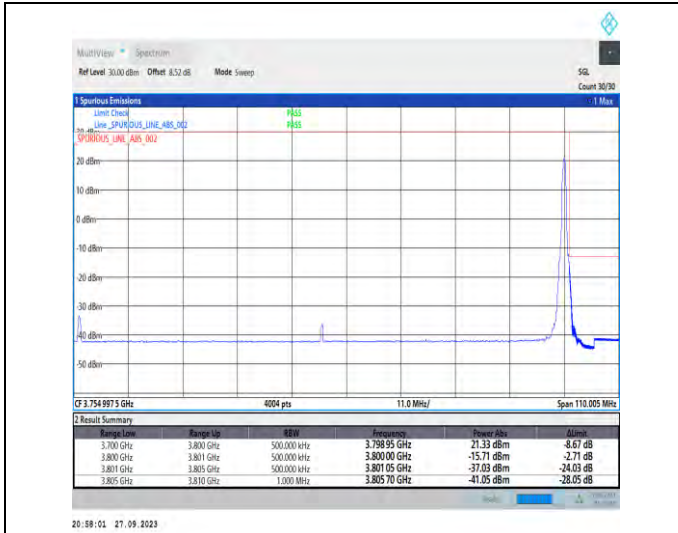
1-N78-3700-3800-PC2-30-100-H-2-DFT-PI2BPSK-Edge_1_RB_Right-1@272-Ant7-1--PASS-see graph
