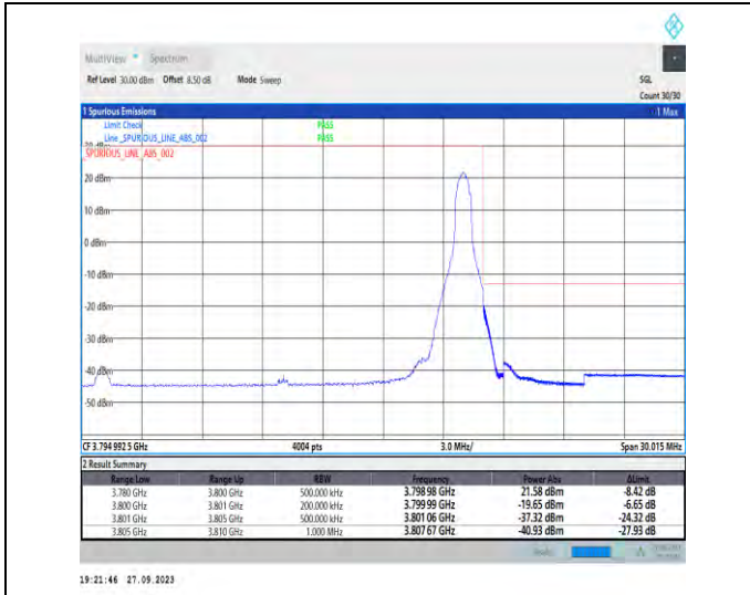
1-N78-3700-3800-PC2-30-20-H-2-DFT-PI2BPSK-Edge_1RB_Right-1@50-Ant7-1--PASS-see graph
