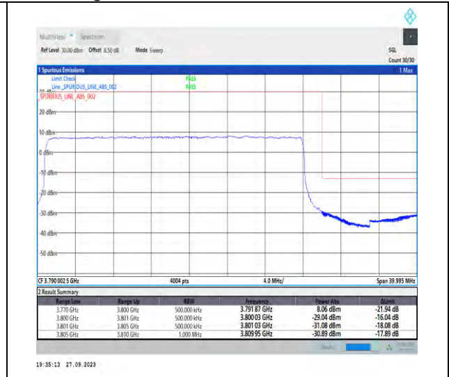
1-N78-3700-3800-PC2-30-30-H-3-DFT-PI2BPSK-Outer_Full-75@0-Ant7-1--PASS-see graph
