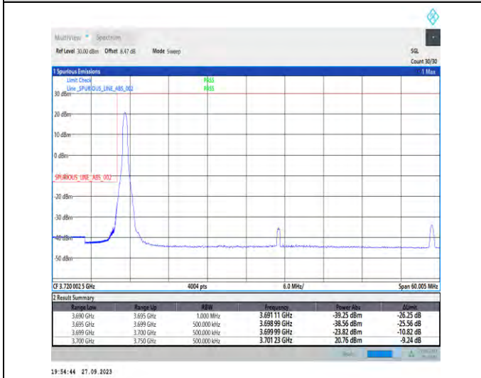
1-N78-3700-3800-PC2-30-50-L-4-CP-QPSK-Edge_1RB_Left-1@0-Ant7-1--PASS-see graph
