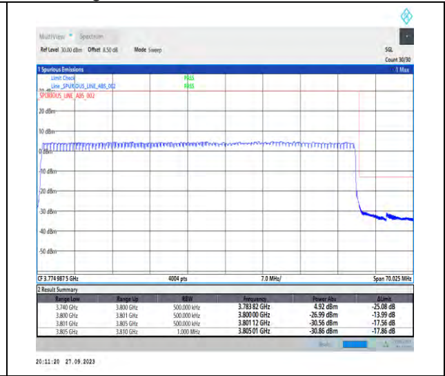
1-N78-3700-3800-PC2-30-60-H-3-DFT-PI2BPSK-Outer_Full-162@0-Ant7-1--PASS-see graph
