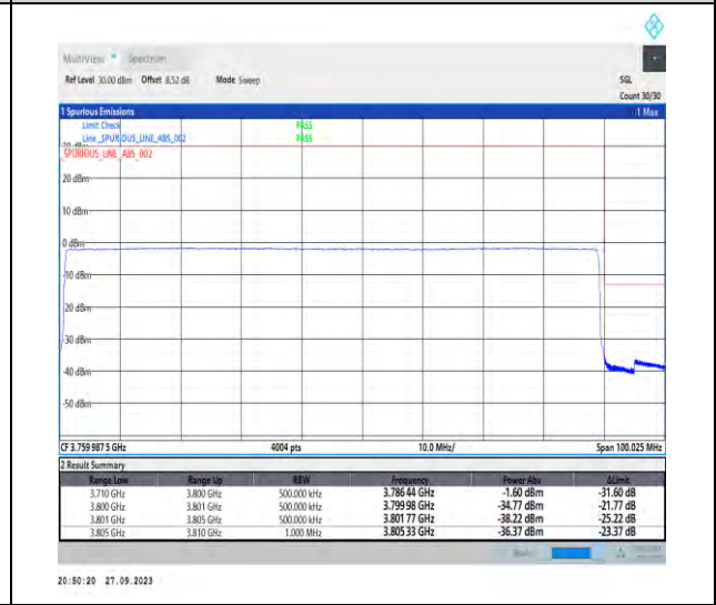
1-N78-3700-3800-PC2-30-90-H-6-CP-QPSK-Outer_Full-245@0-Ant7-1--PASS-see graph
