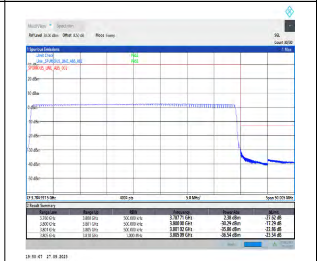
1-N78-3700-3800-PC2-30-40-H-6-CP-QPSK-Outer_Full-106@0-Ant7-1--PASS-see graph
