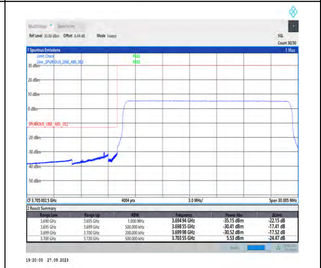
1-N78-3700-3800-PC2-30-20-L-6-CP-QPSK-Outer_Full-51@0-Ant7-1--PASS-see graph
