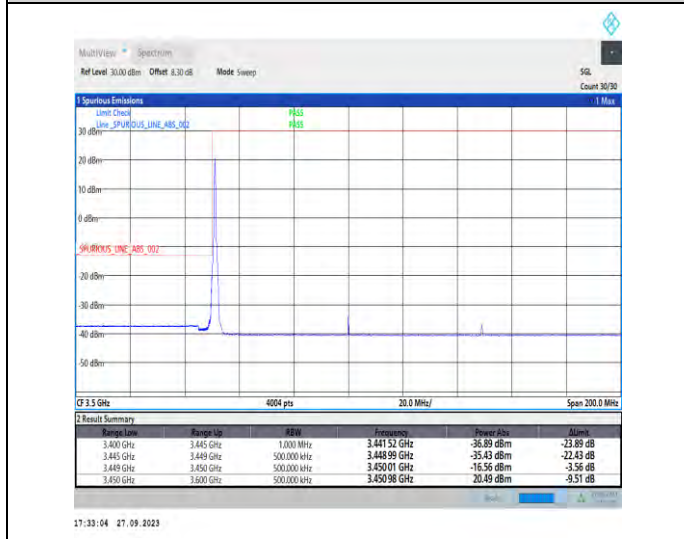
1-N78-3450-3550-PC2-30-100-L-4-CP-QPSK-Edge_1_RB_Left-1@0-Ant7-1--PASS-see graph
