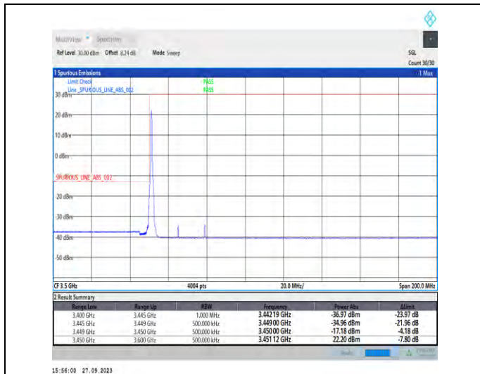
1-N78-3450-3550-PC2-30-30-L-1-DFT-PI2BPSK-Edge_1RB_Left-1@0-Ant7-1--PASS-see graph
