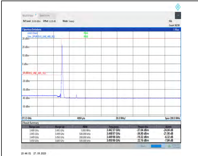
1-N78-3450-3550-PC2-30-20-L-1-DFT-PI2BPSK-Edge_1RB_Left-1@0-Ant7-1--PASS-see graph
