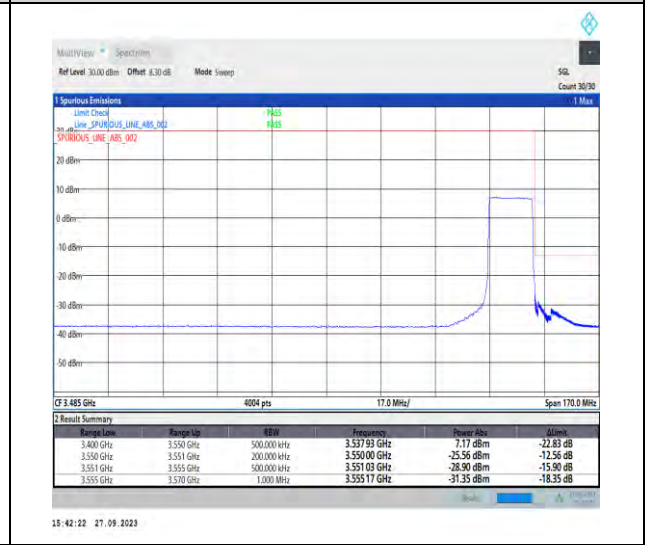
1-N78-3450-3550-PC2-30-15-H-6-CP-QPSK-Outer_Full-38@0-Ant7-1--PASS-see graph
