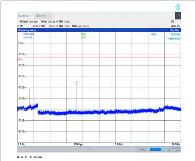
1-N78-3450-3550-PC2-30-100-H-1-DFT-PI2BPSK-In ner_1RB_Left-1@1-6000-18000-Ant7-10354.08--38. 81--13-PASS
