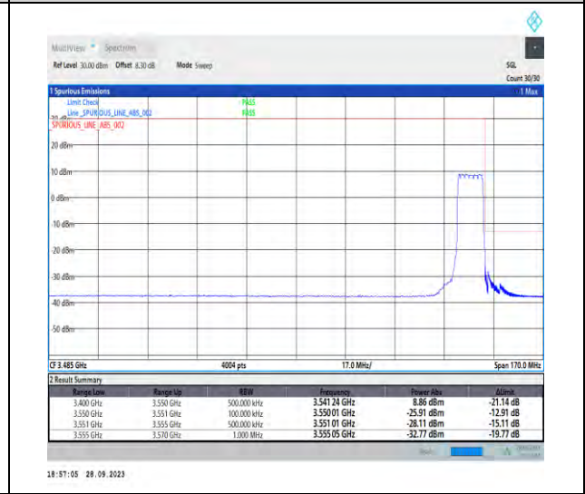
1-N78-3450-3550-PC2-30-10-H-6-CP-QPSK-Outer_Full-24@0-Ant7-1--PASS-see graph
