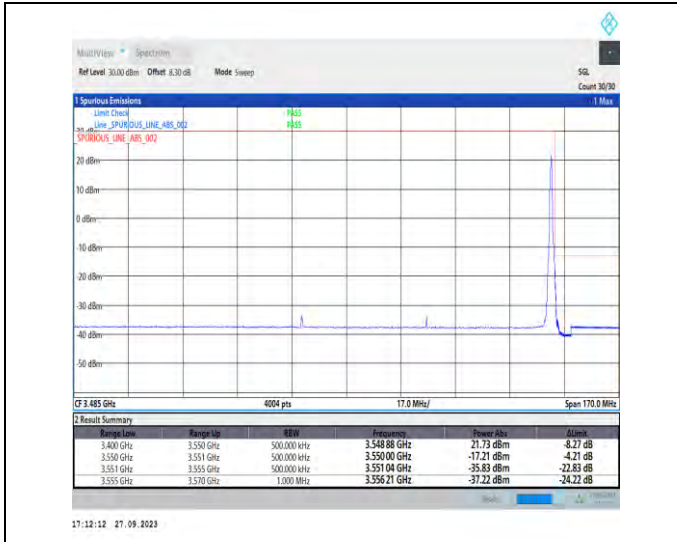
1-N78-3450-3550-PC2-30-80-H-2-DFT-PI2BPSK-Edge_1RB_Right-1@216-Ant7-1--PASS-see graph
