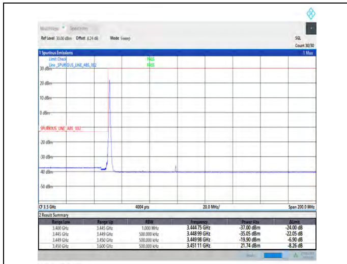
1-N78-3450-3550-PC2-30-50-L-1-DFT-PI2BPSK-Edge_1RB_Left-1@0-Ant7-1--PASS-see graph
