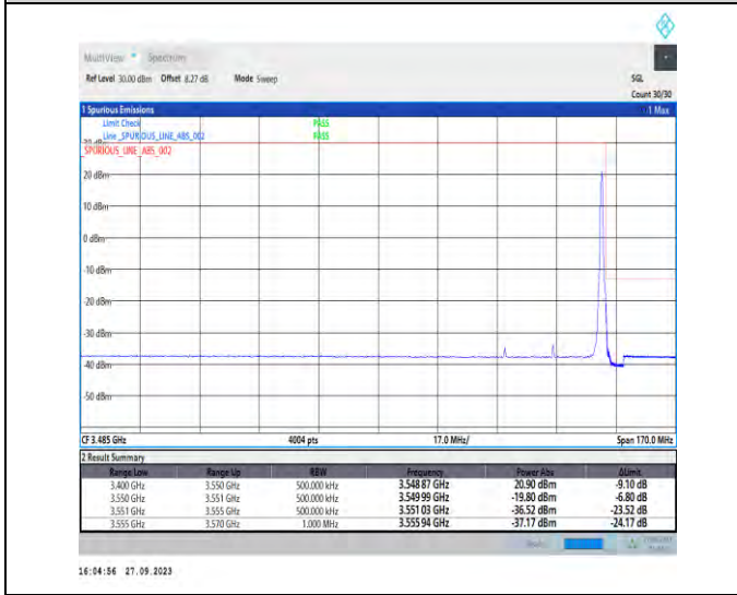
1-N78-3450-3550-PC2-30-30-H-5-CP-QPSK-Edge_1RB_Right-1@77-Ant7-1--PASS-see graph
