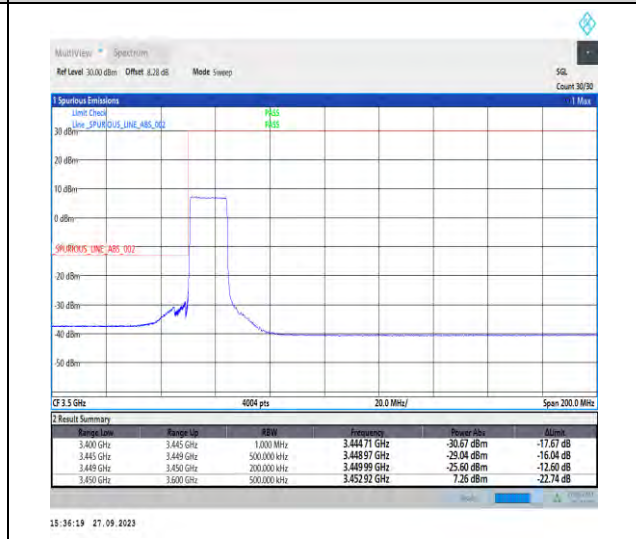
1-N78-3450-3550-PC2-30-15-L-6-CP-QPSK-Outer_Full-38@0-Ant7-1--PASS-see graph
