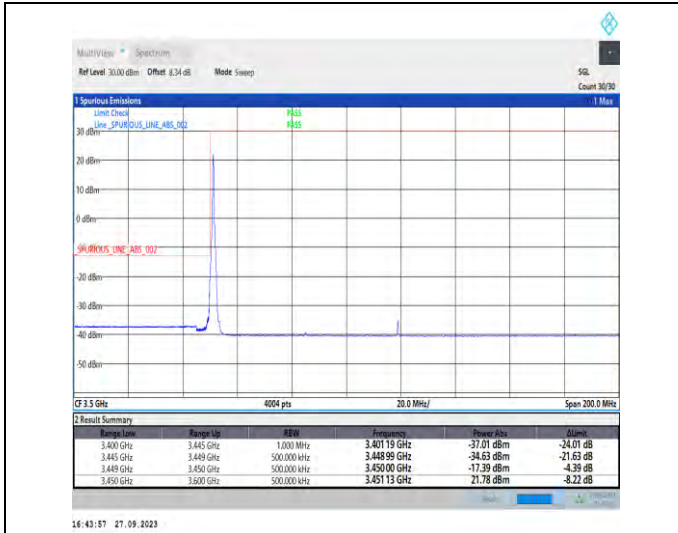
1-N78-3450-3550-PC2-30-70-L-1-DFT-PI2BPSK-Edge_1RB_Left-1@0-Ant7-1--PASS-see graph
