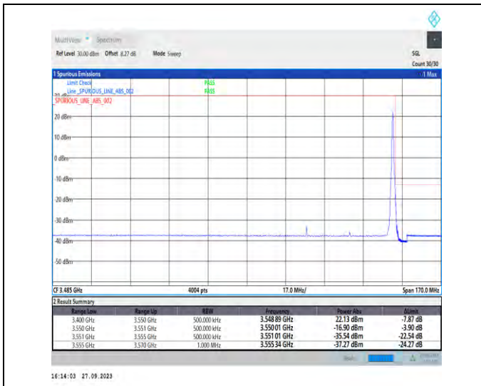
1-N78-3450-3550-PC2-30-40-H-2-DFT-PI2BPSK-Edge_1RB_Right-1@105-Ant7-1--PASS-see graph
