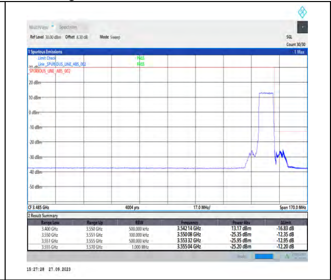
1-N78-3450-3550-PC2-30-10-H-3-DFT-PI2BPSK-Outer_Full-24@0-Ant7-1--PASS-see graph
