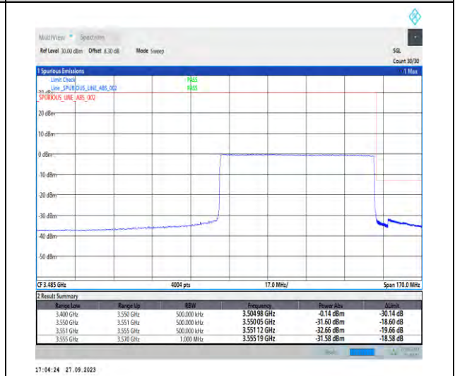
1-N78-3450-3550-PC2-30-70-H-6-CP-QPSK-Outer_Full-189@0-Ant7-1--PASS-see graph
