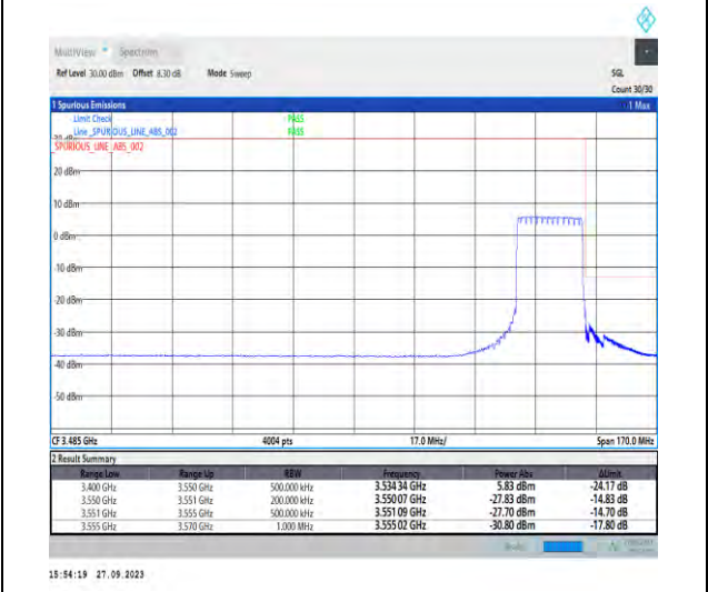
1-N78-3450-3550-PC2-30-20-H-6-CP-QPSK-Outer_Full-51@0-Ant7-1--PASS-see graph
