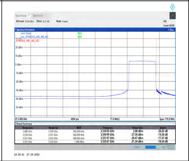
1-N78-3450-3550-PC2-30-30-H-6-CP-QPSK-Outer_Full-78@0-Ant7-1--PASS-see graph
