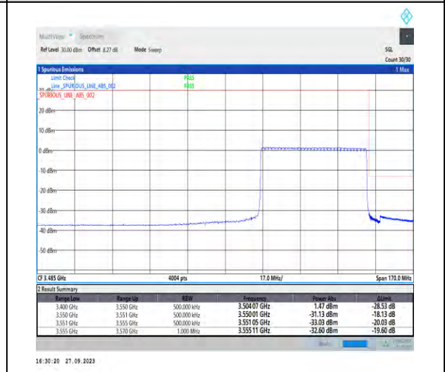
1-N78-3450-3550-PC2-30-50-H-6-CP-QPSK-Outer_Full-133@0-Ant7-1--PASS-see graph
