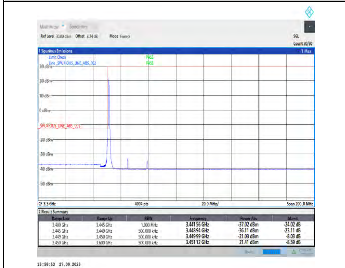
1-N78-3450-3550-PC2-30-30-L-4-CP-QPSK-Edge_1RB_Left-1@0-Ant7-1--PASS-see graph
