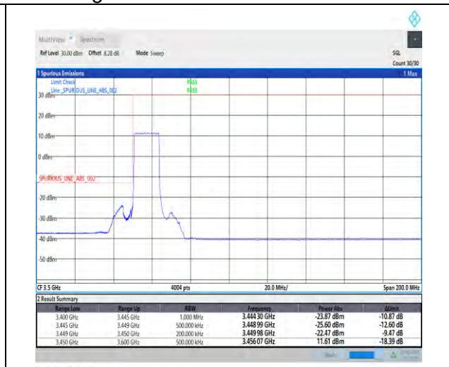
1-N78-3450-3550-PC2-30-15-L-3-DFT-PI2BPSK-Outer_Full-36@0-Ant7-1--PASS-see graph
