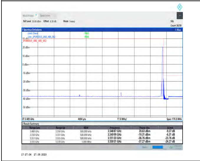
1-N78-3450-3550-PC2-30-90-H-5-CP-QPSK-Edge_1RB_Right-1@244-Ant7-1--PASS-see graph
