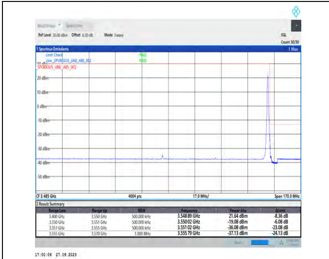
1-N78-3450-3550-PC2-30-70-H-2-DFT-PI2BPSK-Edge_1RB_Right-1@188-Ant7-1--PASS-see graph
