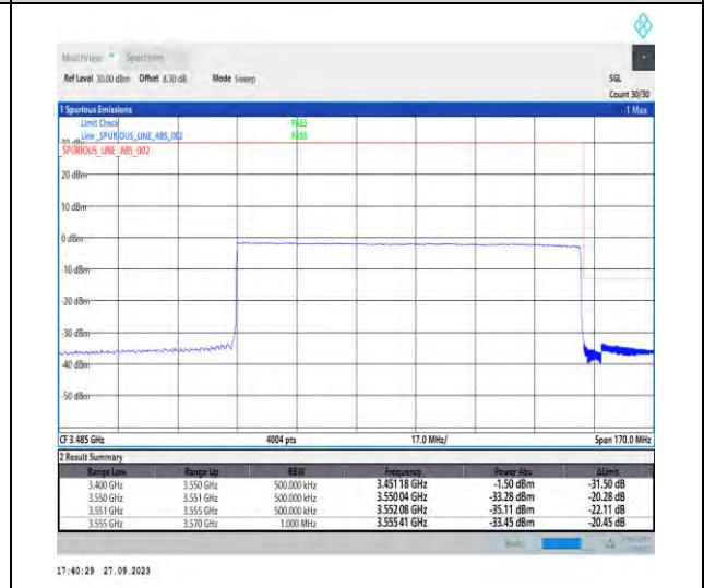
1-N78-3450-3550-PC2-30-100-H-6-CP-QPSK-Outer_Full-273@0-Ant7-1--PASS-see graph
