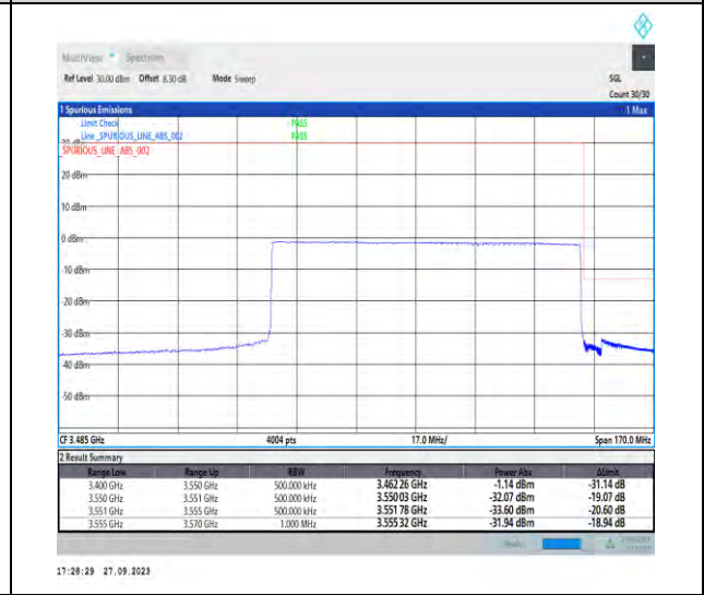
1-N78-3450-3550-PC2-30-90-H-6-CP-QPSK-Outer_Full-245@0-Ant7-1--PASS-see graph
