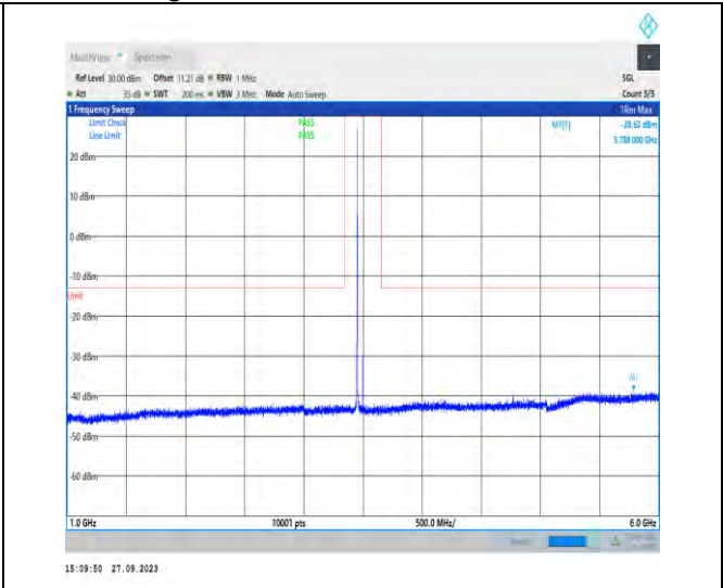
1-N78-3450-3550-PC2-30-100-M-1-DFT-PI2BPSK-In ner_1RB_Left-1@1-1000-6000-Ant7-5788.00--38.62- -13-PASS
