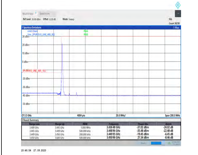
1-N78-3450-3550-PC2-30-20-L-4-CP-QPSK-Edge_1RB_Left-1@0-Ant7-1--PASS-see graph
