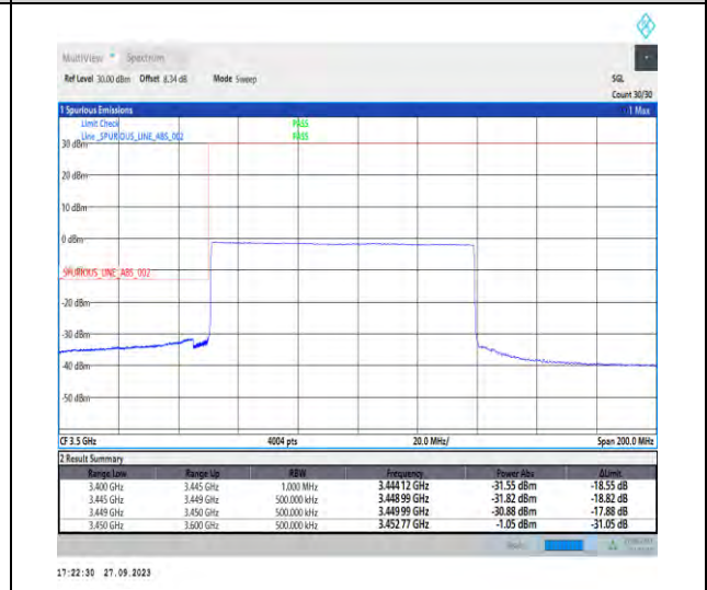
1-N78-3450-3550-PC2-30-90-L-6-CP-QPSK-Outer_Full-245@0-Ant7-1--PASS-see graph
