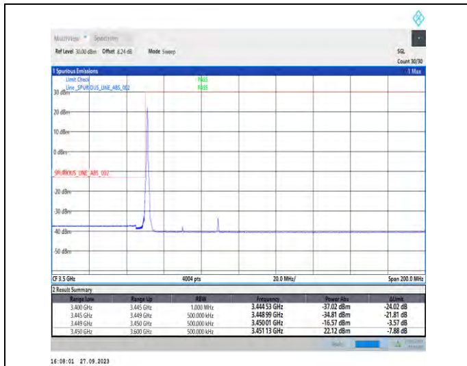
1-N78-3450-3550-PC2-30-40-L-1-DFT-PI2BPSK-Edge_1RB_Left-1@0-Ant7-1--PASS-see graph
