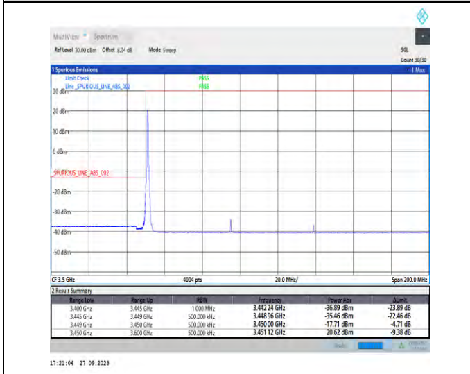
1-N78-3450-3550-PC2-30-90-L-4-CP-QPSK-Edge_1RB_Left-1@0-Ant7-1--PASS-see graph
