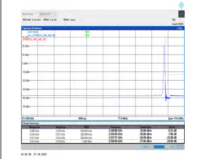
1-N78-3450-3550-PC2-30-20-H-5-CP-QPSK-Edge_1RB_Right-1@50-Ant7-1--PASS-see graph
