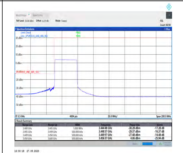
1-N78-3450-3550-PC2-30-30-L-6-CP-QPSK-Outer_Full-78@0-Ant7-1--PASS-see graph
