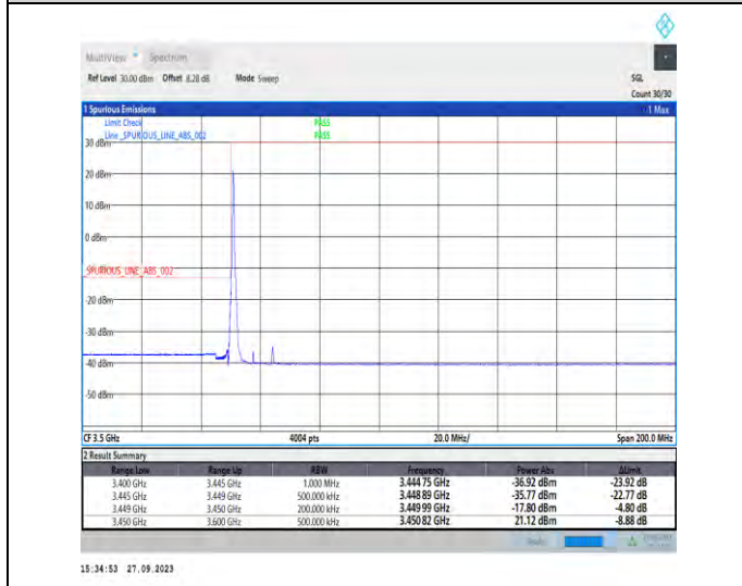
1-N78-3450-3550-PC2-30-15-L-4-CP-QPSK-Edge_1RB_Left-1@0-Ant7-1--PASS-see graph
