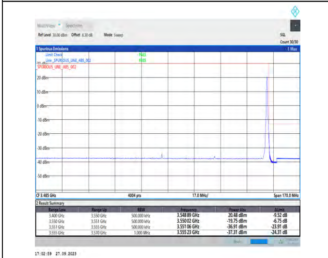
1-N78-3450-3550-PC2-30-70-H-5-CP-QPSK-Edge_1RB_Right-1@188-Ant7-1--PASS-see graph
