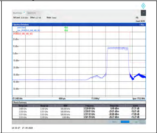
1-N78-3450-3550-PC2-30-30-H-3-DFT-PI2BPSK-Outer_Full-75@0-Ant7-1--PASS-see graph
