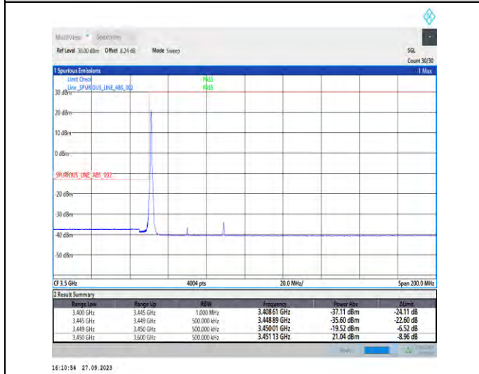
1-N78-3450-3550-PC2-30-40-L-4-CP-QPSK-Edge_1RB_Left-1@0-Ant7-1--PASS-see graph
