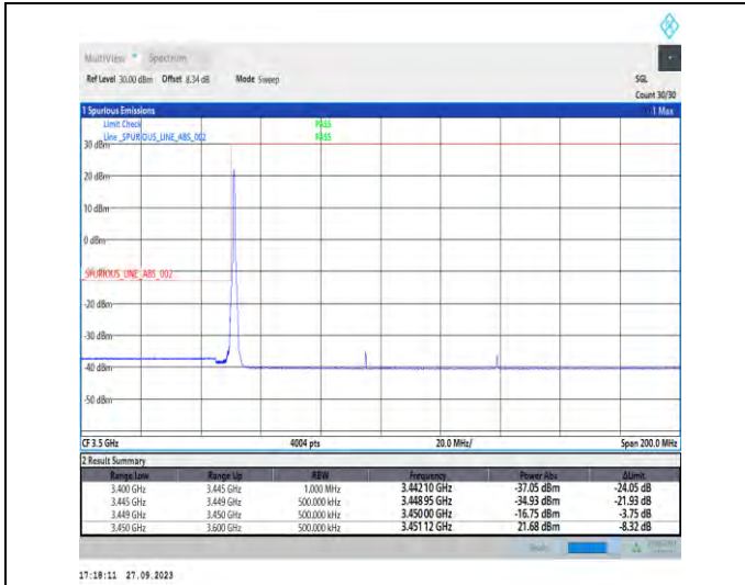
1-N78-3450-3550-PC2-30-90-L-1-DFT-PI2BPSK-Edge_1RB_Left-1@0-Ant7-1--PASS-see graph
