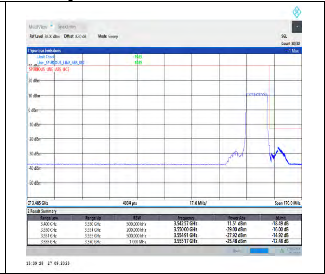
1-N78-3450-3550-PC2-30-15-H-3-DFT-PI2BPSK-Outer_Full-36@0-Ant7-1--PASS-see graph
