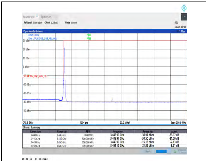
1-N78-3450-3550-PC2-30-60-L-1-DFT-PI2BPSK-Edge_1RB_Left-1@0-Ant7-1--PASS-see graph
