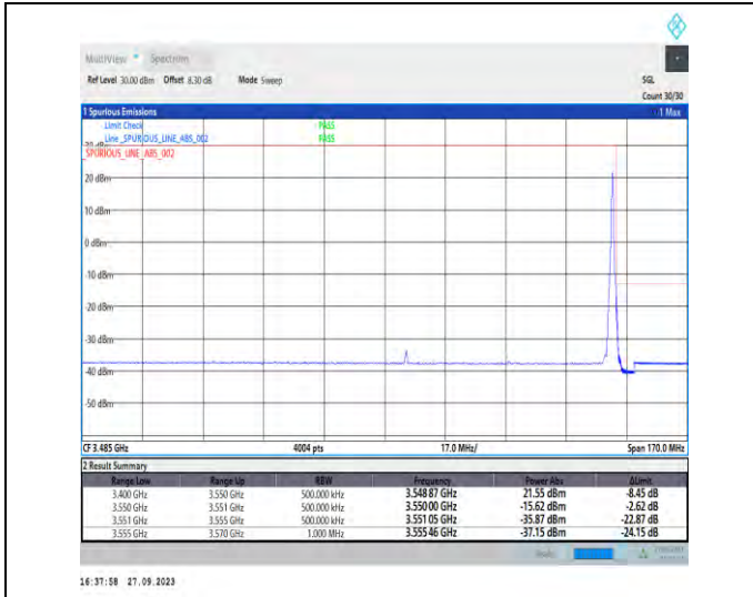
1-N78-3450-3550-PC2-30-60-H-2-DFT-PI2BPSK-Edge_1RB_Right-1@161-Ant7-1--PASS-see graph
