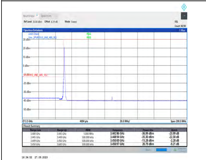
1-N78-3450-3550-PC2-30-60-L-4-CP-QPSK-Edge_1RB_Left-1@0-Ant7-1--PASS-see graph
