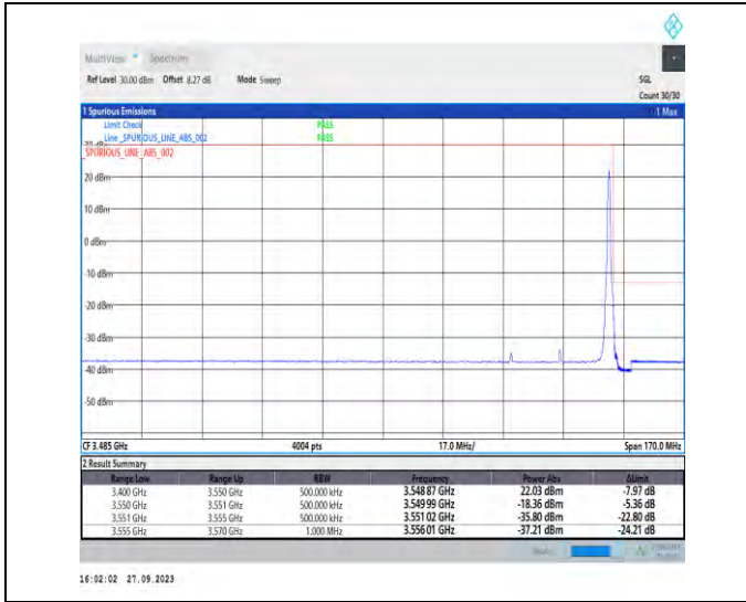
1-N78-3450-3550-PC2-30-30-H-2-DFT-PI2BPSK-Edge_1RB_Right-1@77-Ant7-1--PASS-see graph
