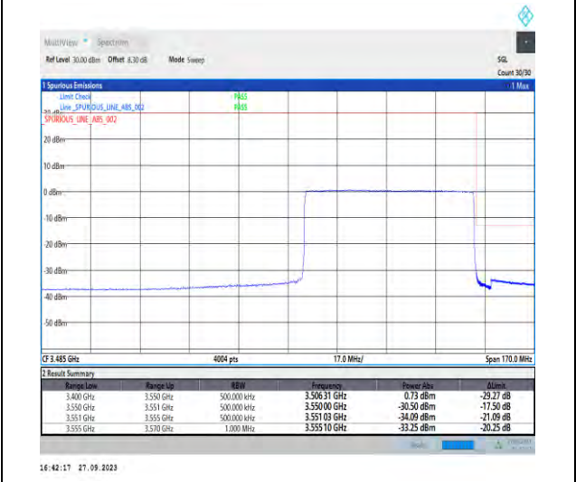
1-N78-3450-3550-PC2-30-60-H-6-CP-QPSK-Outer_Full-162@0-Ant7-1--PASS-see graph
