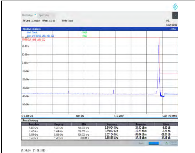
1-N78-3450-3550-PC2-30-100-H-2-DFT-PI2BPSK-Edge_1RB_Right-1@272-Ant7-1--PASS-see graph
