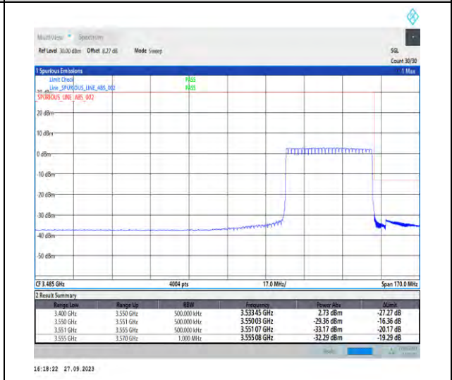
1-N78-3450-3550-PC2-30-40-H-6-CP-QPSK-Outer_Full-106@0-Ant7-1--PASS-see graph
