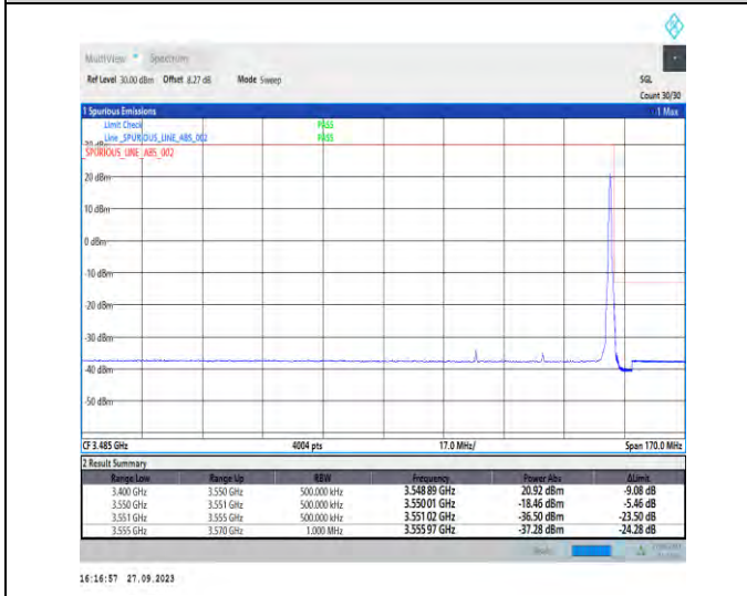
1-N78-3450-3550-PC2-30-40-H-5-CP-QPSK-Edge_1RB_Right-1@105-Ant7-1--PASS-see graph
