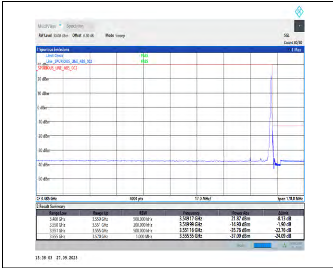
1-N78-3450-3550-PC2-30-15-H-2-DFT-PI2BPSK-Edge_1RB_Right-1@37-Ant7-1--PASS-see graph
