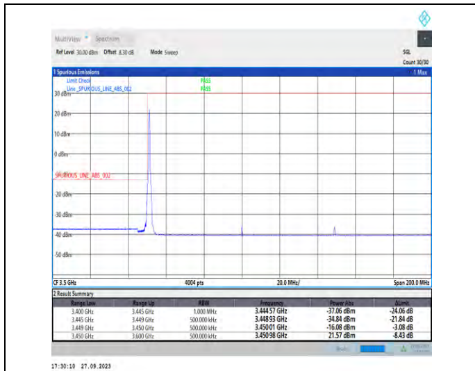
1-N78-3450-3550-PC2-30-100-L-1-DFT-PI2BPSK-Edge_1_RB_Left-1@0-Ant7-1--PASS-see graph
