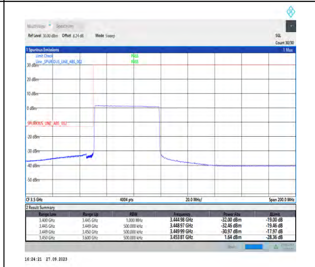
1-N78-3450-3550-PC2-30-50-L-6-CP-QPSK-Outer_Full-133@0-Ant7-1--PASS-see graph
