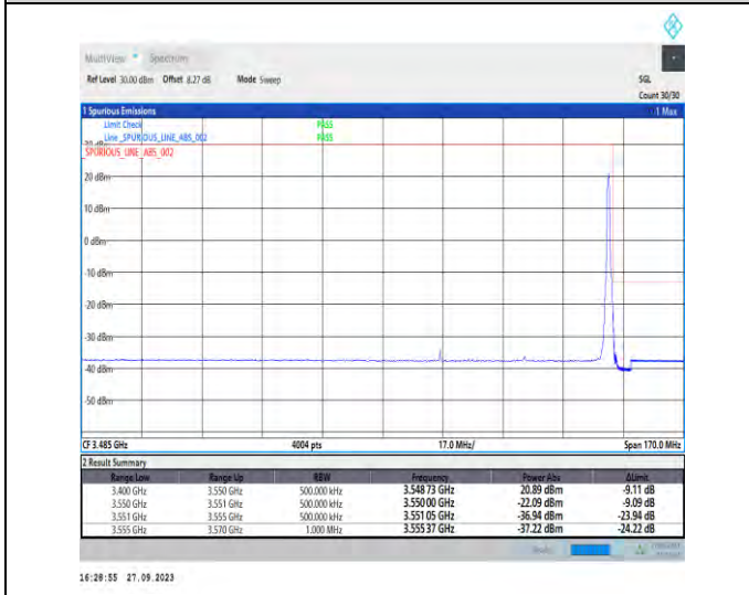
1-N78-3450-3550-PC2-30-50-H-5-CP-QPSK-Edge_1RB_Right-1@132-Ant7-1--PASS-see graph
