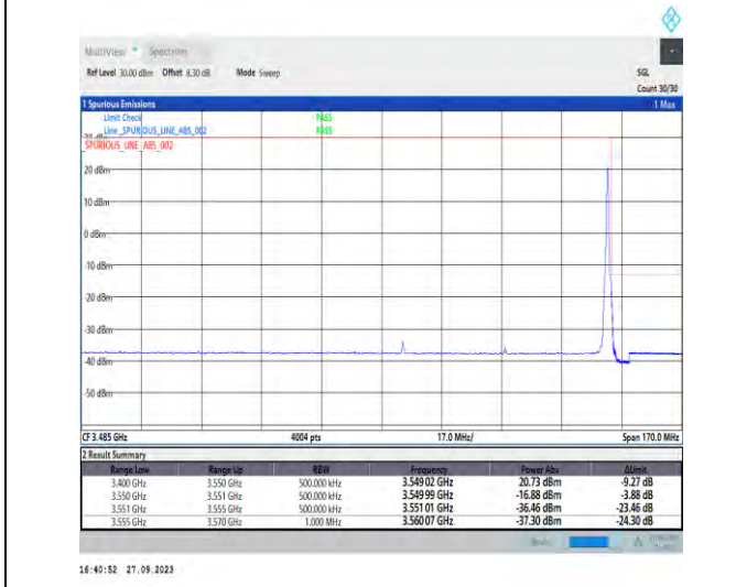
1-N78-3450-3550-PC2-30-60-H-5-CP-QPSK-Edge_1RB_Right-1@161-Ant7-1--PASS-see graph
