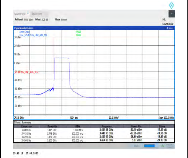
1-N78-3450-3550-PC2-30-20-L-6-CP-QPSK-Outer_Full-51@0-Ant7-1--PASS-see graph
