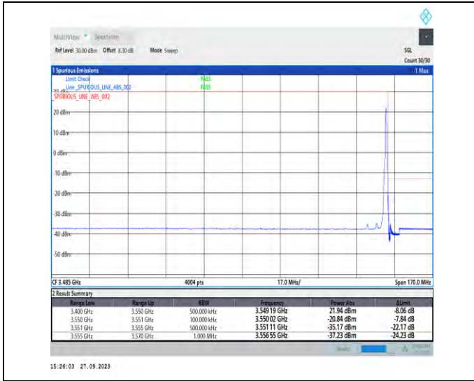
1-N78-3450-3550-PC2-30-10-H-2-DFT-PI2BPSK-Edge_1RB_Right-1@23-Ant7-1--PASS-see graph
