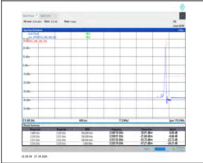
1-N78-3450-3550-PC2-30-10-H-5-CP-QPSK-Edge_1RB_Right-1@23-Ant7-1--PASS-see graph
