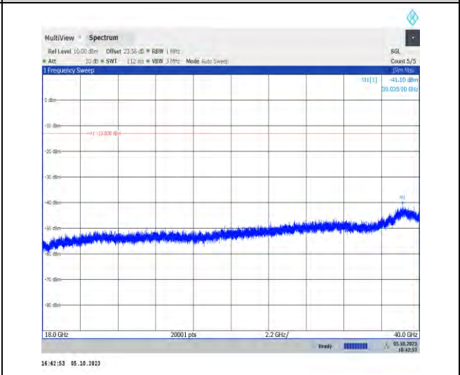
1-N78-3450-3550-PC2-30-100-M-1-DFT-PI2BPSK-In ner_1RB_Left-1@1-18000-40000-Ant7-18000.00--58 .27--13-PASS
