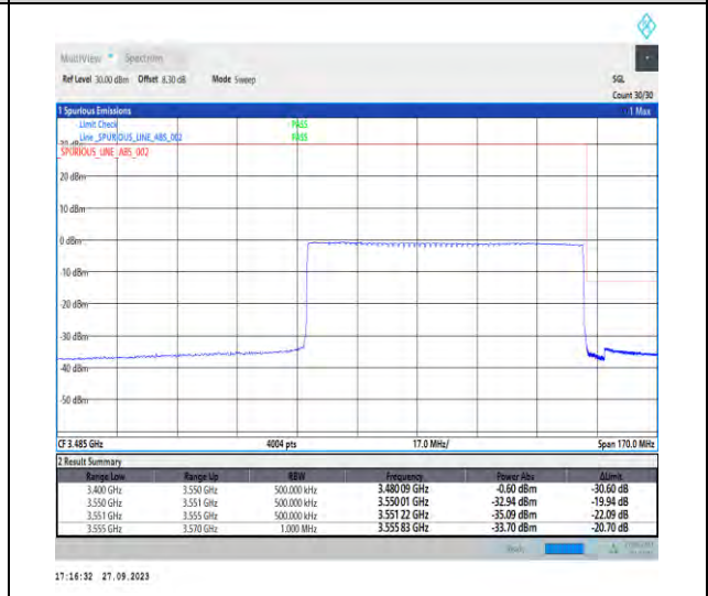
1-N78-3450-3550-PC2-30-80-H-6-CP-QPSK-Outer_Full-217@0-Ant7-1--PASS-see graph
