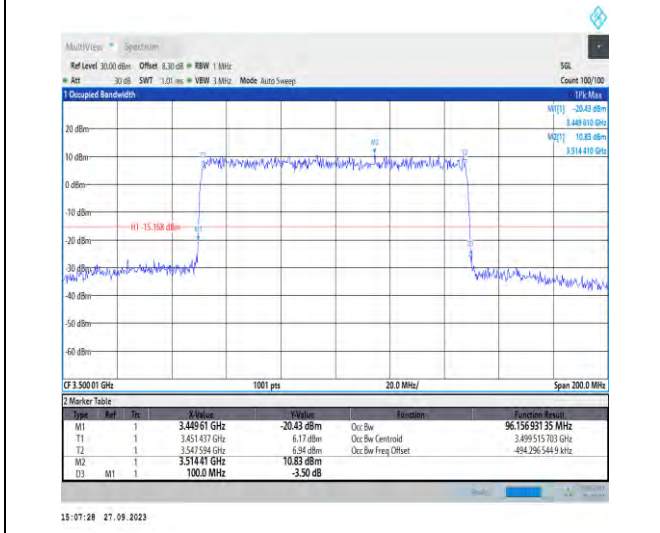
1-N78-3450-3550-PC2-30-100-M-5-DFT-256QAM-Out er_Full-270@0-Ant7-96.157-100.000-≤100-PASS
