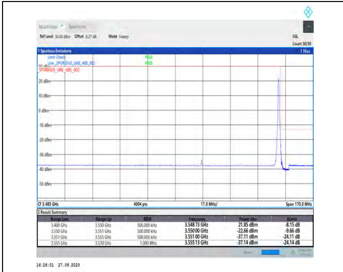
1-N78-3450-3550-PC2-30-50-H-2-DFT-PI2BPSK-Edge_1RB_Right-1@132-Ant7-1--PASS-see graph
