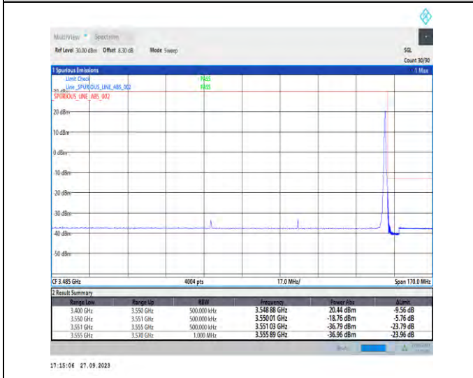
1-N78-3450-3550-PC2-30-80-H-5-CP-QPSK-Edge_1RB_Right-1@216-Ant7-1--PASS-see graph
