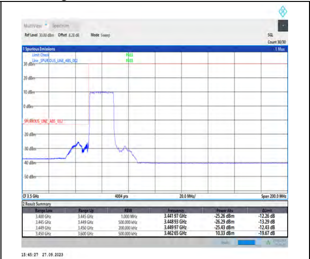
1-N78-3450-3550-PC2-30-20-L-3-DFT-PI2BPSK-Outer_Full-50@0-Ant7-1--PASS-see graph
