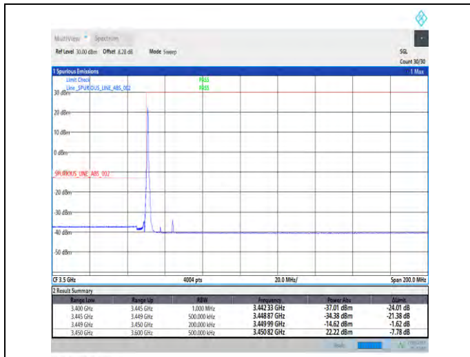
1-N78-3450-3550-PC2-30-15-L-1-DFT-PI2BPSK-Edge_1RB_Left-1@0-Ant7-1--PASS-see graph
