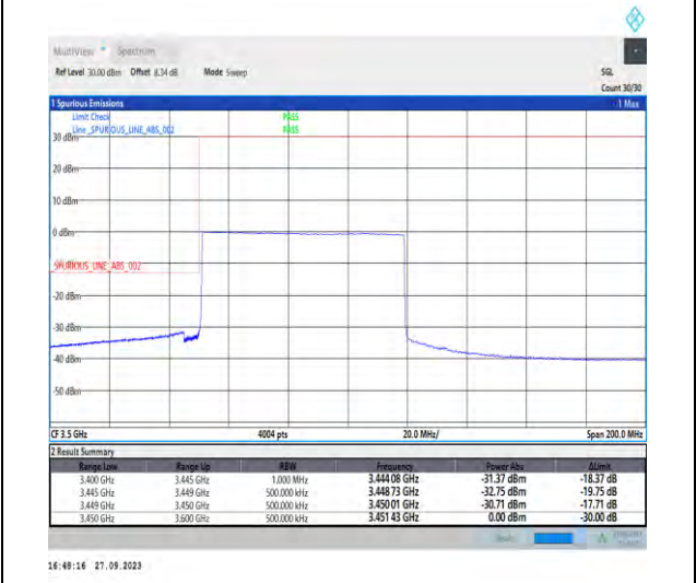
1-N78-3450-3550-PC2-30-70-L-6-CP-QPSK-Outer_Full-189@0-Ant7-1--PASS-see graph
