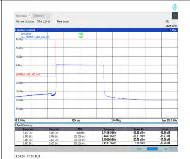
1-N78-3450-3550-PC2-30-60-L-6-CP-QPSK-Outer_Full-162@0-Ant7-1--PASS-see graph
