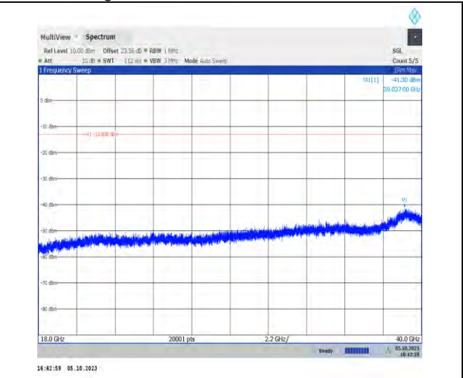
1-N78-3450-3550-PC2-30-100-H-1-DFT-PI2BPSK-In ner_1RB_Left-1@1-18000-40000-Ant7-18000.00--58. .25--13-PASS
