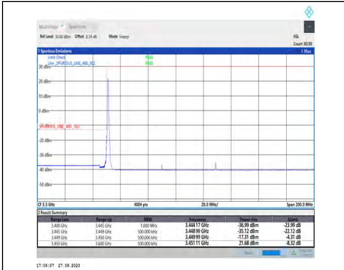
1-N78-3450-3550-PC2-30-80-L-1-DFT-PI2BPSK-Edge_1RB_Left-1@0-Ant7-1--PASS-see graph
