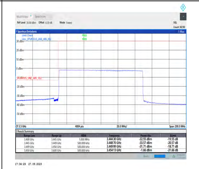
1-N78-3450-3550-PC2-30-100-L-6-CP-QPSK-Outer_Full-273@0-Ant7-1--PASS-see graph
