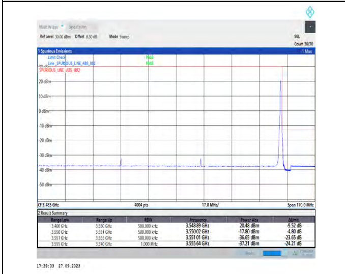
1-N78-3450-3550-PC2-30-100-H-5-CP-QPSK-Edge_1RB_Right-1@272-Ant7-1--PASS-see graph
