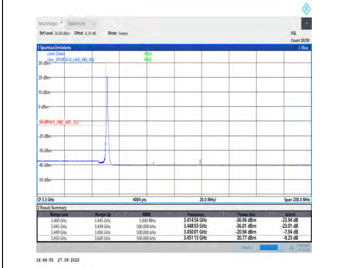
1-N78-3450-3550-PC2-30-70-L-4-CP-QPSK-Edge_1RB_Left-1@0-Ant7-1--PASS-see graph
