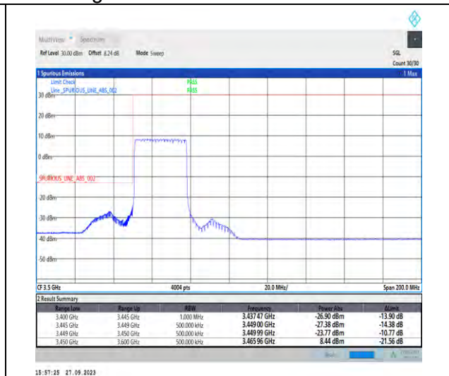
1-N78-3450-3550-PC2-30-30-L-3-DFT-PI2BPSK-Outer_Full-75@0-Ant7-1--PASS-see graph
