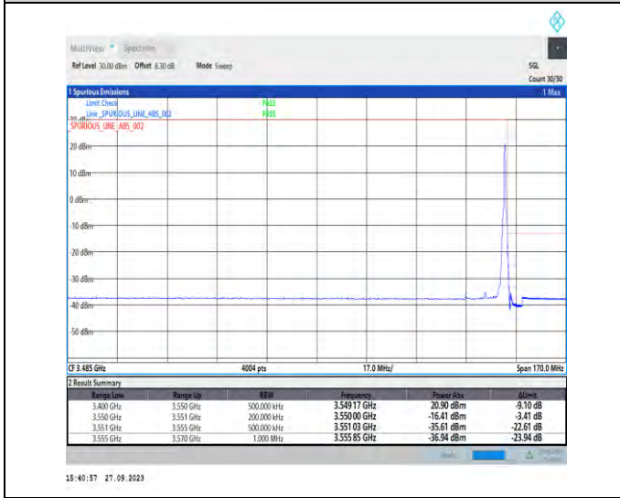
1-N78-3450-3550-PC2-30-15-H-5-CP-QPSK-Edge_1RB_Right-1@37-Ant7-1--PASS-see graph
