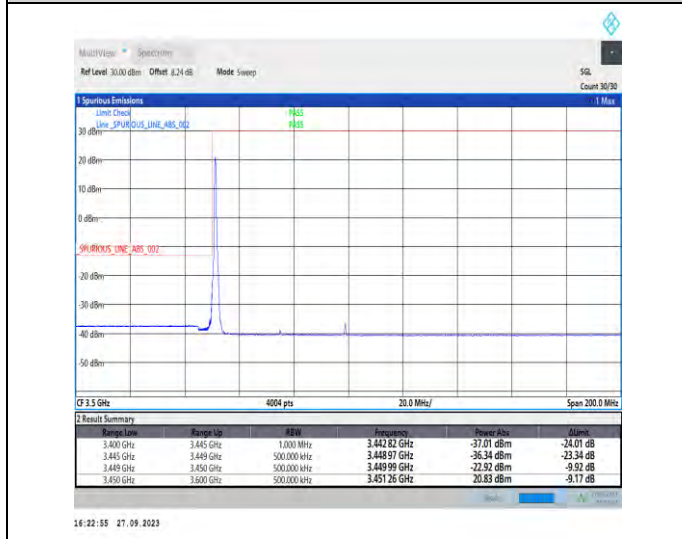
1-N78-3450-3550-PC2-30-50-L-4-CP-QPSK-Edge_1RB_Left-1@0-Ant7-1--PASS-see graph
