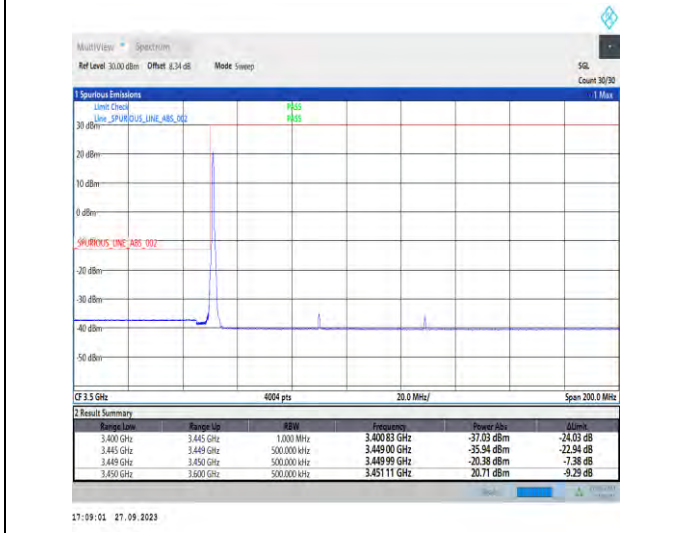
1-N78-3450-3550-PC2-30-80-L-4-CP-QPSK-Edge_1RB_Left-1@0-Ant7-1--PASS-see graph
