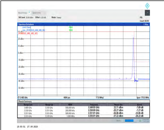
1-N78-3450-3550-PC2-30-20-H-2-DFT-PI2BPSK-Edge_1RB_Right-1@50-Ant7-1--PASS-see graph
