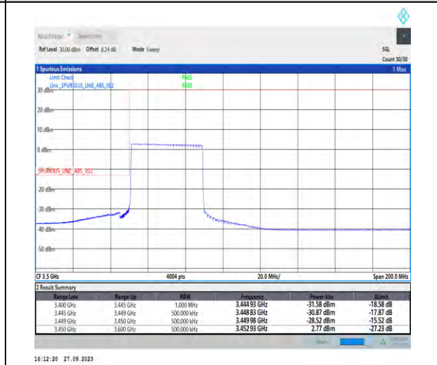
1-N78-3450-3550-PC2-30-40-L-6-CP-QPSK-Outer_Full-106@0-Ant7-1--PASS-see graph
