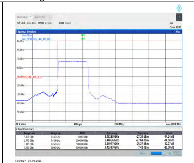
1-N78-3450-3550-PC2-30-40-L-3-DFT-PI2BPSK-Outer_Full-100@0-Ant7-1--PASS-see graph
