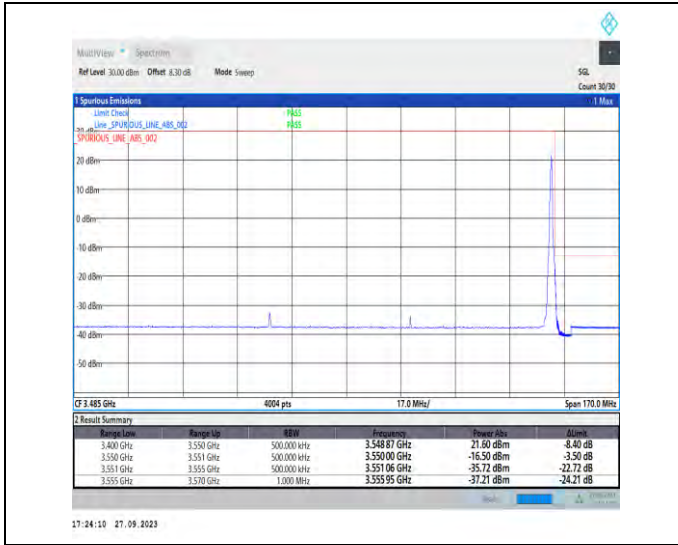
1-N78-3450-3550-PC2-30-90-H-2-DFT-PI2BPSK-Edge_1RB_Right-1@244-Ant7-1--PASS-see graph
