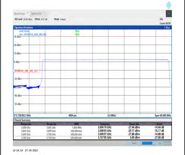
1-N77-3700-3980-PC2-30-50-L-6-CP-QPSK-Outer_Full-133@0-Ant7-1--PASS-see graph
