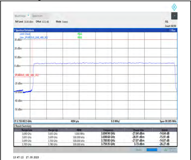
1-N77-3700-3980-PC2-30-80-L-3-DFT-PI2BPSK-Outer_Full-216@0-Ant7-1--PASS-see graph
