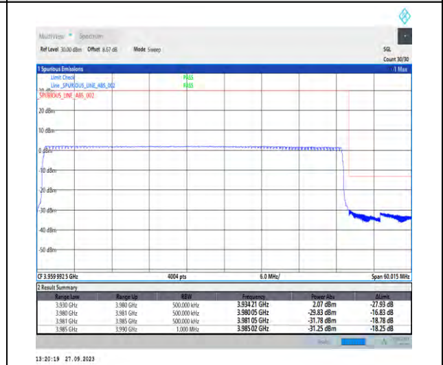
1-N77-3700-3980-PC2-30-50-H-6-CP-QPSK-Outer_Full-133@0-Ant7-1--PASS-see graph
