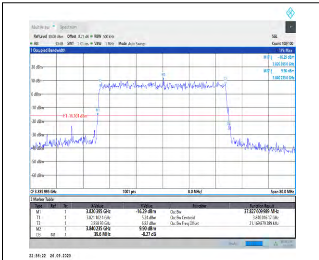
1-N77-3700-3980-PC2-30-40-M-9-CP-256QAM-Out er_Full-106@0-Ant7-37.828-39.600-≤40-PASS
