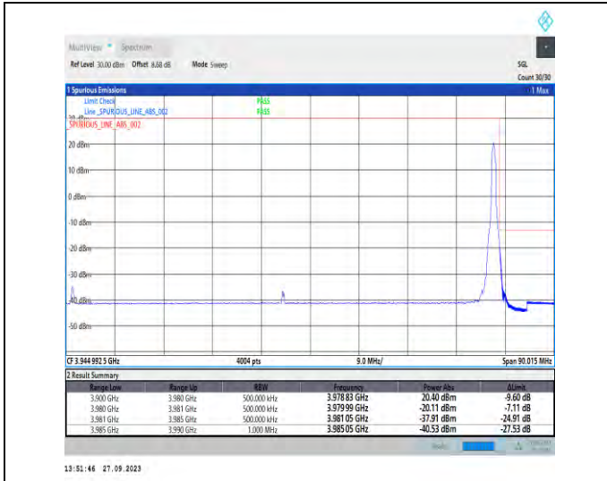
1-N77-3700-3980-PC2-30-80-H-2-DFT-PI2BPSK-Edge_1RB_Right-1@216-Ant7-1--PASS-see graph
