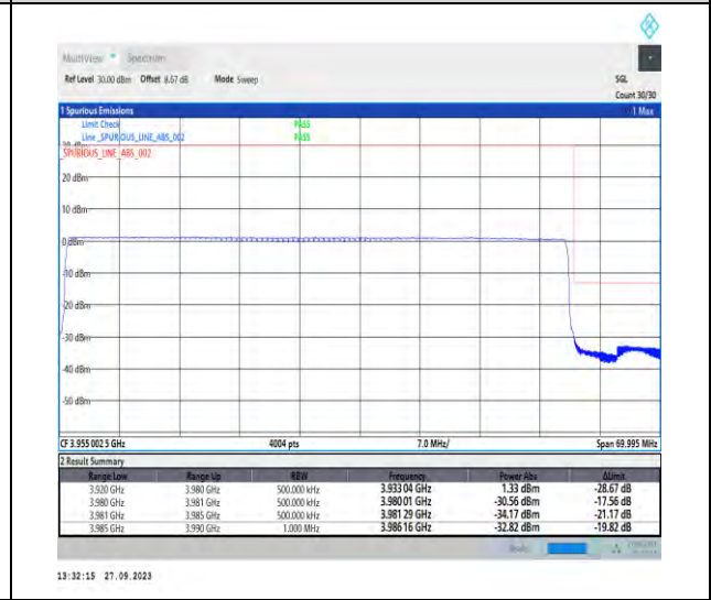
1-N77-3700-3980-PC2-30-60-H-6-CP-QPSK-Outer_Full-162@0-Ant7-1--PASS-see graph
