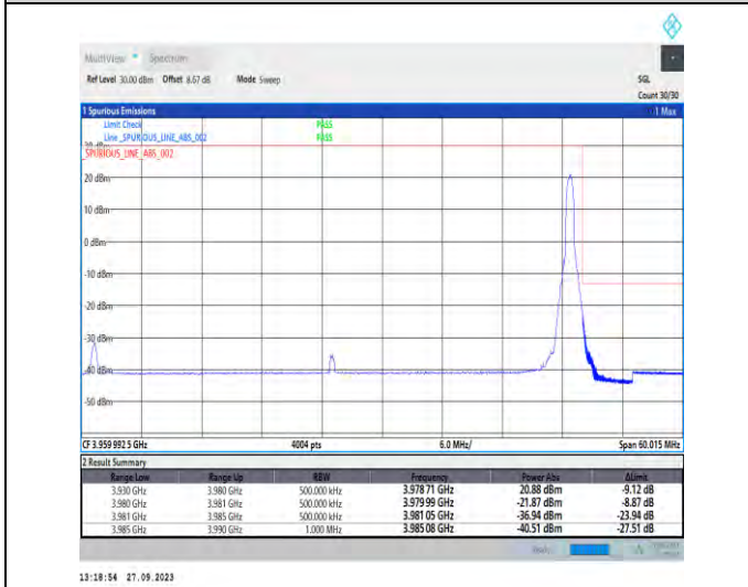
1-N77-3700-3980-PC2-30-50-H-5-CP-QPSK-Edge_1RB_Right-1@132-Ant7-1--PASS-see graph
