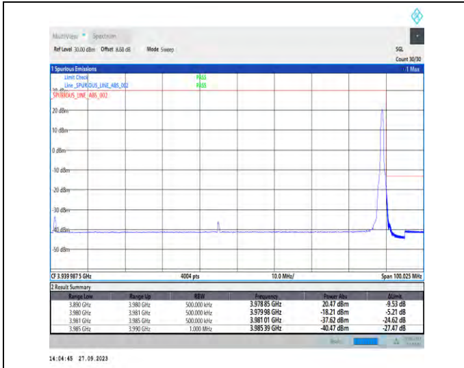
1-N77-3700-3980-PC2-30-90-H-2-DFT-PI2BPSK-Edge_1RB_Right-1@244-Ant7-1--PASS-see graph
