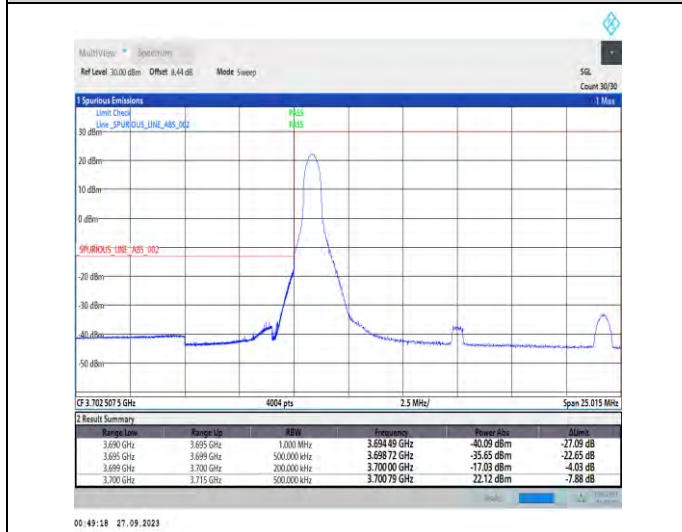
1-N77-3700-3980-PC2-30-15-L-4-CP-QPSK-Edge_1RB_Left-1@0-Ant7-1--PASS-see graph
