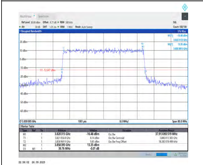
1-N77-3700-3980-PC2-30-40-M-7-CP-16QAM-Outer _Full-106@0-Ant7-37.913-39.760-≤40-PASS
