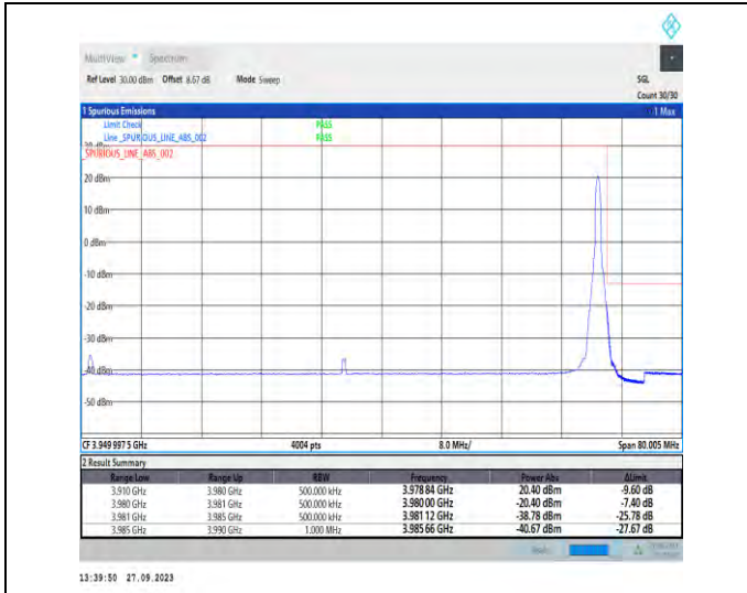
1-N77-3700-3980-PC2-30-70-H-2-DFT-PI2BPSK-Edge_1RB_Right-1@188-Ant7-1--PASS-see graph
