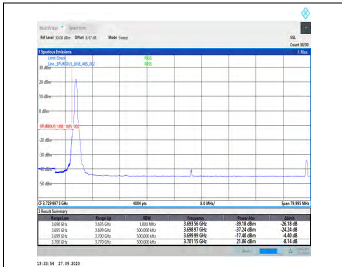
1-N77-3700-3980-PC2-30-70-L-1-DFT-PI2BPSK-Edge_1RB_Left-1@0-Ant7-1--PASS-see graph
