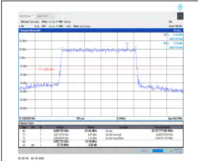
1-N77-3700-3980-PC2-30-40-M-5-DFT-256QAM-Out er_Full-100@0-Ant7-35.738-37.760-≤40-PASS
