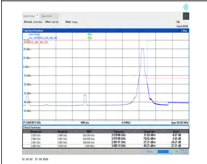
1-N77-3700-3980-PC2-30-30-H-5-CP-QPSK-Edge_1RB_Right-1@77-Ant7-1--PASS-see graph
