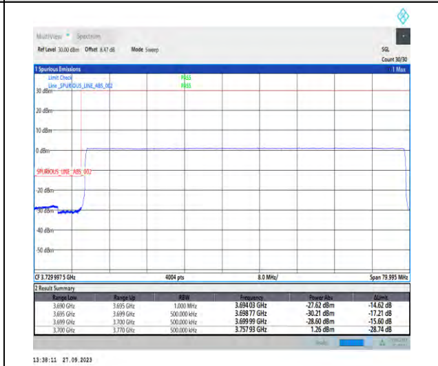
1-N77-3700-3980-PC2-30-70-L-6-CP-QPSK-Outer_Full-189@0-Ant7-1--PASS-see graph
