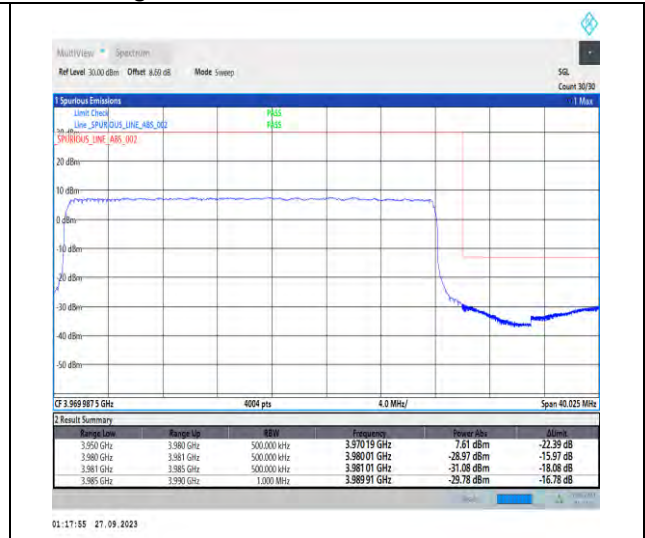
1-N77-3700-3980-PC2-30-30-H-3-DFT-PI2BPSK-Outer_Full-75@0-Ant7-1--PASS-see graph
