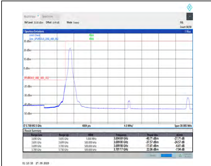
1-N77-3700-3980-PC2-30-30-L-1-DFT-PI2BPSK-Edge_1RB_Left-1@0-Ant7-1--PASS-see graph
