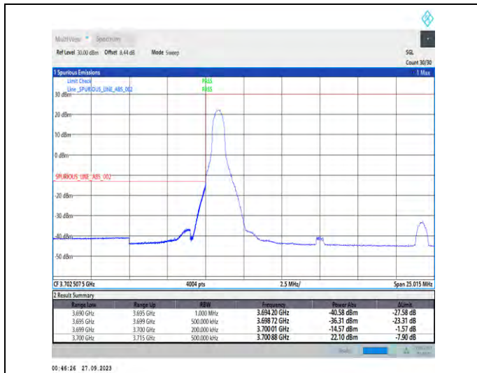
1-N77-3700-3980-PC2-30-15-L-1-DFT-PI2BPSK-Edge_1RB_Left-1@0-Ant7-1--PASS-see graph
