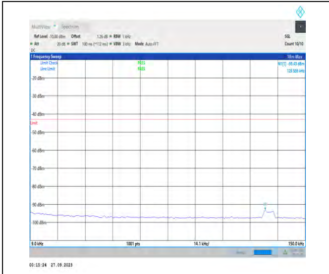
1-N77-3700-3980-PC2-30-100-H-1-DFT-PI2BPSK- Inner_1RB_Left-1@1-0.009-0.15-Ant7-0.13--93.43--4 3-PASS
