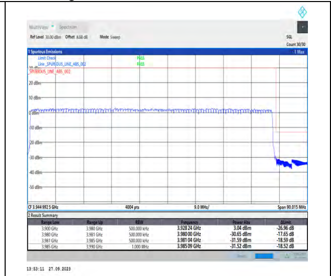
1-N77-3700-3980-PC2-30-80-H-3-DFT-PI2BPSK-Outer_Full-216@0-Ant7-1--PASS-see graph
