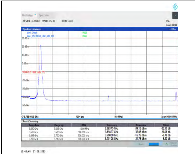
1-N77-3700-3980-PC2-30-80-L-1-DFT-PI2BPSK-Edge_1RB_Left-1@0-Ant7-1--PASS-see graph
