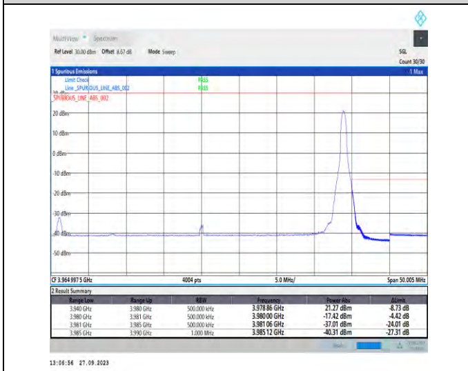
1-N77-3700-3980-PC2-30-40-H-5-CP-QPSK-Edge_1RB_Right-1@105-Ant7-1--PASS-see graph
