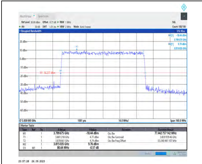
1-N77-3700-3980-PC2-30-80-M-9-CP-256QAM-Out er_Full-217@0-Ant7-77.443-80.640-≤80-PASS
