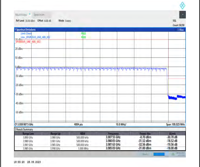
1-N77-3700-3980-PC2-30-90-H-6-CP-QPSK-Outer_Full-245@0-Ant7-1--PASS-see graph
