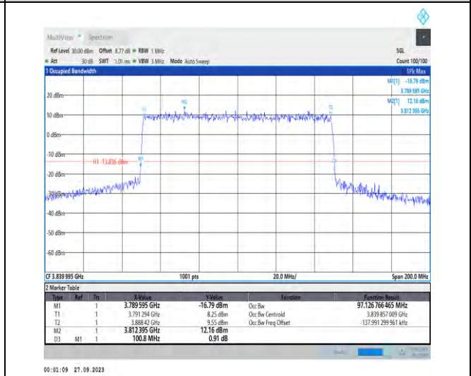
1-N77-3700-3980-PC2-30-100-M-6-CP-QPSK-Outer _Full-273@0-Ant7-97.127-100.800-≤100-PASS
