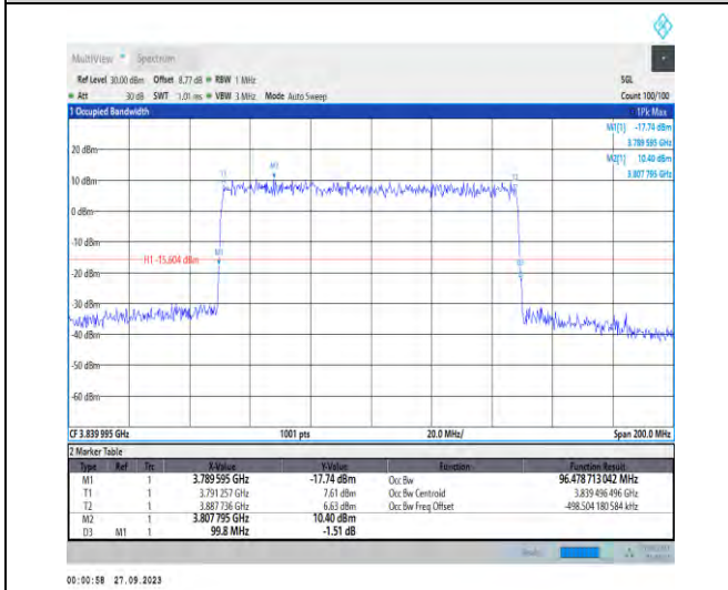
1-N77-3700-3980-PC2-30-100-M-5-DFT-256QAM-Out uter_Full-270@0-Ant7-96.479-99.800-≤100-PASS
