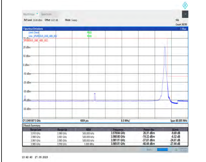
1-N77-3700-3980-PC2-30-70-H-5-CP-QPSK-Edge_1RB_Right-1@188-Ant7-1--PASS-see graph
