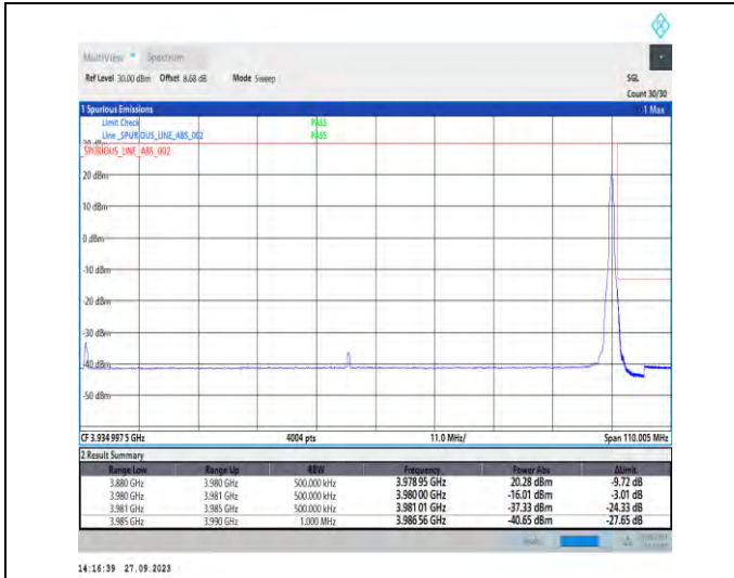
1-N77-3700-3980-PC2-30-100-H-2-DFT-PI2BPSK-Edge_1RB_Right-1@272-Ant7-1--PASS-see graph
