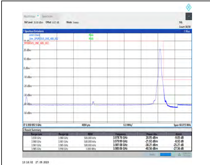
1-N77-3700-3980-PC2-30-50-H-2-DFT-PI2BPSK-Edge_1RB_Right-1@132-Ant7-1--PASS-see graph
