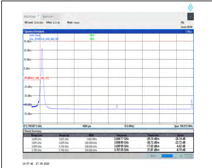
1-N77-3700-3980-PC2-30-90-L-1-DFT-PI2BPSK-Edge_1RB_Left-1@0-Ant7-1--PASS-see graph
