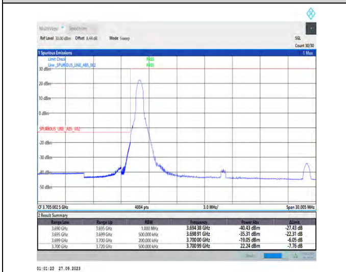
1-N77-3700-3980-PC2-30-20-L-4-CP-QPSK-Edge_1RB_Left-1@0-Ant7-1--PASS-see graph
