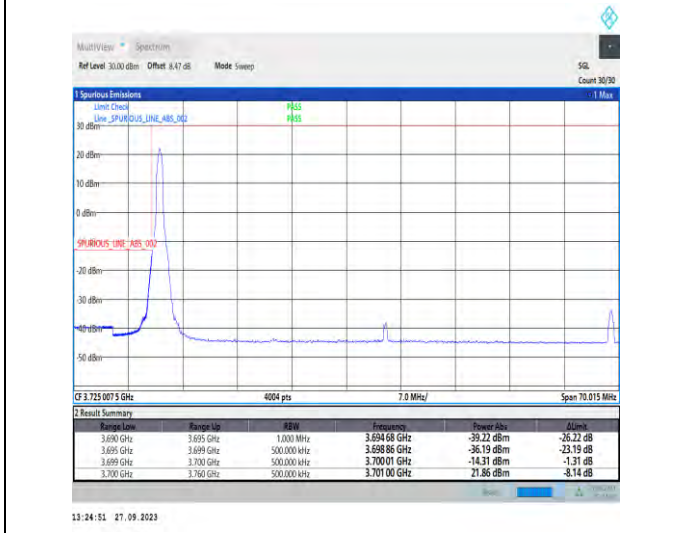
1-N77-3700-3980-PC2-30-60-L-4-CP-QPSK-Edge_1RB_Left-1@0-Ant7-1--PASS-see graph
