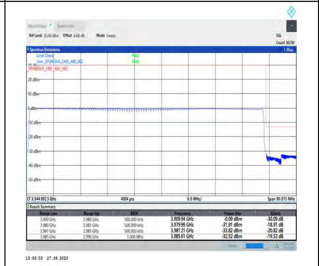
1-N77-3700-3980-PC2-30-80-H-6-CP-QPSK-Outer_Full-217@0-Ant7-1--PASS-see graph
