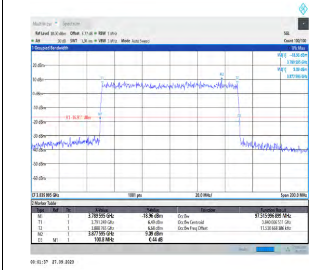
1-N77-3700-3980-PC2-30-100-M-9-CP-256QAM-Outer er_Full-273@0-Ant7-97.516-100.800-≤100-PASS
