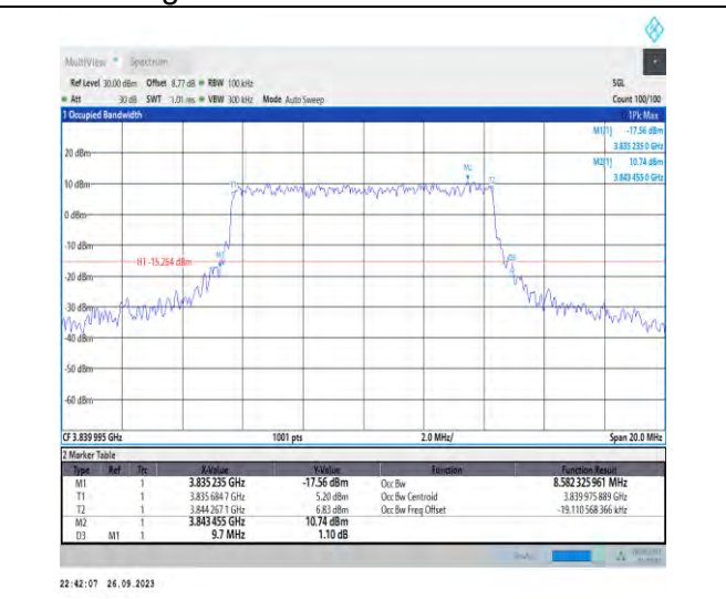
1-N77-3700-3980-PC2-30-10-M-6-CP-QPSK-Outer Full-24@0-Ant7-8.582-9.700-≤10-PASS
