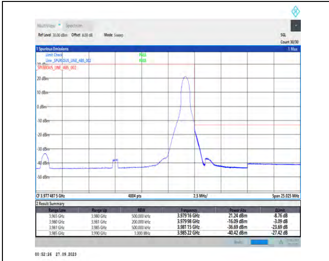
1-N77-3700-3980-PC2-30-15-H-2-DFT-PI2BPSK-Edge_1RB_Right-1@37-Ant7-1--PASS-see graph
