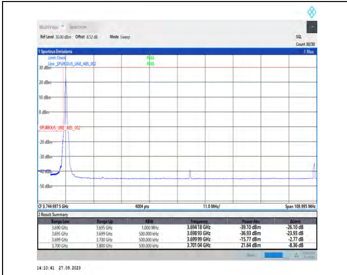
1-N77-3700-3980-PC2-30-100-L-1-DFT-PI2BPSK-Edge_e_1RB_Left-1@0-Ant7-1--PASS-see graph
