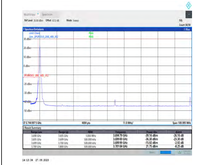
1-N77-3700-3980-PC2-30-100-L-4-CP-QPSK-Edge_1RB_Left-1@0-Ant7-1--PASS-see graph
