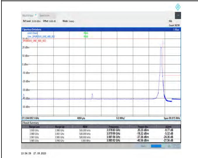
1-N77-3700-3980-PC2-30-80-H-5-CP-QPSK-Edge_1RB_Right-1@216-Ant7-1--PASS-see graph
