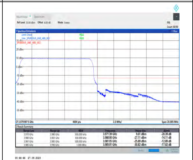
1-N77-3700-3980-PC2-30-10-H-6-CP-QPSK-Outer_Full-24@0-Ant7-1--PASS-see graph
