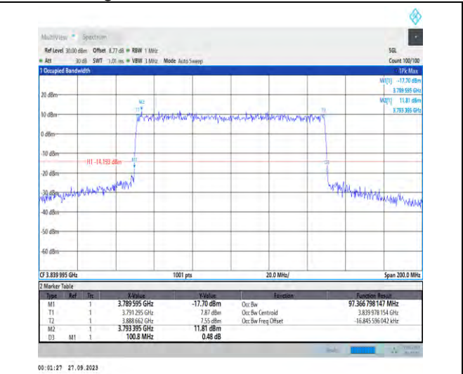
1-N77-3700-3980-PC2-30-100-M-8-CP-64QAM-Outer r_Full-273@0-Ant7-97.367-100.800-≤100-PASS
