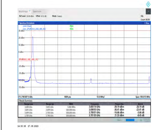
1-N77-3700-3980-PC2-30-90-L-4-CP-QPSK-Edge_1RB_Left-1@0-Ant7-1--PASS-see graph
