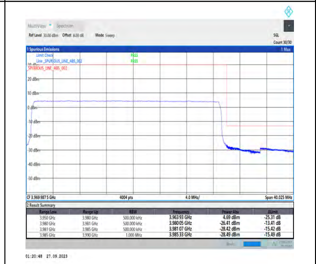
1-N77-3700-3980-PC2-30-30-H-6-CP-QPSK-Outer_Full-78@0-Ant7-1--PASS-see graph
