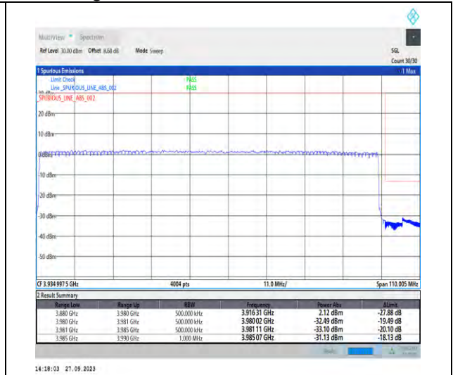
1-N77-3700-3980-PC2-30-100-H-3-DFT-PI2BPSK-Outer_Full-270@0-Ant7-1--PASS-see graph
