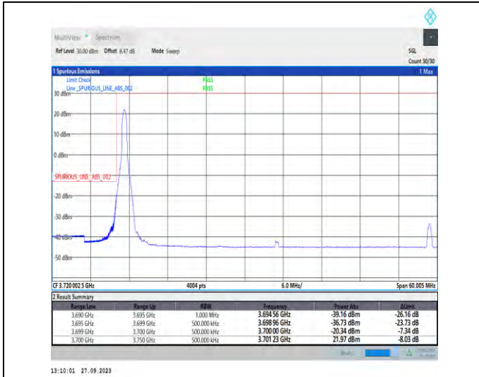
1-N77-3700-3980-PC2-30-50-L-1-DFT-PI2BPSK-Edge_1RB_Left-1@0-Ant7-1--PASS-see graph
