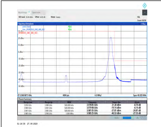
1-N77-3700-3980-PC2-30-30-H-2-DFT-PI2BPSK-Edge_1RB_Right-1@77-Ant7-1--PASS-see graph
