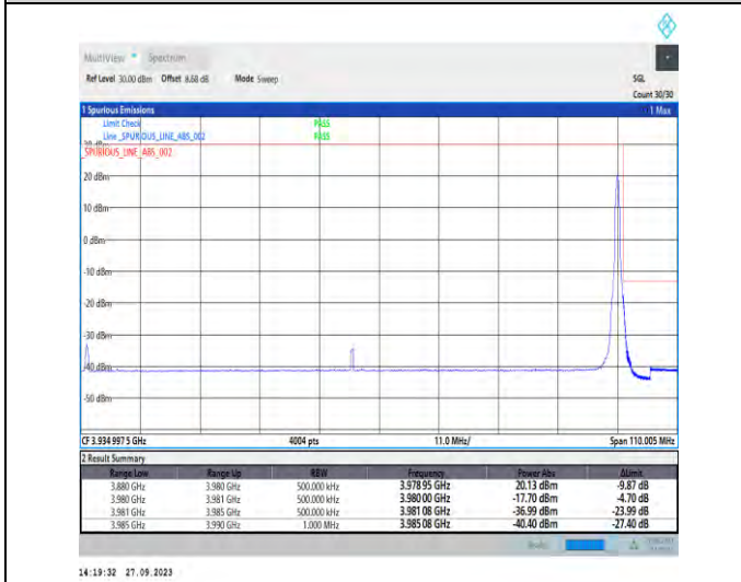
1-N77-3700-3980-PC2-30-100-H-5-CP-QPSK-Edge_1RB_Right-1@272-Ant7-1--PASS-see graph
