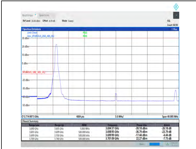
1-N77-3700-3980-PC2-30-40-L-1-DFT-PI2BPSK-Edge_1RB_Left-1@0-Ant7-1--PASS-see graph
