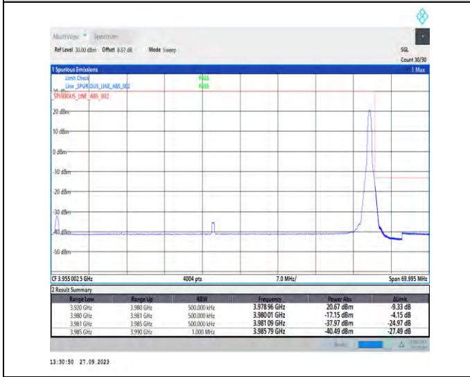
1-N77-3700-3980-PC2-30-60-H-5-CP-QPSK-Edge_1RB_Right-1@161-Ant7-1--PASS-see graph
