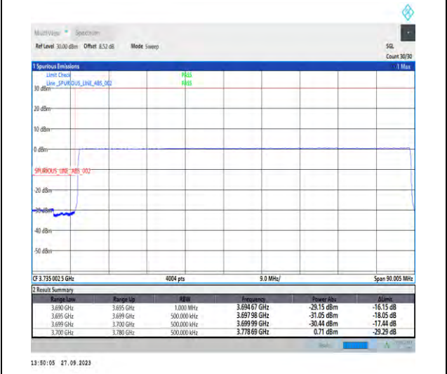
1-N77-3700-3980-PC2-30-80-L-6-CP-QPSK-Outer_Full-217@0-Ant7-1--PASS-see graph
