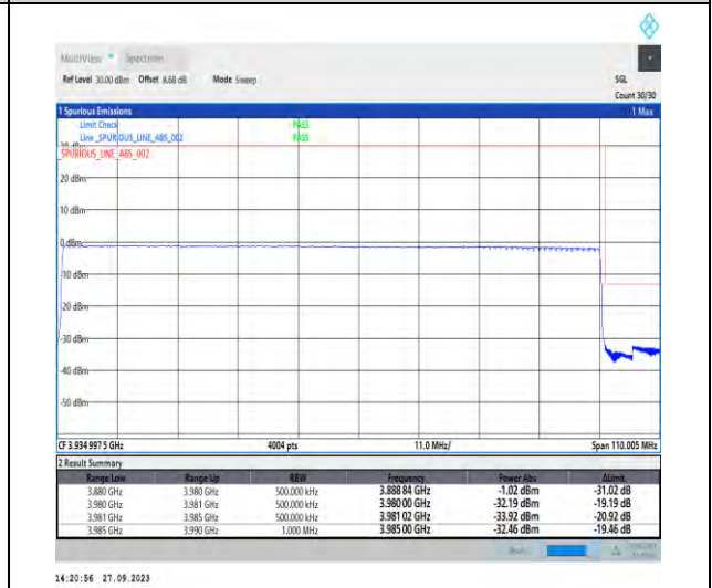
1-N77-3700-3980-PC2-30-100-H-6-CP-QPSK-Outer_Full-273@0-Ant7-1--PASS-see graph
