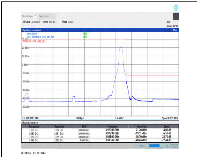
1-N77-3700-3980-PC2-30-20-H-2-DFT-PI2BPSK-Edge_1RB_Right-1@50-Ant7-1--PASS-see graph
