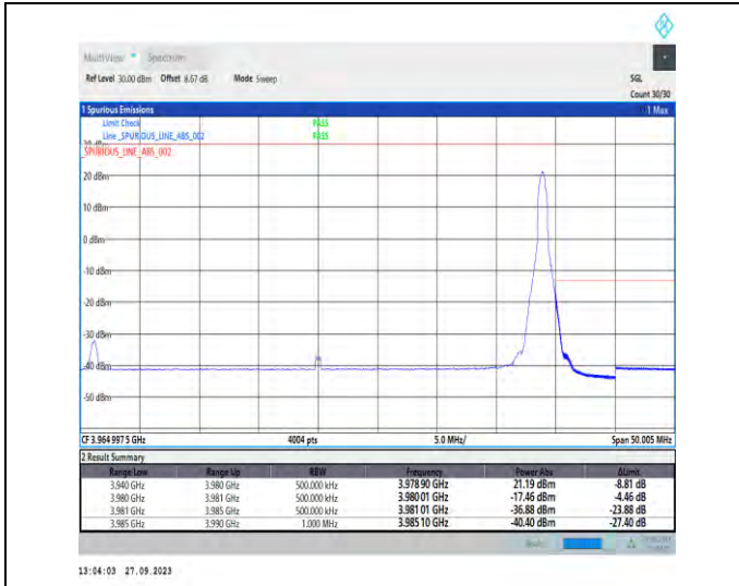
1-N77-3700-3980-PC2-30-40-H-2-DFT-PI2BPSK-Edge_1RB_Right-1@105-Ant7-1--PASS-see graph
