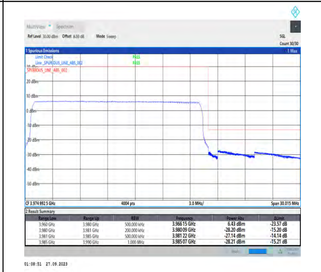
1-N77-3700-3980-PC2-30-20-H-6-CP-QPSK-Outer_Full-51@0-Ant7-1--PASS-see graph
