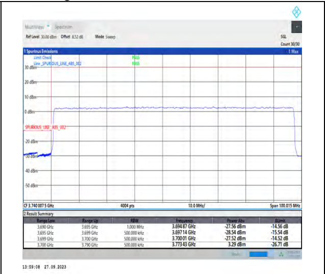
1-N77-3700-3980-PC2-30-90-L-3-DFT-PI2BPSK-Outer_Full-240@0-Ant7-1--PASS-see graph
