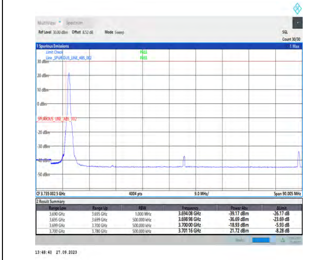
1-N77-3700-3980-PC2-30-80-L-4-CP-QPSK-Edge_1RB_Left-1@0-Ant7-1--PASS-see graph
