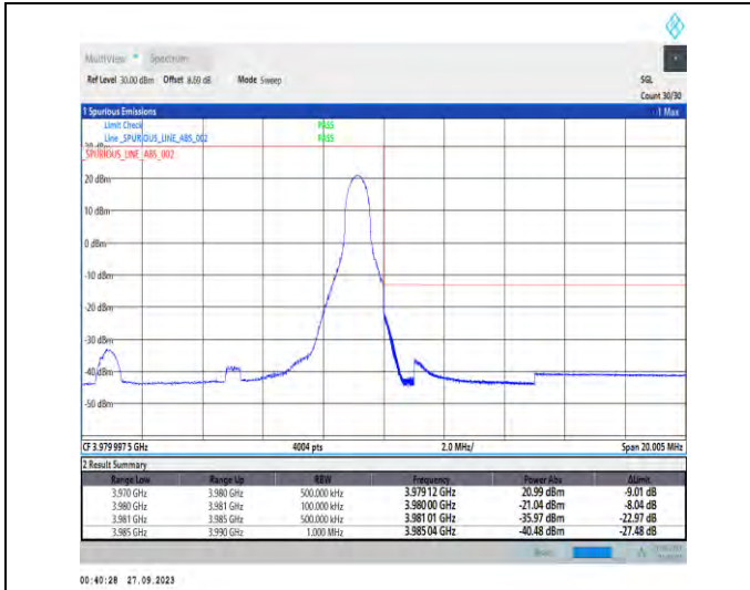
1-N77-3700-3980-PC2-30-10-H-2-DFT-PI2BPSK-Edge_1RB_Right-1@23-Ant7-1--PASS-see graph
