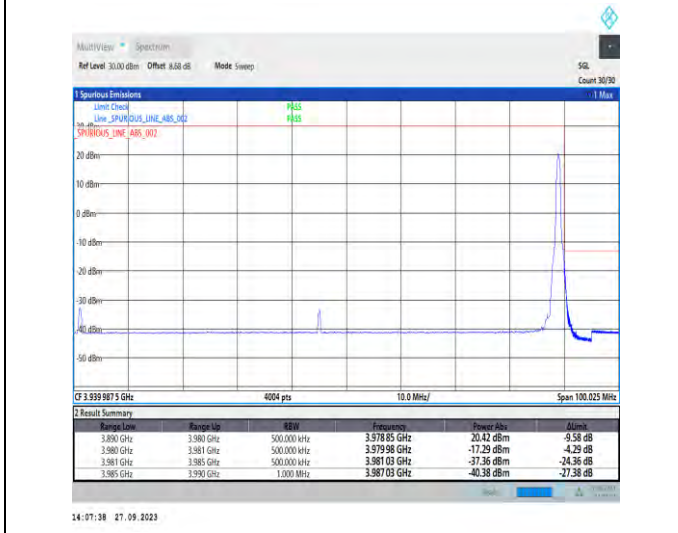
1-N77-3700-3980-PC2-30-90-H-5-CP-QPSK-Edge_1RB_Right-1@244-Ant7-1--PASS-see graph
