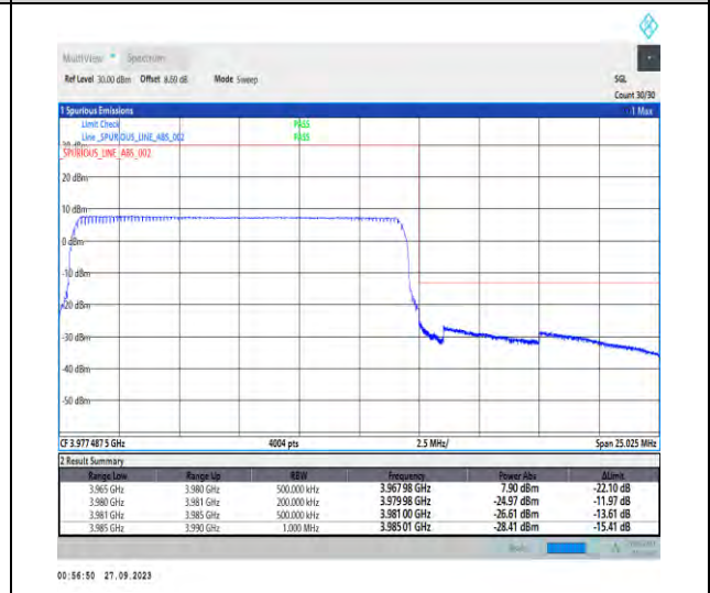
1-N77-3700-3980-PC2-30-15-H-6-CP-QPSK-Outer_Full-38@0-Ant7-1--PASS-see graph
