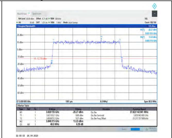
1-N77-3700-3980-PC2-30-40-M-6-CP-QPSK-Outer_ Full-106@0-Ant7-37.823-40.000-≤40-PASS
