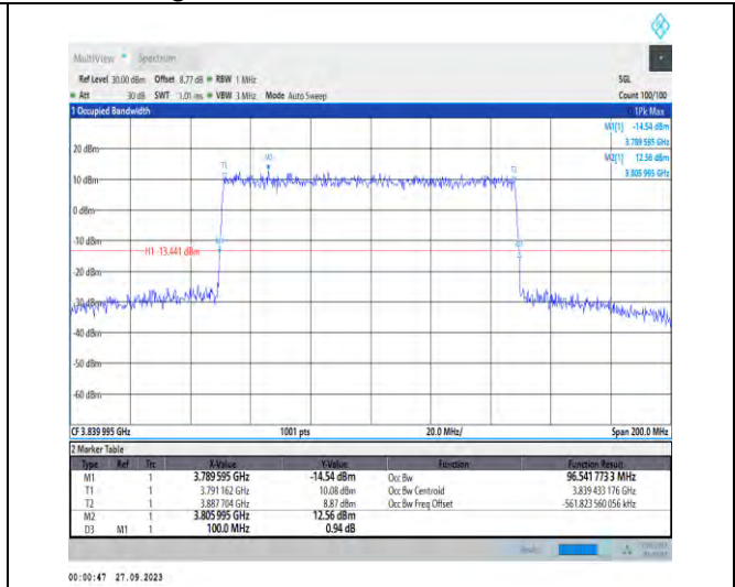
1-N77-3700-3980-PC2-30-100-M-4-DFT-64QAM-Out er_Full-270@0-Ant7-96.542-100.000-≤100-PASS
