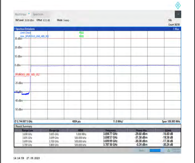
1-N77-3700-3980-PC2-30-100-L-6-CP-QPSK-Outer_Full-273@0-Ant7-1--PASS-see graph
