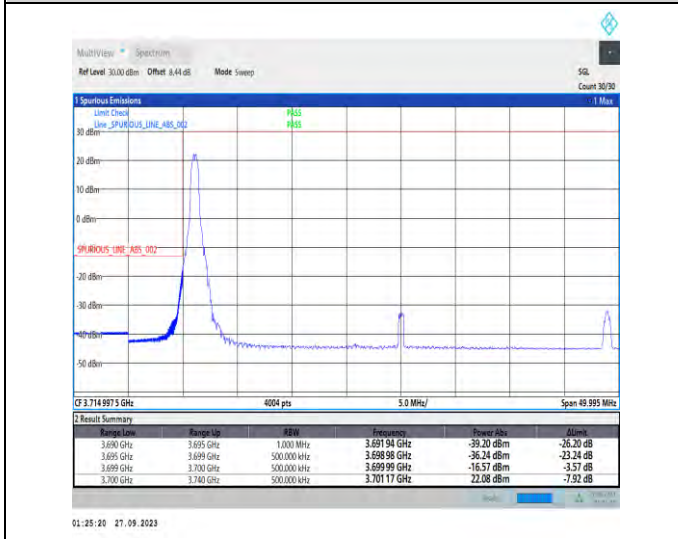
1-N77-3700-3980-PC2-30-40-L-4-CP-QPSK-Edge_1RB_Left-1@0-Ant7-1--PASS-see graph
