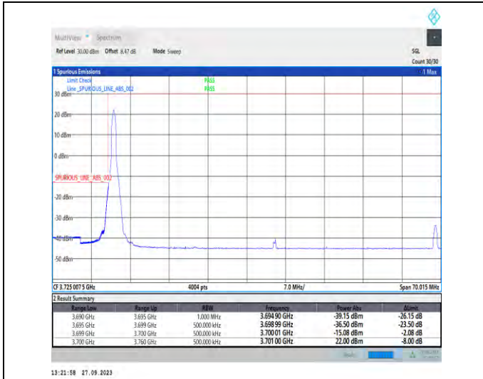
1-N77-3700-3980-PC2-30-60-L-1-DFT-PI2BPSK-Edge_1RB_Left-1@0-Ant7-1--PASS-see graph
