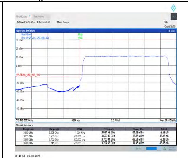
1-N77-3700-3980-PC2-30-15-L-3-DFT-PI2BPSK-Outer_Full-36@0-Ant7-1--PASS-see graph
