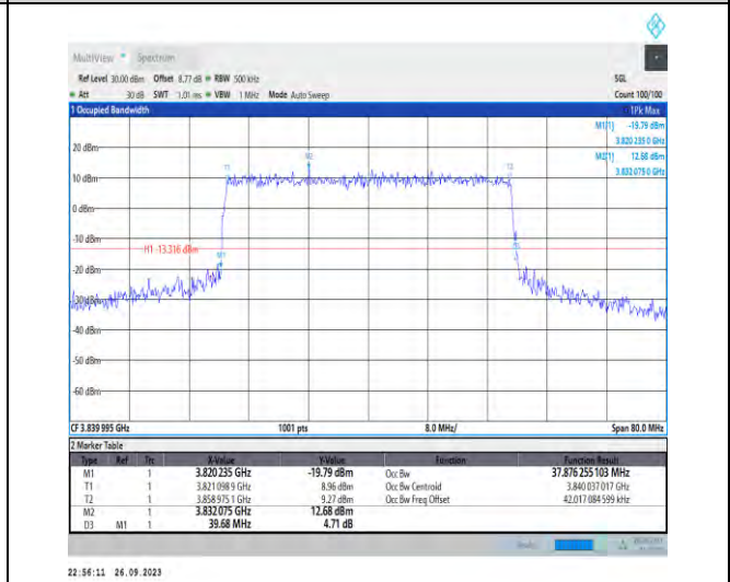
1-N77-3700-3980-PC2-30-40-M-8-CP-64QAM-Outer _Full-106@0-Ant7-37.876-39.680-≤40-PASS
