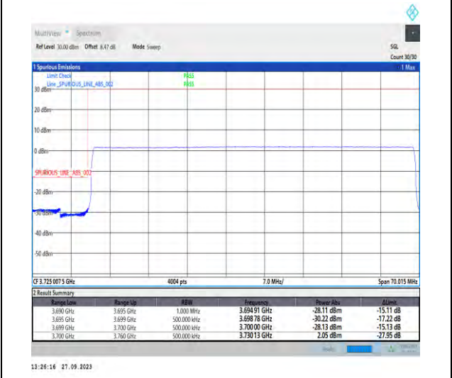
1-N77-3700-3980-PC2-30-60-L-6-CP-QPSK-Outer_Full-162@0-Ant7-1--PASS-see graph
