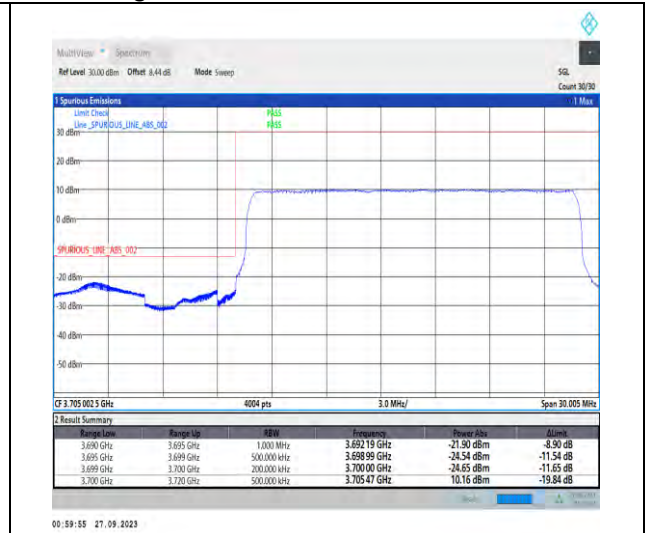
1-N77-3700-3980-PC2-30-20-L-3-DFT-PI2BPSK-Outer_Full-50@0-Ant7-1--PASS-see graph
