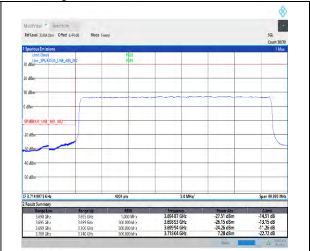
1-N77-3700-3980-PC2-30-40-L-3-DFT-PI2BPSK-Outer_Full-100@0-Ant7-1--PASS-see graph
