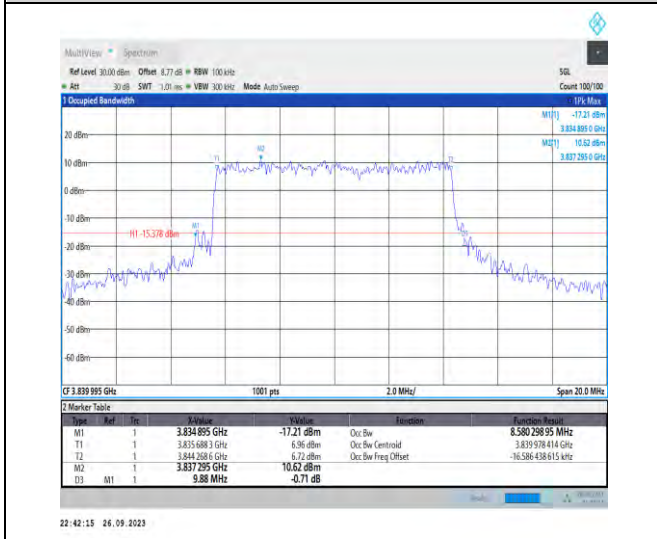
1-N77-3700-3980-PC2-30-10-M-7-CP-16QAM-Outer _Full-24@0-Ant7-8.58-9.880-≤10-PASS
