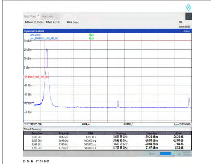
1-N77-3700-3980-PC2-30-70-L-4-CP-QPSK-Edge_1RB_Left-1@0-Ant7-1--PASS-see graph
