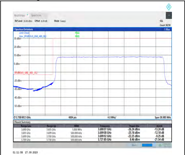
1-N77-3700-3980-PC2-30-30-L-3-DFT-PI2BPSK-Outer_Full-75@0-Ant7-1--PASS-see graph
