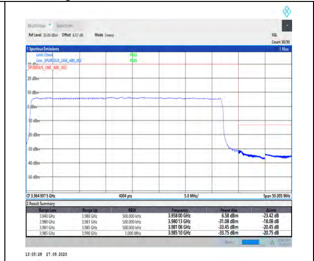
1-N77-3700-3980-PC2-30-40-H-3-DFT-PI2BPSK-Outer_Full-100@0-Ant7-1--PASS-see graph
