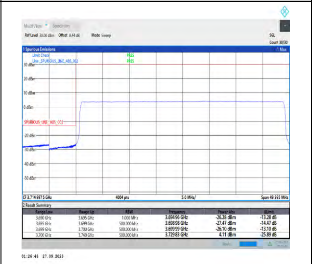
1-N77-3700-3980-PC2-30-40-L-6-CP-QPSK-Outer_Full-106@0-Ant7-1--PASS-see graph
