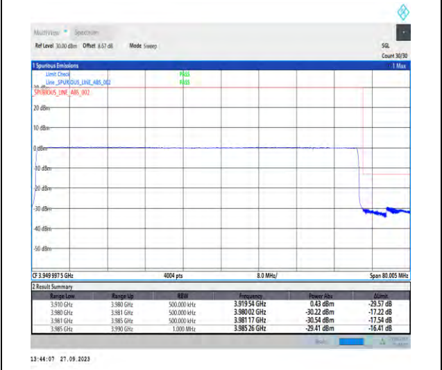
1-N77-3700-3980-PC2-30-70-H-6-CP-QPSK-Outer_Full-189@0-Ant7-1--PASS-see graph
