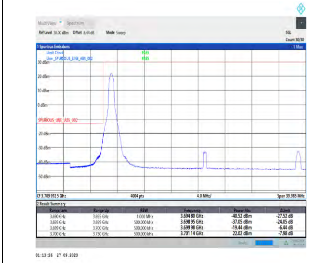
1-N77-3700-3980-PC2-30-30-L-4-CP-QPSK-Edge_1RB_Left-1@0-Ant7-1--PASS-see graph
