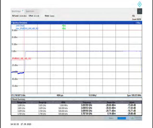
1-N77-3700-3980-PC2-30-90-L-6-CP-QPSK-Outer_Full-245@0-Ant7-1--PASS-see graph
