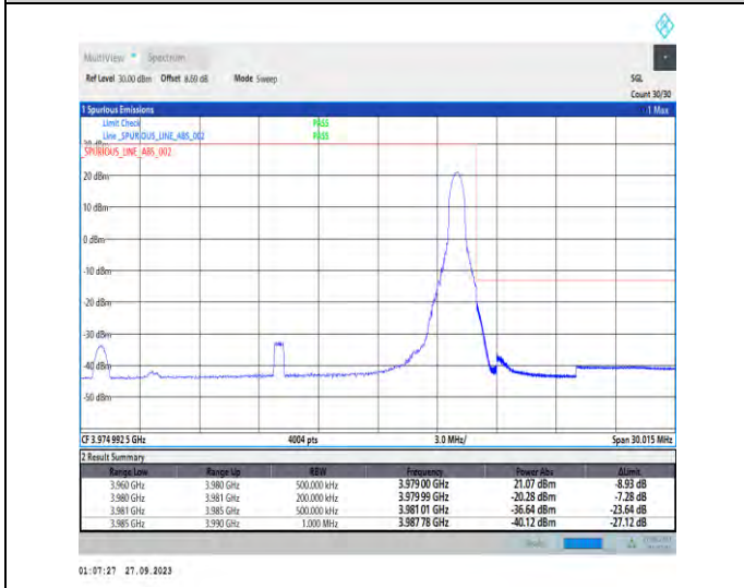
1-N77-3700-3980-PC2-30-20-H-5-CP-QPSK-Edge_1RB_Right-1@50-Ant7-1--PASS-see graph
