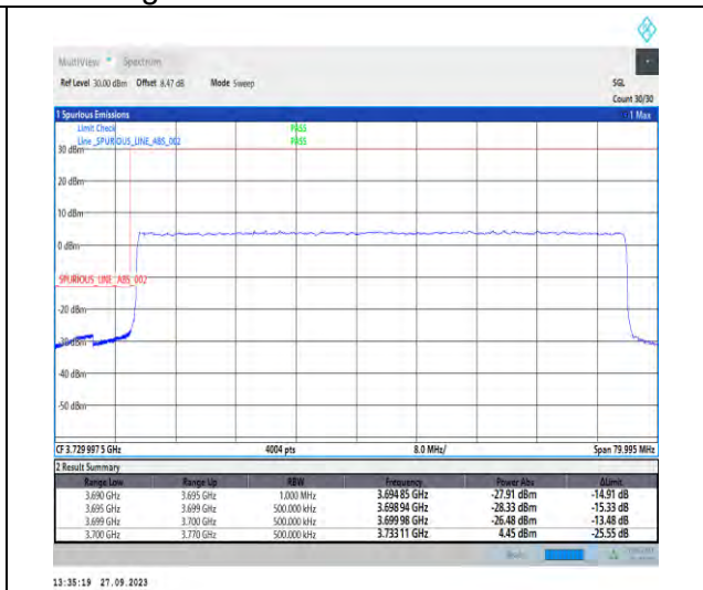
1-N77-3700-3980-PC2-30-70-L-3-DFT-PI2BPSK-Outer_Full-180@0-Ant7-1--PASS-see graph
