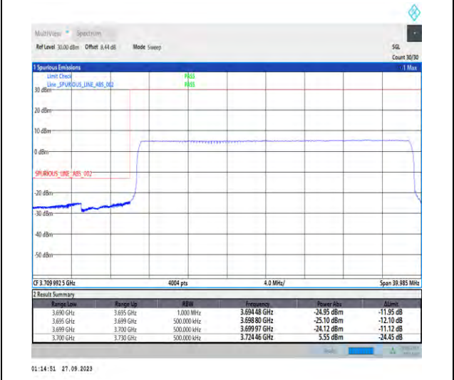
1-N77-3700-3980-PC2-30-30-L-6-CP-QPSK-Outer_Full-78@0-Ant7-1--PASS-see graph
