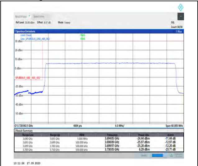
1-N77-3700-3980-PC2-30-50-L-3-DFT-PI2BPSK-Outer_Full-128@0-Ant7-1--PASS-see graph
