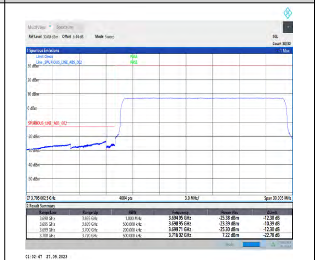
1-N77-3700-3980-PC2-30-20-L-6-CP-QPSK-Outer_Full-51@0-Ant7-1--PASS-see graph
