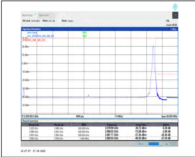
1-N77-3700-3980-PC2-30-60-H-2-DFT-PI2BPSK-Edge_1RB_Right-1@161-Ant7-1--PASS-see graph
