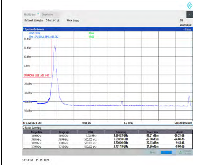
1-N77-3700-3980-PC2-30-50-L-4-CP-QPSK-Edge_1RB_Left-1@0-Ant7-1--PASS-see graph
