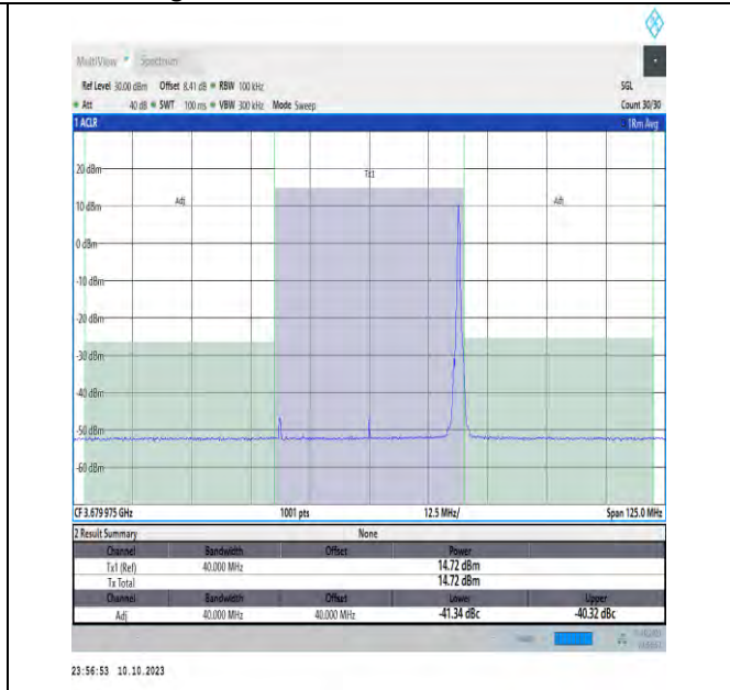
NTVN_N48_PC3_30_40_H_TID3_#1_-40_40
