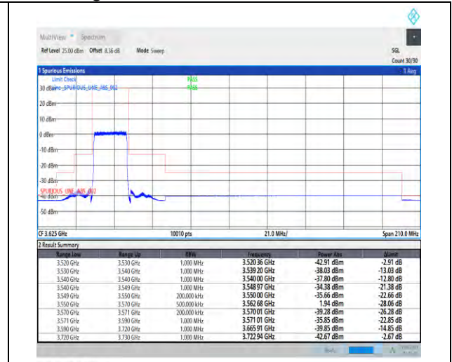
1-N48-PC3-30-20-L-3-DFT-PI2BPSK-Outer_Full-50@0-Ant7-1--PASS-see graph
