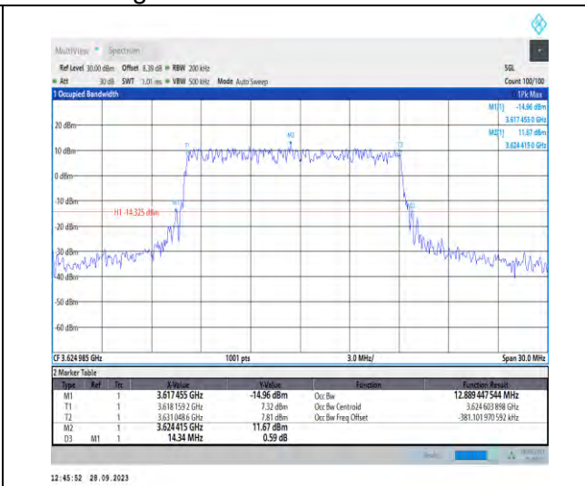
1-N48-PC3-30-15-M-1-DFT-QPSK-Outer_Full-36@ 0-Ant7-12.889-14.340-≤15-PASS
