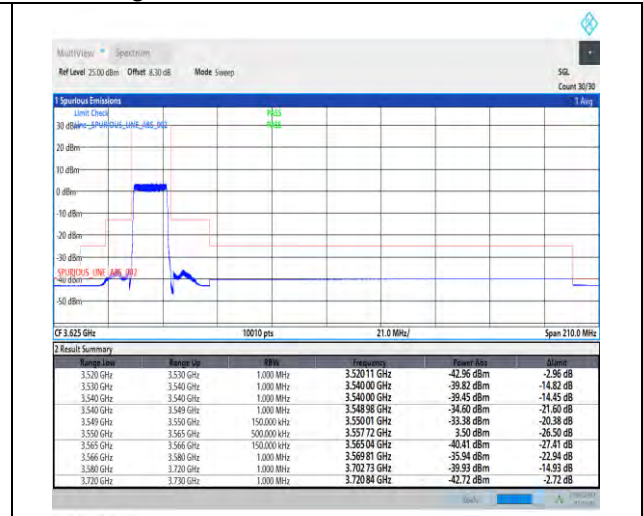
1-N48-PC3-30-15-L-3-DFT-PI2BPSK-Outer_Full-36@0-Ant7-1--PASS-see graph
