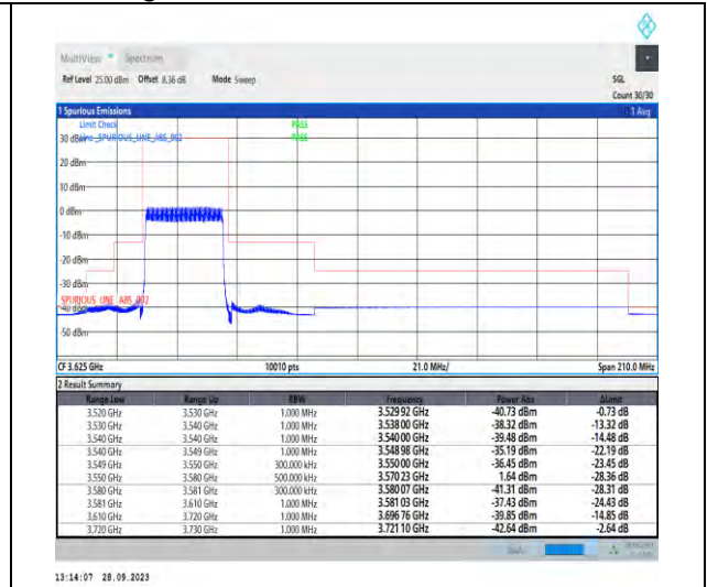
1-N48-PC3-30-30-L-3-DFT-PI2BPSK-Outer_Full-75@0-Ant7-1--PASS-see graph
