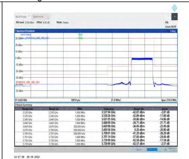
1-N48-PC3-30-30-H-3-DFT-PI2BPSK-Outer_Full-75@0-Ant7-1--PASS-see graph
