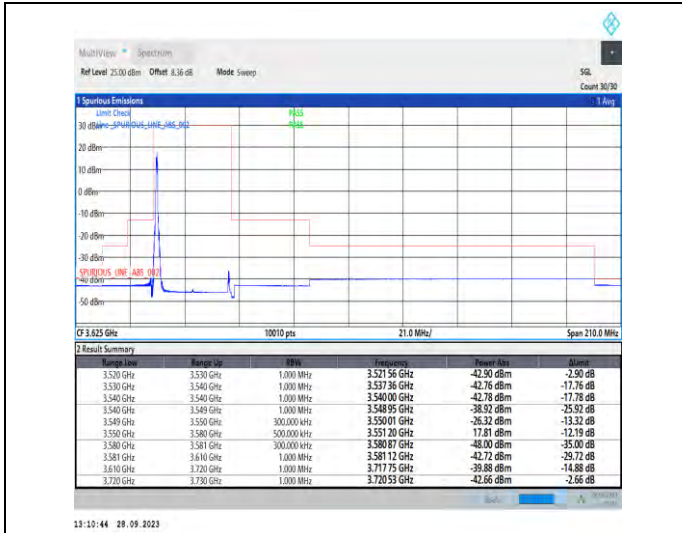
1-N48-PC3-30-30-L-1-DFT-PI2BPSK-Edge_1RB_Left-1@0-Ant7-1--PASS-see graph
