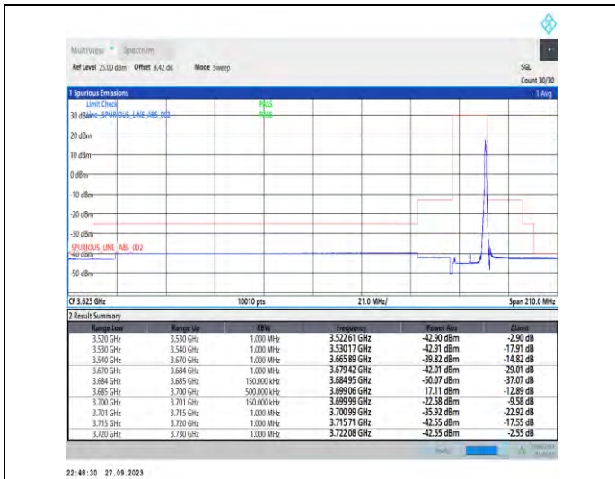
1-N48-PC3-30-15-H-2-DFT-PI2BPSK-Edge_1RB_Right-1@37-Ant7-1--PASS-see graph
