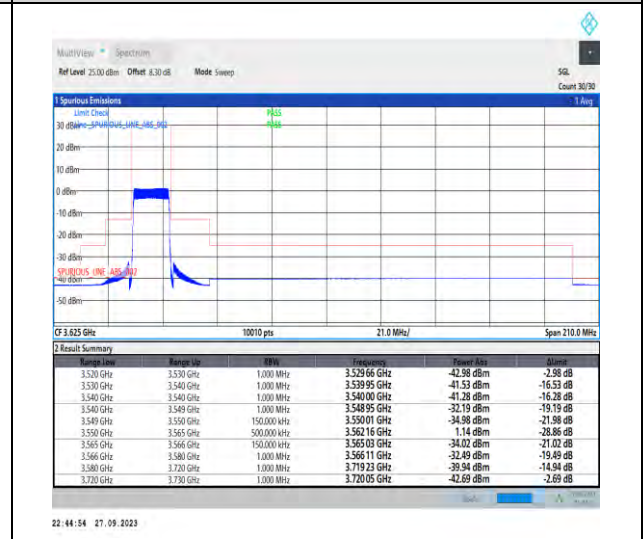
1-N48-PC3-30-15-L-6-CP-QPSK-Outer_Full-38@0-Ant7-1--PASS-see graph
