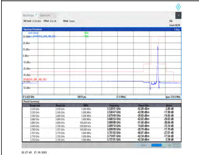
1-N48-PC3-30-10-H-5-CP-QPSK-Edge_1RB_Right-1@23-Ant7-1--PASS-see graph
