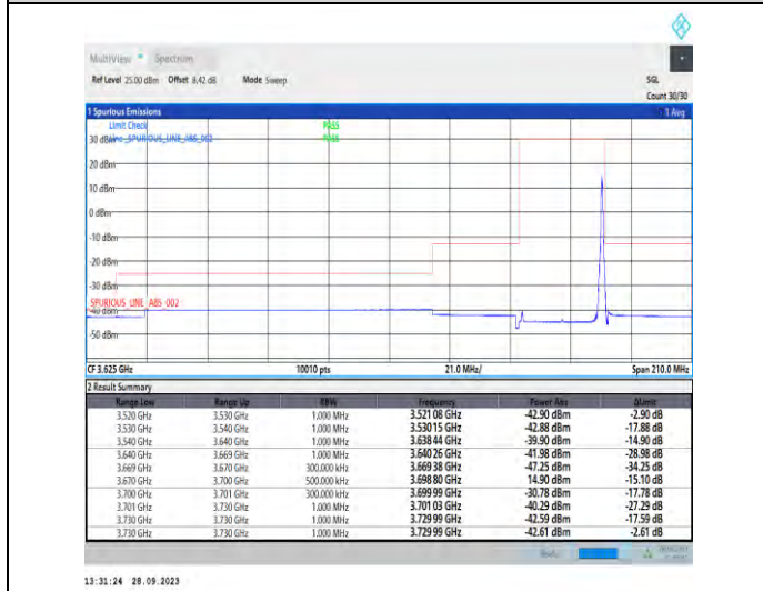
1-N48-PC3-30-30-H-5-CP-QPSK-Edge_1RB_Right-1@77-Ant7-1--PASS-see graph
