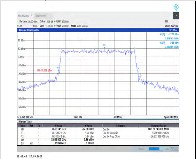
1-N48-PC3-30-20-M-8-CP-64QAM-Outer_Full-51@0 -Ant7-18.172-19.680-<20-PASS
