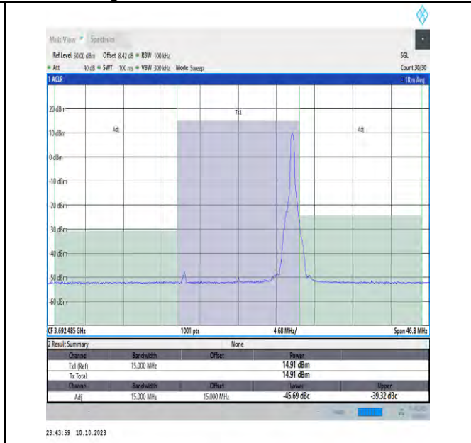
NTVN_N48_PC3_30_15_H_TID3_#1_-15_15
