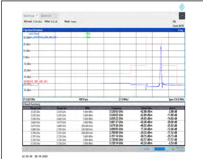
1-N48-PC3-30-20-H-2-DFT-PI2BPSK-Edge_1RB_Righ t-1@50-Ant7-1--PASS-see graph
