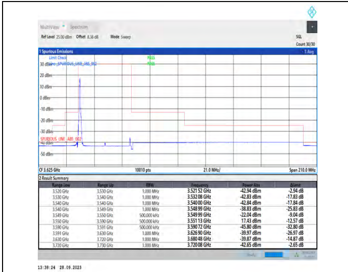
1-N48-PC3-30-40-L-1-DFT-PI2BPSK-Edge_1RB_Left-1@0-Ant7-1--PASS-see graph
