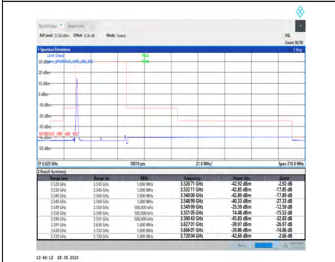
1-N48-PC3-30-40-L-4-CP-QPSK-Edge_1RB_Left-1@0-Ant7-1--PASS-see graph
