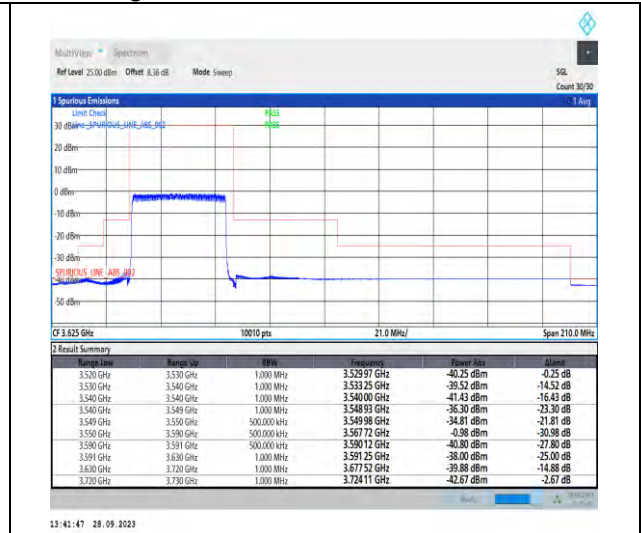
1-N48-PC3-30-40-L-3-DFT-PI2BPSK-Outer_Full-100@0-Ant7-1--PASS-see graph
