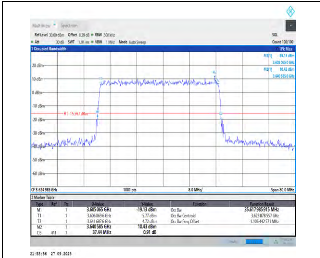
1-N48-PC3-30-40-M-5-DFT-256QAM-Outer_Full-100 @0-Ant7-35.618-37.440-≤40-PASS
