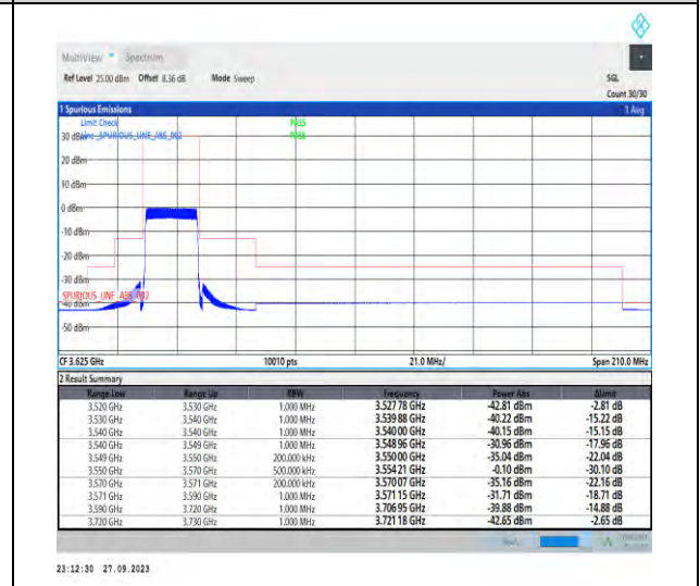
1-N48-PC3-30-20-L-6-CP-QPSK-Outer_Full-51@0-Ant7-1--PASS-see graph
