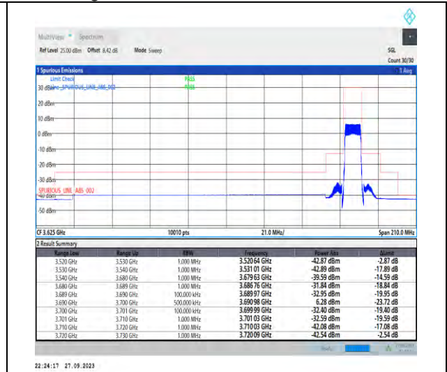
1-N48-PC3-30-10-H-3-DFT-PI2BPSK-Outer_Full-24@0-Ant7-1--PASS-see graph
