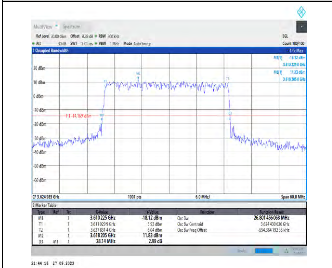
1-N48-PC3-30-30-M-4-DFT-64QAM-Outer_Full-75 @0-Ant7-26.801-28.140-≤30-PASS
