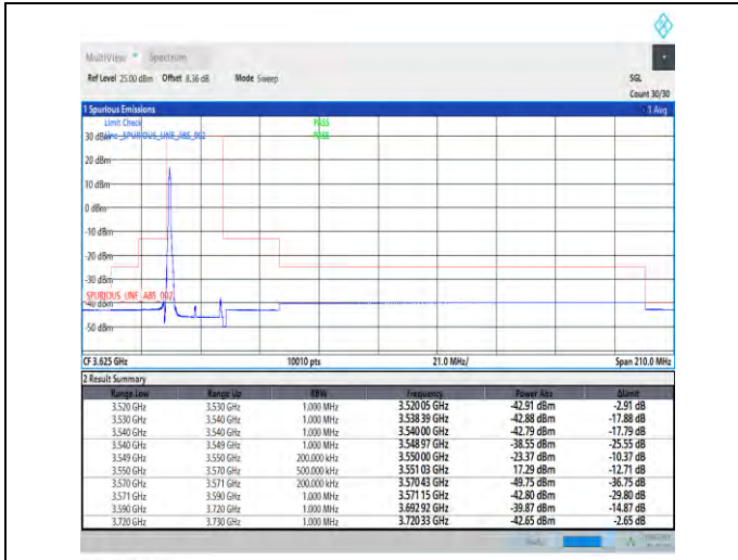
1-N48-PC3-30-20-L-1-DFT-PI2BPSK-Edge_1RB_Left-1@0-Ant7-1--PASS-see graph
