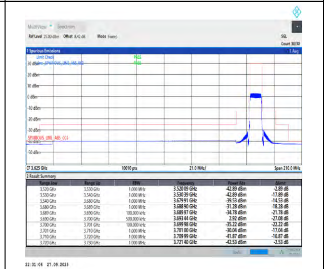
1-N48-PC3-30-10-H-6-CP-QPSK-Outer_Full-24@0-Ant7-1--PASS-see graph
