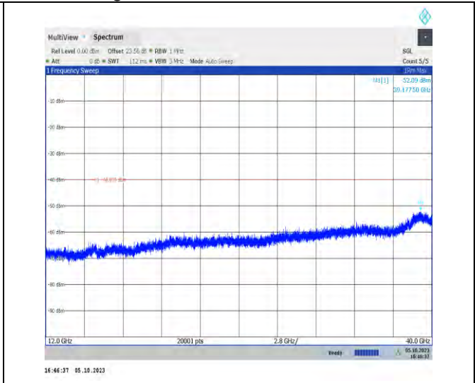
1-N48-PC3-30-40-H-1-DFT-PI2BPSK-Inner_1RB_Lef t-1@1-12000-20000-Ant7-17080.40--44.14--40-PASS
