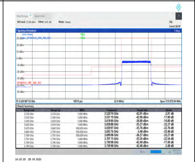
1-N48-PC3-30-40-H-6-CP-QPSK-Outer_Full-106 @0-Ant7-1--PASS-see graph
