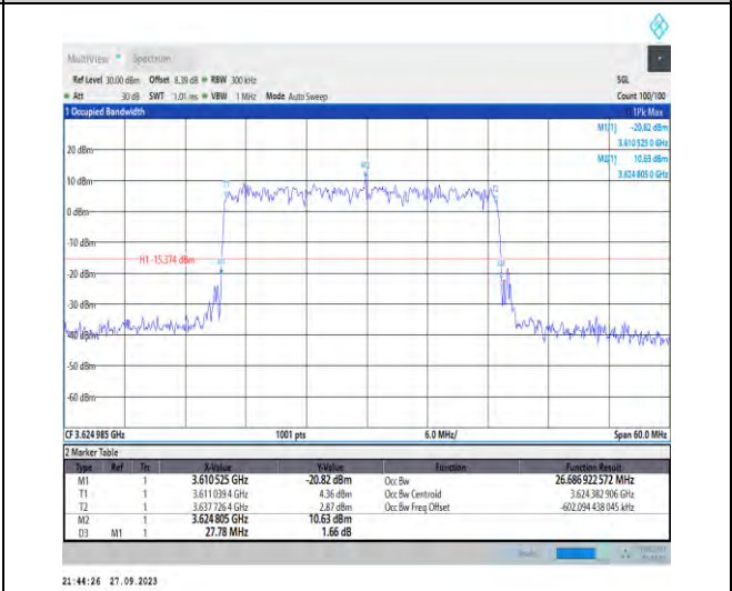
1-N48-PC3-30-30-M-5-DFT-256QAM-Outer_Full-75 @0-Ant7-26.687-27.780-≤30-PASS
