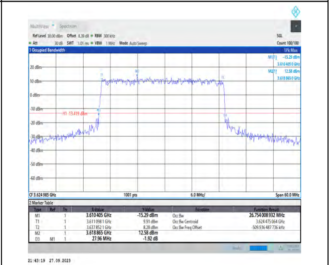
1-N48-PC3-30-30-M-1-DFT-QPSK-Outer_Full-75@0 -Ant7-26.754-27.960-<30-PASS
