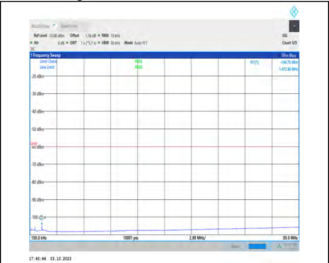
1-N48-PC3-30-40-H-1-DFT-PI2BPSK-Inner_1RB_Lef t-1@1-0.15-30-Ant7-0.15--87.60--60-PASS
