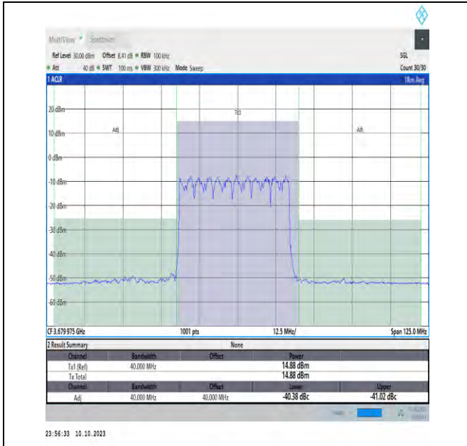
NTVN_N48_PC3_30_40_H_TID1_#1_-40_40
