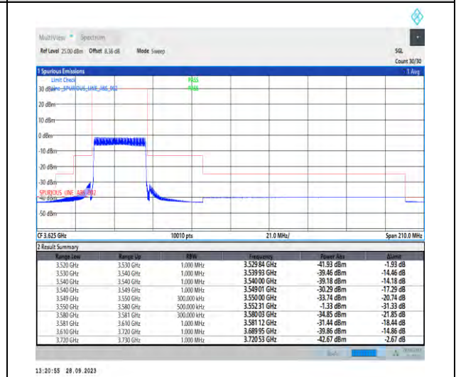
1-N48-PC3-30-30-L-6-CP-QPSK-Outer_Full-78@0-Ant7-1--PASS-see graph
