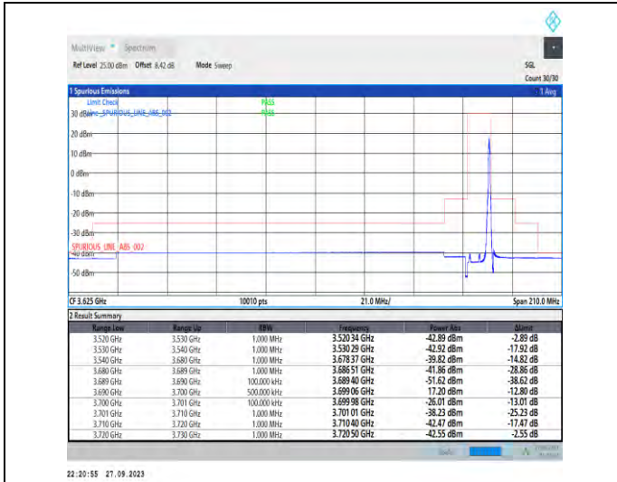
1-N48-PC3-30-10-H-2-DFT-PI2BPSK-Edge_1RB_Right-t-1@23-Ant7-1--PASS-see graph
