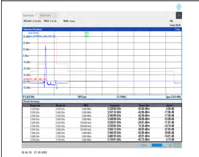
1-N48-PC3-30-15-L-4-CP-QPSK-Edge_1RB_Left-1@0-Ant7-1--PASS-see graph
