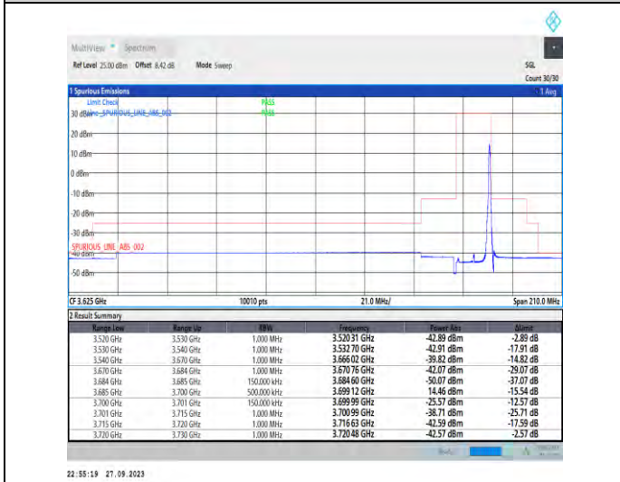
1-N48-PC3-30-15-H-5-CP-QPSK-Edge_1RB_Right-1@37-Ant7-1--PASS-see graph
