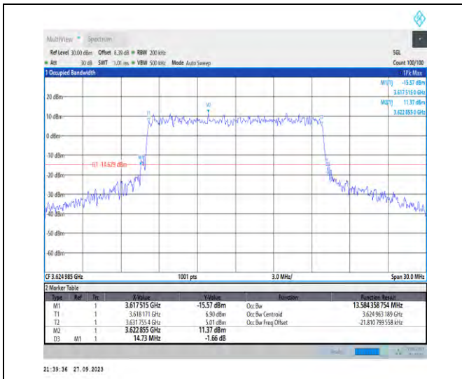
1-N48-PC3-30-15-M-8-CP-64QAM-Outer_Full-38@0 -Ant7-13.584-14.730-≤15-PASS
