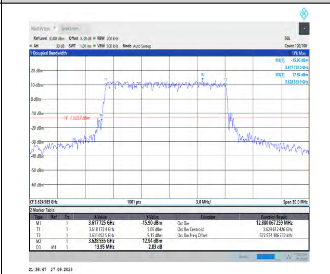
1-N48-PC3-30-15-M-3-DFT-16QAM-Outer_Full-36@ 0-Ant7-12.88-13.950-≤15-PASS
