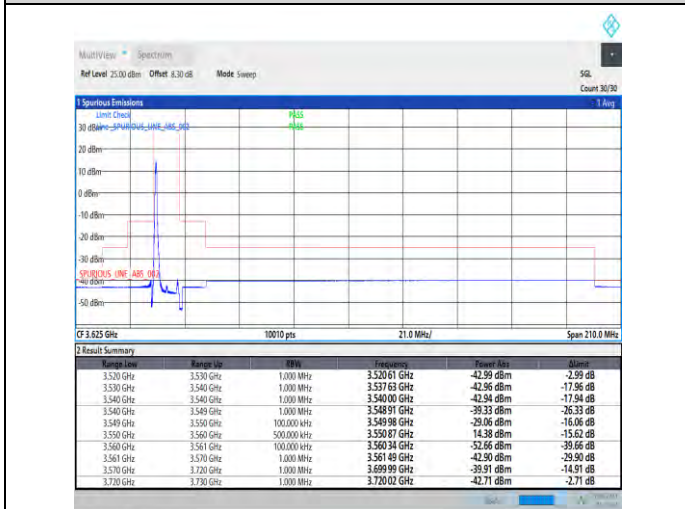
1-N48-PC3-30-10-L-1-DFT-PI2BPSK-Edge_1RB_Left-1@0-Ant7-1--PASS-see graph
