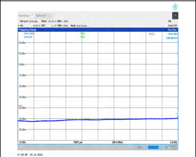
1-N48-PC3-30-40-H-1-DFT-PI2BPSK-Inner_1RB_Lef t-1@1-1000-3000-Ant7-2996.80--47.22--40-PASS
