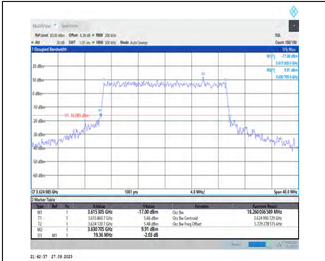
1-N48-PC3-30-20-M-7-CP-16QAM-Outer_Full-51@0 -Ant7-18.26-19.360-<20-PASS
