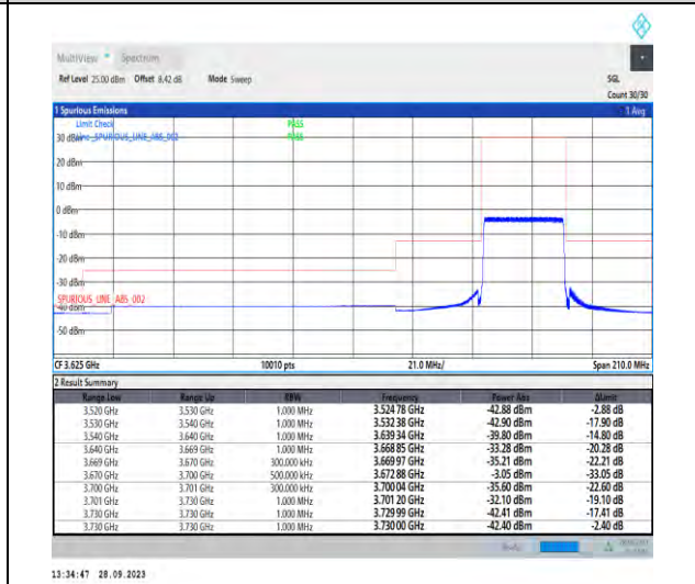
1-N48-PC3-30-30-H-6-CP-QPSK-Outer_Full-78@0-Ant7-1--PASS-see graph
