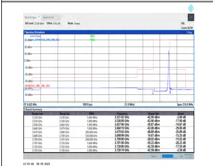
1-N48-PC3-30-20-H-5-CP-QPSK-Edge_1RB_Righ t-1@50-Ant7-1--PASS-see graph
