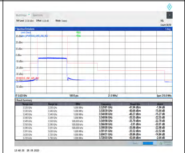
1-N48-PC3-30-40-L-6-CP-QPSK-Outer_Full-106@0-Ant7-1--PASS-see graph
