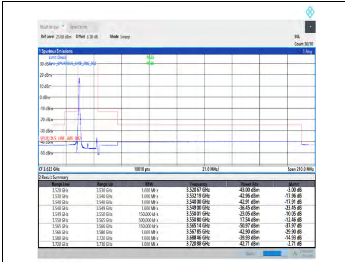
1-N48-PC3-30-15-L-1-DFT-PI2BPSK-Edge_1RB_Left-1@0-Ant7-1--PASS-see graph
