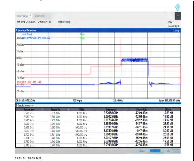
1-N48-PC3-30-40-H-3-DFT-PI2BPSK-Outer_Full-1 00@0-Ant7-1--PASS-see graph
