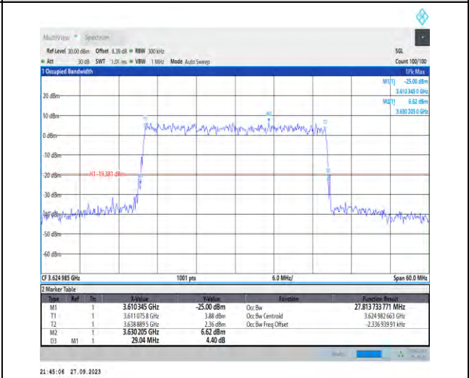
1-N48-PC3-30-30-M-9-CP-256QAM-Outer_Full-78@0-Ant7-27.814-29.040-≤30-PASS
