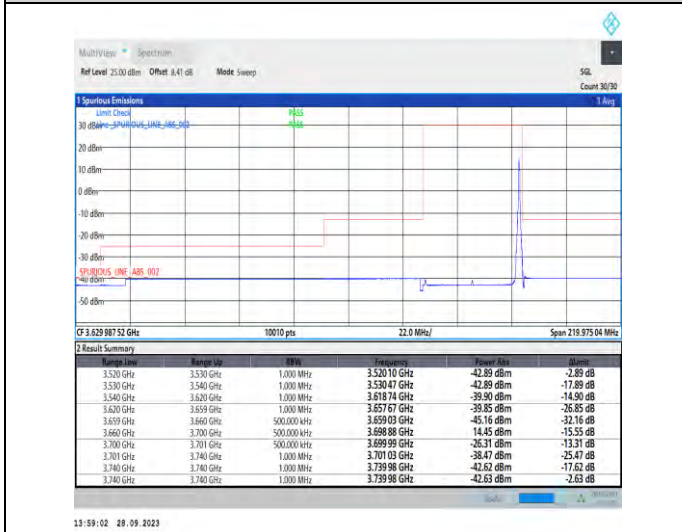
1-N48-PC3-30-40-H-5-CP-QPSK-Edge_1RB_Righ t-1@105-Ant7-1--PASS-see graph
