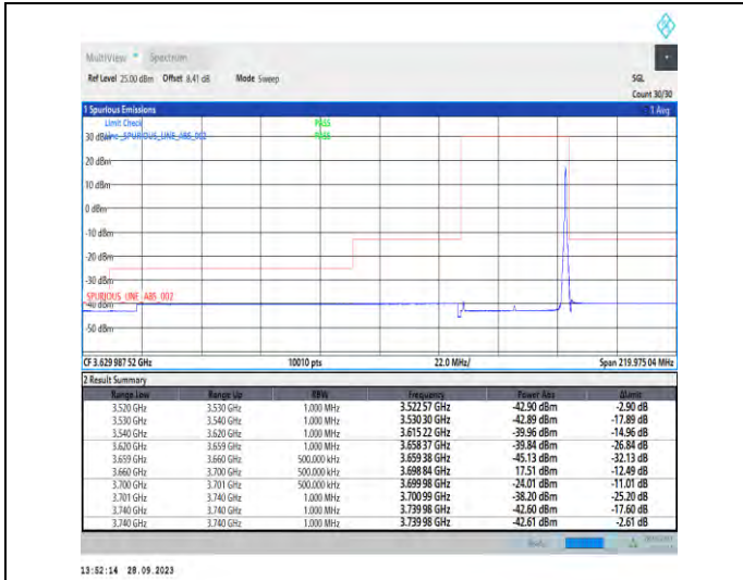
1-N48-PC3-30-40-H-2-DFT-PI2BPSK-Edge_1RB_Righ t-1@105-Ant7-1--PASS-see graph
