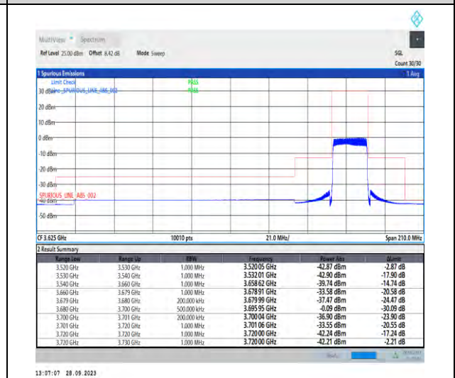
1-N48-PC3-30-20-H-6-CP-QPSK-Outer_Full-51@ 0-Ant7-1--PASS-see graph
