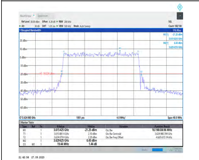
1-N48-PC3-30-20-M-9-CP-256QAM-Outer_Full-51@0 0-Ant7-18.198-19.440-<20-PASS
