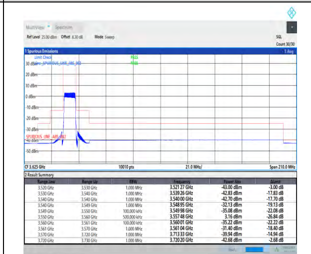
1-N48-PC3-30-10-L-3-DFT-PI2BPSK-Outer_Full-24@0-Ant7-1--PASS-see graph
