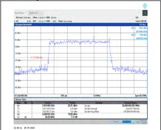
1-N48-PC3-30-30-M-3-DFT-16QAM-Outer_Full-75 @0-Ant7-26.84-28.260-≤30-PASS
