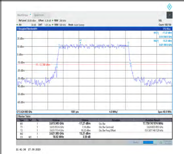
1-N48-PC3-30-20-M-2-DFT-PI2BPSK-Outer_Full-50 @0-Ant7-17.76-18.920-≤20-PASS
