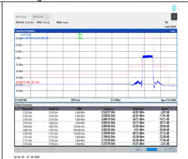
1-N48-PC3-30-15-H-3-DFT-PI2BPSK-Outer_Full-36@0-Ant7-1--PASS-see graph
