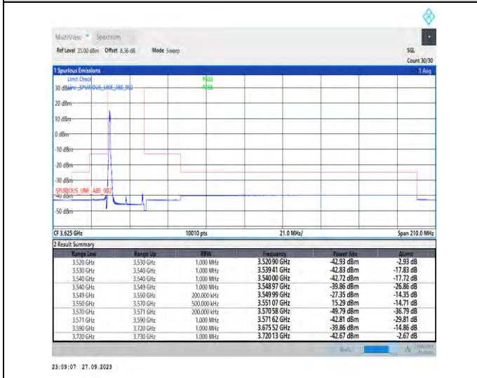
1-N48-PC3-30-20-L-4-CP-QPSK-Edge_1RB_Left-1@0-Ant7-1--PASS-see graph
