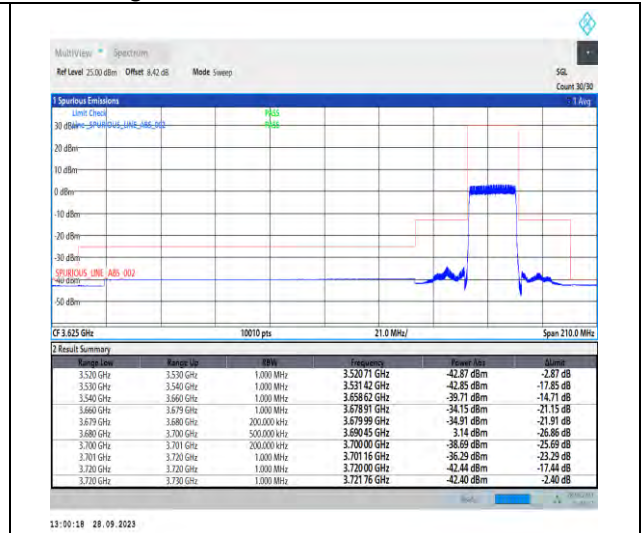
1-N48-PC3-30-20-H-3-DFT-PI2BPSK-Outer_Full-5 0@0-Ant7-1--PASS-see graph
