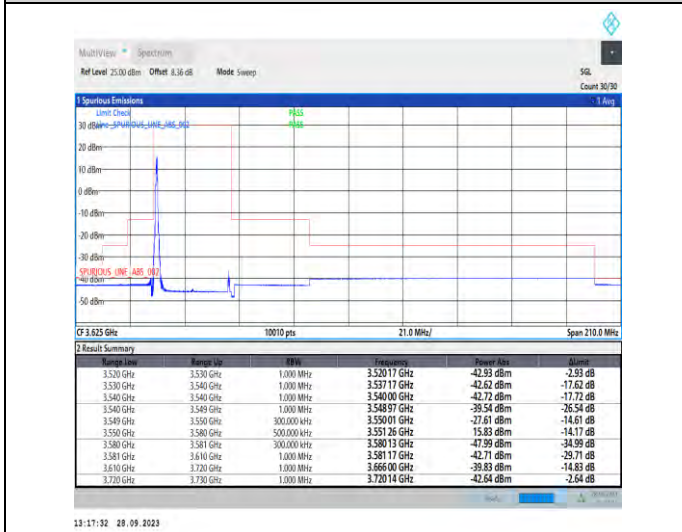
1-N48-PC3-30-30-L-4-CP-QPSK-Edge_1RB_Left-1@0-Ant7-1--PASS-see graph
