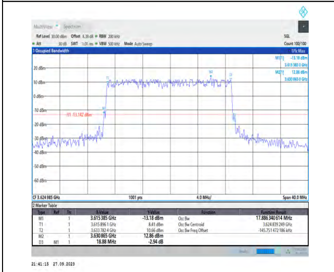
1-N48-PC3-30-20-M-1-DFT-QPSK-Outer_Full-50@0- Ant7-17.886-18.880-≤20-PASS
