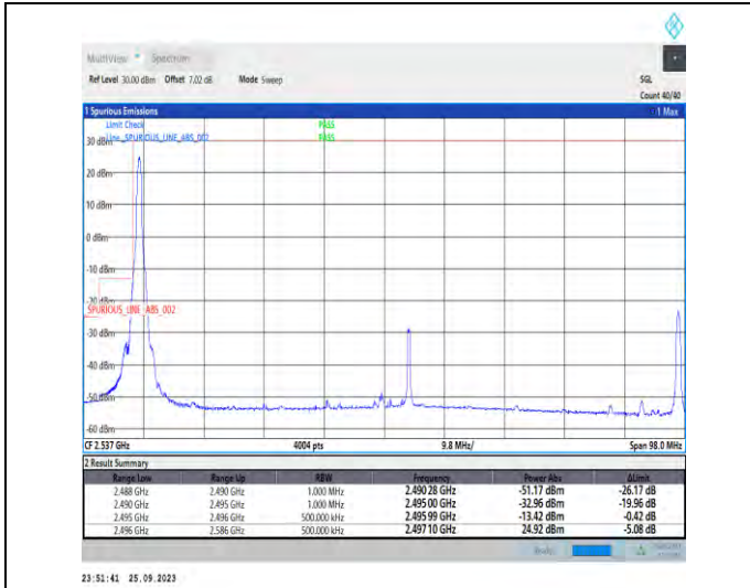
1-N41-PC3-30-90-L-1-DFT-PI2BPSK-Edge_1RB_Left-1@0-Ant5-1--PASS-see graph
