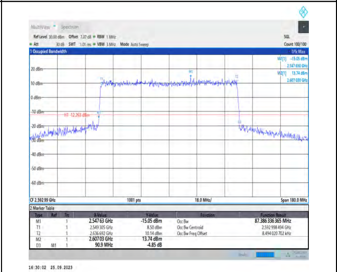
1-N41-PC3-30-90-M-7-CP-16QAM-Outer_Full-245@0 -Ant5-87.386-90.900-≤90-PASS
