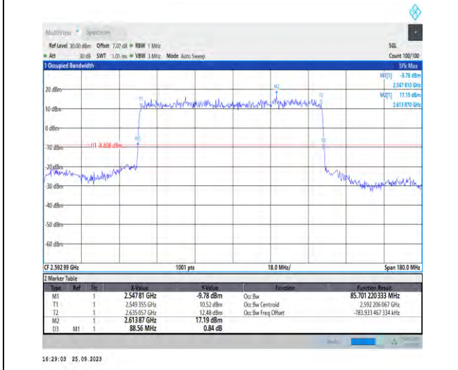
1-N41-PC3-30-90-M-2-DFT-PI2BPSK-Outer_Full-240 @0-Ant5-85.701-88.560-≤90-PASS
