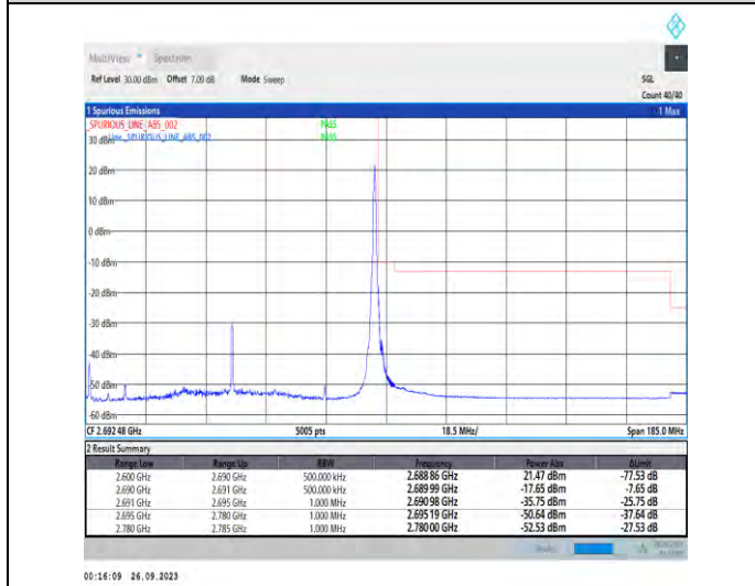
1-N41-PC3-30-90-H-5-CP-QPSK-Edge_1RB_Righ t-1@244-Ant5-1--PASS-see graph
