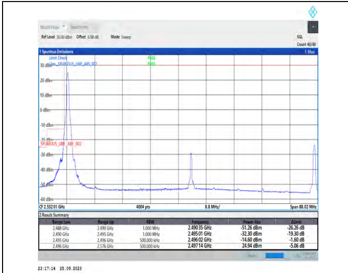
1-N41-PC3-30-80-L-1-DFT-PI2BPSK-Edge_1RB_Left-1@0-Ant5-1--PASS-see graph
