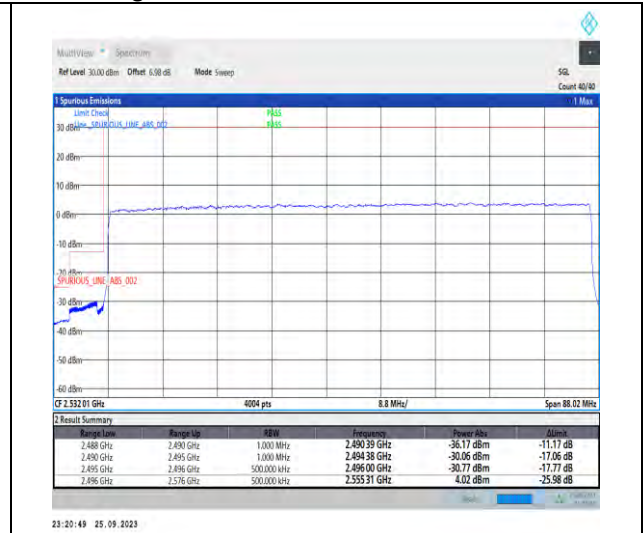
1-N41-PC3-30-80-L-3-DFT-PI2BPSK-Outer_Full-216@0-Ant5-1--PASS-see graph
