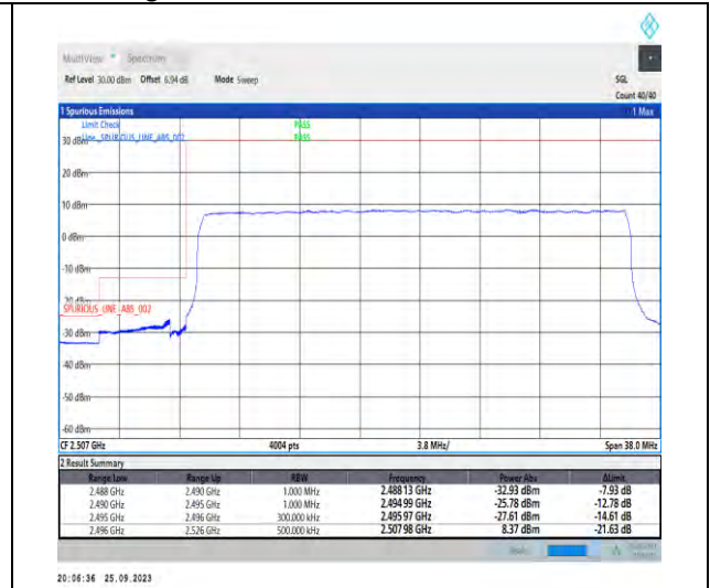
1-N41-PC3-30-30-L-3-DFT-PI2BPSK-Outer_Full-75@0-Ant5-1--PASS-see graph
