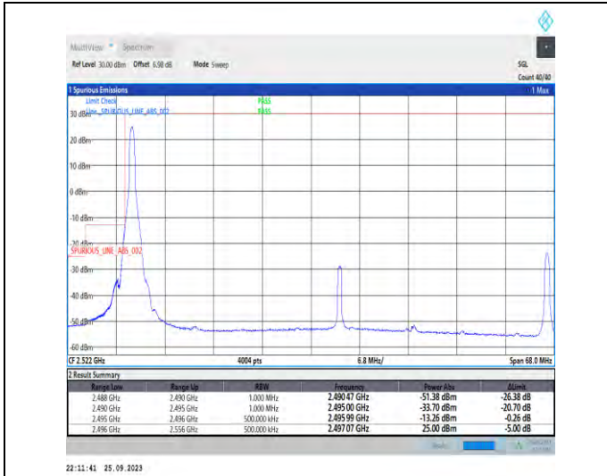
1-N41-PC3-30-60-L-1-DFT-PI2BPSK-Edge_1RB_Left-1@0-Ant5-1--PASS-see graph
