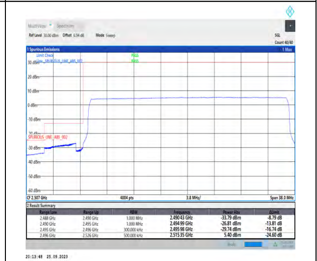
1-N41-PC3-30-30-L-6-CP-QPSK-Outer_Full-78@0-Ant5-1--PASS-see graph
