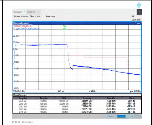
1-N41-PC3-30-20-H-6-CP-QPSK-Outer_Full-51@ 0-Ant5-1--PASS-see graph
