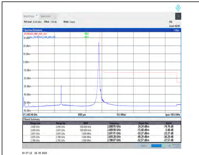
1-N41-PC3-30-90-H-2-DFT-PI2BPSK-Edge_1RB_Righ t-1@244-Ant5-1--PASS-see graph
