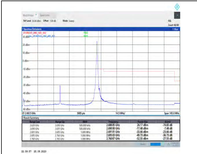
1-N41-PC3-30-70-H-2-DFT-PI2BPSK-Edge_1RB_Righ t-1@188-Ant5-1--PASS-see graph
