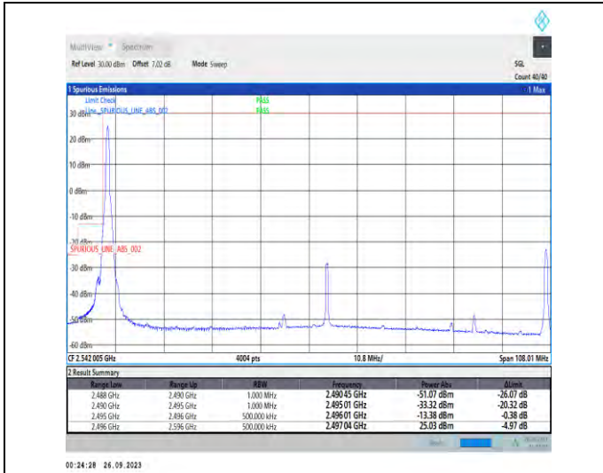
1-N41-PC3-30-100-L-1-DFT-PI2BPSK-Edge_1RB_Left-1@0-Ant5-1--PASS-see graph
