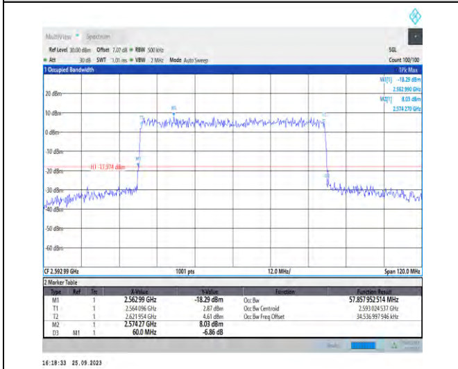
1-N41-PC3-30-60-M-9-CP-256QAM-Outer_Full-162 @0-Ant5-57.858-60.000-≤60-PASS
