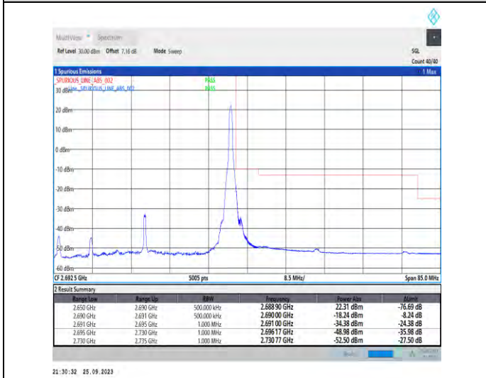
1-N41-PC3-30-40-H-5-CP-QPSK-Edge_1RB_Righ t-1@105-Ant5-1--PASS-see graph
