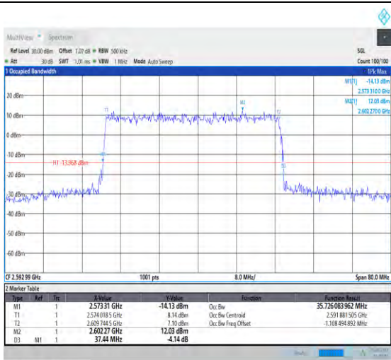
1-N41-PC3-30-40-M-5-DFT-256QAM-Outer_Full-100 @0-Ant5-35.726-37.440-≤40-PASS
