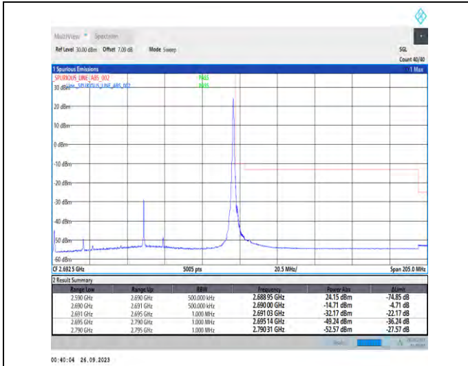
1-N41-PC3-30-100-H-2-DFT-PI2BPSK-Edge_1RB_Rig ht-1@272-Ant5-1--PASS-see graph
