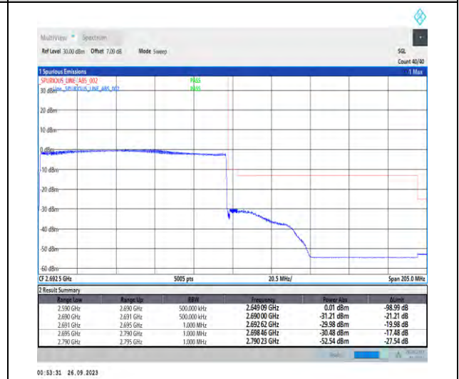
1-N41-PC3-30-100-H-6-CP-QPSK-Outer_Full-273 @0-Ant5-1--PASS-see graph
