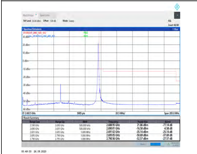
1-N41-PC3-30-100-H-5-CP-QPSK-Edge_1RB_Right-1 @272-Ant5-1--PASS-see graph
