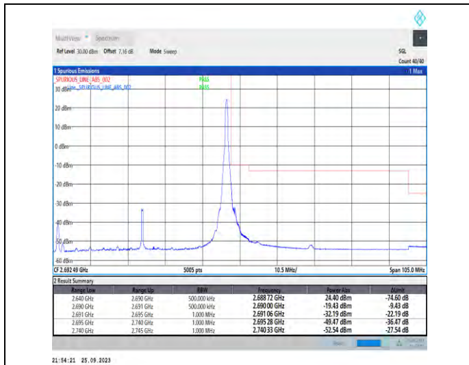
1-N41-PC3-30-50-H-2-DFT-PI2BPSK-Edge_1RB_Righ t-1@132-Ant5-1--PASS-see graph
