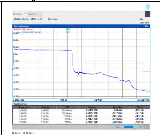
1-N41-PC3-30-40-H-3-DFT-PI2BPSK-Outer_Full-1 00@0-Ant5-1--PASS-see graph
