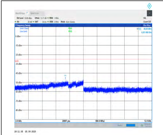
1-N41-PC3-30-100-L-1-DFT-PI2BPSK-Inner_1RB_Left-1@1-3000-12000-Ant5-6321.00--46.00--25-PASS S
