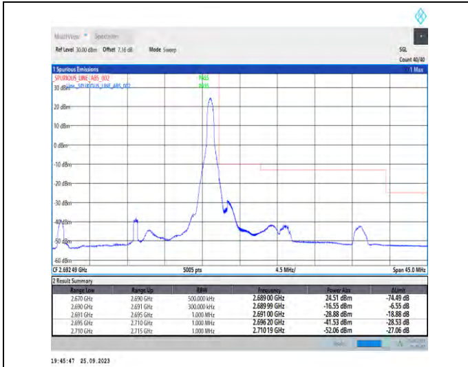
1-N41-PC3-30-20-H-2-DFT-PI2BPSK-Edge_1RB_Righ t-1@50-Ant5-1--PASS-see graph
