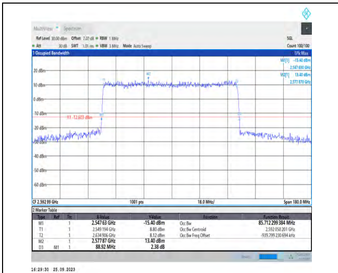
1-N41-PC3-30-90-M-4-DFT-64QAM-Outer_Full-240 @0-Ant5-85.712-88.920-≤90-PASS
