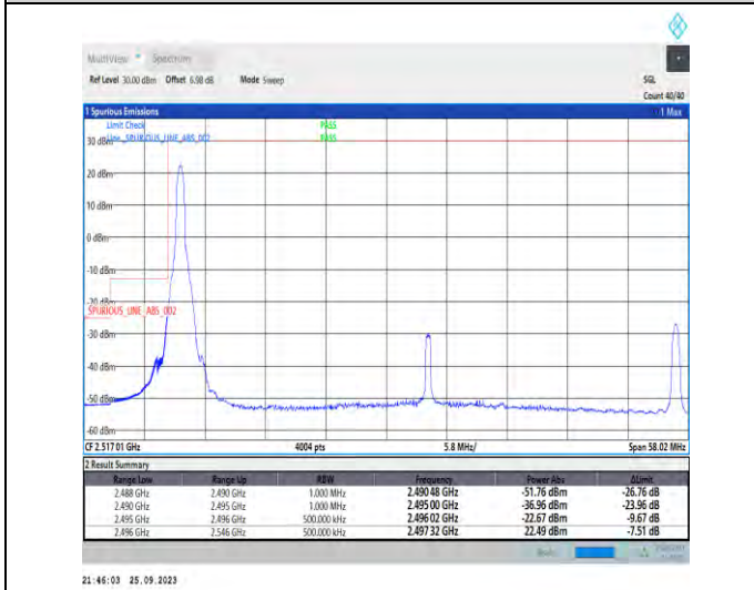
1-N41-PC3-30-50-L-4-CP-QPSK-Edge_1RB_Left-1@0-Ant5-1--PASS-see graph
