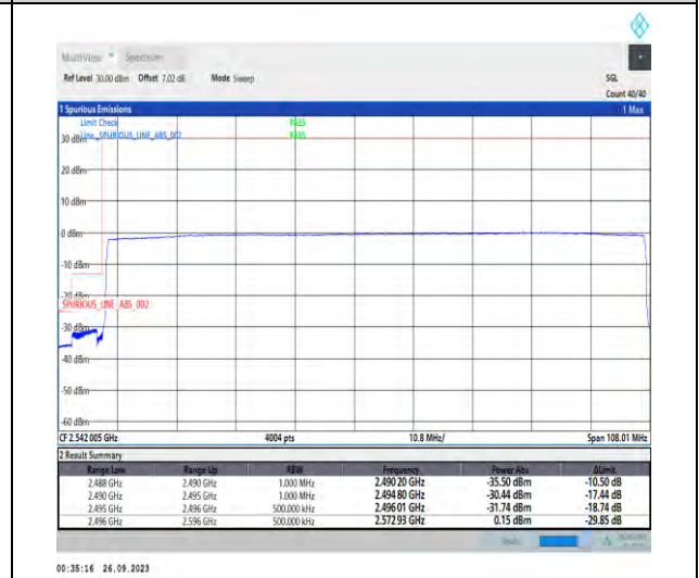
1-N41-PC3-30-100-L-6-CP-QPSK-Outer_Full-273@0-Ant5-1--PASS-see graph
