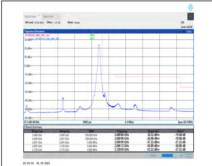
1-N41-PC3-30-30-H-2-DFT-PI2BPSK-Edge_1RB_Righ t-1@77-Ant5-1--PASS-see graph
