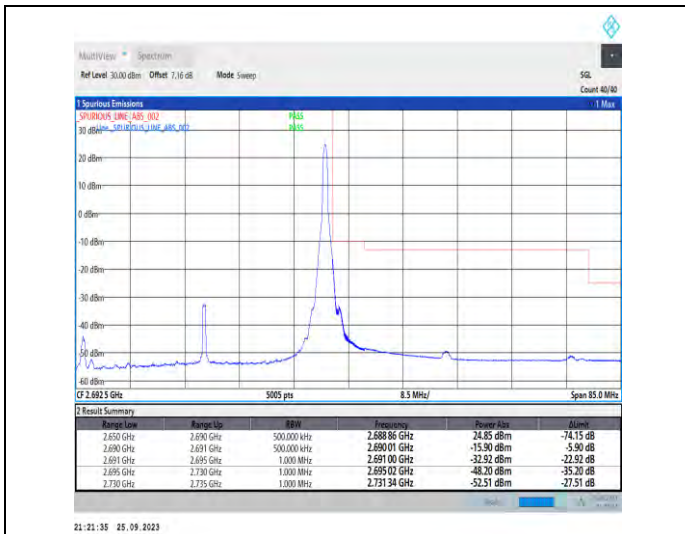
1-N41-PC3-30-40-H-2-DFT-PI2BPSK-Edge_1RB_Righ t-1@105-Ant5-1--PASS-see graph
