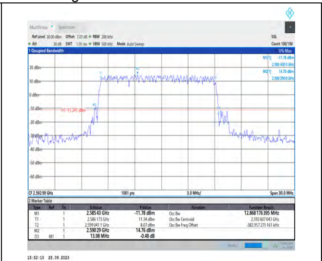
1-N41-PC3-30-15-M-1-DFT-QPSK-Outer_Full-36@ 0-Ant5-12.868-13.980-<=15-PASS
