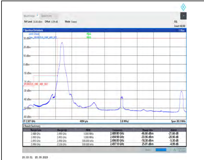
1-N41-PC3-30-30-L-1-DFT-PI2BPSK-Edge_1RB_Left-1@0-Ant5-1--PASS-see graph
