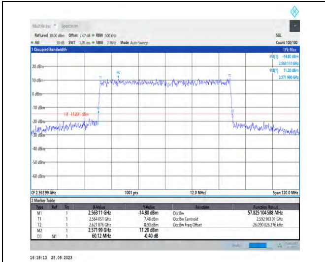
1-N41-PC3-30-60-M-7-CP-16QAM-Outer_Full-162@ 0-Ant5-57.825-60.120-≤60-PASS
