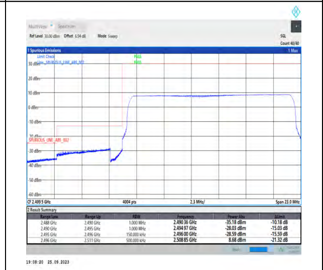
1-N41-PC3-30-15-L-6-CP-QPSK-Outer_Full-38@0-Ant5-1--PASS-see graph
