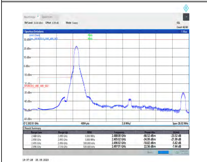
1-N41-PC3-30-20-L-4-CP-QPSK-Edge_1RB_Left-1@0-Ant5-1--PASS-see graph
