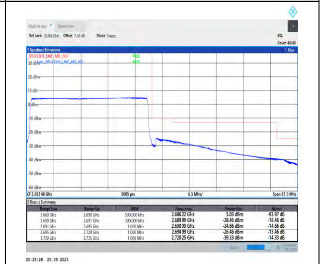
1-N41-PC3-30-30-H-6-CP-QPSK-Outer_Full-78@ 0-Ant5-1--PASS-see graph
