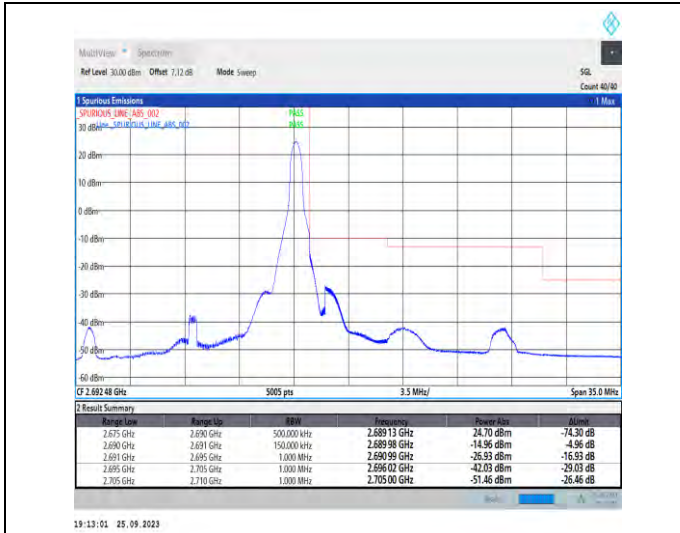
1-N41-PC3-30-15-H-2-DFT-PI2BPSK-Edge_1RB_Righ t-1@37-Ant5-1--PASS-see graph
