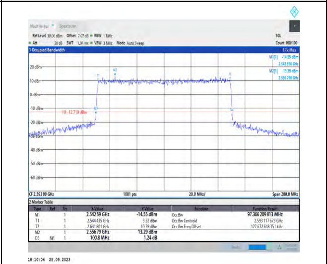
1-N41-PC3-30-100-M-6-CP-QPSK-Outer_Full-273 @0-Ant5-97.366-100.800-≤100-PASS
