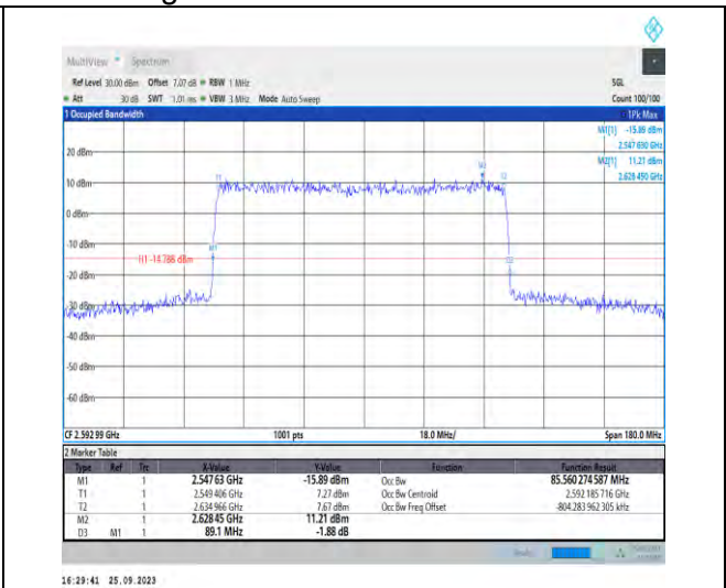
1-N41-PC3-30-90-M-5-DFT-256QAM-Outer_Full-240 @0-Ant5-85.56-89.100-≤90-PASS
