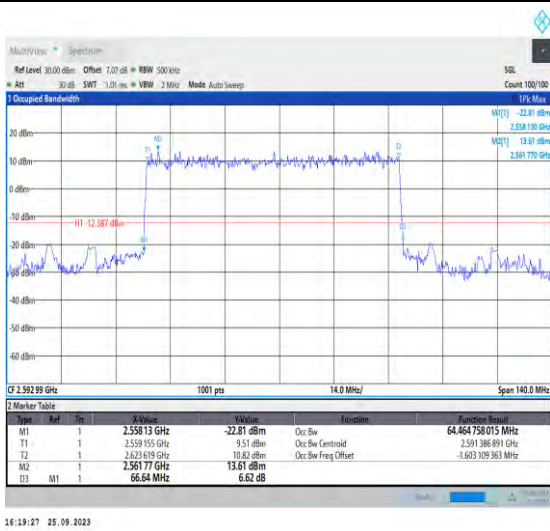
1-N41-PC3-30-70-M-2-DFT-PI2BPSK-Outer_Full-180 @0-Ant5-64.465-66.640-≤70-PASS
