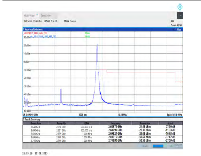
1-N41-PC3-30-50-H-5-CP-QPSK-Edge_1RB_Right-1 @132-Ant5-1--PASS-see graph
