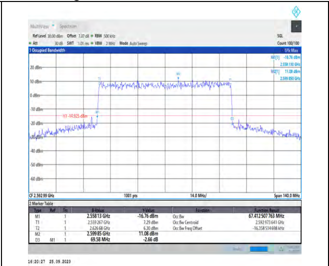
1-N41-PC3-30-70-M-7-CP-16QAM-Outer_Full-189@0 -Ant5-67.413-69.580-≤70-PASS
