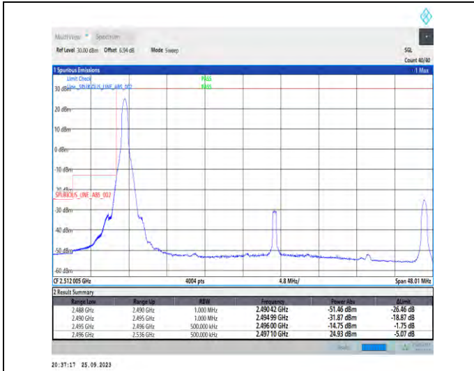
1-N41-PC3-30-40-L-1-DFT-PI2BPSK-Edge_1RB_Left-1@0-Ant5-1--PASS-see graph
