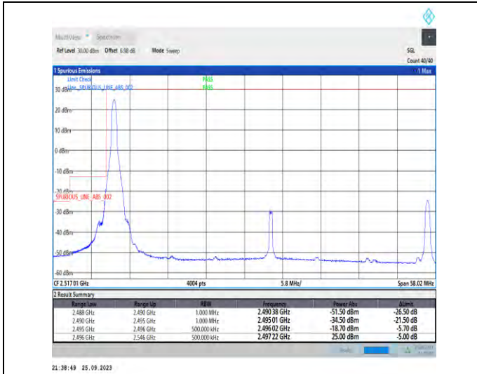
1-N41-PC3-30-50-L-1-DFT-PI2BPSK-Edge_1RB_Left-1@0-Ant5-1--PASS-see graph
