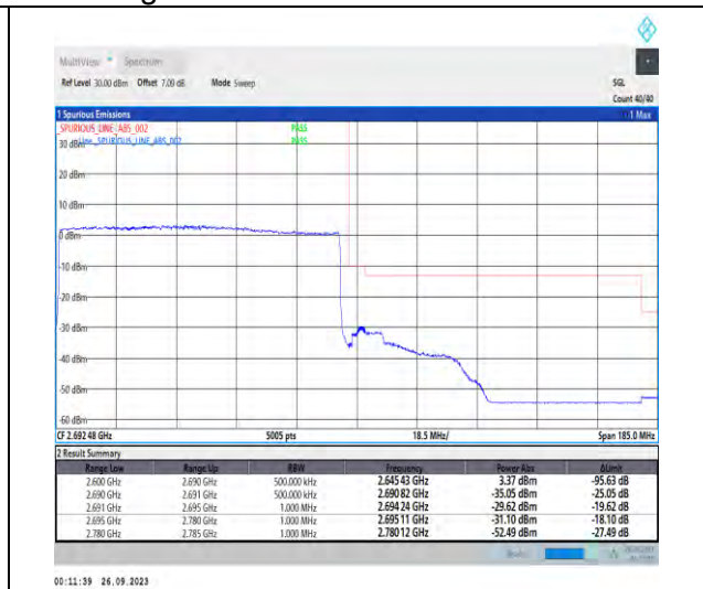
1-N41-PC3-30-90-H-3-DFT-PI2BPSK-Outer_Full-2 40@0-Ant5-1--PASS-see graph
