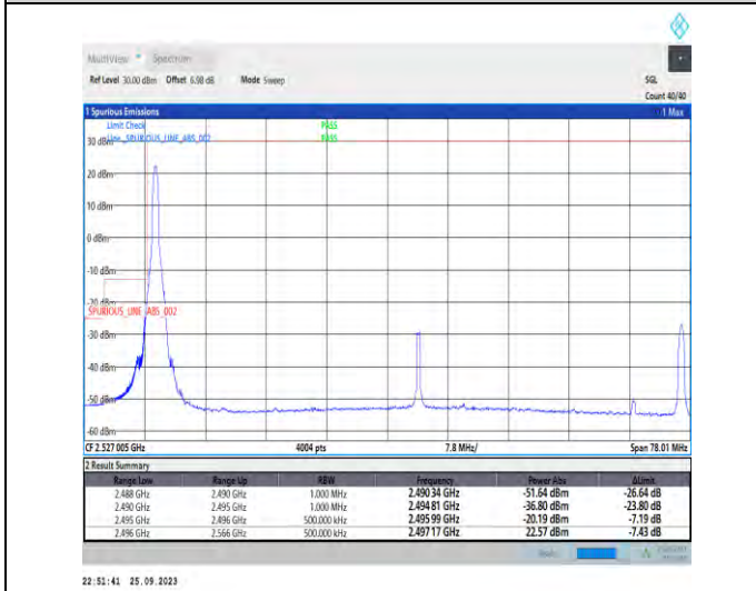
1-N41-PC3-30-70-L-4-CP-QPSK-Edge_1RB_Left-1@0-Ant5-1--PASS-see graph
