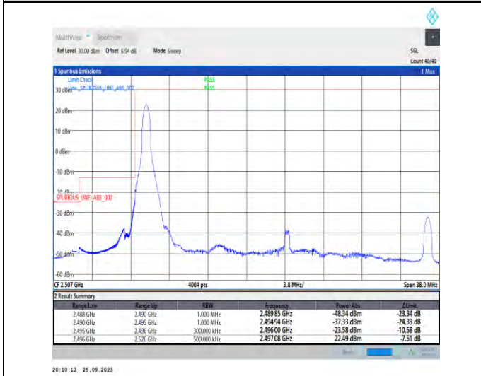
1-N41-PC3-30-30-L-4-CP-QPSK-Edge_1RB_Left-1@0-Ant5-1--PASS-see graph
