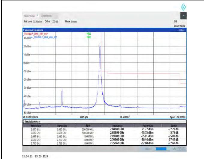
1-N41-PC3-30-60-H-5-CP-QPSK-Edge_1RB_Right-1 @161-Ant5-1--PASS-see graph
