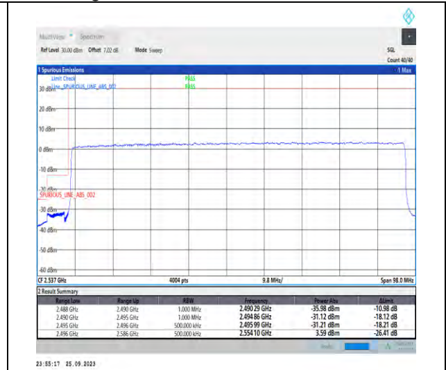
1-N41-PC3-30-90-L-3-DFT-PI2BPSK-Outer_Full-240@0-Ant5-1--PASS-see graph
