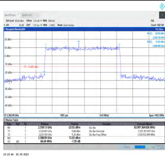
1-N41-PC3-30-70-M-3-DFT-16QAM-Outer_Full-180 @0-Ant5-63.991-66.640-≤70-PASS
