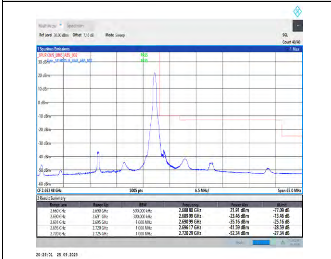
1-N41-PC3-30-30-H-5-CP-QPSK-Edge_1RB_Righ t1 @77-Ant5-1--PASS-see graph
