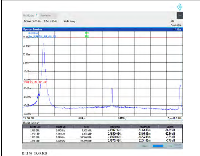
1-N41-PC3-30-60-L-4-CP-QPSK-Edge_1RB_Left-1@0-Ant5-1--PASS-see graph
