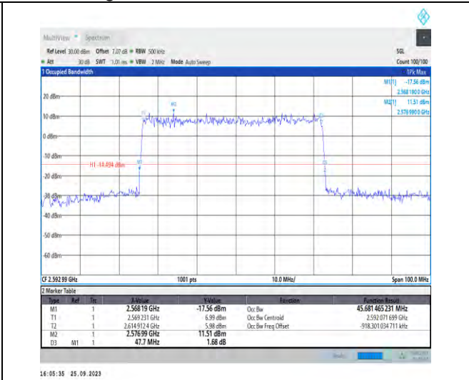
1-N41-PC3-30-50-M-5-DFT-256QAM-Outer_Full-128 @0-Ant5-45.681-47.700-≤50-PASS
