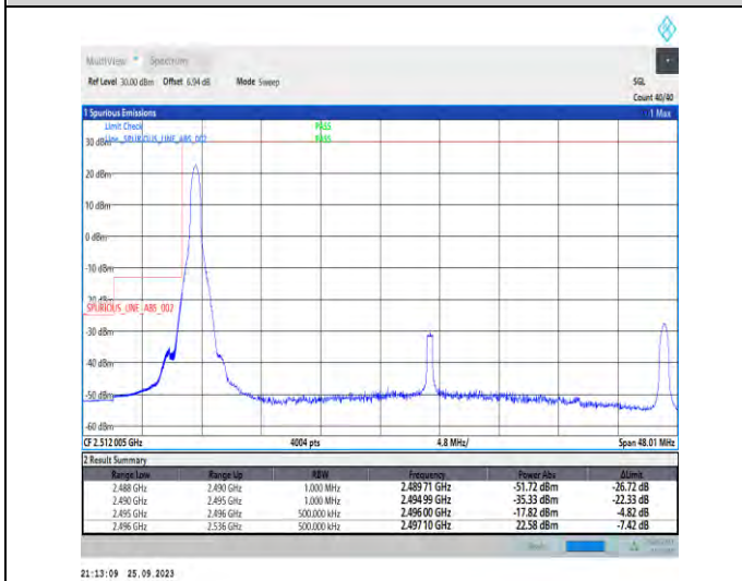
1-N41-PC3-30-40-L-4-CP-QPSK-Edge_1RB_Left-1@0-Ant5-1--PASS-see graph
