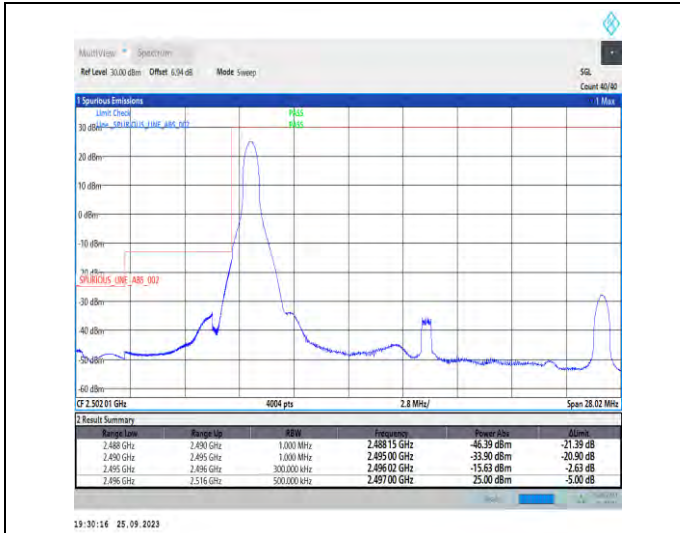
1-N41-PC3-30-20-L-1-DFT-PI2BPSK-Edge_1RB_Left-1@0-Ant5-1--PASS-see graph
