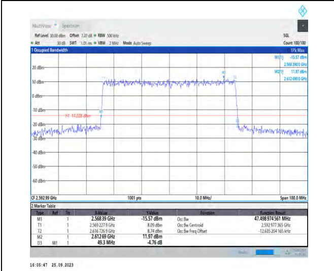
1-N41-PC3-30-50-M-6-CP-QPSK-Outer_Full-133@0 -Ant5-47.499-49.300-≤50-PASS
