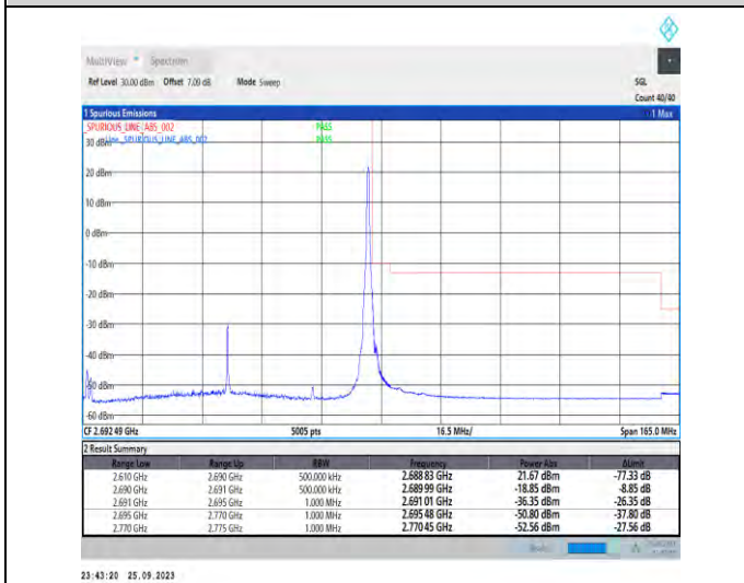
1-N41-PC3-30-80-H-5-CP-QPSK-Edge_1RB_Right-1 @216-Ant5-1--PASS-see graph
