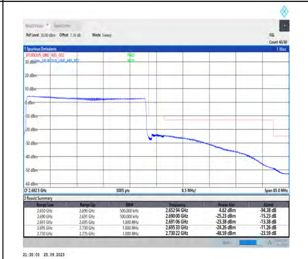
1-N41-PC3-30-40-H-6-CP-QPSK-Outer_Full-106 @0-Ant5-1--PASS-see graph
