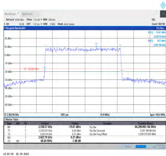
1-N41-PC3-30-70-M-5-DFT-256QAM-Outer_Full-180 @0-Ant5-64.299-66.640-≤70-PASS
