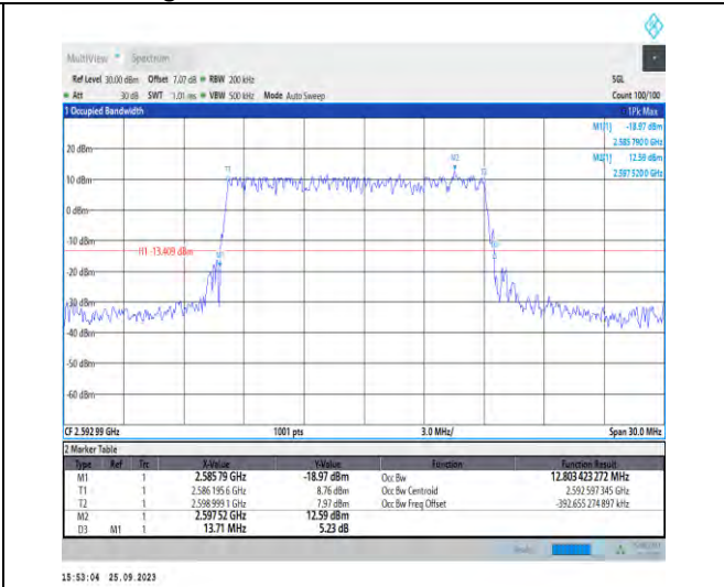
1-N41-PC3-30-15-M-5-DFT-256QAM-Outer_Full-36@0-Ant5-12.803-13.710-≤15-PASS
