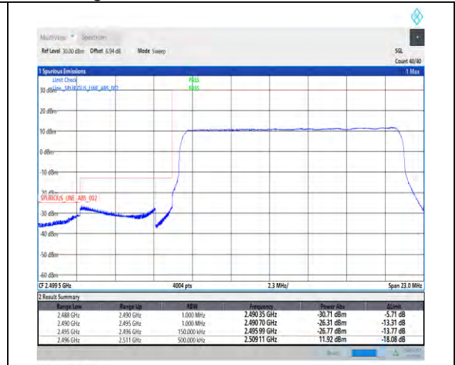
1-N41-PC3-30-15-L-3-DFT-PI2BPSK-Outer_Full-36@0-Ant5-1--PASS-see graph
