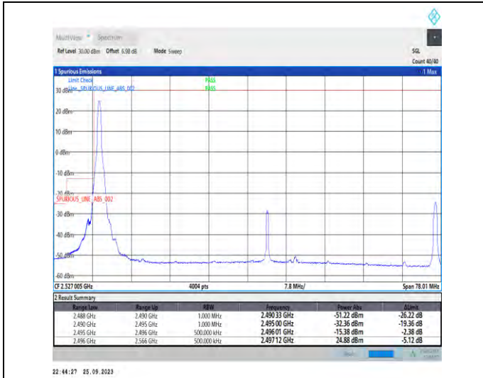
1-N41-PC3-30-70-L-1-DFT-PI2BPSK-Edge_1RB_Left-1@0-Ant5-1--PASS-see graph
