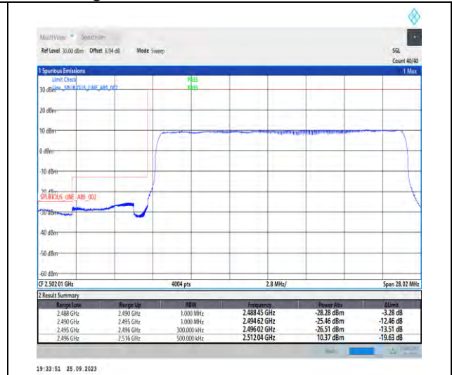
1-N41-PC3-30-20-L-3-DFT-PI2BPSK-Outer_Full-50@0-Ant5-1--PASS-see graph
