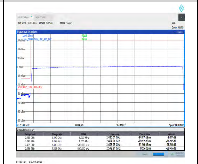
1-N41-PC3-30-90-L-6-CP-QPSK-Outer_Full-245@0-Ant5-1--PASS-see graph
