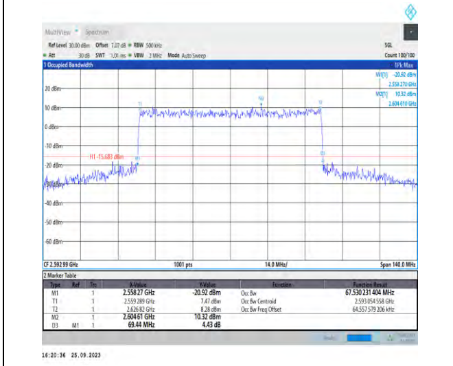
1-N41-PC3-30-70-M-8-CP-64QAM-Outer_Full-189@0 -Ant5-67.53-69.440-≤70-PASS
