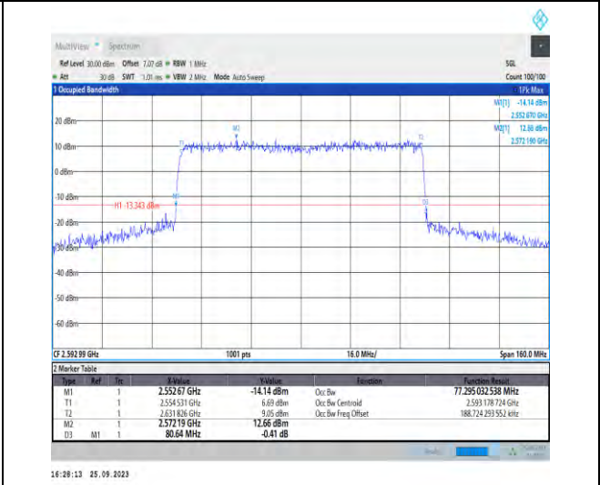
1-N41-PC3-30-80-M-8-CP-64QAM-Outer_Full-217@0-Ant5-77.295-80.640-<80-PASS
