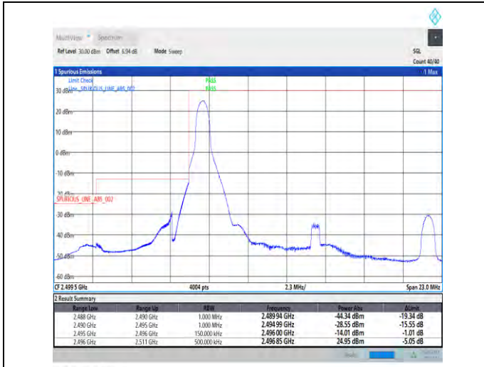
1-N41-PC3-30-15-L-1-DFT-PI2BPSK-Edge_1RB_Left-1@0-Ant5-1--PASS-see graph
