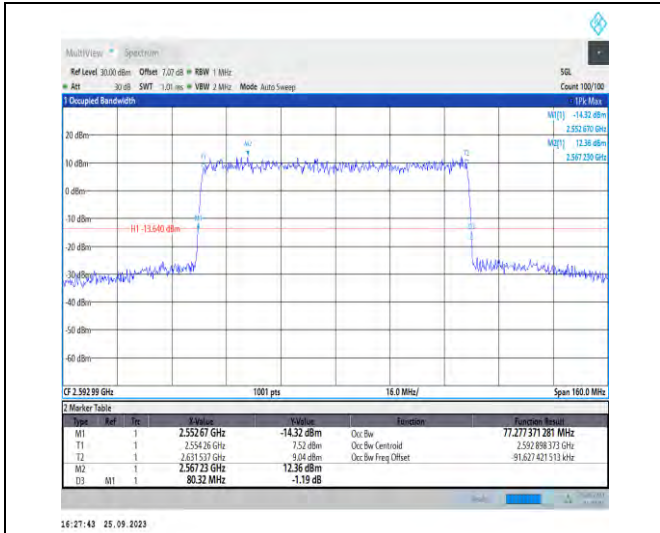
1-N41-PC3-30-80-M-5-DFT-256QAM-Outer_Full-216 @0-Ant5-77.277-80.320-<80-PASS
