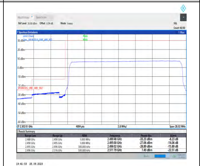
1-N41-PC3-30-20-L-6-CP-QPSK-Outer_Full-51@0-Ant5-1--PASS-see graph
