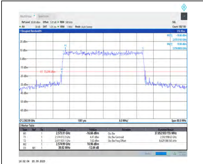
1-N41-PC3-30-40-M-9-CP-256QAM-Outer_Full-106 @0-Ant5-37.853-39.920-≤40-PASS
