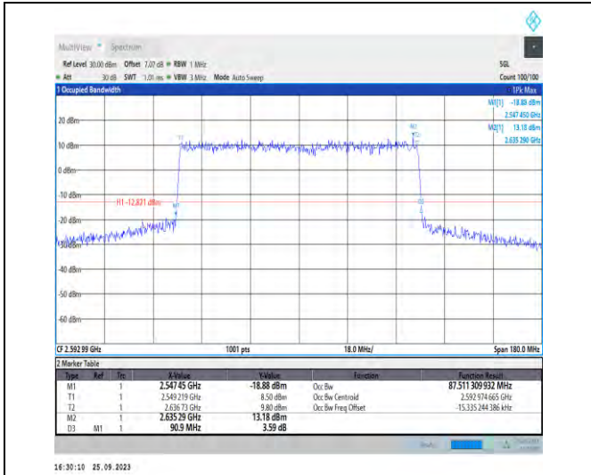
1-N41-PC3-30-90-M-8-CP-64QAM-Outer_Full-245@0-Ant5-87.511-90.900-<=90-PASS
