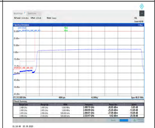
1-N41-PC3-30-40-L-6-CP-QPSK-Outer_Full-106@0-Ant5-1--PASS-see graph
