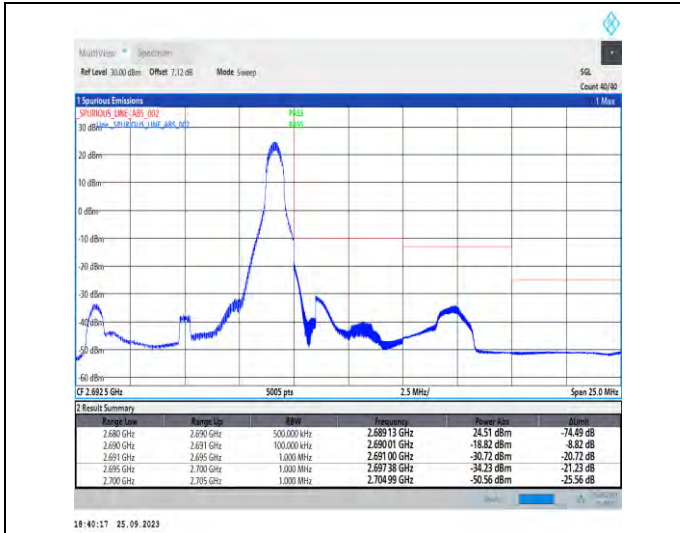
1-N41-PC3-30-10-H-2-DFT-PI2BPSK-Edge_1RB_Righ t-1@23-Ant5-1--PASS-see graph
