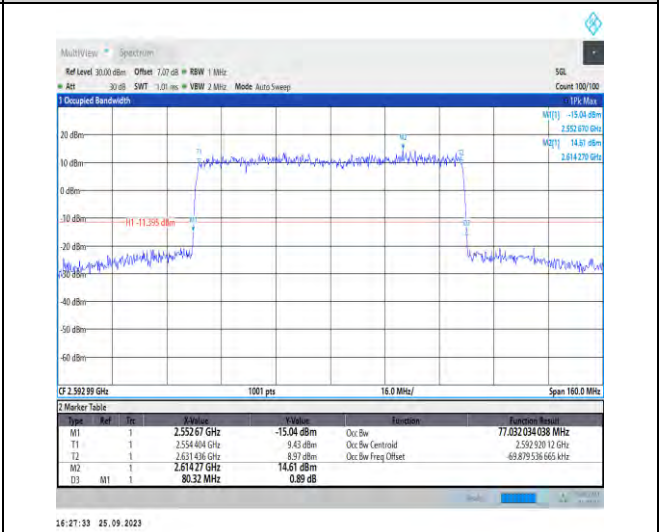
1-N41-PC3-30-80-M-4-DFT-64QAM-Outer_Full-216@0-Ant5-77.032-80.320-≤80-PASS
