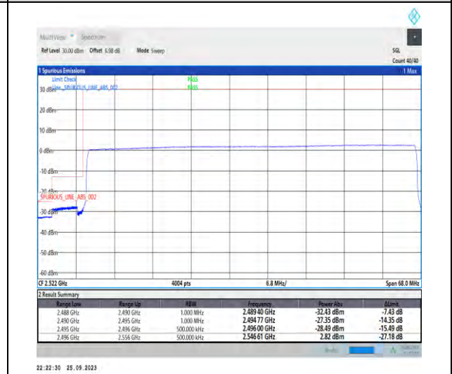
1-N41-PC3-30-60-L-6-CP-QPSK-Outer_Full-162@0-Ant5-1--PASS-see graph
