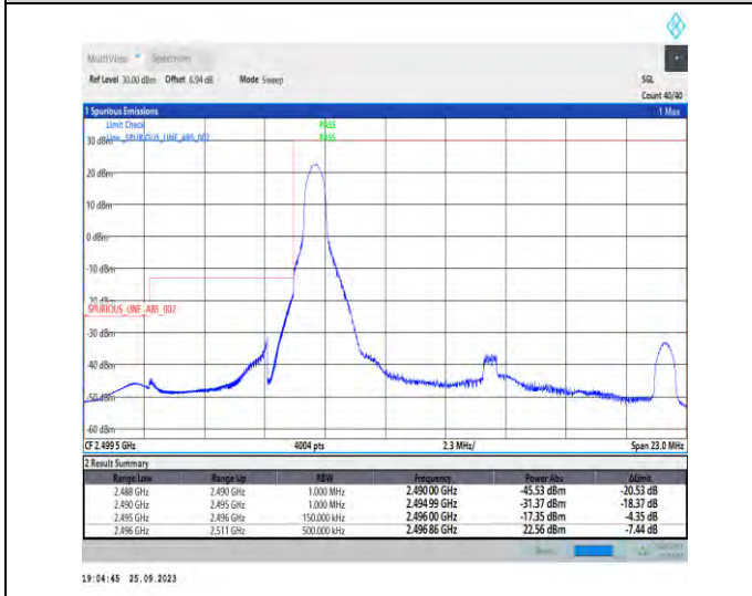
1-N41-PC3-30-15-L-4-CP-QPSK-Edge_1RB_Left-1@0-Ant5-1--PASS-see graph
