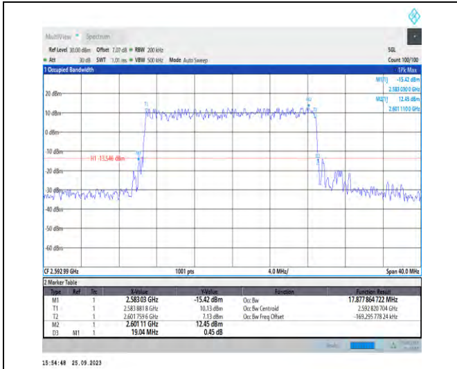
1-N41-PC3-30-20-M-3-DFT-16QAM-Outer_Full-50@0-Ant5-17.878-19.040-≤20-PASS
