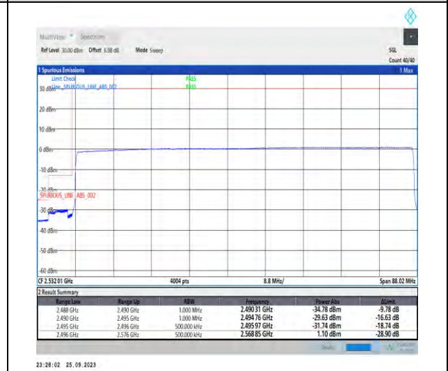
1-N41-PC3-30-80-L-6-CP-QPSK-Outer_Full-217@0-Ant5-1--PASS-see graph
