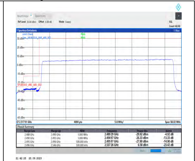
1-N41-PC3-30-50-L-3-DFT-PI2BPSK-Outer_Full-128@0-Ant5-1--PASS-see graph
