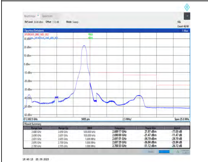
1-N41-PC3-30-10-H-5-CP-QPSK-Edge_1RB_Right-1 @23-Ant5-1--PASS-see graph
