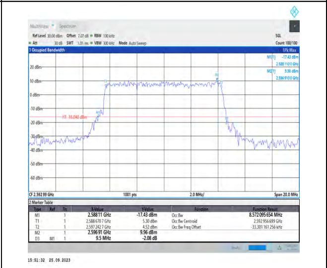
1-N41-PC3-30-10-M-8-CP-64QAM-Outer_Full-24@0-Ant5-8.572-9.500-≤10-PASS
