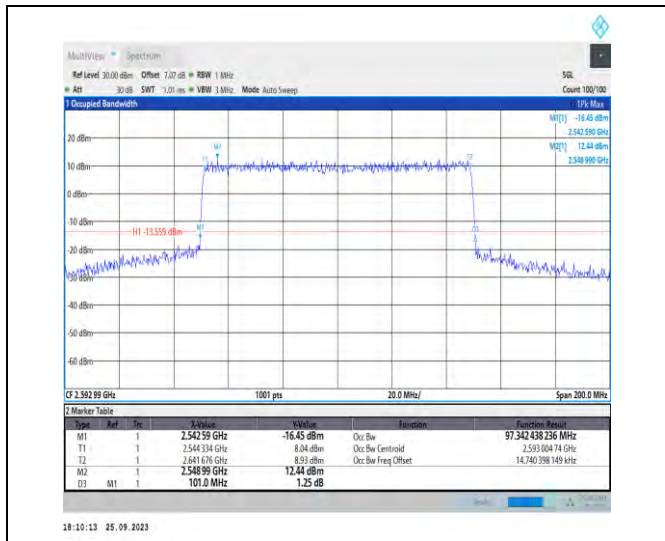
1-N41-PC3-30-100-M-7-CP-16QAM-Outer_Full-273 @0-Ant5-97.342-101.000-≤100-PASS
