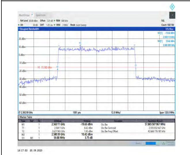
1-N41-PC3-30-60-M-5-DFT-256QAM-Outer_Full-162 @0-Ant5-57.866-59.880-≤60-PASS
