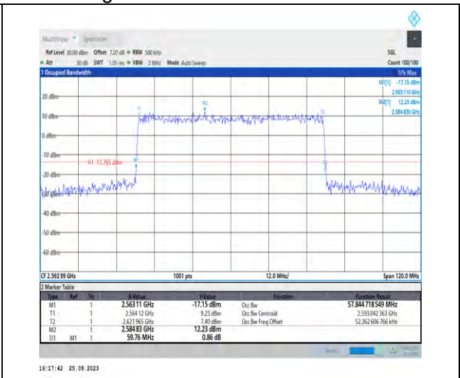
1-N41-PC3-30-60-M-4-DFT-64QAM-Outer_Full-162 @0-Ant5-57.845-59.760-≤60-PASS
