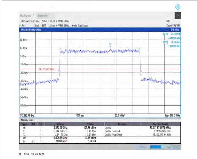
1-N41-PC3-30-100-M-9-CP-256QAM-Outer_Full-273 @0-Ant5-97.572-101.000-≤100-PASS
