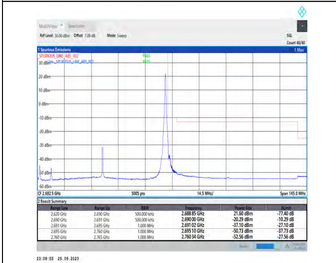
1-N41-PC3-30-70-H-5-CP-QPSK-Edge_1RB_Righ t-1@188-Ant5-1--PASS-see graph
