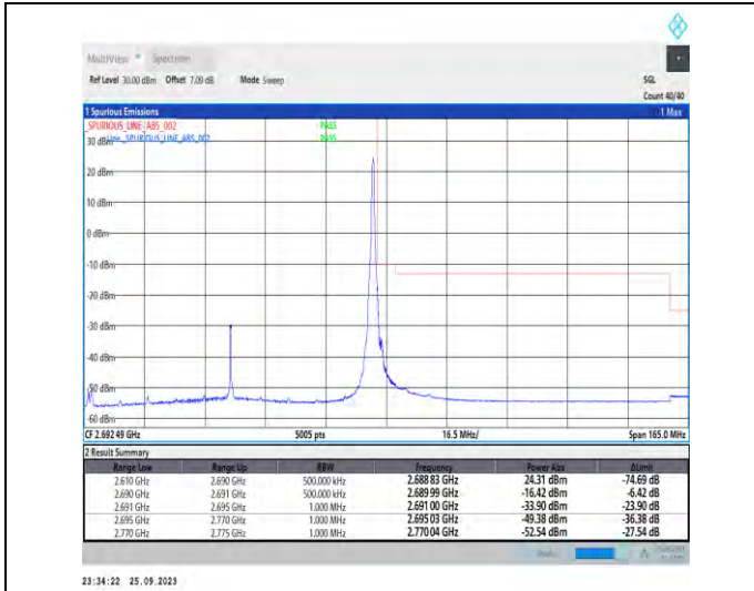
1-N41-PC3-30-80-H-2-DFT-PI2BPSK-Edge_1RB_Righ t-1@216-Ant5-1--PASS-see graph
