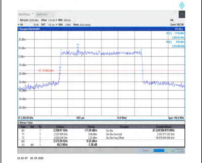
1-N41-PC3-30-70-M-9-CP-256QAM-Outer_Full-189@0 -Ant5-67.325-69.300-≤70-PASS
