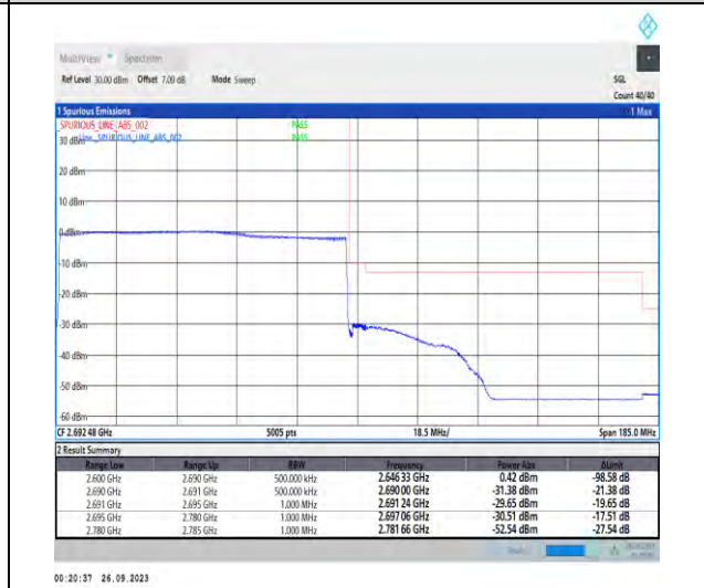
1-N41-PC3-30-90-H-6-CP-QPSK-Outer_Full-245 @0-Ant5-1--PASS-see graph
