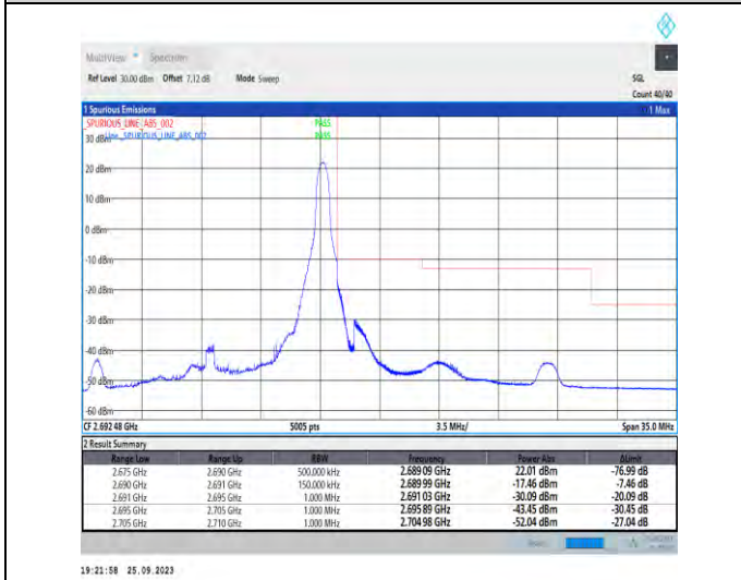
1-N41-PC3-30-15-H-5-CP-QPSK-Edge_1RB_Right-1 @37-Ant5-1--PASS-see graph
