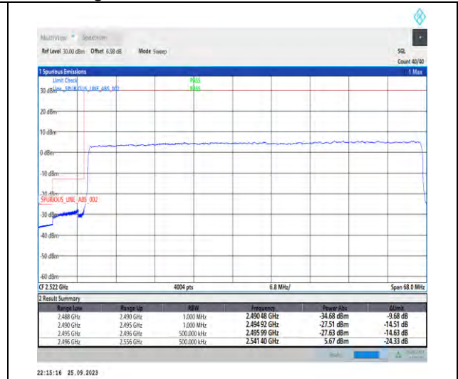
1-N41-PC3-30-60-L-3-DFT-PI2BPSK-Outer_Full-162@0-Ant5-1--PASS-see graph
