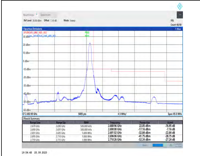
1-N41-PC3-30-20-H-5-CP-QPSK-Edge_1RB_Righ t-1@50-Ant5-1--PASS-see graph
