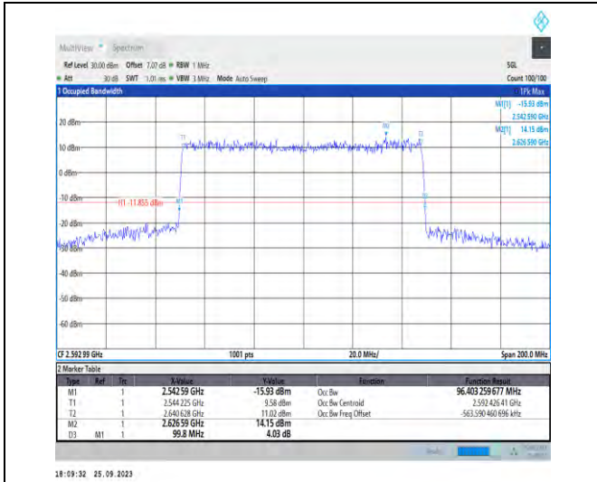
1-N41-PC3-30-100-M-3-DFT-16QAM-Outer_Full-270 @0-Ant5-96.403-99.800-≤100-PASS
