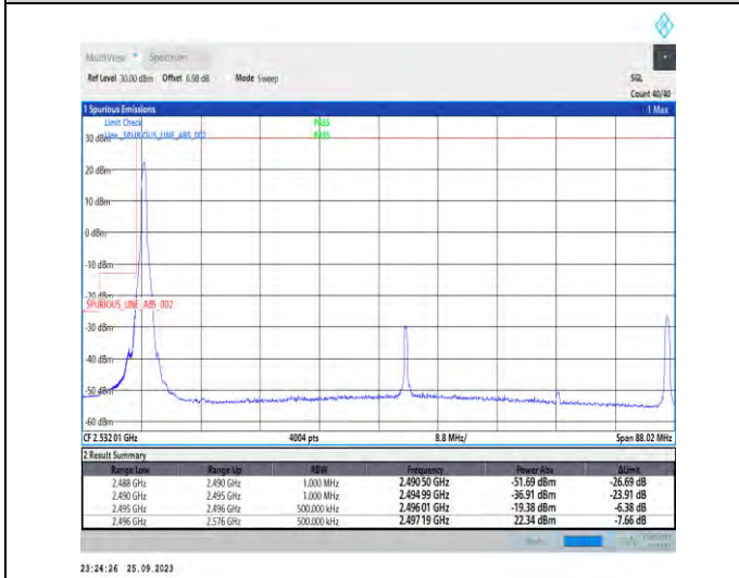
1-N41-PC3-30-80-L-4-CP-QPSK-Edge_1RB_Left-1@0-Ant5-1--PASS-see graph
