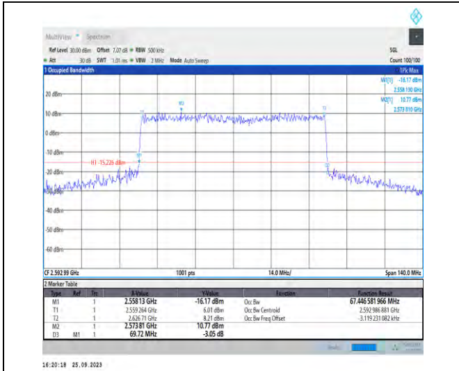
1-N41-PC3-30-70-M-6-CP-QPSK-Outer_Full-189@0 -Ant5-67.447-69.720-≤70-PASS
