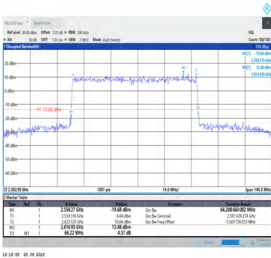
1-N41-PC3-30-70-M-4-DFT-64QAM-Outer_Full-180 @0-Ant5-64.209-66.220-≤70-PASS
