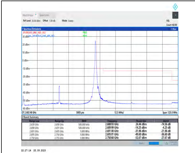
1-N41-PC3-30-60-H-2-DFT-PI2BPSK-Edge_1RB_Righ t-1@161-Ant5-1--PASS-see graph
