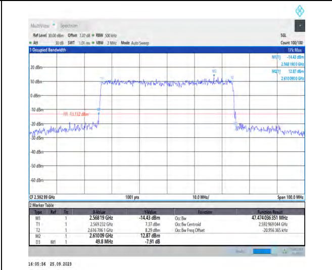
1-N41-PC3-30-50-M-7-CP-16QAM-Outer_Full-133@0 -Ant5-47.474-49.800-≤50-PASS
