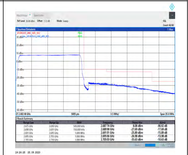
1-N41-PC3-30-15-H-6-CP-QPSK-Outer_Full-38@ 0-Ant5-1--PASS-see graph
