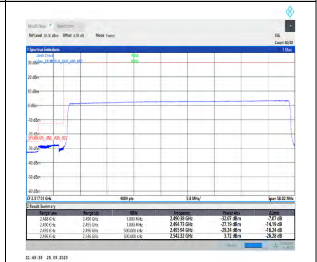
1-N41-PC3-30-50-L-6-CP-QPSK-Outer_Full-133@0-Ant5-1--PASS-see graph
