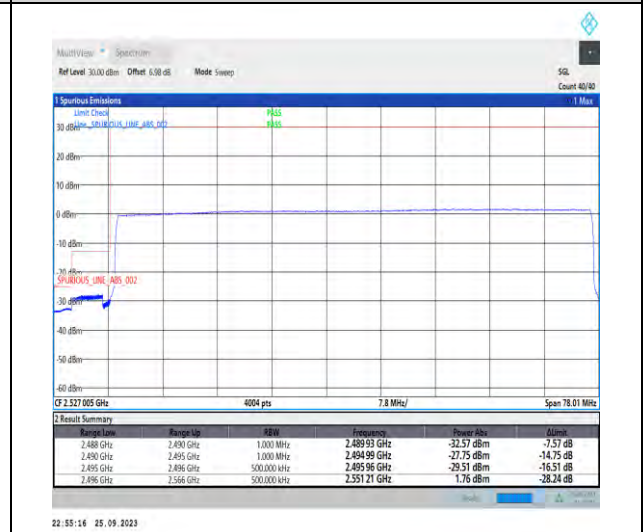
1-N41-PC3-30-70-L-6-CP-QPSK-Outer_Full-189@0-Ant5-1--PASS-see graph
