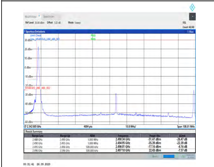
1-N41-PC3-30-100-L-4-CP-QPSK-Edge_1RB_Left1@0-Ant5-1--PASS-see graph
