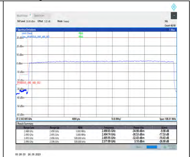
1-N41-PC3-30-100-L-3-DFT-PI2BPSK-Outer_Full-270@0-Ant5-1--PASS-see graph
