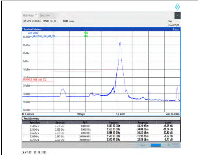
1-N38-PC3-30-20-L-1-DFT-PI2BPSK-Edge_1RB_Left-1@0-Ant5-1--PASS-see graph
