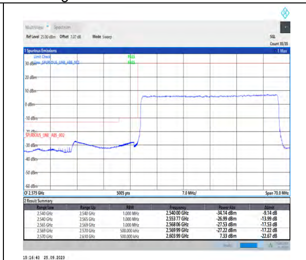
1-N38-PC3-30-40-L-3-DFT-PI2BPSK-Outer_Full-100@0-Ant5-1--PASS-see graph
