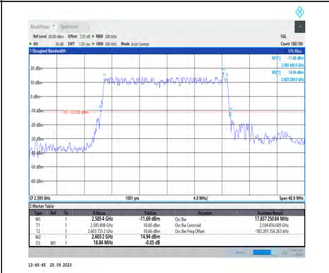
1-N38-PC3-30-20-M-2-DFT-PI2BPSK-Outer_Full-50@0 -Ant5-17.837-18.840-≤20-PASS
