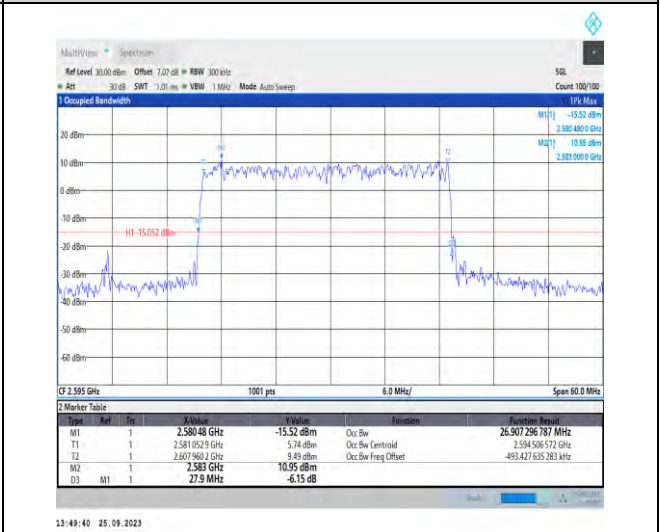
1-N38-PC3-30-30-M-5-DFT-256QAM-Outer_Full-75 @0-Ant5-26.907-27.900-<30-PASS
