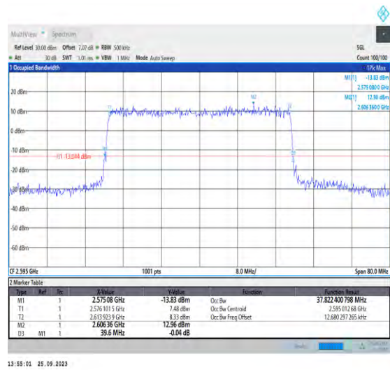
1-N38-PC3-30-40-M-6-CP-QPSK-Outer_Full-106@0-Ant5-37.822-39.600-≤40-PASS
