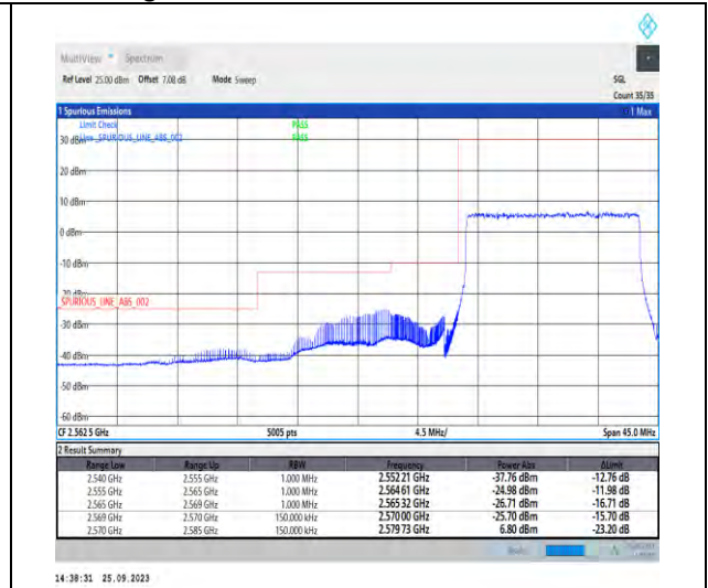
1-N38-PC3-30-15-L-3-DFT-PI2BPSK-Outer_Full-36@0-Ant5-1--PASS-see graph
