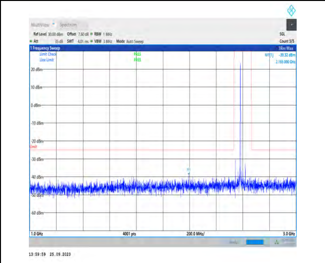
1-N38-PC3-30-40-H-1-DFT-PI2BPSK-Inner_1RB_Lef t-1@1-1000-3000-Ant5-2193.00--39.32--25-PASS
