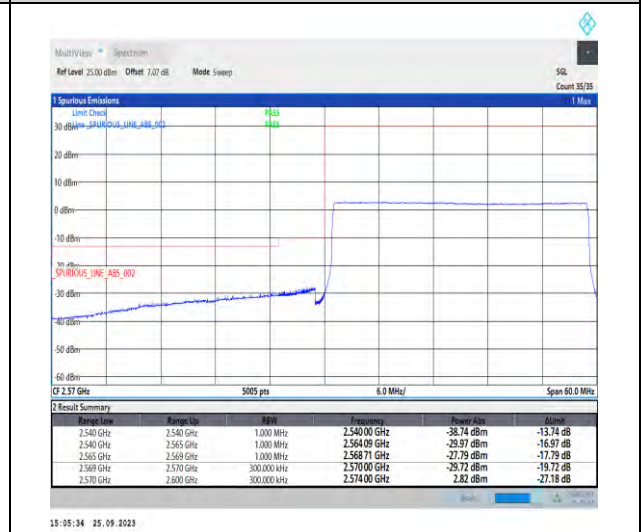
1-N38-PC3-30-30-L-6-CP-QPSK-Outer_Full-78@0-Ant5-1--PASS-see graph
