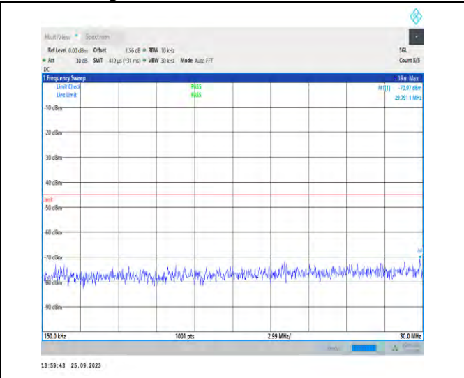
1-N38-PC3-30-40-H-1-DFT-PI2BPSK-Inner_1RB_Lef t-1@1-0.15-30-Ant5-29.79--70.97--45-PASS
