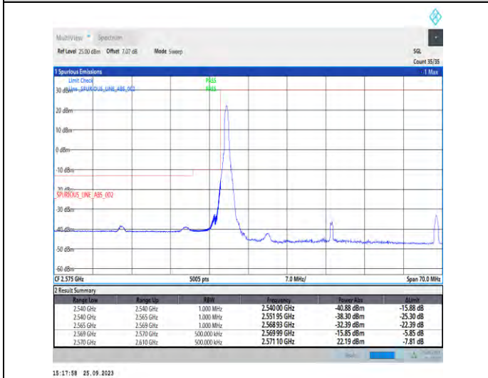
1-N38-PC3-30-40-L-4-CP-QPSK-Edge_1RB_Left-1@0-Ant5-1--PASS-see graph
