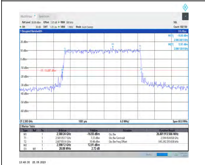
1-N38-PC3-30-30-M-4-DFT-64QAM-Outer_Full-75 @0-Ant5-26.802-28.080-<30-PASS
