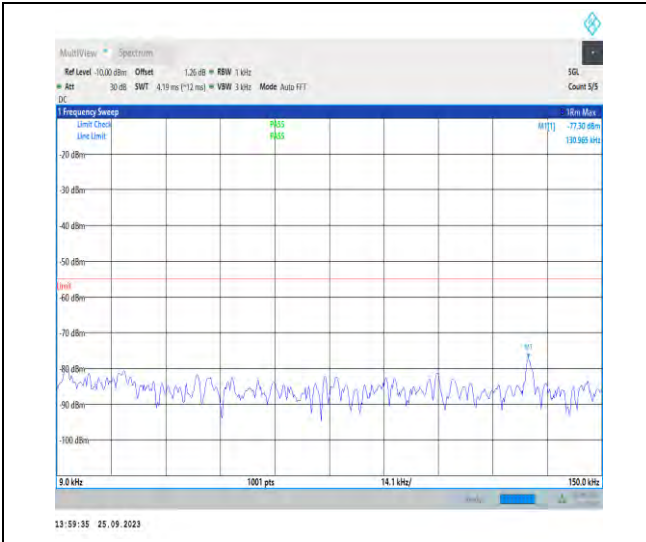
1-N38-PC3-30-40-H-1-DFT-PI2BPSK-Inner_1RB_L eft-1@1-0.009-0.15-Ant5-0.13--77.30--55-PASS
