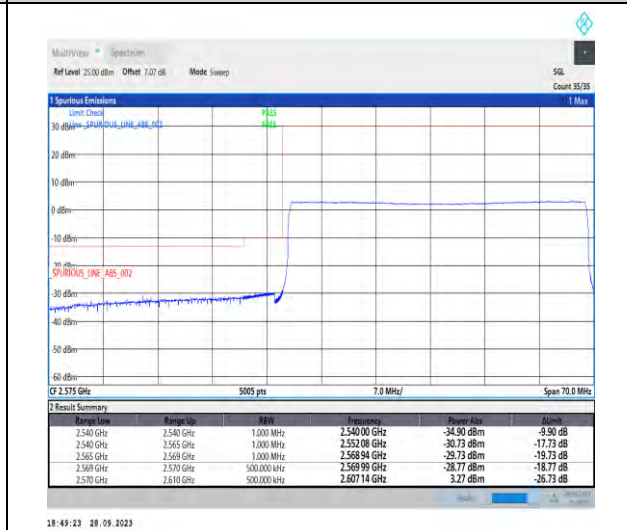
1-N38-PC3-30-40-L-6-CP-QPSK-Outer_Full-106@0-Ant5-1--PASS-see graph
