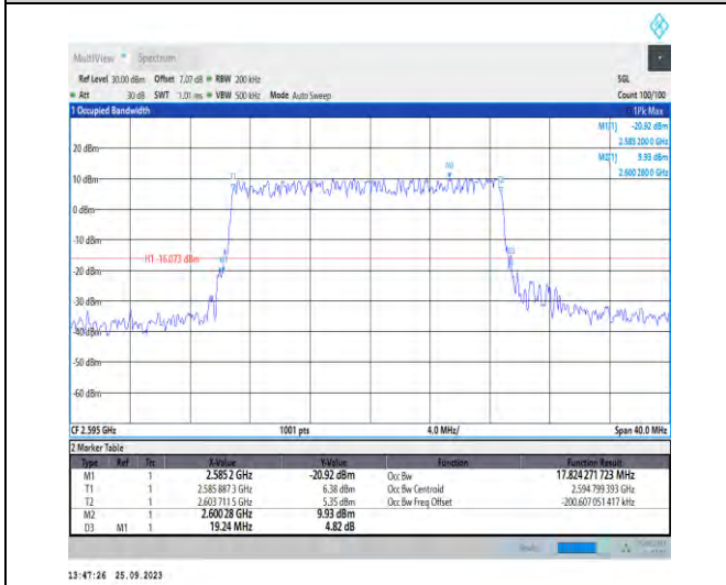
1-N38-PC3-30-20-M-5-DFT-256QAM-Outer_Full-50 @0-Ant5-17.824-19.240-≤20-PASS
