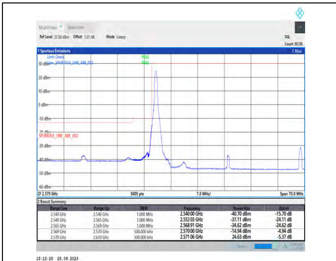
1-N38-PC3-30-40-L-1-DFT-PI2BPSK-Edge_1RB_Left-1@0-Ant5-1--PASS-see graph
