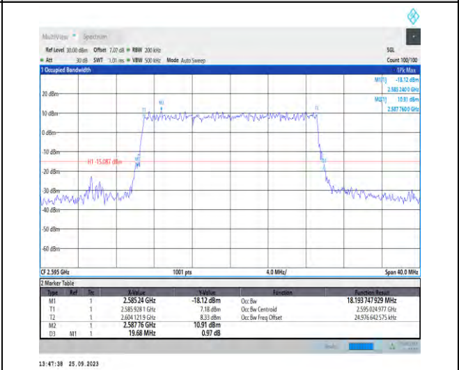
1-N38-PC3-30-20-M-6-CP-QPSK-Outer_Full-51@0- Ant5-18.194-19.680-≤20-PASS
