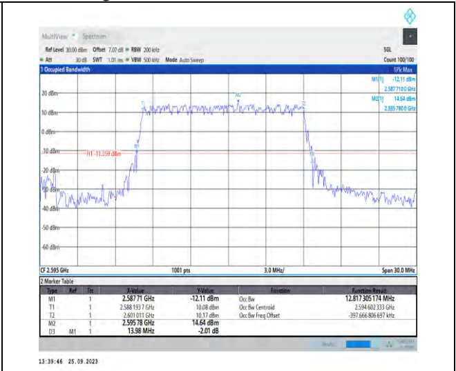
1-N38-PC3-30-15-M-1-DFT-QPSK-Outer_Full-36@ 0-Ant5-12.817-13.980-≤15-PASS
