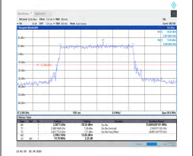
1-N38-PC3-30-15-M-7-CP-16QAM-Outer_Full-38@0-Ant5-13.605-14.790-≤15-PASS
