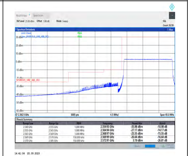
1-N38-PC3-30-15-L-6-CP-QPSK-Outer_Full-38@0-Ant5-1--PASS-see graph
