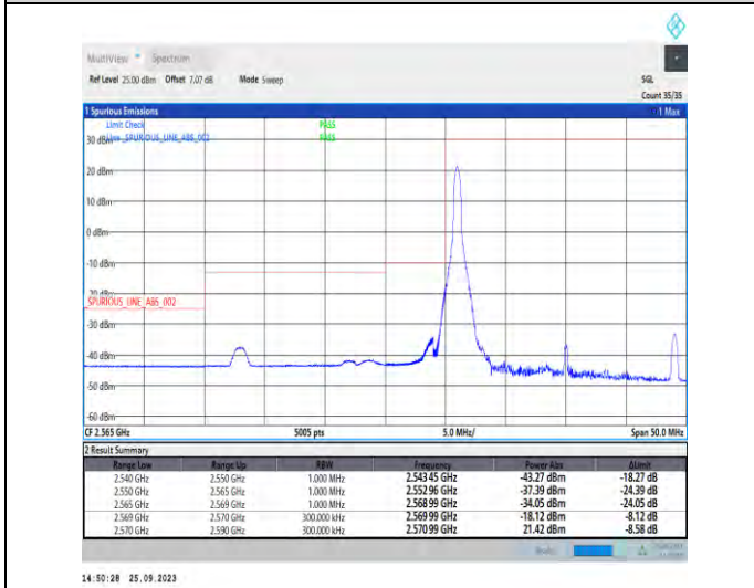
1-N38-PC3-30-20-L-4-CP-QPSK-Edge_1RB_Left-1@0-Ant5-1--PASS-see graph
