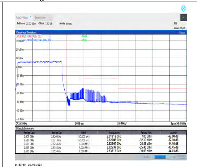
1-N38-PC3-30-15-H-3-DFT-PI2BPSK-Outer_Full-36@0-Ant5-1--PASS-see graph
