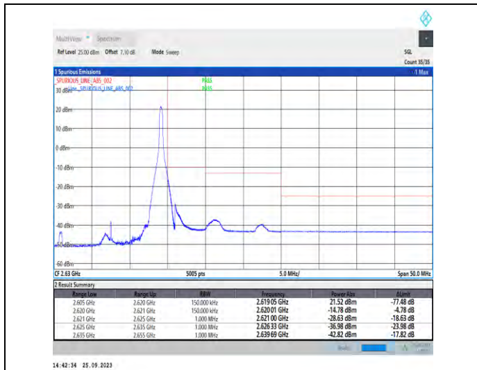
1-N38-PC3-30-15-H-2-DFT-PI2BPSK-Edge_1RB_Right-1@37-Ant5-1--PASS-see graph
