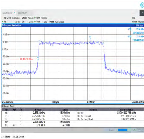
1-N38-PC3-30-40-M-5-DFT-256QAM-Outer_Full-100 @0-Ant5-35.704-37.600-≤40-PASS
