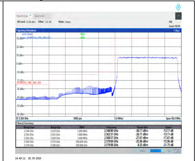
1-N38-PC3-30-20-L-3-DFT-PI2BPSK-Outer_Full-50@0-Ant5-1--PASS-see graph
