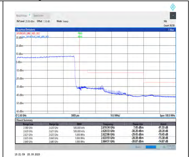
1-N38-PC3-30-40-H-3-DFT-PI2BPSK-Outer_Full-1 00@0-Ant5-1--PASS-see graph
