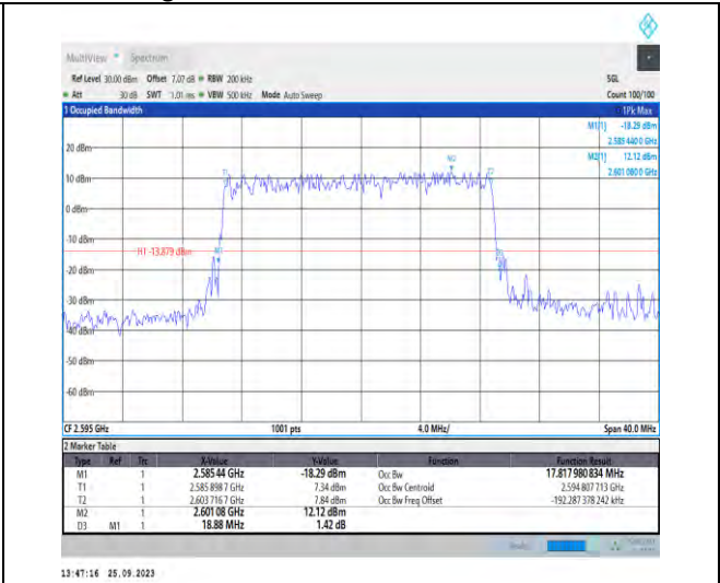
1-N38-PC3-30-20-M-4-DFT-64QAM-Outer_Full-50@ 0-Ant5-17.818-18.880-≤20-PASS
