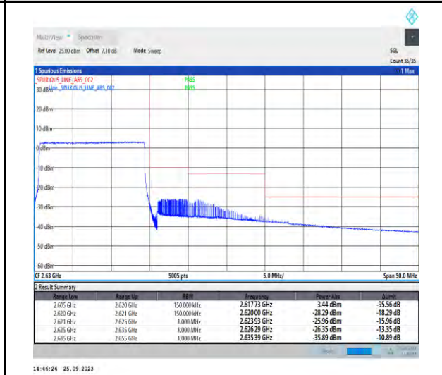
1-N38-PC3-30-15-H-6-CP-QPSK-Outer_Full-38@0-Ant5-1--PASS-see graph
