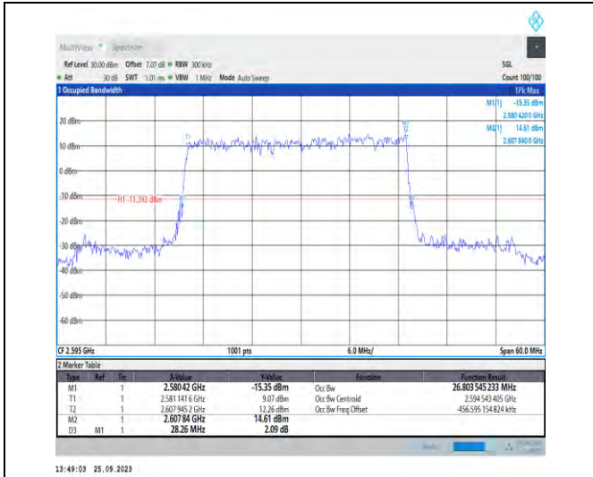
1-N38-PC3-30-30-M-2-DFT-PI2BPSK-Outer_Full-75 @0-Ant5-26.804-28.260-<30-PASS
