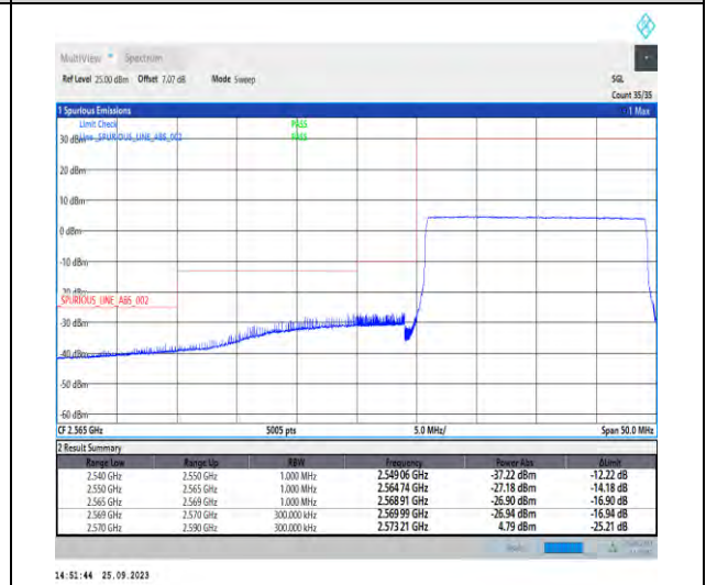
1-N38-PC3-30-20-L-6-CP-QPSK-Outer_Full-51@0-Ant5-1--PASS-see graph
