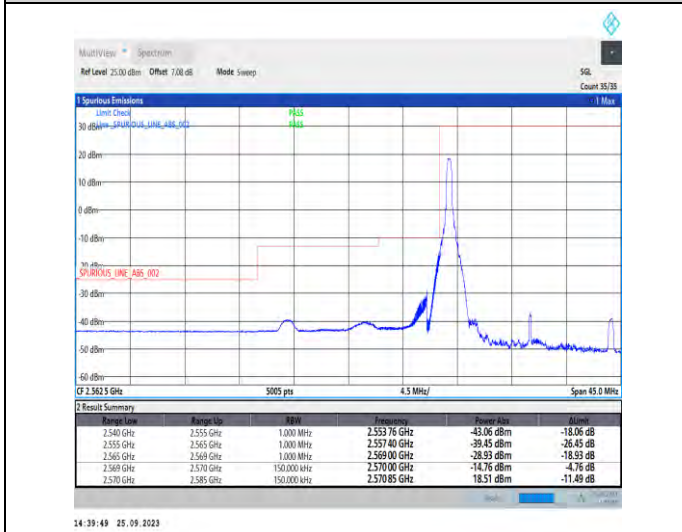
1-N38-PC3-30-15-L-4-CP-QPSK-Edge_1RB_Left-1@0-Ant5-1--PASS-see graph
