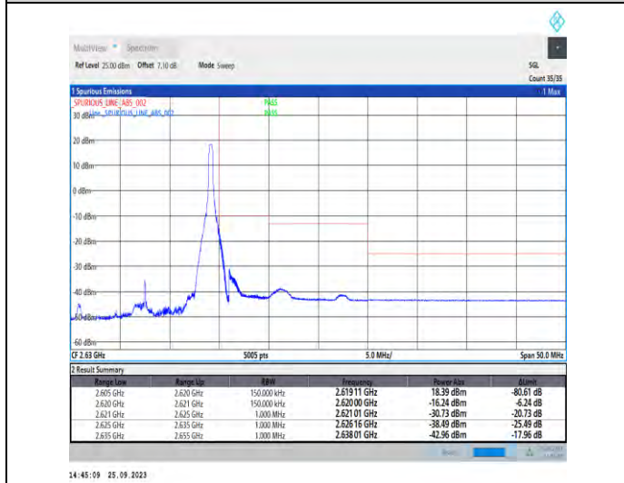
1-N38-PC3-30-15-H-5-CP-QPSK-Edge_1RB_Right-1@37-Ant5-1--PASS-see graph
