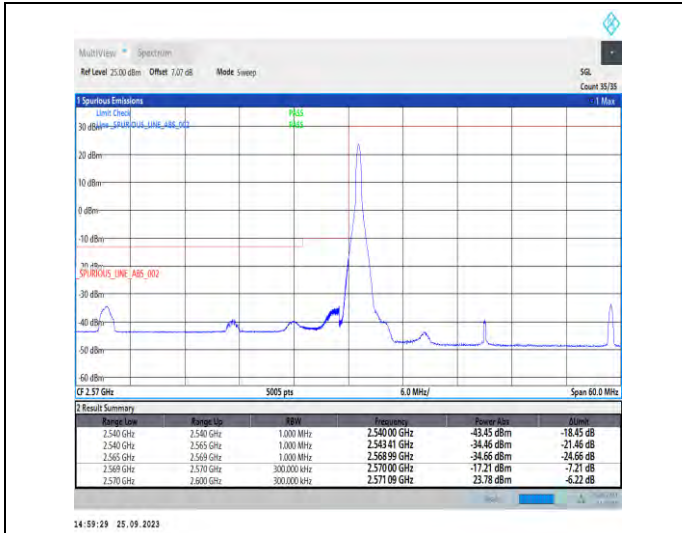
1-N38-PC3-30-30-L-1-DFT-PI2BPSK-Edge_1RB_Left-1@0-Ant5-1--PASS-see graph
