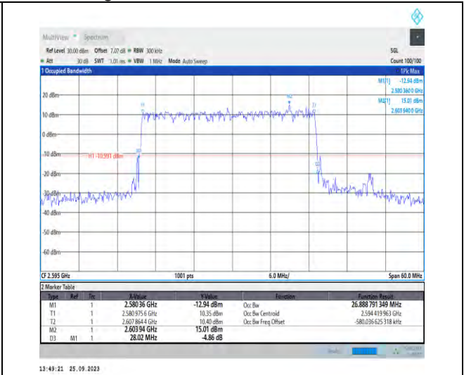
1-N38-PC3-30-30-M-3-DFT-16QAM-Outer_Full-75 @0-Ant5-26.889-28.020-<30-PASS
