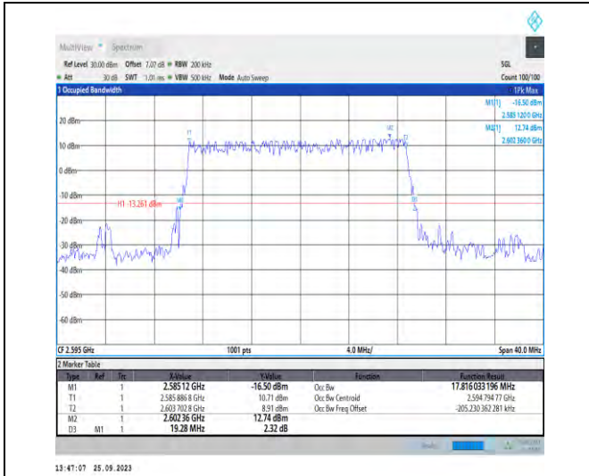
1-N38-PC3-30-20-M-3-DFT-16QAM-Outer_Full-50@ 0-Ant5-17.816-19.280-≤20-PASS
