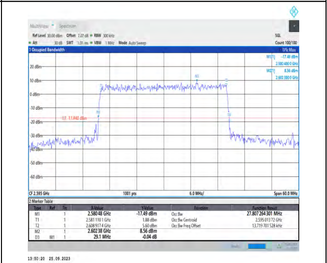
1-N38-PC3-30-30-M-9-CP-256QAM-Outer_Full-78@0-Ant5-27.807-29.100-≤30-PASS
