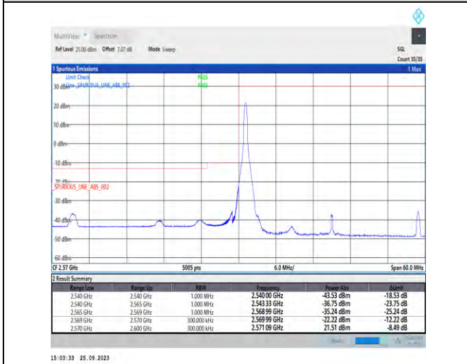
1-N38-PC3-30-30-L-4-CP-QPSK-Edge_1RB_Left-1@0-Ant5-1--PASS-see graph
