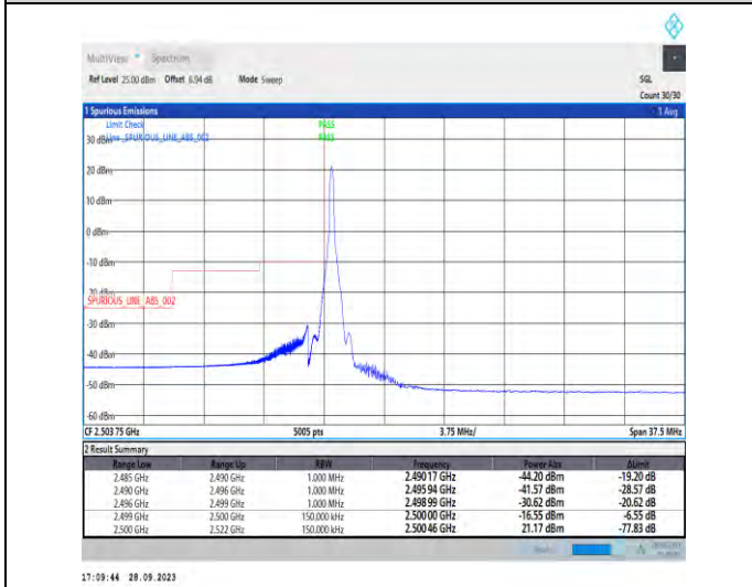
1-N7-PC3-15-15-L-4-CP-QPSK-Edge_1RB_Left-1@0-Ant5-1--PASS-see graph
