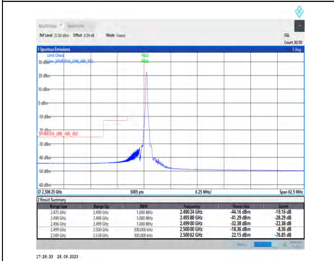
1-N7-PC3-15-25-L-4-CP-QPSK-Edge_1RB_Left-1@0-Ant5-1--PASS-see graph
