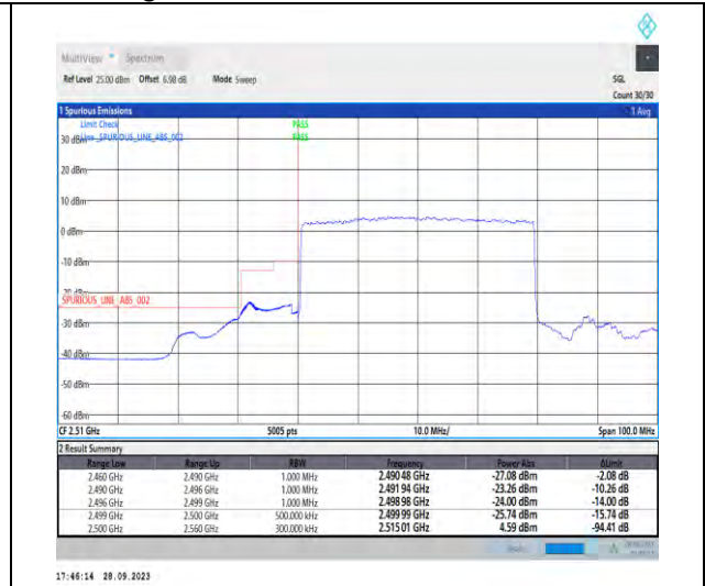
1-N7-PC3-15-40-L-3-DFT-PI2BPSK-Outer_Full-21 6@0-Ant5-1--PASS-see graph
