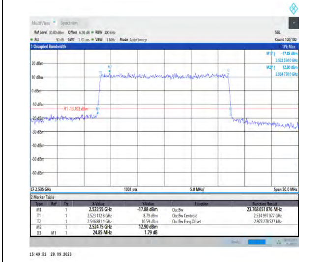
1-N7-PC3-15-25-M-7-CP-16QAM-Outer_Full-133@0 -Ant5-23.769-24.850-≤25-PASS
