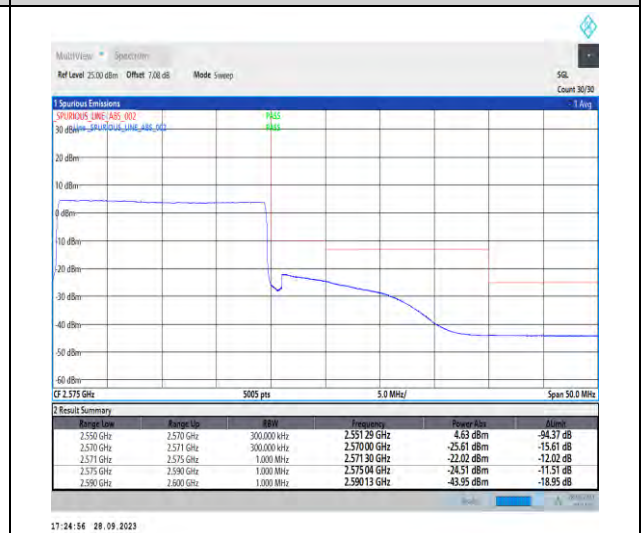
1-N7-PC3-15-20-H-6-CP-QPSK-Outer_Full-106@0-Ant5-1--PASS-see graph
