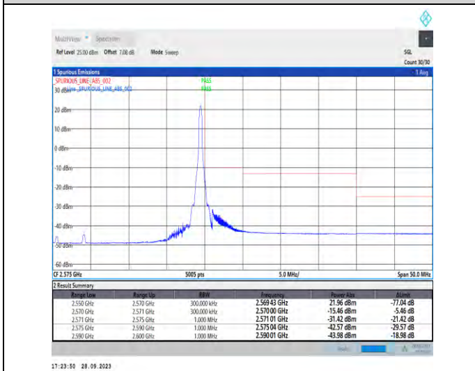
1-N7-PC3-15-20-H-5-CP-QPSK-Edge_1RB_Right-1@105-Ant5-1--PASS-see graph
