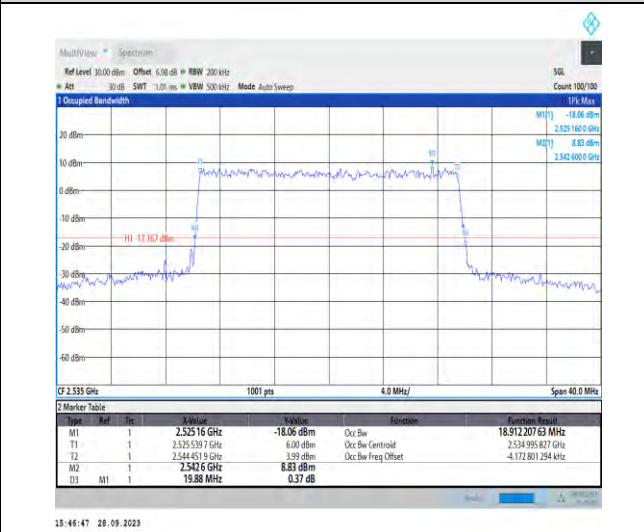
1-N7-PC3-15-20-M-9-CP-256QAM-Outer_Full-106@0-Ant5-18.912-19.880-<=20-PASS
