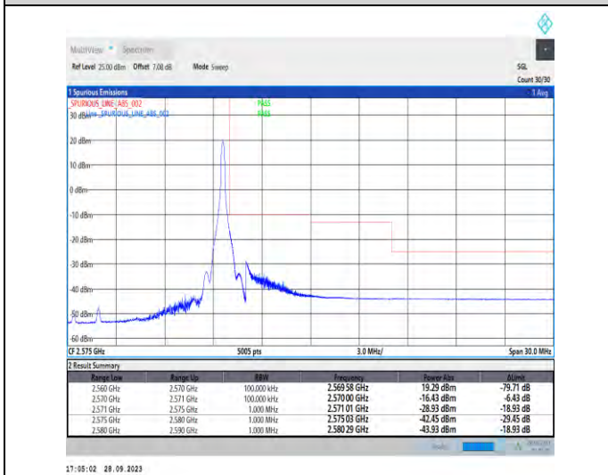
1-N7-PC3-15-10-H-5-CP-QPSK-Edge_1RB_Right-1@51-Ant5-1--PASS-see graph
