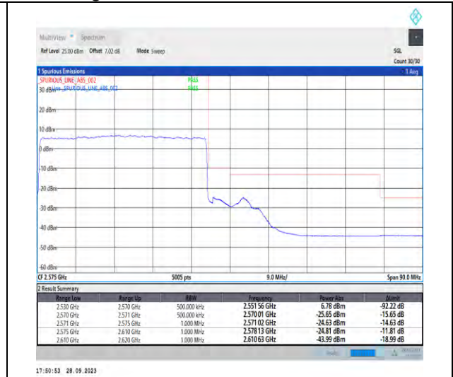
1-N7-PC3-15-40-H-3-DFT-PI2BPSK-Outer_Full-216@0-Ant5-1--PASS-see graph
