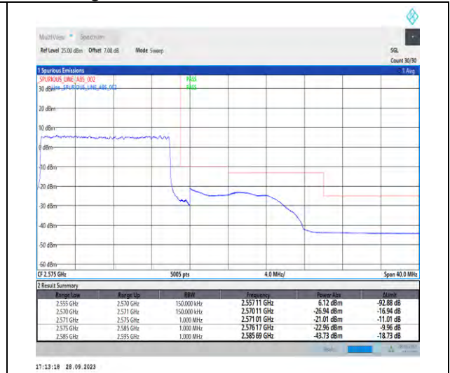
1-N7-PC3-15-15-H-3-DFT-PI2BPSK-Outer_Full-75@0-Ant5-1--PASS-see graph
