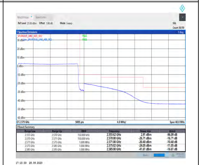
1-N7-PC3-15-15-H-6-CP-QPSK-Outer_Full-79@0-Ant5-1--PASS-see graph
