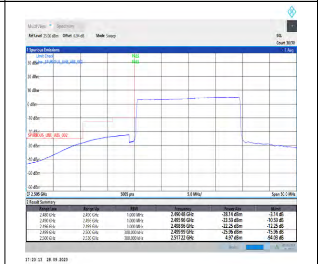
1-N7-PC3-15-20-L-6-CP-QPSK-Outer_Full-106@0-Ant5-1--PASS-see graph
