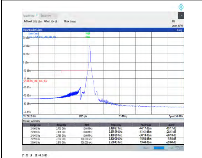
1-N7-PC3-15-10-L-4-CP-QPSK-Edge_1RB_Left-1@0-Ant5-1--PASS-see graph
