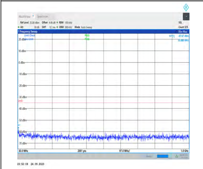
1-N7-PC3-15-40-H-1-DFT-PI2BPSK-Inner_1RB_Lef t-1@1-30-1000-Ant5-33.88--57.67--35-PASS
