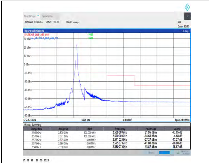
1-N7-PC3-15-10-H-2-DFT-PI2BPSK-Edge_1RB_Right-1@51-Ant5-1--PASS-see graph
