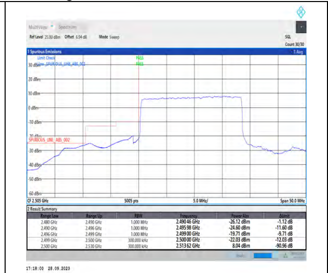
1-N7-PC3-15-20-L-3-DFT-PI2BPSK-Outer_Full-10@0-Ant5-1--PASS-see graph
