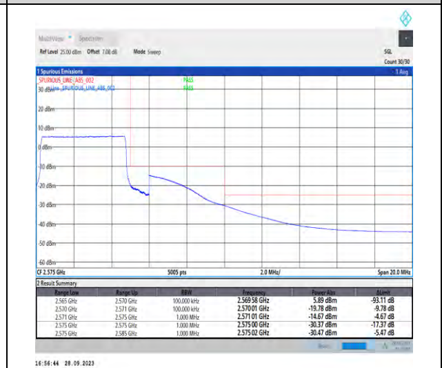
1-N7-PC3-15-5-H-6-CP-QPSK-Outer_Full-25@0-Ant5-1--PASS-see graph
