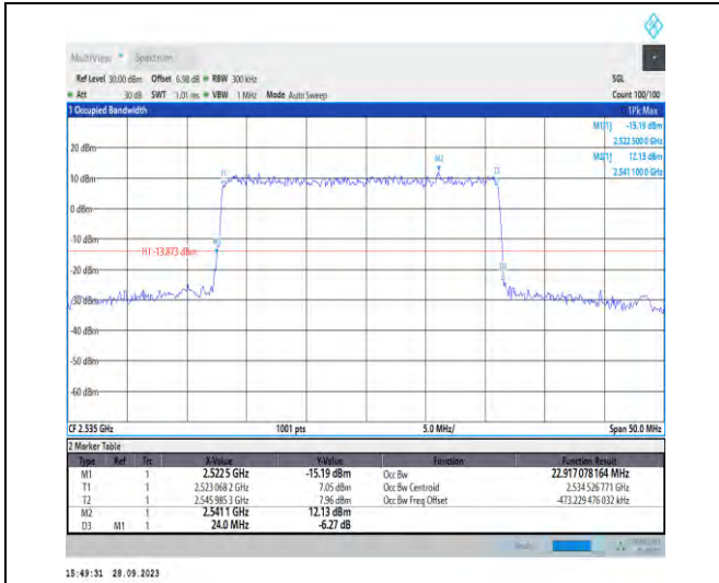
1-N7-PC3-15-25-M-5-DFT-256QAM-Outer_Full-128 @0-Ant5-22.917-24.000-≤25-PASS
