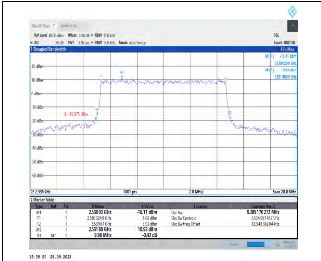
1-N7-PC3-15-10-M-8-CP-64QAM-Outer_Full-52@0-Ant5-9.285-9.980-≤10-PASS
