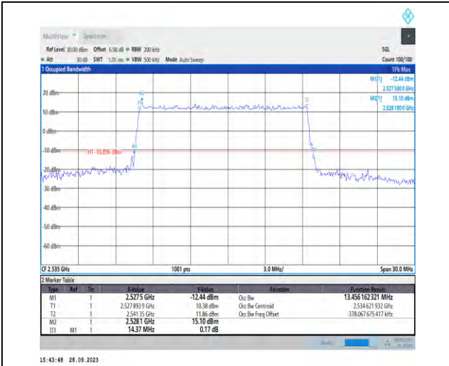
1-N7-PC3-15-15-M-3-DFT-16QAM-Outer_Full-75@0 -Ant5-13.456-14.370-≤15-PASS
