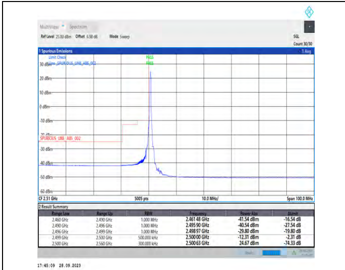
1-N7-PC3-15-40-L-1-DFT-PI2BPSK-Edge_1RB_Left-1 @0-Ant5-1--PASS-see graph
