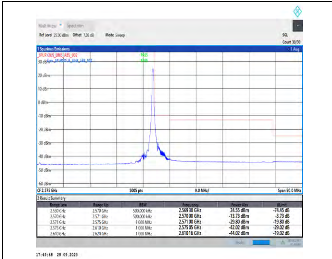
1-N7-PC3-15-40-H-2-DFT-PI2BPSK-Edge_1RB_Right-1@215-Ant5-1--PASS-see graph
