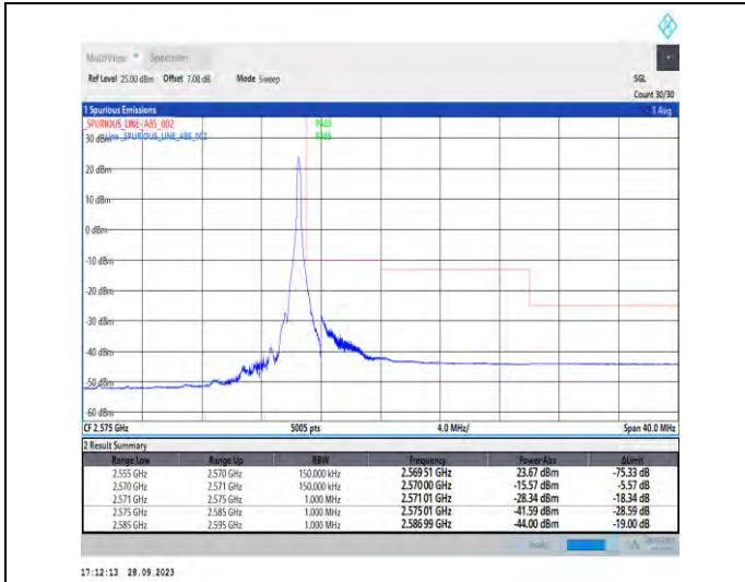
1-N7-PC3-15-15-H-2-DFT-PI2BPSK-Edge_1RB_Right-1@78-Ant5-1--PASS-see graph
