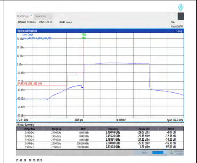
1-N7-PC3-15-40-L-6-CP-QPSK-Outer_Full-216@0-Ant5-1--PASS-see graph
