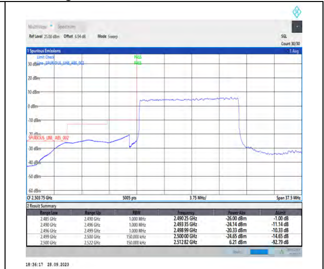
1-N7-PC3-15-15-L-3-DFT-PI2BPSK-Outer_Full-75 @0-Ant5-1--PASS-see graph
