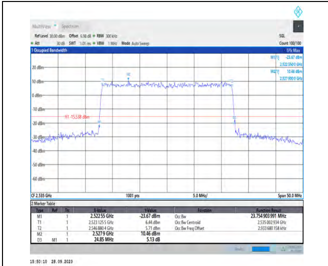
1-N7-PC3-15-25-M-9-CP-256QAM-Outer_Full-133@ 0-Ant5-23.755-24.850-≤25-PASS
