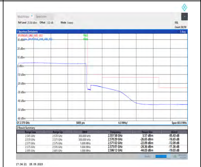
1-N7-PC3-15-25-H-6-CP-QPSK-Outer_Full-133@0-Ant5-1--PASS-see graph
