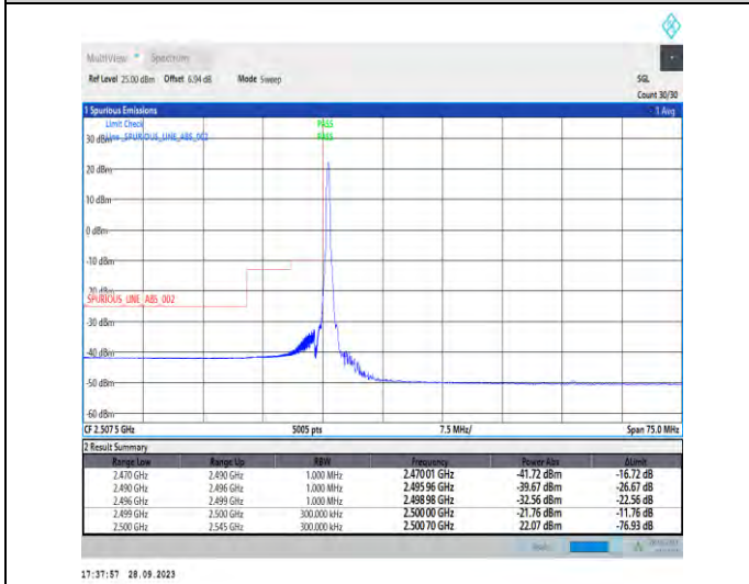
1-N7-PC3-15-30-L-4-CP-QPSK-Edge_1RB_Left-1@0-Ant5-1--PASS-see graph
