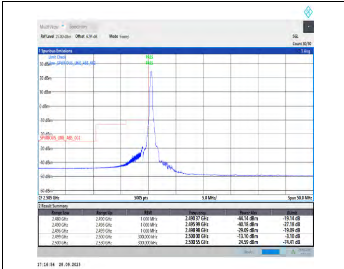
1-N7-PC3-15-20-L-1-DFT-PI2BPSK-Edge_1RB_Left-1@0-Ant5-1--PASS-see graph
