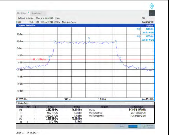
1-N7-PC3-15-5-M-8-CP-64QAM-Outer_Full-25@0-Ant5-4.48-5.120-≤5-PASS
