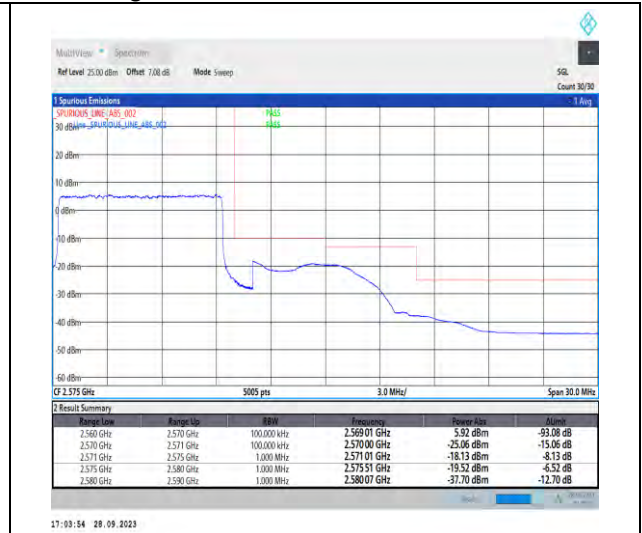
1-N7-PC3-15-10-H-3-DFT-PI2BPSK-Outer_Full-50@0-Ant5-1--PASS-see graph
