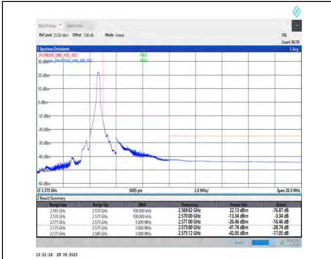
1-N7-PC3-15-5-H-2-DFT-PI2BPSK-Edge_1RB_Right-1 @24-Ant5-1--PASS-see graph
