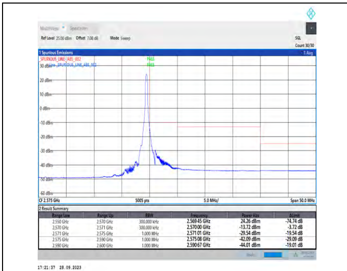
1-N7-PC3-15-20-H-2-DFT-PI2BPSK-Edge_1RB_Right-1@105-Ant5-1--PASS-see graph
