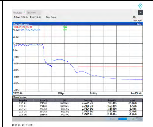
1-N7-PC3-15-5-H-3-DFT-PI2BPSK-Outer_Full-25 @0-Ant5-1--PASS-see graph
