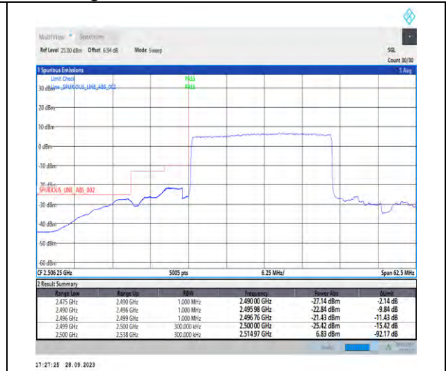
1-N7-PC3-15-25-L-3-DFT-PI2BPSK-Outer_Full-12 8@0-Ant5-1--PASS-see graph
