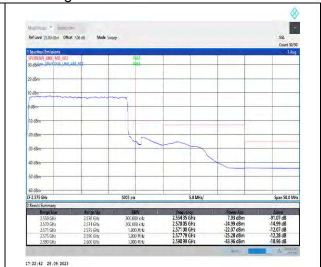
1-N7-PC3-15-20-H-3-DFT-PI2BPSK-Outer_Full-100@0-Ant5-1--PASS-see graph
