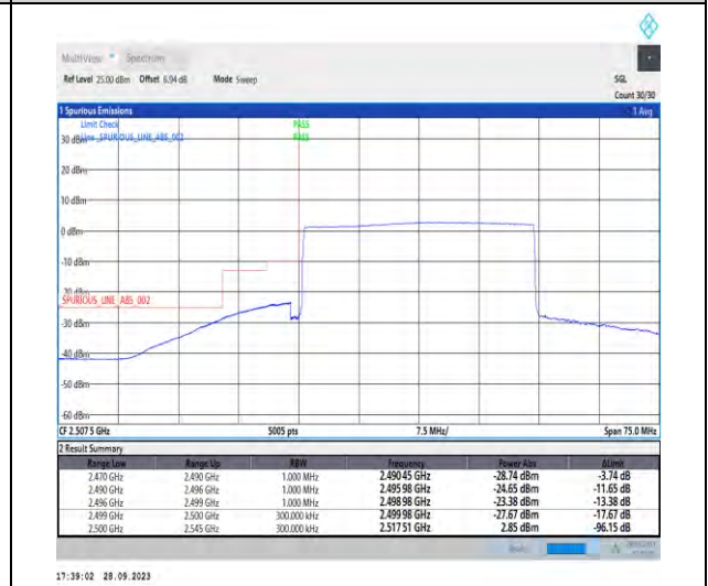
1-N7-PC3-15-30-L-6-CP-QPSK-Outer_Full-160@0-Ant5-1--PASS-see graph
