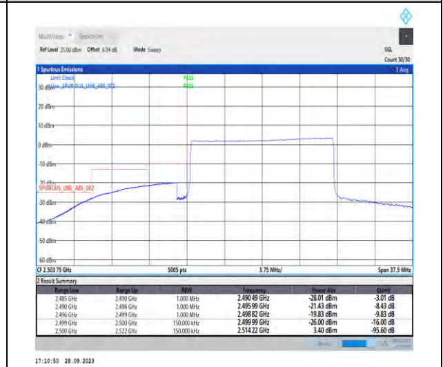
1-N7-PC3-15-15-L-6-CP-QPSK-Outer_Full-79@0-Ant5-1--PASS-see graph
