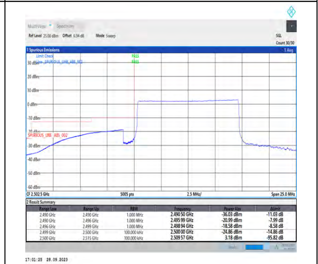
1-N7-PC3-15-10-L-6-CP-QPSK-Outer_Full-52@0-Ant5-1--PASS-see graph
