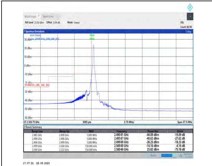
1-N7-PC3-15-15-L-1-DFT-PI2BPSK-Edge_1RB_Left-1 @0-Ant5-1--PASS-see graph
