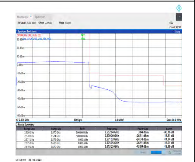
1-N7-PC3-15-40-H-6-CP-QPSK-Outer_Full-216@0-Ant5-1--PASS-see graph
