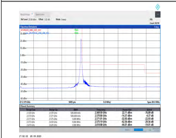
1-N7-PC3-15-40-H-5-CP-QPSK-Edge_1RB_Right-1@215-Ant5-1--PASS-see graph
