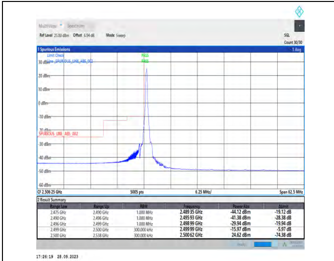
1-N7-PC3-15-25-L-1-DFT-PI2BPSK-Edge_1RB_Left-1 @0-Ant5-1--PASS-see graph
