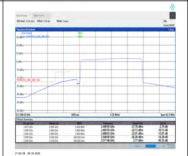
1-N7-PC3-15-25-L-6-CP-QPSK-Outer_Full-133@0-Ant5-1--PASS-see graph
