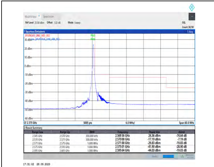
1-N7-PC3-15-25-H-2-DFT-PI2BPSK-Edge_1RB_Right-1@132-Ant5-1--PASS-see graph
