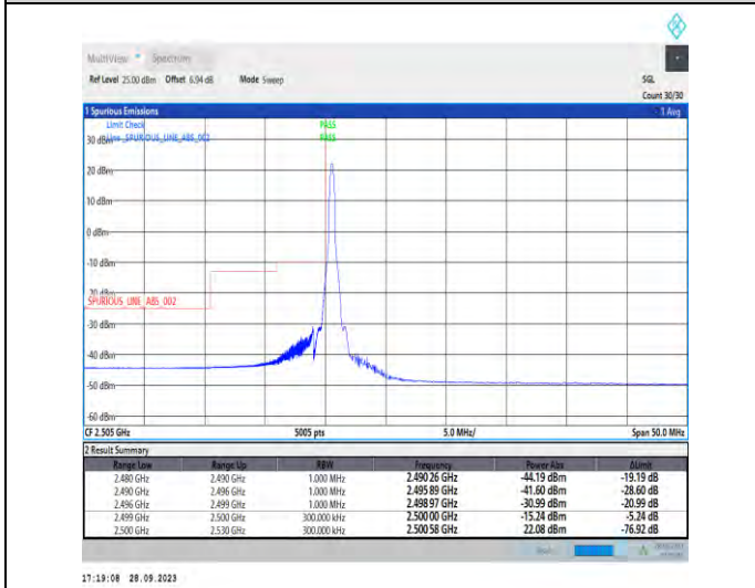
1-N7-PC3-15-20-L-4-CP-QPSK-Edge_1RB_Left-1@0-Ant5-1--PASS-see graph
