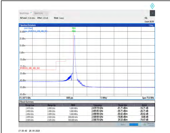
1-N7-PC3-15-30-L-1-DFT-PI2BPSK-Edge_1RB_Left-1 @0-Ant5-1--PASS-see graph
