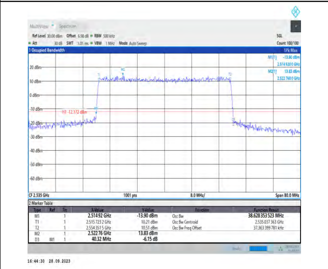
1-N7-PC3-15-40-M-6-CP-QPSK-Outer_Full-216@0- Ant5-38.628-40.320-≤40-PASS
