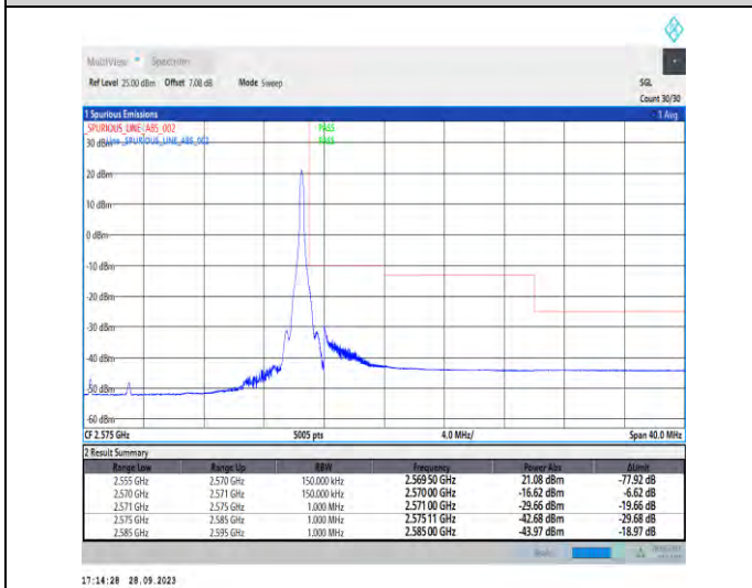
1-N7-PC3-15-15-H-5-CP-QPSK-Edge_1RB_Right-1@78-Ant5-1--PASS-see graph
