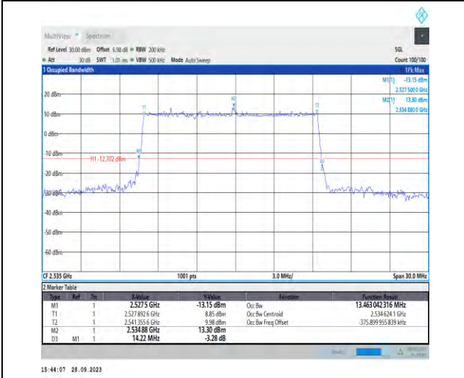
1-N7-PC3-15-15-M-5-DFT-256QAM-Outer_Full-75@0 0-Ant5-13.463-14.220-≤15-PASS
