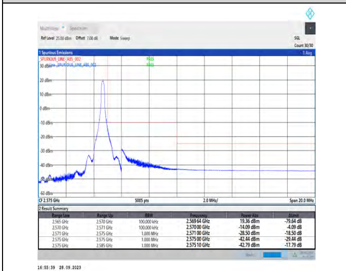
1-N7-PC3-15-5-H-5-CP-QPSK-Edge_1RB_Right-1@2 4-Ant5-1--PASS-see graph
