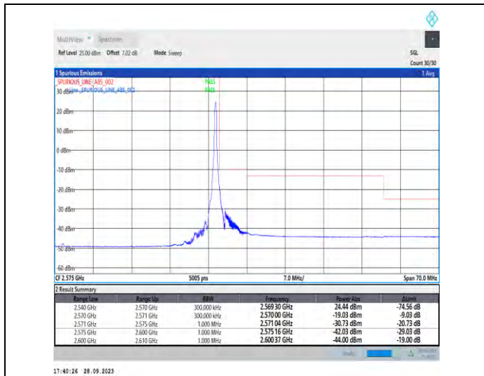
1-N7-PC3-15-30-H-2-DFT-PI2BPSK-Edge_1RB_Right-1@159-Ant5-1--PASS-see graph
