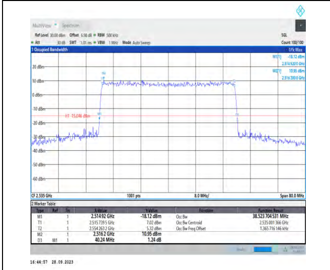
1-N7-PC3-15-40-M-9-CP-256QAM-Outer_Full-216@0 0-Ant5-38.524-40.240-≤40-PASS
