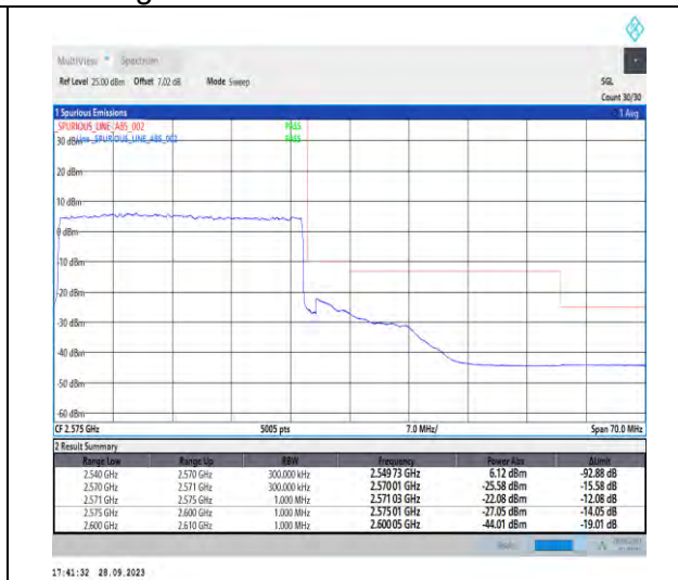
1-N7-PC3-15-30-H-3-DFT-PI2BPSK-Outer_Full-160@0-Ant5-1--PASS-see graph
