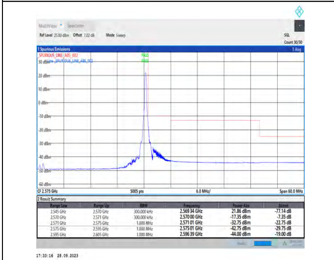
1-N7-PC3-15-25-H-5-CP-QPSK-Edge_1RB_Right-1@132-Ant5-1--PASS-see graph
