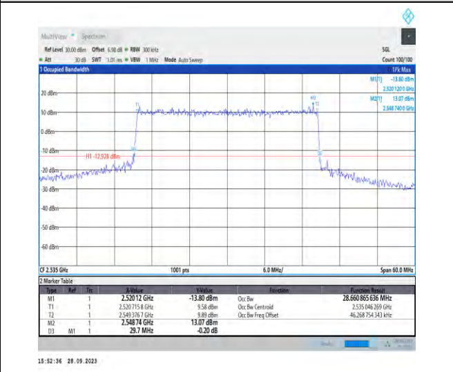
1-N7-PC3-15-30-M-7-CP-16QAM-Outer_Full-160@0- -Ant5-28.661-29.700-≤30-PASS
