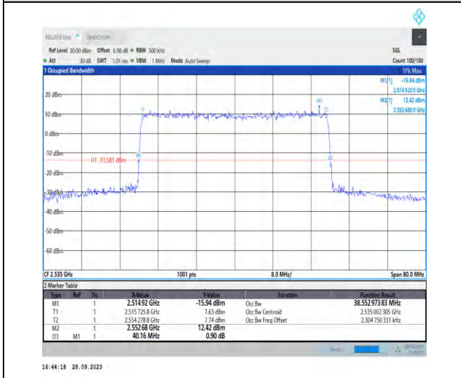
1-N7-PC3-15-40-M-5-DFT-256QAM-Outer_Full-216 @0-Ant5-38.553-40.160-≤40-PASS
