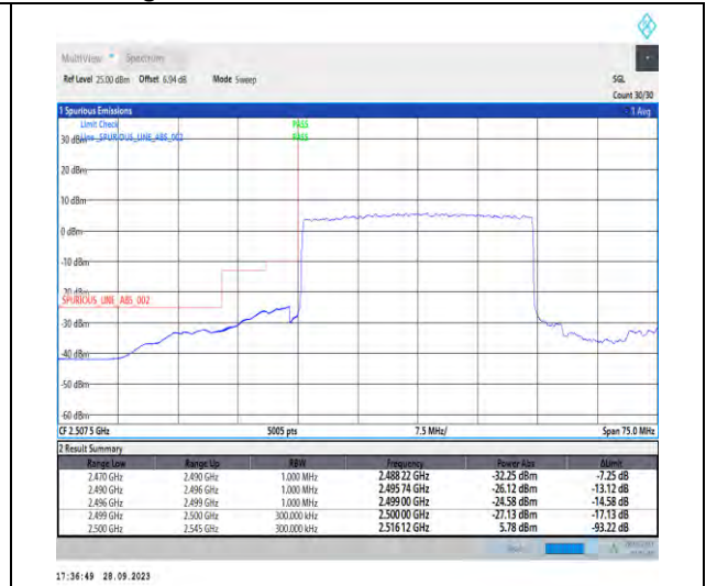
1-N7-PC3-15-30-L-3-DFT-PI2BPSK-Outer_Full-16 0@0-Ant5-1--PASS-see graph
