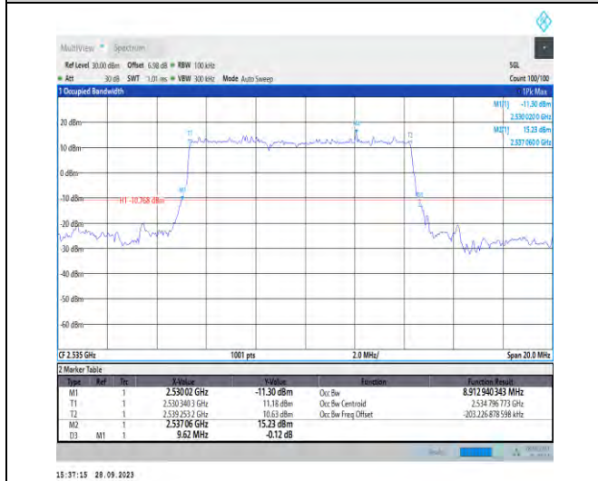
1-N7-PC3-15-10-M-2-DFT-PI2BPSK-Outer_Full-50@0-Ant5-8.913-9.620-≤10-PASS
