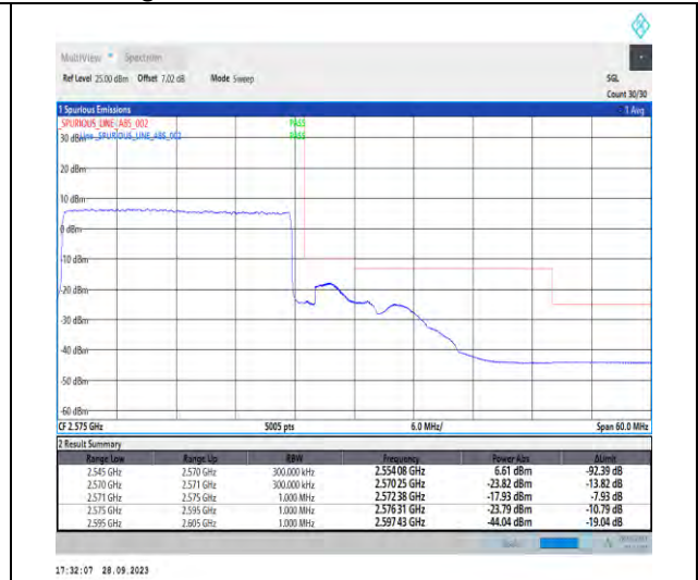
1-N7-PC3-15-25-H-3-DFT-PI2BPSK-Outer_Full-128@0-Ant5-1--PASS-see graph
