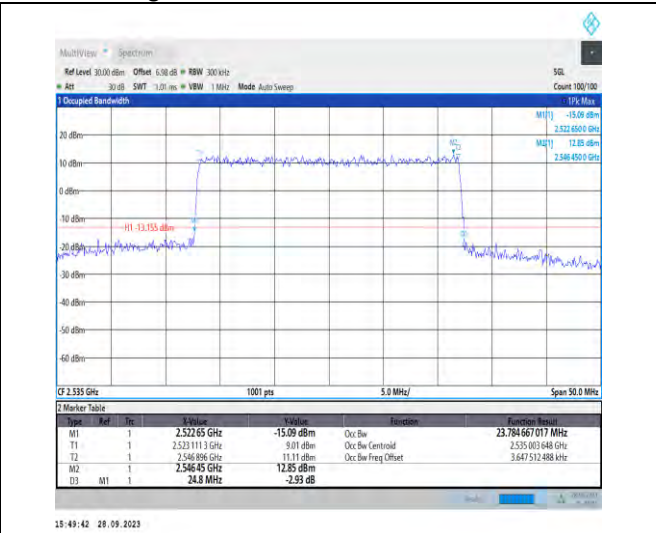
1-N7-PC3-15-25-M-6-CP-QPSK-Outer_Full-133@0-Ant5-23.785-24.800-≤25-PASS
