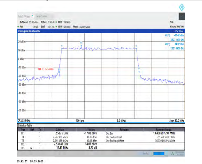
1-N7-PC3-15-15-M-4-DFT-64QAM-Outer_Full-75@0 -Ant5-13.408-14.310-≤15-PASS
