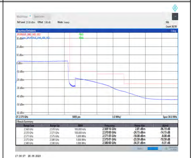
1-N7-PC3-15-10-H-6-CP-QPSK-Outer_Full-52@0-Ant5-1--PASS-see graph
