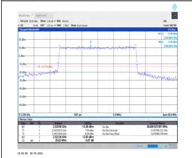
1-N7-PC3-15-30-M-6-CP-QPSK-Outer_Full-160@0- Ant5-28.607-29.820-≤30-PASS
