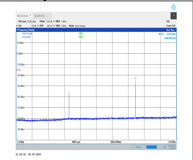
1-N5-PC3-15-20-H-1-DFT-PI2BPSK-Inner_1RB_Left -1@1-1000-3000-Ant1-2489.00--26.29--13-PASS
