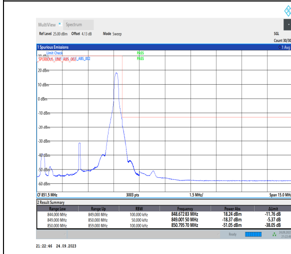
1-N5-PC3-15-5-H-5-CP-QPSK-Edge_1RB_Right-1@2 4-Ant1-1--PASS-see graph
