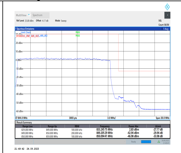
1-N5-PC3-15-20-H-3-DFT-PI2BPSK-Outer_Full-100@0-Ant1-1--PASS-see graph
