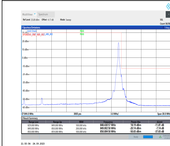
1-N5-PC3-15-20-H-5-CP-QPSK-Edge_1RB_Right-1@105-Ant1-1--PASS-see graph
