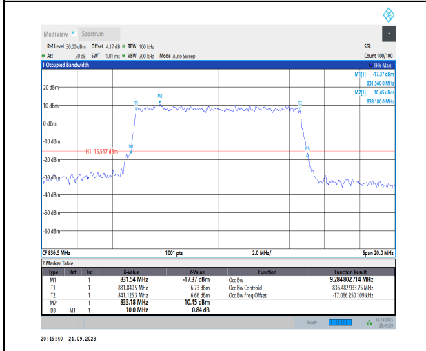
1-N5-PC3-15-10-M-6-CP-QPSK-Outer_Full-52@0-A nt1-9.285-10.000-≤10-PASS
