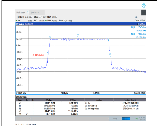
1-N5-PC3-15-15-M-5-DFT-256QAM-Outer_Full-75@0 -Ant1-13.453-14.310-≤15-PASS
