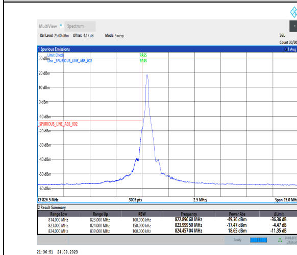
1-N5-PC3-15-15-L-4-CP-QPSK-Edge_1RB_Left-1@0- Ant1-1--PASS-see graph
