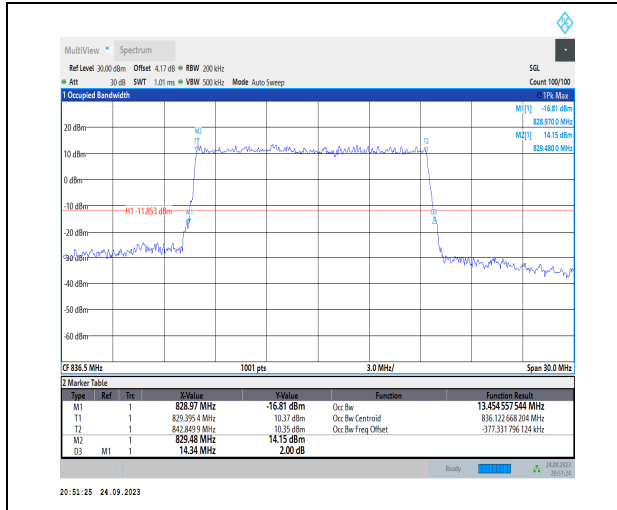
1-N5-PC3-15-15-M-3-DFT-16QAM-Outer_Full-75@0 -Ant1-13.455-14.340-≤15-PASS
