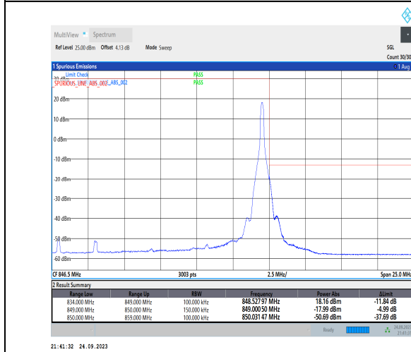
1-N5-PC3-15-15-H-5-CP-QPSK-Edge_1RB_Right-1@78-Ant1-1--PASS-see graph
