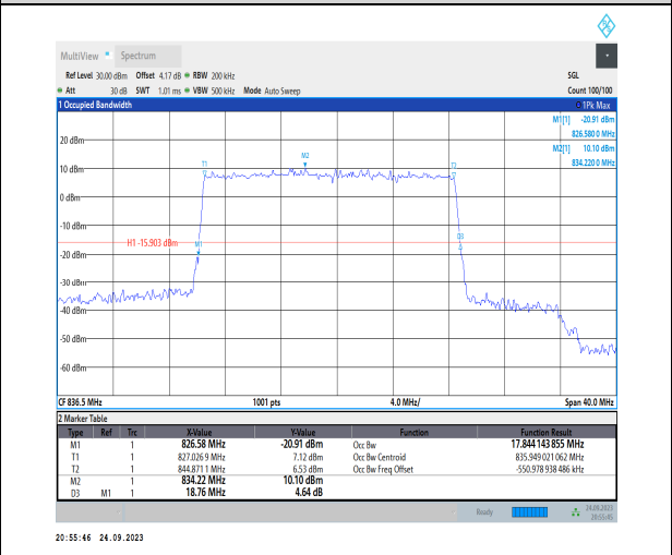
1-N5-PC3-15-20-M-5-DFT-256QAM-Outer_Full-100 @0-Ant1-17.844-18.760-≤20-PASS
