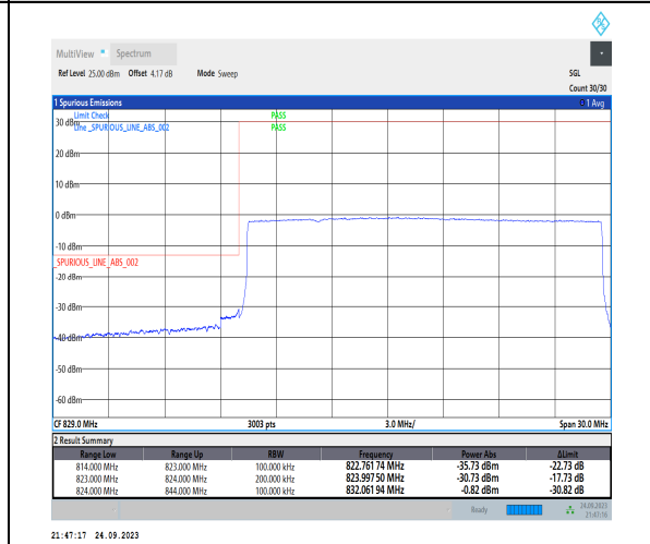
1-N5-PC3-15-20-L-6-CP-QPSK-Outer_Full-106@ 0-Ant1-1--PASS-see graph
