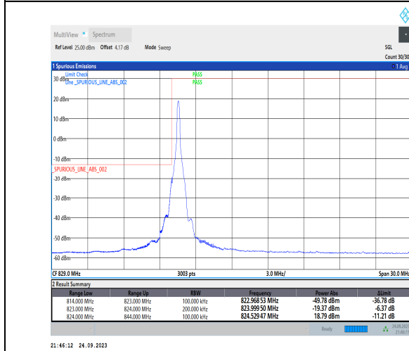
1-N5-PC3-15-20-L-4-CP-QPSK-Edge_1RB_Left-1@0- Ant1-1--PASS-see graph
