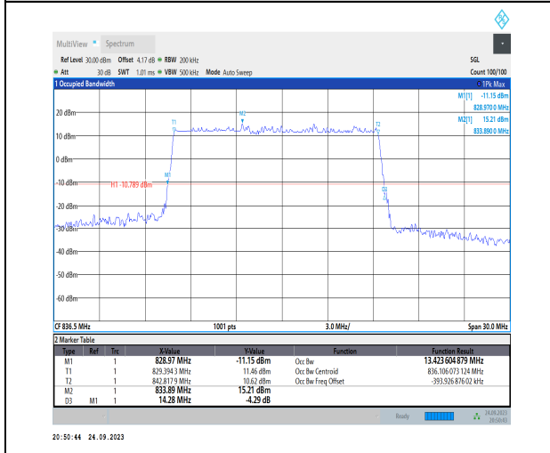
1-N5-PC3-15-15-M-1-DFT-QPSK-Outer_Full-75@0-Ant1-13.424-14.280-≤15-PASS
