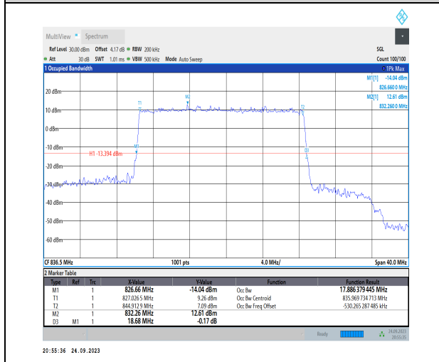
1-N5-PC3-15-20-M-4-DFT-64QAM-Outer_Full-100@ 0-Ant1-17.886-18.680-≤20-PASS
