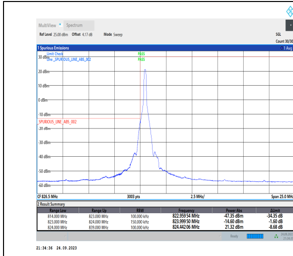
1-N5-PC3-15-15-L-1-DFT-PI2BPSK-Edge_1RB_Left-1 @0-Ant1-1--PASS-see graph
