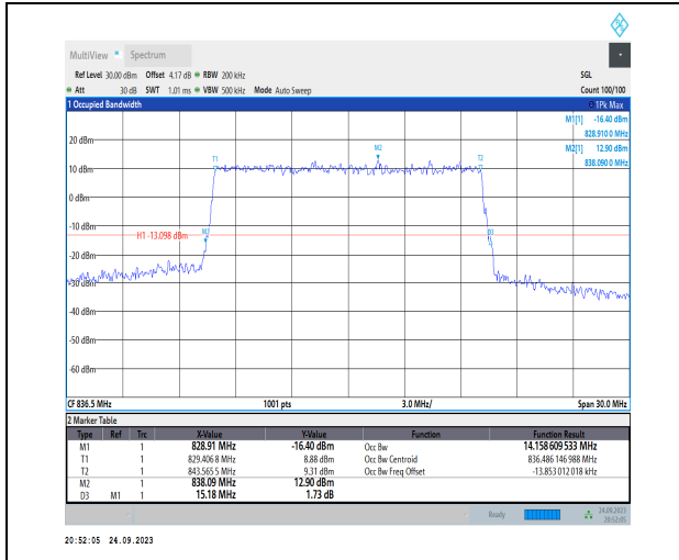
1-N5-PC3-15-15-M-7-CP-16QAM-Outer_Full-79@0-Ant1-14.159-15.180-≤15-PASS
