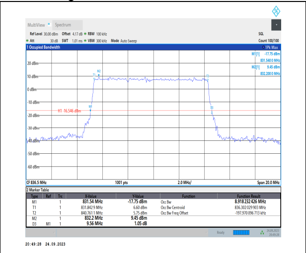
1-N5-PC3-15-10-M-5-DFT-256QAM-Outer_Full-50@0-Ant1-8.918-9.560-≤10-PASS
