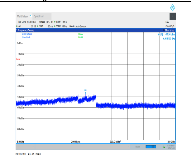
1-N5-PC3-15-20-M-1-DFT-PI2BPSK-Inner_1RB_Left -1@1-3000-12000-Ant1-6914.10--47.54--13-PASS
