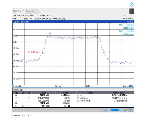
1-N5-PC3-15-5-M-8-CP-64QAM-Outer_Full-25@0-A nt1-4.478-5.010-<math>\leq 5</math>-PASS
