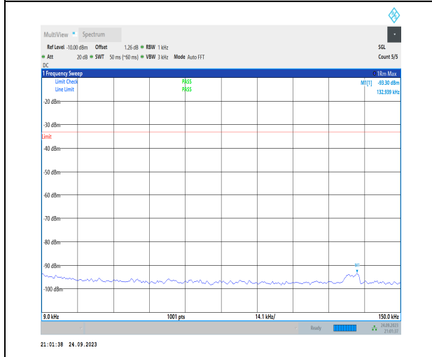
1-N5-PC3-15-20-H-1-DFT-PI2BPSK-Inner_1RB_Left -1@1-0.009-0.15-Ant1-0.13--93.30--33-PASS
