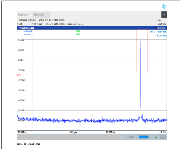
1-N5-PC3-15-20-H-1-DFT-PI2BPSK-Inner_1RB_Left -1@1-30-1000-Ant1-34.85--54.90--13-PASS
