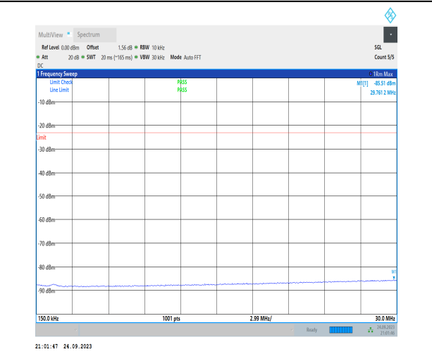
1-N5-PC3-15-20-H-1-DFT-PI2BPSK-Inner_1RB_Left -1@1-0.15-30-Ant1-29.76--85.51--23-PASS
