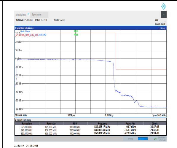
1-N5-PC3-15-20-H-6-CP-QPSK-Outer_Full-106@0-Ant1-1--PASS-see graph
