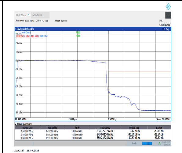
1-N5-PC3-15-15-H-6-CP-QPSK-Outer_Full-79@0-Ant1-1--PASS-see graph
