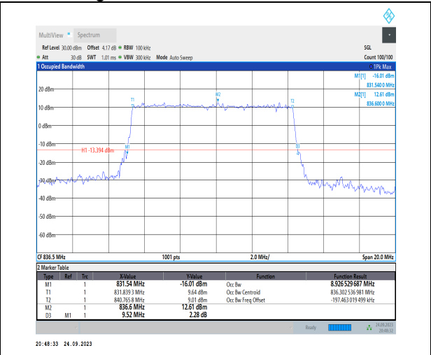
1-N5-PC3-15-10-M-1-DFT-QPSK-Outer_Full-50@0-Ant1-8.927-9.520-≤10-PASS
