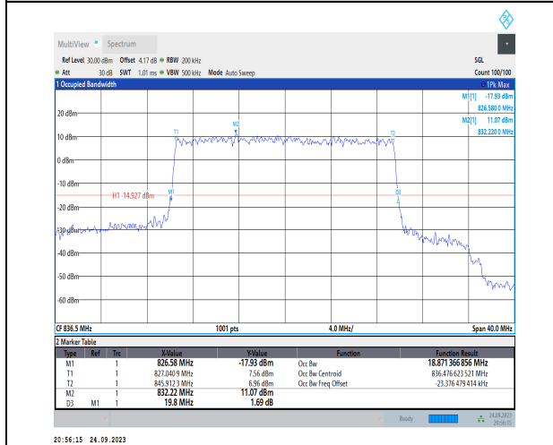
1-N5-PC3-15-20-M-8-CP-64QAM-Outer_Full-106@0-Ant1-18.871-19.800-≤20-PASS
