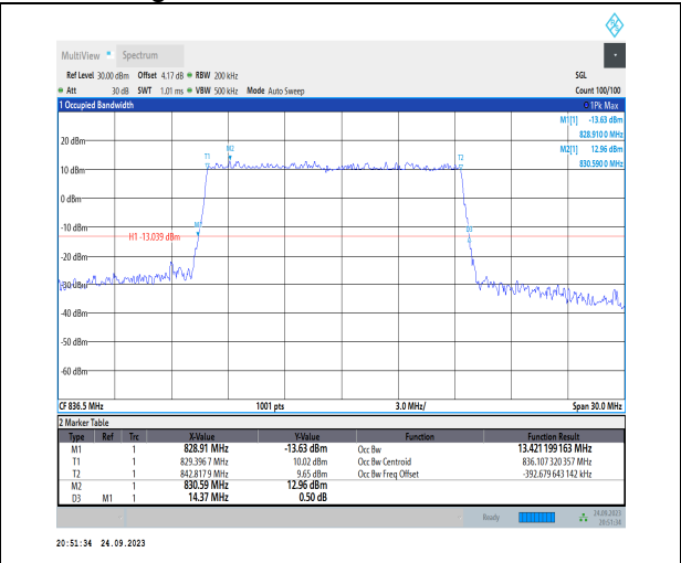
1-N5-PC3-15-15-M-4-DFT-64QAM-Outer_Full-75@0 -Ant1-13.421-14.370-≤15-PASS
