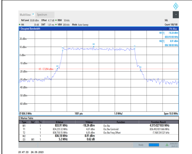
1-N5-PC3-15-5-M-7-CP-16QAM-Outer_Full-25@0-A nt1-4.515-5.200-<math>\leq 5</math>-PASS
