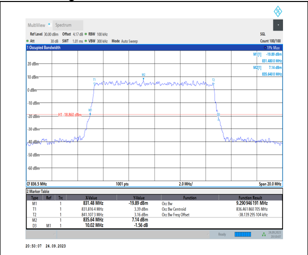
1-N5-PC3-15-10-M-9-CP-256QAM-Outer_Full-52@0-Ant1-9.291-10.020-≤10-PASS
