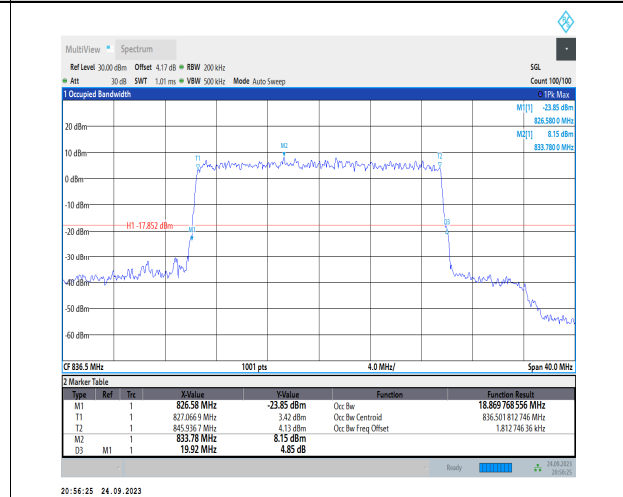
1-N5-PC3-15-20-M-9-CP-256QAM-Outer_Full-106@0-Ant1-18.87-19.920-≤20-PASS
