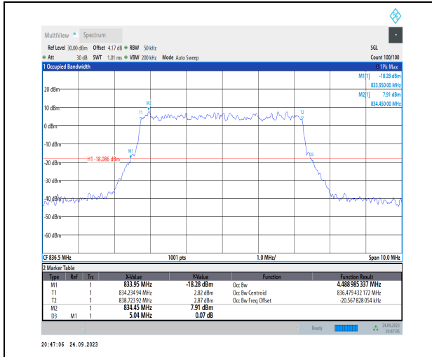
1-N5-PC3-15-5-M-5-DFT-256QAM-Outer_Full-25@0 -Ant1-4.489-5.040-<math>\leq 5</math>-PASS
