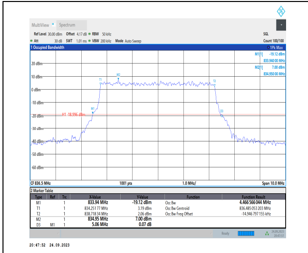
1-N5-PC3-15-5-M-9-CP-256QAM-Outer_Full-25@0-Ant1-4.467-5.060-≤5-PASS
