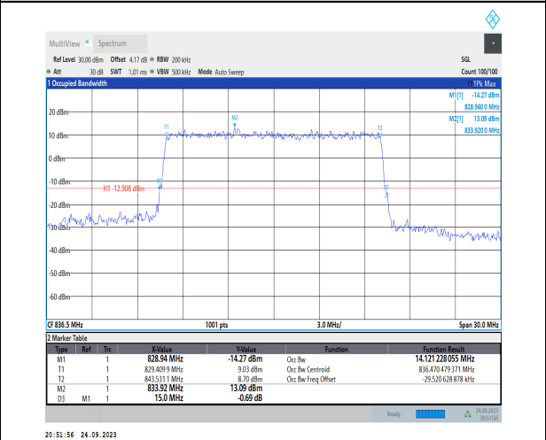
1-N5-PC3-15-15-M-6-CP-QPSK-Outer_Full-79@0-A nt1-14.121-15.000-≤15-PASS
