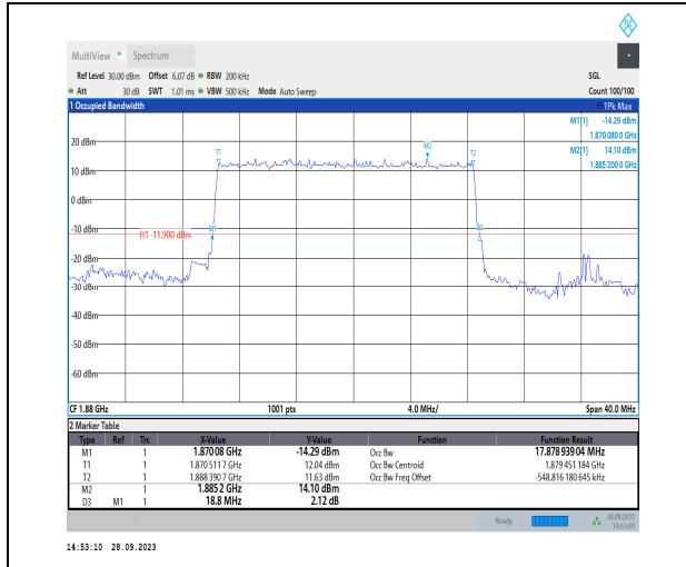
1-N2-PC3-15-20-M-2-DFT-PI2BPSK-Outer_Full-100 @0-Ant2-17.879-18.800-≤20-PASS
