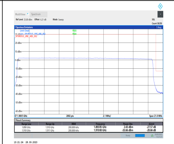
1-N2-PC3-15-20-H-6-CP-QPSK-Outer_Full-106@0-Ant2-1-seegraph-PASS-see graph
