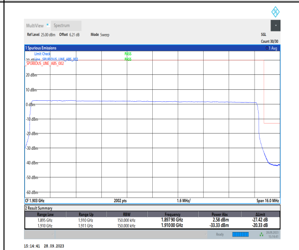
1-N2-PC3-15-15-H-6-CP-QPSK-Outer_Full-79@0-Ant2-1-seegraph-PASS-see graph
