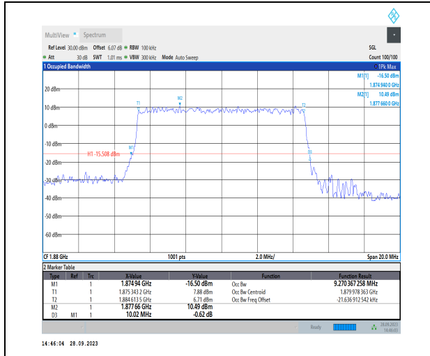
1-N2-PC3-15-10-M-8-CP-64QAM-Outer_Full-52@0-Ant2-9.27-10.020-≤10-PASS
