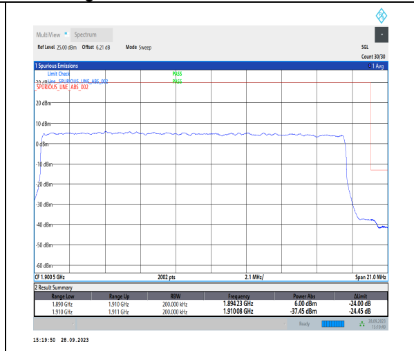
1-N2-PC3-15-20-H-3-DFT-PI2BPSK-Outer_Full-100@0-Ant2-1-seegraph-PASS-see graph
