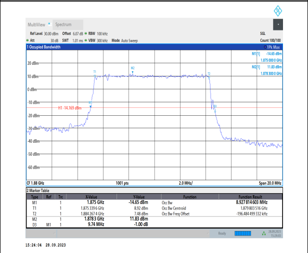
1-N2-PC3-15-10-M-3-DFT-16QAM-Outer_Full-50@0-Ant2-8.928-9.740-≤10-PASS
