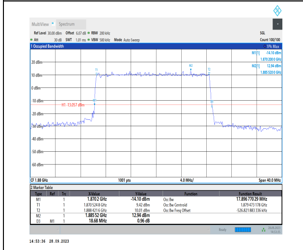
1-N2-PC3-15-20-M-4-DFT-64QAM-Outer_Full-100 @0-Ant2-17.897-18.680-≤20-PASS
