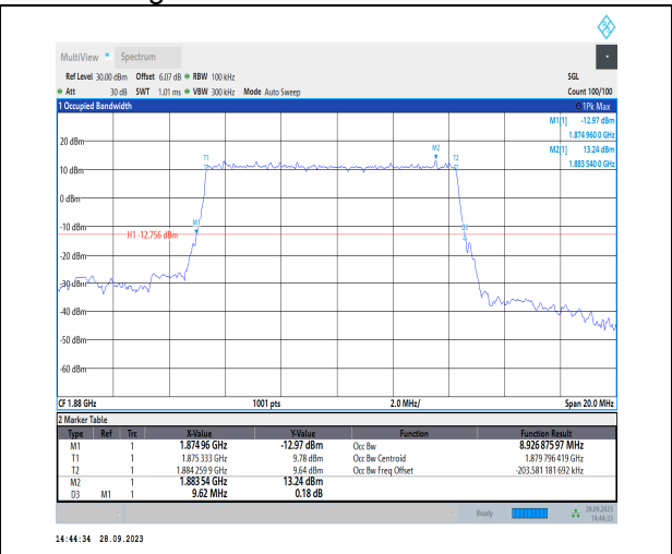
1-N2-PC3-15-10-M-1-DFT-QPSK-Outer_Full-50@0-Ant2-8.927-9.620-≤10-PASS
