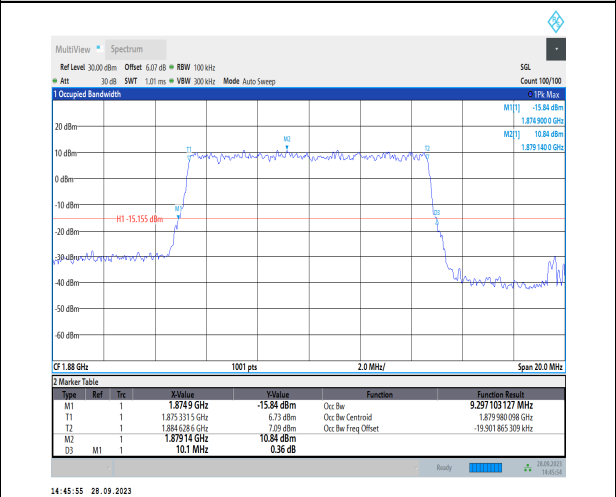
1-N2-PC3-15-10-M-7-CP-16QAM-Outer_Full-52@0-Ant2-9.297-10.100-≤10-PASS
