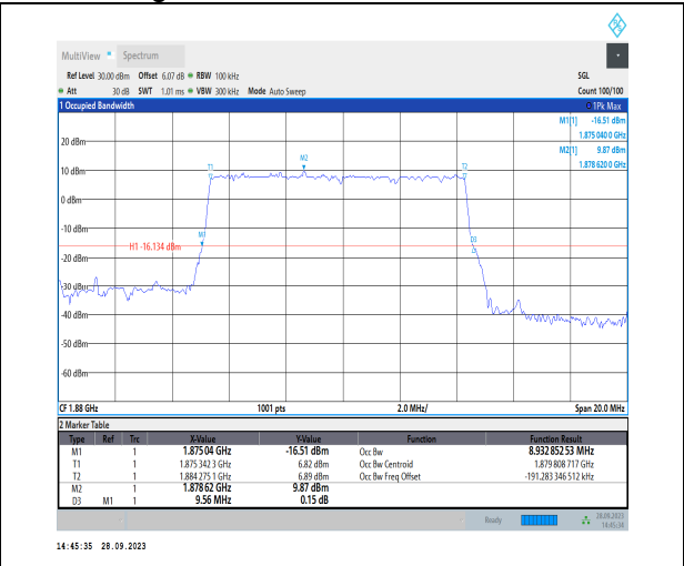
1-N2-PC3-15-10-M-5-DFT-256QAM-Outer_Full-50@0-Ant2-8.933-9.560-≤10-PASS
