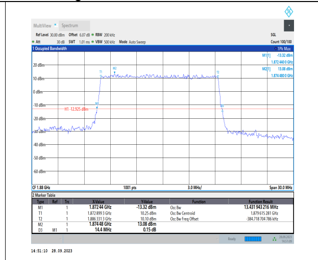
1-N2-PC3-15-15-M-4-DFT-64QAM-Outer_Full-75@0 -Ant2-13.432-14.400-≤15-PASS
