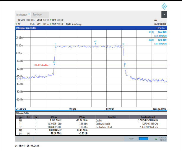
1-N2-PC3-15-20-M-5-DFT-256QAM-Outer_Full-100 @0-Ant2-17.876-18.640-≤20-PASS
