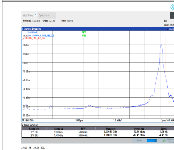
1-N2-PC3-15-15-H-5-CP-QPSK-Edge_1RB_Right-1@78-Ant2-1-seegraph-PASS-see graph
