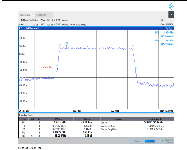
1-N2-PC3-15-15-M-9-CP-256QAM-Outer_Full-79@0-Ant2-14.081-15.090-≤15-PASS
