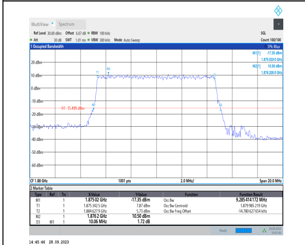
1-N2-PC3-15-10-M-6-CP-QPSK-Outer_Full-52@0-Ant2-9.285-10.060-≤10-PASS
