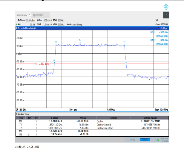
1-N2-PC3-15-20-M-3-DFT-16QAM-Outer_Full-100 @0-Ant2-17.88-18.760-≤20-PASS
