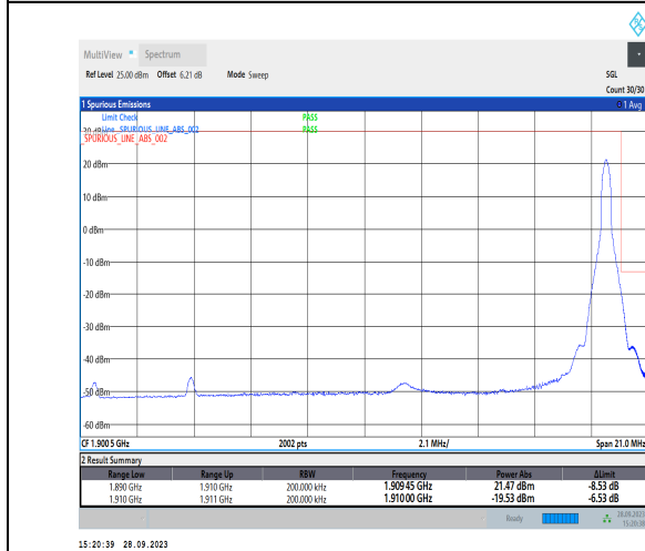
1-N2-PC3-15-20-H-5-CP-QPSK-Edge_1RB_Right-1@105-Ant2-1-seegraph-PASS-see graph
