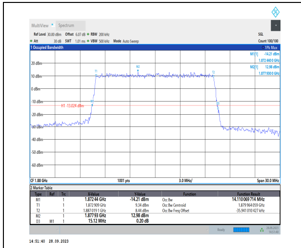
1-N2-PC3-15-15-M-7-CP-16QAM-Outer_Full-79@0-Ant2-14.11-15.120-≤15-PASS
