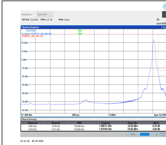
1-N2-PC3-15-15-H-2-DFT-PI2BPSK-Edge_1RB_Right-1@78-Ant2-1-seegraph-PASS-see graph
