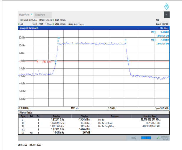
1-N2-PC3-15-15-M-3-DFT-16QAM-Outer_Full-75@0 -Ant2-13.447-14.430-≤15-PASS
