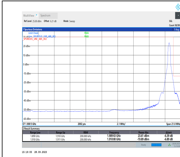
1-N2-PC3-15-20-H-2-DFT-PI2BPSK-Edge_1RB_Right-1@105-Ant2-1-seegraph-PASS-see graph
