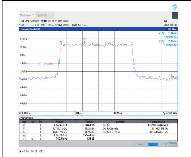
1-N2-PC3-15-15-M-1-DFT-QPSK-Outer_Full-75@0-Ant2-13.391-14.250-≤15-PASS
