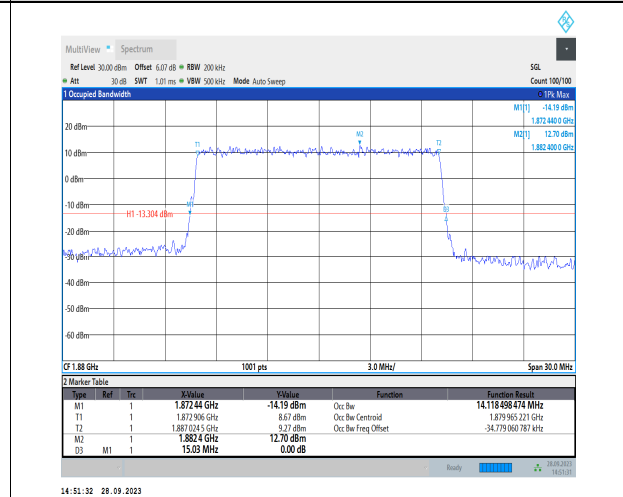
1-N2-PC3-15-15-M-6-CP-QPSK-Outer_Full-79@0-A nt2-14.118-15.030-≤15-PASS
