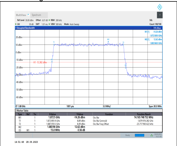
1-N2-PC3-15-15-M-8-CP-64QAM-Outer_Full-79@0-Ant2-14.166-15.000-≤15-PASS
