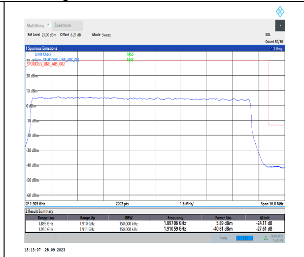
1-N2-PC3-15-15-H-3-DFT-PI2BPSK-Outer_Full-75@0-Ant2-1-seegraph-PASS-see graph
