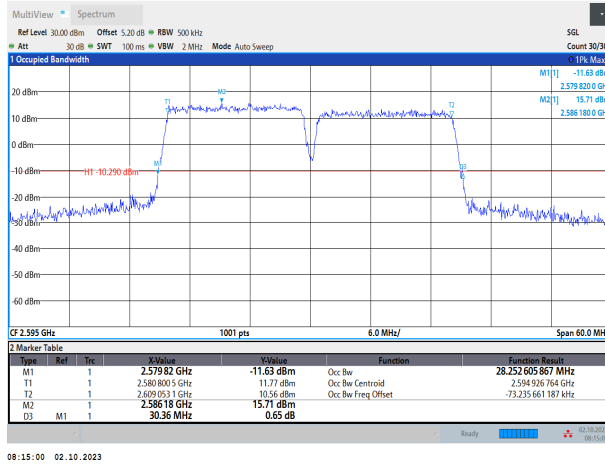
38-38-15MHz-15MHz-16QAM-16QAM-37925-38075-75RB#0-75RB#0
