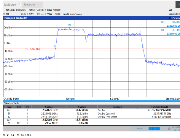
7-7-10MHz-20MHz-16QAM-16QAM-21006-21150-50RB#0-100RB#0
