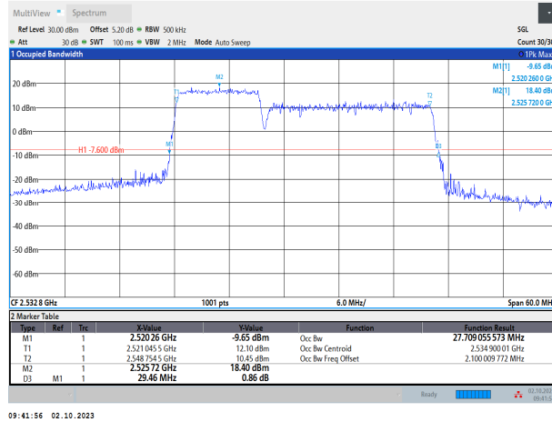
7-7-10MHz-20MHz-16QAM-16QAM-21006-21150-50RB#0-100RB#0
