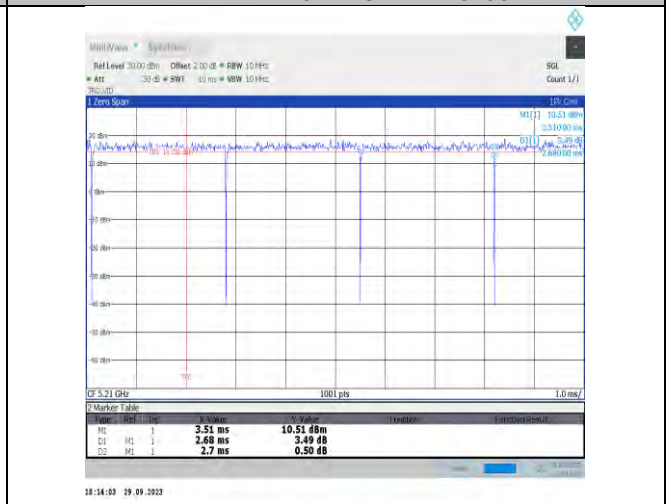
NTNV-11be80MIMO-Ant17-5210
