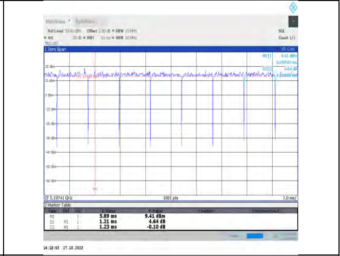
NTNV-11be80MIMO-Ant17-5210-P-20M-484+242Tone-RU65+64
