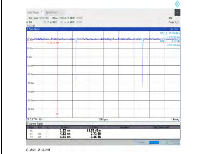
NTNV-11be20MIMO-Ant17-5180-106+26Tone-RU53+4
