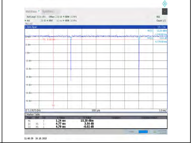
NTNV-11be20MIMO-Ant17-5180-106Tone-RU53
