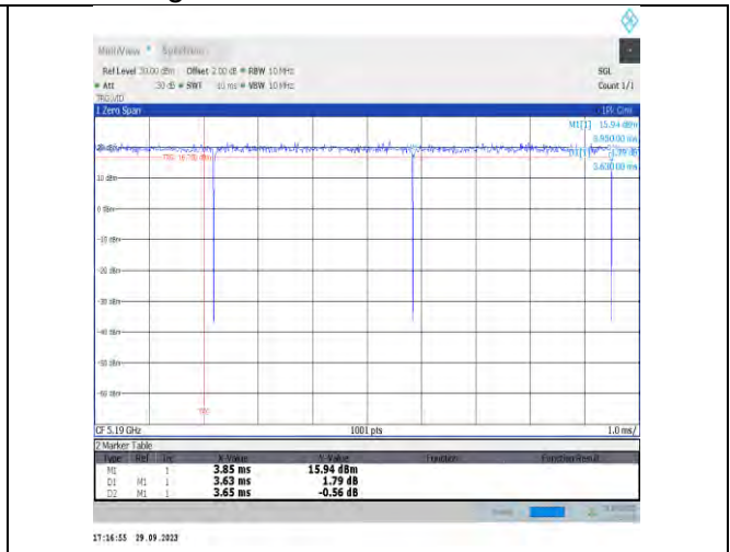
NTNV-11be40MIMO-Ant17-5190
