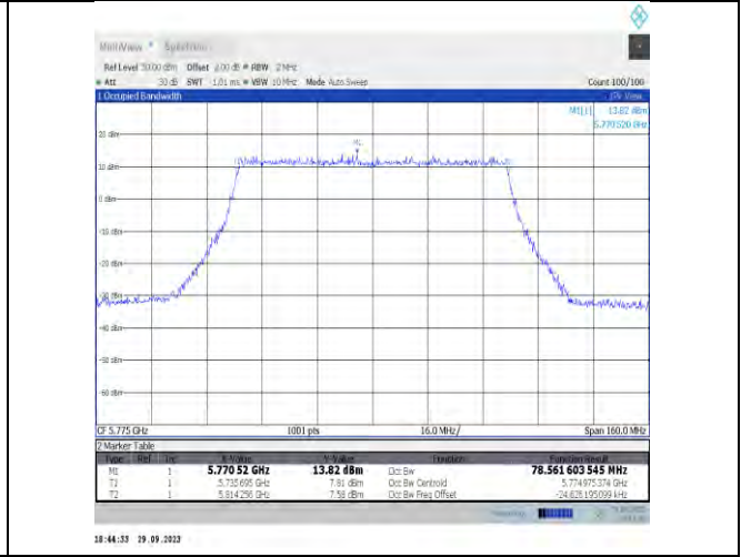
11be80MIMO-Ant17-5775
