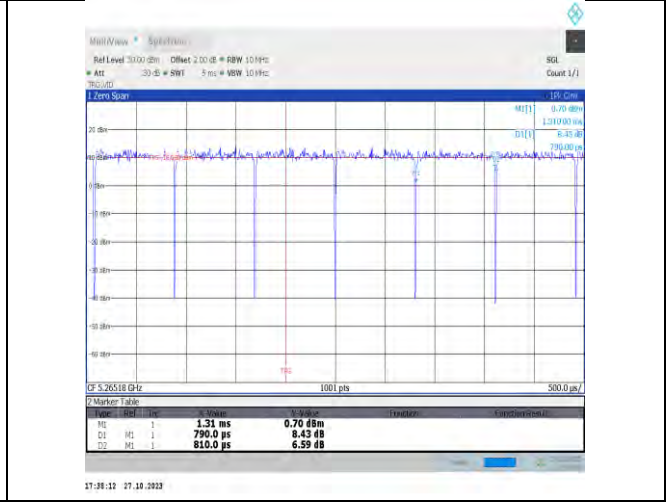
NTNV-11be160MIMO-Ant6-5250-P-20M-
