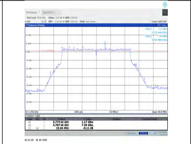
11be20MIMO-Ant17-5785-PASS
