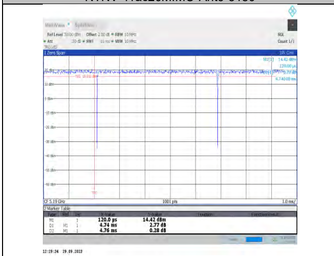
NTNV-11ac40MIMO-Ant6-5190
