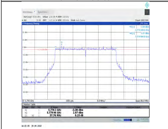
11be40MIMO-Ant6-5795-PASS
