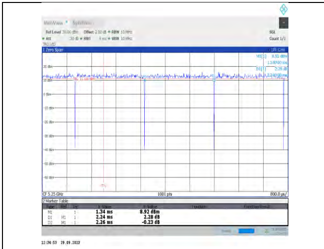
NTVN-11ac160MIMO-Ant6-5250
