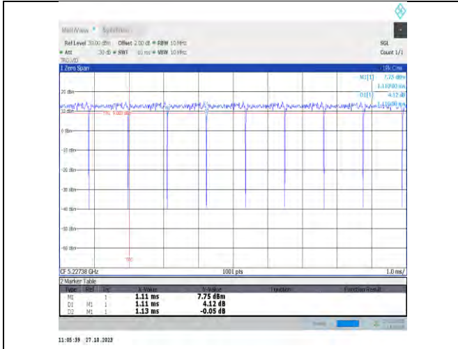
NTNV-11be80MIMO-Ant6-5210-Large-484+242Tone-RU65+63
