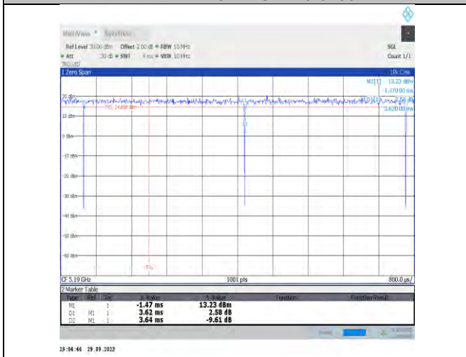
NTVN-11ax40MIMO-Ant6-5190
