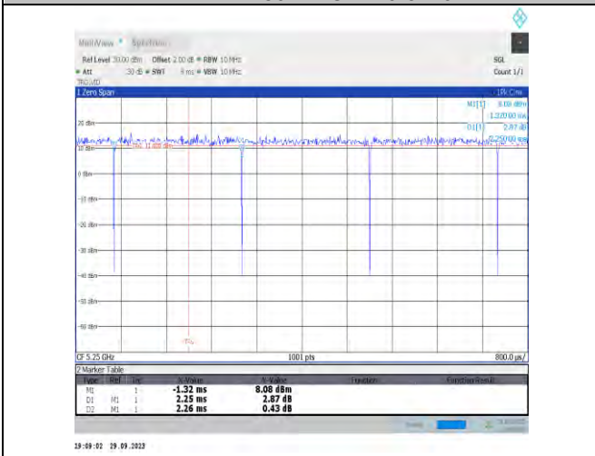
NTNV-11ax160MIMO-Ant6-5250
