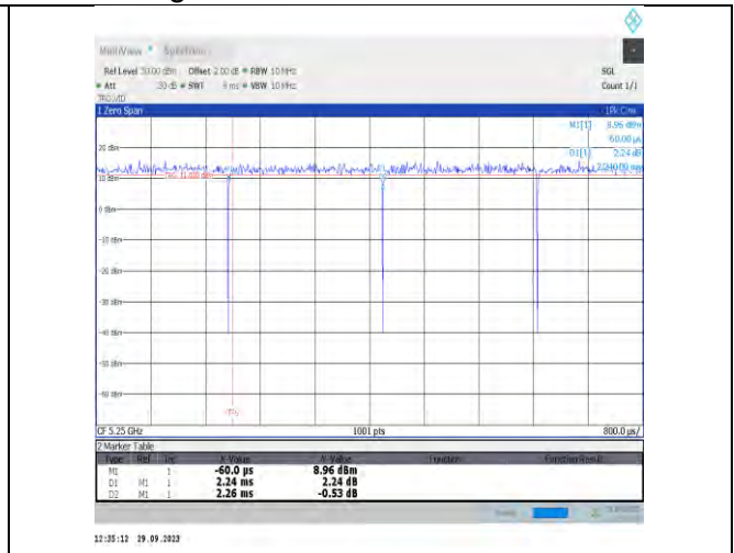
NTVN-11ac160MIMO-Ant17-5250
