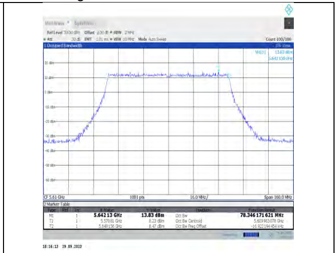
11be80MIMO-Ant17-5610
