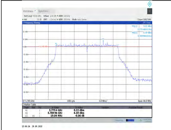
11be20MIMO-Ant6-5785-PASS
