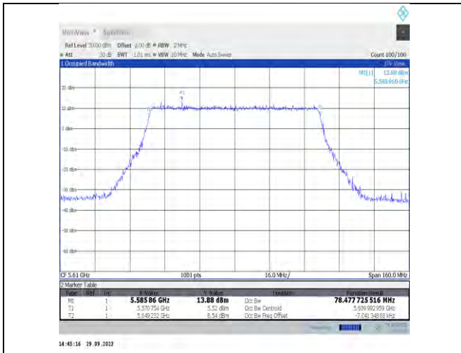
11be80MIMO-Ant6-5610
