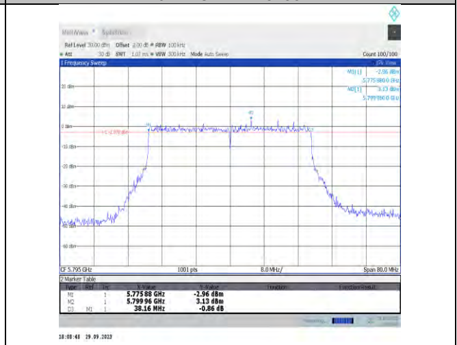
11be40MIMO-Ant17-5795-PASS
