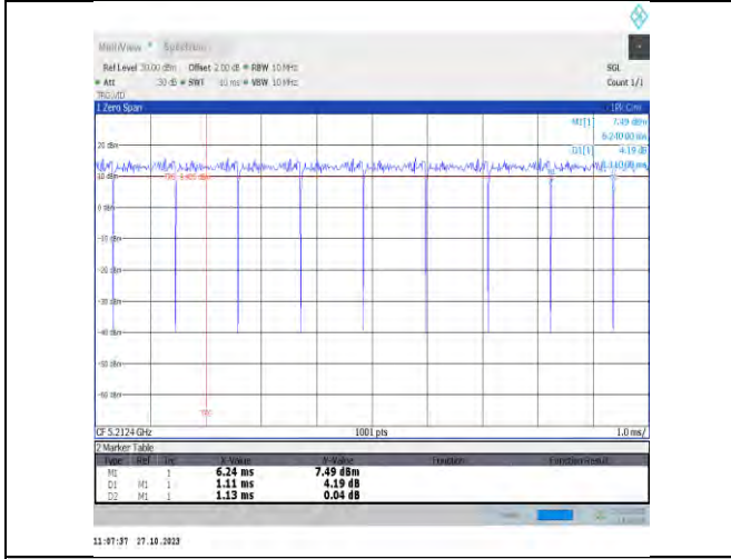
NTNV-11be80MIMO-Ant17-5210-Large-484+242Tone-RU65+63
