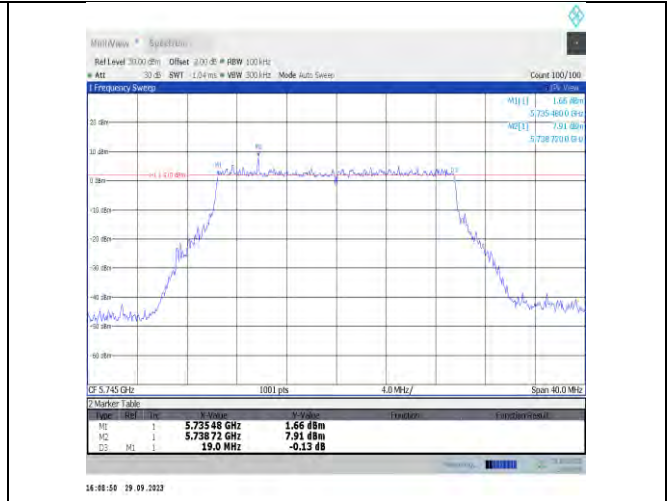
11be20MIMO-Ant17-5745-PASS
