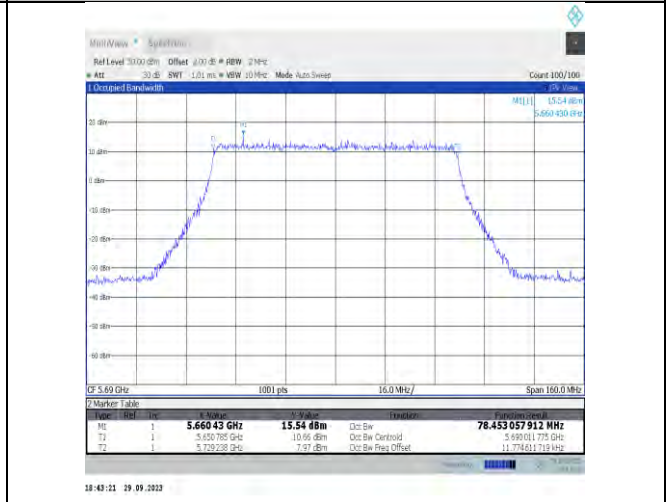
11be80MIMO-Ant17-5690
