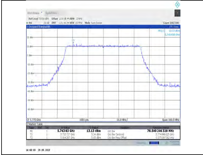
11be80MIMO-Ant6-5775
