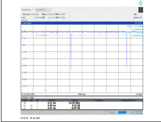
NTNV-11be20MIMO-Ant17-5180-52+26Tone-RU37+2
