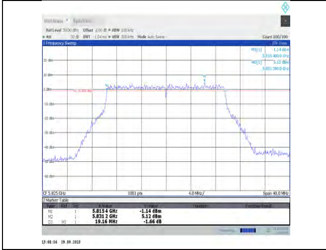
11be20MIMO-Ant6-5825-PASS
