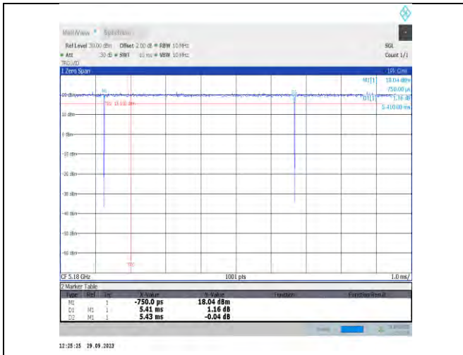
NTNV-11ac20MIMO-Ant6-5180
