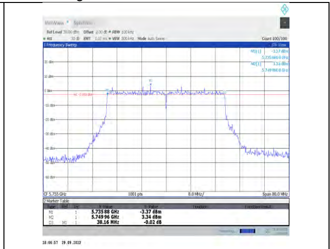
11be40MIMO-Ant17-5755-PASS
