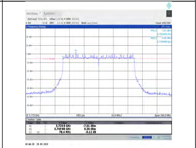
11be80MIMO-Ant17-5775-PASS
