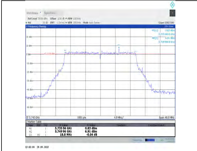
11be20MIMO-Ant6-5745-PASS
