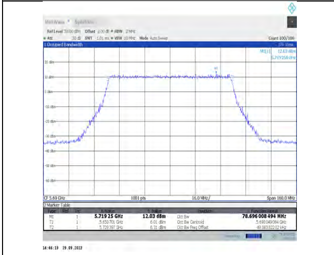
11be80MIMO-Ant6-5690
