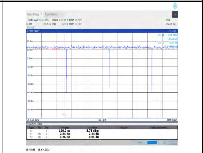
NTNV-11ax160MIMO-Ant17-5250
