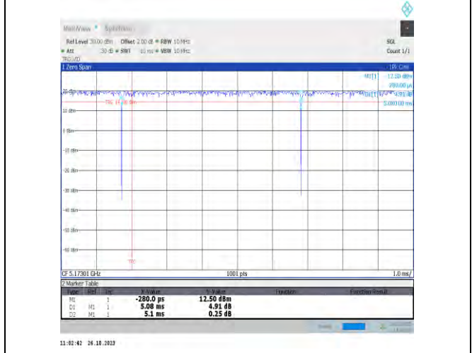
NTNV-11be20MIMO-Ant17-5180-52Tone-RU37
