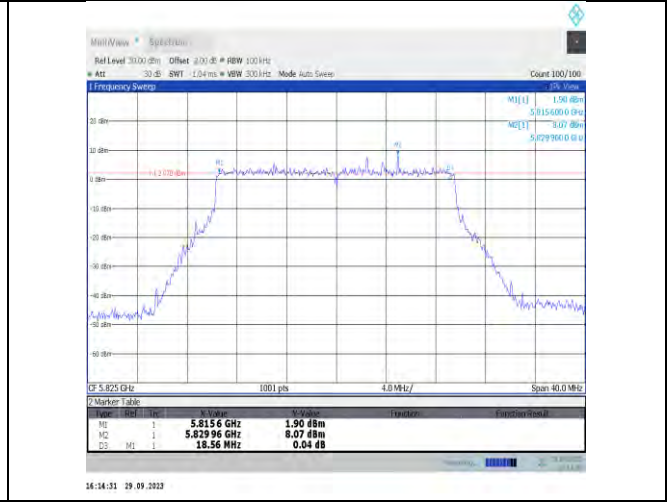
11be20MIMO-Ant17-5825-PASS
