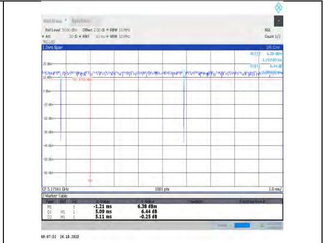
NTNV-11be20MIMO-Ant17-5180-26Tone-RU0
