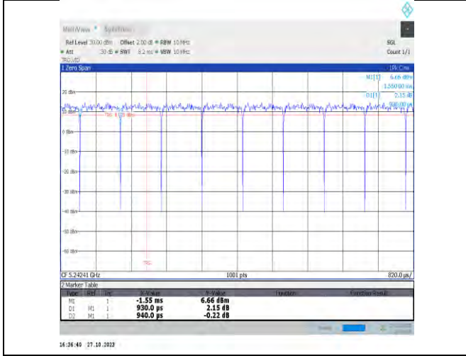
NTNV-11be160MIMO-Ant6-5250-Large-996+484Tone-
