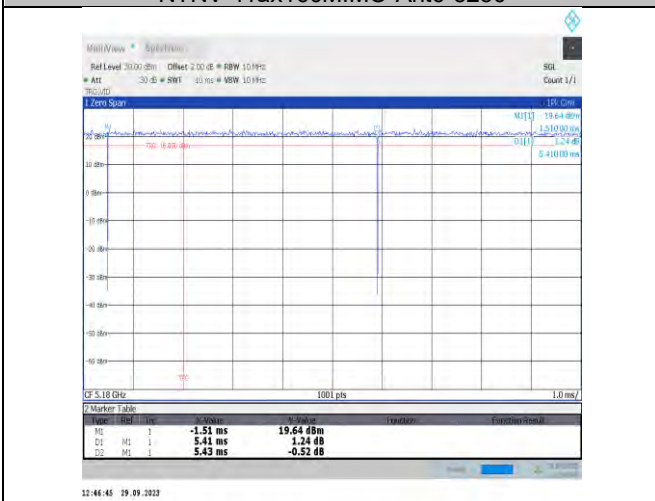
NTNV-11be20MIMO-Ant6-5180
