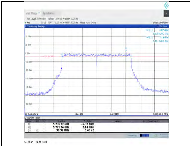
11be40MIMO-Ant6-5755-PASS
