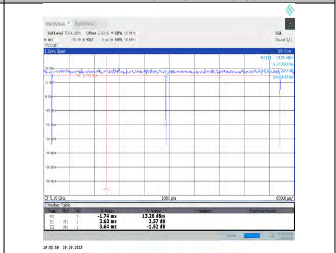
NTVN-11ax40MIMO-Ant17-5190
