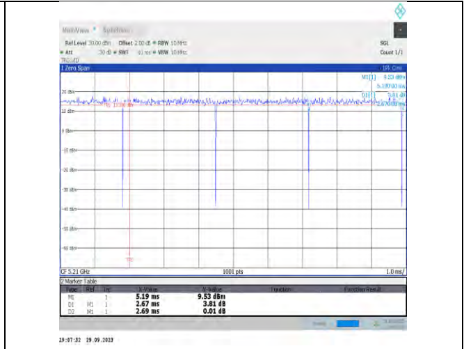
NTNV-11ax80MIMO-Ant17-5210
