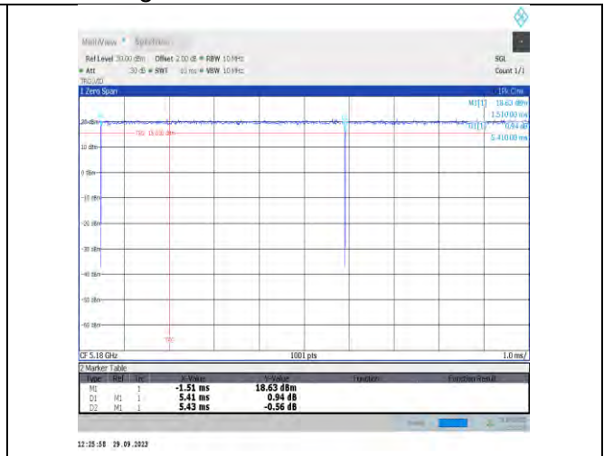
NTNV-11ac20MIMO-Ant17-5180
