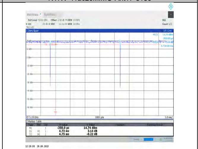
NTNV-11ac40MIMO-Ant17-5190
