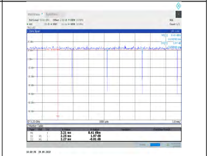
NTNV-11be160MIMO-Ant17-5250
