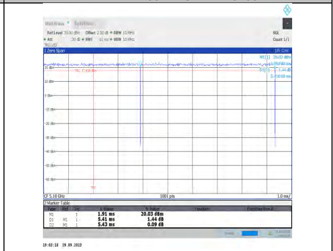
NTVN-11ax20MIMO-Ant17-5180
