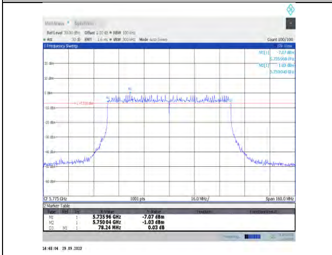
11be80MIMO-Ant6-5775-PASS
