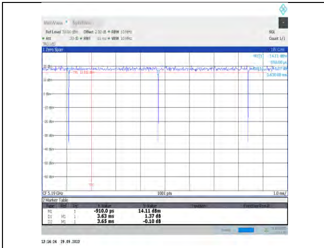
NTNV-11be40MIMO-Ant6-5190
