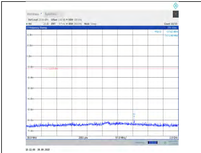
11be20MIMO-Ant7-2462-30~1000-PASS
