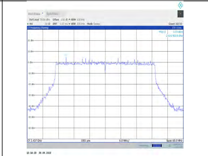
11be40MIMO-Ant7-2437-0~Reference-PASS
