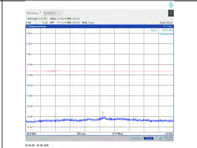
11be40MIMO-Ant16-2437-30~1000-PASS
