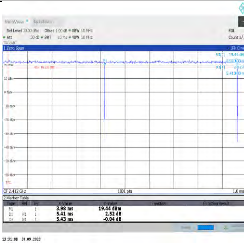
NTVN-11VHT20MIMO-Ant16-2412
