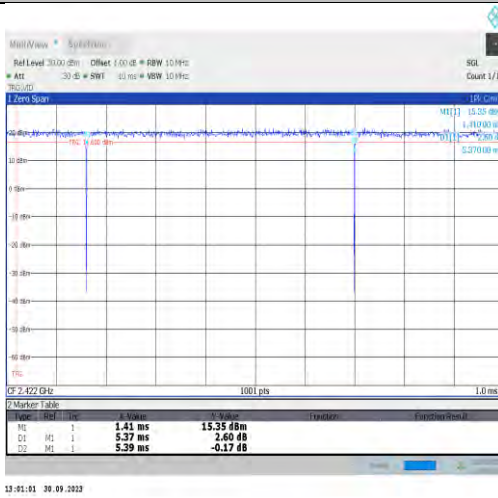
NTVN-11n40MIMO-Ant16-2422
