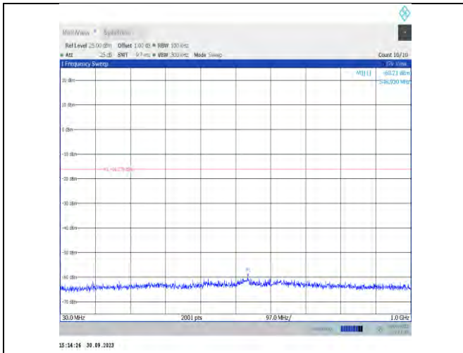
11be40MIMO-Ant7-2437-30~1000-PASS
