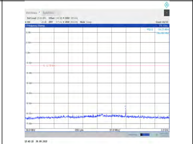
11be20MIMO-Ant16-2462-30~1000-PASS
