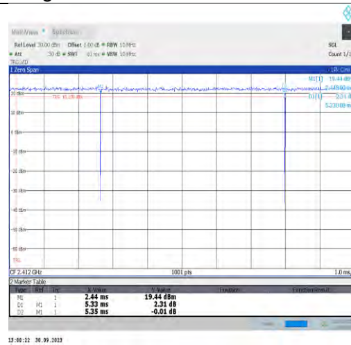
NTVN-11n20MIMO-Ant7-2412
