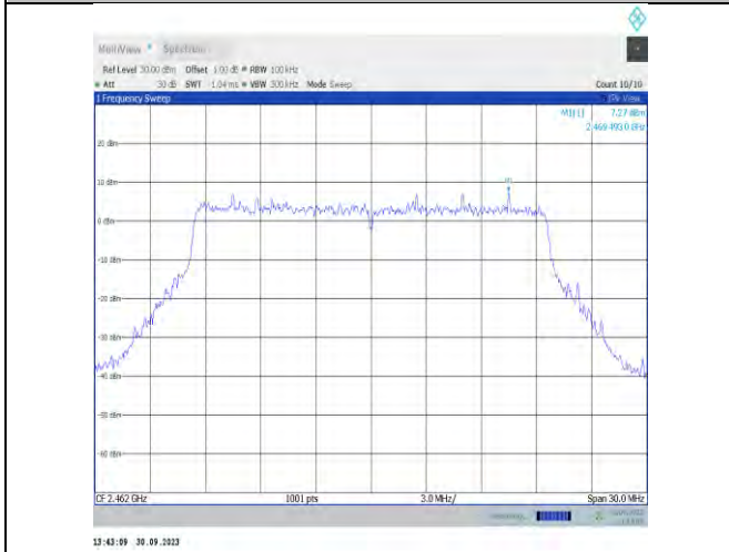
11be20MIMO-Ant16-2462-0~Reference-PASS
