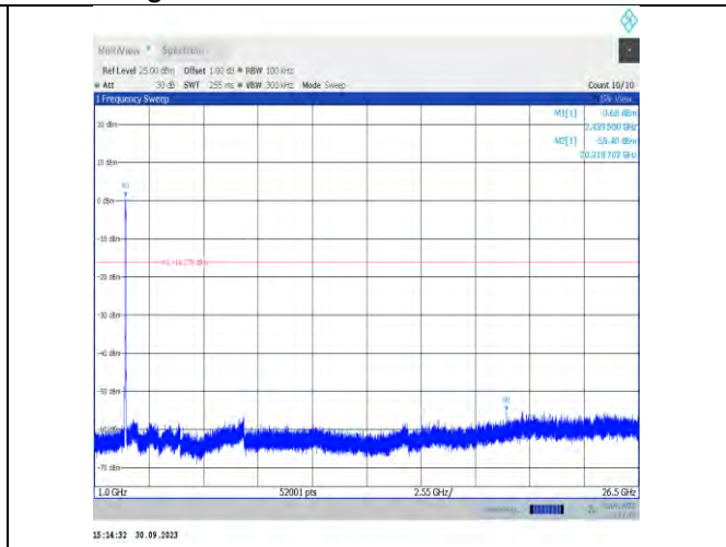
11be40MIMO-Ant7-2437-1000~26500-PASS
