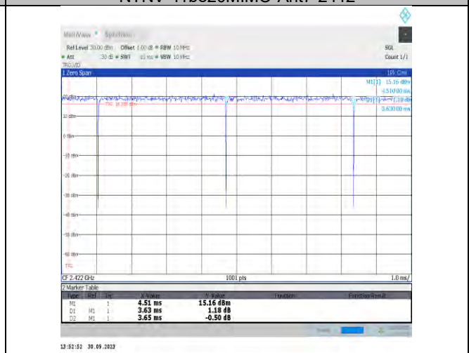
NTVN-11be40MIMO-Ant7-2422
