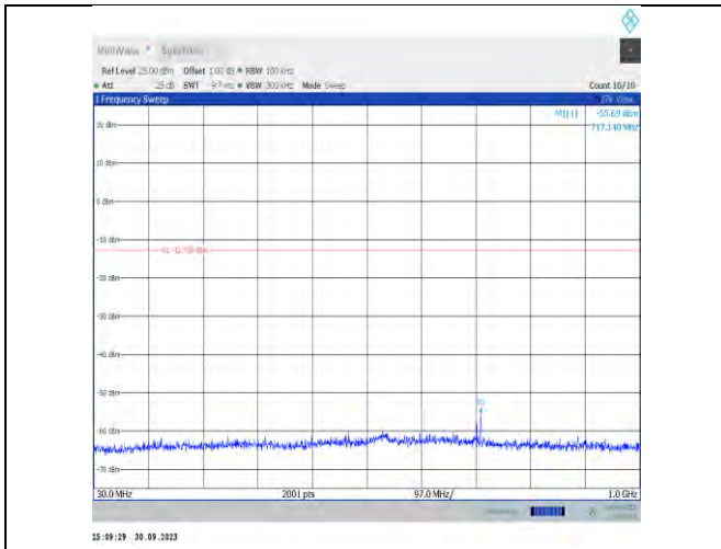
11be20MIMO-Ant7-2437-30~1000-PASS
