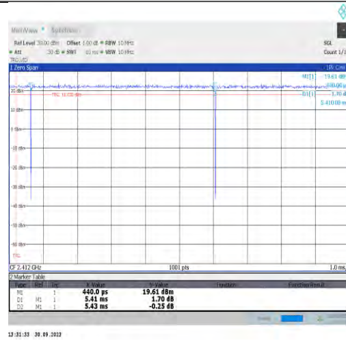
NTVN-11VHT20MIMO-Ant7-2412
