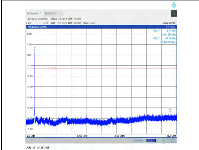
11be20MIMO-Ant16-2462-1000~26500-PASS
