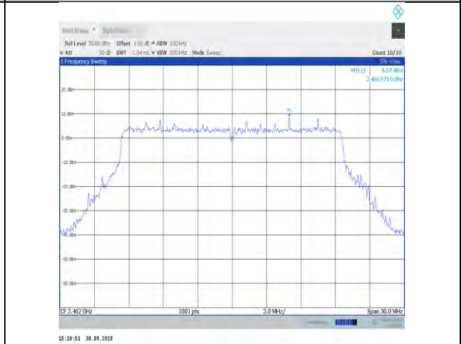
11be20MIMO-Ant7-2462-0~Reference-PASS
