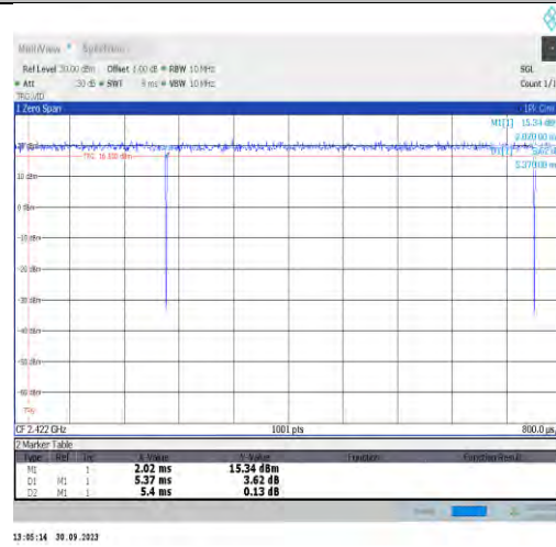
NTVN-11n40MIMO-Ant7-2422
