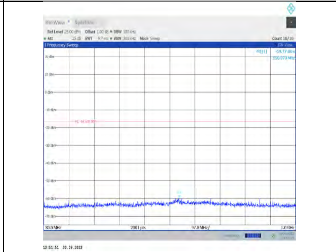
11be40MIMO-Ant16-2422-30~1000-PASS
