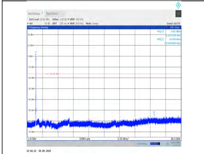
11be40MIMO-Ant16-2437-1000~26500-PASS
