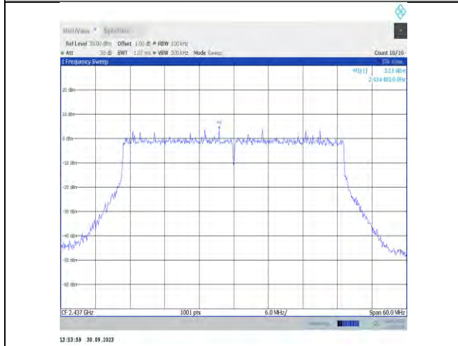
11be40MIMO-Ant16-2437-0~Reference-PASS
