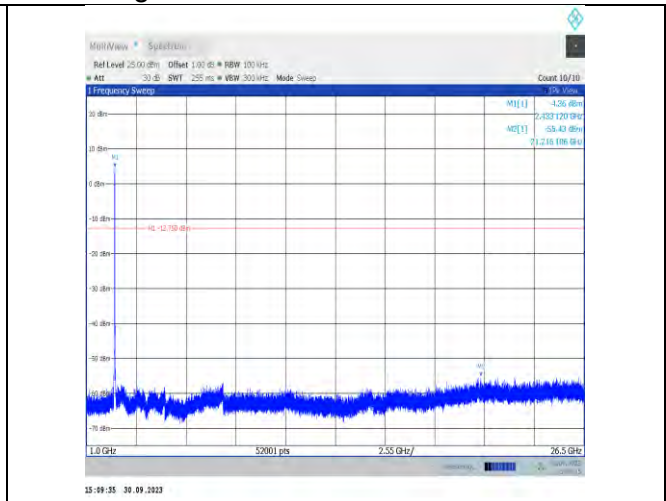
11be20MIMO-Ant7-2437-1000~26500-PASS
