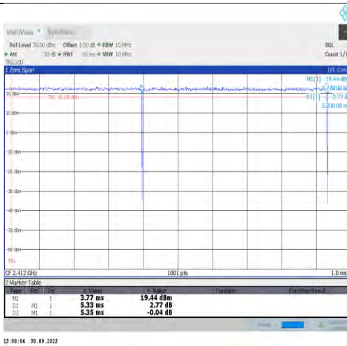
NTVN-11n20MIMO-Ant16-2412
