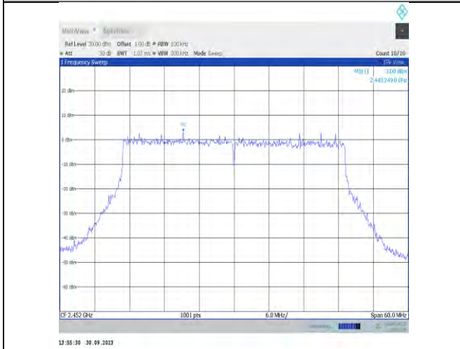
11be40MIMO-Ant16-2452-0~Reference-PASS
