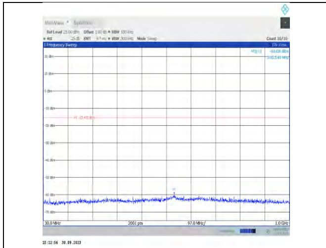
11be40MIMO-Ant7-2422-30~1000-PASS
