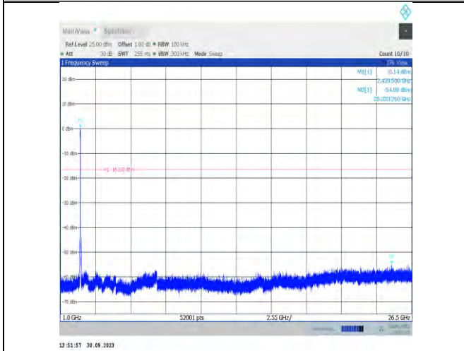
11be40MIMO-Ant16-2422-1000~26500-PASS
