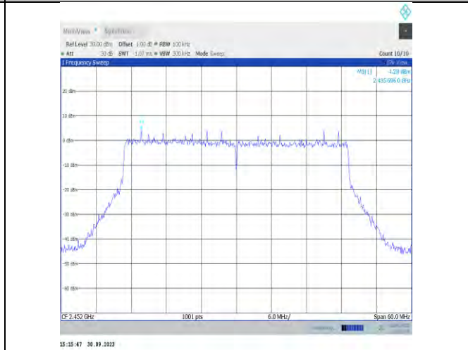
11be40MIMO-Ant7-2452-0~Reference-PASS
