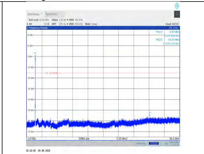
11be40MIMO-Ant7-2422-1000~26500-PASS
