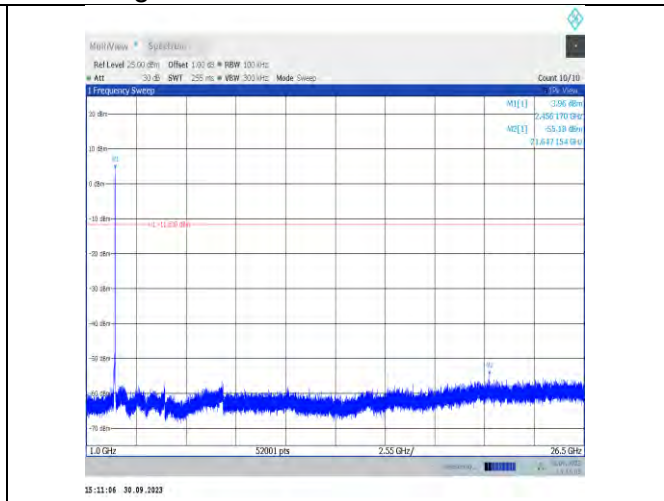
11be20MIMO-Ant7-2462-1000~26500-PASS
