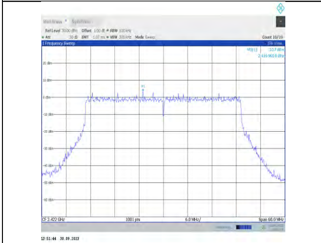
11be40MIMO-Ant16-2422-0~Reference-PASS
