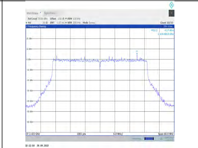
11be40MIMO-Ant7-2422-0~Reference-PASS
