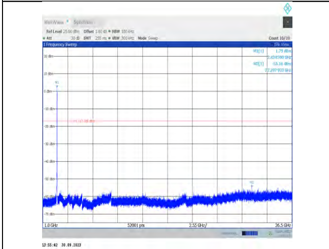
11be40MIMO-Ant16-2452-1000~26500-PASS
