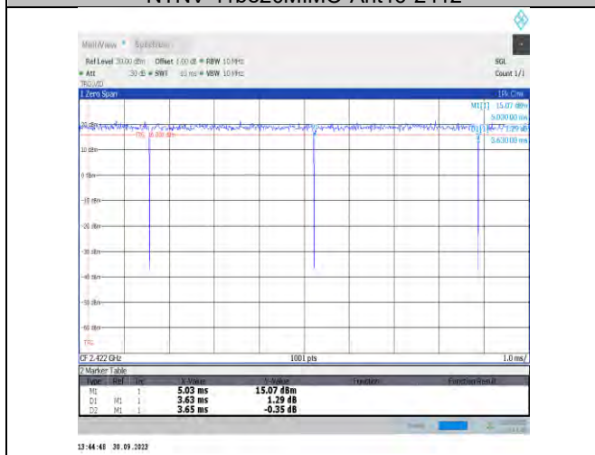
NTVN-11be40MIMO-Ant16-2422
