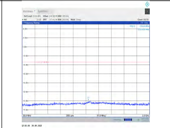
11be40MIMO-Ant16-2452-30~1000-PASS
