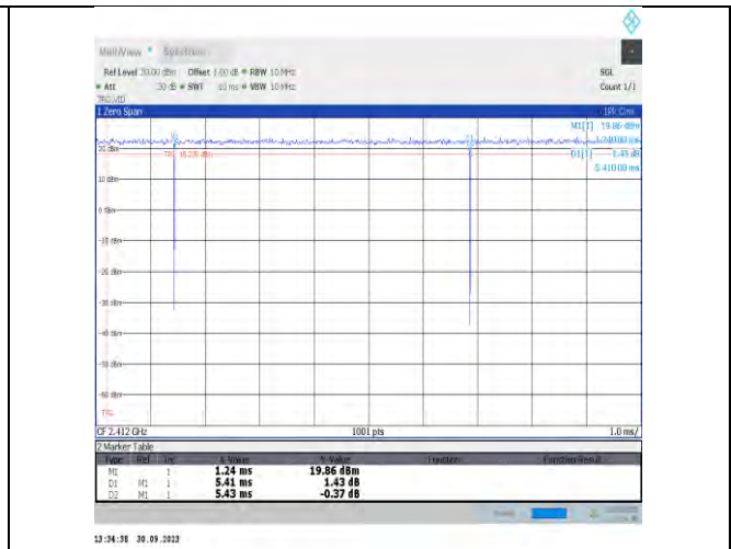
NTVN-11be20MIMO-Ant7-2412
