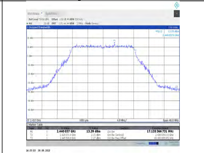
11g-CDD-Ant7-2437
