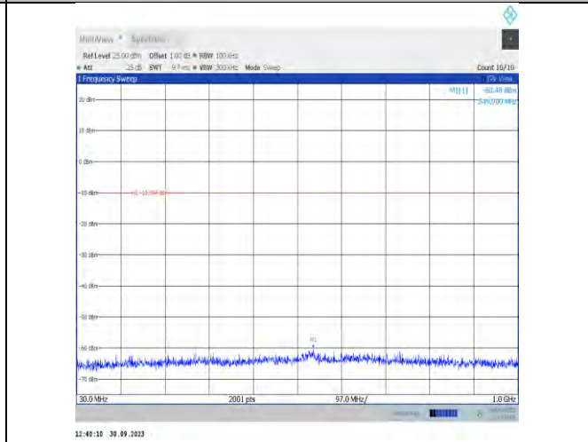
11b-CDD-Ant16-2462-30~1000-PASS
