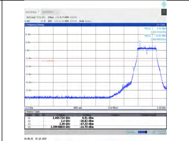
11n20MIMO-Ant7-2412-PASS
