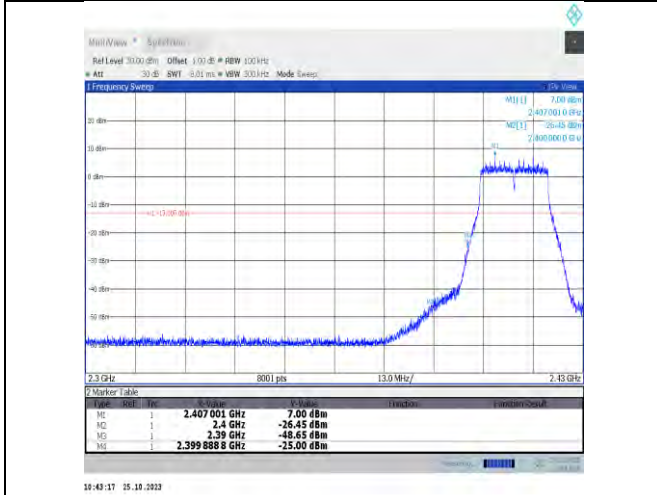
11n20MIMO-Ant16-2412-PASS
