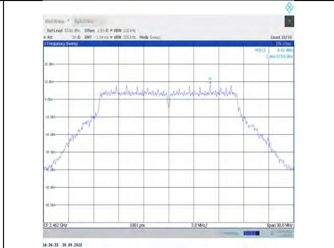
11g-CDD-Ant7-2462-0~Reference-PASS
