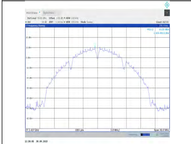
11b-CDD-Ant16-2437-0~Reference-PASS
