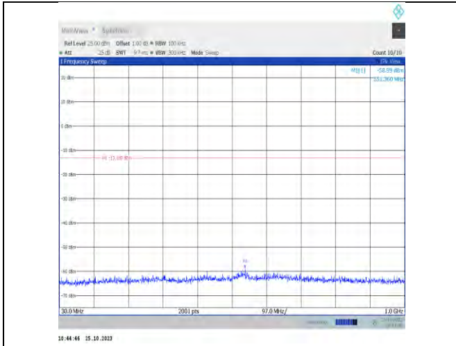
11n20MIMO-Ant7-2412-30~1000-PASS
