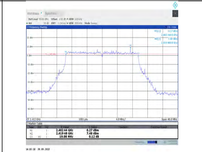
11be20MIMO-Ant7-2412-PASS
