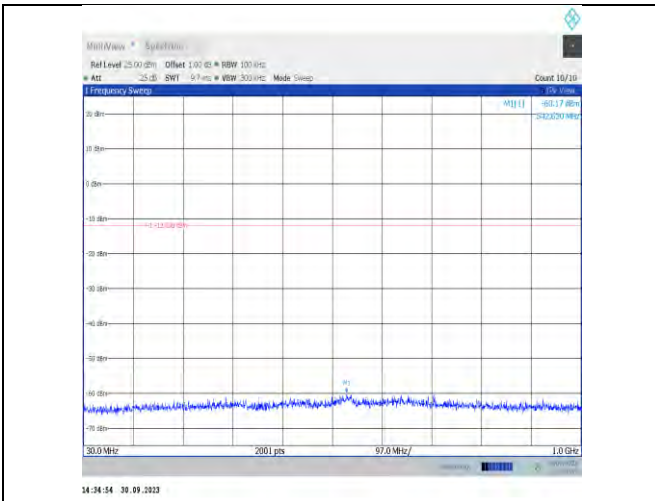
11g-CDD-Ant7-2437-30~1000-PASS
