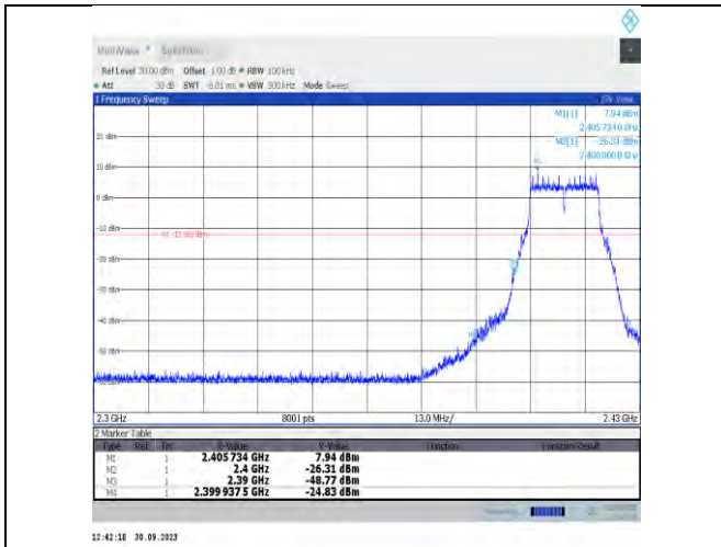
11g-CDD-Ant16-2412-PASS
