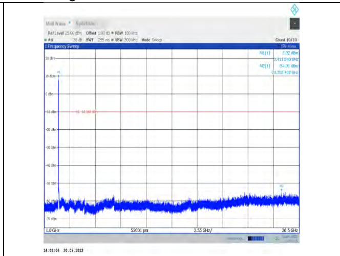
11b-CDD-Ant7-2412-1000~26500-PASS
