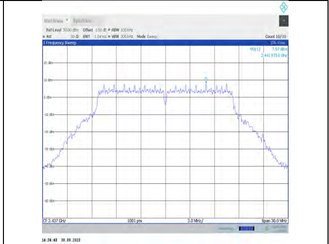
11g-CDD-Ant7-2437-0~Reference-PASS
