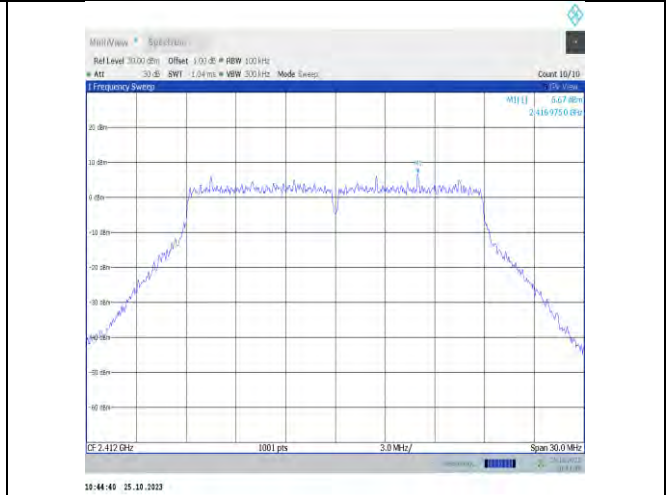
11n20MIMO-Ant7-2412-0~Reference-PASS
