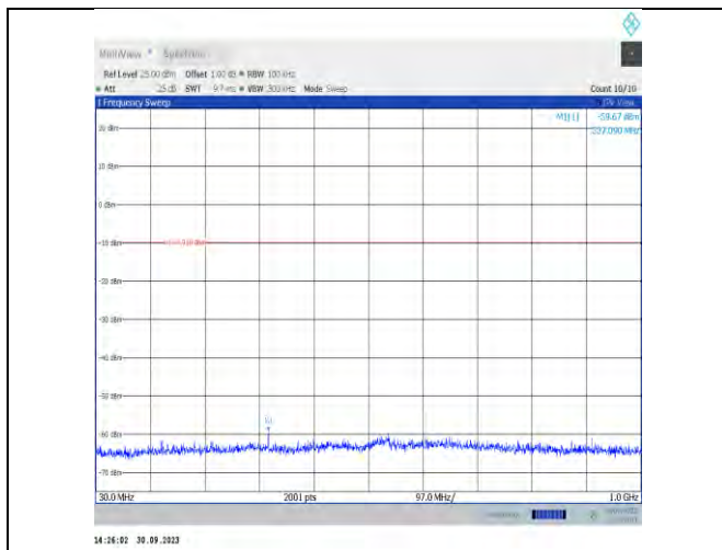
11b-CDD-Ant7-2462-30~1000-PASS
