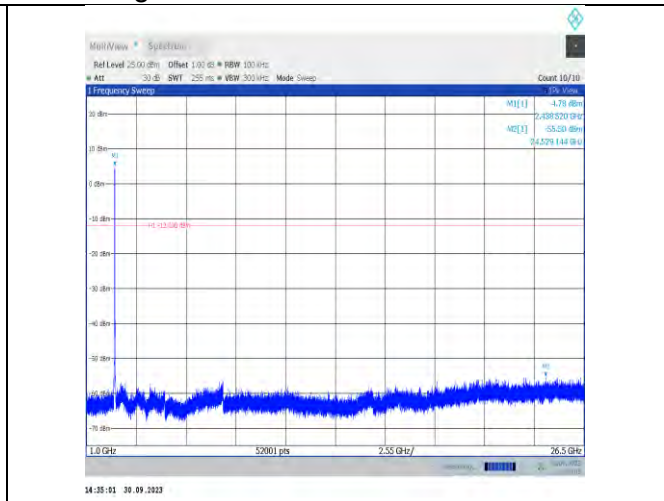
11g-CDD-Ant7-2437-1000~26500-PASS
