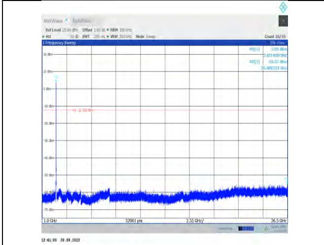
11be20MIMO-Ant16-2437-1000~26500-PASS
