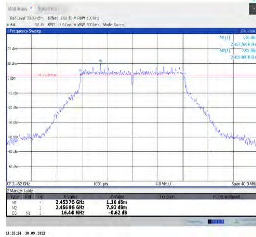
11g-CDD-Ant7-2462-PASS
