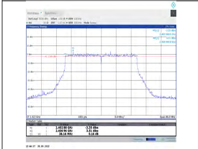
11be40MIMO-Ant16-2422-PASS
