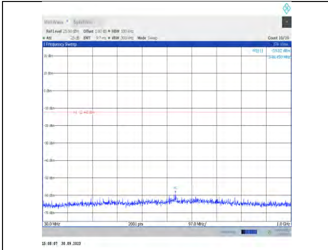
11be20MIMO-Ant7-2412-30~1000-PASS
