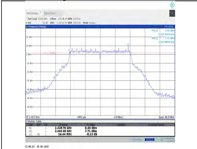
11g-CDD-Ant16-2437-PASS
