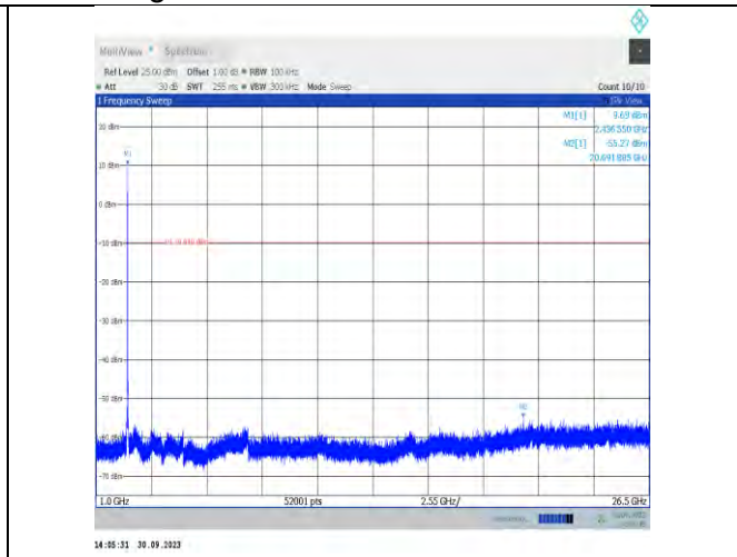
11b-CDD-Ant7-2437-1000~26500-PASS
