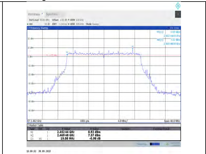
11be20MIMO-Ant7-2462-PASS
