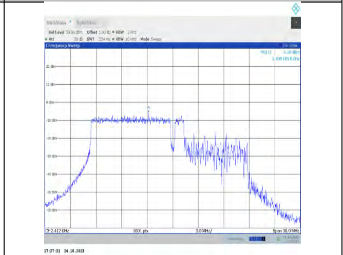
11be20MIMO-Ant7-2412-106+26Tone-RU53+4-PASS
