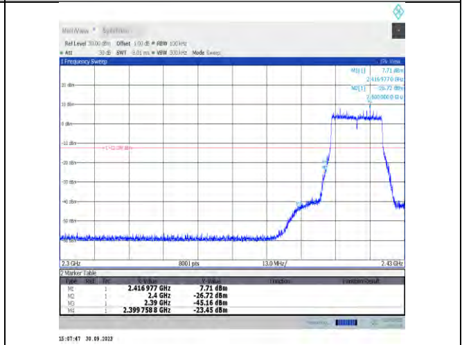
11be20MIMO-Ant7-2412-PASS
