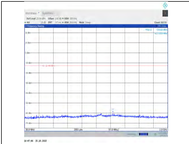
11n20MIMO-Ant7-2437-30~1000-PASS
