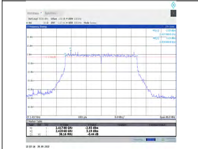
11be40MIMO-Ant16-2437-PASS
