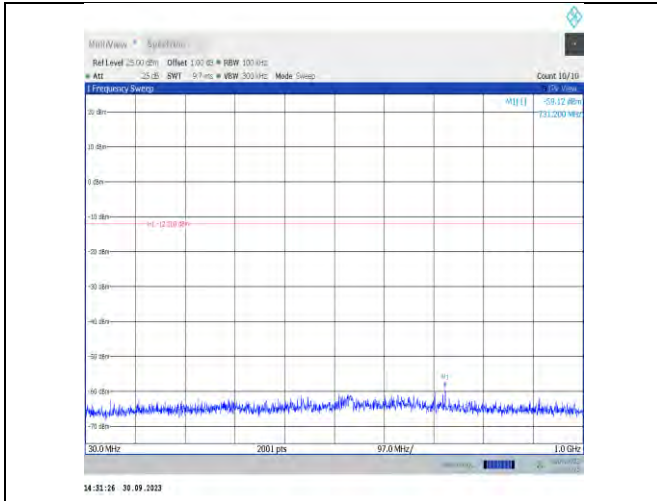
11g-CDD-Ant7-2412-30~1000-PASS
