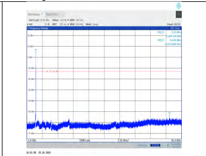
11n20MIMO-Ant7-2462-1000~26500-PASS
