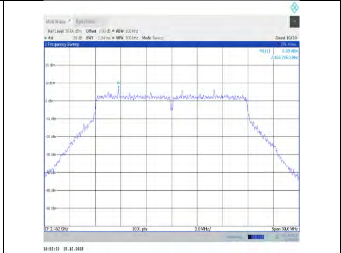
11n20MIMO-Ant7-2462-0~Reference-PASS
