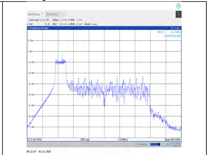
11be20MIMO-Ant7-2412-26Tone-RU0-PASS
