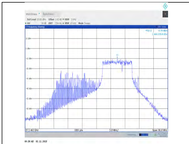
11be20MIMO-Ant7-2462-52+26Tone-RU40+6-PASS
