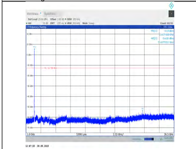
11g-CDD-Ant16-2412-1000~26500-PASS
