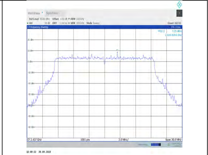
11be20MIMO-Ant7-2437-0~Reference-PASS
