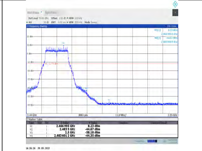
11g-CDD-Ant7-2462-PASS
