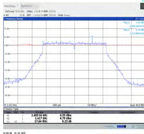
11n20MIMO-Ant7-2412-PASS
