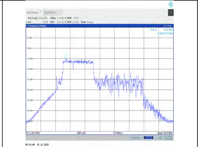
11be20MIMO-Ant7-2412-52+26Tone-RU37+2-PASS
