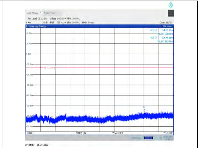
11n20MIMO-Ant7-2412-1000~26500-PASS
