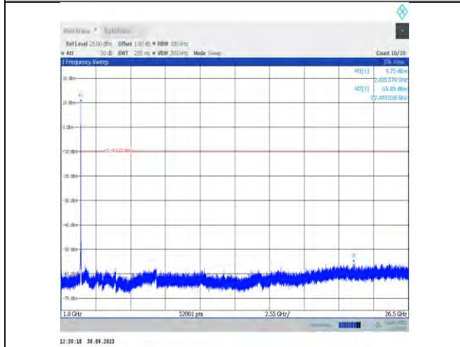
11b-CDD-Ant16-2437-1000~26500-PASS
