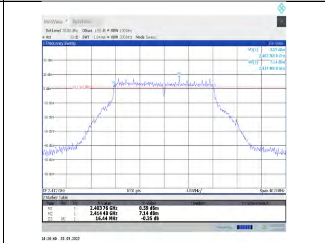
11g-CDD-Ant7-2412-PASS
