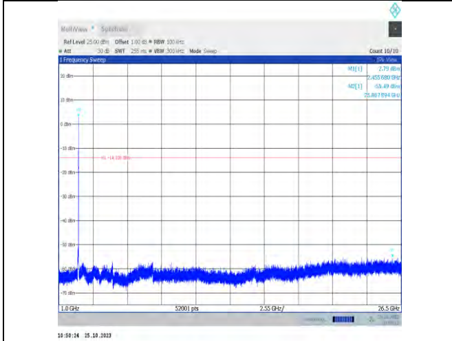
11n20MIMO-Ant16-2462-1000~26500-PASS
