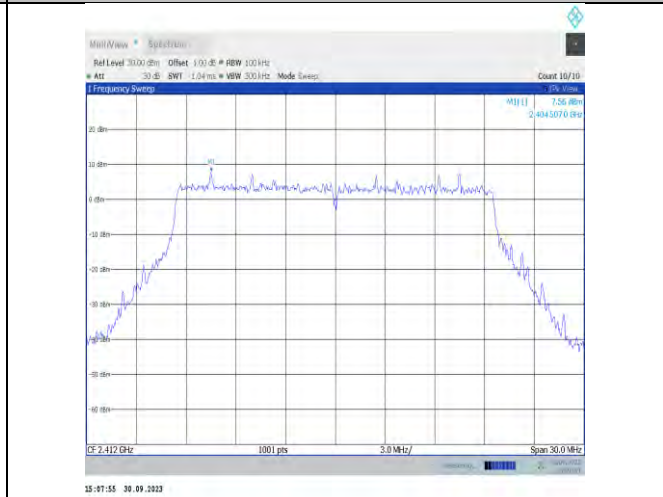
11be20MIMO-Ant7-2412-0~Reference-PASS
