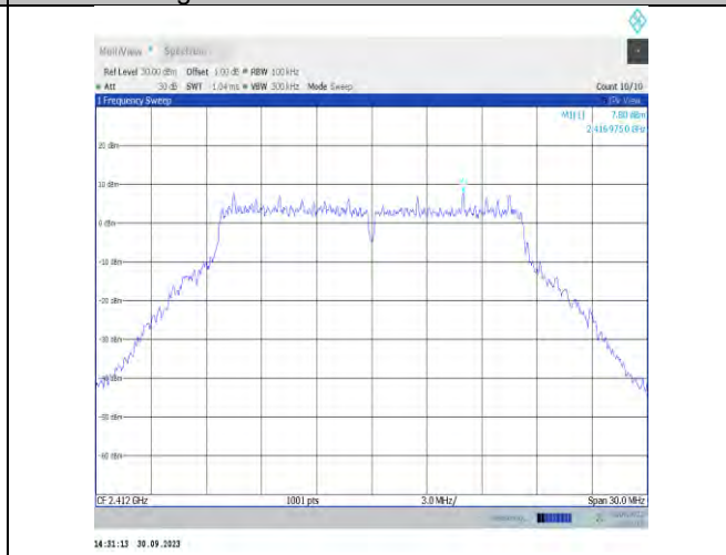
11g-CDD-Ant7-2412-0~Reference-PASS
