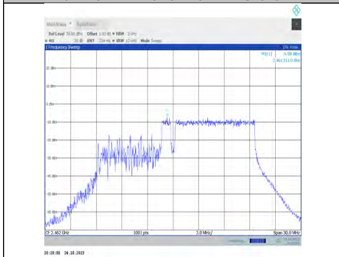
11be20MIMO-Ant7-2462-106+26Tone-RU54+4-PASS
