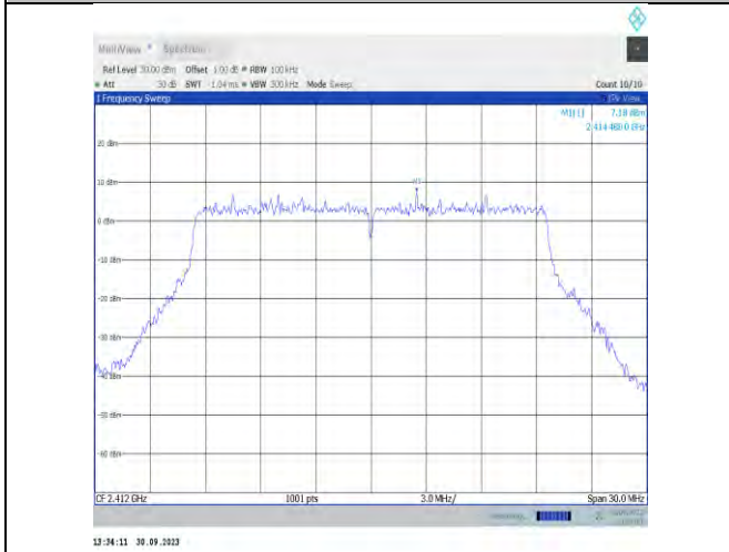
11be20MIMO-Ant16-2412-0~Reference-PASS
