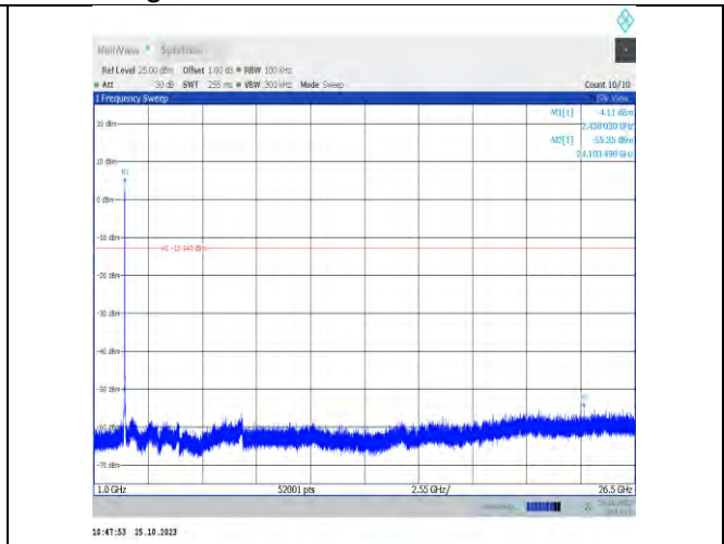
11n20MIMO-Ant7-2437-1000~26500-PASS
