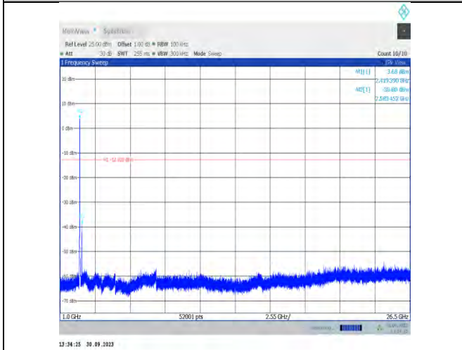
11be20MIMO-Ant16-2412-1000~26500-PASS
