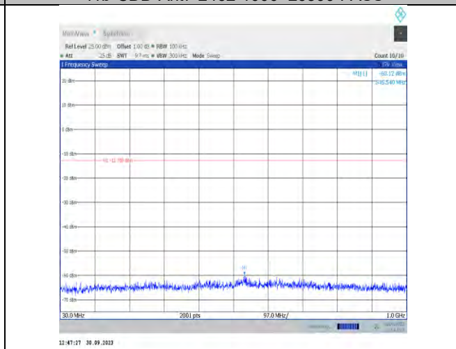
11g-CDD-Ant16-2412-30~1000-PASS
