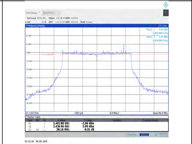
11be40MIMO-Ant7-2422-PASS
