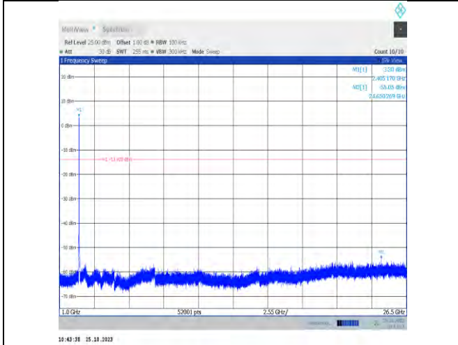
11n20MIMO-Ant16-2412-1000~26500-PASS
