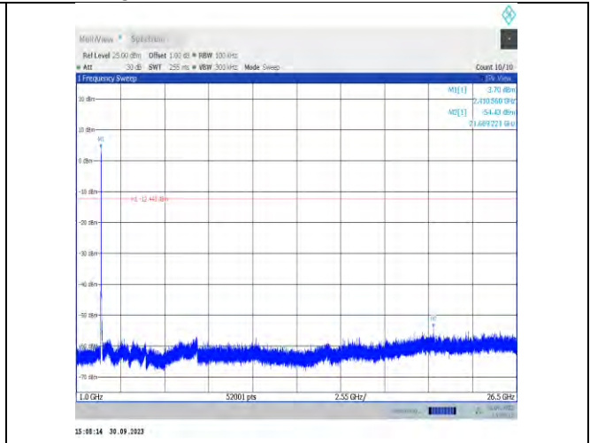
11be20MIMO-Ant7-2412-1000~26500-PASS
