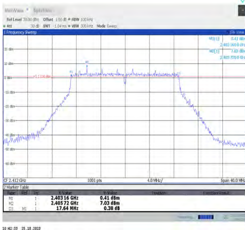
11n20MIMO-Ant16-2412-PASS
