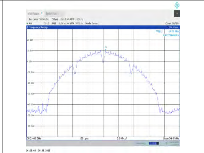
11b-CDD-Ant7-2462-0~Reference-PASS
