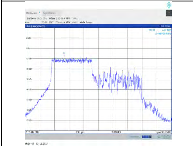
11be20MIMO-Ant7-2412-106Tone-RU53-PASS
