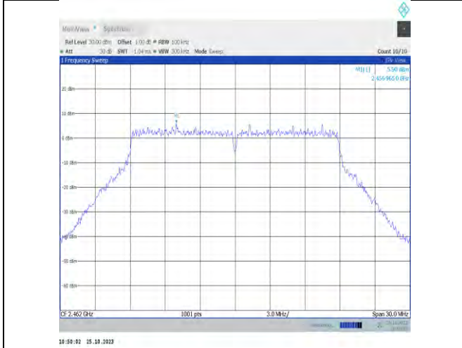
11n20MIMO-Ant16-2462-0~Reference-PASS
