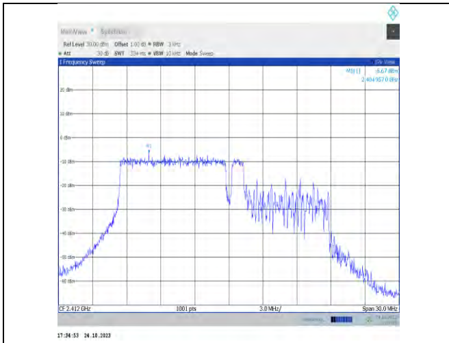
11be20MIMO-Ant16-2412-106+26Tone-RU53+4-PASS
