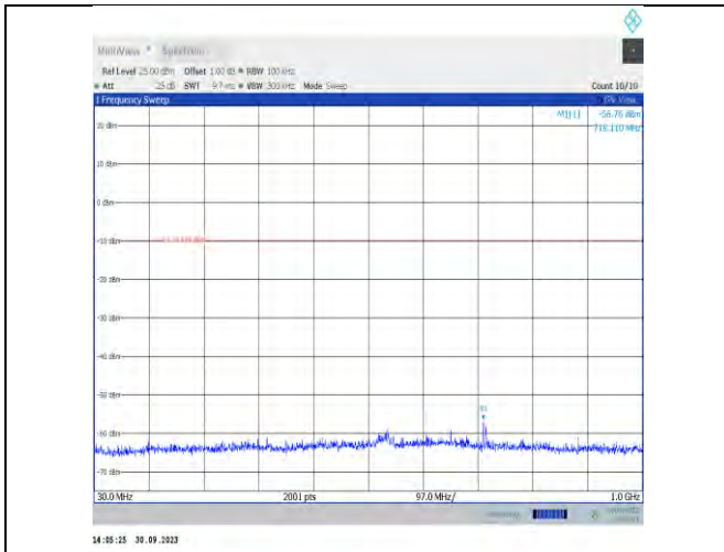
11b-CDD-Ant7-2437-30~1000-PASS
