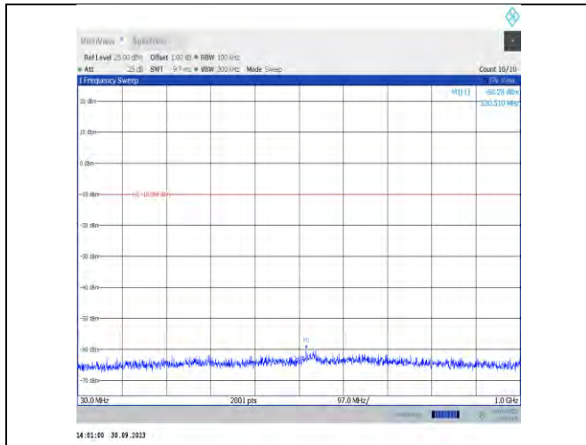
11b-CDD-Ant7-2412-30~1000-PASS
