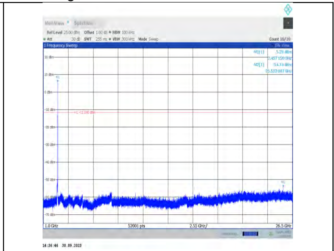
11g-CDD-Ant7-2462-1000~26500-PASS
