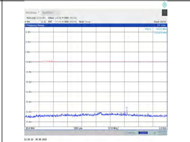
11b-CDD-Ant16-2437-30~1000-PASS
