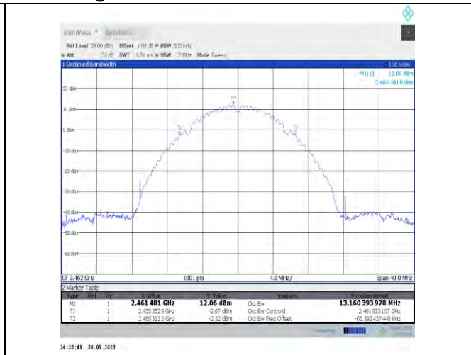
11b-CDD-Ant7-2462
