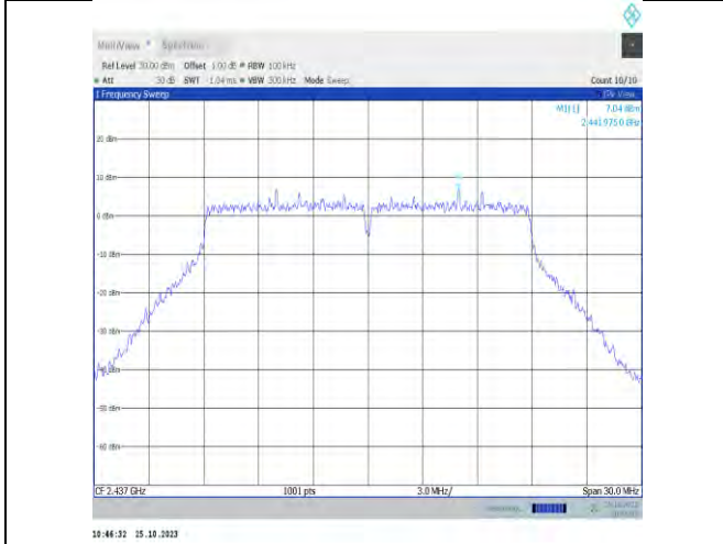
11n20MIMO-Ant16-2437-0~Reference-PASS
