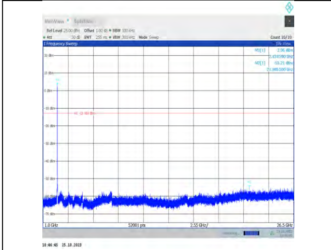
11n20MIMO-Ant16-2437-1000~26500-PASS
