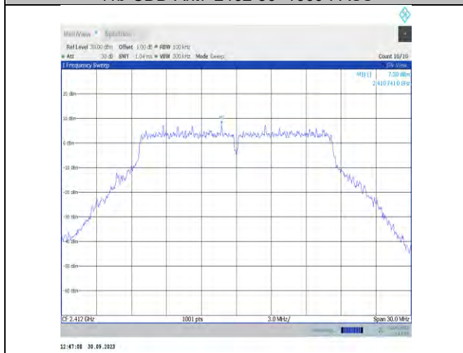
11g-CDD-Ant16-2412-0~Reference-PASS
