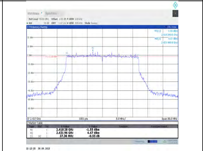
11be40MIMO-Ant7-2437-PASS
