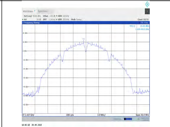
11b-CDD-Ant7-2437-0~Reference-PASS
