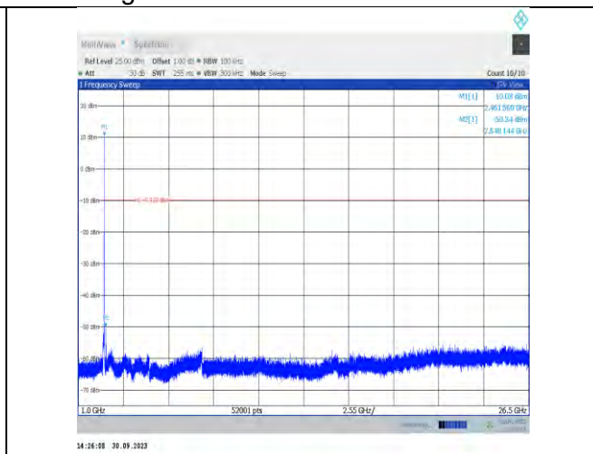
11b-CDD-Ant7-2462-1000~26500-PASS
