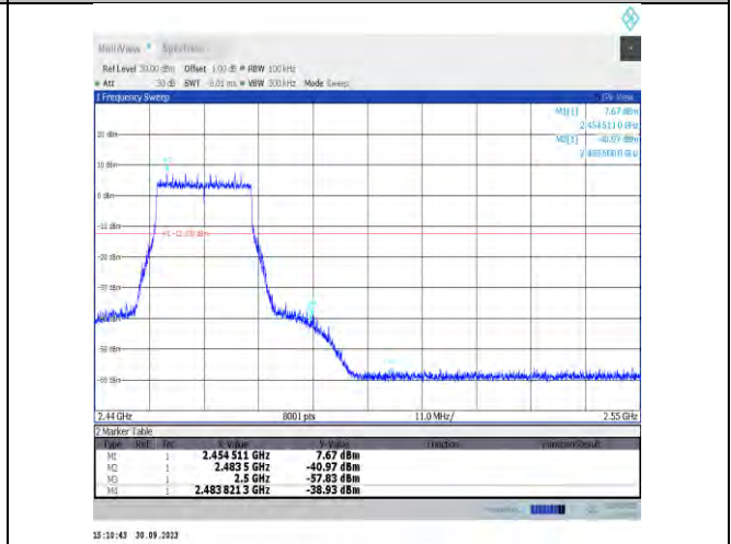
11be20MIMO-Ant7-2462-PASS
