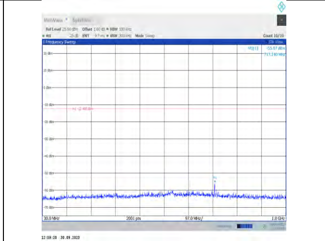
11g-CDD-Ant16-2462-30~1000-PASS
