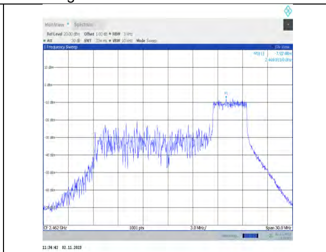
11be20MIMO-Ant7-2462-52Tone-RU40-PASS
