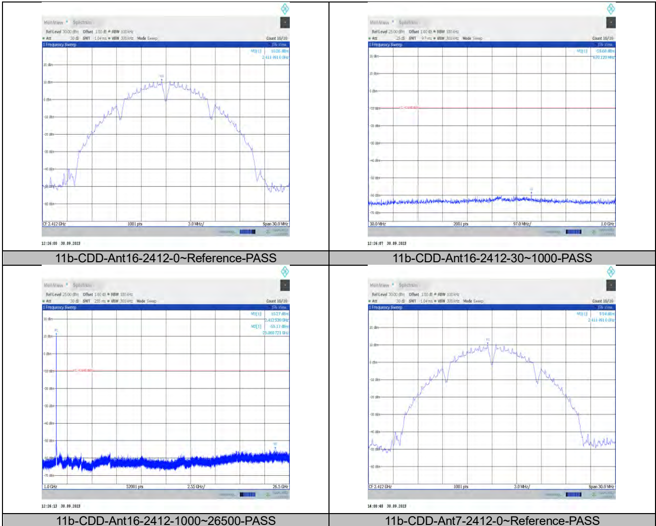
11b-CDD-Ant16-2412-1000~26500-PASS
