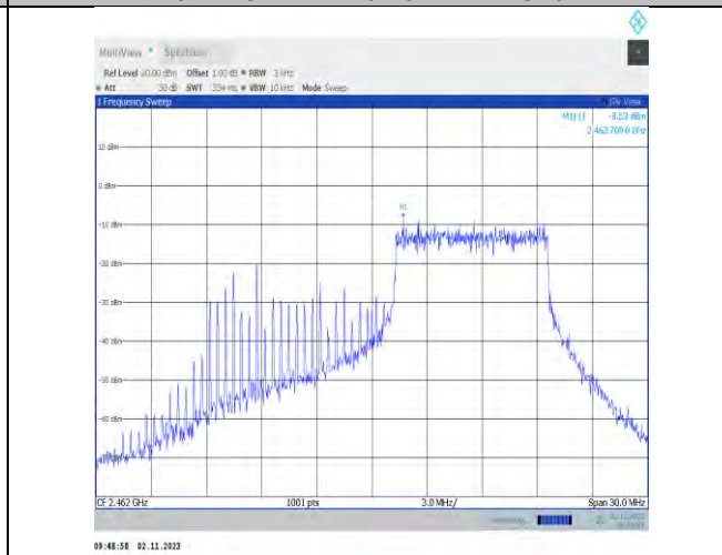
11be20MIMO-Ant7-2462-106Tone-RU54-PASS
