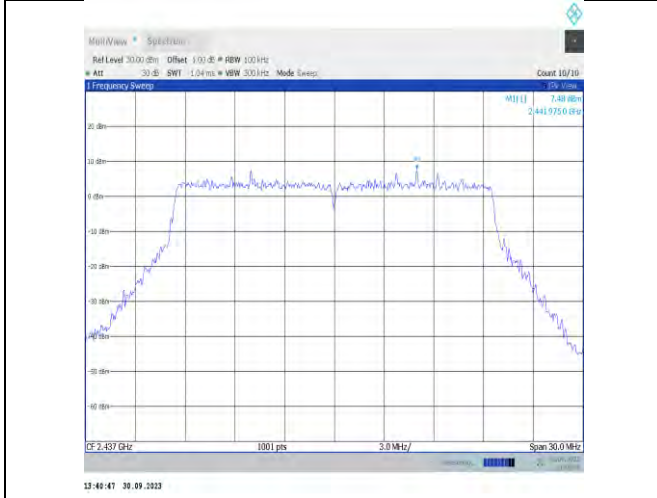
11be20MIMO-Ant16-2437-0~Reference-PASS
