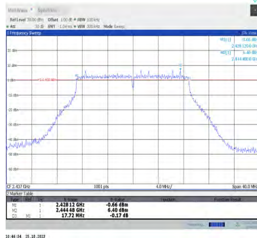
11n20MIMO-Ant7-2437-PASS
