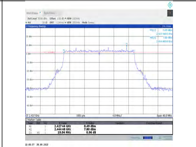
11be20MIMO-Ant7-2437-PASS
