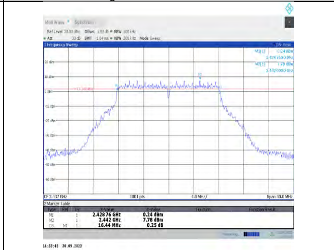
11g-CDD-Ant7-2437-PASS
