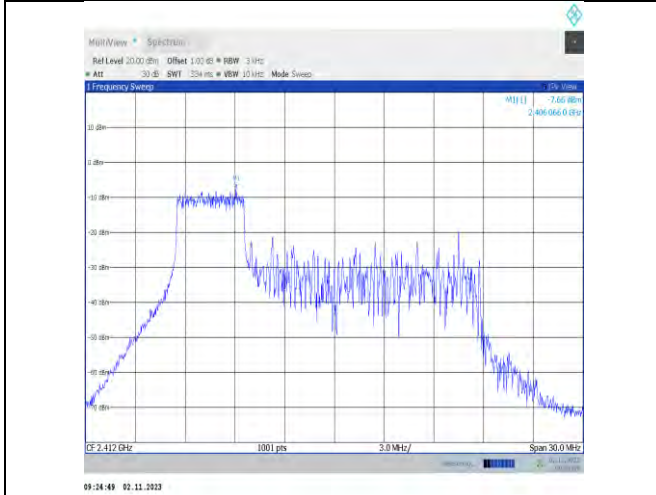
11be20MIMO-Ant7-2412-52Tone-RU37-PASS
