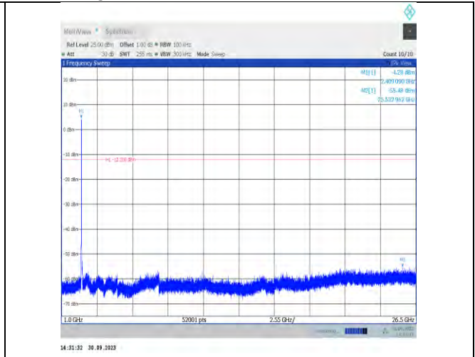
11g-CDD-Ant7-2412-1000~26500-PASS
