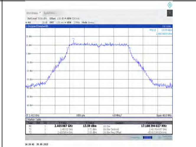
11g-CDD-Ant7-2412
