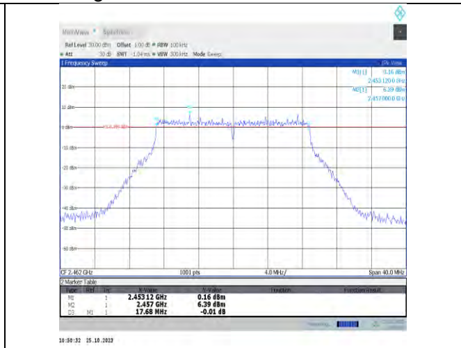
11n20MIMO-Ant7-2462-PASS
