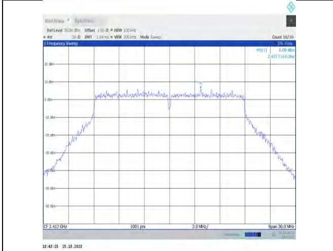
11n20MIMO-Ant16-2412-0~Reference-PASS
