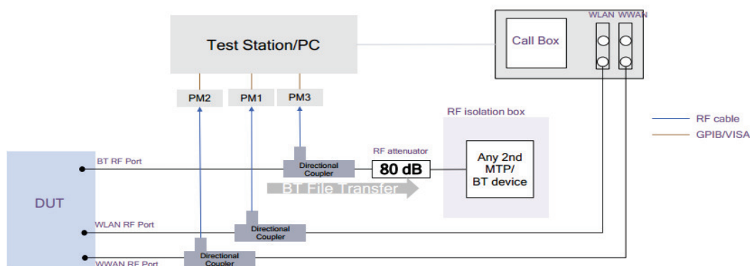
Figure5-3 System Level Continuity test setup
