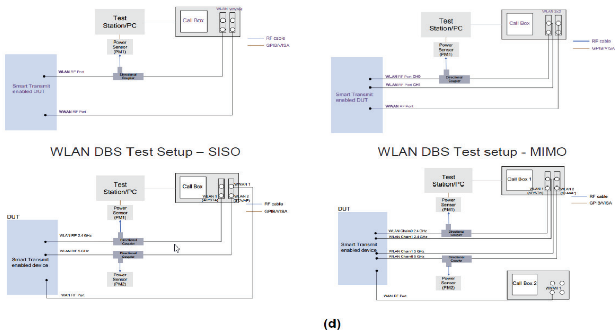
Figure5-2 Conducted power measurement setup for WLAN/BT Band
