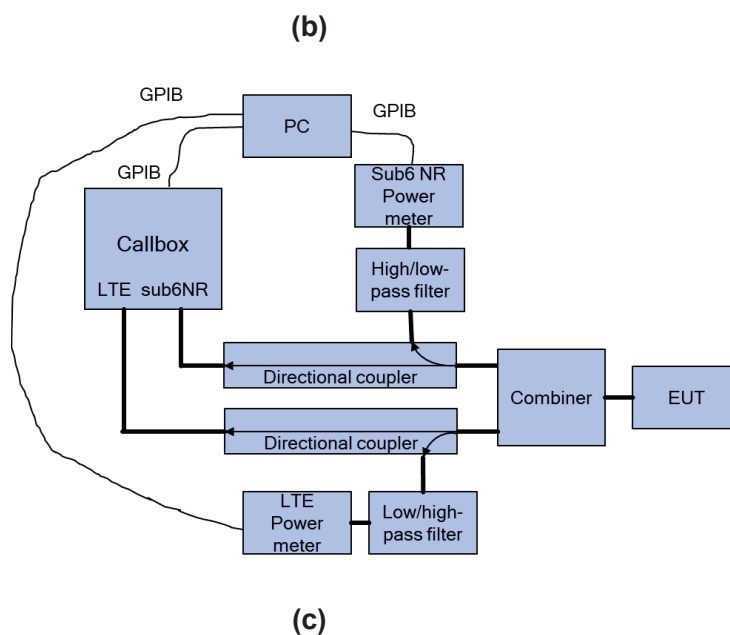
Figure 5-1 Conducted power measurement setup
