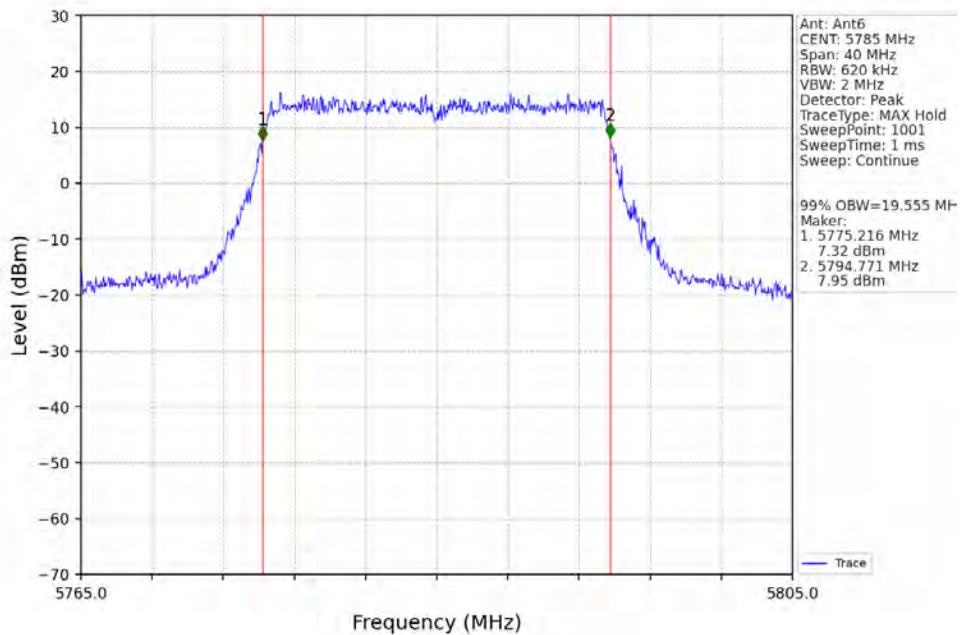
802.11ax(HEW20)_MCH_5785MHz_RU242_Left_Ant6_NTNV
