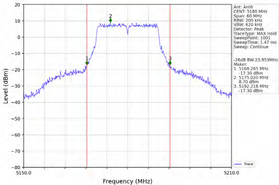
802.11ac(VHT20)_LCH_5180MHz_Ant6_NTNV
