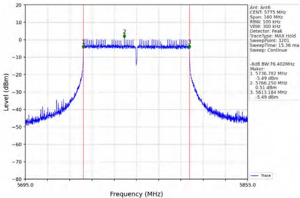
802.11ac(VHT80) MCH 5775MHz Ant6 NTN
