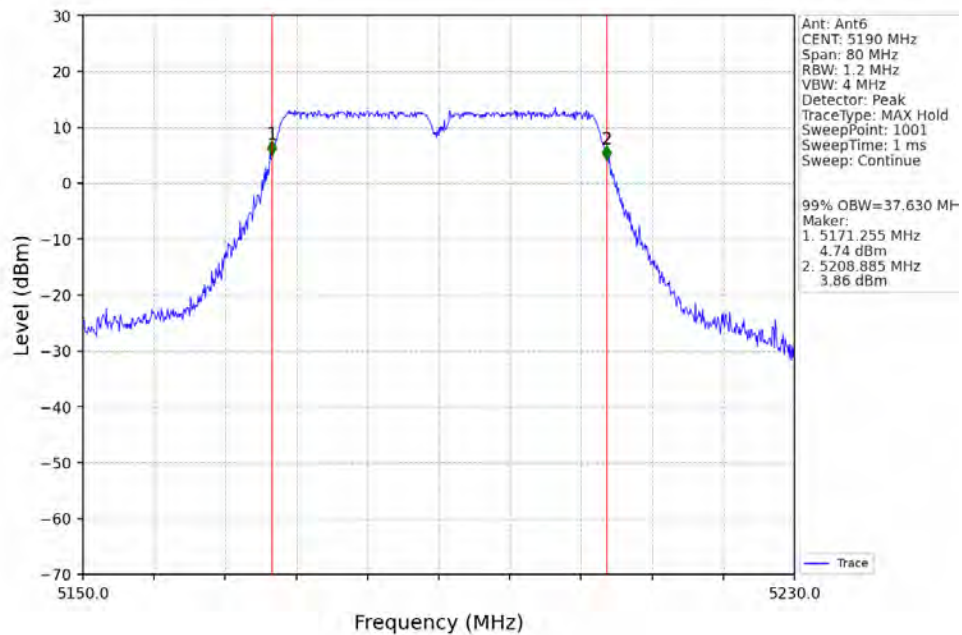
802.11ac(VHT40)_LCH_5190MHz_Ant6_NTNV
