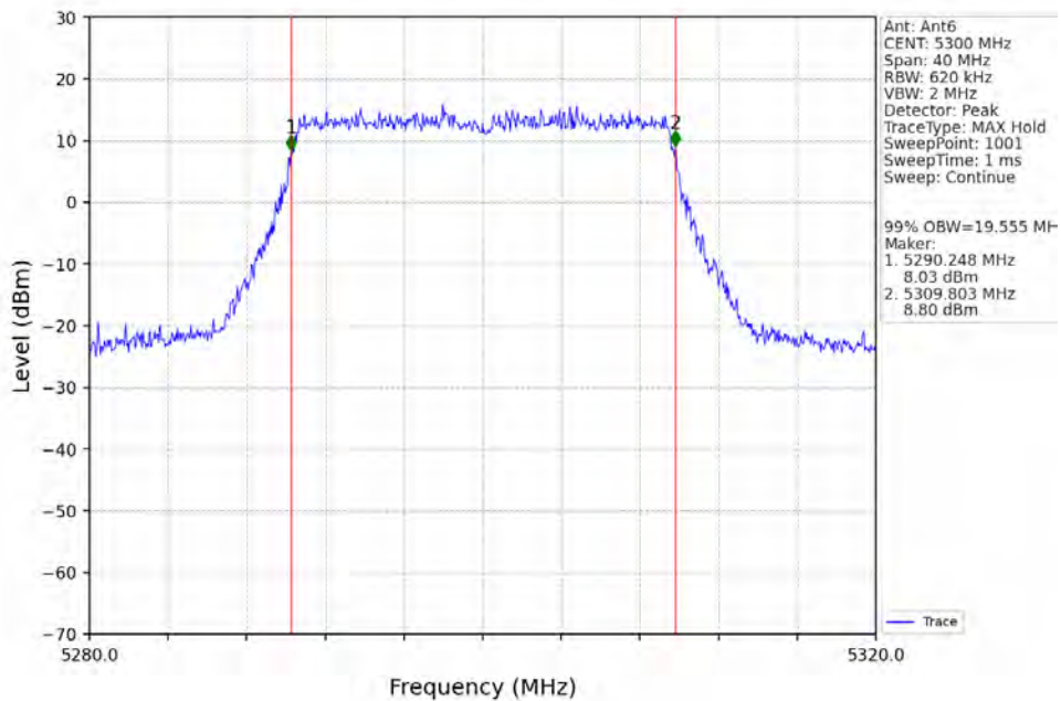
802.11ax(HEW20)_MCH_5300MHz_RU242_Left_Ant6_NTNV
