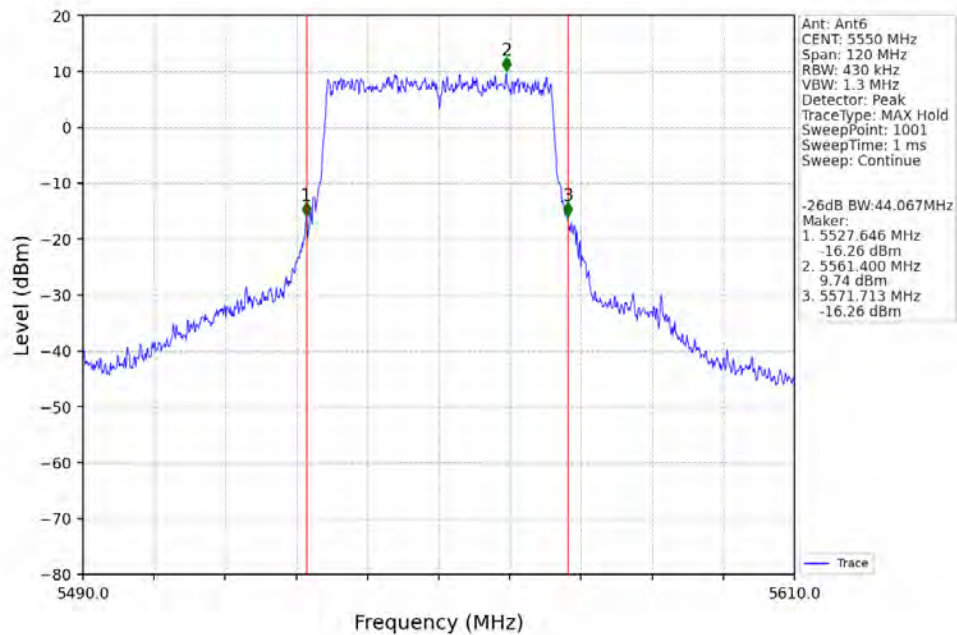
802.11ax(HEW40)_MCH_5550MHz_RU484_Left_Ant6_NTNV
