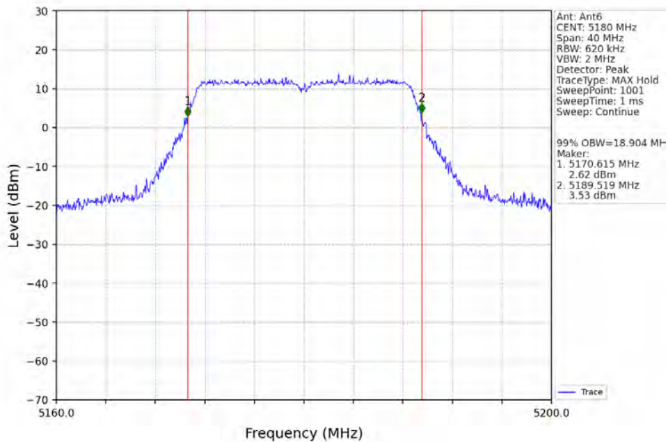
802.11ac(VHT20)_LCH_5180MHz_Ant6_NTNV
