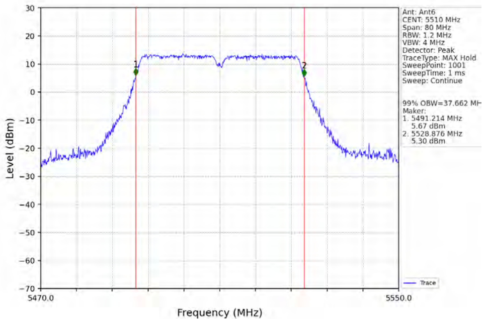
802.11ac(VHT40)_LCH_5510MHz_Ant6_NTNV
