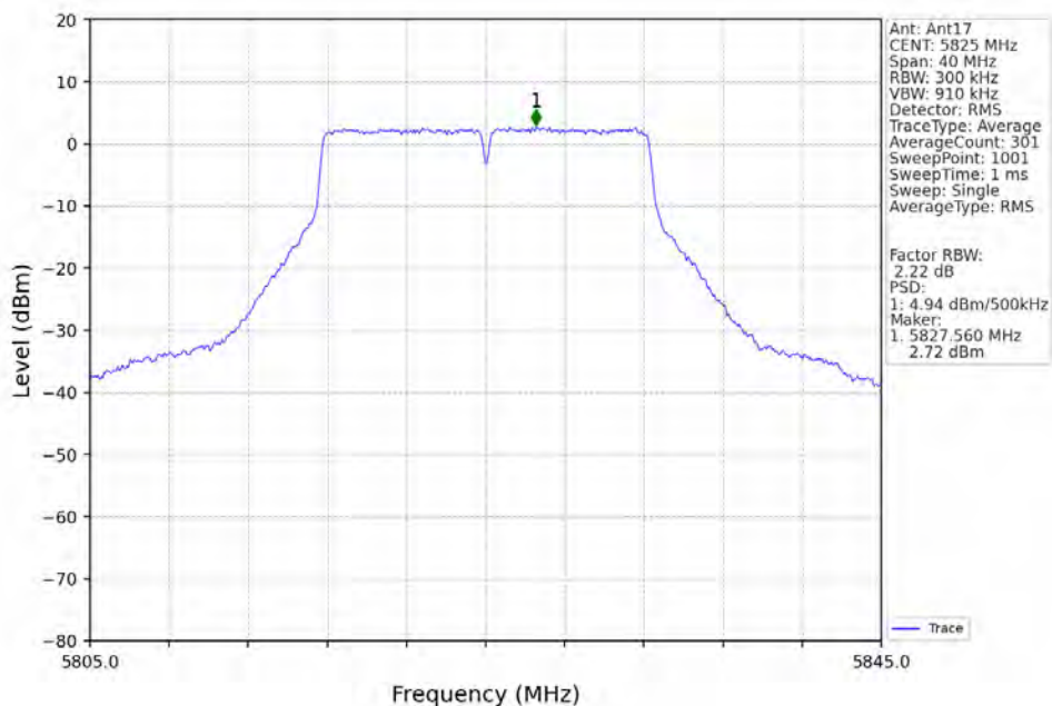
802.11a_HCH_5825MHz_Ant17_NTNV
