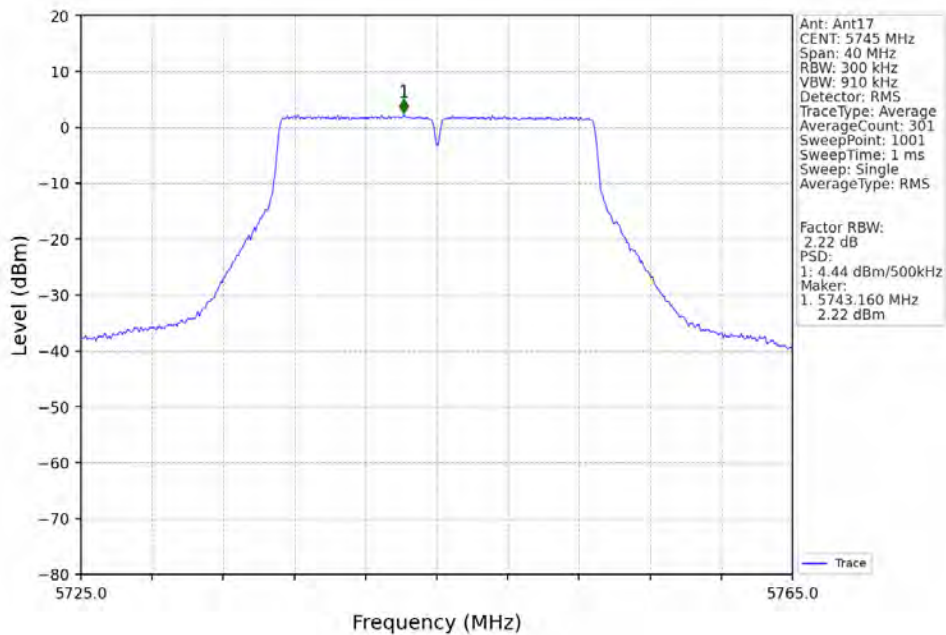
802.11ac(VHT20)_LCH_5745MHz_Ant17_NTNV
