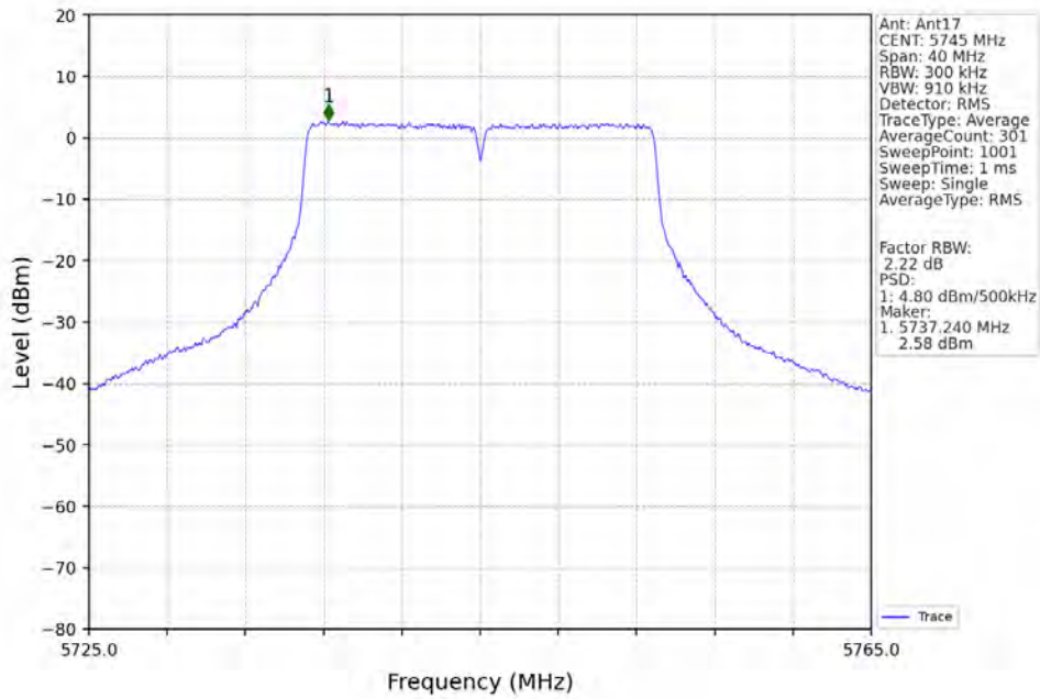
802.11n(HT20)_LCH_5745MHz_MIMO_NTNV
