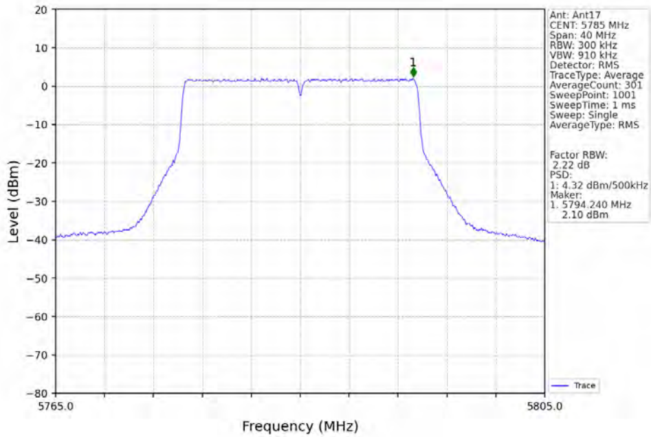
802.11ax(HEW20)_MCH_5785MHz_RU242_Left_MIMO_NTNV
