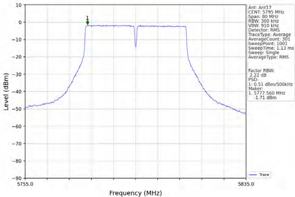
802.11ac(VHT40)_HCH_5795MHz_Ant17_NTNV
