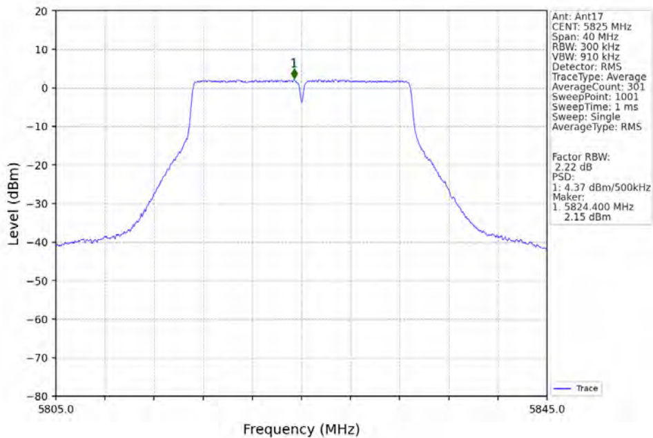
802.11ac(VHT20)_HCH_5825MHz_Ant17_NTNV
