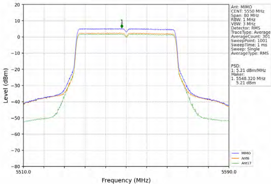
802.11ax(HEW40)_MCH_5550MHz_RU484_Left_MIMO_NTNV
