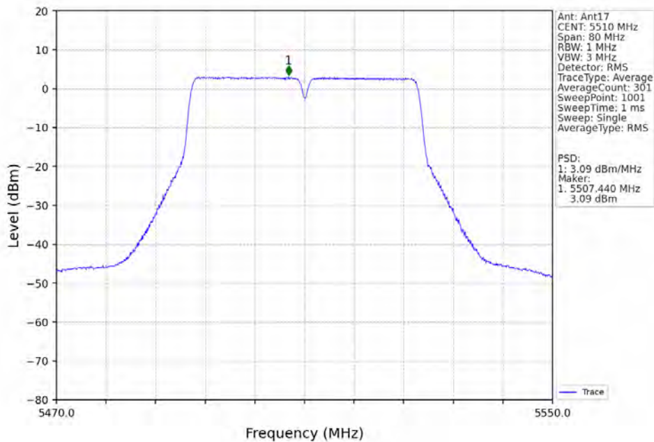
802.11ac(VHT40)_LCH_5510MHz_Ant17_NTNV
