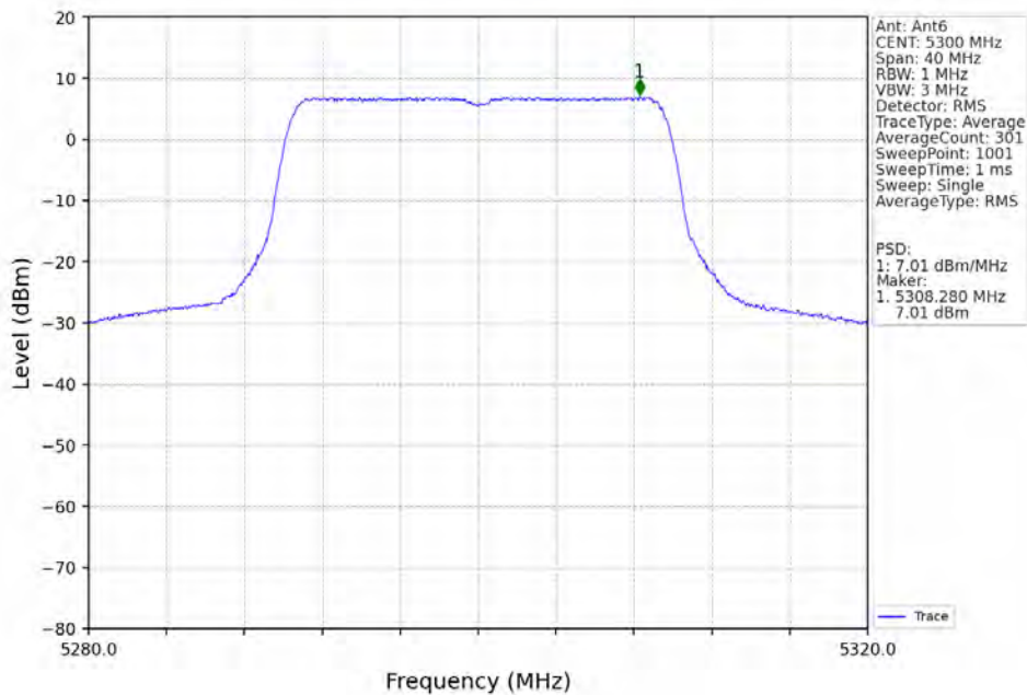
802.11ax(HEW20)_MCH_5300MHz_RU242_Left_Ant6_NTNV
