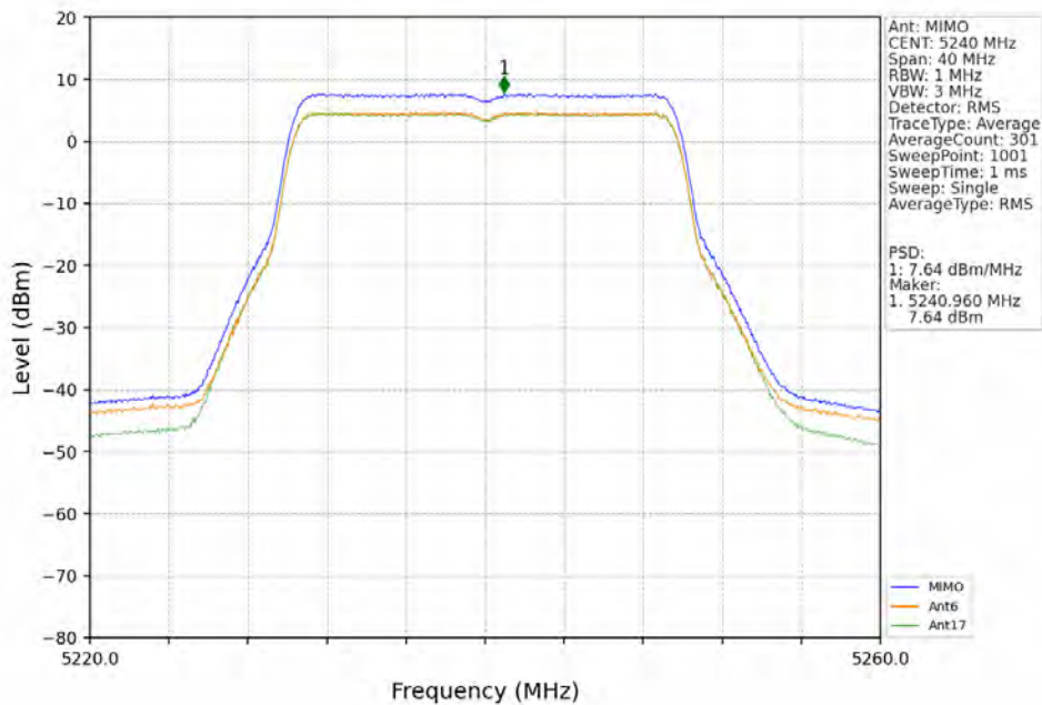
802.11ax(HEW20)_HCH_5240MHz_RU242_Left MIMO NTN
