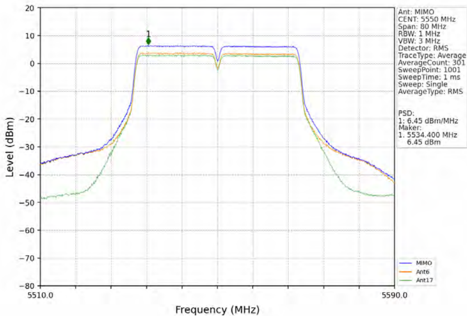
802.11ac(VHT40)_MCH_5550MHz MIMO NTN
