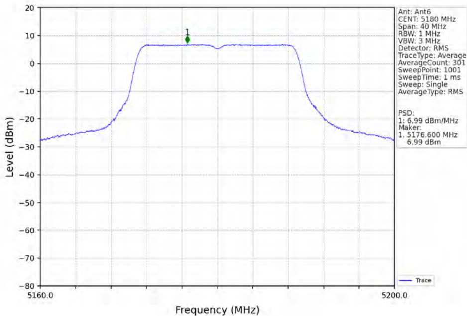
802.11ac(VHT20)_LCH_5180MHz_Ant6_NTNV
