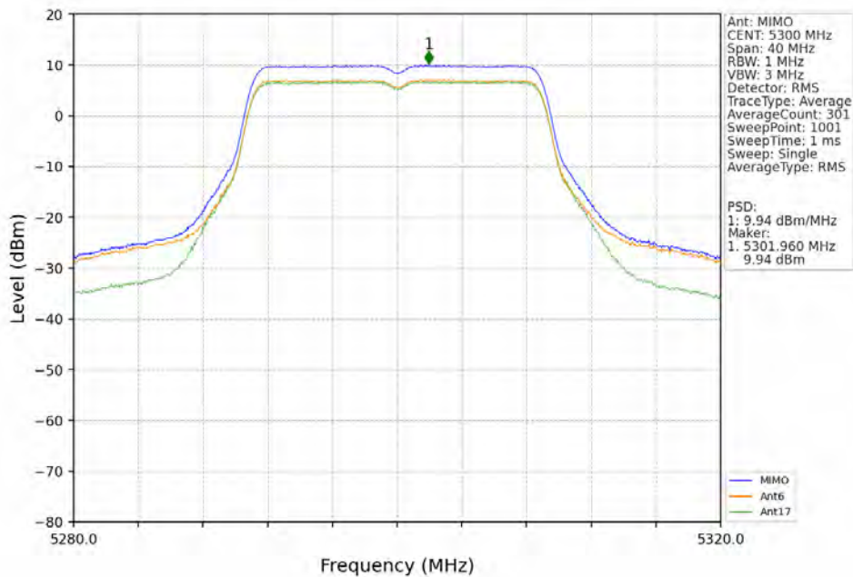
802.11ac(VHT20)_MCH_5300MHz MIMO NTN
