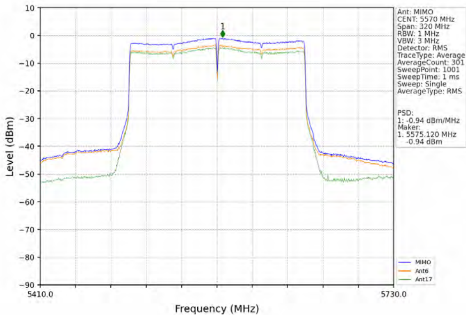
802.11ax(HEW160) MCH 5570MHz 2xRU996 Left MIMO NTN
