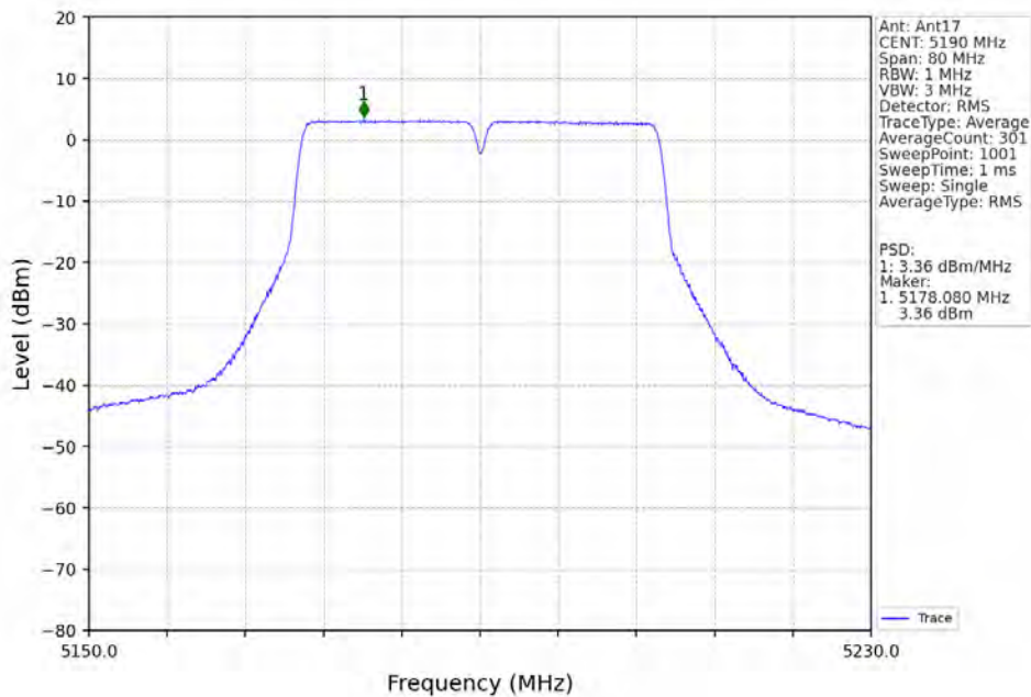
802.11ac(VHT40)_LCH_5190MHz_Ant17_NTNV
