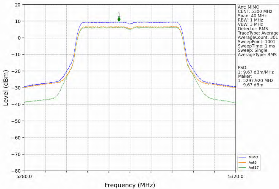
802.11ax(HEW20)_MCH_5300MHz_RU242_Left_MIMO_NTNV
