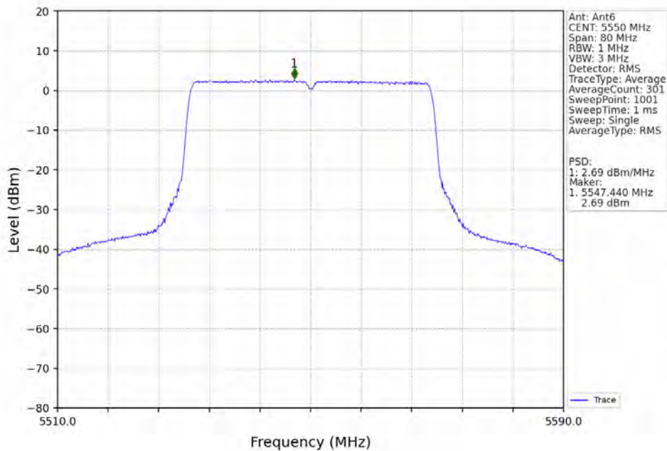
802.11ax(HEW40)_MCH_5550MHz_RU484_Left_Ant6_NTNV
