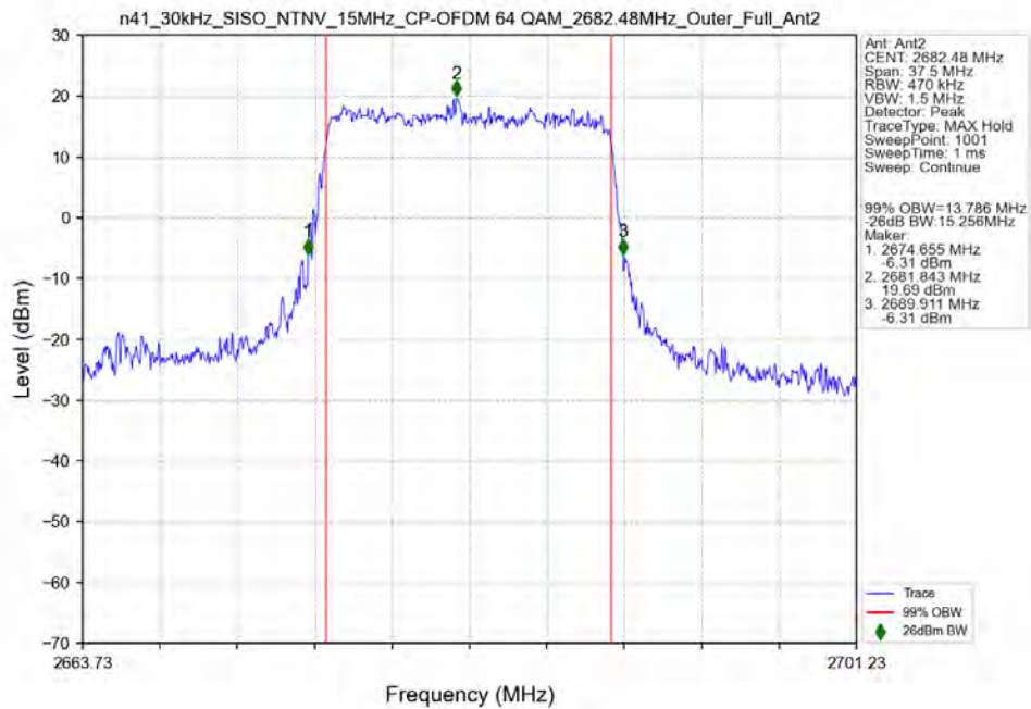
n41_30kHz_SISO_NTNV_15MHz_CP-OFDM_64_QAM_2682.48MHz_Outer_Full_Ant2
