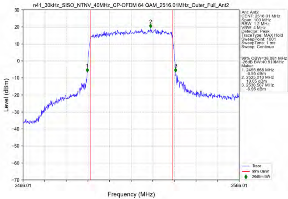
n41_30kHz_SISO_NTNV_40MHz_CP-OFDM_64_QAM_2516.01MHz_Outer_Full_Ant2
