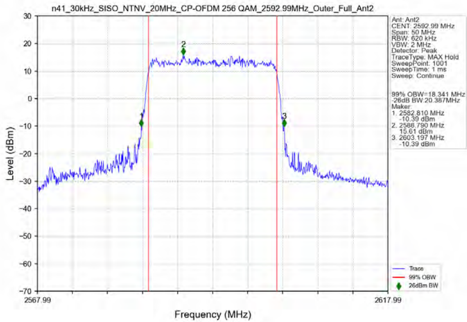
n41_30kHz_SISO_NTNV_20MHz_CP-OFDM_256_QAM_2592.99MHz_Outer_Full_Ant2
