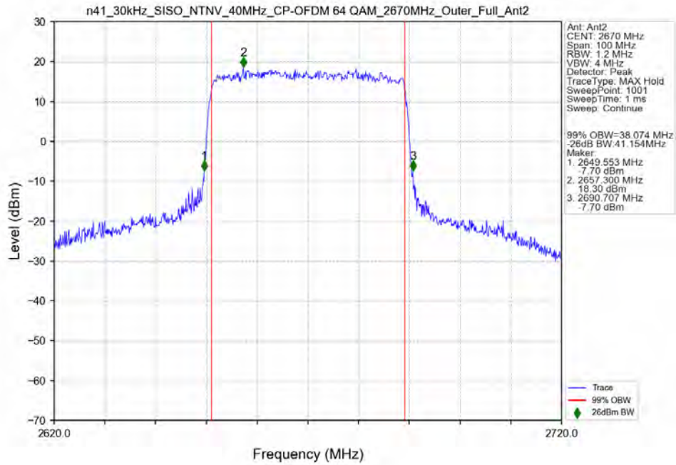
n41_30kHz_SISO_NTNV_40MHz_CP-OFDM_64_QAM_2670MHz_Outer_Full_Ant2
