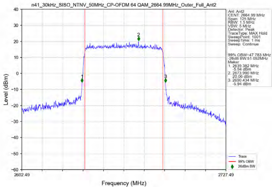
n41_30kHz_SISO_NTNV_50MHz_CP-OFDM_64_QAM_2664.99MHz_Outer_Full_Ant2
