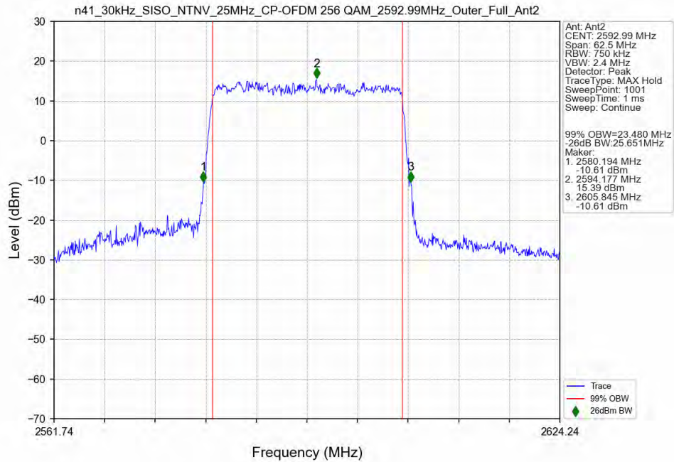
n41_30kHz_SISO_NTNV_25MHz_CP-OFDM_256_QAM_2592.99MHz_Outer_Full_Ant2
