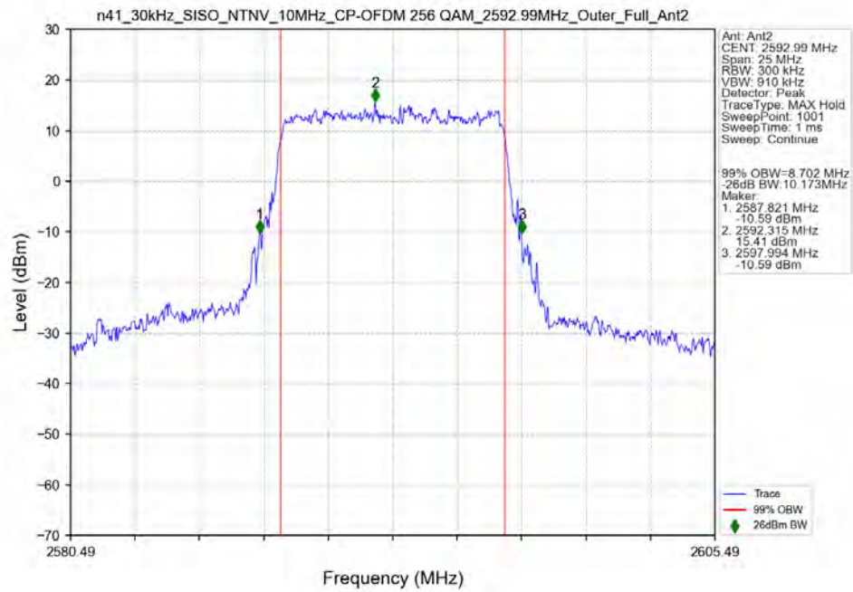
n41_30kHz_SISO_NTNV_10MHz_CP-OFDM_256_QAM_2592.99MHz_Outer_Full_Ant2
