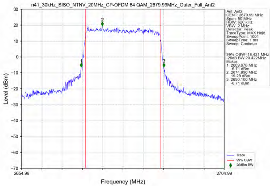
n41_30kHz_SISO_NTNV_20MHz_CP-OFDM_64_QAM_2679.99MHz_Outer_Full_Ant2
