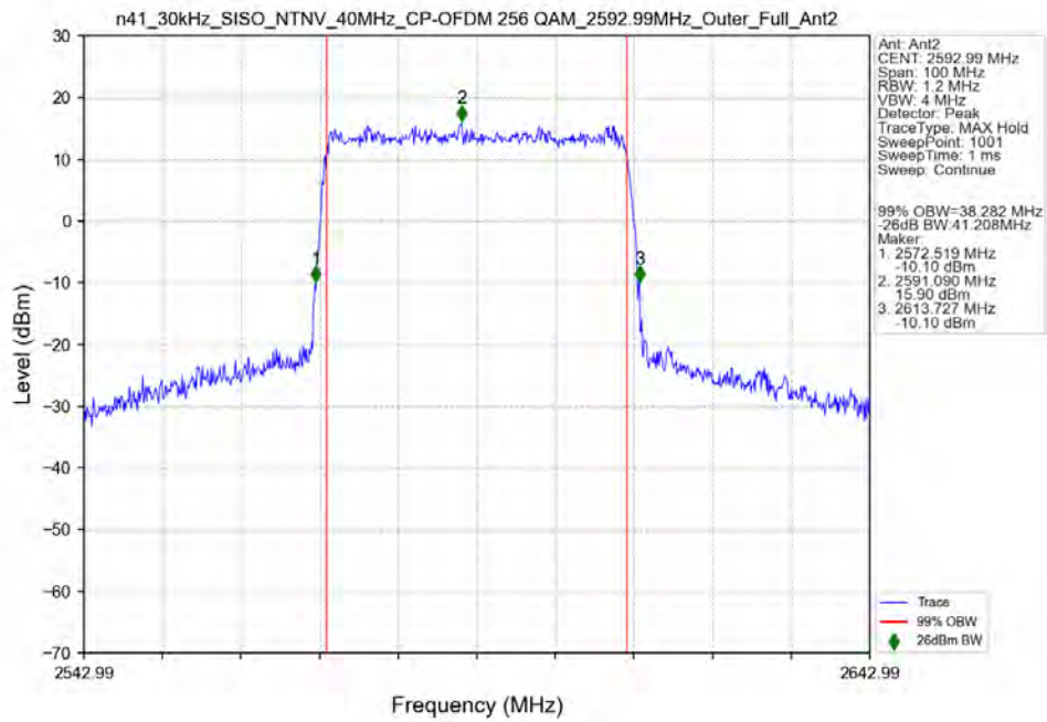
n41_30kHz_SISO_NTNV_40MHz_CP-OFDM_256_QAM_2592.99MHz_Outer_Full_Ant2
