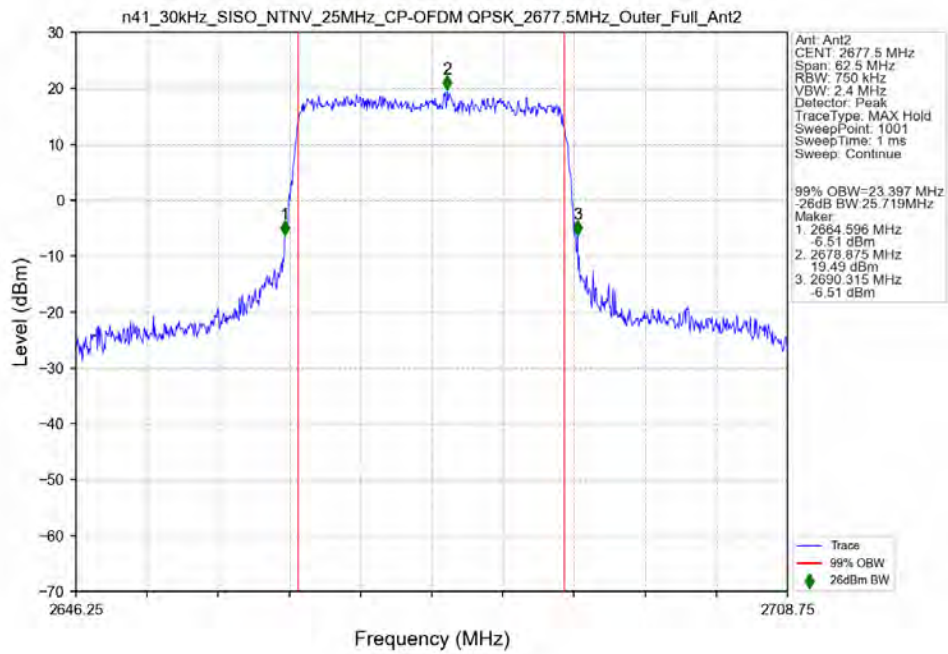
n41_30kHz_SISO_NTNV_25MHz_CP-OFDM_QPSK_2677.5MHz_Outer_Full_Ant2
