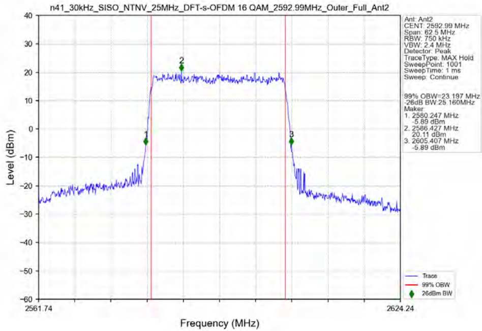
n41_30kHz_SISO_NTNV_25MHz_DFT-s-OFDM_16_QAM_2592.99MHz_Outer_Full_Ant2
