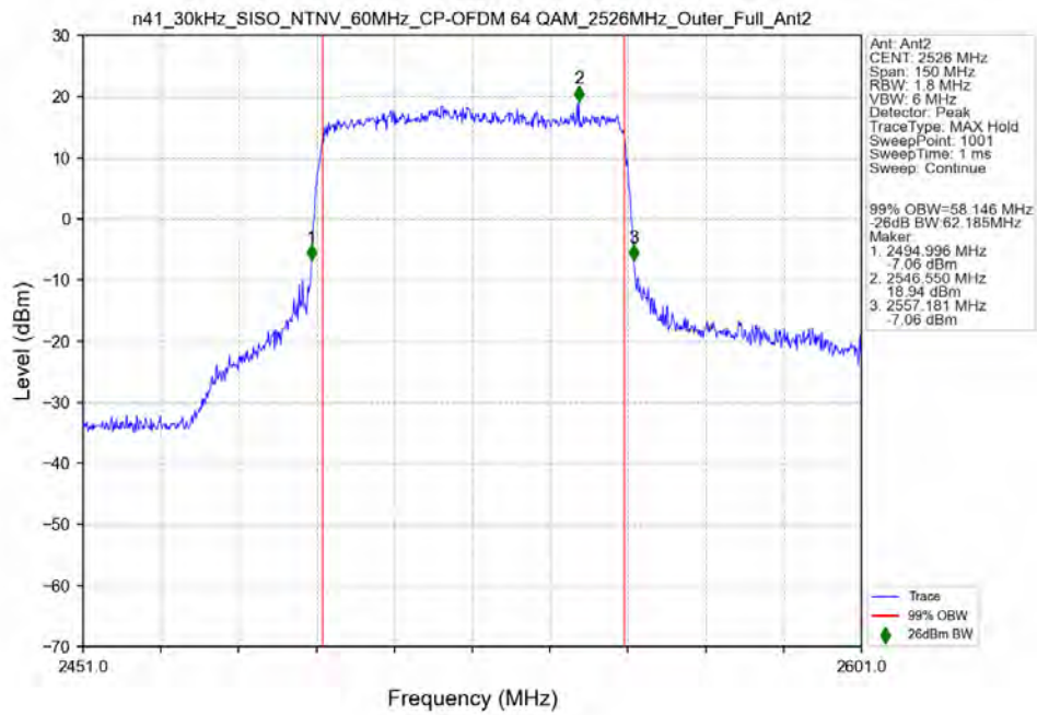
n41_30kHz_SISO_NTNV_60MHz_CP-OFDM_64_QAM_2526MHz_Outer_Full_Ant2
