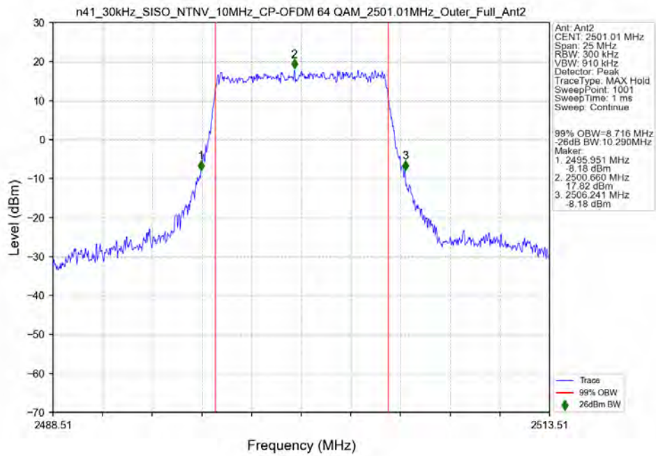
n41_30kHz_SISO_NTNV_10MHz_CP-OFDM_64_QAM_2501.01MHz_Outer_Full_Ant2
