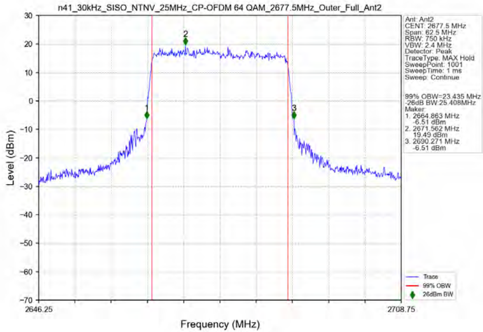
n41_30kHz_SISO_NTNV_25MHz_CP-OFDM_64_QAM_2677.5MHz_Outer_Full_Ant2
