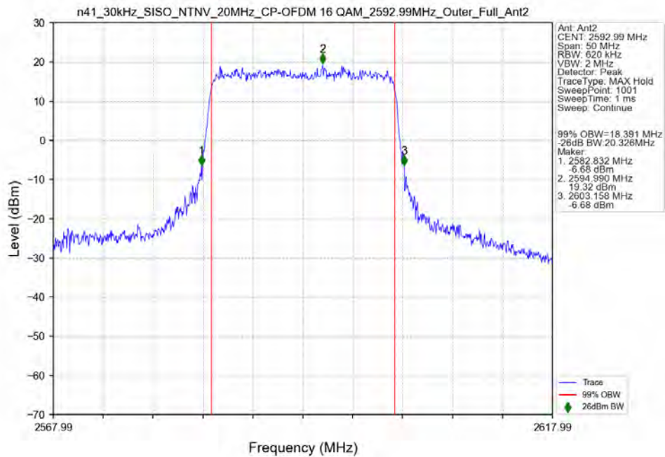
n41_30kHz_SISO_NTNV_20MHz_CP-OFDM_16_QAM_2592.99MHz_Outer_Full_Ant2
