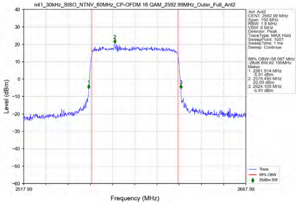
n41_30kHz_SISO_NTNV_60MHz_CP-OFDM_16_QAM_2592.99MHz_Outer_Full_Ant2
