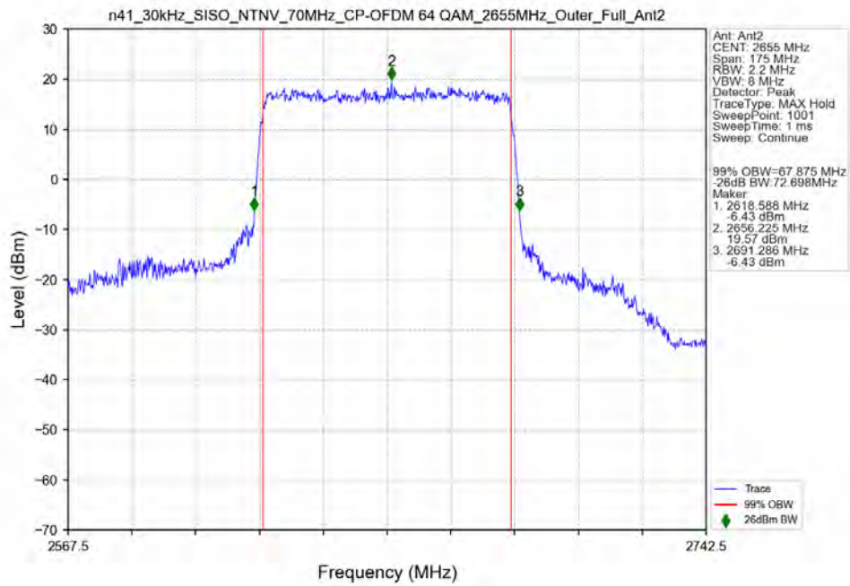
n41_30kHz_SISO_NTNV_70MHz_CP-OFDM_64_QAM_2655MHz_Outer_Full_Ant2
