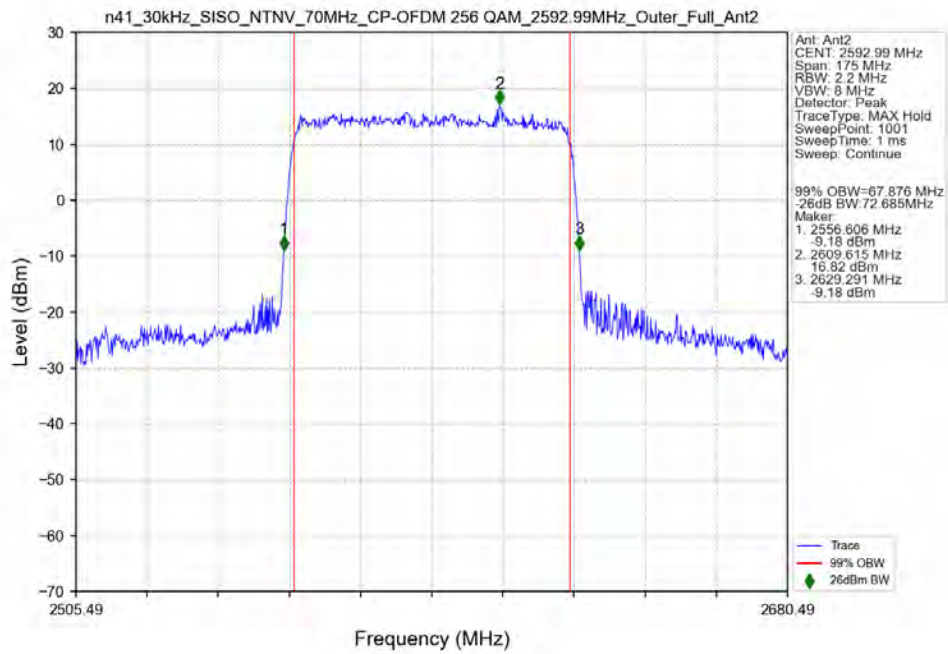
n41_30kHz_SISO_NTNV_70MHz_CP-OFDM_256_QAM_2592.99MHz_Outer_Full_Ant2
