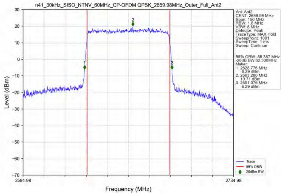
n41_30kHz_SISO_NTNV_60MHz_CP-OFDM_QPSK_2659.98MHz_Outer_Full_Ant2
