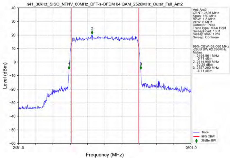
n41_30kHz_SISO_NTNV_60MHz_DFT-s-OFDM_64_QAM_2526MHz_Outer_Full_Ant2
