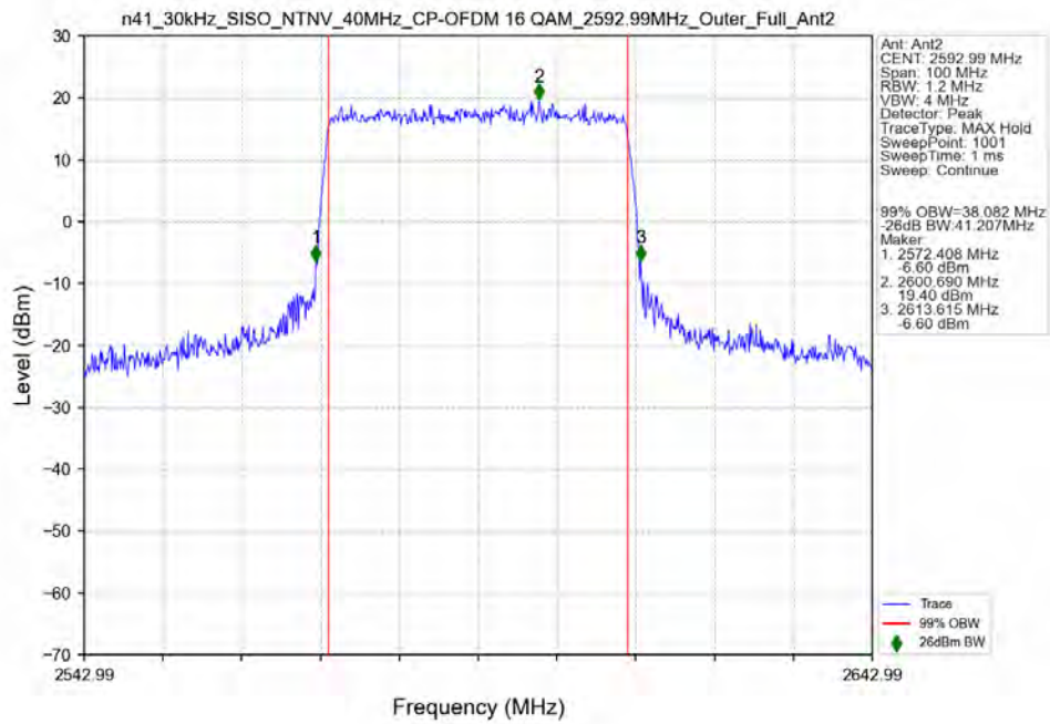
n41_30kHz_SISO_NTNV_40MHz_CP-OFDM_16_QAM_2592.99MHz_Outer_Full_Ant2
