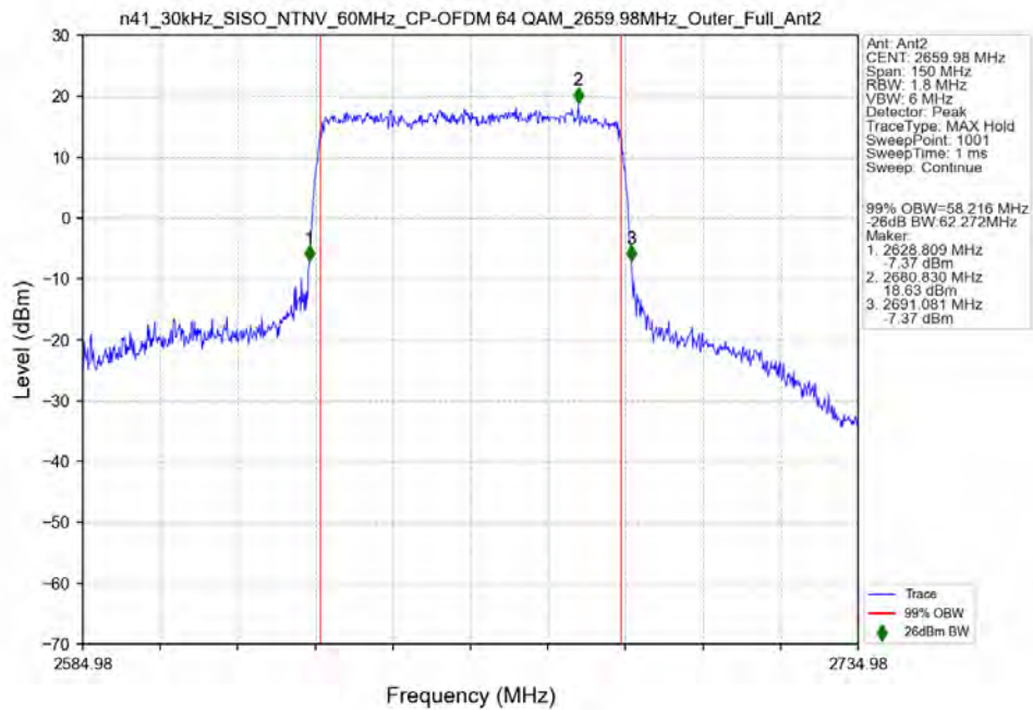
n41_30kHz_SISO_NTNV_60MHz_CP-OFDM_64_QAM_2659.98MHz_Outer_Full_Ant2
