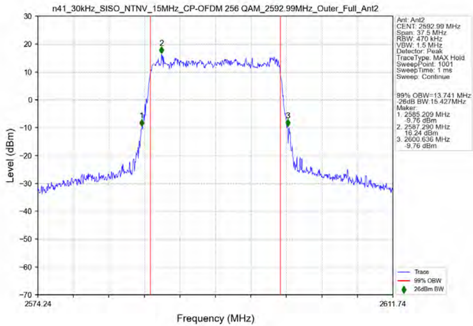
n41_30kHz_SISO_NTNV_15MHz_CP-OFDM_256_QAM_2592.99MHz_Outer_Full_Ant2
