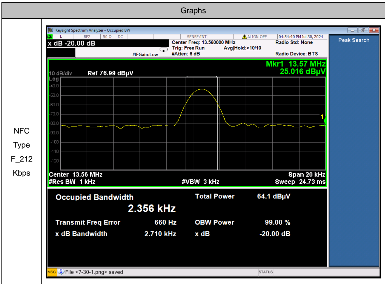
20dB Bandwidth & 99% Bandwidth Plot
