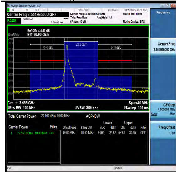
NTNV-N48-PC3-30-100-H-DFT-QPSK-Edge_1RB-Right-Ant1-PASS
