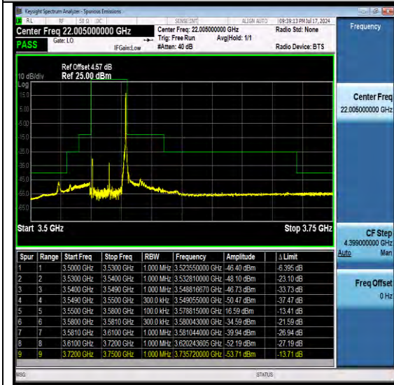
NTVN-N48-PC3-30-30-L-DFT-QPSK-Edge_1RB_ Right-Ant1-PASS
