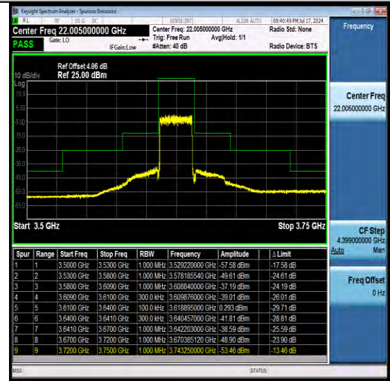
NTVN-N48-PC3-30-30-M-DFT-QPSK-Outer_Full- Ant1-PASS
