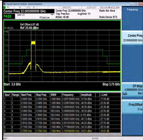
NTNV-N48-PC3-30-10-L-DFT-QPSK-Outer_Full-Ant1-PASS
