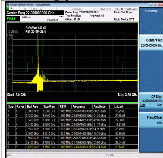
NTNV-N48-PC3-30-100-H-DFT-QPSK-Edge_1RB Right-Ant1-PASS
