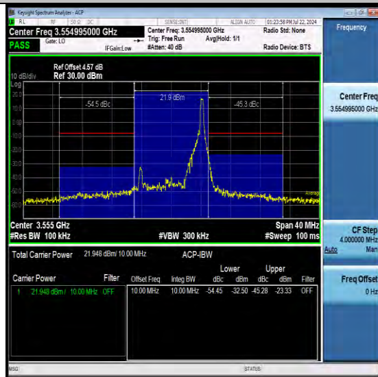
NTNV-N48-PC3-30-10-L-DFT-QPSK-Outer_Full-Ant1-PASS
