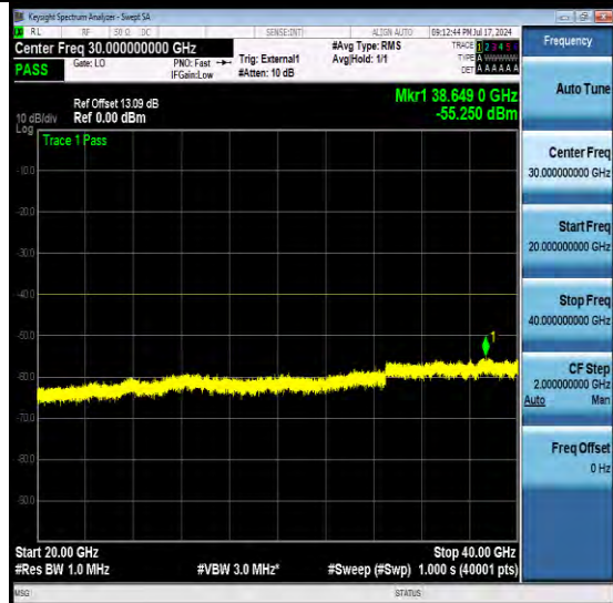
NTNV-N48-PC3-30-100-L-DFT-QPSK-Edge_1RB Left-Ant1-PASS
